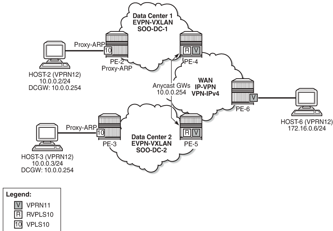
Figure 39: DCI inter-subnet forwarding with Anycast GWs and ARP-ND host routes
