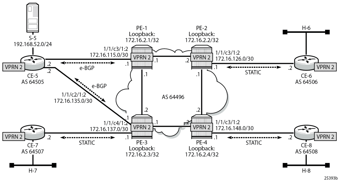
Figure 371: VPRN 2 Topology used for MVPN Source Redundancy
