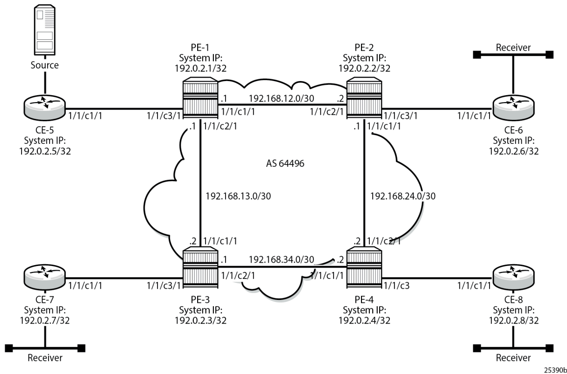
Figure 368: Network Topology
