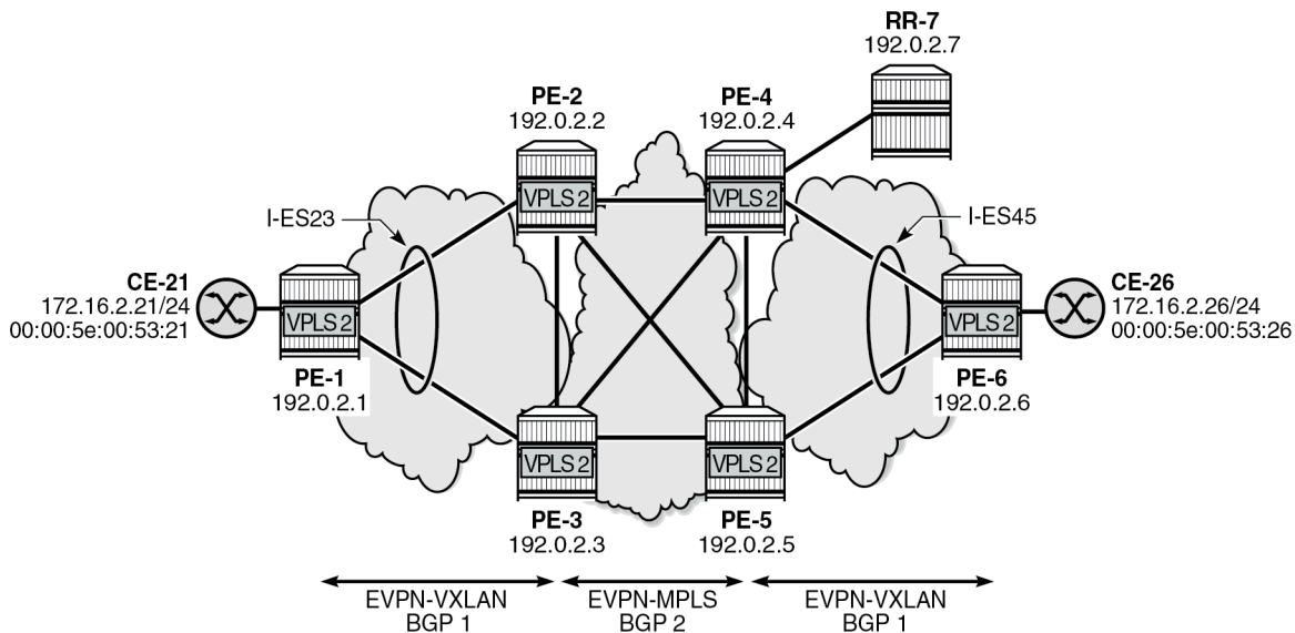
Figure 319: Example topology with dual-instance VPLS
