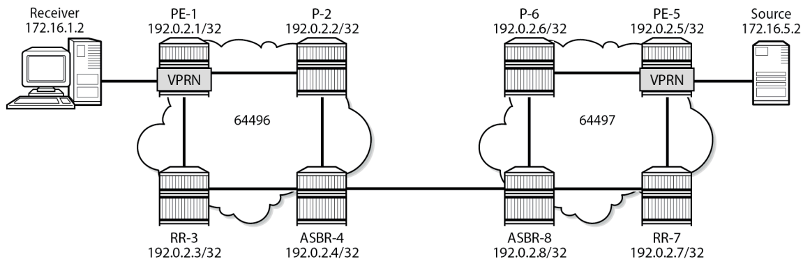
Figure 384: NG-MVPN Inter-AS Model C
