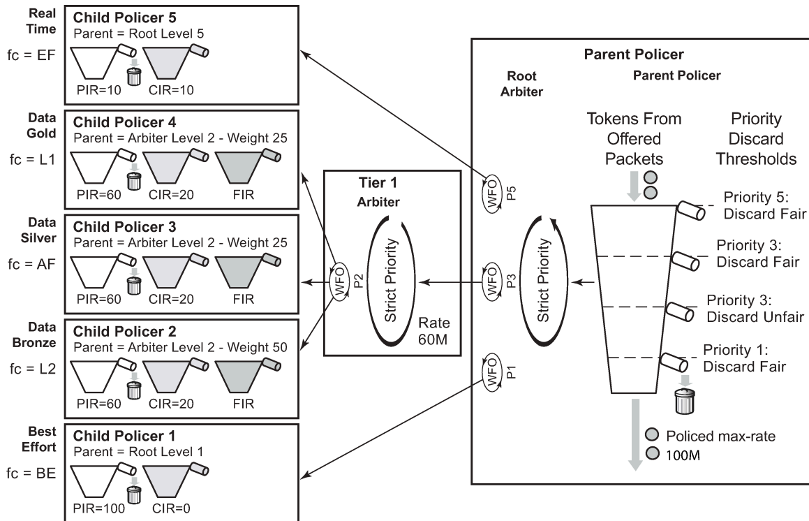
Figure 443: Configuration Example
