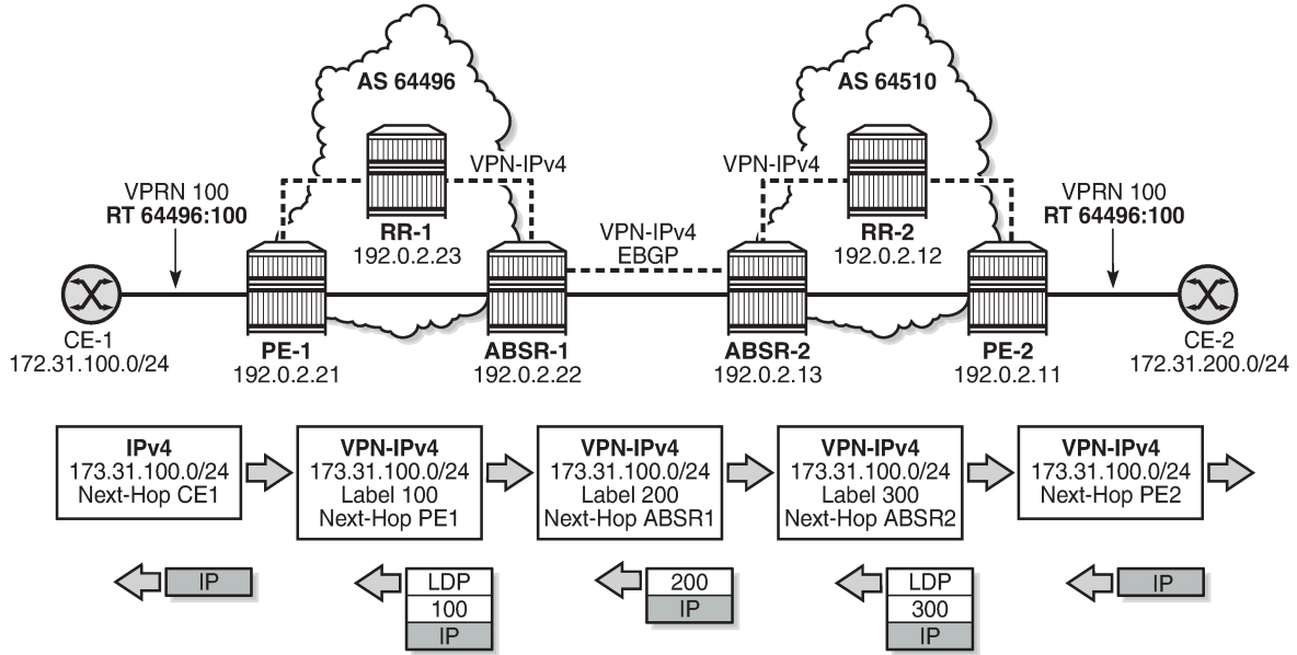
Figure 350: Inter-AS VPRN Model B control and data plane example
