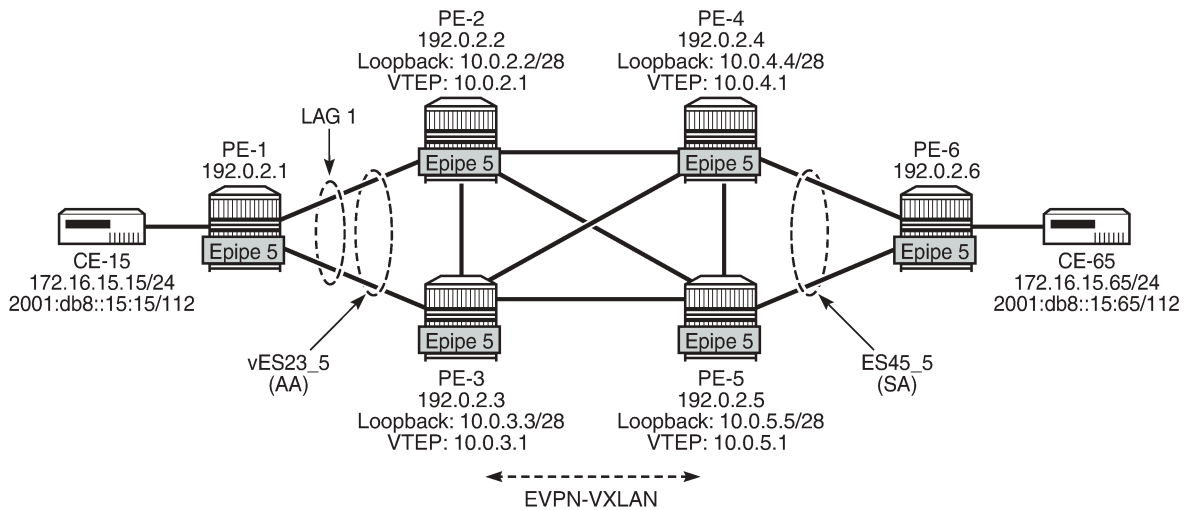
Figure 181: EVPN-VXLAN Epipe 5 with AA MH and SA MH using non-system IPv4 addresses
