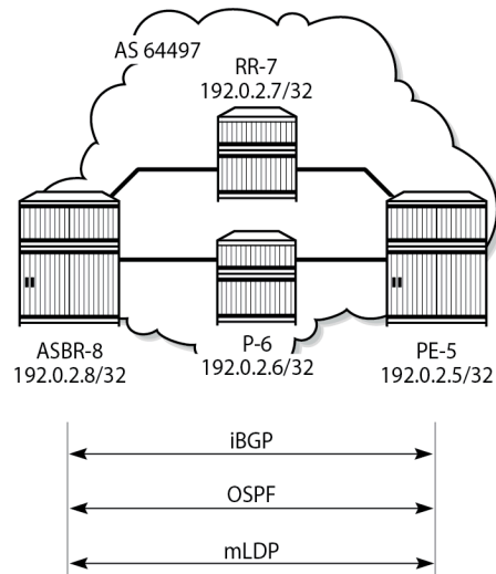
Figure 387: AS 64497 Protocols
