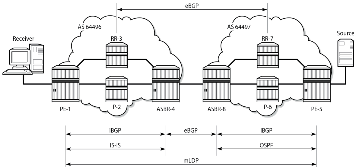
Figure 385: Inter-AS MVPN Protocol Requirements
