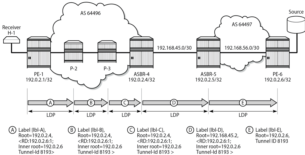
Figure 383: P2MP LDP Label Mapping
