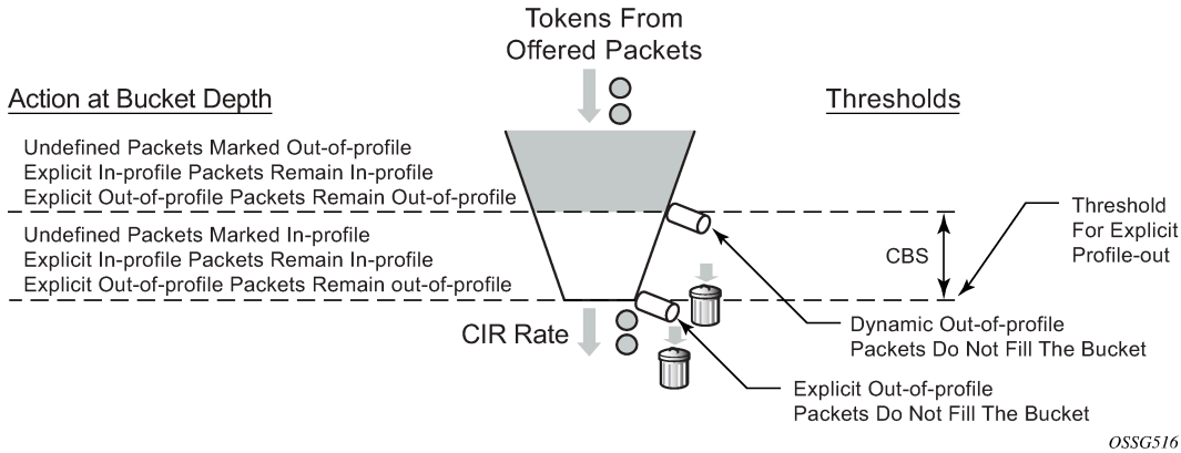
Figure 439: Committed Information Rate (CIR) Bucket
