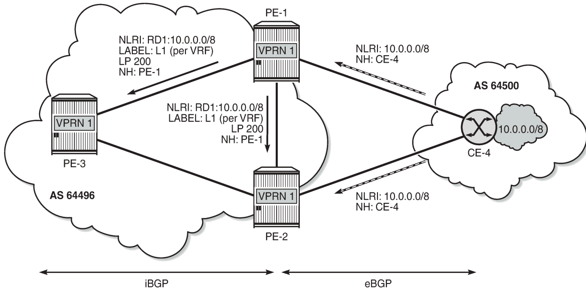
Figure 341: Default BGP behavior: BGP advertises best route only
