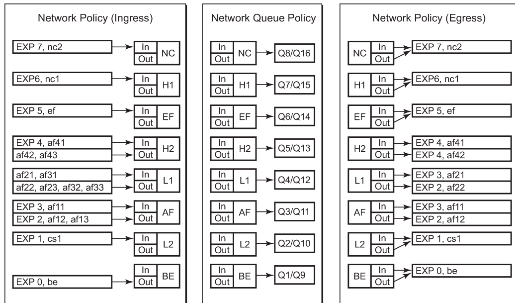
Figure 454: Visualization of Default Network Policies
