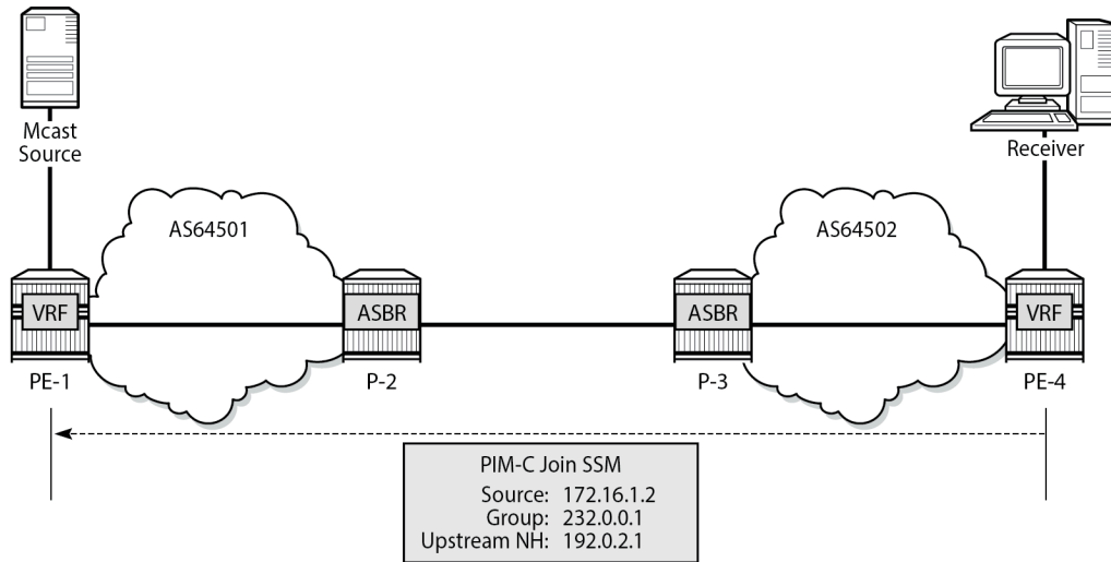
Figure 416: PIM-C Signaling
