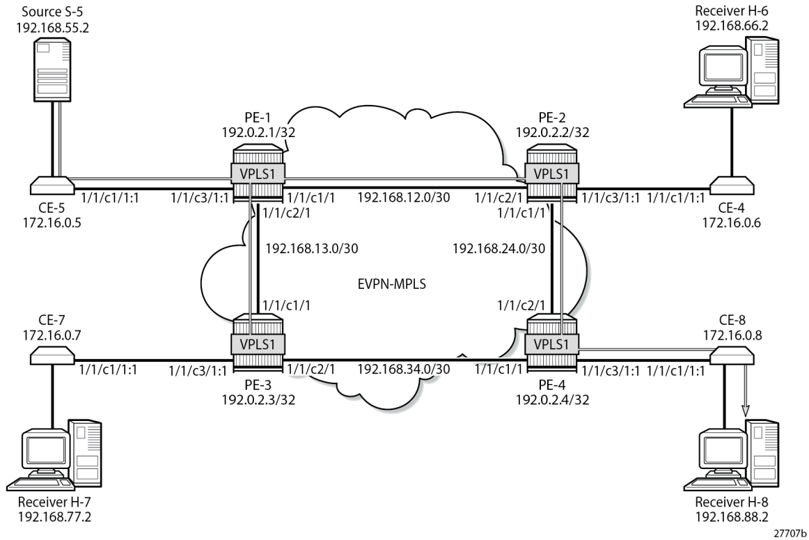
Figure 288: Multicast Stream (192.168.55.2, 232.1.1.1) with PIM Snooping Enabled
