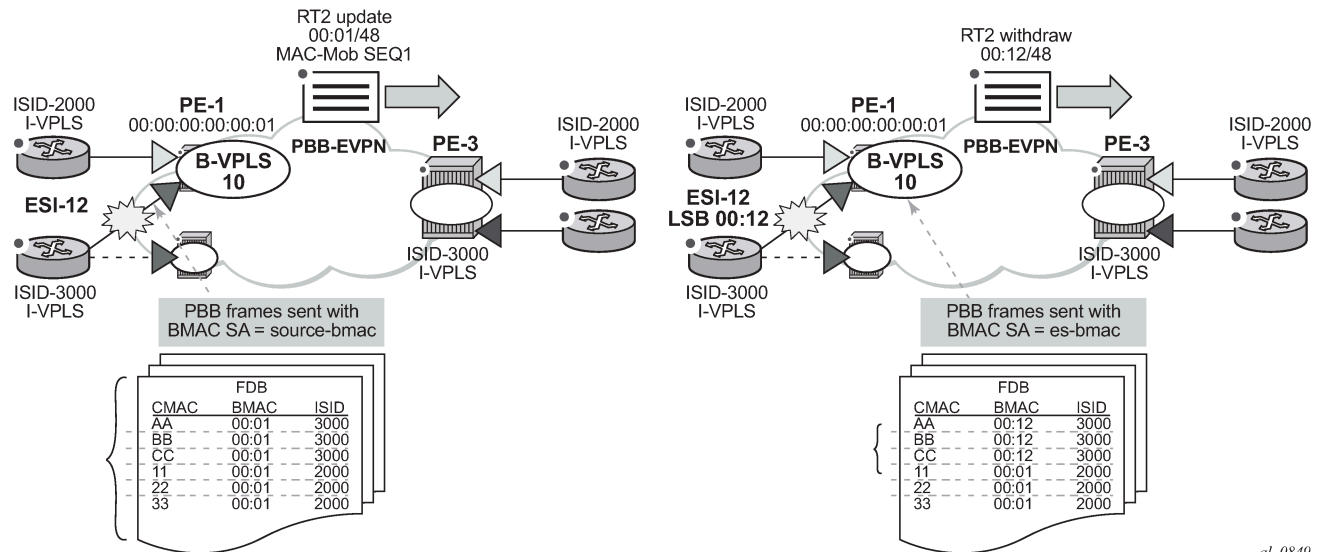
Figure 105: The use of ES BMAC to minimize CMAC flush
