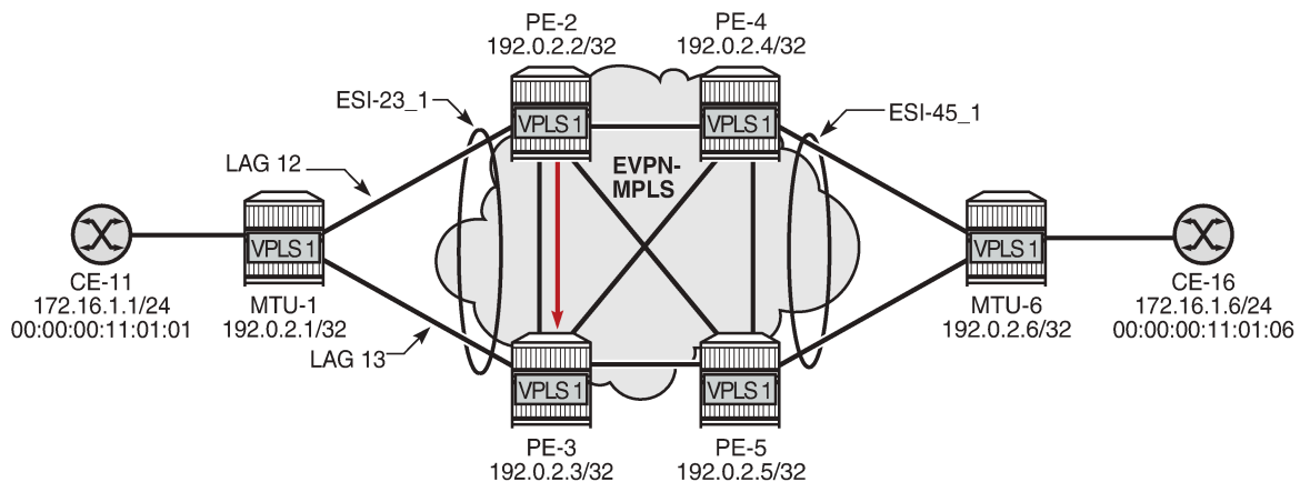
Figure 242: DF switchover in single-active ESI-23_1
