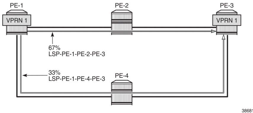
Figure 433: Weighted ECMP in AS 64496
