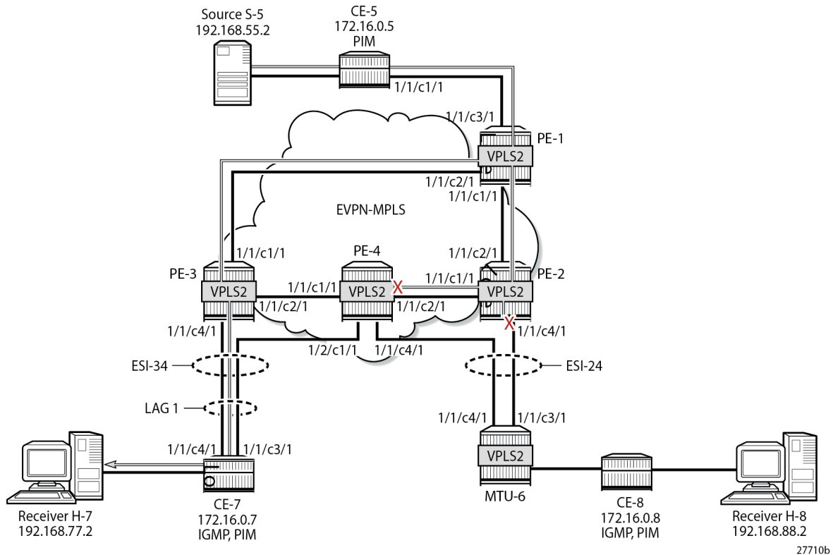
Figure 291: EVPN-MPLS with All-active Multi-homing and PIM Snooping Enabled – Receiver H-7 Joined
