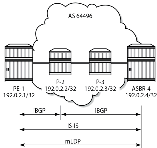
Figure 379: AS 64496 Protocols
