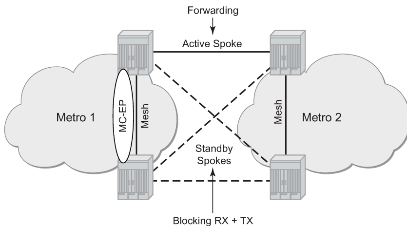
Figure 220: Multi-chassis endpoint with mesh resiliency
