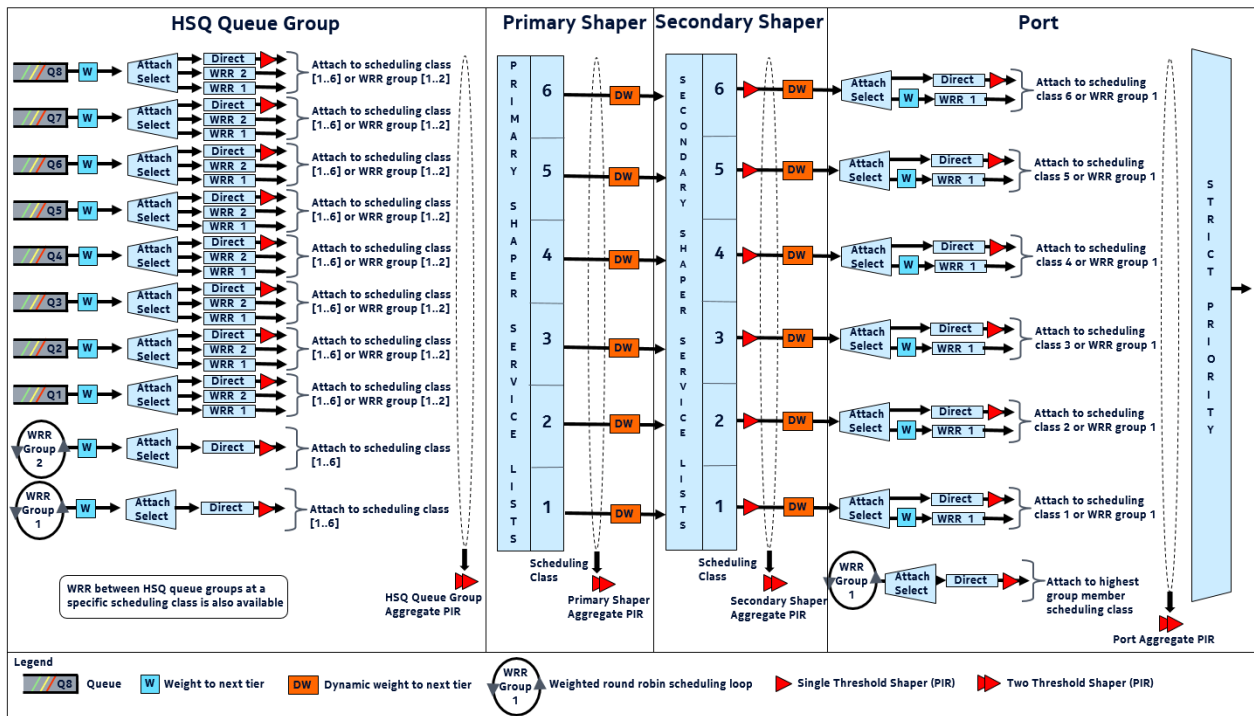
Figure 446: Egress HSQ IOM Scheduling Hierarchy
