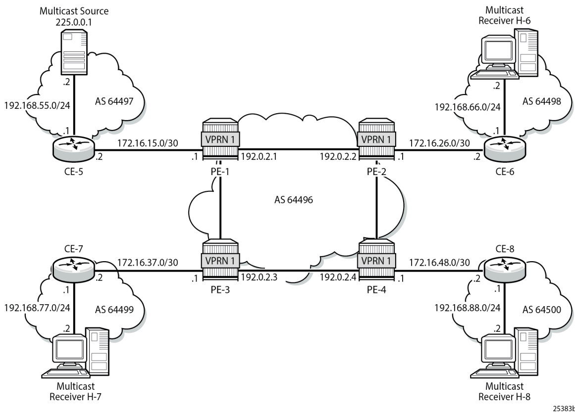
Figure 373: Network Topology
