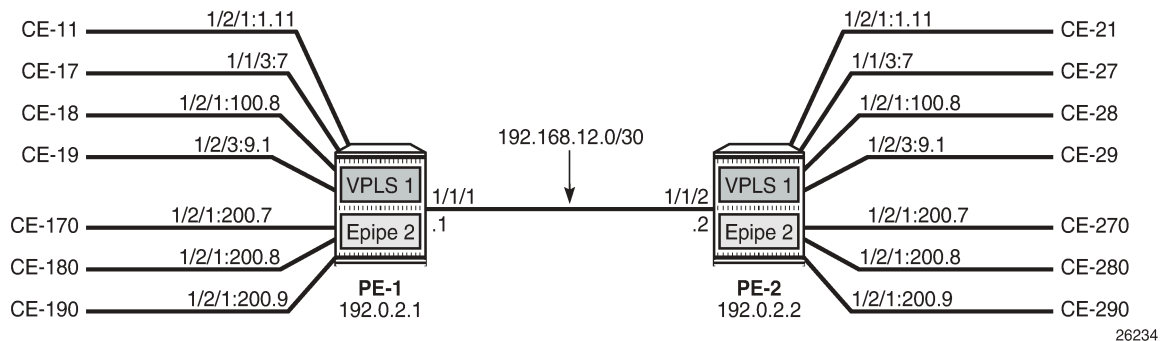
Figure 328: Example topology
