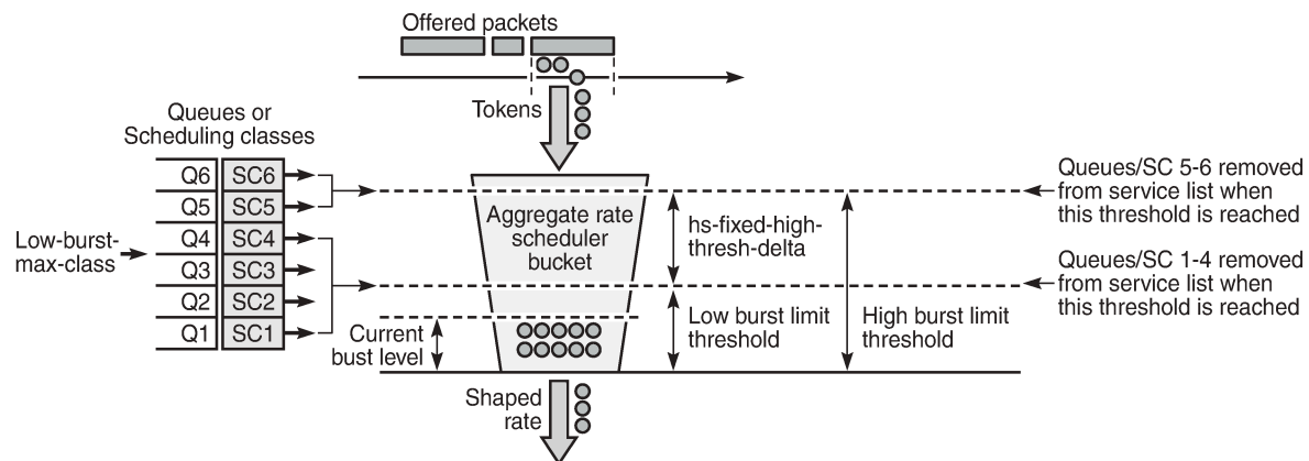
Figure 447: HSQ Queue Group and Secondary Shaper Aggregate Scheduler Bucket
