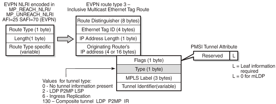
Figure 258: BGP-EVPN route type 3 with PTA
