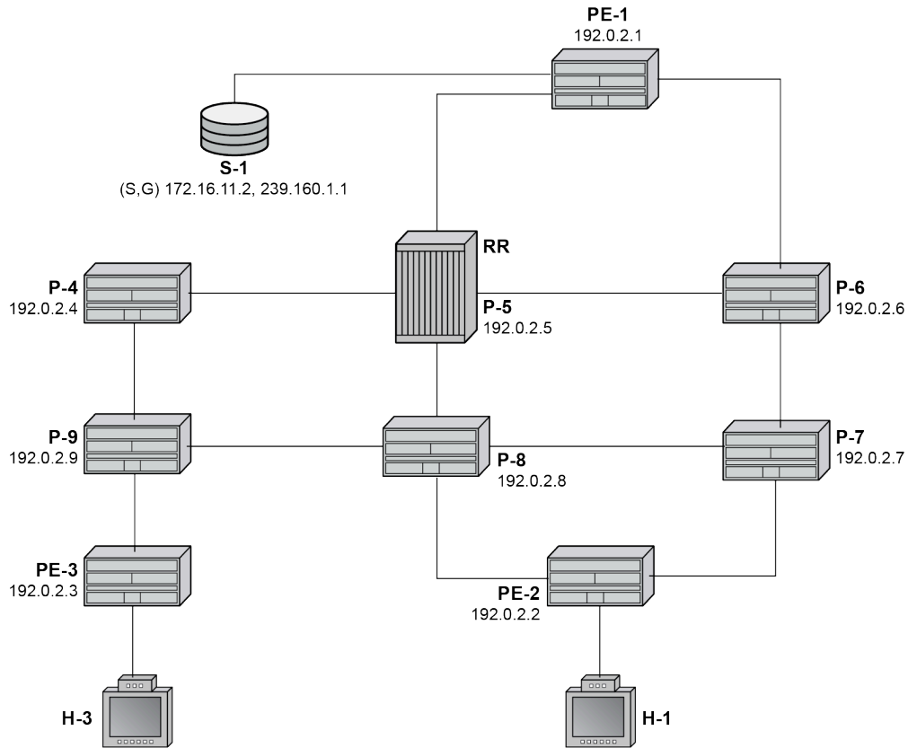
Figure 405: Core Diversity Network — Base OSPF
