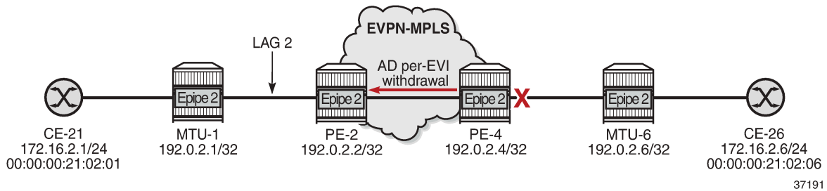
Figure 244: LLF in Epipe 2 - PE-4 failure
