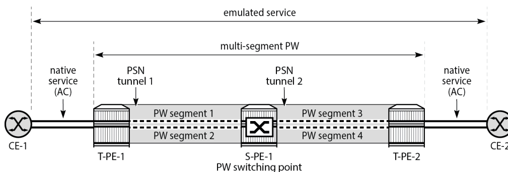
Figure 321: PW reference model
