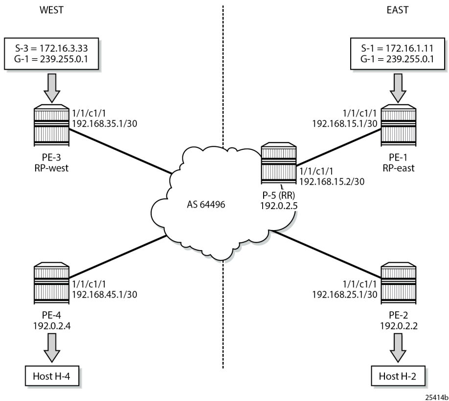
Figure 399: Schematic Topology
