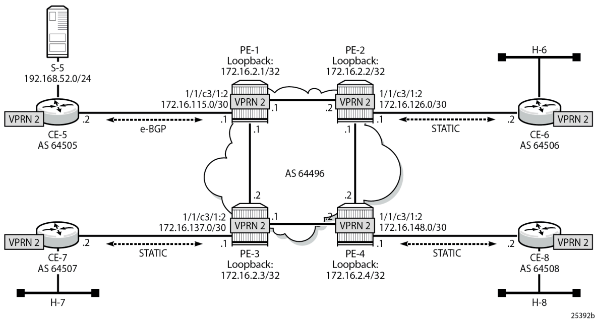
Figure 370: VPRN 2 Topology used for RSVP-TE P2MP
