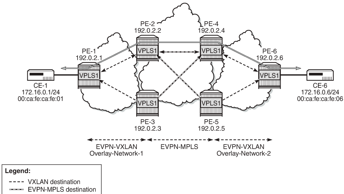
Figure 171: EVPN destinations created on multi-homed anycast DC GWs
