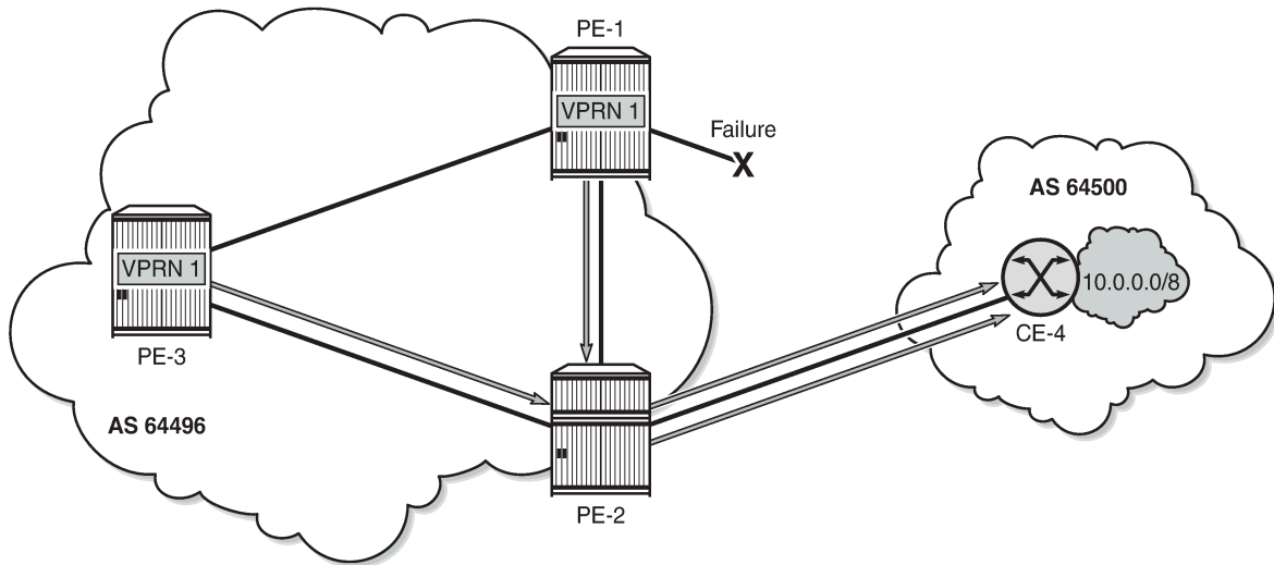
Figure 345: Traffic destined for prefix 10.0.0.0/8 after control plane convergence
