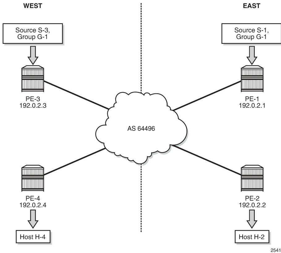
Figure 398: Source Redundancy Example.
