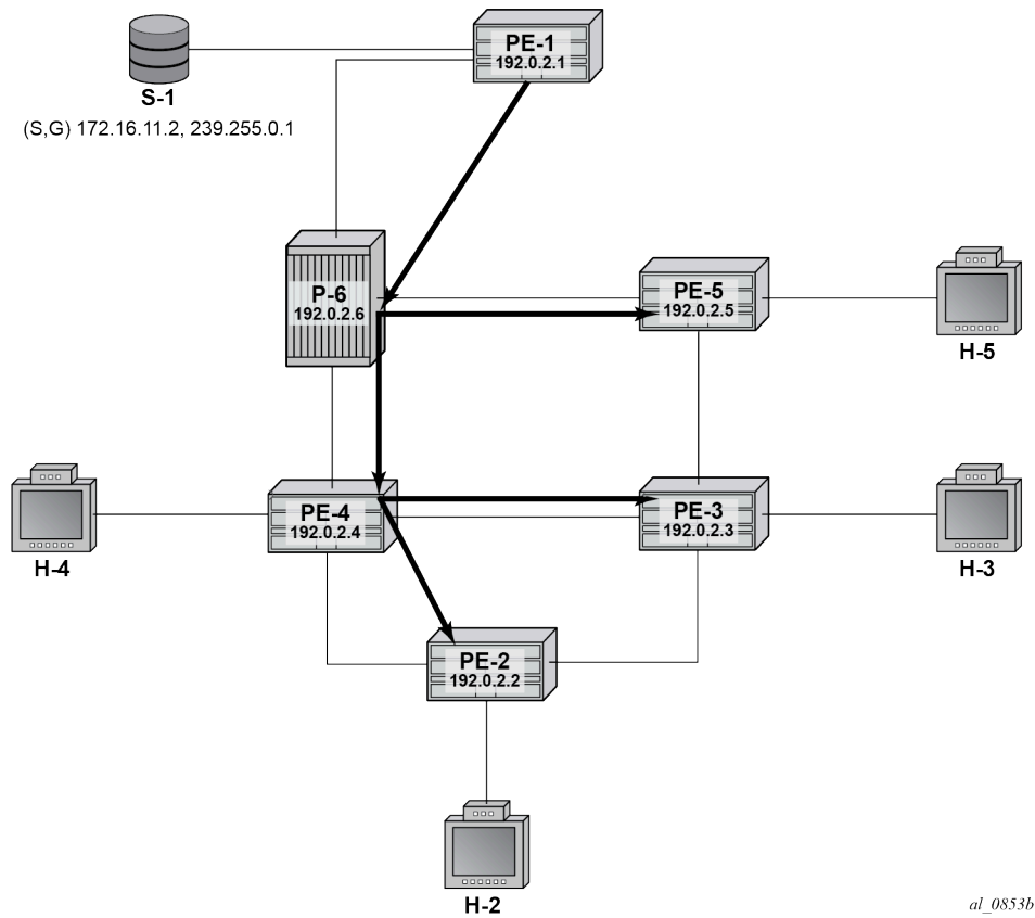
Figure 402: S-PMSI P2MP LSP Schematic
