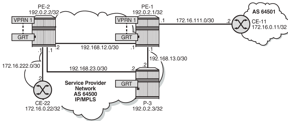
Figure 429: Example topology with IPv4 addresses
