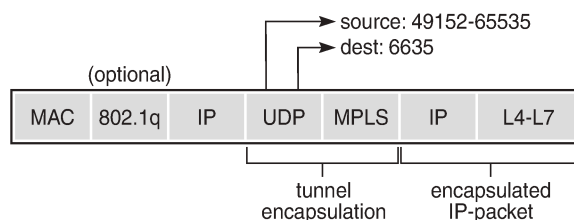
Figure 352: IP over MPLS over UDP packet format
