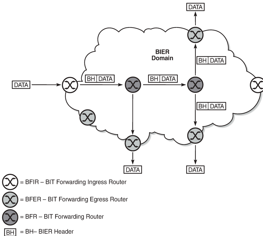
Figure 356: Bit Forwarding Router types
