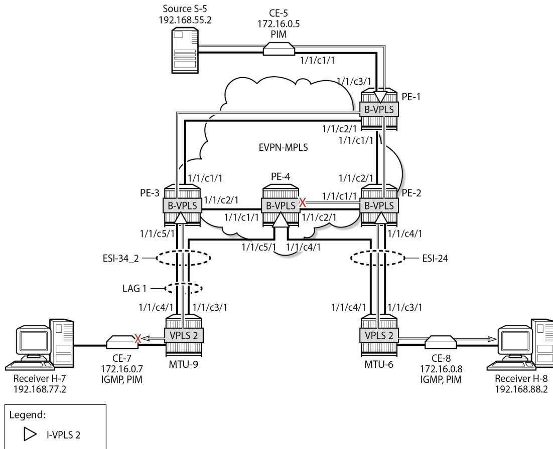
Figure 299: EVPN-MPLS with MH - PIM Snooping Disabled – Receiver H-8 Joined
