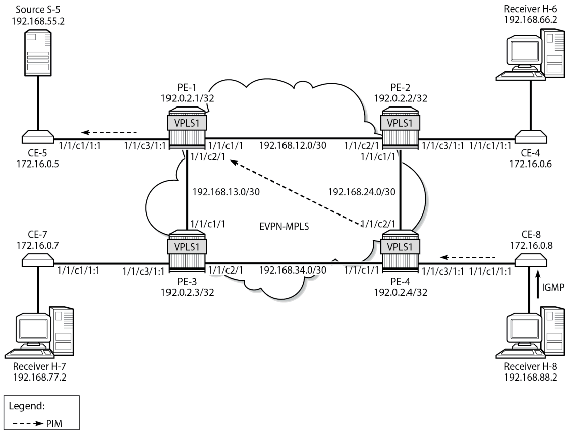
Figure 287: H-8 Joins (192.168.55.2, 232.1.1.1) and PIM Snooping is Enabled in Proxy Mode
