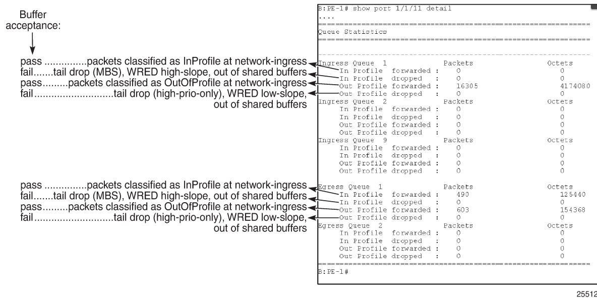
Figure 462: Ingress and Egress Network Port Queue Statistics
