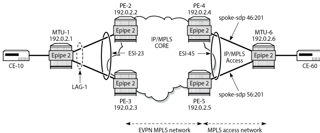
Figure 156: Example topology EVPN-VPWS with multihoming
