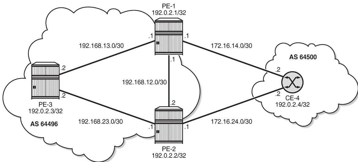
Figure 346: Example topology
