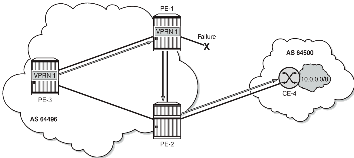
Figure 343: BGP FRR on PE-1 after failure of active link to CE
