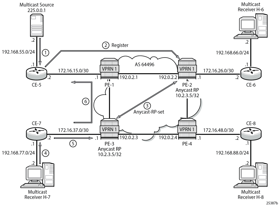
Figure 375: IGMP and PIM Control Messaging Schematic shows the sequence of IGMP and PIM control messaging.
