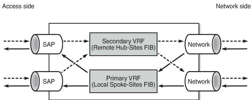
Figure 366: Internal VPRN logic on a PE router
