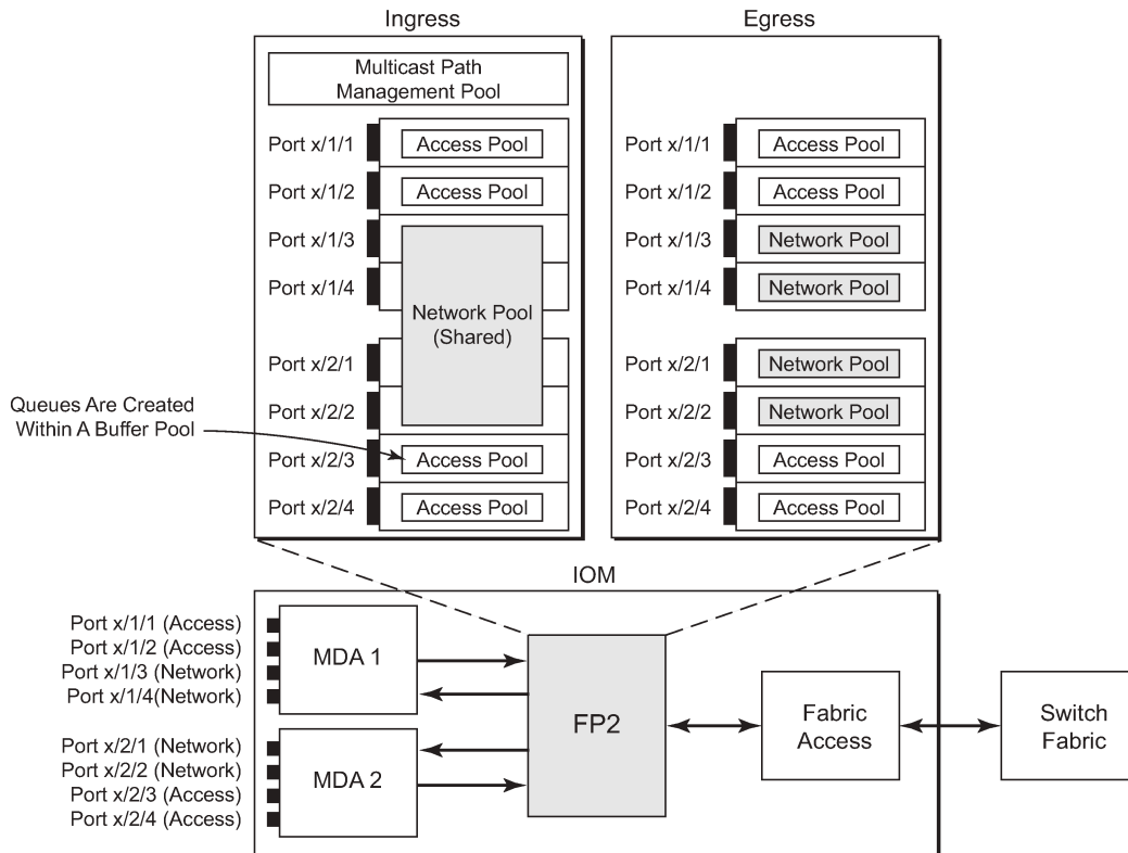
Figure 455: Default Buffer Pools
