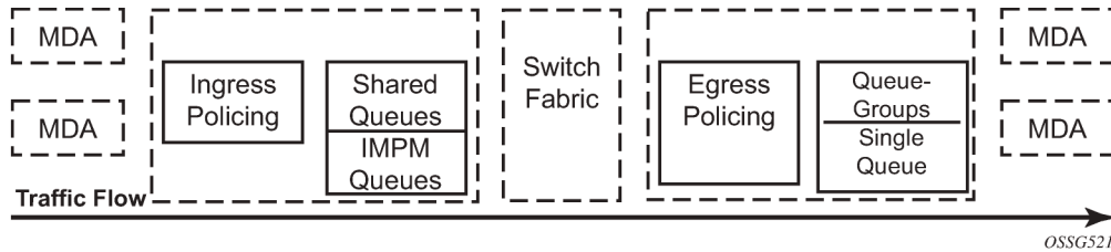
Figure 444: Post Policing Queues
