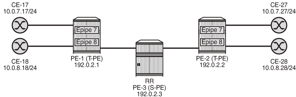
Figure 194: Dynamic MS-PW spoke-SDP FEC with auto-GRE spoke-SDPs
