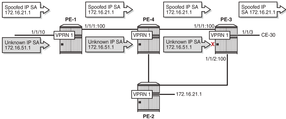
Figure 421: uRPF Checking in VPRN 1 on PE-3
