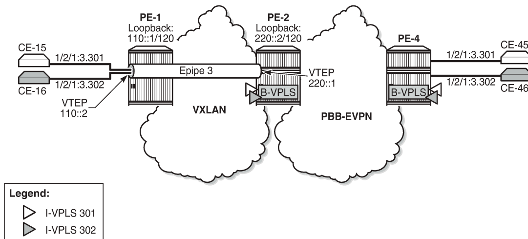
Figure 316: Example topology for static VXLAN termination on IPv6 addresses
