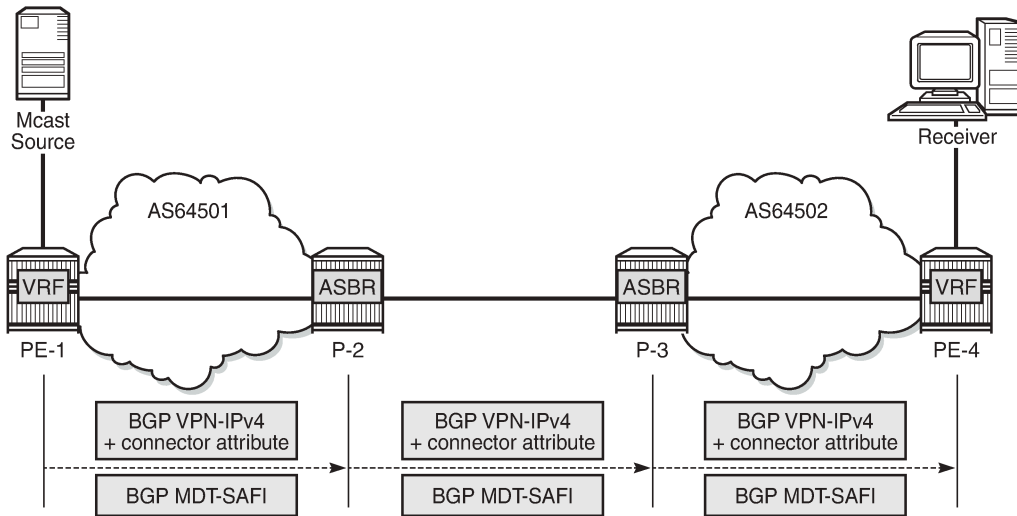
Figure 409: BGP Signaling Steps
