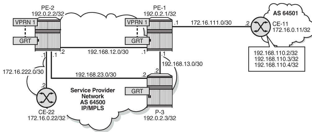
Figure 430: IPv4 VPRN to GRT route leaking for IS-IS
