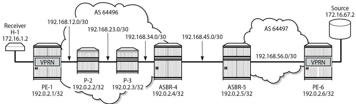
Figure 377: NG-MVPN Inter-AS Model B
