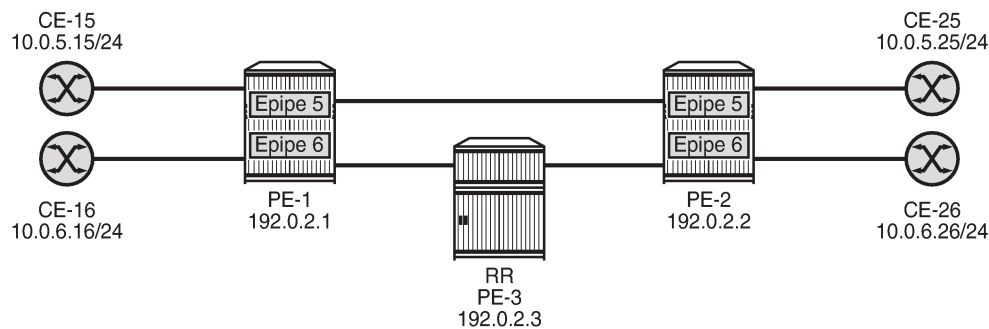
Figure 193: BGP-VPWS with auto-GRE spoke-SDPs
