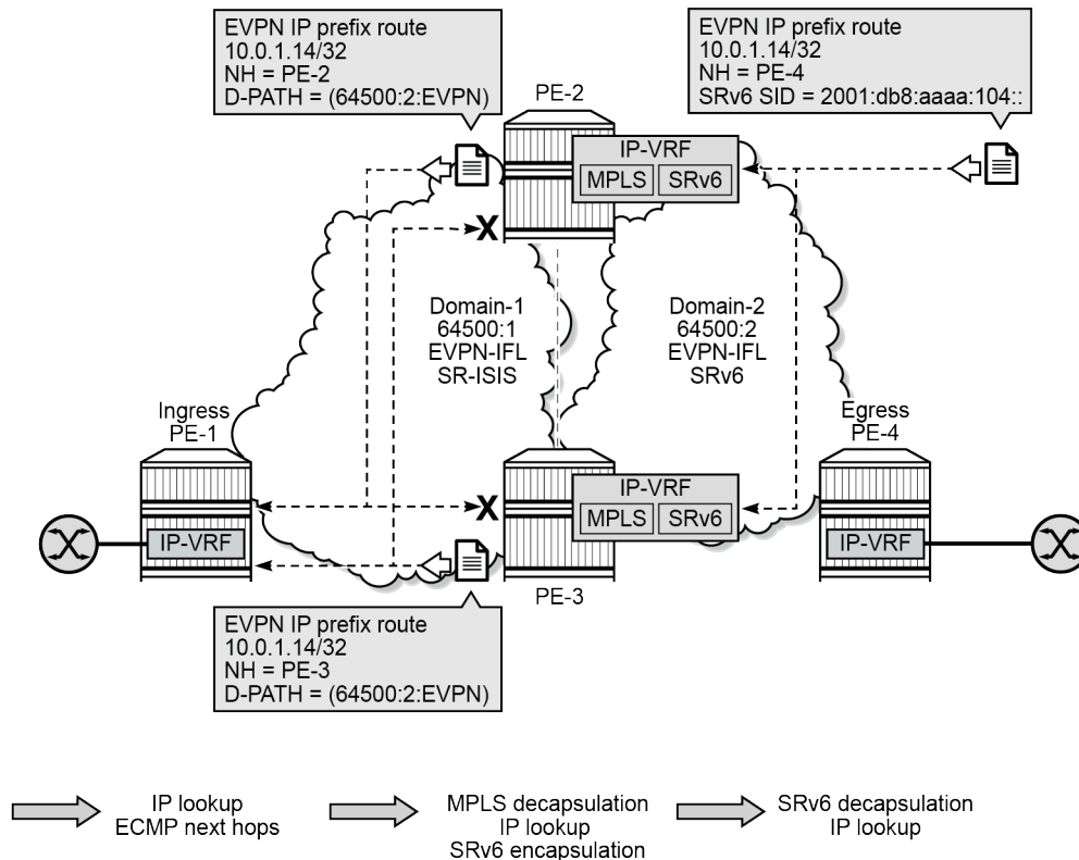
Figure 226: EVPN IP prefix routes readvertised between domains
