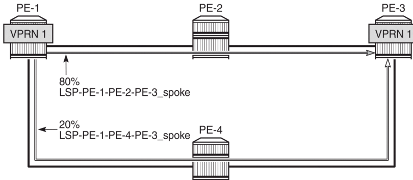
Figure 435: Weighted ECMP over RSVP LSPs used in a spoke SDP
