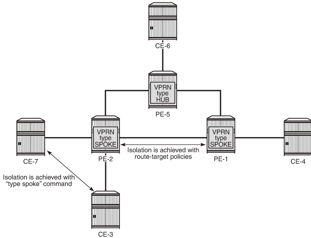
Figure 365: CE hub and spoke control plane isolation
