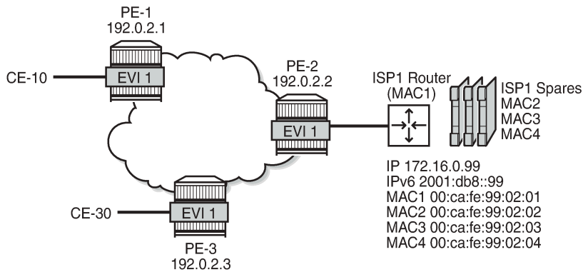
Figure 308: Example topology
