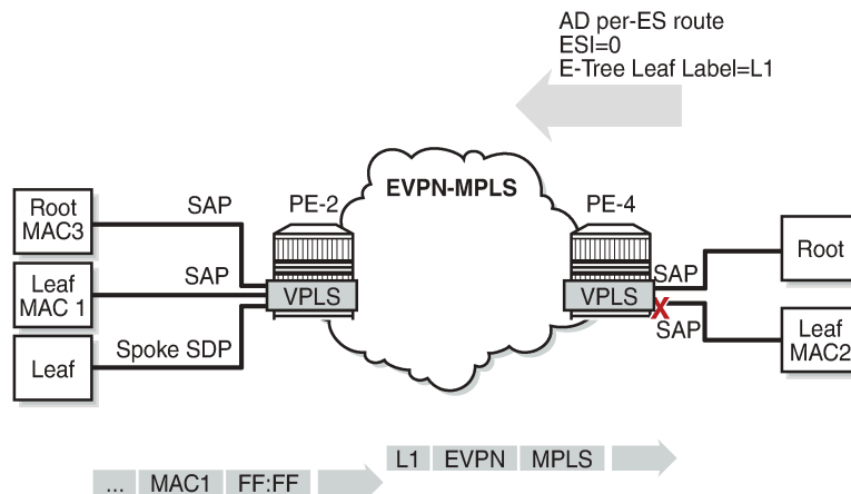
Figure 166: Egress Leaf Filtering for BUM Traffic
