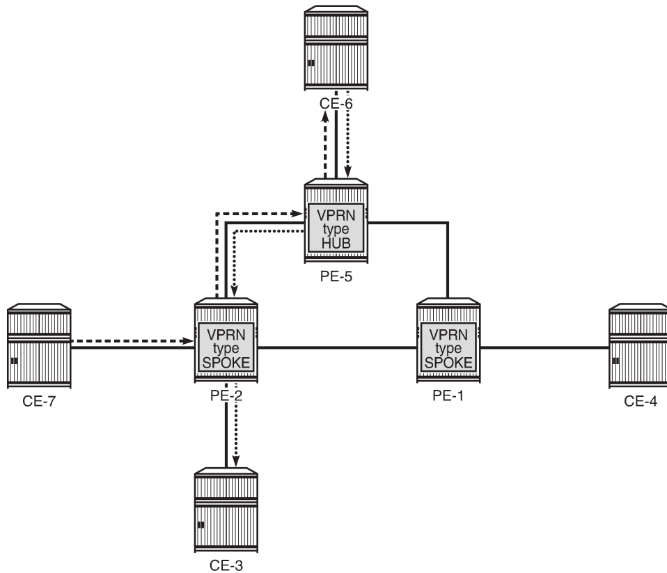
Figure 364: CE hub and spoke data path
