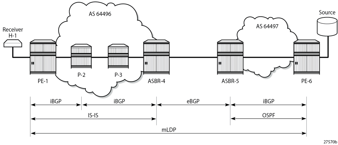
Figure 378: Inter-AS MVPN Protocol Requirements
