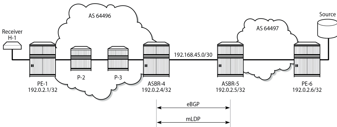
Figure 381: Inter-AS Protocols
