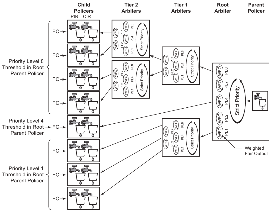
Figure 441: Policer and Arbiter Hierarchy
