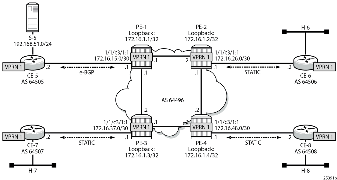
Figure 369: VPRN 1 Topology used for mLDP
