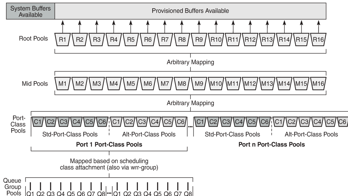
Figure 448: HSQ Buffer Pool Hierarchy
