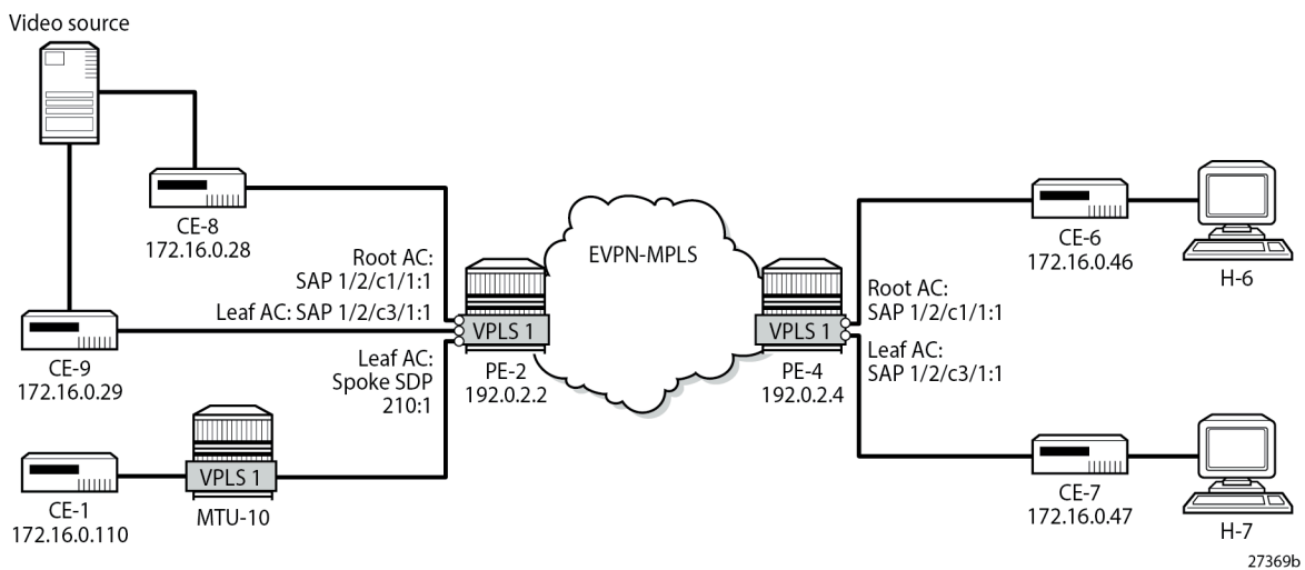
Figure 167: Example Topology for EVPN-MPLS E-Tree without Multi-homing
