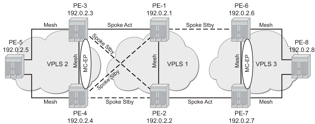
Figure 222: Example topology
