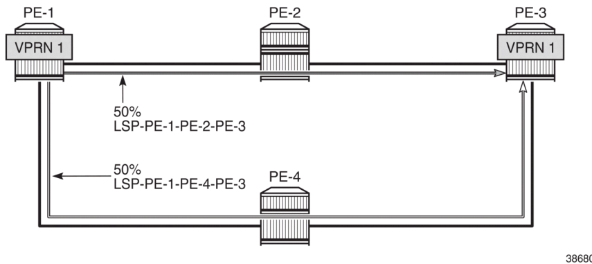
Figure 432: Regular ECMP in AS 64496
