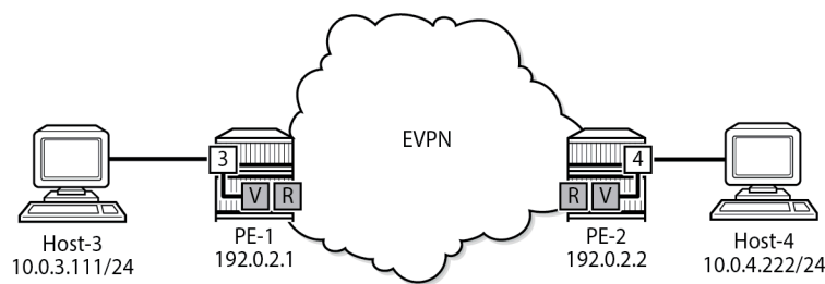
Figure 134: Example topology with services - EVPN-MPLS
