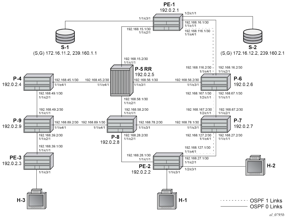
Figure 404: Core Diversity Network
