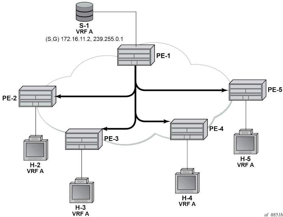
Figure 400: Multicast VPN
