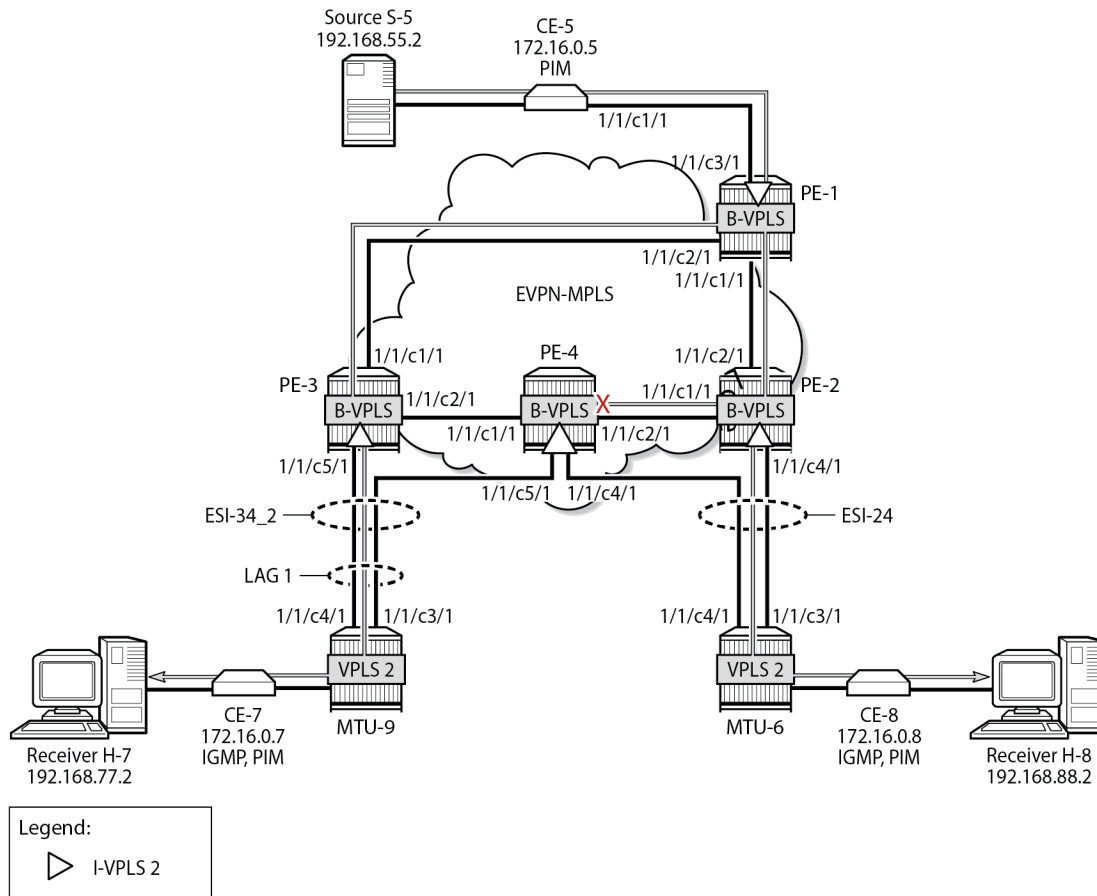
Figure 300: EVPN-MPLS with MH and PIM Snooping – Receivers H-7 and H-8 Joined
