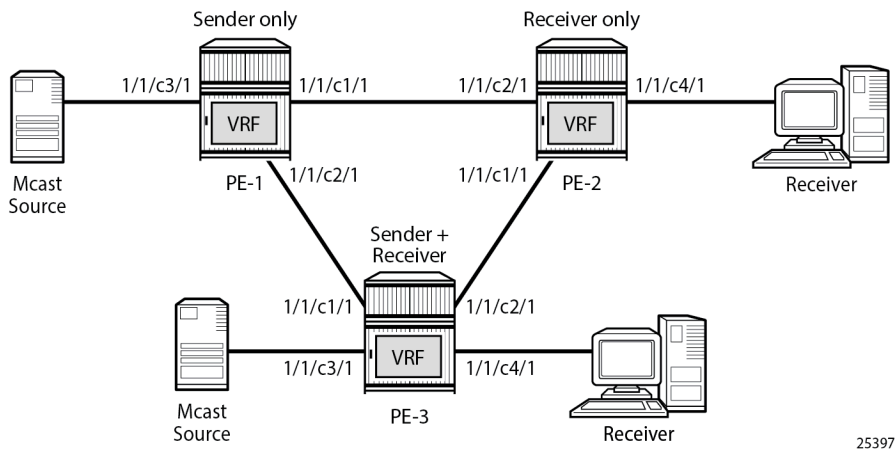
Figure 393: Example Topology
