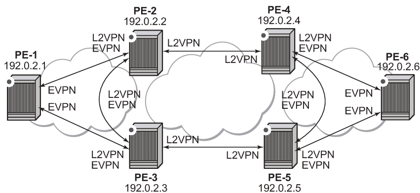
Figure 108: BGP adjacencies and enabled families
