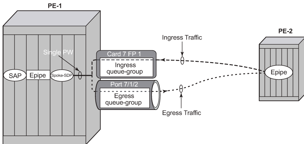
Figure 452: Example Epipe Pseudowire Topology
