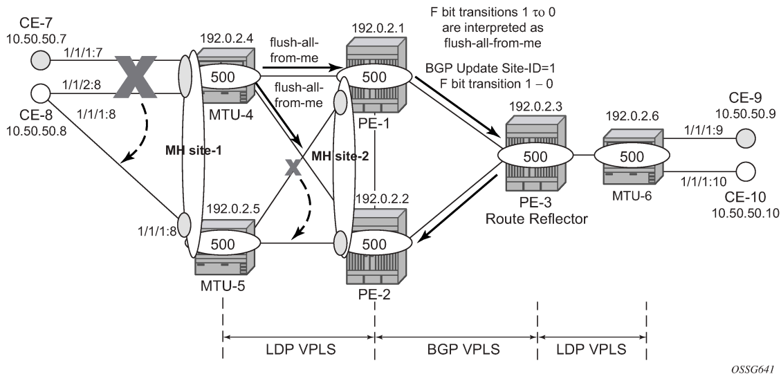
Figure 50: MAC flush for BGP MH
