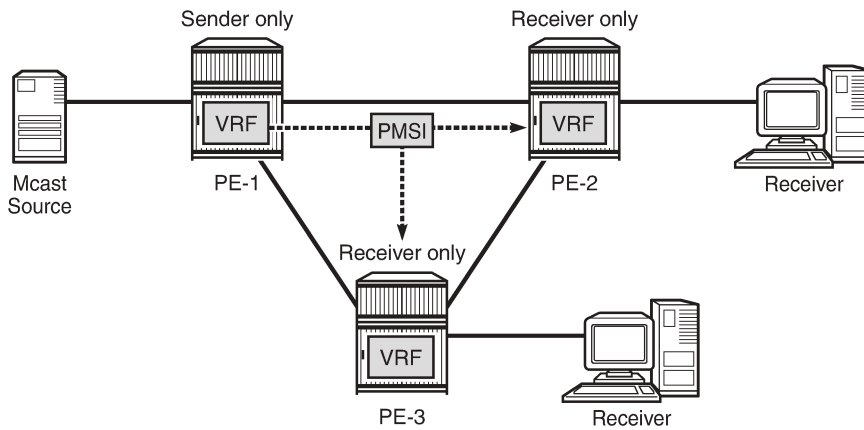
Figure 392: Optimized PMSI Structure
