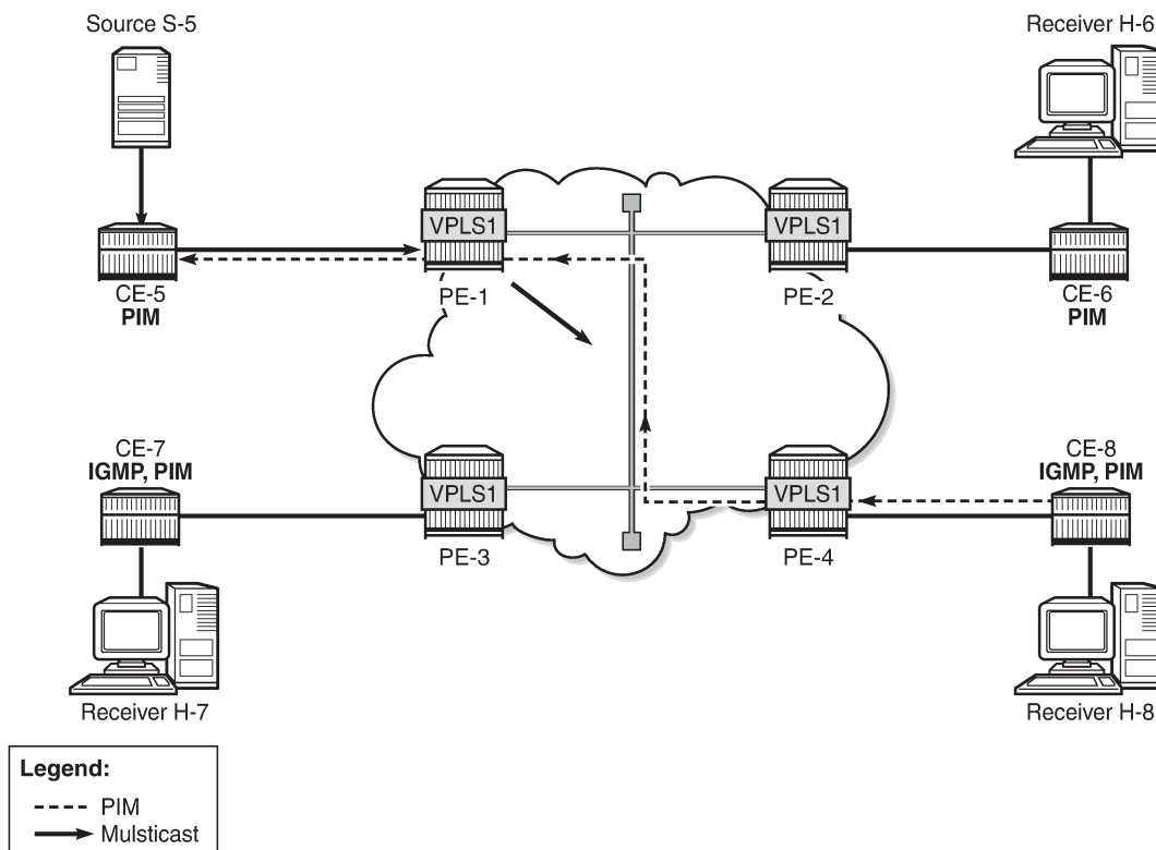
Figure 280: Multicast in VPLS with PIM Snooping in Snooping Mode
