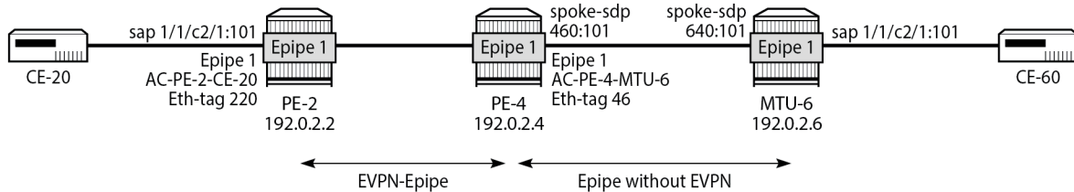
Figure 155: Example topology for EVPN-VPWS without multihoming
