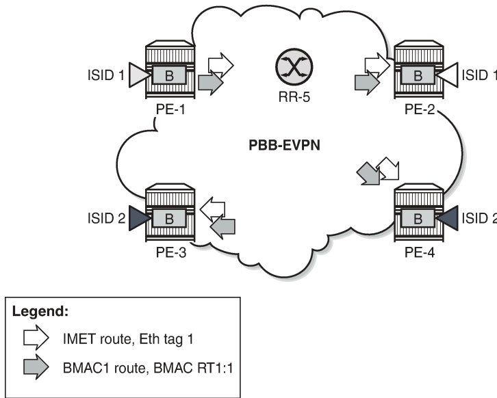
Figure 270: PBB-EVPN B-VPLS-based RT
