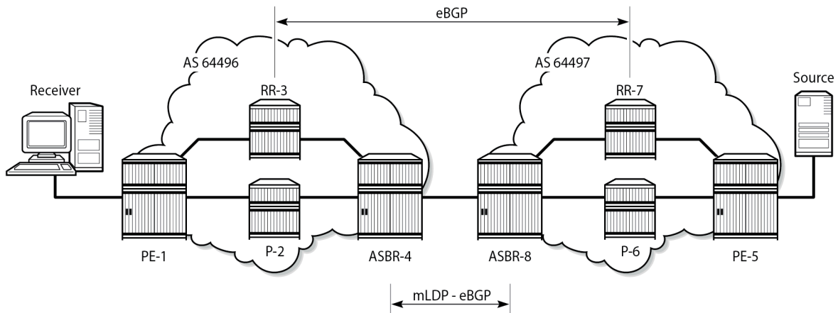
Figure 388: Inter-AS Protocols
