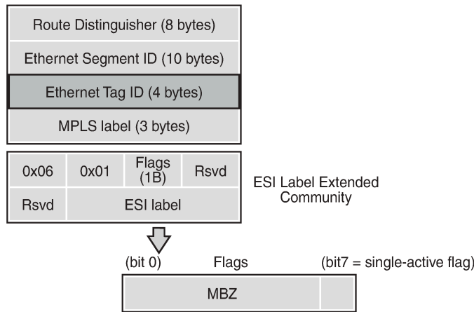
Figure 174: BGP-EVPN AD per-ES route
