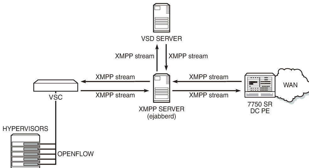
Figure 185: F-D XMPP provisioning setup
