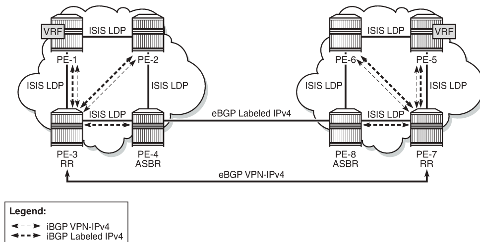
Figure 355: Protocol overview
