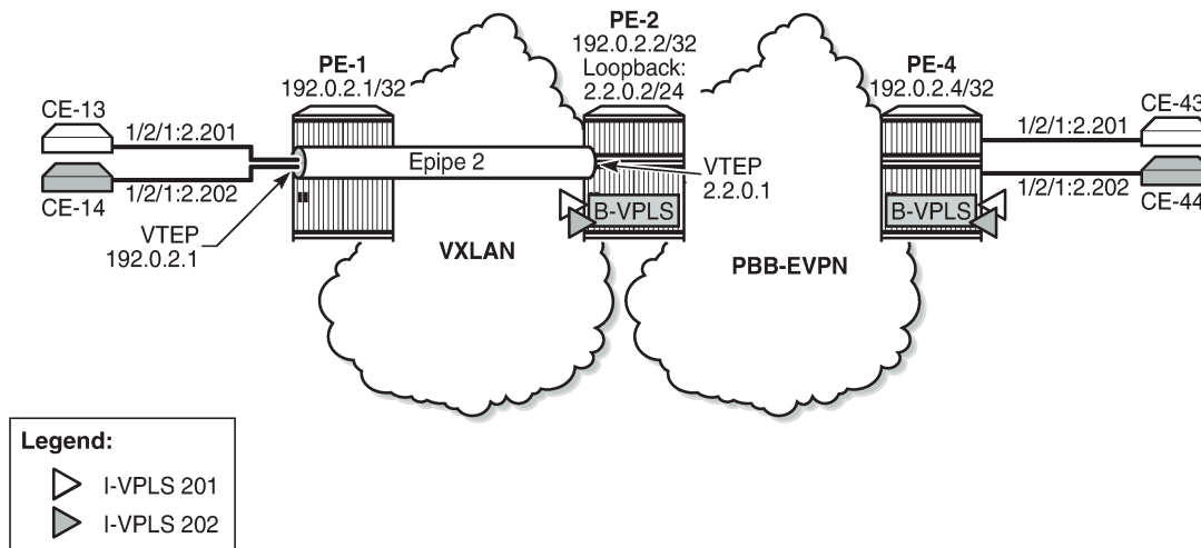
Figure 315: Example topology for static VXLAN termination on non-system IPv4 addresses
