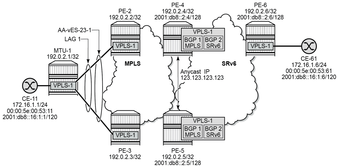
Figure 146: Example topology with VPLS-1
