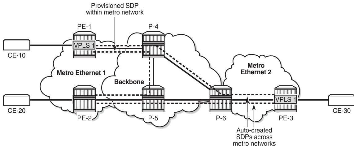
Figure 206: SDP bindings in VPLS 1 with prefer-provisioned-sdp option
