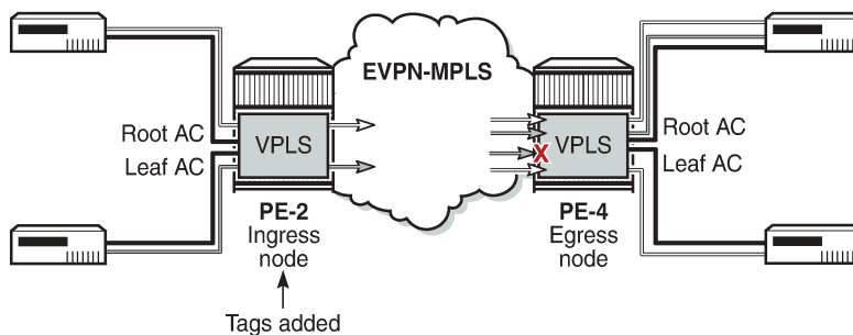
Figure 162: Frame Forwarding in a VPLS E-Tree without EVPN
