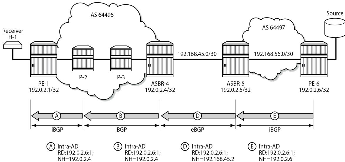
Figure 382: BGP MVPN Intra-AD Route Advertisement
