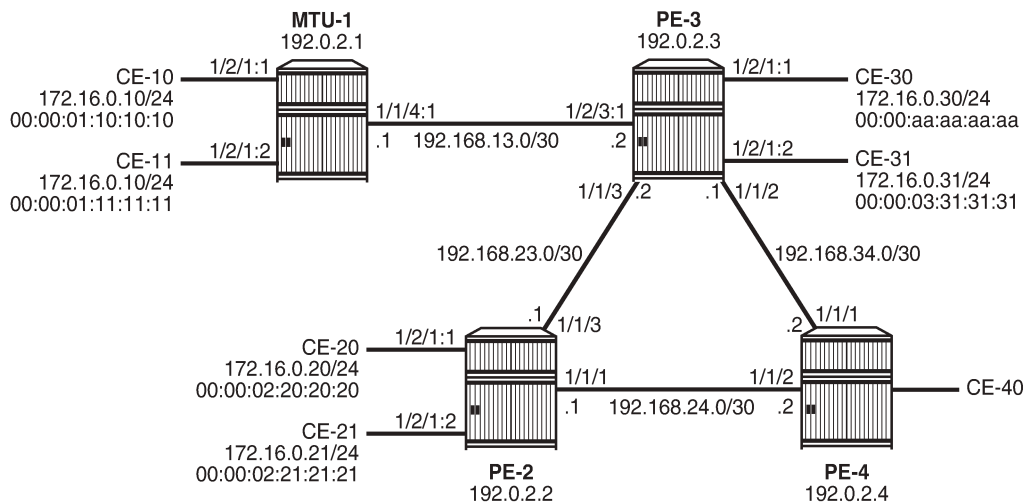
Figure 66: Example topology
