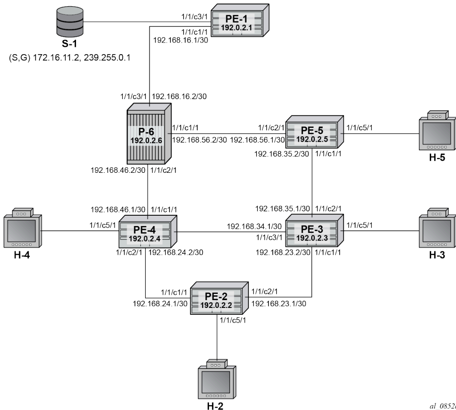
Figure 401: Schematic Topology
