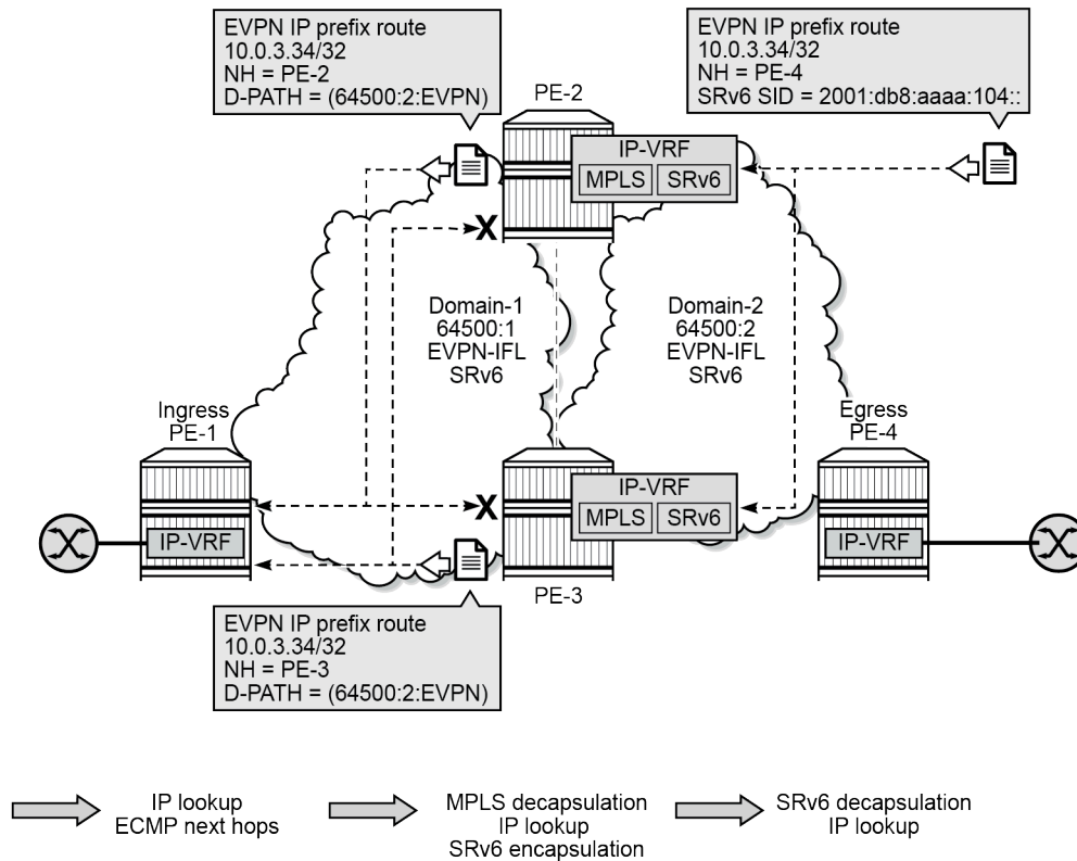
Figure 229: EVPN IP prefix routes readvertised between SRv6 domains
