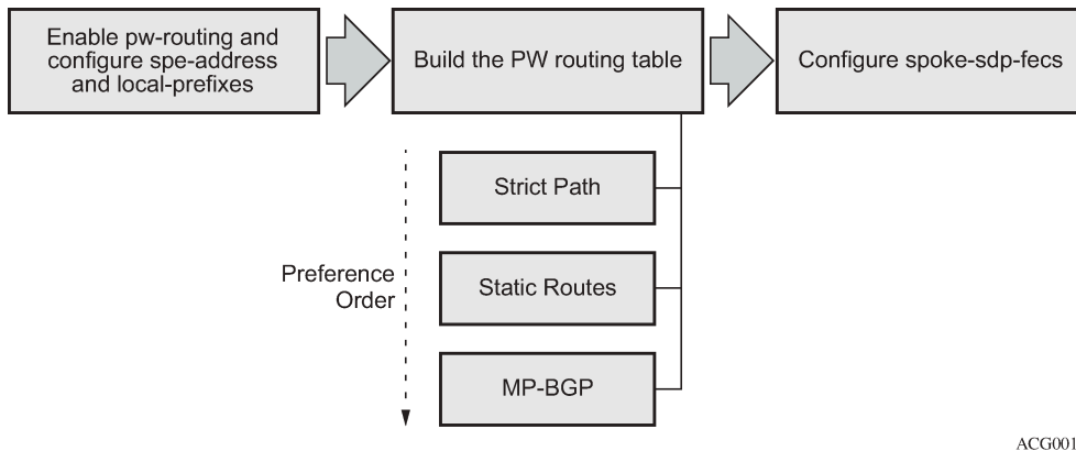
Figure 233: Configuration flowchart
