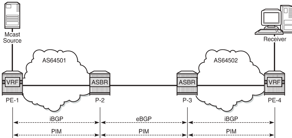
Figure 408: Protocols Used for Inter-AS MVPN
