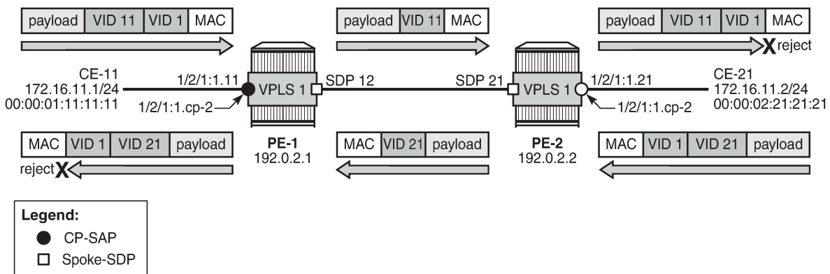
Figure 334: No traffic between two QinQ CP SAPs - VLAN translation not supported
