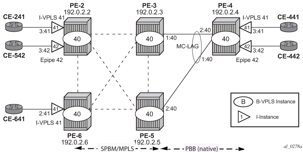
Figure 312: Access resiliency example topology
