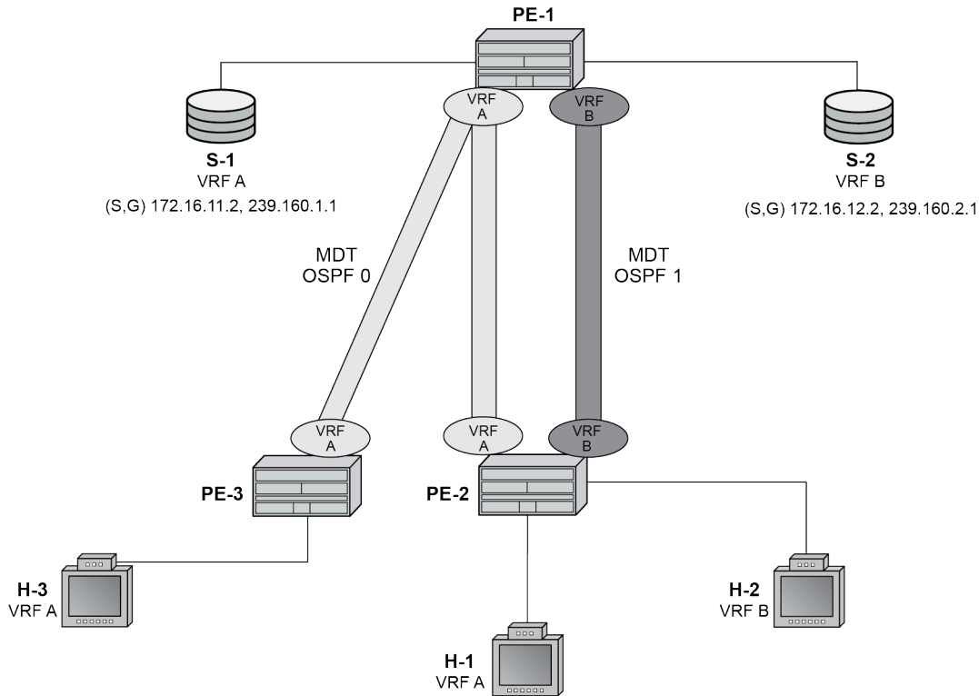
Figure 403: Core Diversity Schematic
