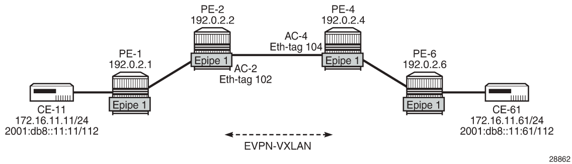
Figure 177: Single-homed EVPN-VXLAN Epipe 1 using system IP addresses
