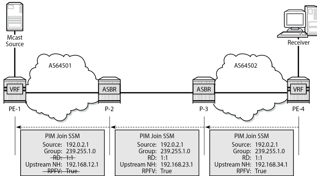
Figure 417: PIM-P Signaling Steps for Data MDT
