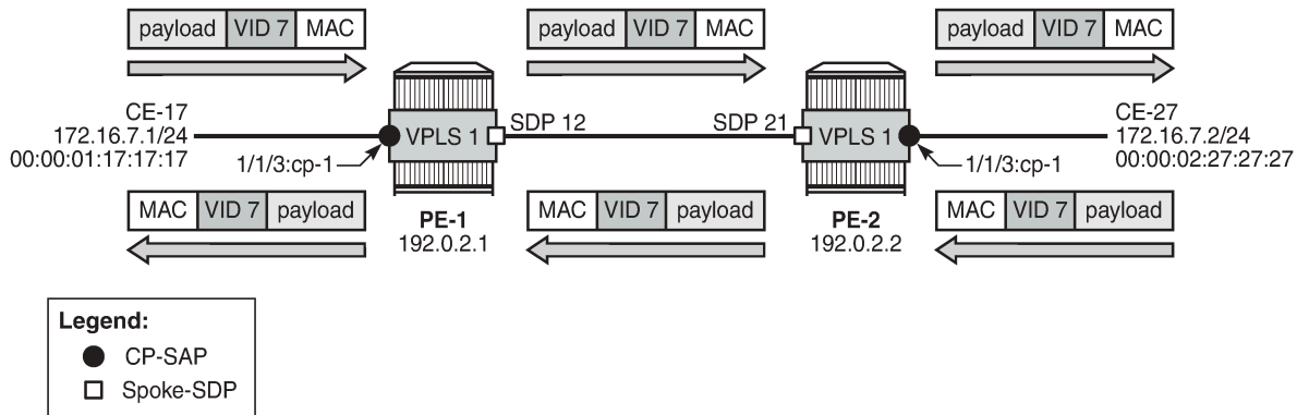
Figure 326: Customer VID is preserved between dot1q CP SAPs - no VLAN translation
