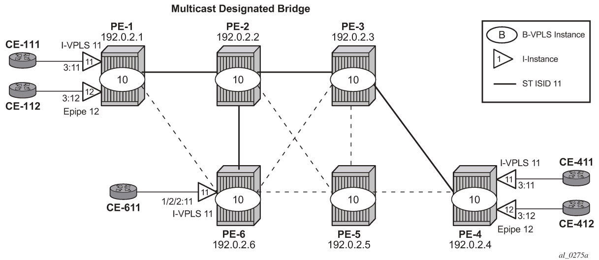
Figure 309: Basic SPBM topology
