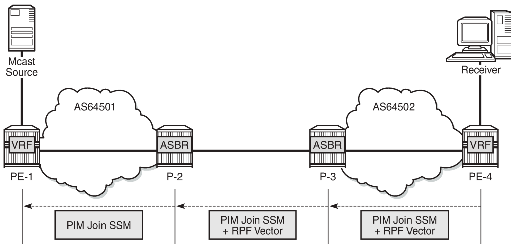
Figure 410: PIM-P Signaling Steps for Default MDT
