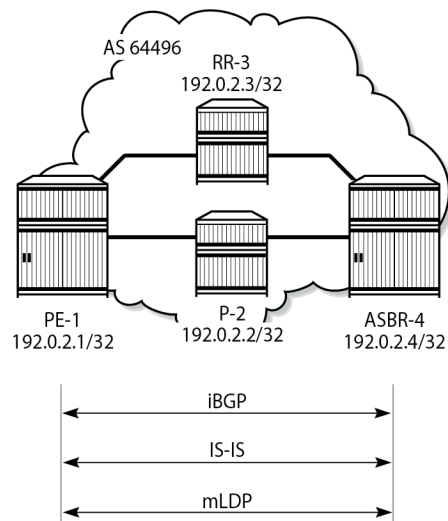
Figure 386: AS 64496 Protocols
