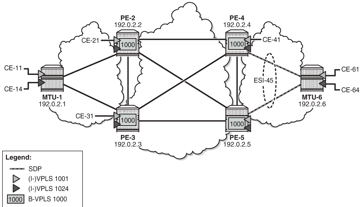
Figure 269: Example topology with single-active ES
