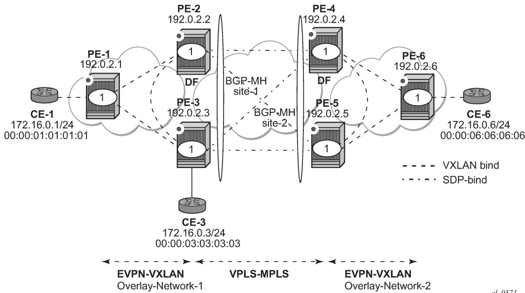
Figure 107: EVPN-VXLAN example topology
