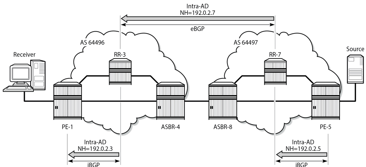
Figure 389: BGP MVPN Intra-AD Route Advertisement
