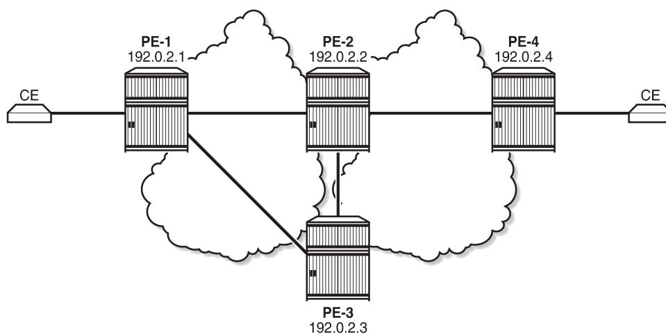
Figure 238: Example topology
