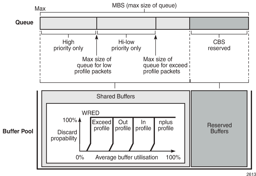
Figure 458: Egress Buffer Pools and Queue Sizing
