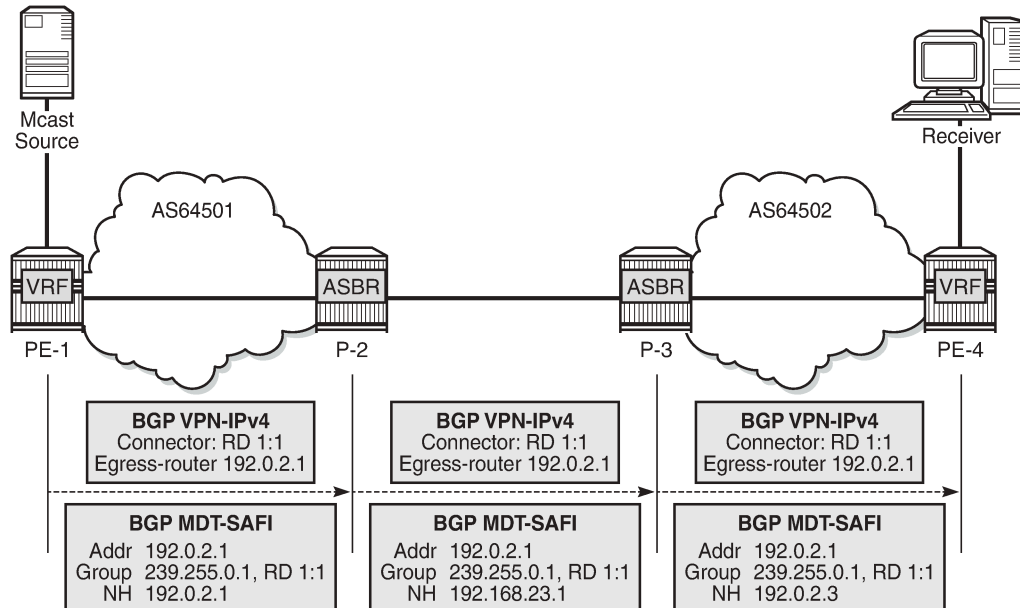
Figure 414: BGP Signaling Steps
