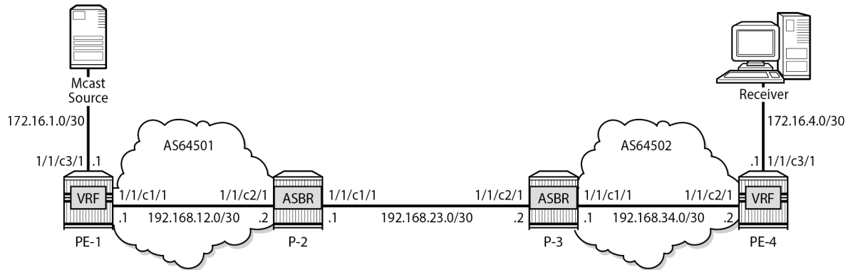
Figure 413: Example Topology Details
