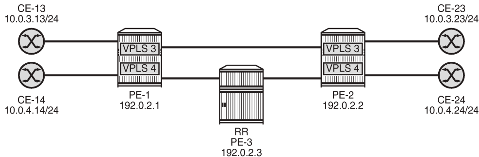
Figure 192: LDP-VPLS using BGP-AD with auto-GRE Spoke-SDPs
