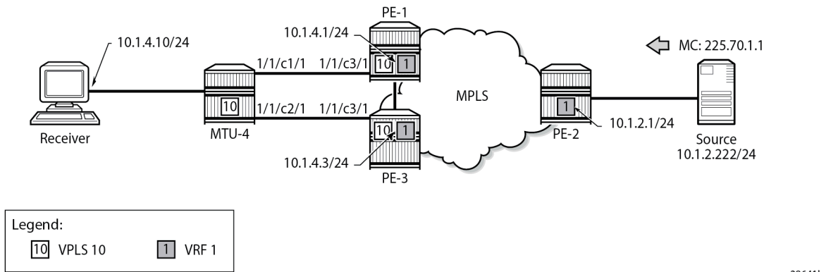
Figure 189: Multicast From an EVPN-MPLS Service Into an R-VPLS With All-Active EVPN Multi-Homing
