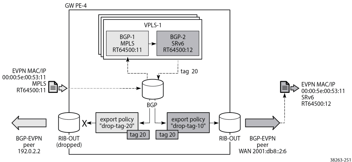
Figure 145: Default route tags per service instance avoid loops
