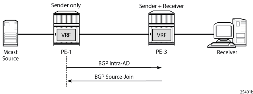
Figure 397: mLDP-Based BGP Message Flow Between PE-1 and PE-3
