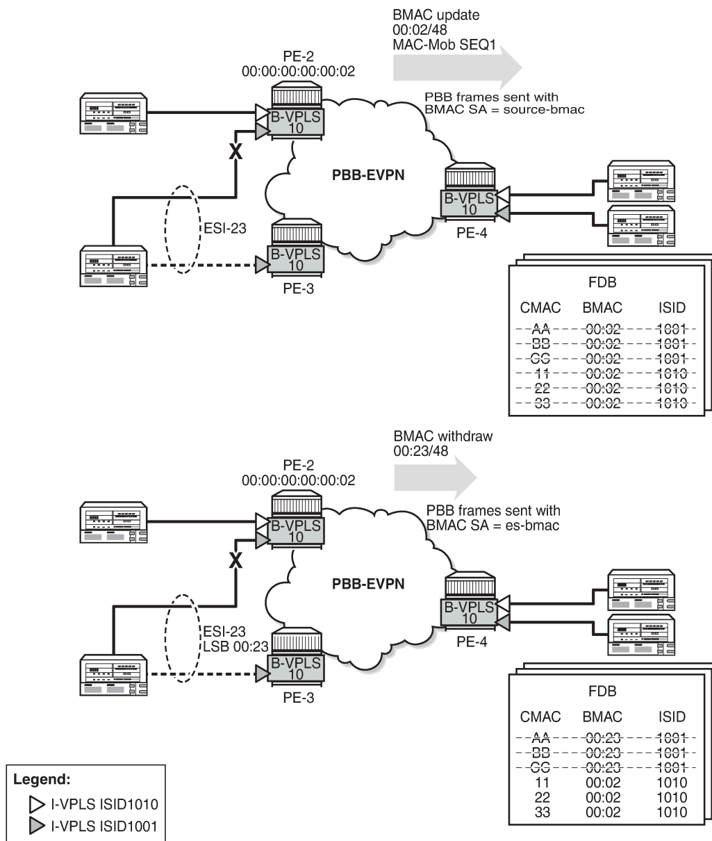
Figure 266: ISID-independent CMAC flush when ES fails
