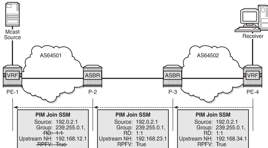
Figure 415: PIM-P Signaling Steps for Default MDT
