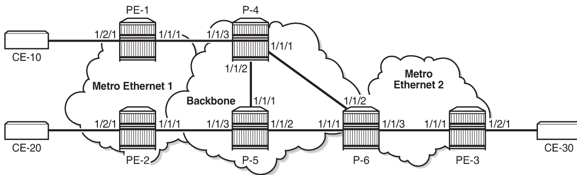
Figure 203: Example topology
