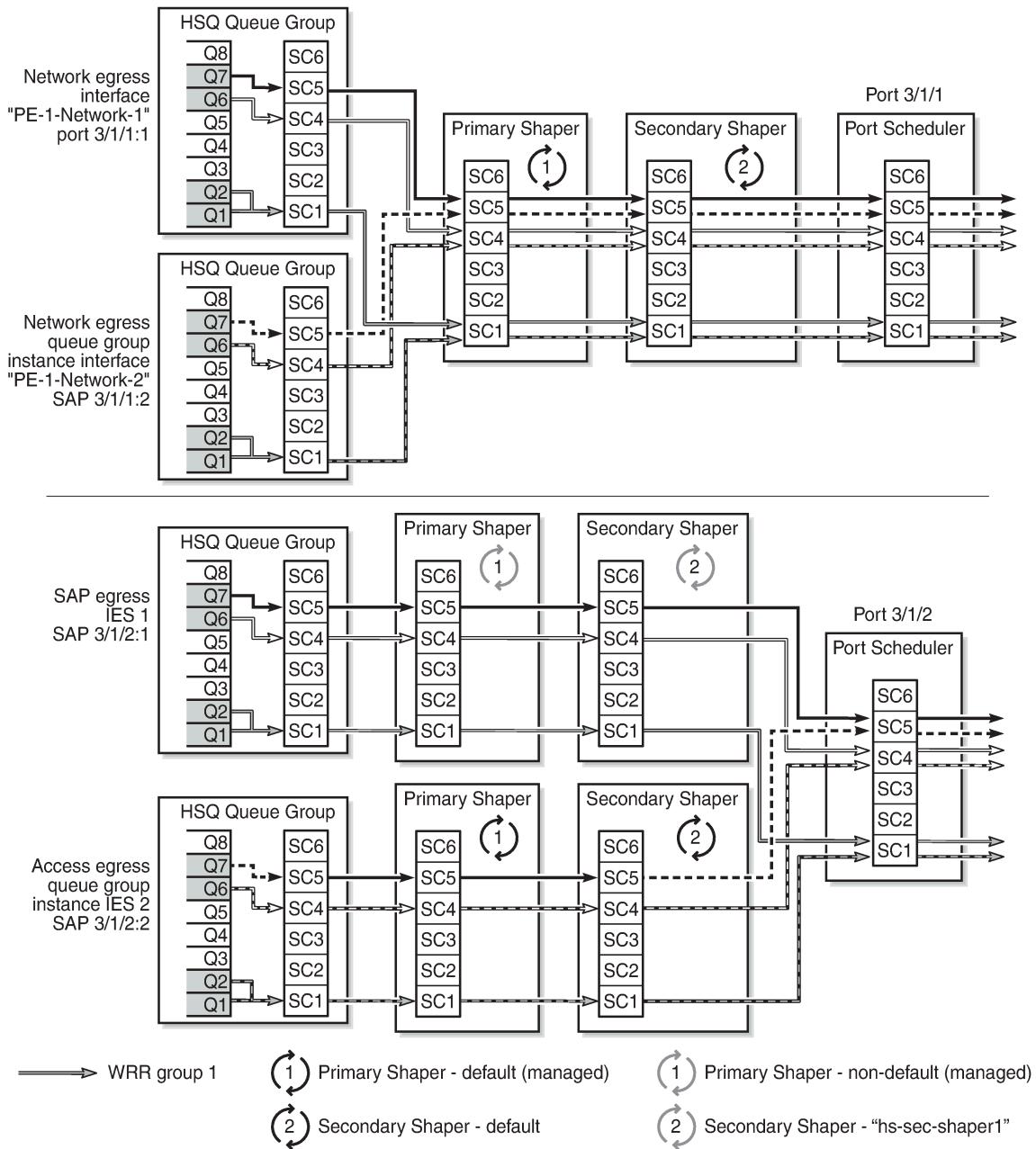
Figure 449: Configured QoS Paths
