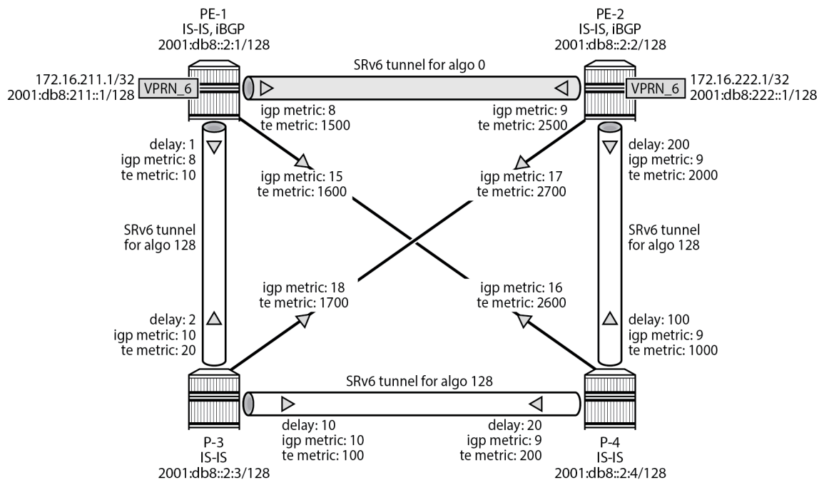
Figure 349: Example topology
