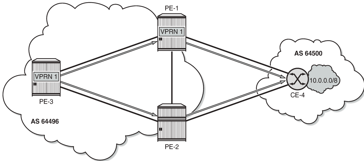
Figure 347: Loadsharing for traffic from PE-3 destined to 10.0.0.0/8
