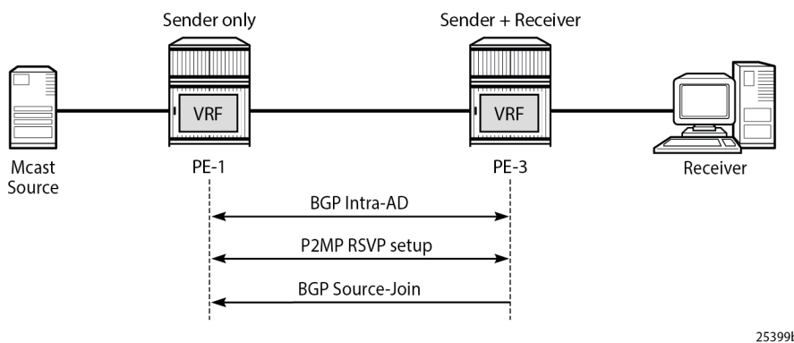
Figure 395: RSVP-Based BGP Message Flow Between PE-1 and PE-3
