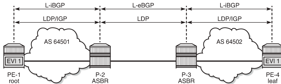
Figure 245: Example topology for inter-AS model C
