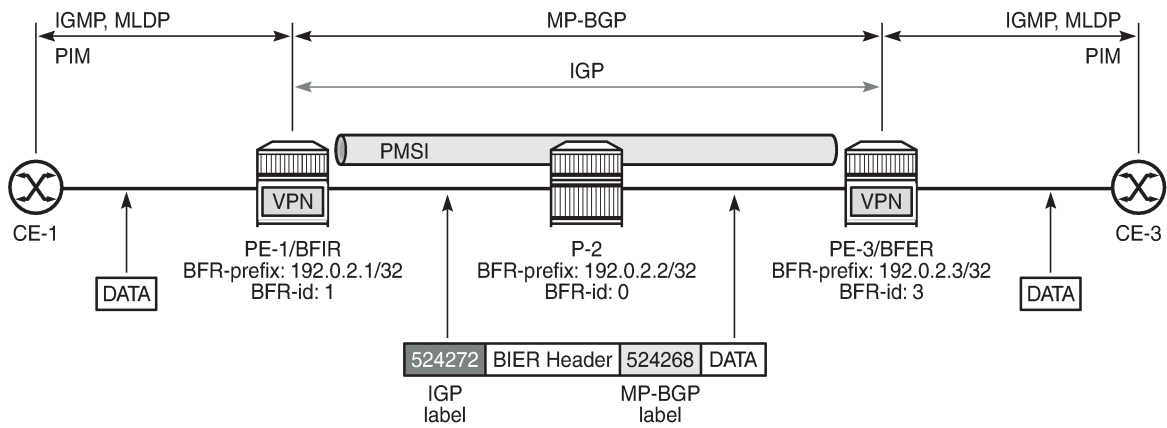
Figure 361: MVPN over BIER
