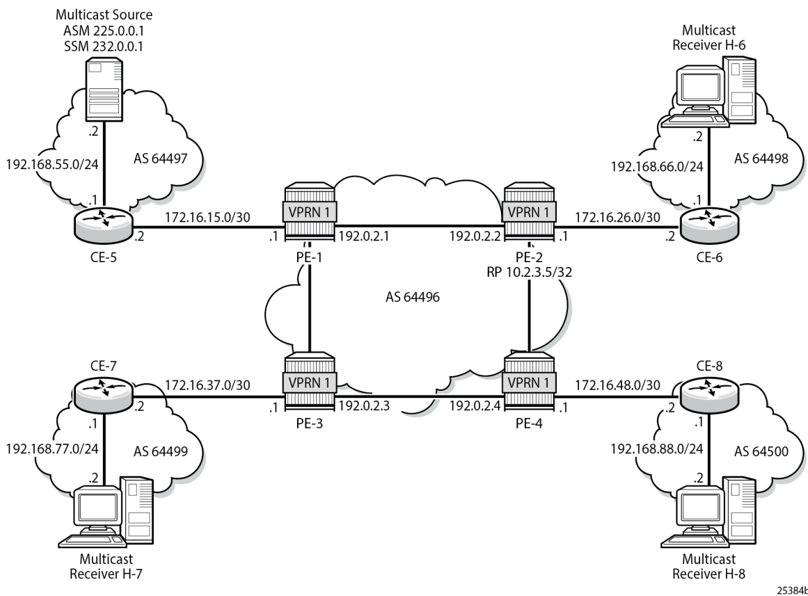
Figure 376: PIM SSM in Customer Signaling Plane
