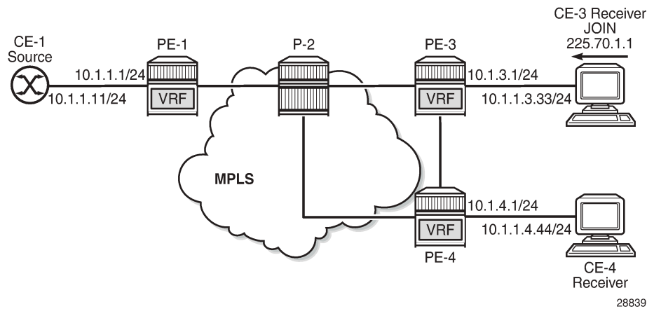
Figure 363: Intra-AS NG-MVPN over BIER
