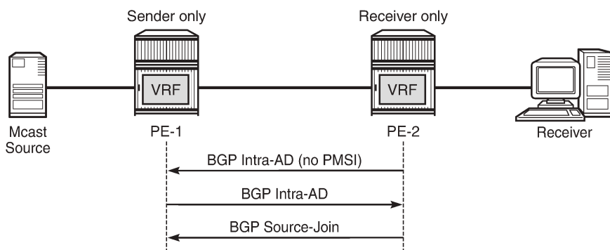
Figure 396: mLDP-Based BGP Message Flow Between PE-1 and PE-2
