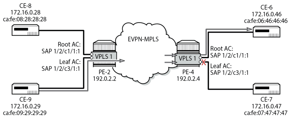
Figure 168: EVPN E-Tree Egress Filtering Based on MAC SA
