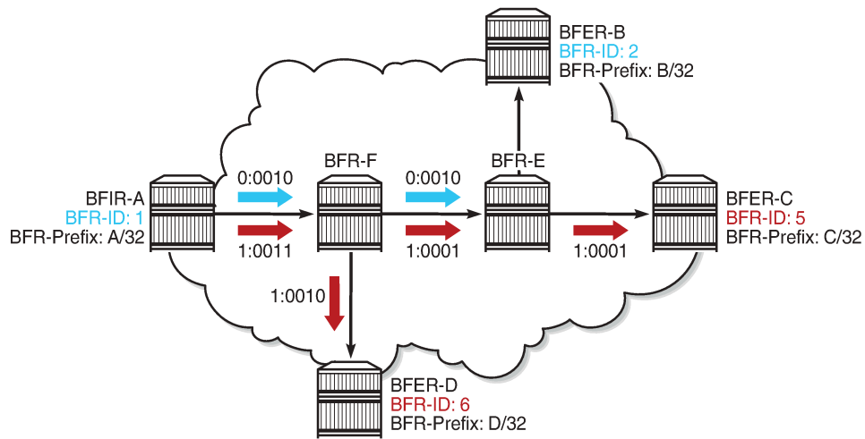
Figure 360: BIER sets
