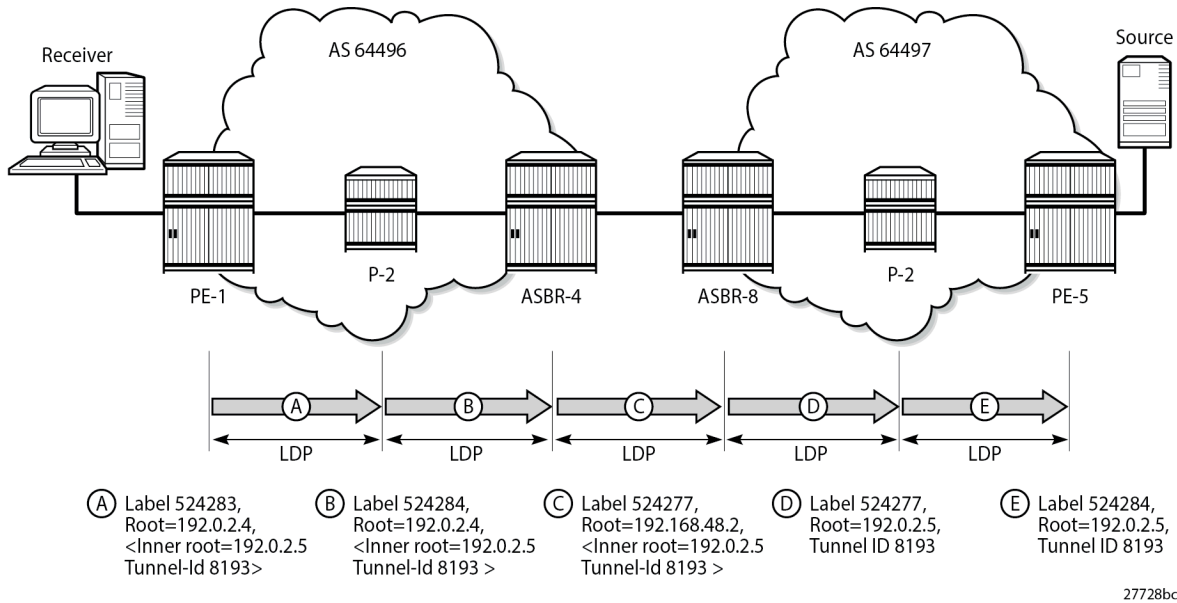
Figure 390: P2MP LDP Label Mapping
