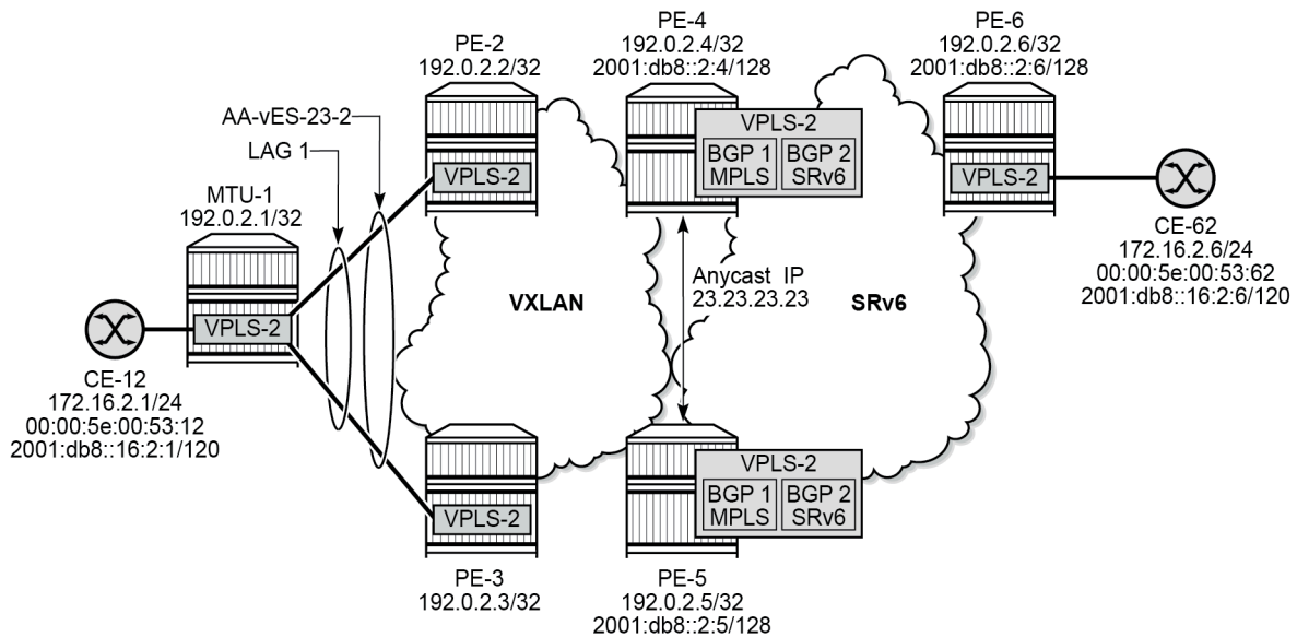
Figure 147: Example topology with VPLS-2
