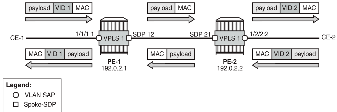
Figure 325: Customer VID is popped and pushed by VLAN SAPs - VLAN translation
