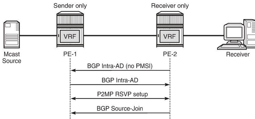
Figure 394: RSVP-Based BGP Message Flow Between PE-1 and PE-2
