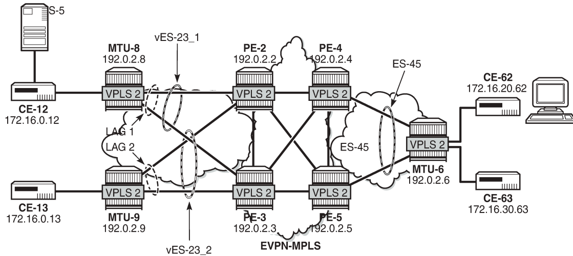
Figure 169: Example Topology with All-active ESs and Single-active ES
