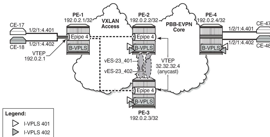
Figure 317: Example topology for static VXLAN termination using anycast
