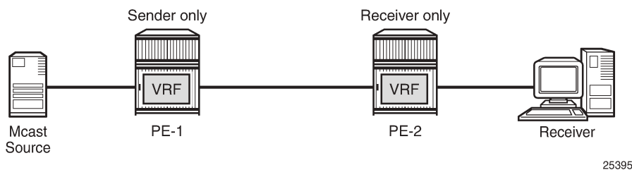
Figure 391: Default PMSI Hierarchy
