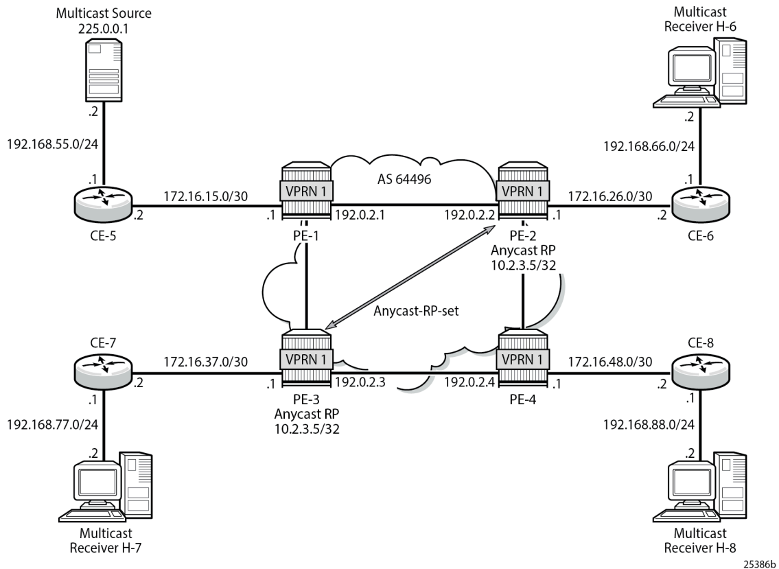
Figure 374: Example Topology for Anycast RP
