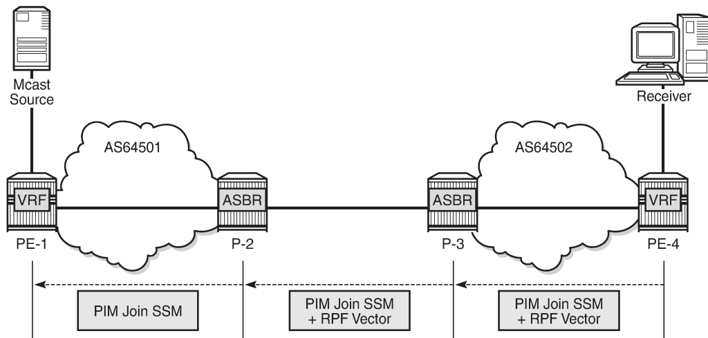
Figure 412: PIM-P Signaling Steps for Data MDT
