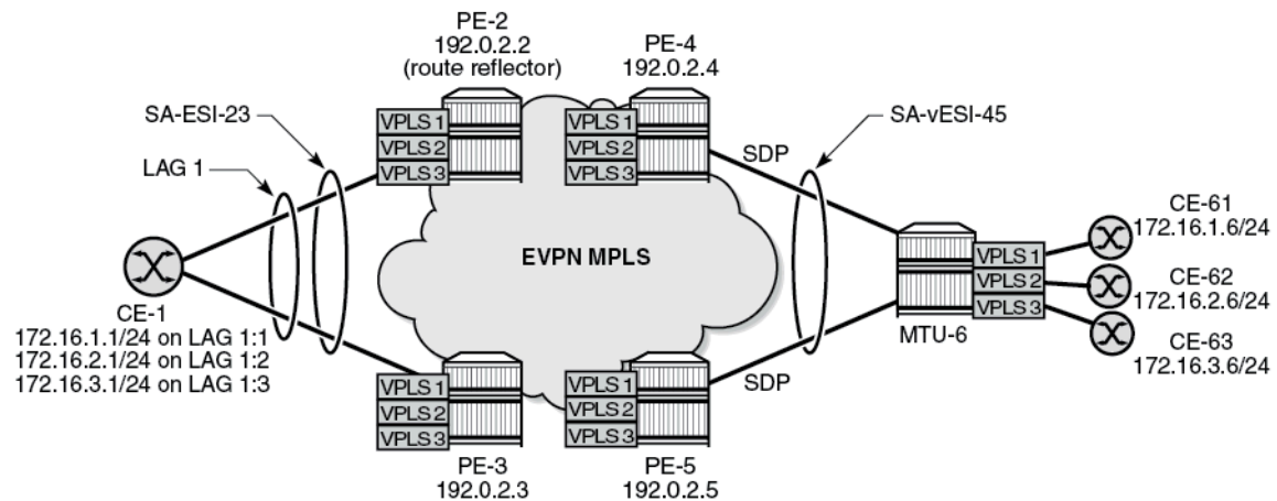
Figure 34: Example topology
