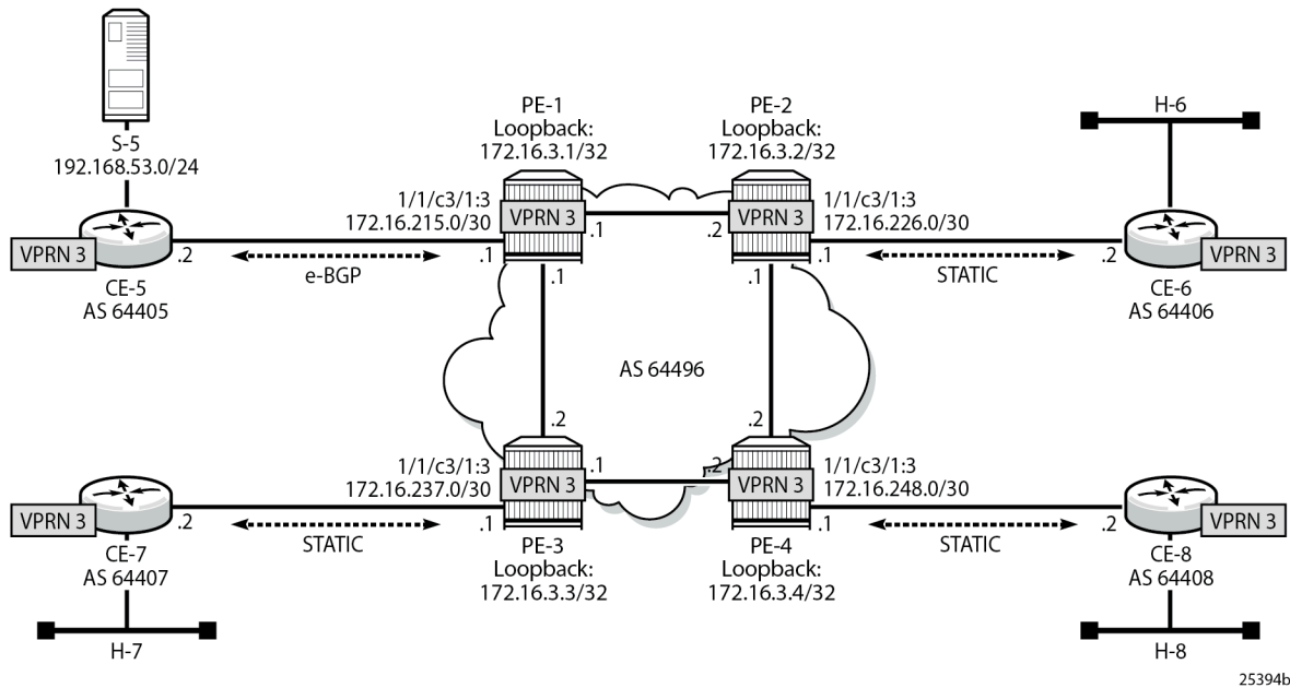
Figure 372: VPRN 3 Topology used for MDT SAFI
