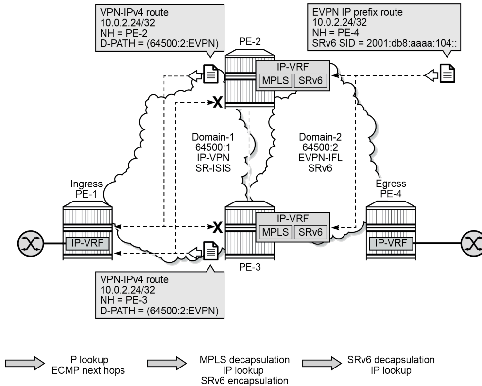
Figure 227: Interworking between EVPN-IFL and IP-VPN
