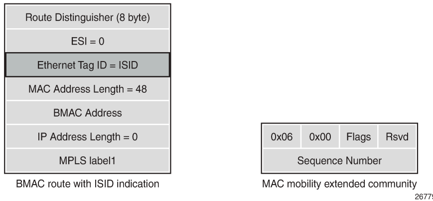
Figure 265: EVPN BMAC route with ISID indication
