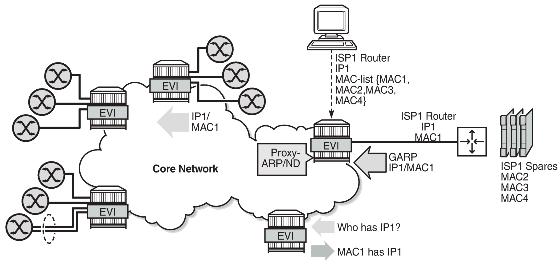
Figure 307: IXP with proxy-ARP/ND MAC list for dynamic entries
