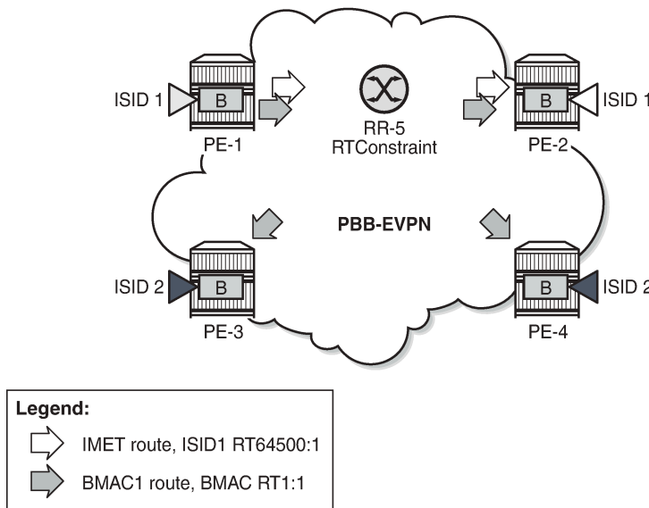
Figure 271: PBB-EVPN ISID-based RT
