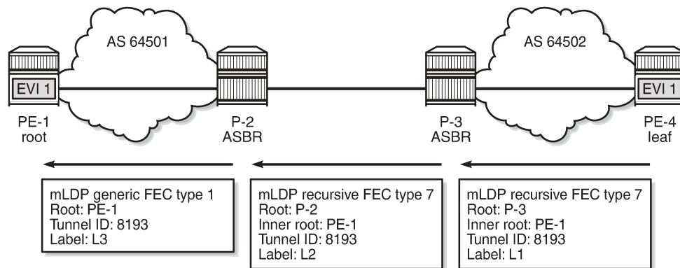
Figure 246: mLDP FEC label mapping messages for inter-AS model C
