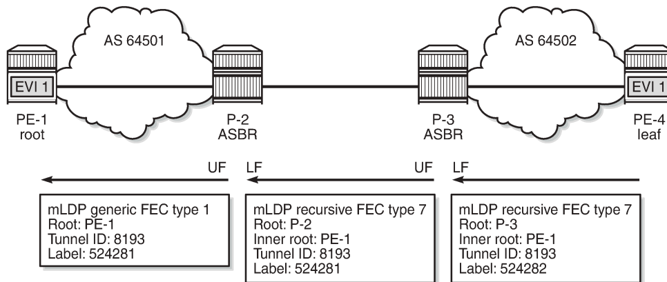
Figure 249: Recursive mLDP FEC for inter-AS model C
