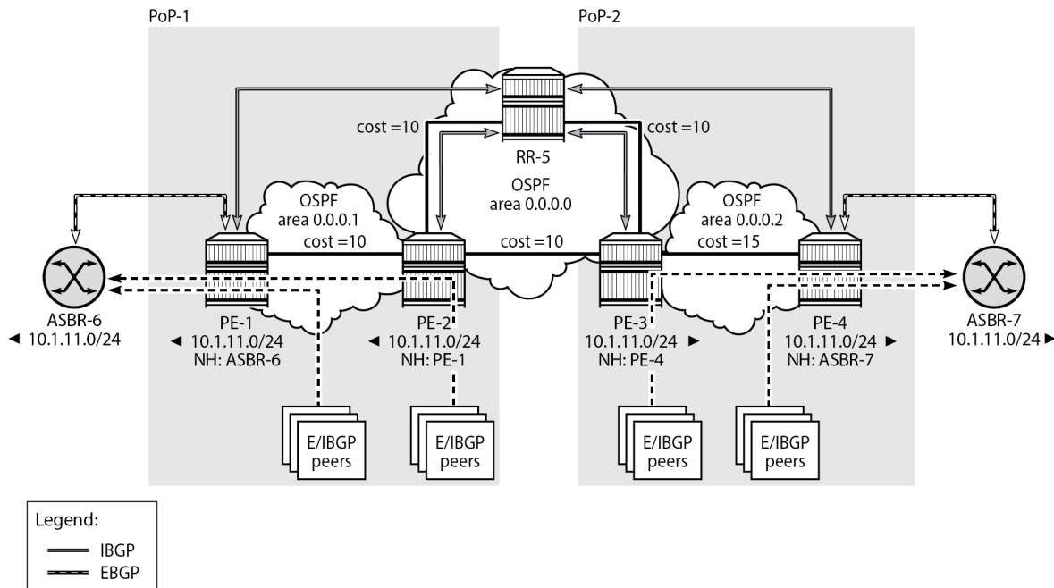
Figure 148: Optimal route reflection
