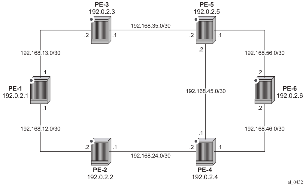
Figure 232: Example Topology
