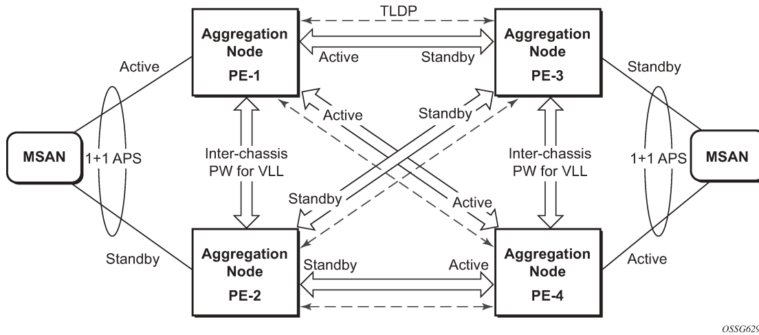
Figure 24: Access node and network resilience (part 2)
