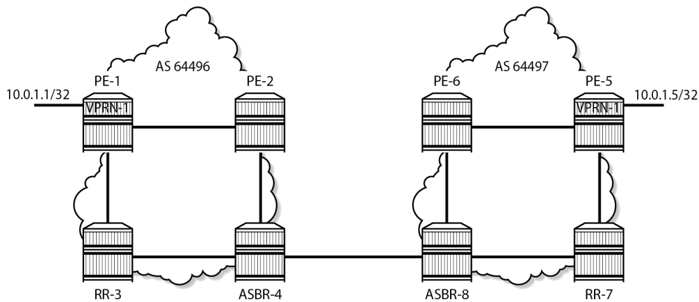
Figure 215: Example topology
