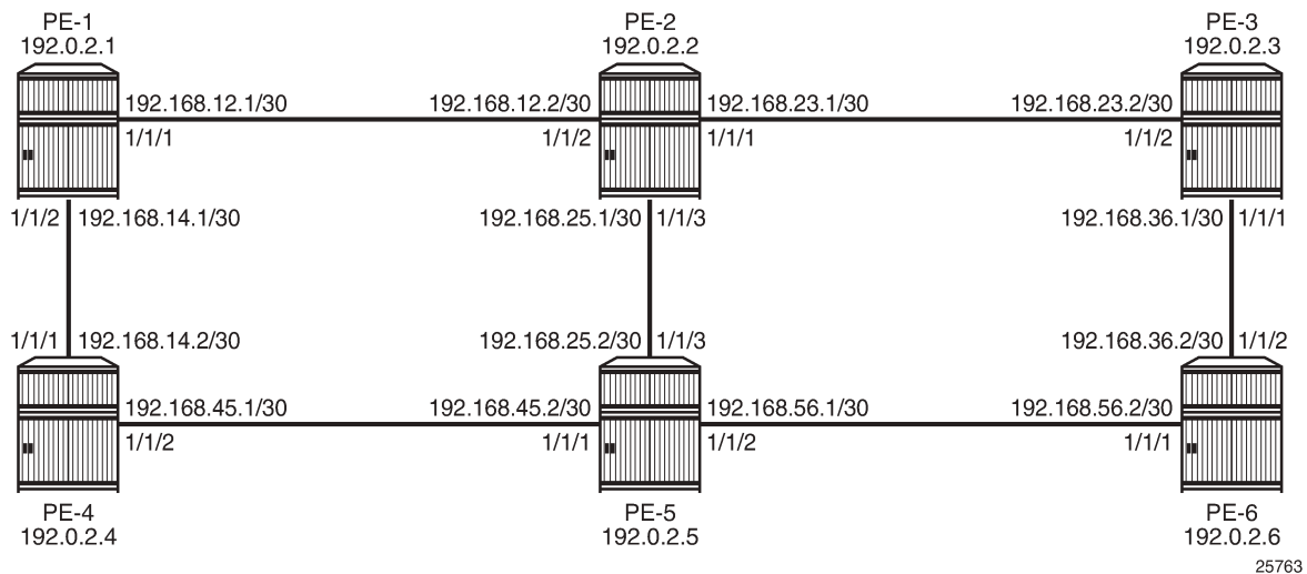
Figure 295: MPLS example topology
