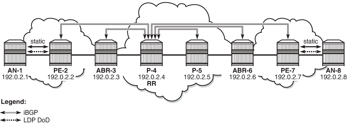
Figure 287: BGP enabled with P-4 as RR
