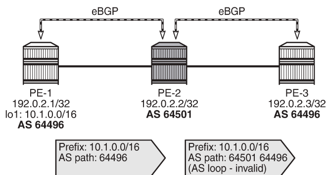
Figure 93: PE-2 detects AS-path loop and advertises the route to PE-3 as invalid
