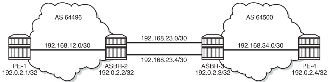
Figure 196: Example topology
