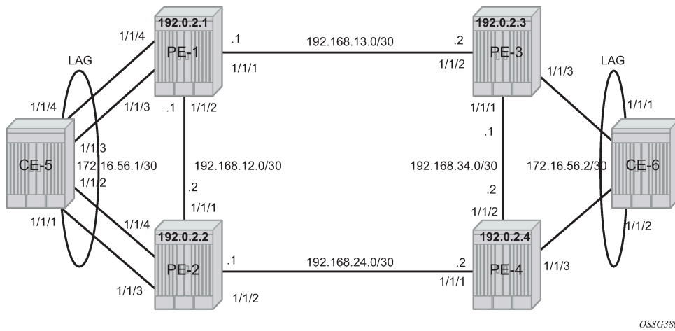
Figure 32: MC-LAG example topology
