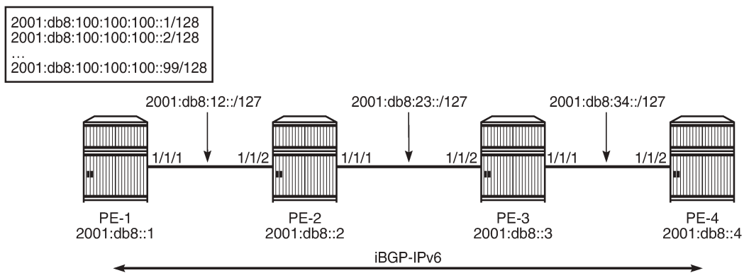
Figure 323: BGP-IPv6
