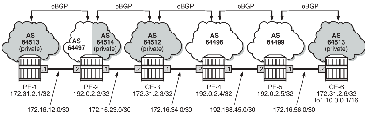
Figure 165: Use case 3 topology with private ASN 64513 on CE-1 and CE-6
