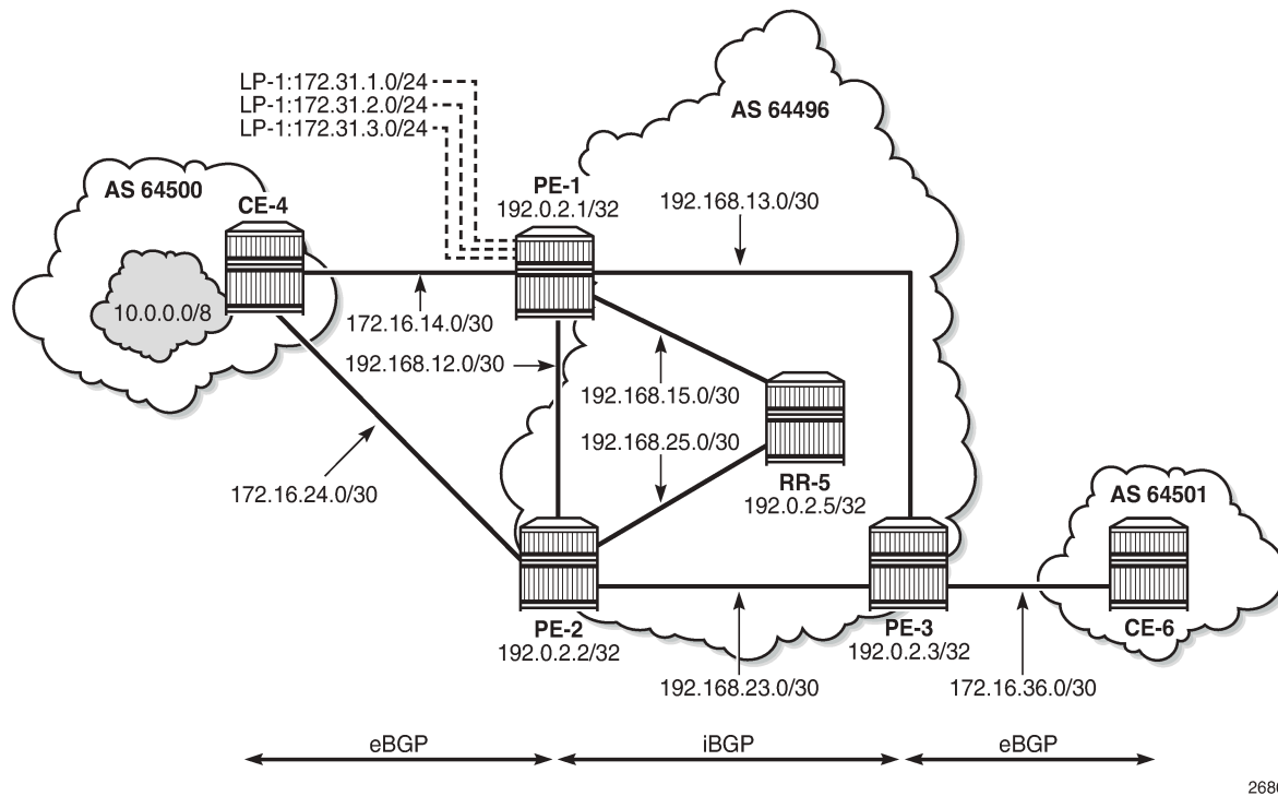
Figure 103: Example Topology
