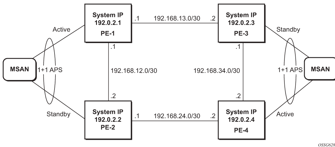
Figure 22: MC-APS network topology
