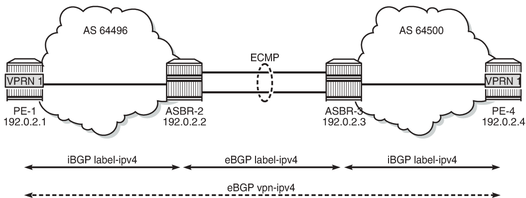
Figure 197: BGP peering
