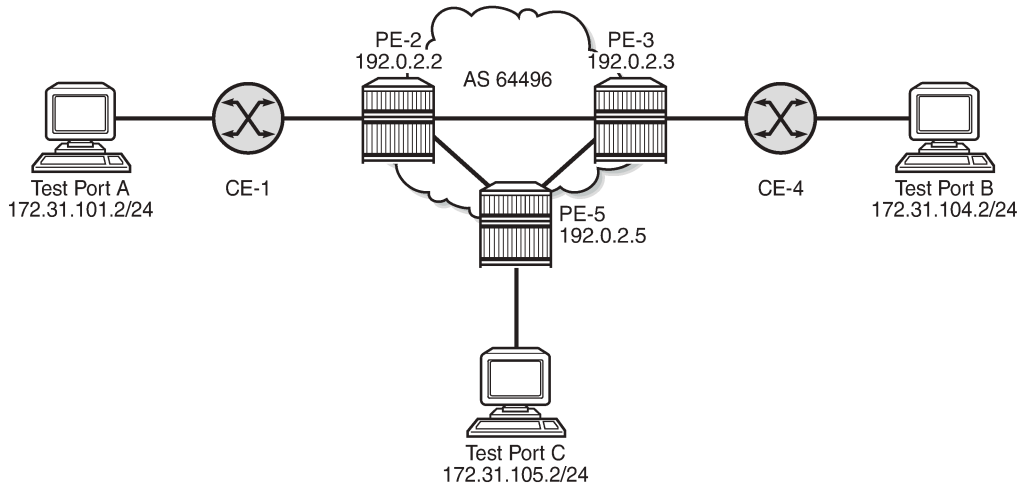
Figure 38: Example topology
