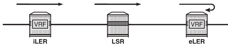
Figure 381: Tunneling of ICMP reply packets over an MPLS LSP
