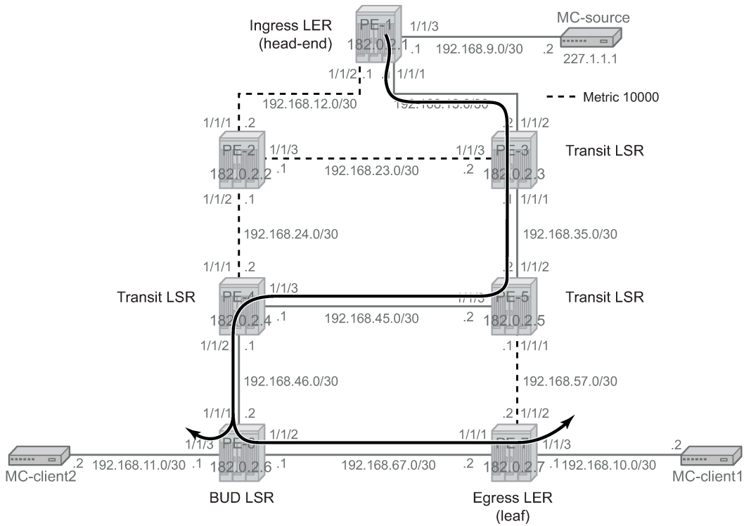
Figure 348: P2MP LSP p-to-mp-1 with Metric Change
