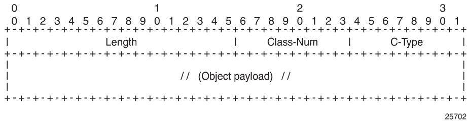
Figure 384: ICMP extension object: object header and payload
