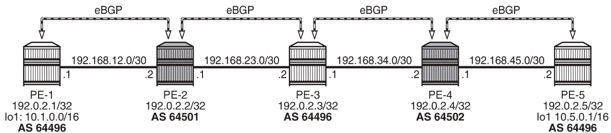
Figure 95: Example topology
