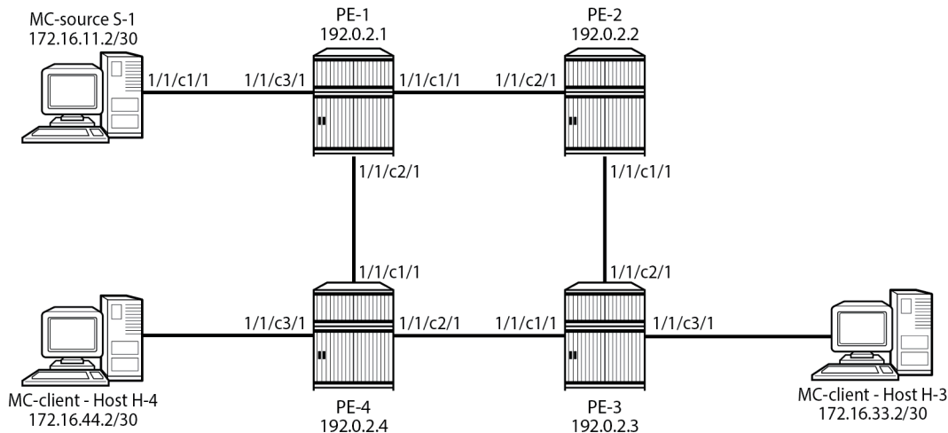
Figure 311: Example topology
