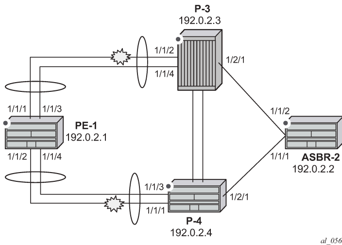
Figure 208: Second link failure
