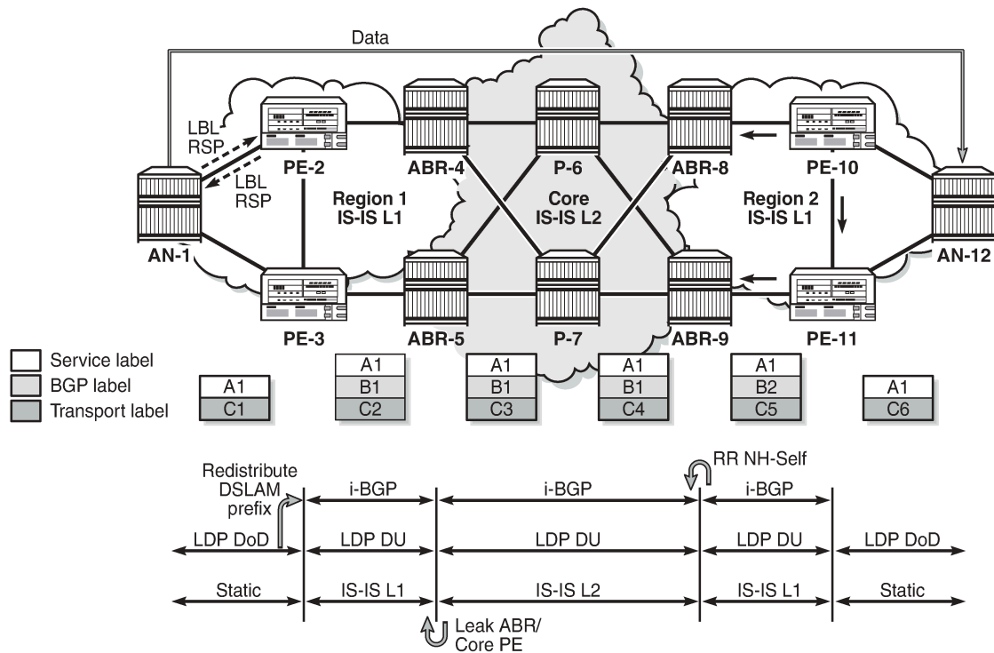
Figure 285: LDP FEC to BGP label route stitching
