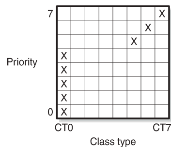
Figure 251: Mapping of TE classes
