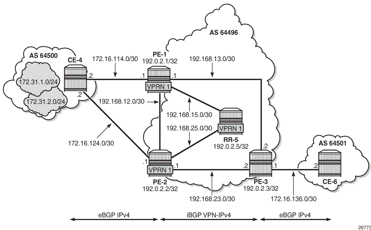
Figure 117: Example topology - VPN-IPv4
