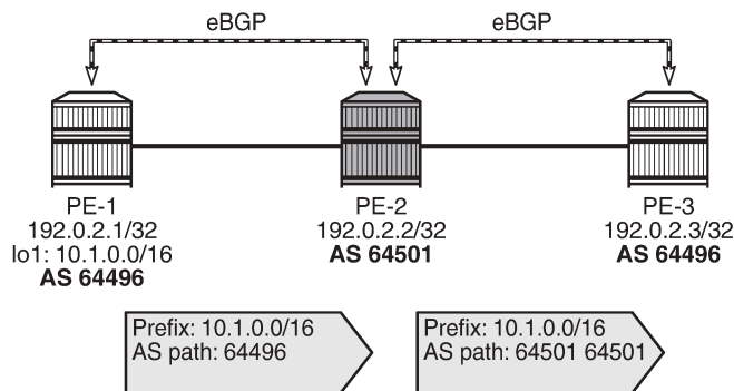
Figure 94: BGP AS override replaces the peer ASN in the AS-path with the local ASN
