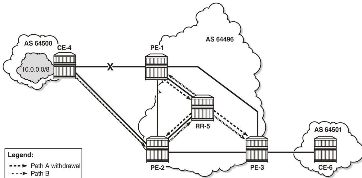
Figure 84: Reconvergence after path failure (without add-path)
