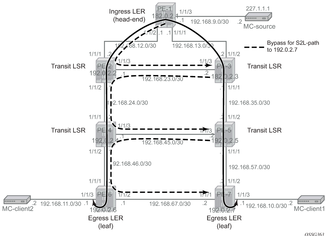
Figure 347: P2MP LSP LSP-p2mp-1 with Bypass Tunnels
