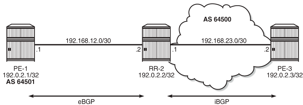
Figure 216: Example topology
