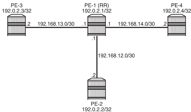
Figure 221: Example IPv4 topology
