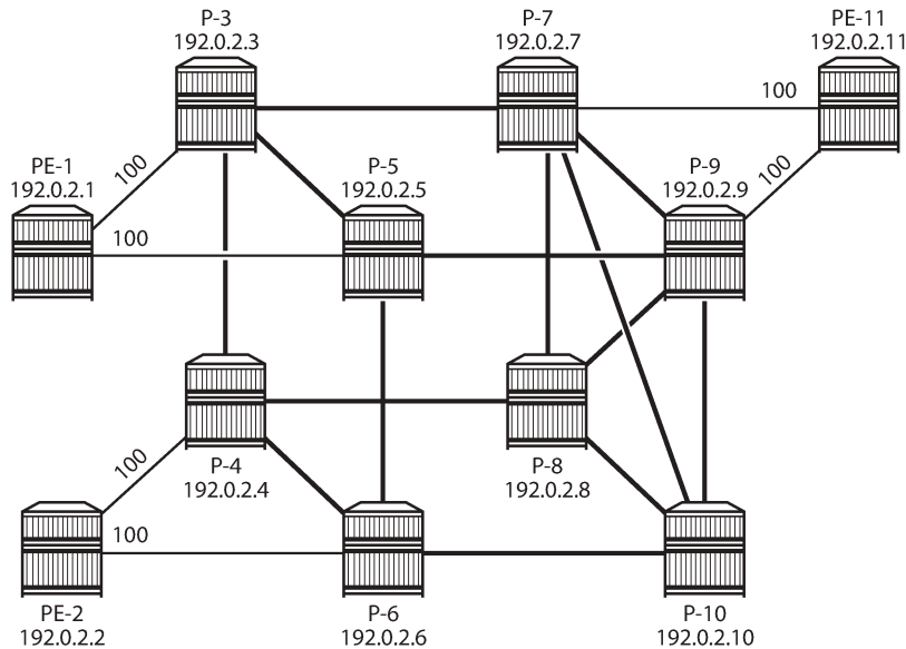
Figure 449: Example topology
