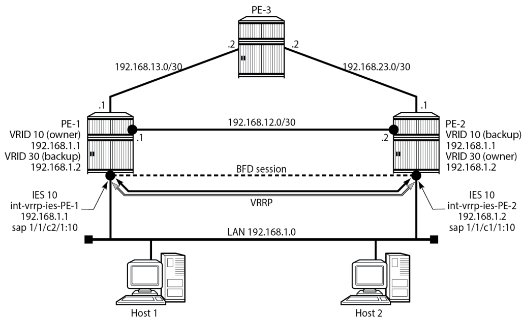
Figure 62: BFD for VRRP
