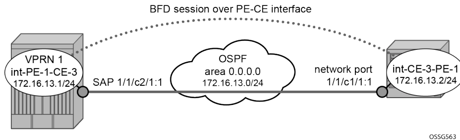
Figure 61: BFD for OSPF PE-CE interfaces
