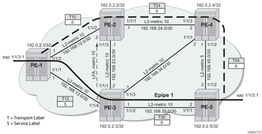
Figure 302: Data verification in the direction from PE-1 to PE-5 using Epipe service
