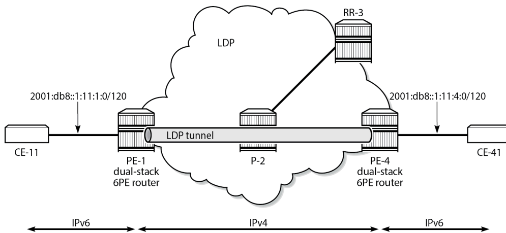
Figure 44: 6PE next hop resolved to an LDP tunnel
