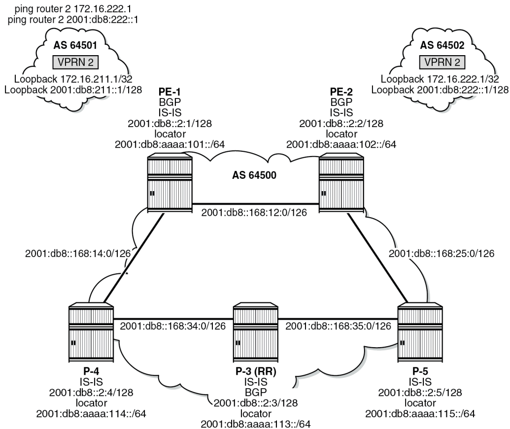
Figure 456: Example topology
