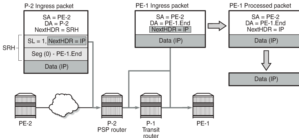
Figure 441: Penultimate SRH hop P-2 processes and removes the SRH
