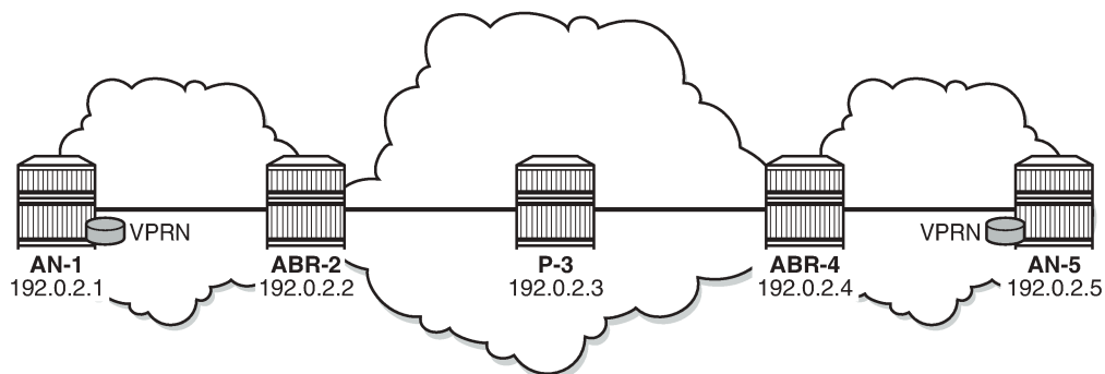
Figure 357: L3 VPN service
