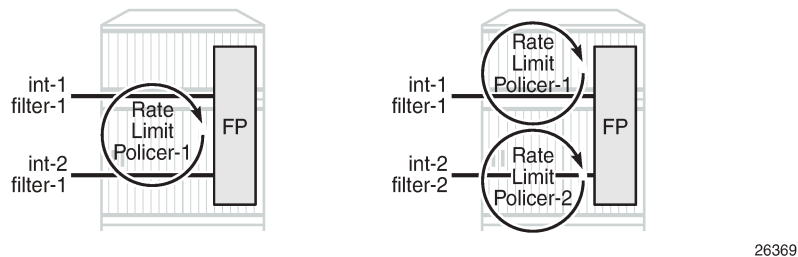
Figure 72: Rate Limit Filters and FlexPaths
