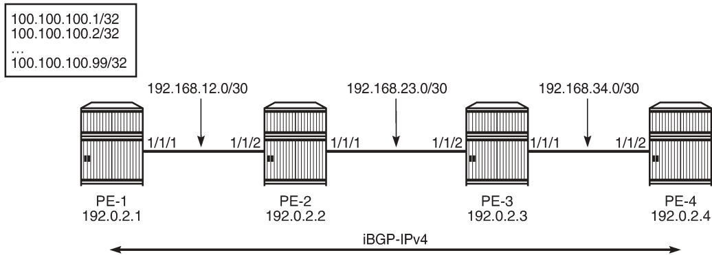
Figure 322: BGP-IPv4
