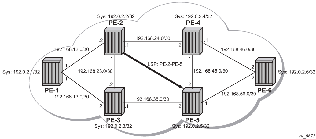
Figure 276: RSVP Shortcuts LFA Use Case Example
