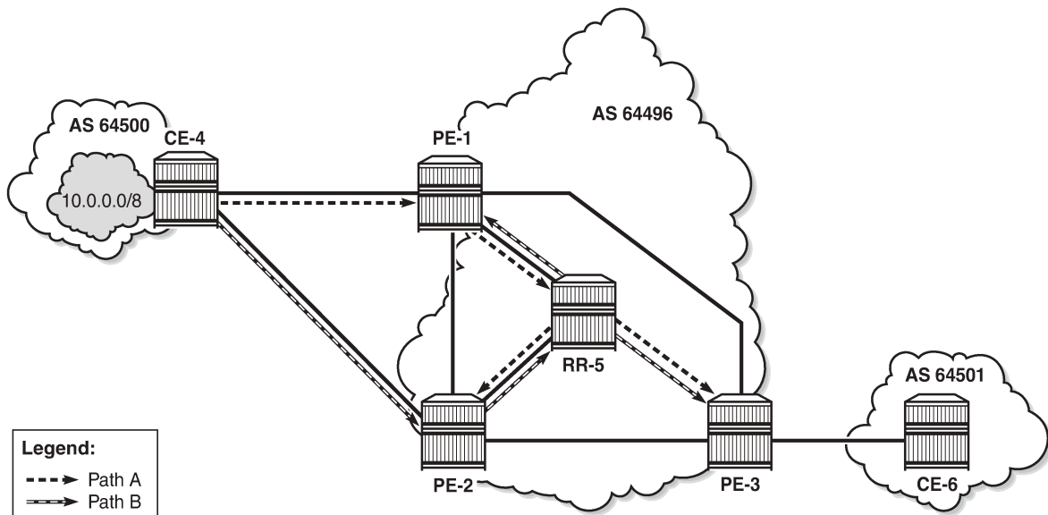
Figure 85: Advertised paths when BGP add-path is enabled in PEs and RR
