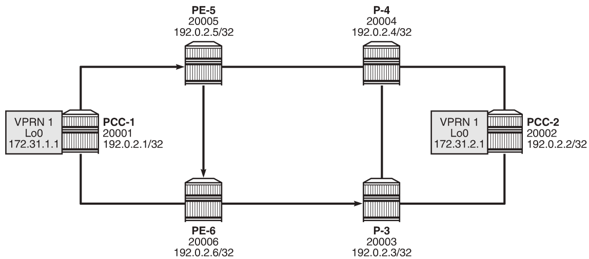
Figure 429: VPRN service schematic
