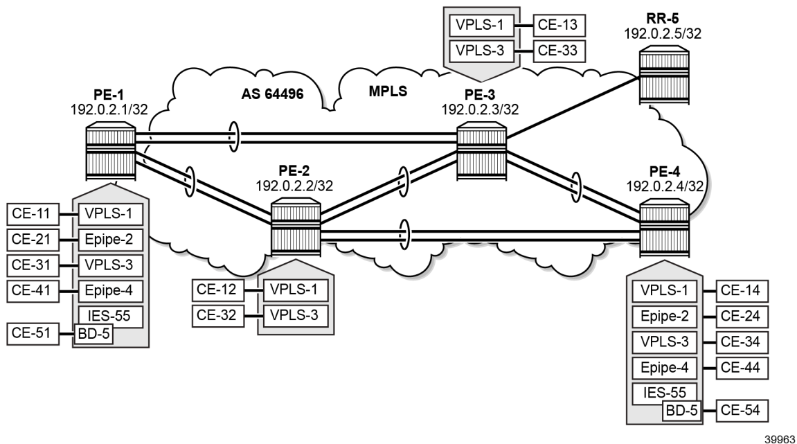
Figure 174: Example topology
