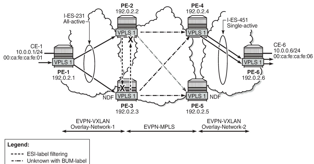
Figure 95: All-active multi-homing and send-imet-ir-on-ndf
