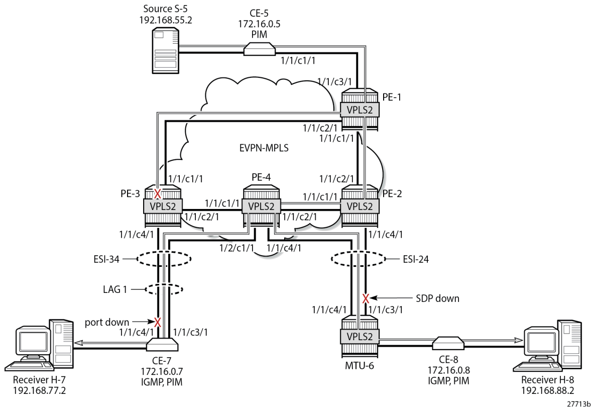
Figure 299: EVPN-MPLS with Multi-homing and PIM Snooping - Multicast Flow after Failover
