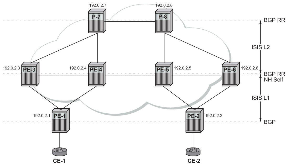
Figure 231: Intra-AS MS-PW example topology
