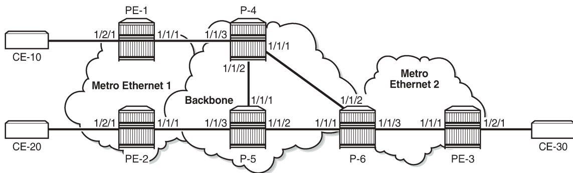
Figure 195: Example topology
