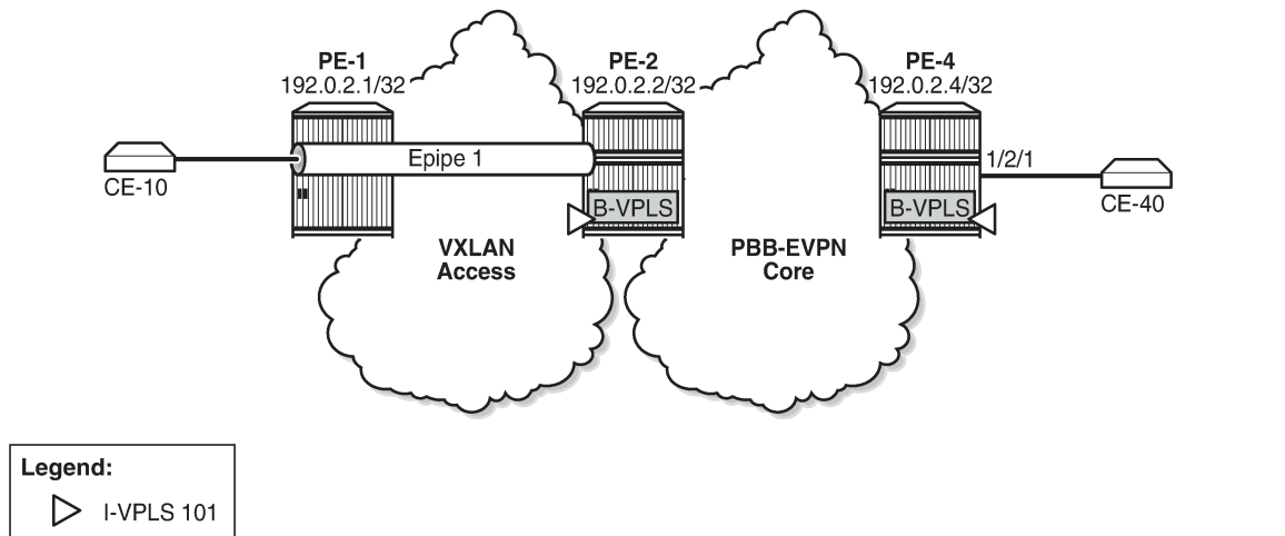
Figure 319: Static VXLAN termination on system IP addresses
