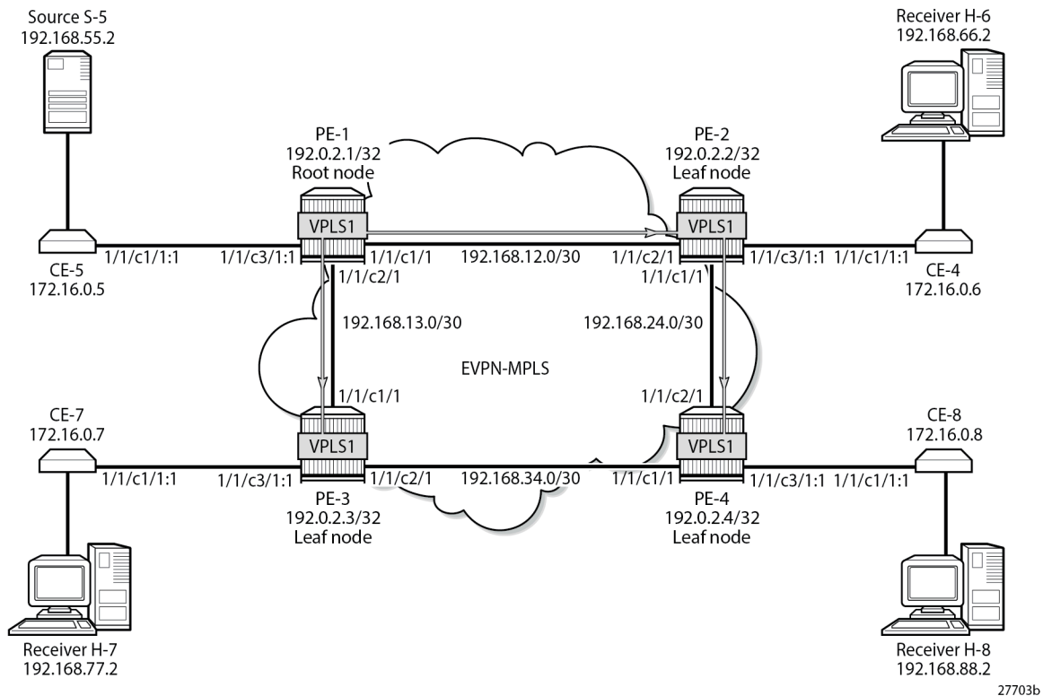
Figure 289: P2MP mLDP Multicast Tree
