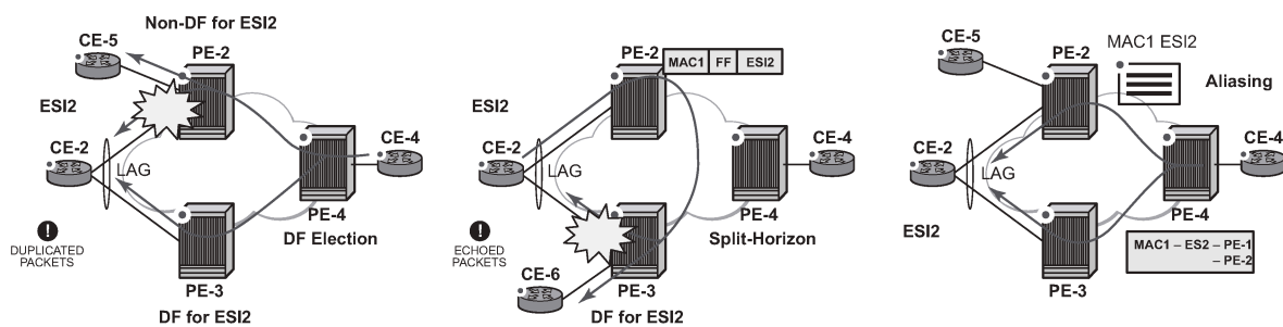
Figure 64: EVPN-MPLS all-active multi-homing concepts
