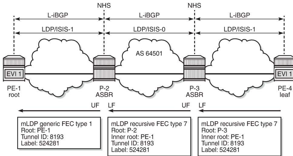
Figure 257: Recursive mLDP FEC for seamless MPLS
