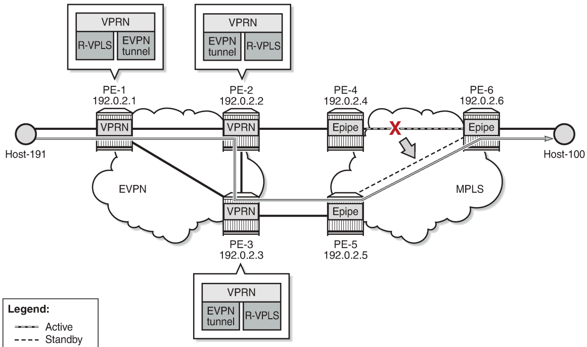
Figure 199: Hairpinning in a broadcast domain after switchover for SR OS Releases earlier than Release 19.10.R3
