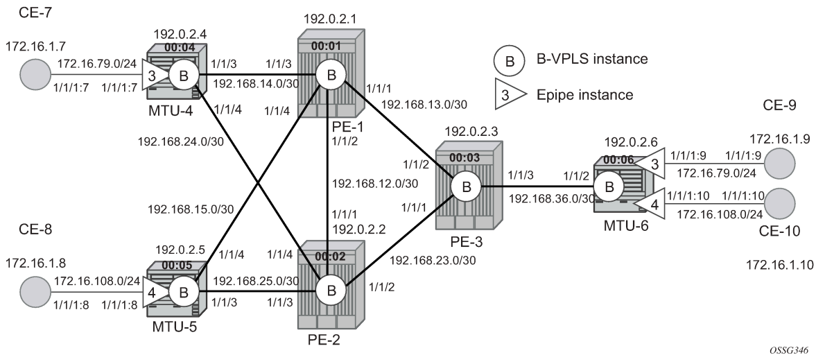
Figure 267: Setup detailed view
