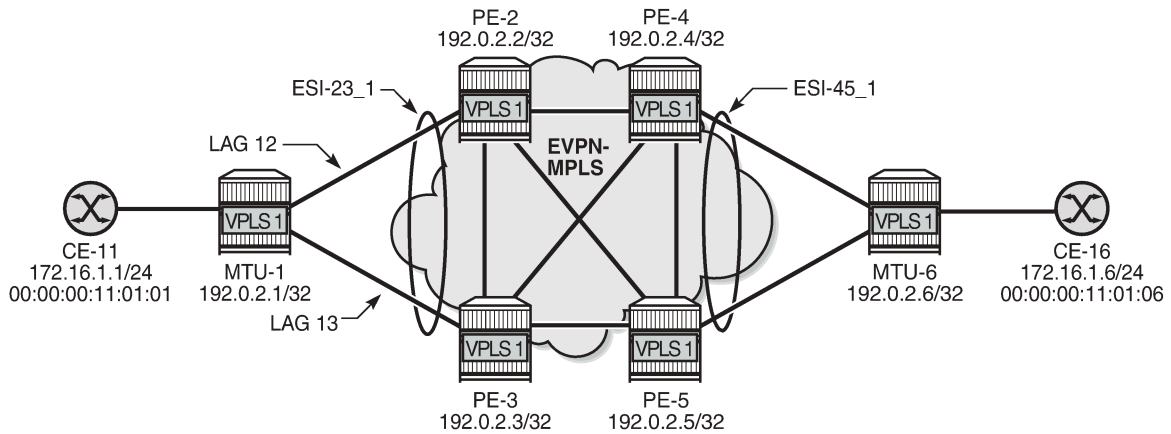
Figure 246: Sample topology with VPLS 1
