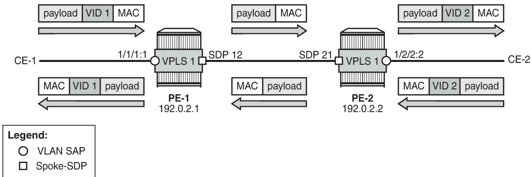
Figure 331: Customer VID is popped and pushed by VLAN SAPs - VLAN translation
