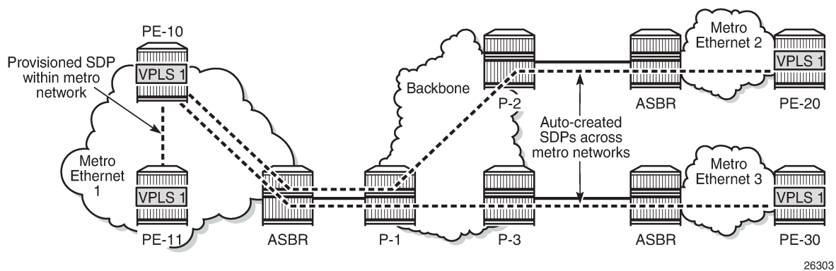
Figure 194: LDP VPLS using BGP-AD with prefer-provisioned-sdp option
