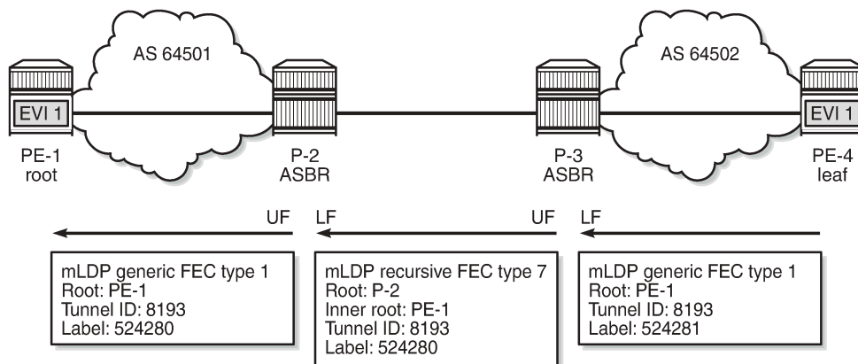
Figure 255: Non-recursive mLDP FEC for inter-AS model C
