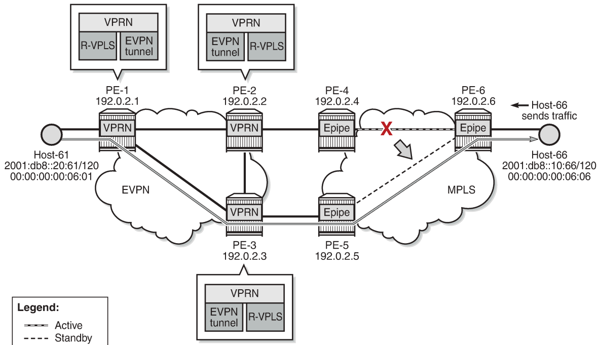
Figure 208: Host generates non-ND traffic after switchover
