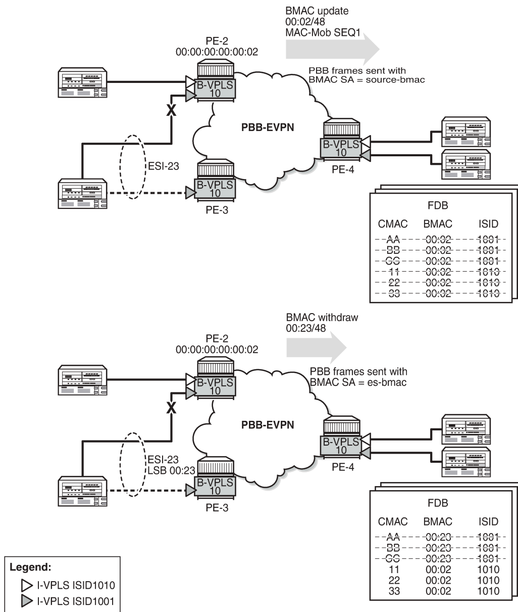
Figure 271: ISID-independent CMAC flush when ES fails
