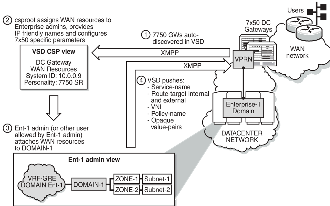
Figure 176: DC Gateway fully dynamic provisioning workflow
