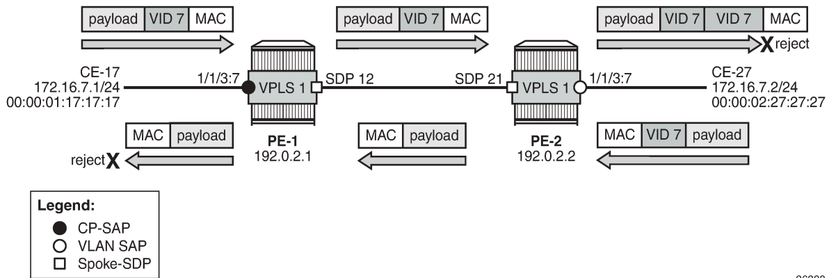
Figure 338: No traffic between dot1q CP SAP and dot1q VLAN SAP
