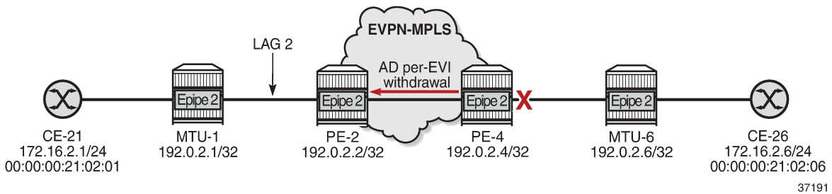
Figure 249: LLF in Epipe 2 - PE-4 failure
