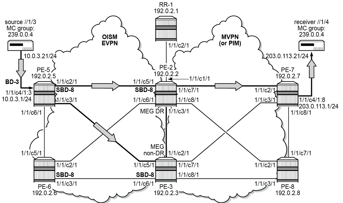
Figure 236: EVPN MC source - MVPN/PIM MC receiver example setup, with DR as UMH for PE-7
