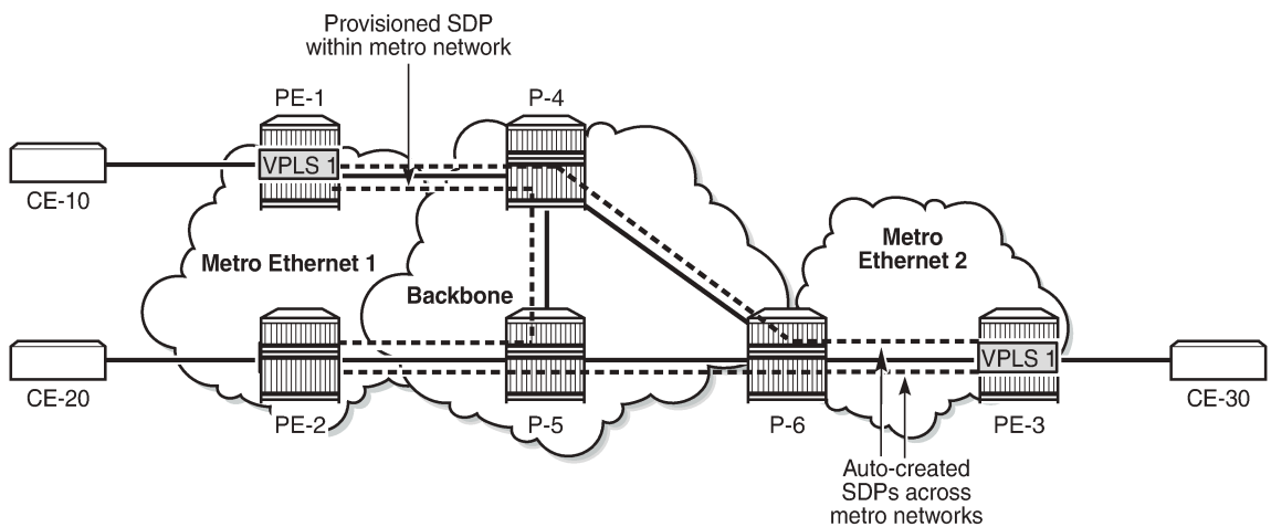
Figure 198: SDP bindings in VPLS 1 with prefer-provisioned-sdp option
