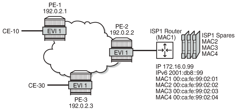
Figure 313: Example topology
