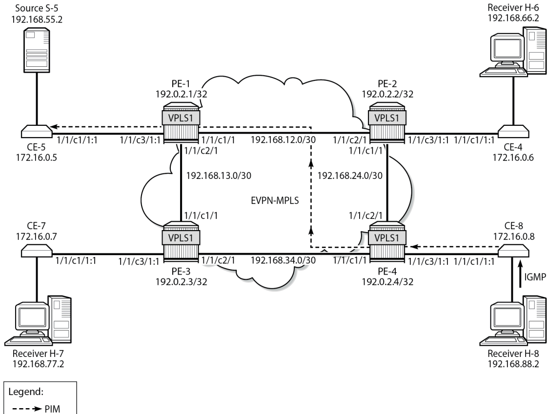
Figure 290: H-8 Joins Group (192.168.55.2, 232.1.1.1) and PIM Snooping is Disabled
