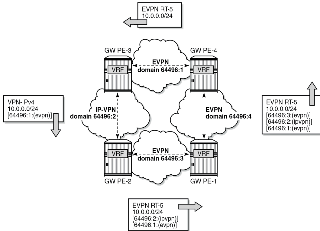
Figure 45: Loop prevention in networks with multiple IP-VPN and EVPN domains
