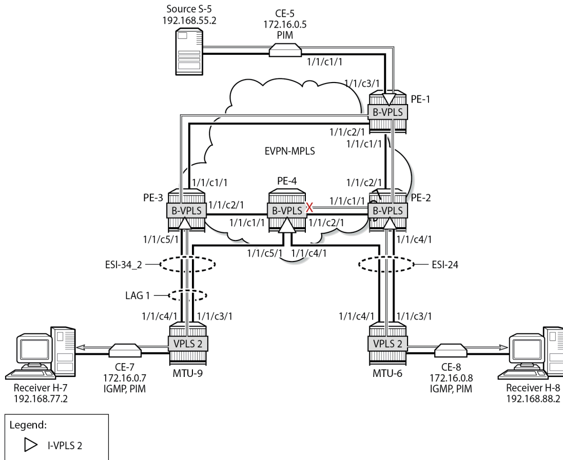
Figure 305: EVPN-MPLS with MH and PIM Snooping – Receivers H-7 and H-8 Joined
