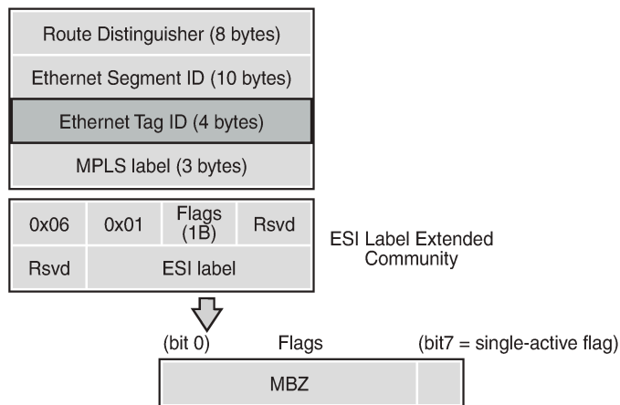
Figure 163: BGP-EVPN AD per-ES route
