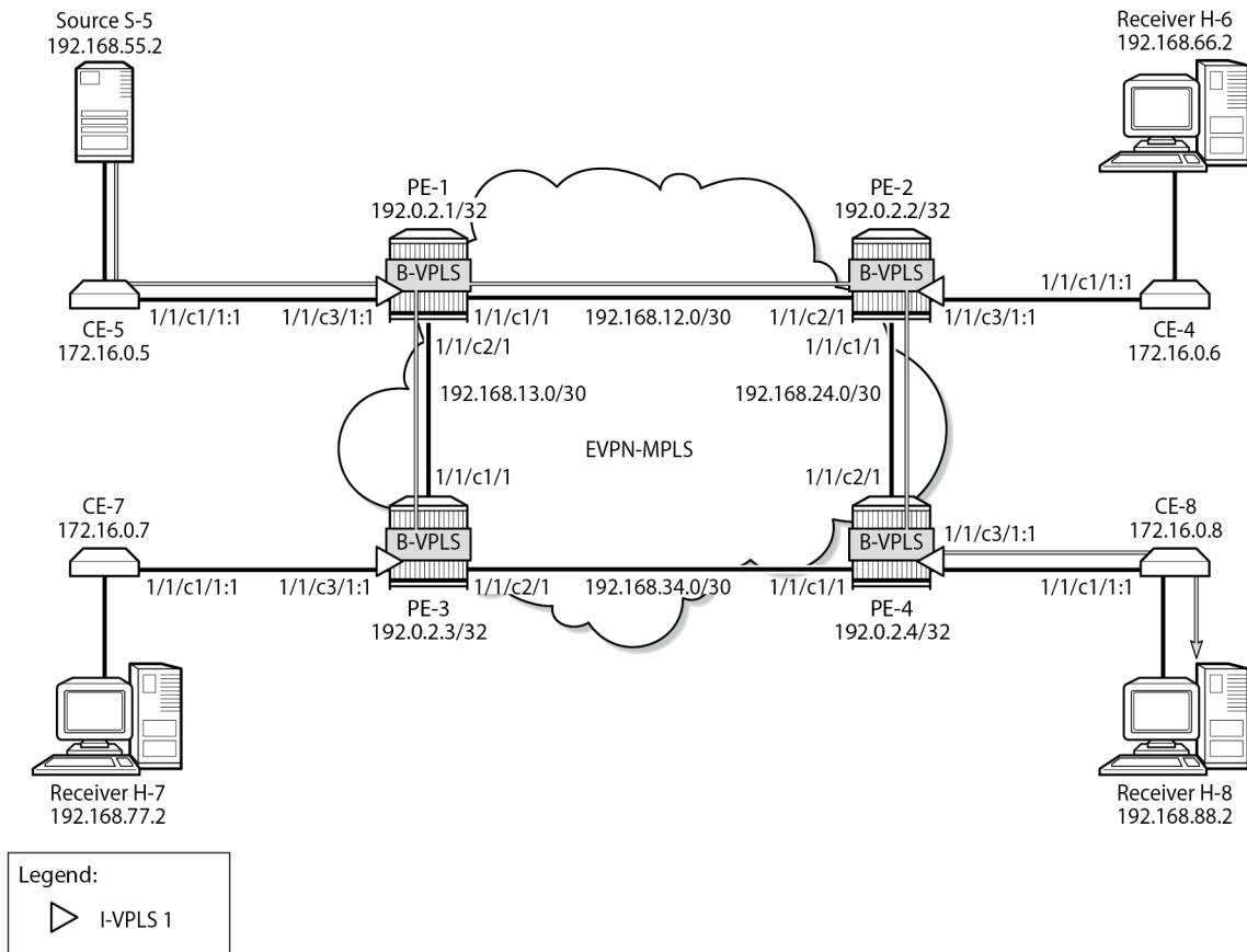
Figure 302: Multicast Stream to Receiver H-8 with PIM Snooping Enabled
