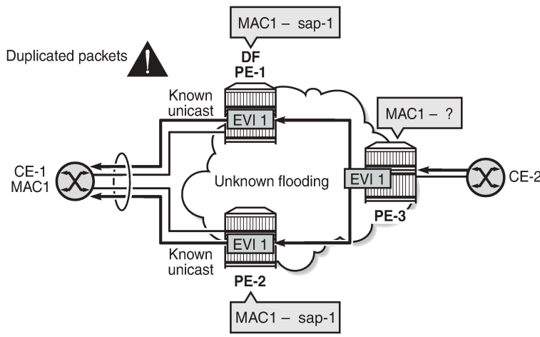
Figure 115: Duplicate unicast packets when MAC1 is unknown on PE-3 only
