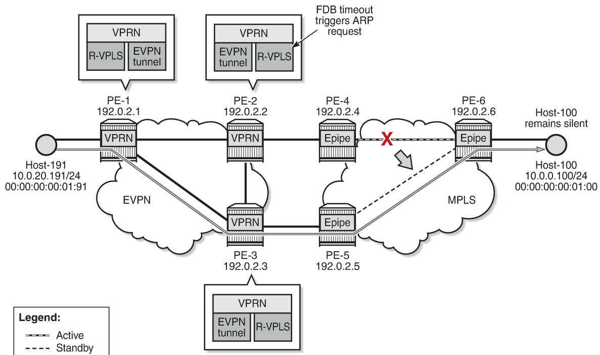
Figure 205: Host does not send any traffic after switchover
