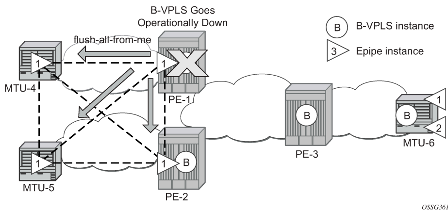
Figure 282: Send flush on B-VPLS failure example
