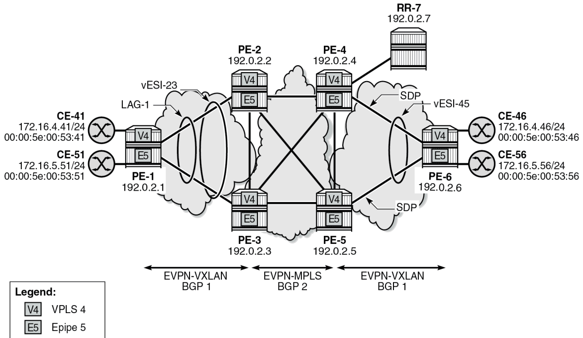
Figure 326: Example topology with VPLS 4 and Epipe 5
