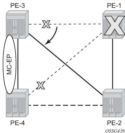
Figure 215: Core node failure
