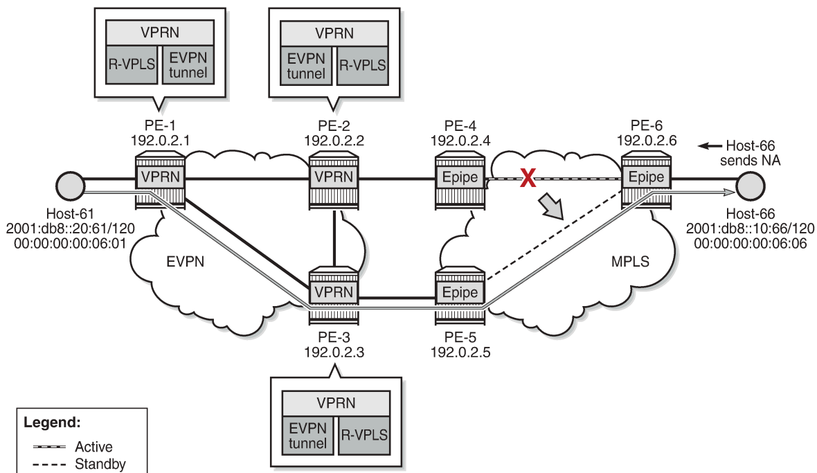
Figure 207: Host-66 sends unsolicited NA message after switchover
