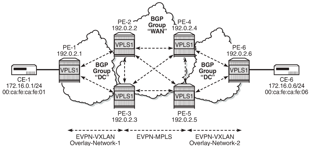
Figure 159: EVPN-MPLS interconnect for EVPN-VXLAN - example topology
