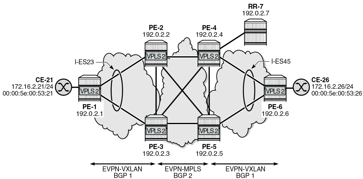
Figure 325: Example topology with dual-instance VPLS
