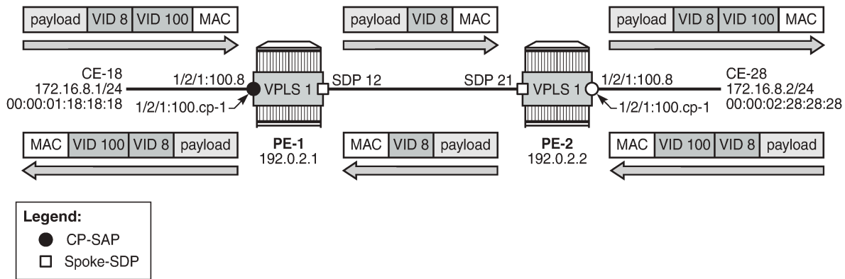
Figure 341: Traffic between two QinQ CP SAPs - no VLAN translation
