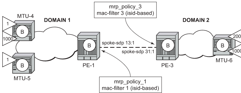
Figure 283: Inter-domain B-VPLS and MMRP policies/ISID-based filters example
