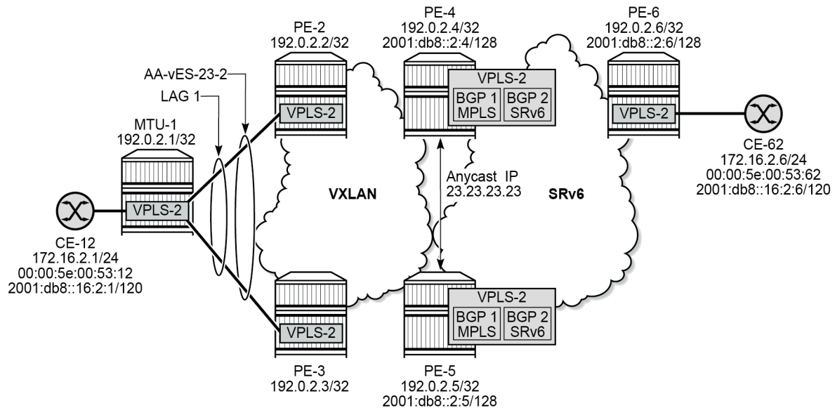
Figure 136: Example topology with VPLS-2
