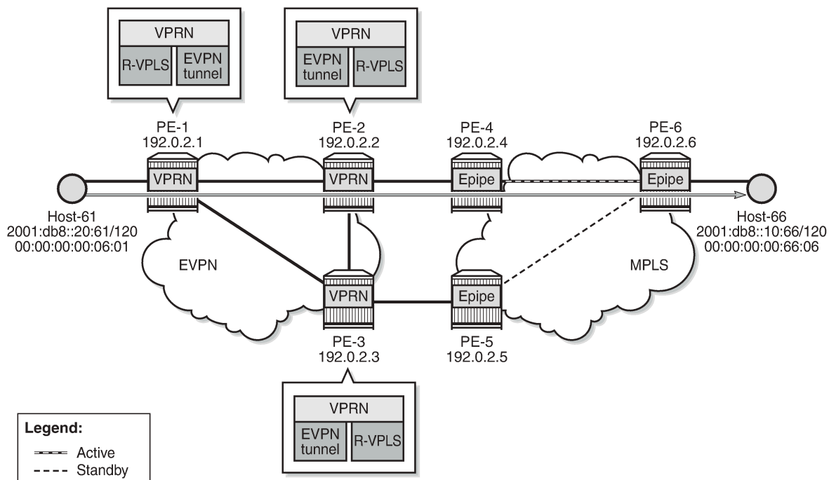
Figure 206: Example topology for initial forwarding path via PE-2 with IPv6 addresses
