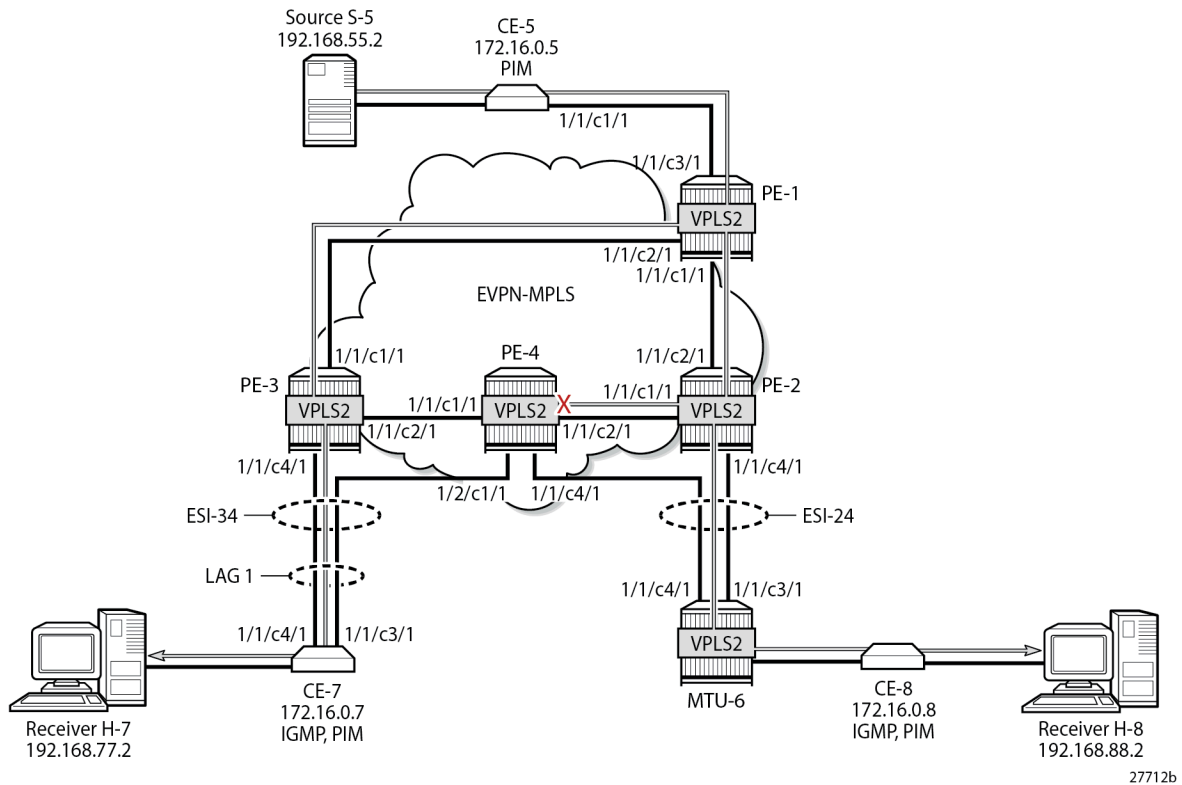
Figure 298: EVPN-MPLS with Multi-homing and PIM Snooping - Receivers H-7 and H-8 Joined
