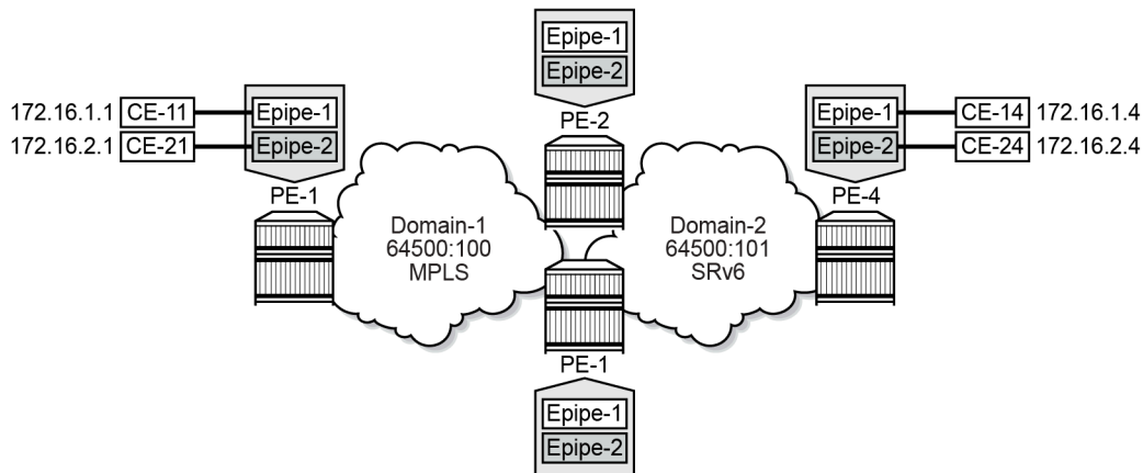
Figure 219: Example topology
