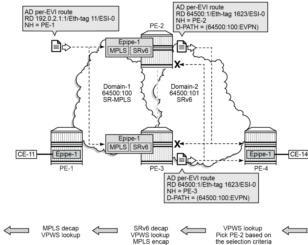
Figure 221: AD per-EVI route from MPLS domain redistributed into SRv6 domain
