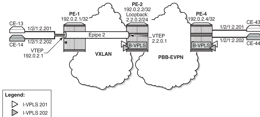
Figure 321: Example topology for static VXLAN termination on non-system IPv4 addresses
