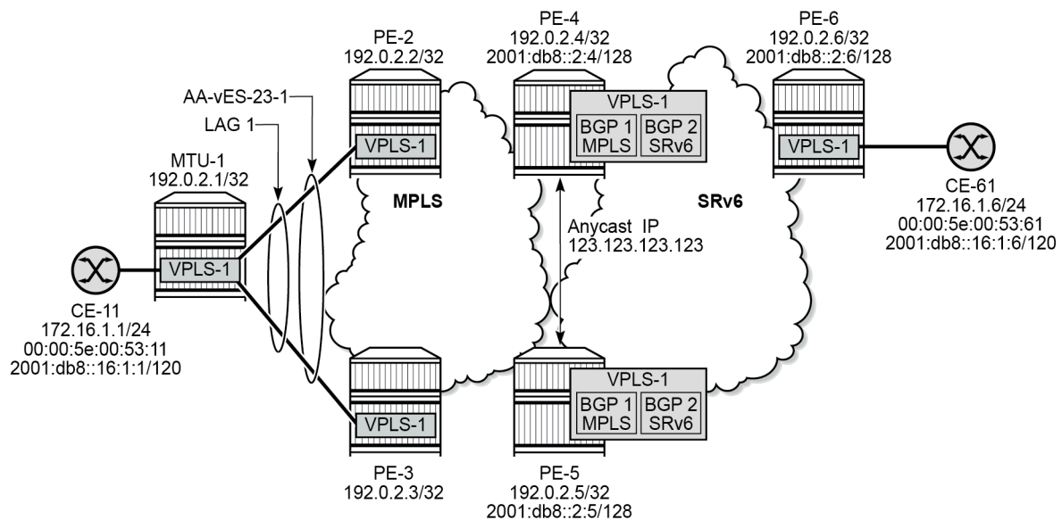
Figure 135: Example topology with VPLS-1
