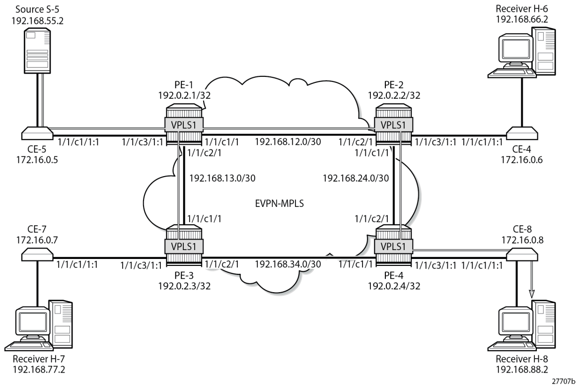
Figure 293: Multicast Stream (192.168.55.2, 232.1.1.1) with PIM Snooping Enabled
