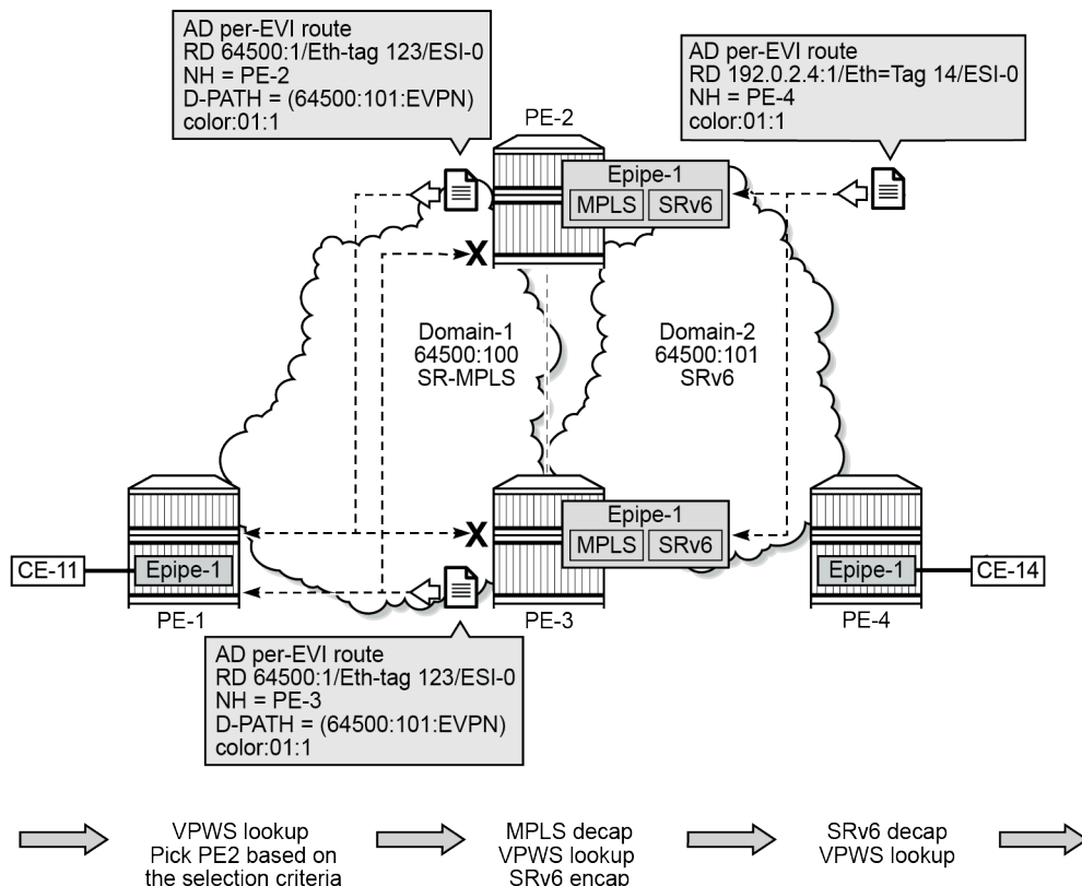
Figure 222: Redistributing AD per-EVI routes from the SRv6 domain into the MPLS domain with attribute propagation
