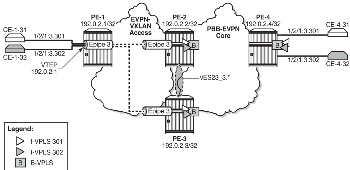
Figure 244: Epipe 3 with EVPN-VXLAN and SA MH ES
