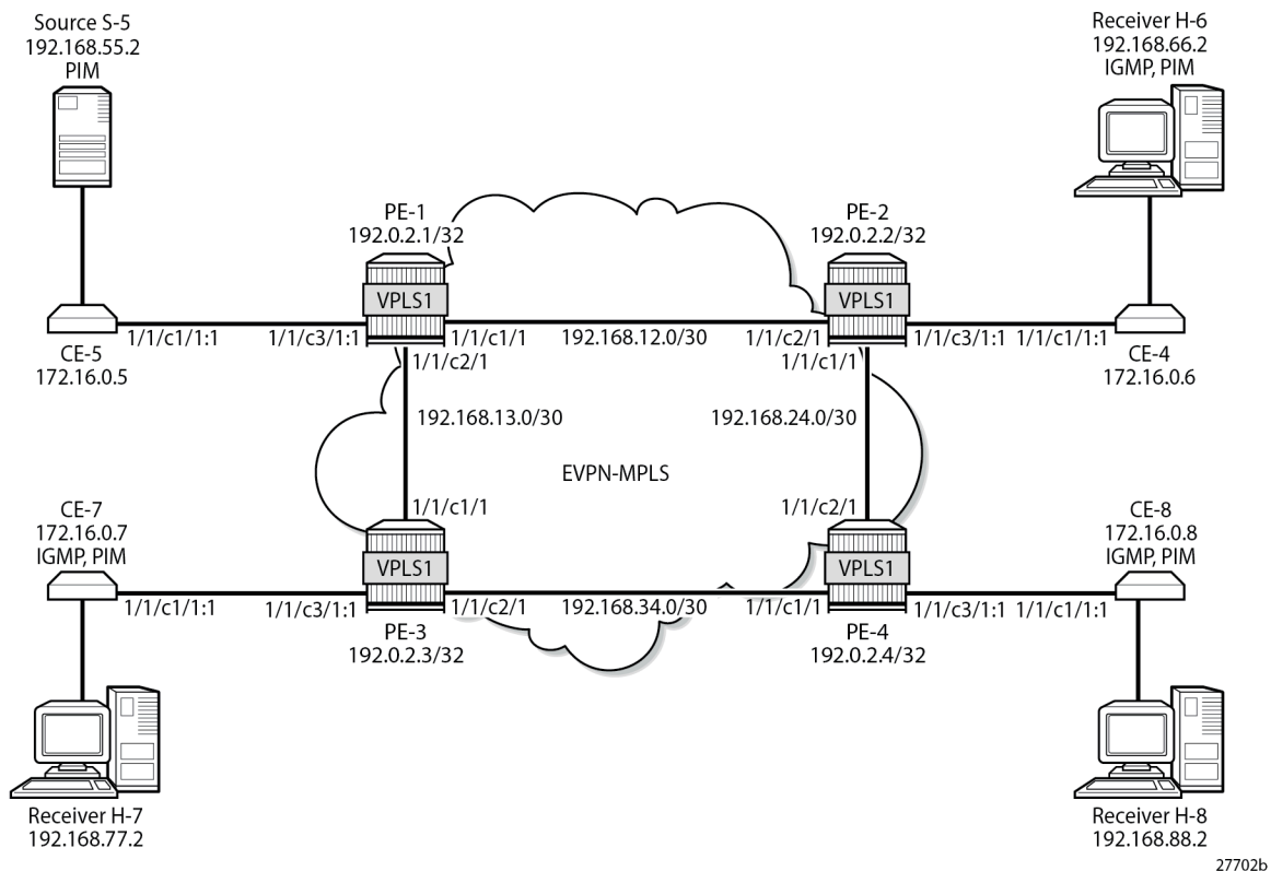
Figure 288: Example Topology
