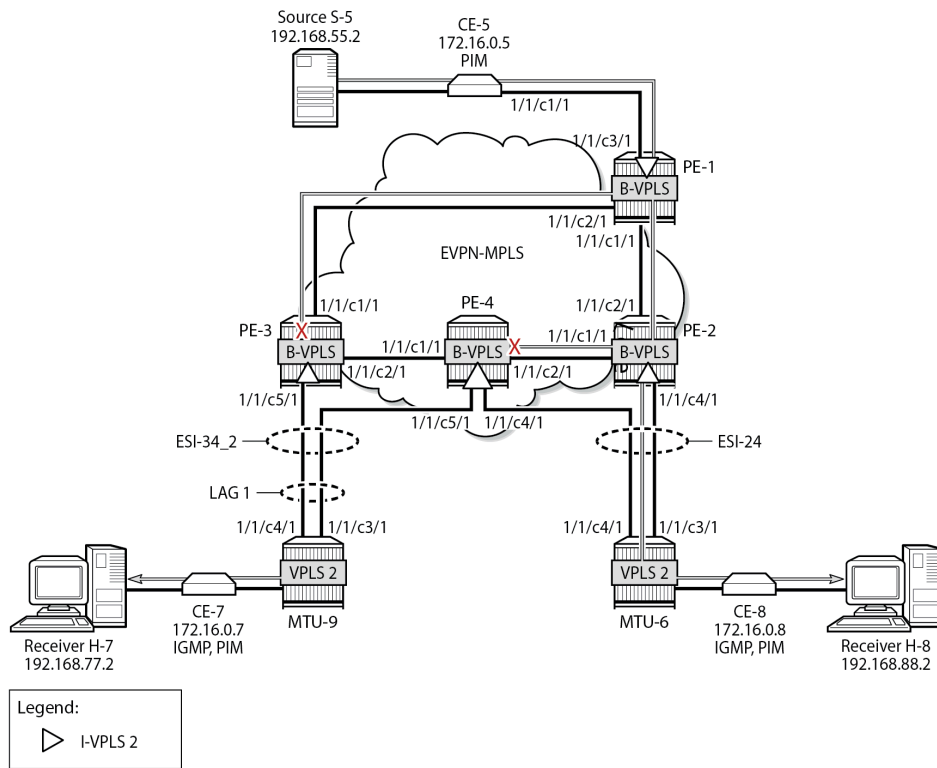
Figure 306: PBB-EVPN with MH and PIM Snooping – Receiver H-8 Joined
