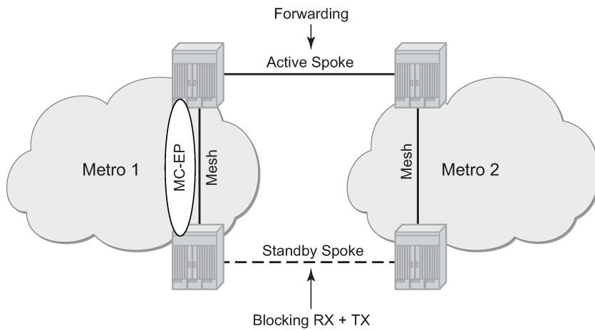
Figure 213: Multi-chassis endpoint with square resiliency
