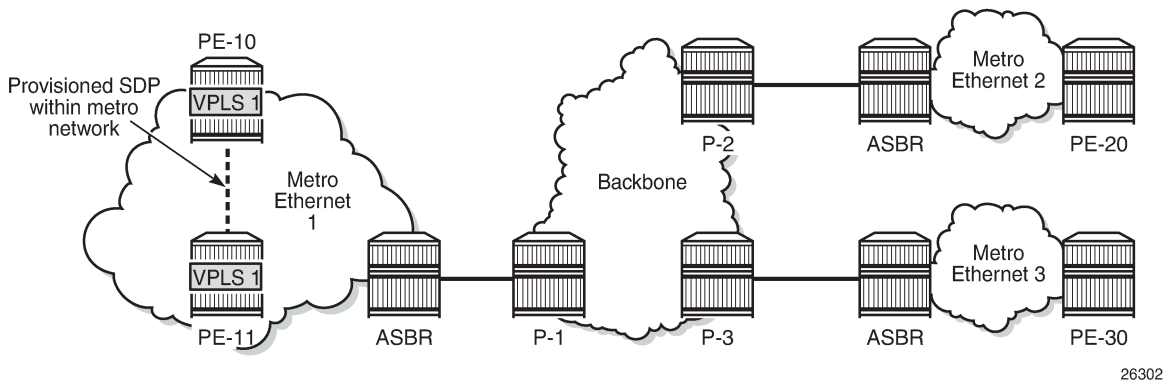
Figure 193: LDP VPLS using BGP-AD with use-provisioned-sdp option
