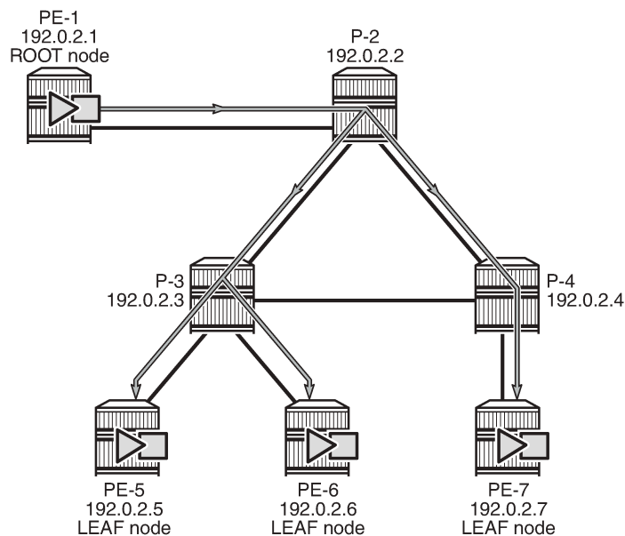
Figure 265: P2MP mLDP in PBB-EVPN
