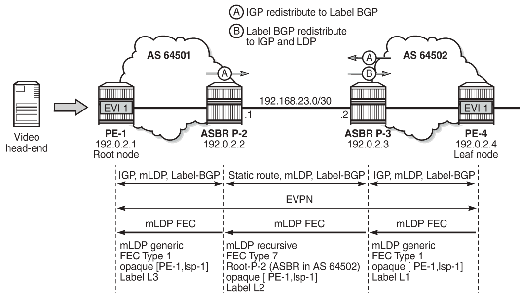
Figure 261: Example topology for optimized Inter-AS Model C for mLDP
