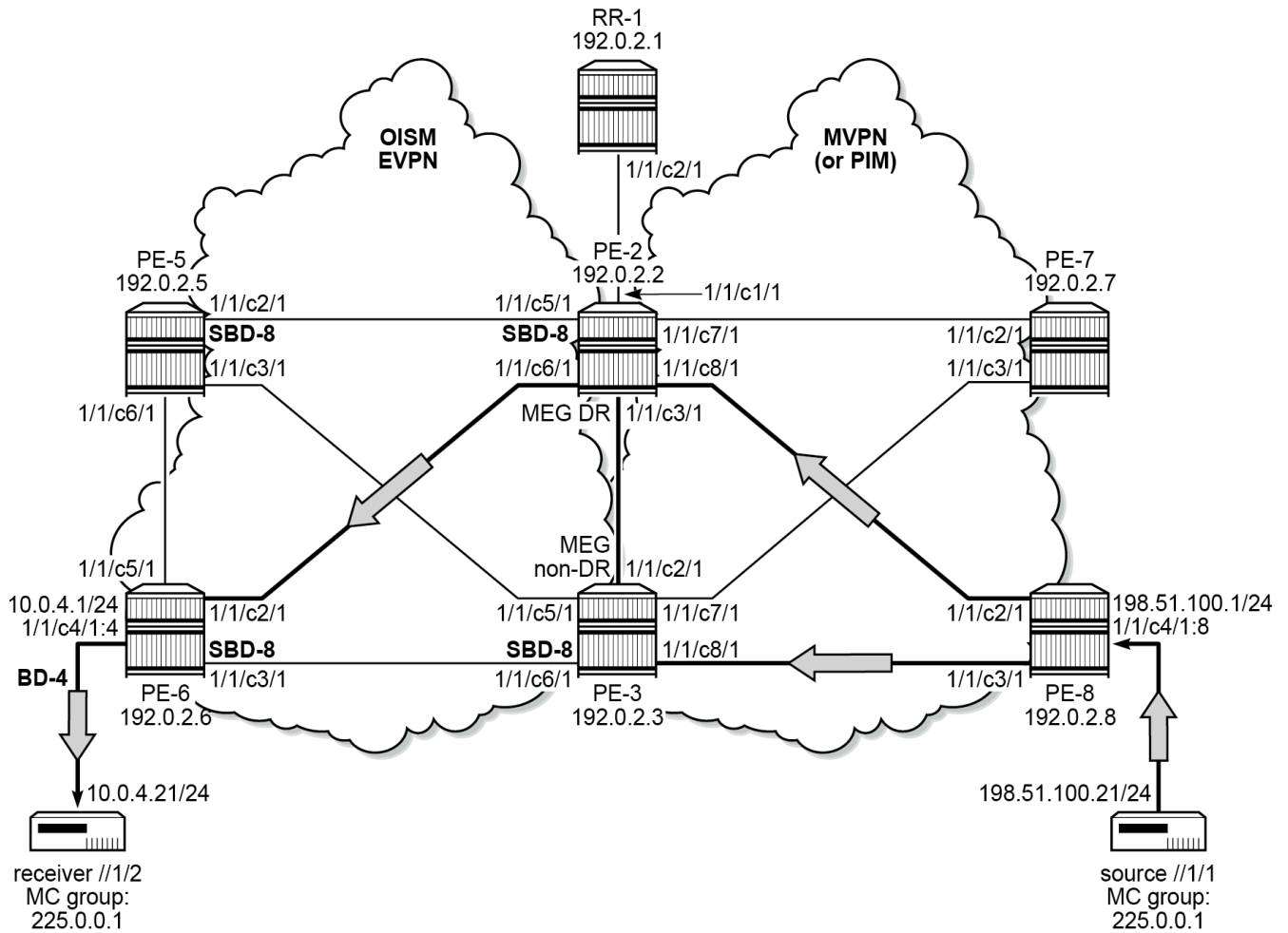
Figure 238: MVPN/PIM MC source - EVPN MC receiver example setup
