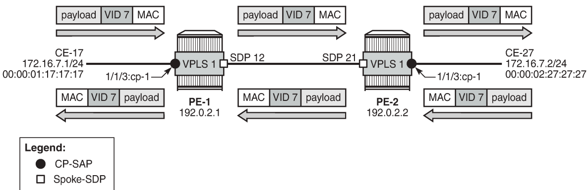
Figure 332: Customer VID is preserved between dot1q CP SAPs - no VLAN translation
