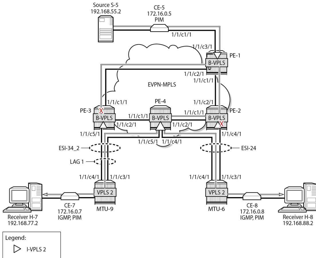
Figure 307: EVPN-MPLS with MH and PIM Snooping – Multicast Flow after Failover
