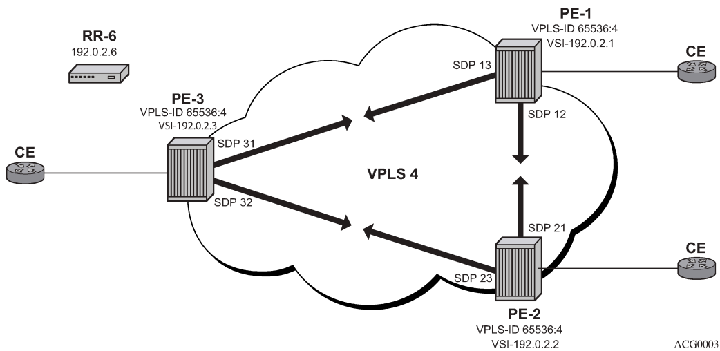
Figure 192: VPLS instance using pre-provisioned SDPs shows a VPLS instance configured across three PE routers as before.
