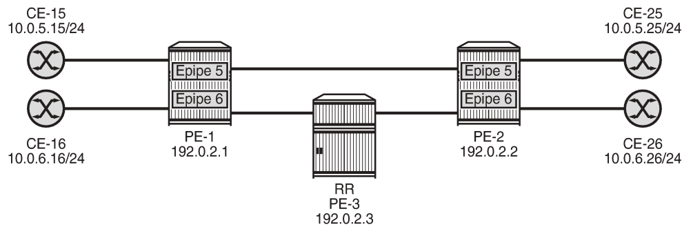
Figure 185: BGP-VPWS with auto-GRE spoke-SDPs
