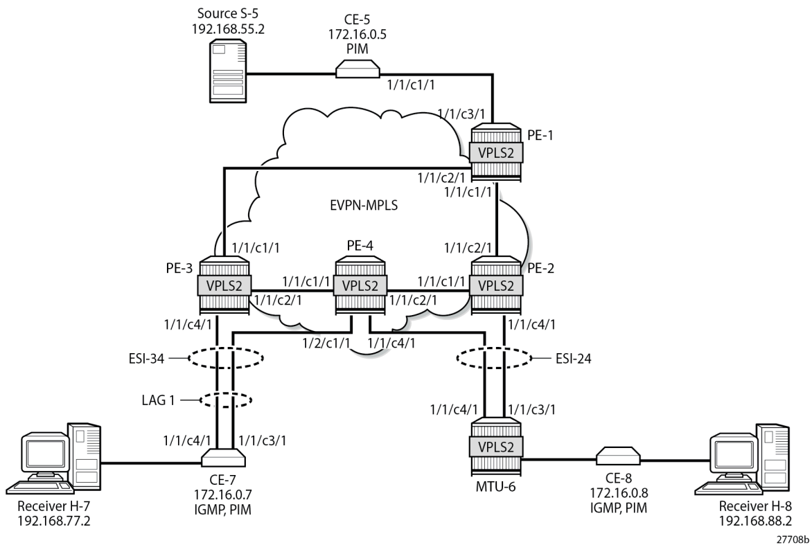
Figure 294: Example Topology with Multi-homing ESs
