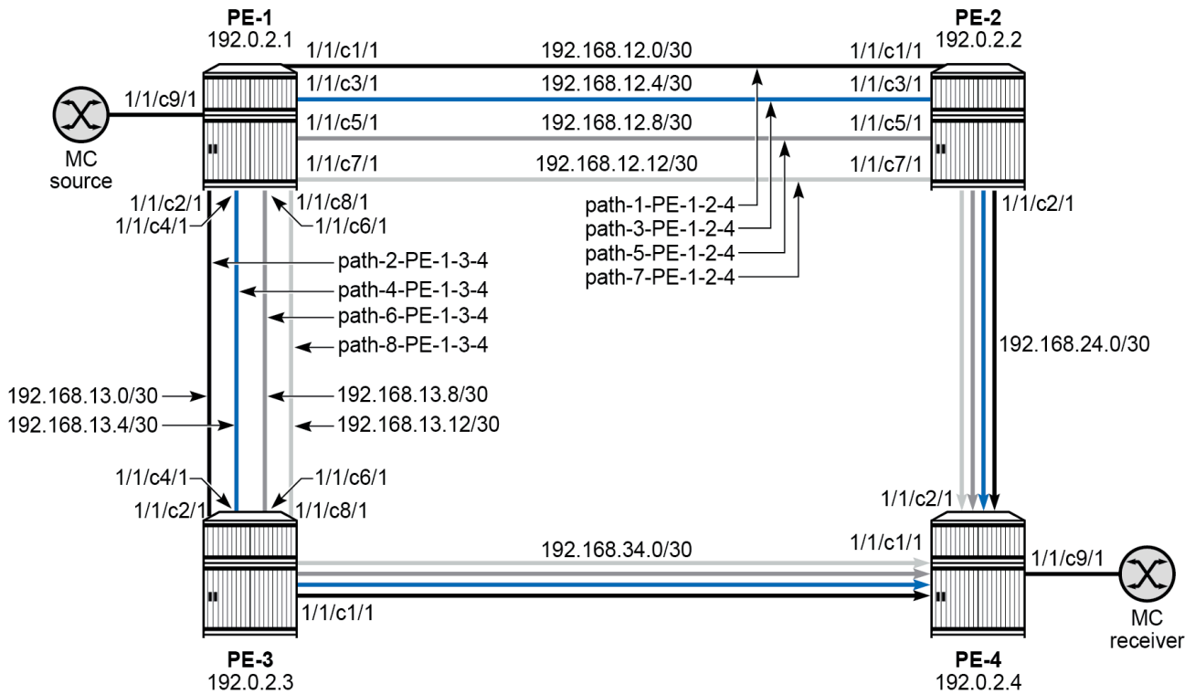
Figure 318: Example topology
