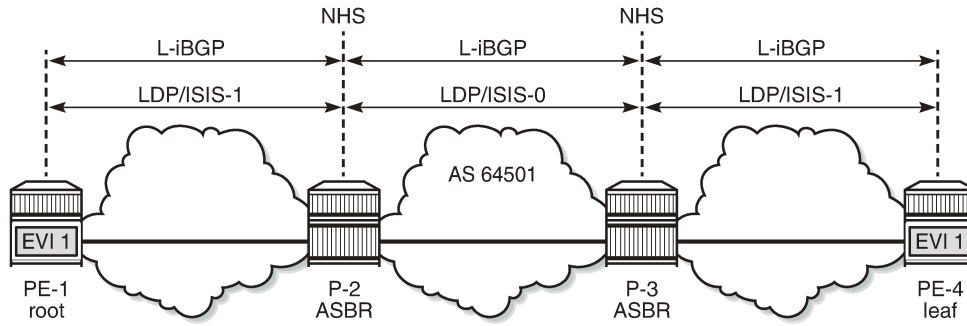
Figure 256: Example topology for seamless MPLS
