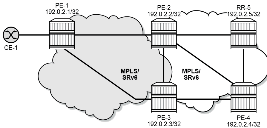
Figure 139: Example topology
