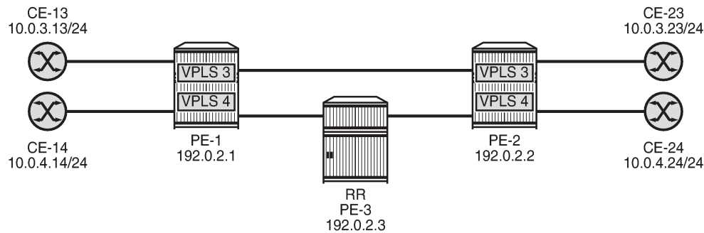
Figure 184: LDP-VPLS using BGP-AD with auto-GRE Spoke-SDPs
