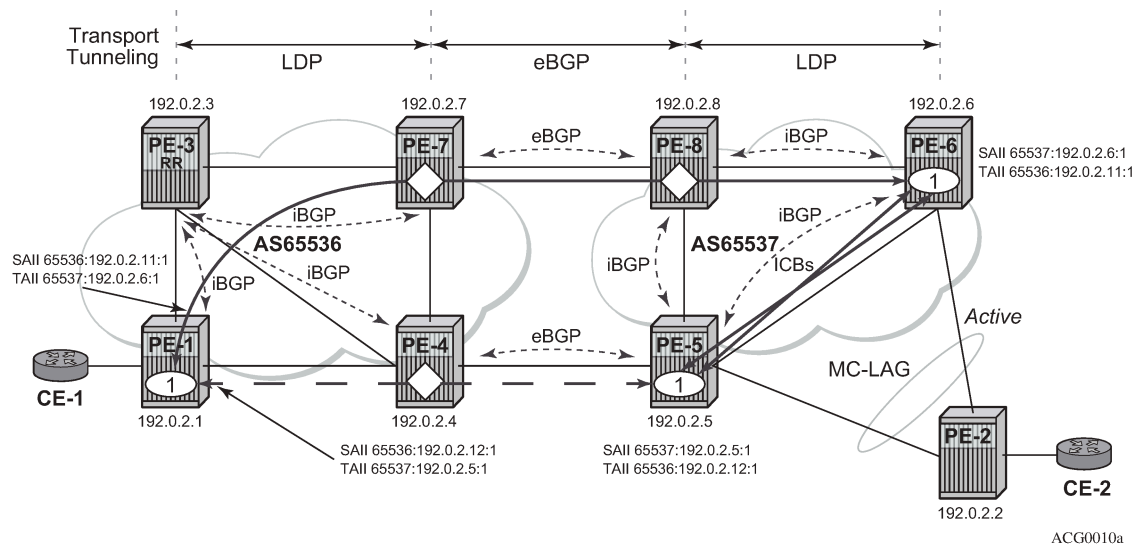
Figure 232: Inter-AS MS-PW example topology
