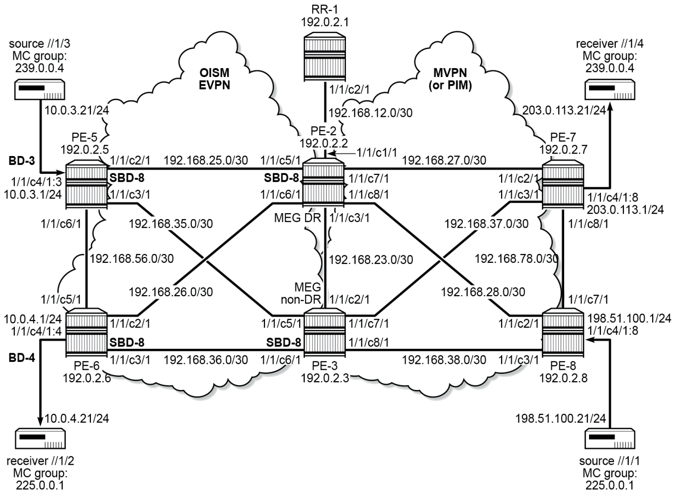
Figure 233: Example topology
