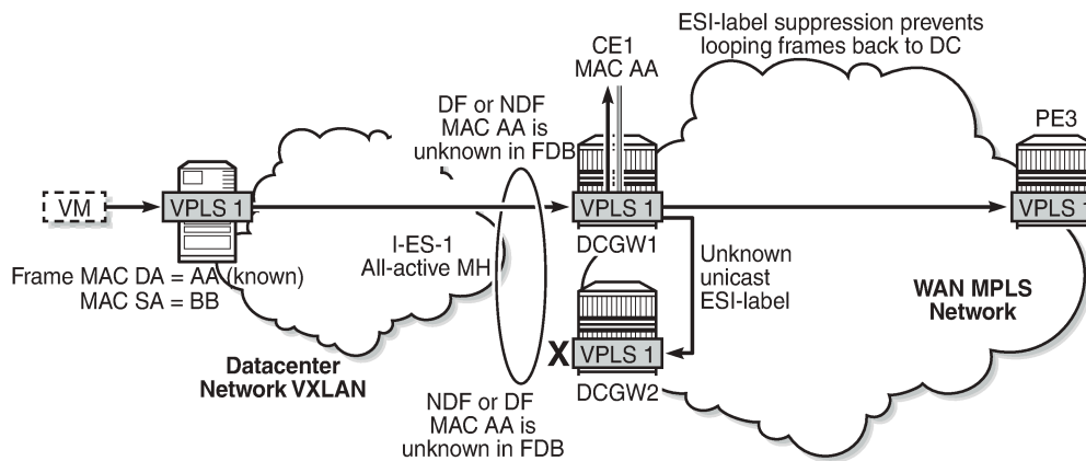
Figure 92: All-active multi-homing and unknown unicast example 1
