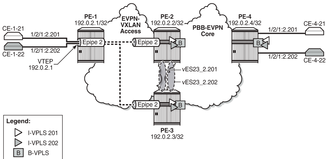
Figure 242: Epipe 2 with EVPN-VXLAN and all-active multi-homing
