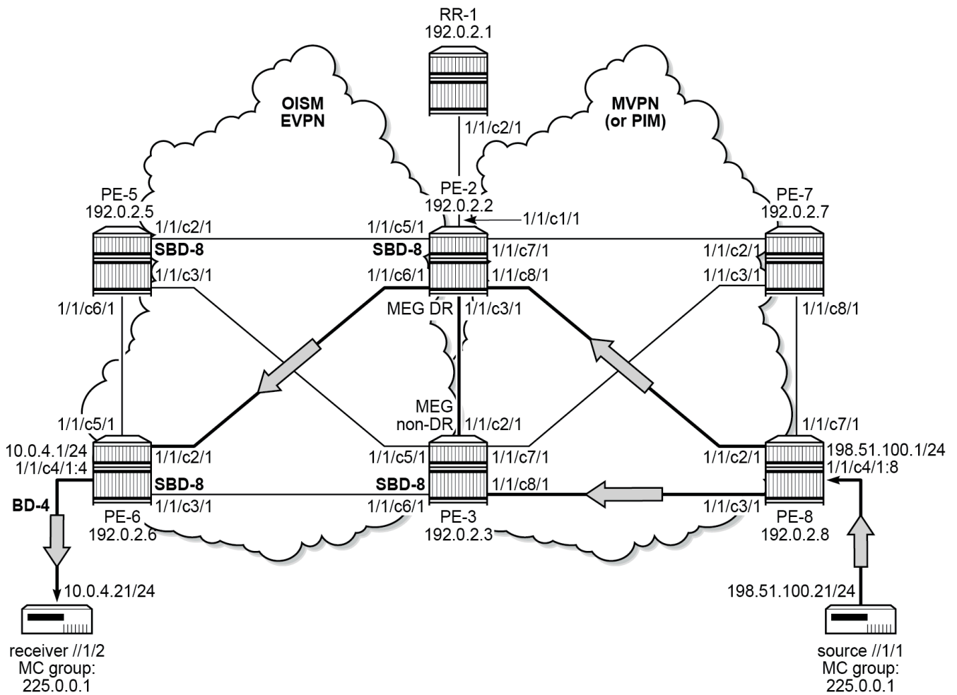
Figure 234: MVPN/PIM MC source - EVPN MC receiver example setup
