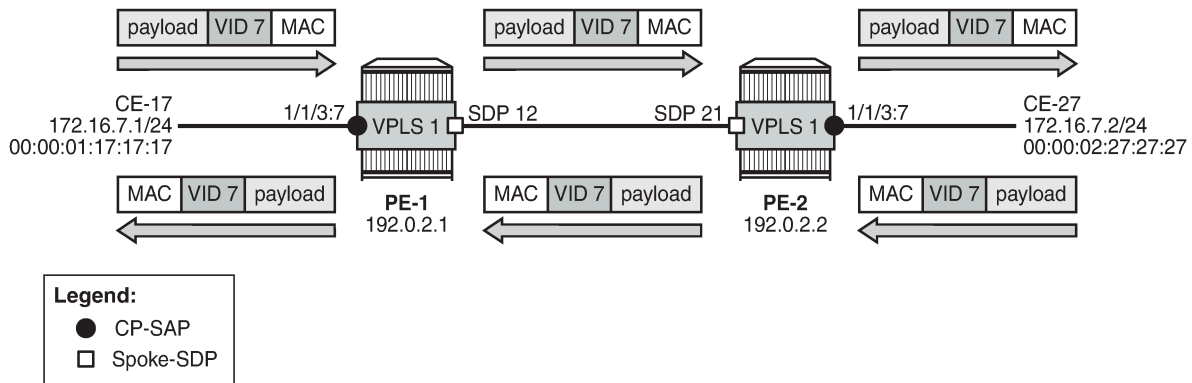
Figure 337: Customer VID is preserved between two dot1q CP SAPs
