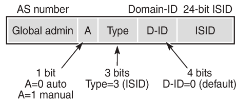
Figure 277: PBB-EVPN ISID-based RT format
