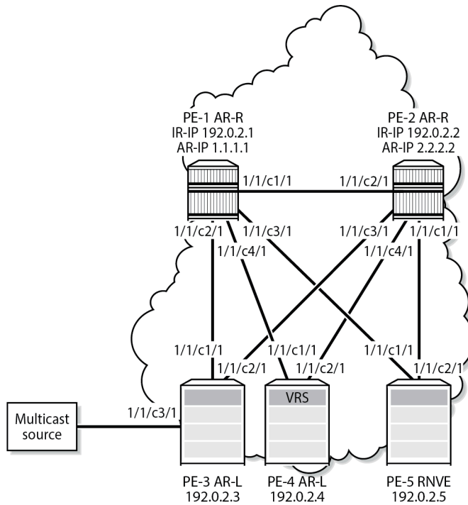
Figure 189: Example topology
