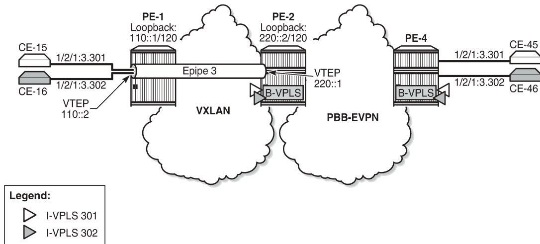
Figure 322: Example topology for static VXLAN termination on IPv6 addresses
