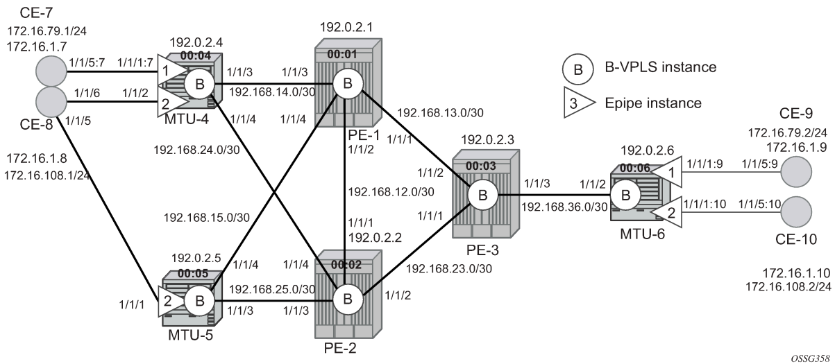
Figure 280: Example topology with port numbers and IP addresses
