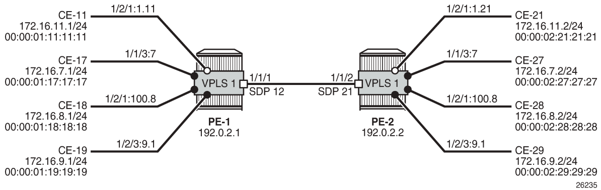
Figure 335: Example topology for VLAN ranges in VPLS 1
