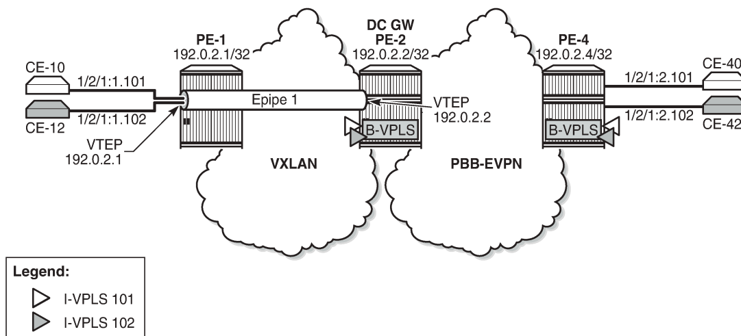
Figure 320: Example topology for static VXLAN termination on system IP addresses
