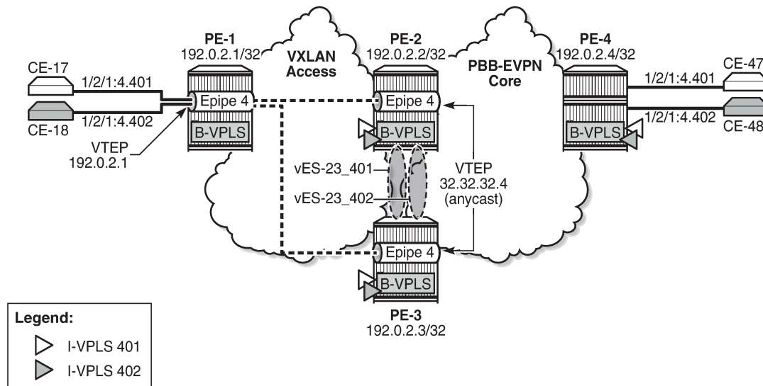
Figure 323: Example topology for static VXLAN termination using anycast
