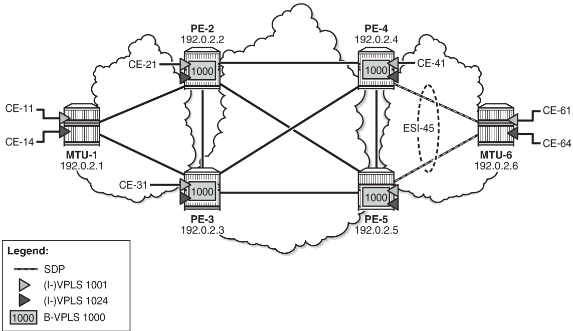
Figure 274: Example topology with single-active ES
