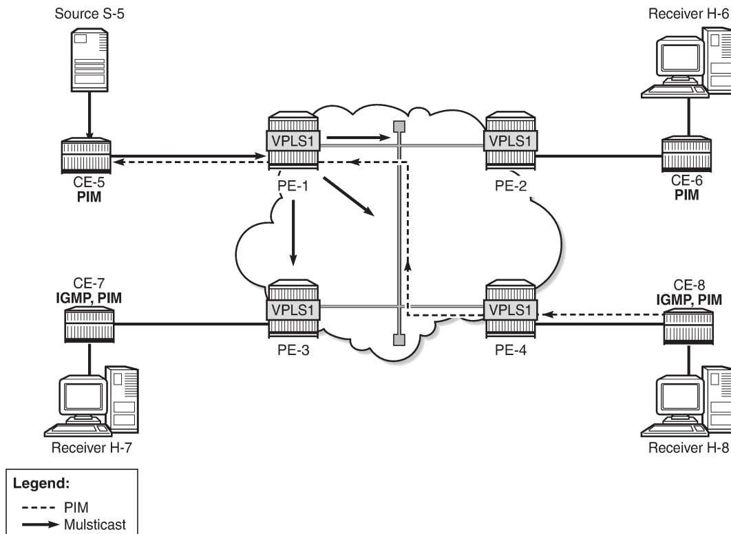
Figure 284: Multicast in VPLS without PIM Snooping
