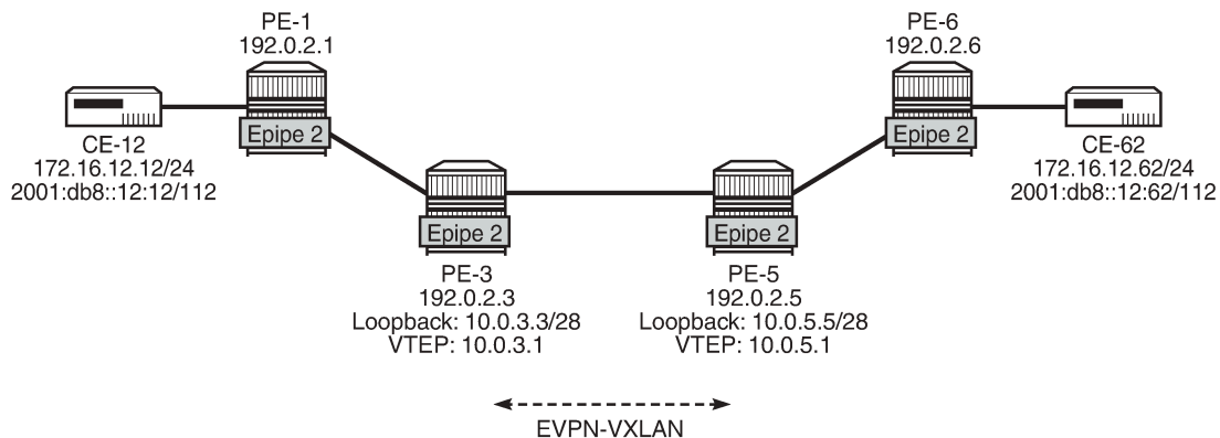
Figure 167: Single-homed EVPN-VXLAN Epipe 2 using non-system IP addresses
