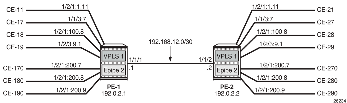
Figure 334: Example topology
