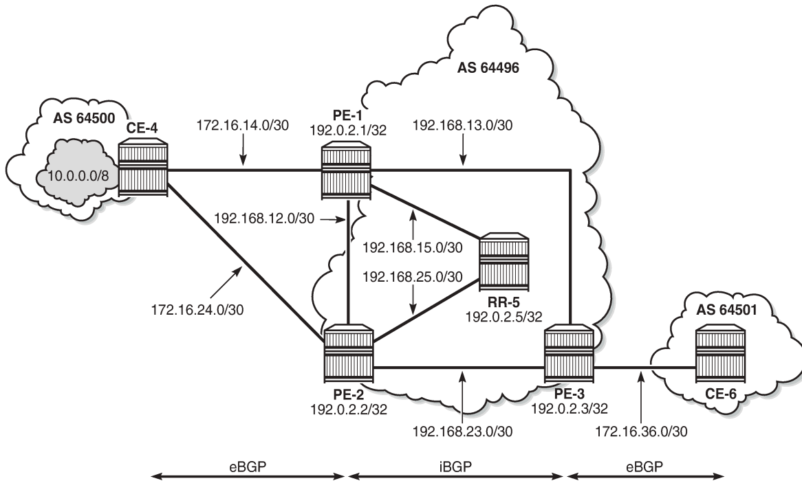
Figure 12: Example topology
