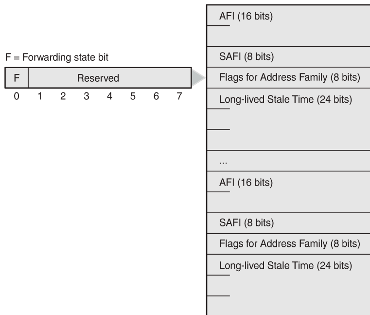
Figure 47: LLGR capability
