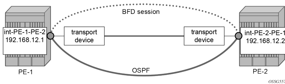
Figure 14: BFD for OSPF
