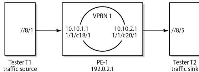
Figure 32: Example Configuration
