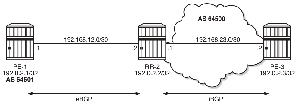
Figure 141: Example topology
