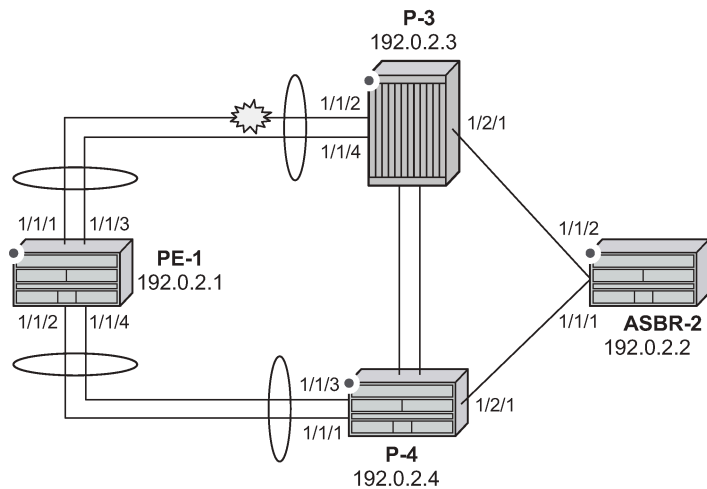
Figure 132: Link failure
