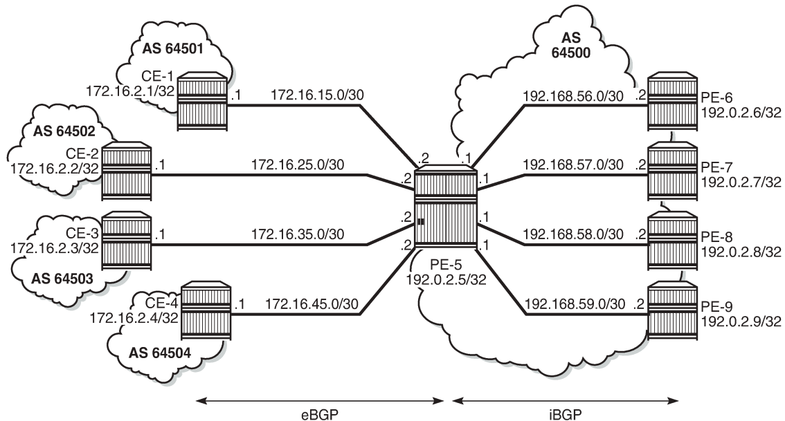
Figure 52: Example topology
