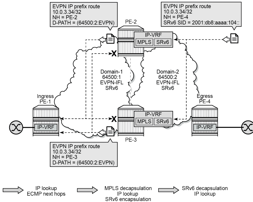
Figure 215: EVPN IP prefix routes readadvertised between SRv6 domains
