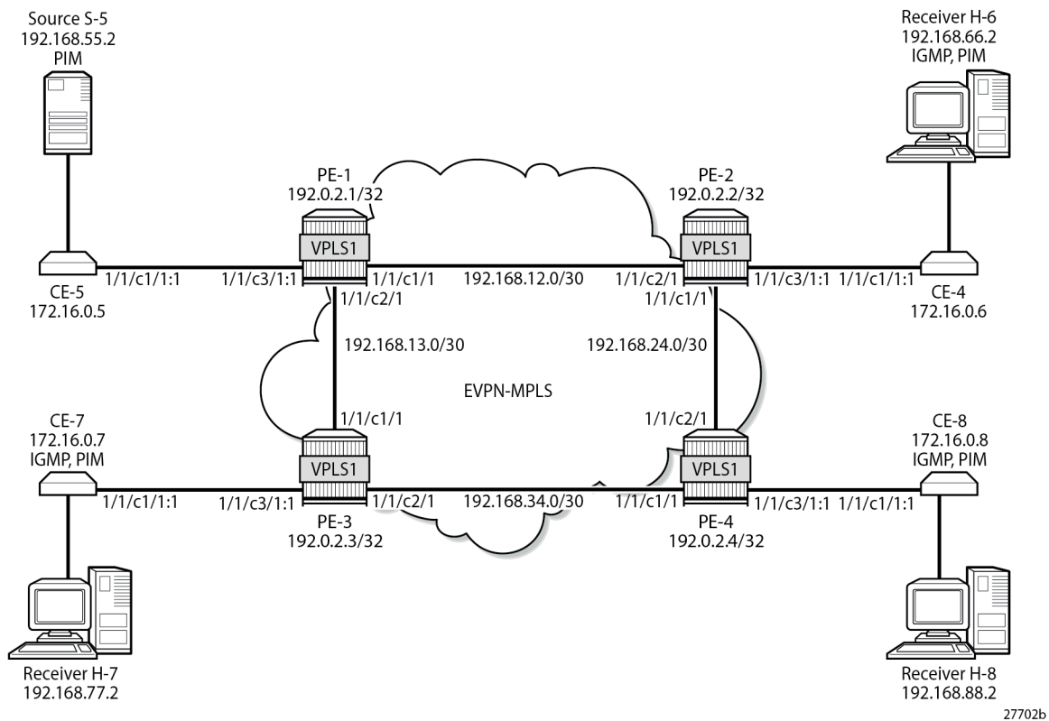
Figure 269: Example Topology
