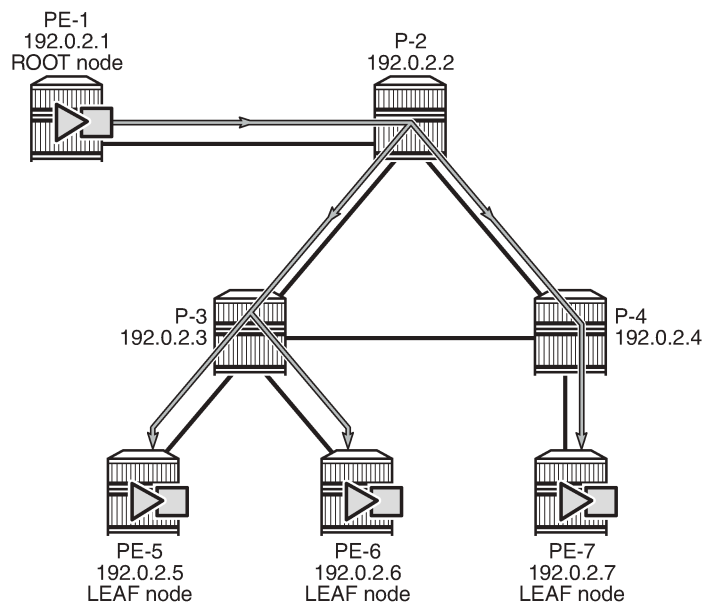
Figure 246: P2MP mLDP in PBB-EVPN
