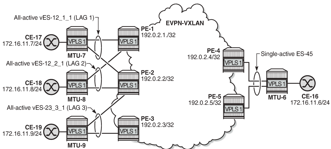
Figure 117: Example topology
