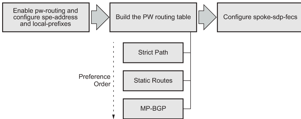
Figure 219: Configuration flowchart
