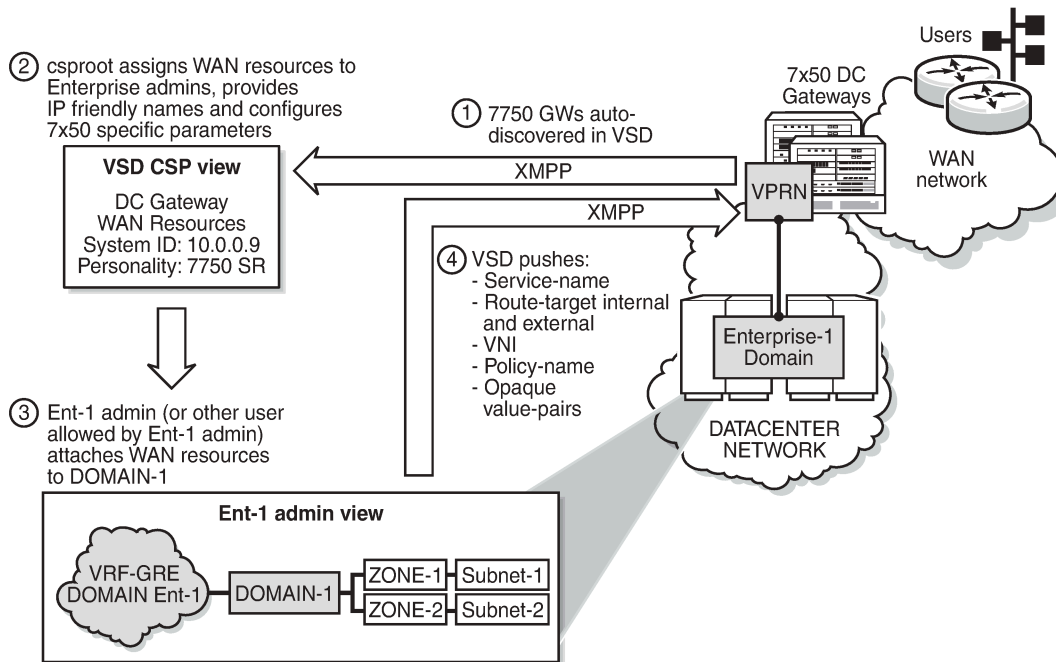
Figure 170: DC Gateway fully dynamic provisioning workflow
