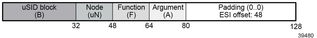
Figure 123: SRv6 micro-SID encoding
