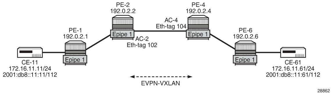
Figure 160: Single-homed EVPN-VXLAN Epipe 1 using system IP addresses
