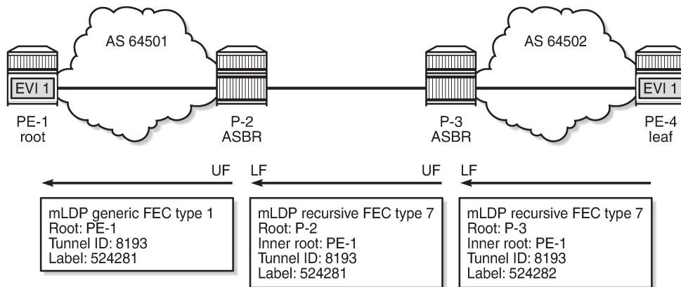
Figure 235: Recursive mLDP FEC for inter-AS model C
