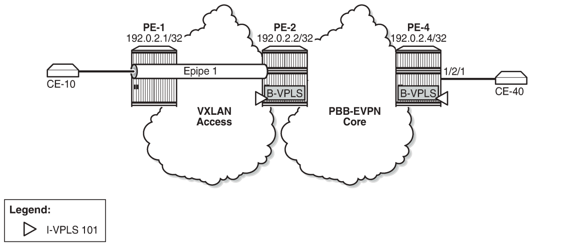
Figure 300: Static VXLAN termination on system IP addresses
