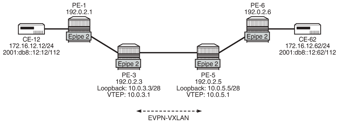
Figure 161: Single-homed EVPN-VXLAN Epipe 2 using non-system IP addresses
