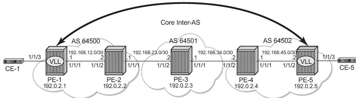
Figure 174: Network setup configuration
