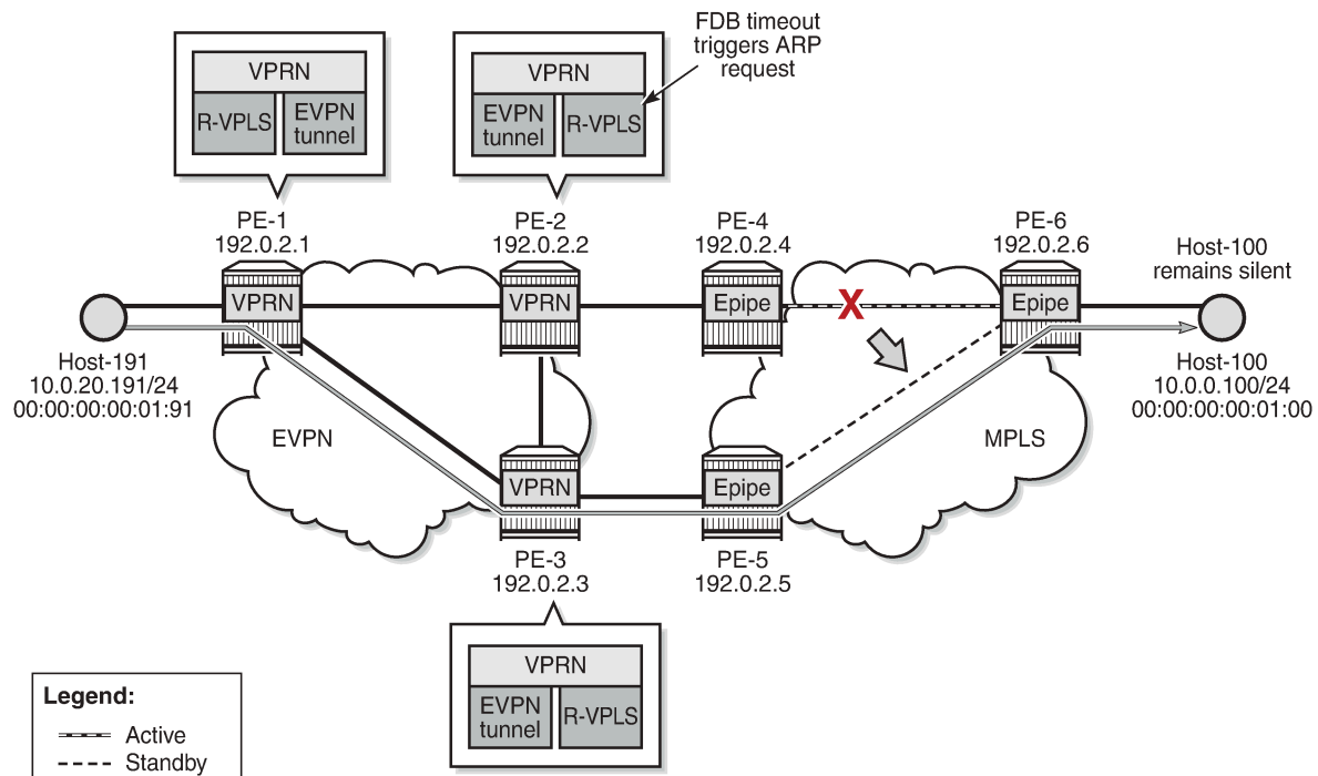
Figure 199: Host does not send any traffic after switchover
