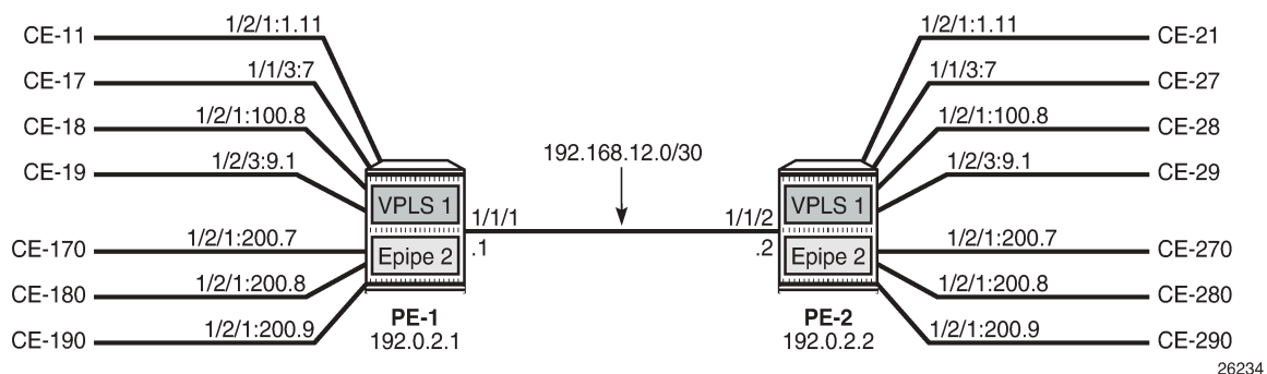
Figure 315: Example topology
