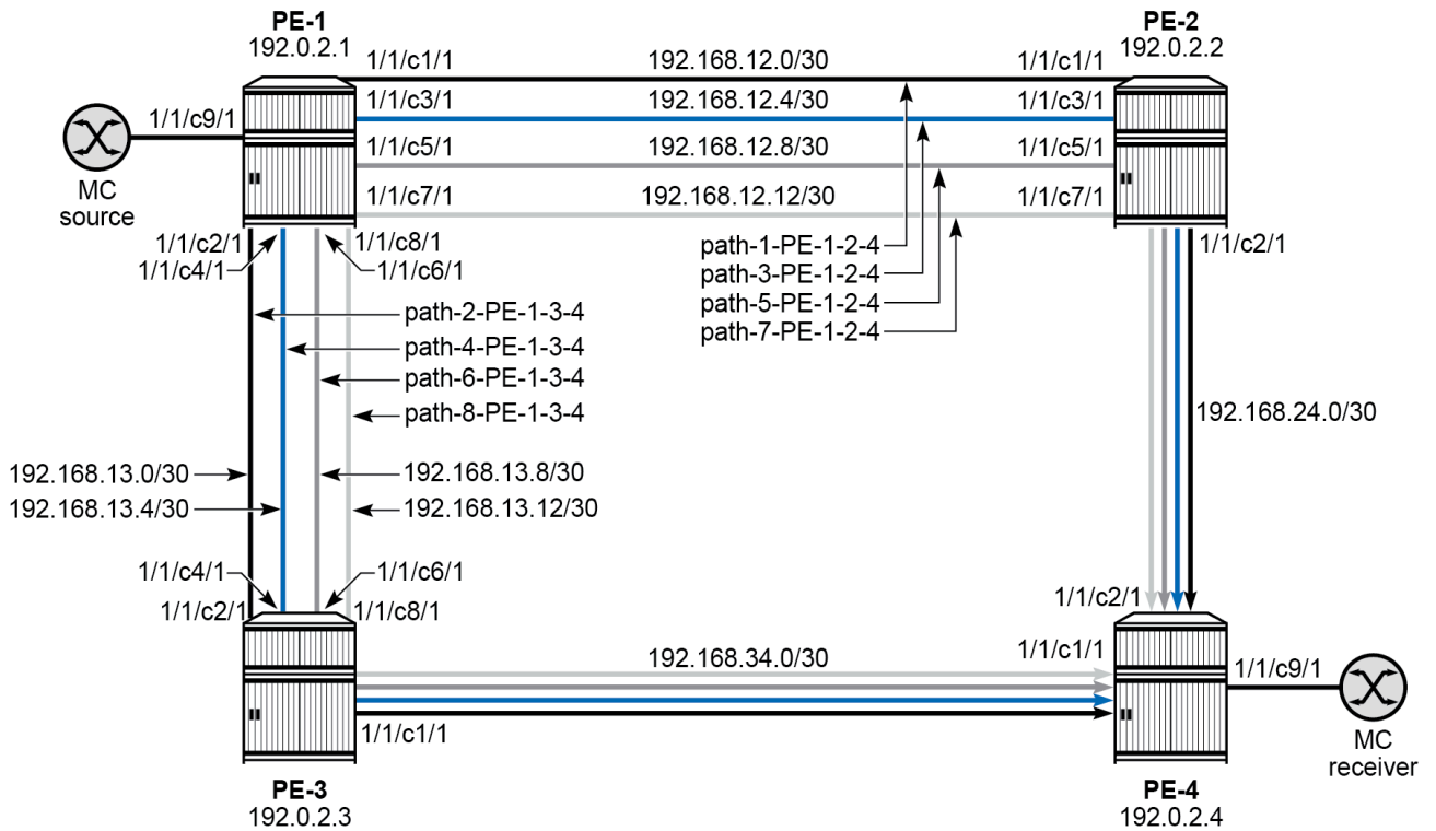
Figure 299: Example topology
