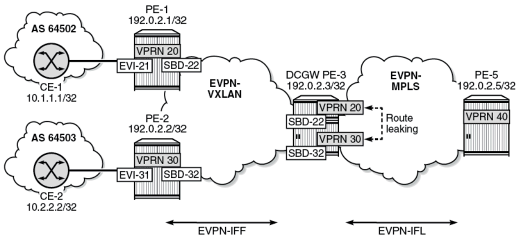
Figure 143: Example topology
