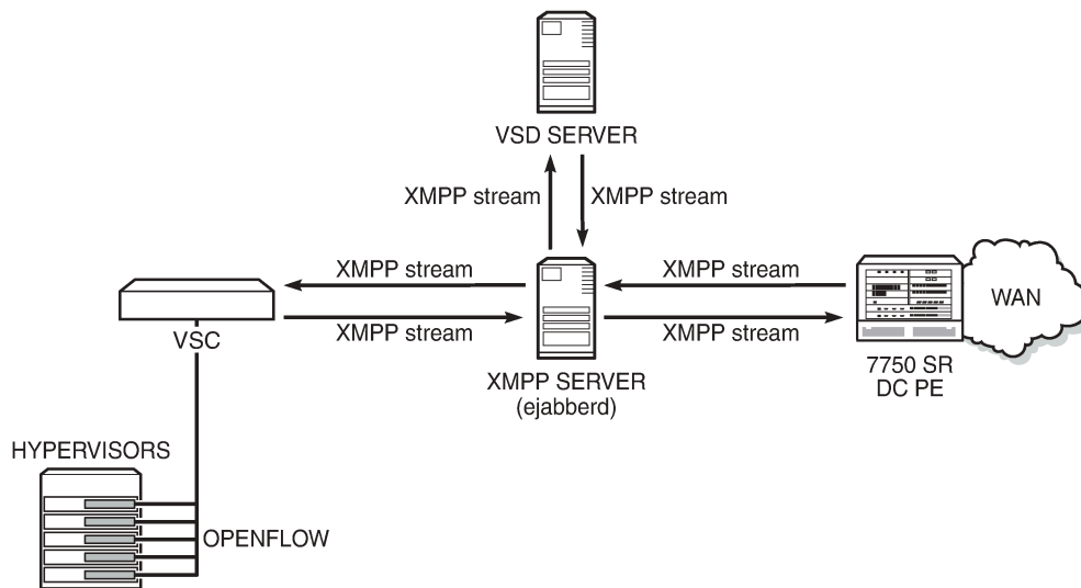
Figure 171: F-D XMPP provisioning setup
