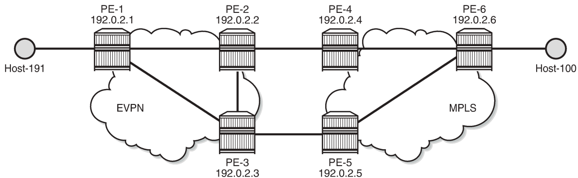
Figure 195: Example topology with system IP addresses
