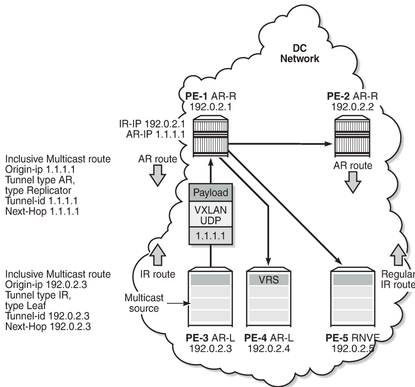
Figure 182: EVPN Assisted Replication for VXLAN
