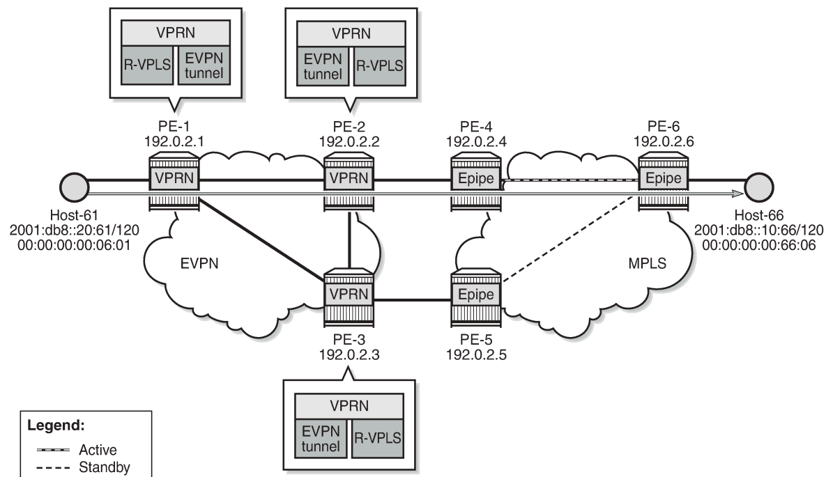
Figure 200: Example topology for initial forwarding path via PE-2 with IPv6 addresses
