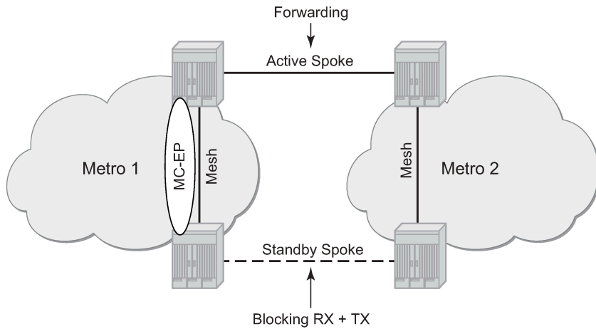
Figure 207: Multi-chassis endpoint with square resiliency
