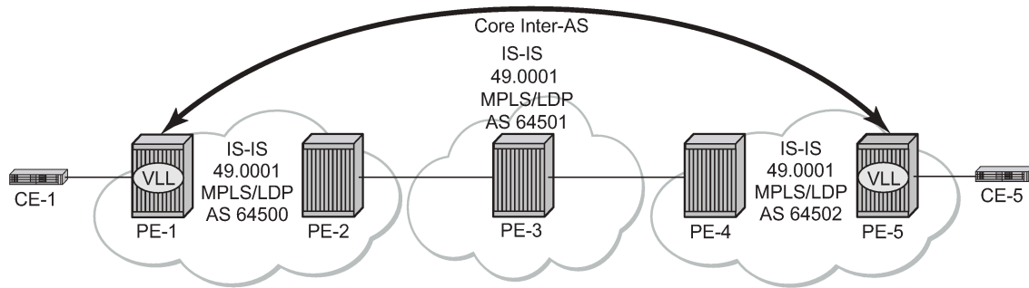
Figure 172: Example topology – Inter-AS model C for VLL
