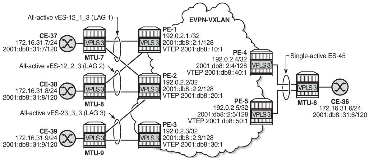
Figure 119: Non-system IPv6 VTEP multi-homing for VXLAN VPLS 2
