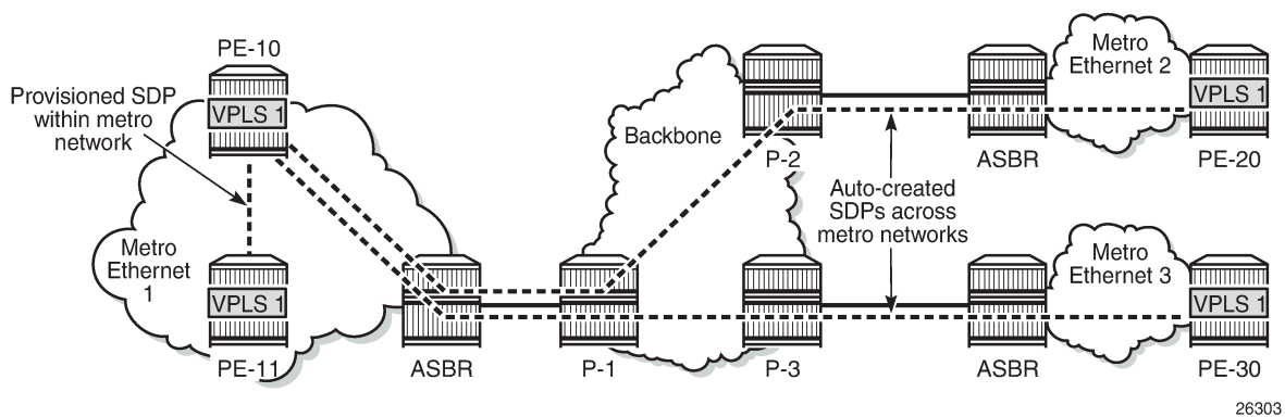
Figure 188: LDP VPLS using BGP-AD with prefer-provisioned-sdp option
