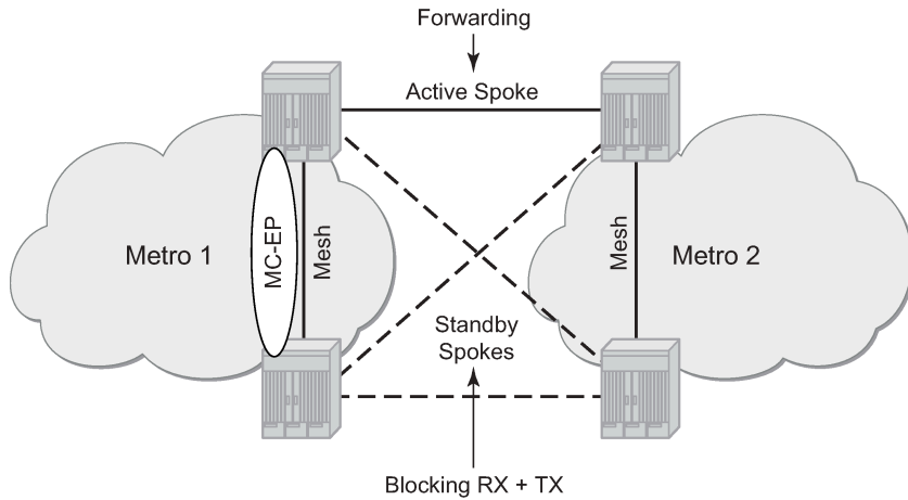
Figure 206: Multi-chassis endpoint with mesh resiliency
