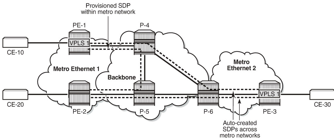
Figure 192: SDP bindings in VPLS 1 with prefer-provisioned-sdp option
