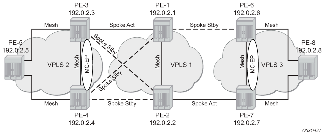
Figure 208: Example topology
