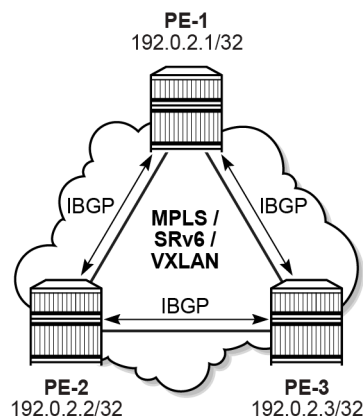
Figure 103: Nodes in AS 64500 with IBGP sessions
