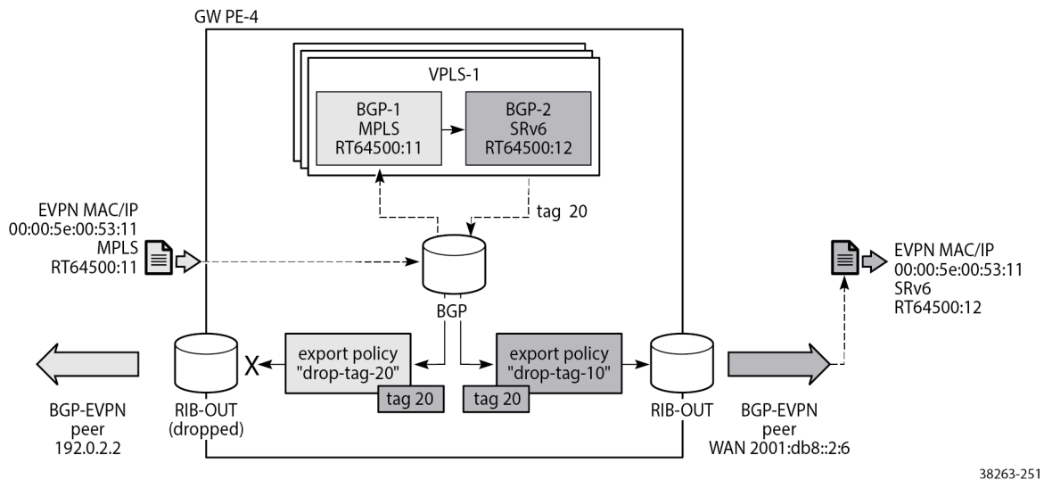
Figure 128: Default route tags per service instance avoid loops
