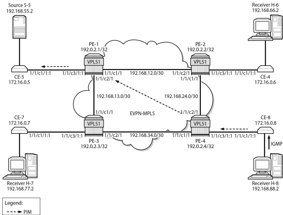
Figure 273: H-8 Joins (192.168.55.2, 232.1.1.1) and PIM Snooping is Enabled in Proxy Mode
