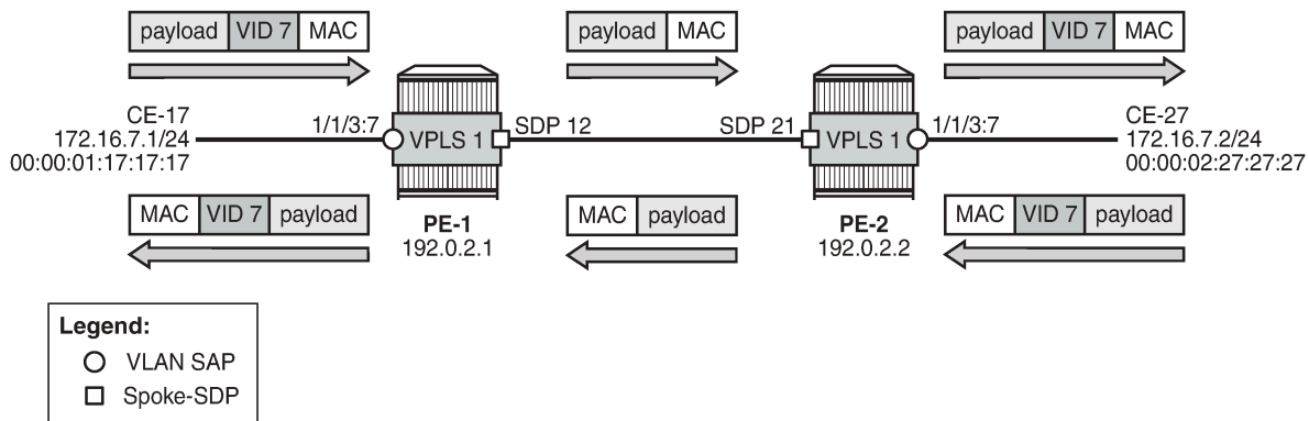
Figure 318: Customer VID is preserved between two dot1q CP SAPs shows how the customer VID 7 is preserved between CE-17 and CE-27 when CP SAPs are used instead of VLAN SAPs. The configuration for the SAPs is modified as follows:
