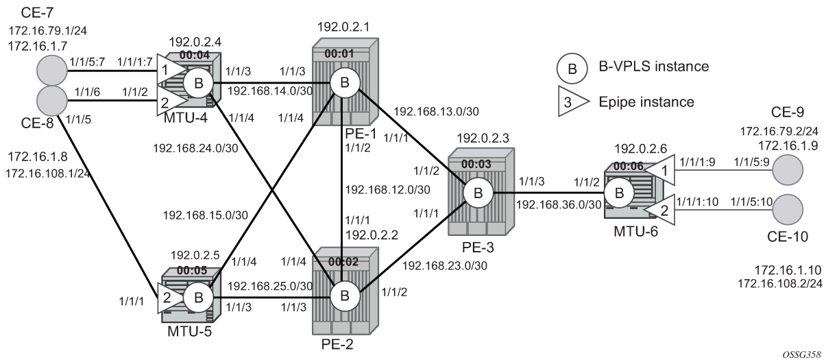
Figure 251: Example topology with port numbers and IP addresses
