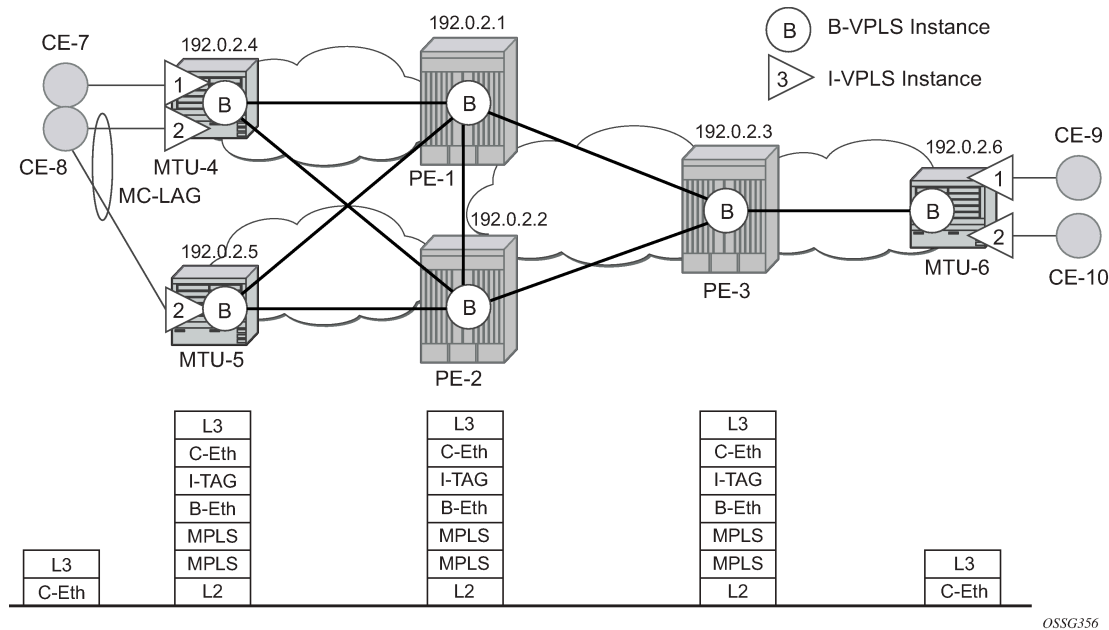
Figure 250: Example topology including B-VPLS, I-VPLSs, and protocol stacks
