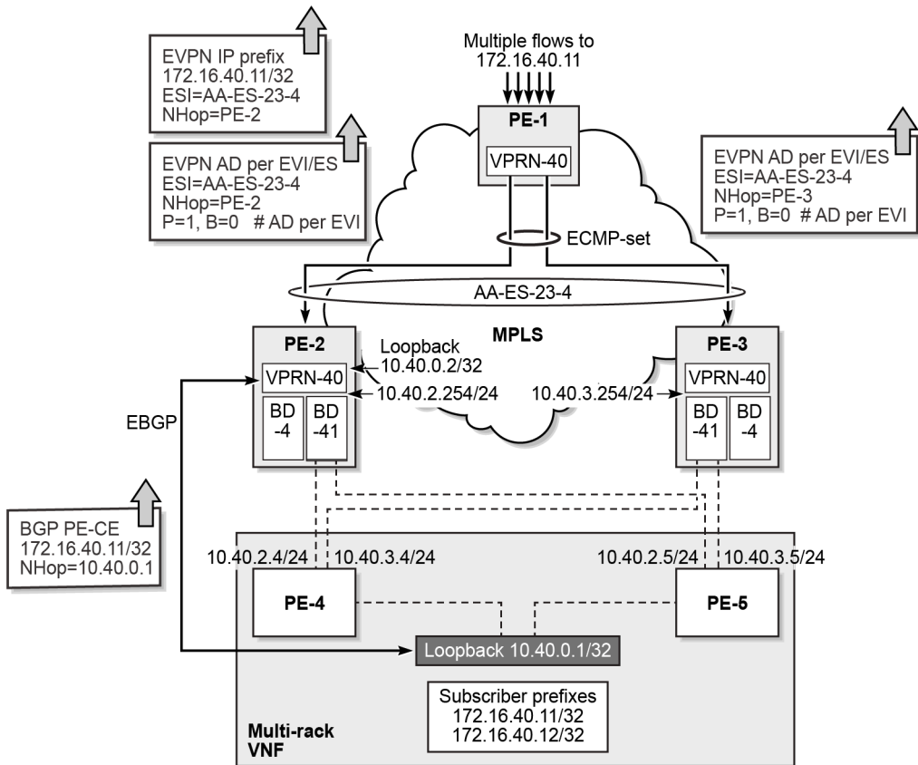
Figure 107: EVPN IP alias for EVPN IFF VPRN-40 over MPLS
