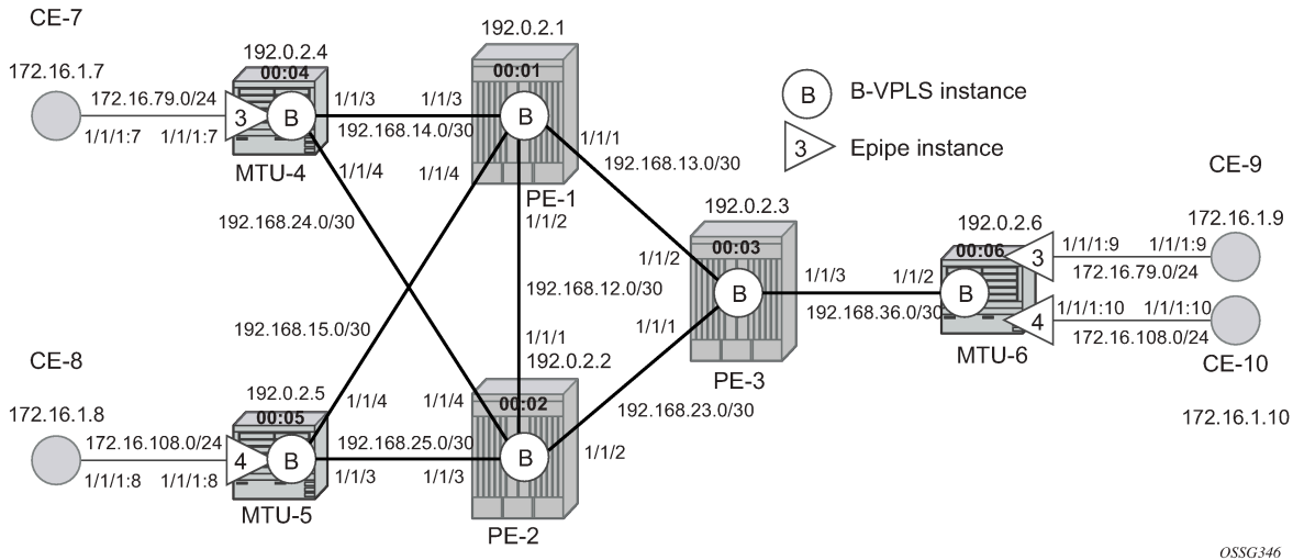
Figure 238: Setup detailed view
