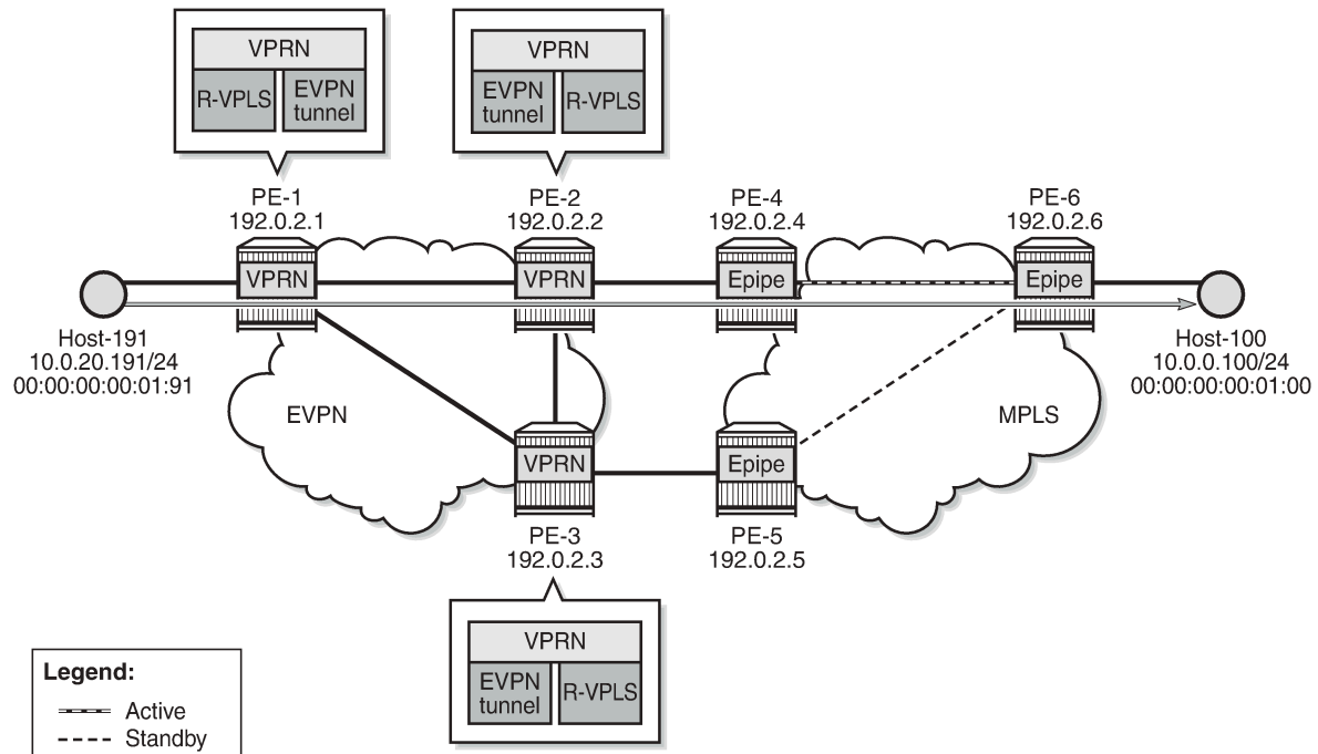
Figure 192: Initial situation with forwarding path via PE-2
