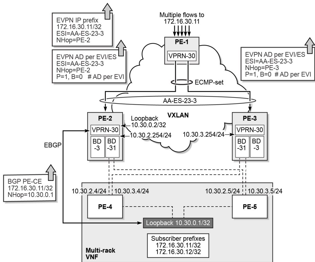
Figure 106: EVPN IP alias for EVPN IFF VPRN-30 over VXLAN
