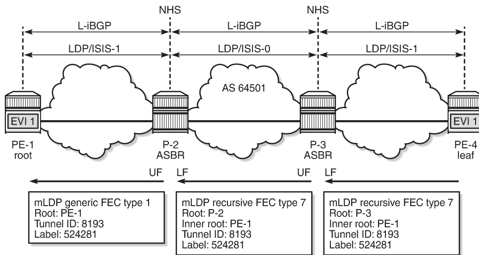
Figure 228: Recursive mLDP FEC for seamless MPLS
