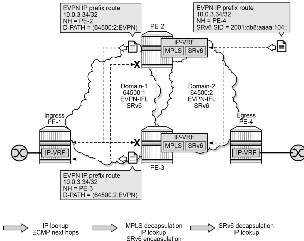
Figure 211: EVPN IP prefix routes readadvertised between SRv6 domains
