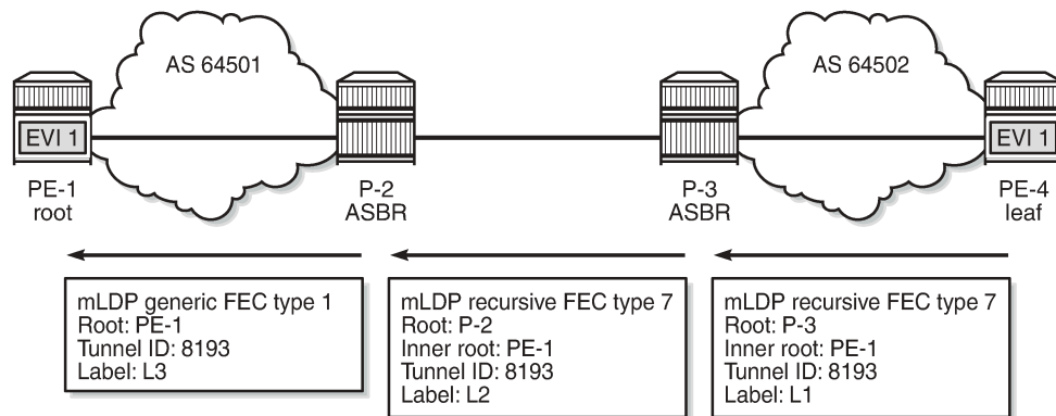
Figure 222: mLDP FEC label mapping messages for inter-AS model C
