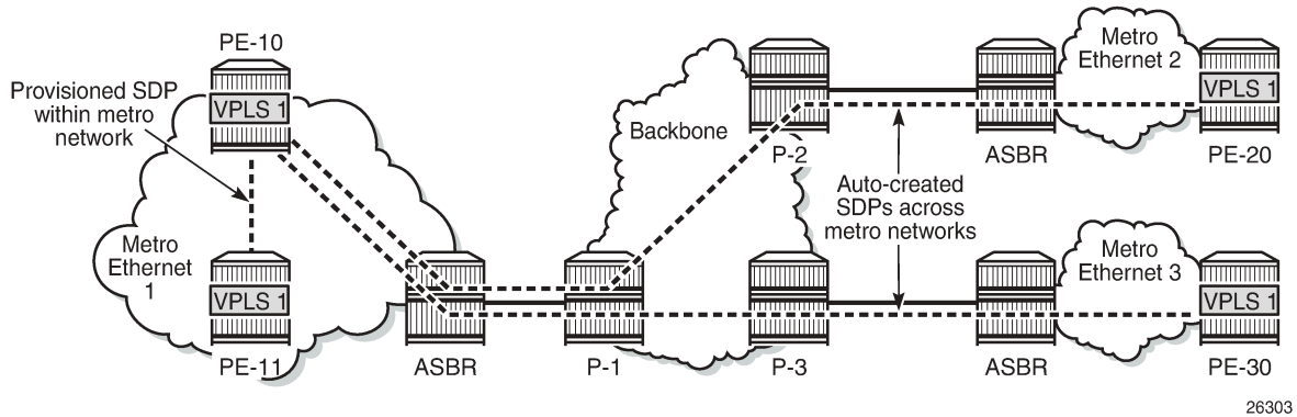
Figure 184: LDP VPLS using BGP-AD with provisioned-sdp prefer option
