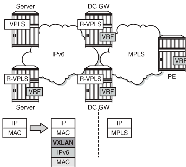
Figure 314: VXLAN IPv6 underlay for DC
