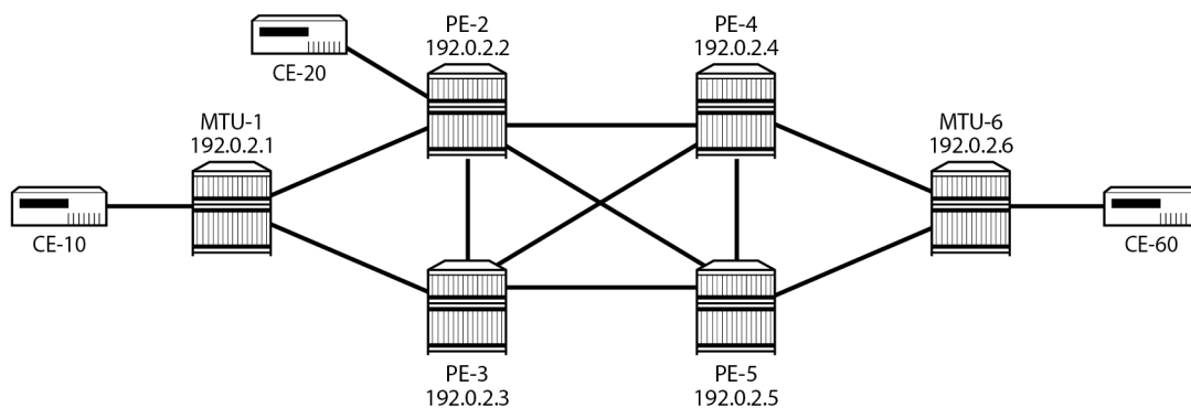
Figure 137: EVPN-VPWS example topology
