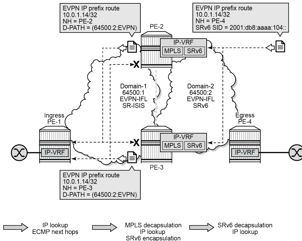
Figure 208: EVPN IP prefix routes readvertised between domains
