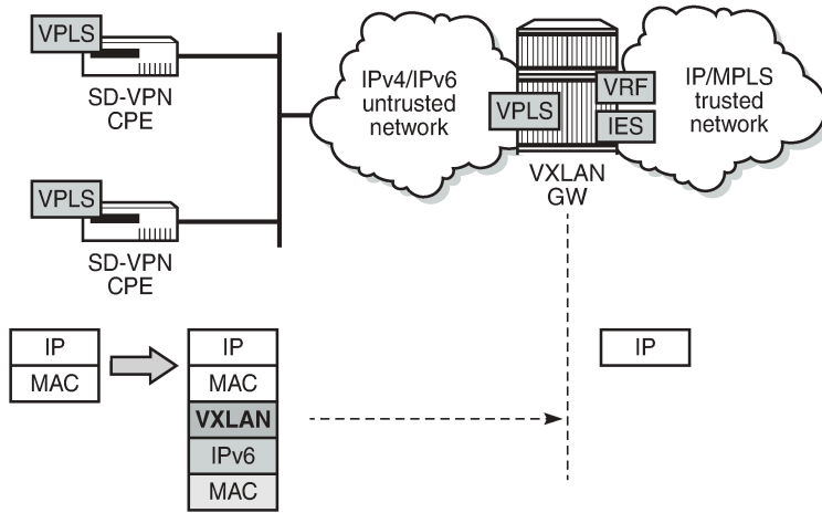
Figure 313: VXLAN GW in an SD-VPN
