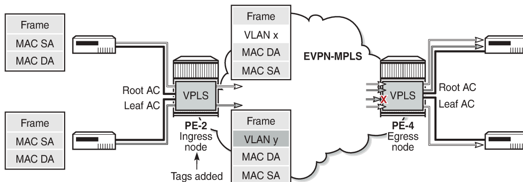
Figure 146: VLAN Tags Added by Ingress Node and Filtered by Egress Node in VPLS E-Tree
