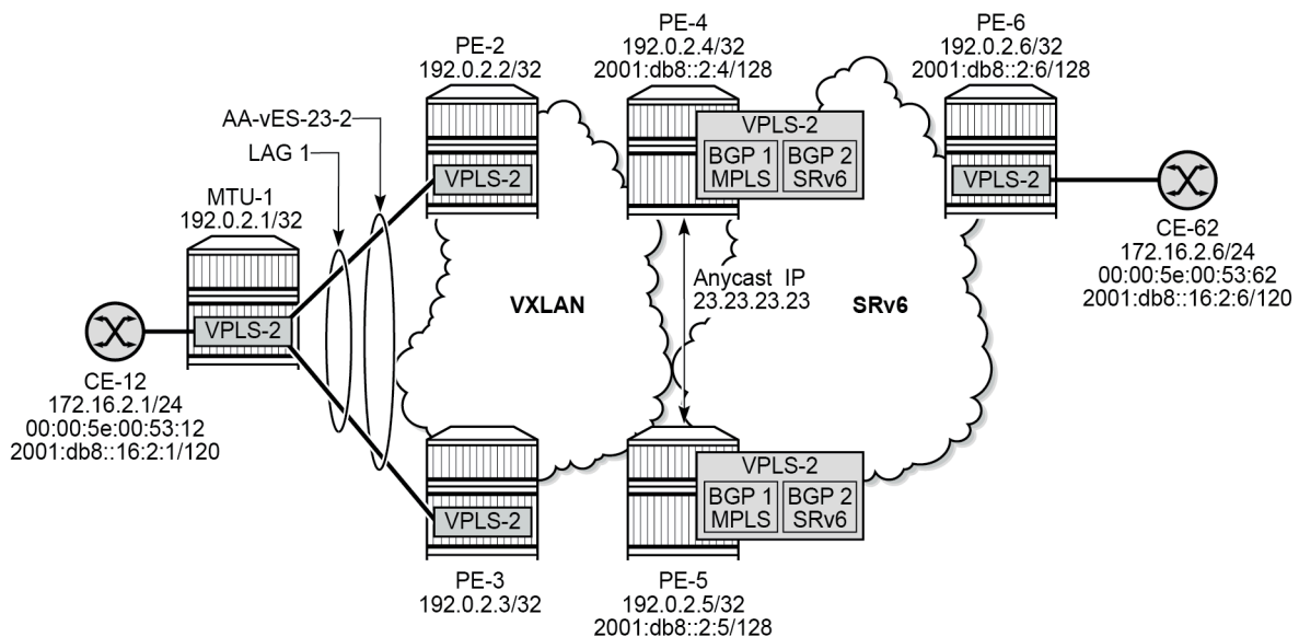
Figure 130: Example topology with VPLS-2
