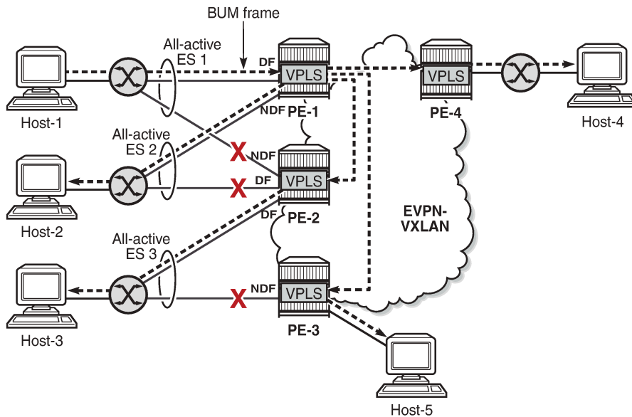
Figure 113: Split-horizon filtering based on tunnel source IP address
