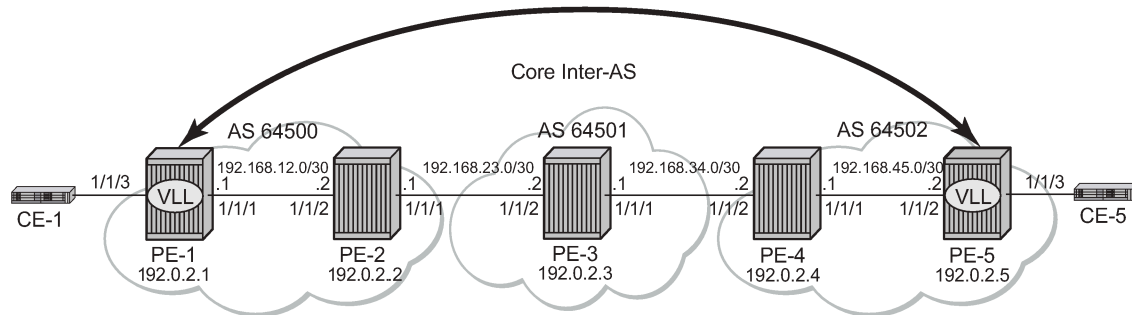
Figure 171: Network setup configuration
