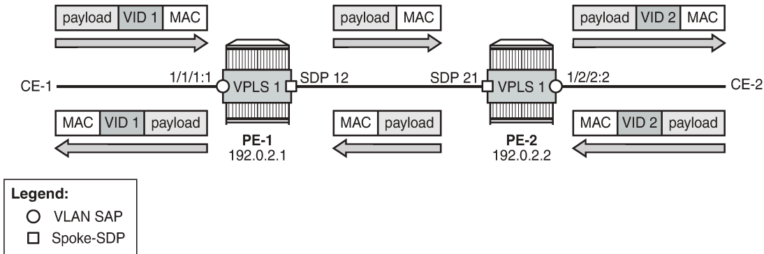
Figure 301: Customer VID is popped and pushed by VLAN SAPs - VLAN translation
