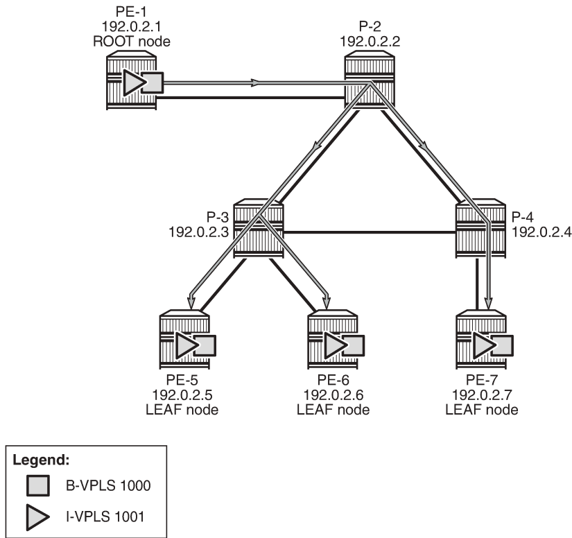
Figure 236: P2MP mLDP in PBB-EVPN
