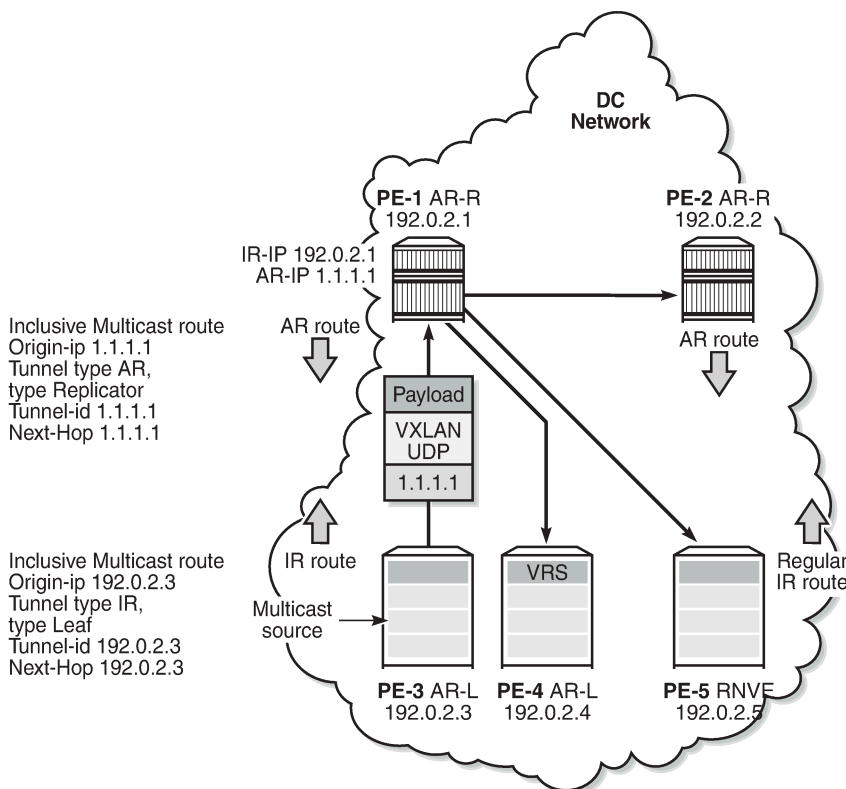
Figure 178: EVPN Assisted Replication for VXLAN
