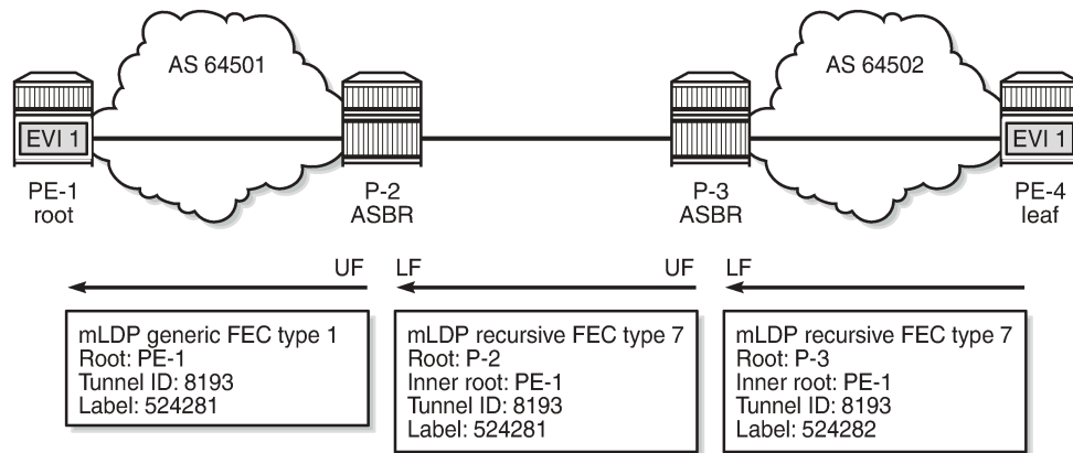
Figure 225: Recursive mLDP FEC for inter-AS model C
