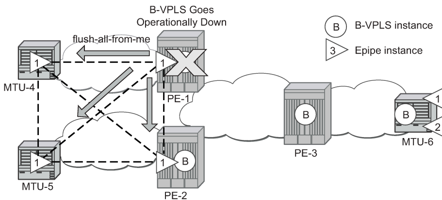
Figure 253: Send flush on B-VPLS failure example
