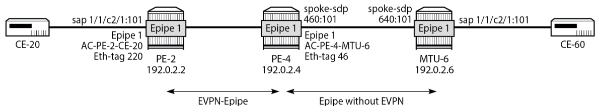
Figure 138: Example topology for EVPN-VPWS without multihoming
