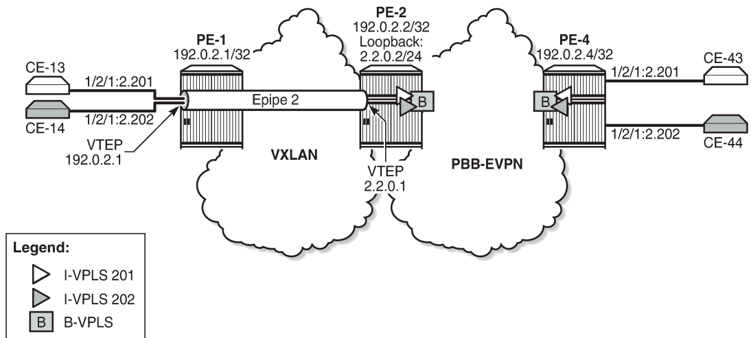
Figure 291: Example topology for static VXLAN termination on non-system IPv4 addresses
