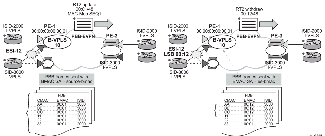
Figure 77: The use of ES BMAC to minimize CMAC flush
