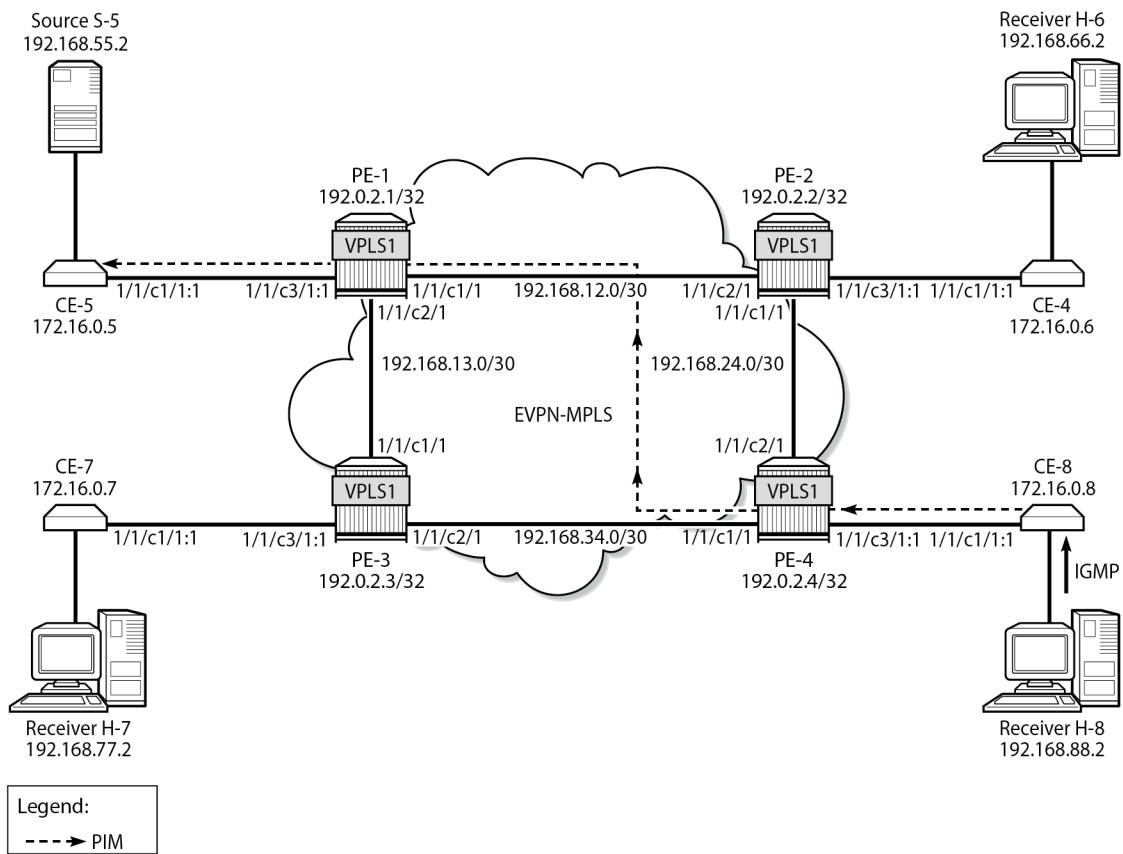
Figure 261: H-8 Joins Group (192.168.55.2, 232.1.1.1) and PIM Snooping is Disabled
