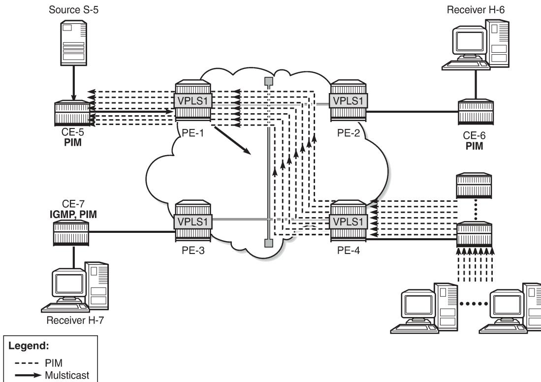
Figure 257: Multicast in VPLS with PIM Snooping in Snoop Mode – Multiple CEs
