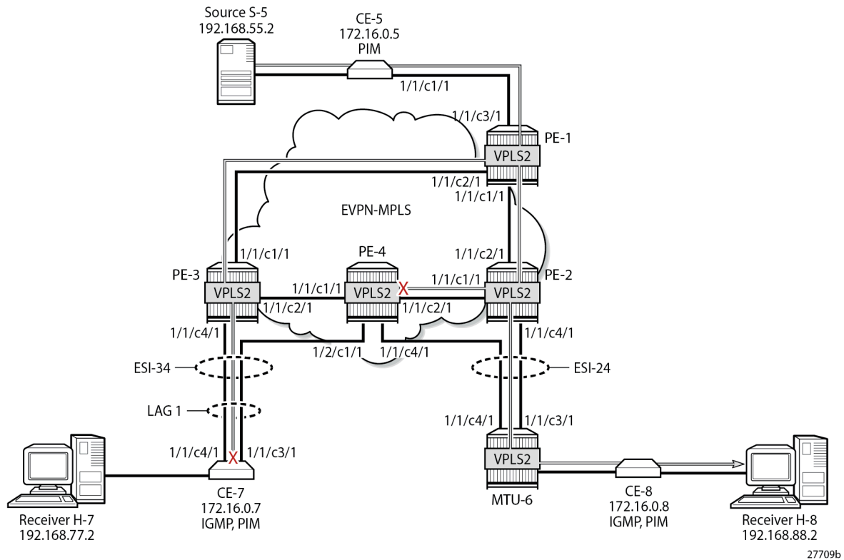
Figure 266: EVPN-MPLS with Multi-homing – Receiver H-8 Joined
