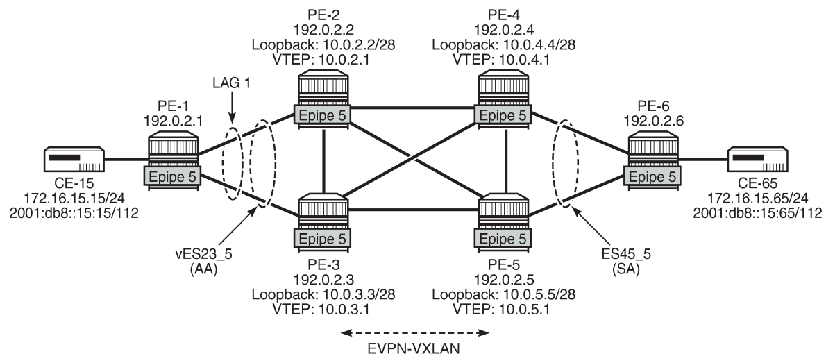
Figure 164: EVPN-VXLAN Epipe 5 with AA MH and SA MH using non-system IPv4 addresses
