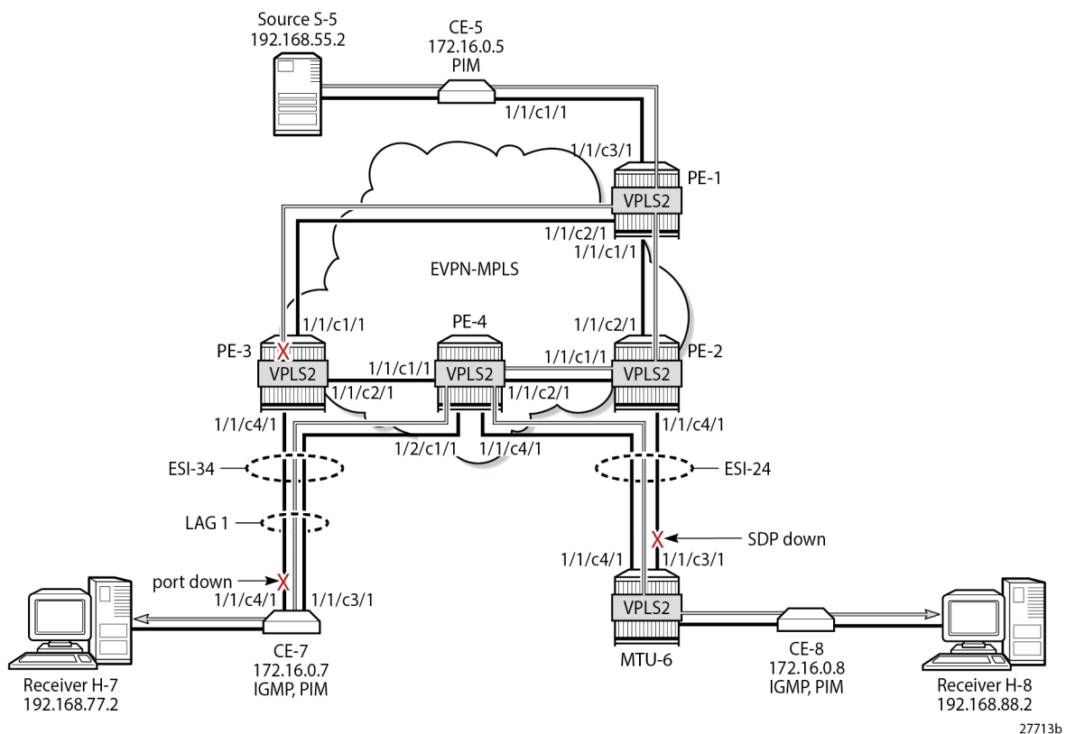
Figure 270: EVPN-MPLS with Multi-homing and PIM Snooping - Multicast Flow after Failover
