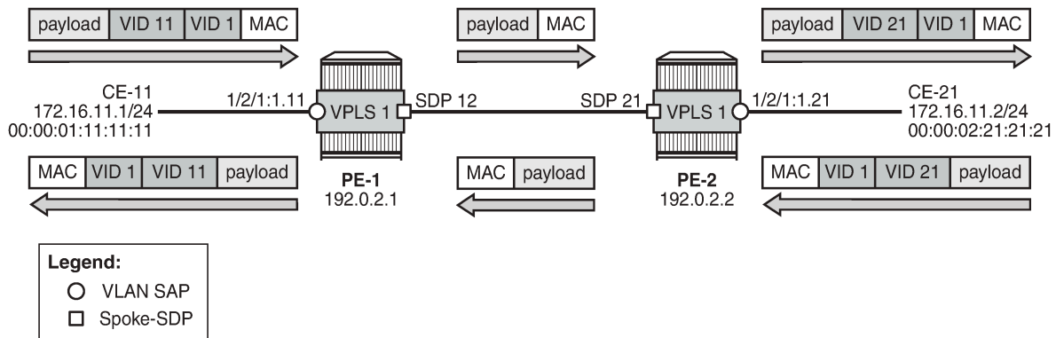
Figure 309: Traffic between two QinQ VLAN SAPs - VLAN translation
