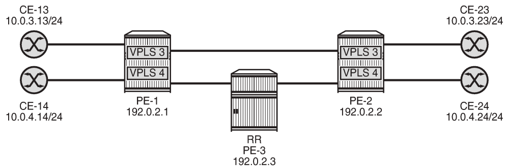
Figure 175: LDP-VPLS using BGP-AD with auto-GRE Spoke-SDPs
