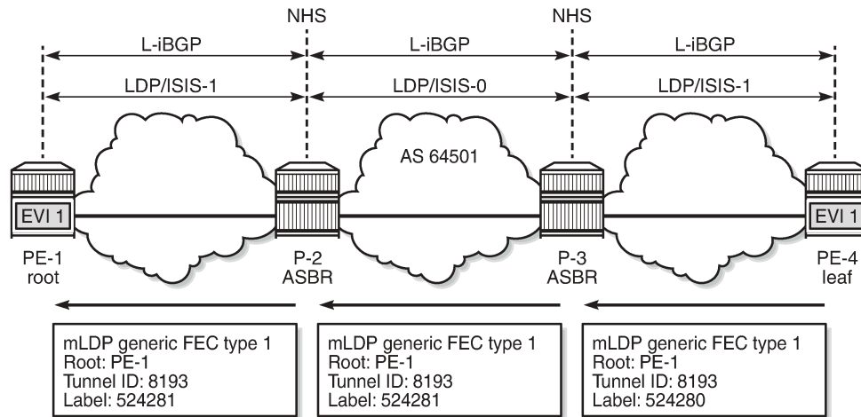
Figure 230: ABRs and leaf node send basic FEC in seamless MPLS
