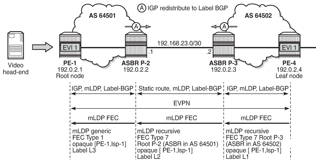
Figure 231: Inter-AS Model C for P2MP mLDP
