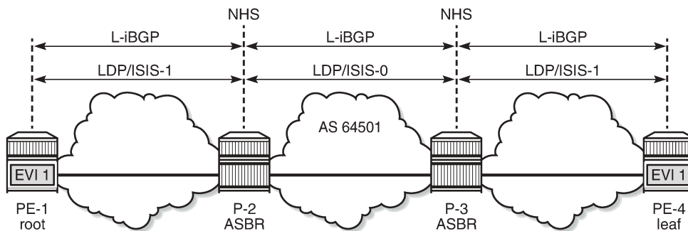
Figure 227: Example topology for seamless MPLS
