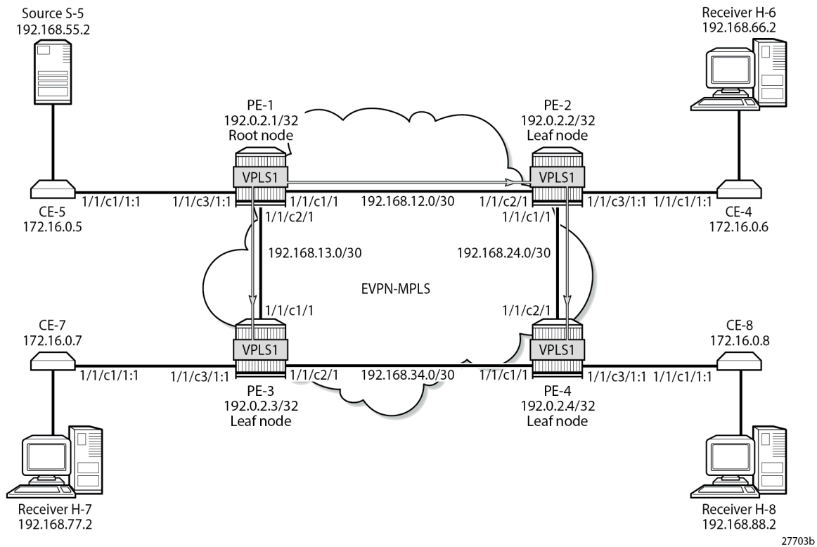
Figure 260: P2MP mLDP Multicast Tree
