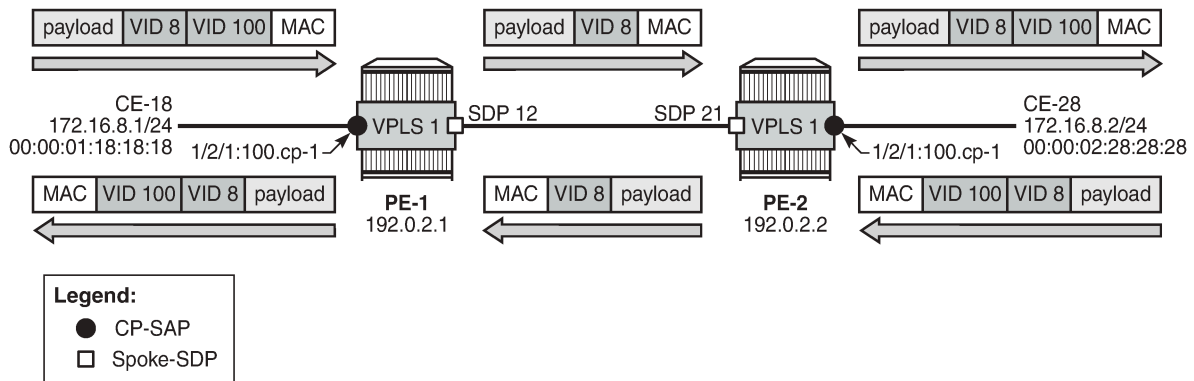
Figure 303: Customer VID is preserved between QinQ CP SAPs - no VLAN translation
