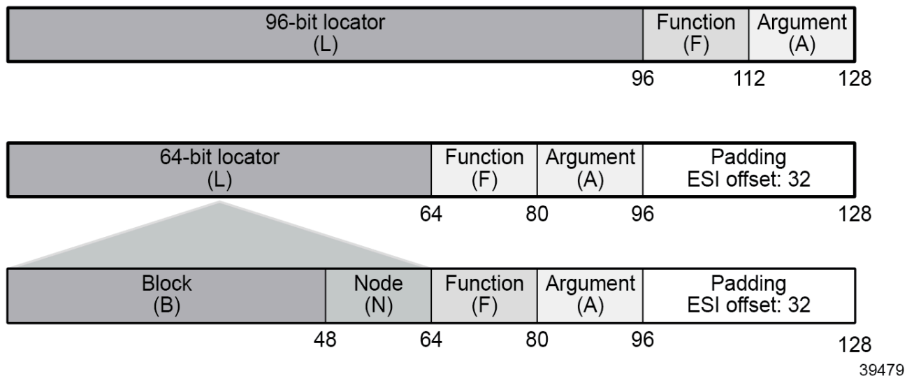
Figure 122: SRv6 SID encoding
