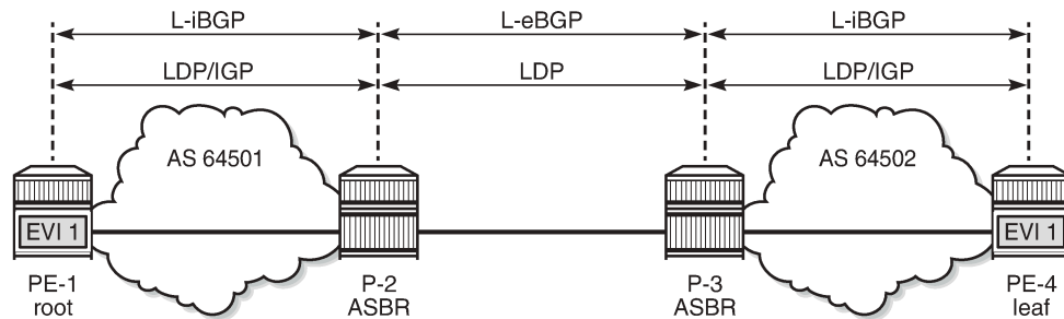
Figure 221: Example topology for inter-AS model C
