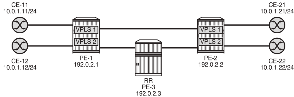
Figure 174: BGP-VPLS with auto-GRE spoke-SDPs
