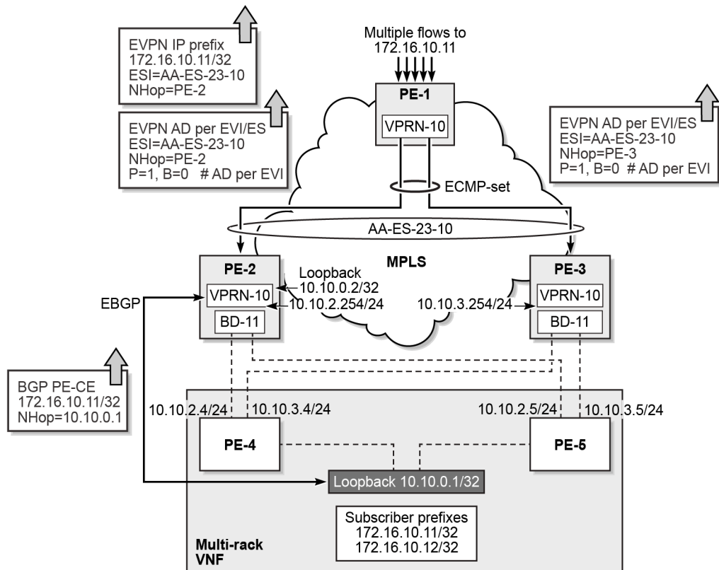
Figure 104: EVPN IP alias for EVPN IFL VPRN-10 over MPLS
