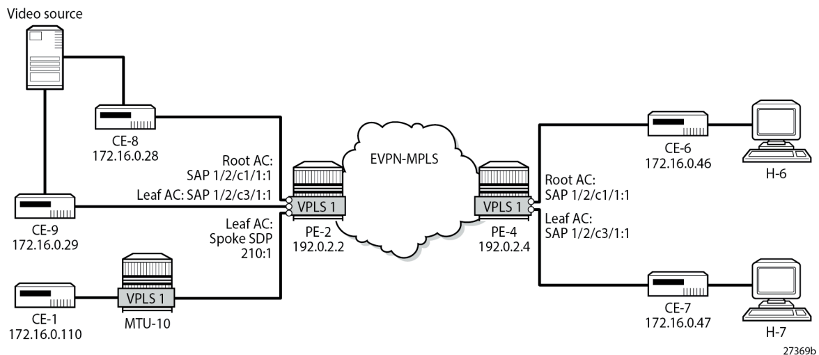
Figure 150: Example Topology for EVPN-MPLS E-Tree without Multi-homing
