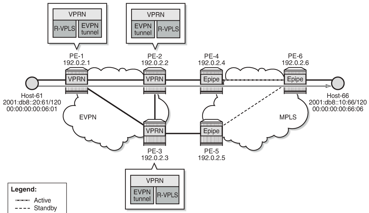
Figure 196: Example topology for initial forwarding path via PE-2 with IPv6 addresses
