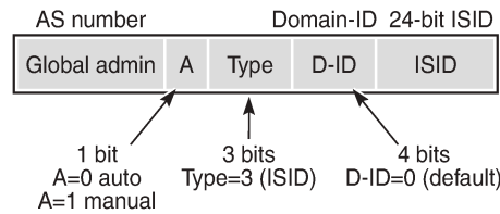
Figure 248: PBB-EVPN ISID-based RT format
