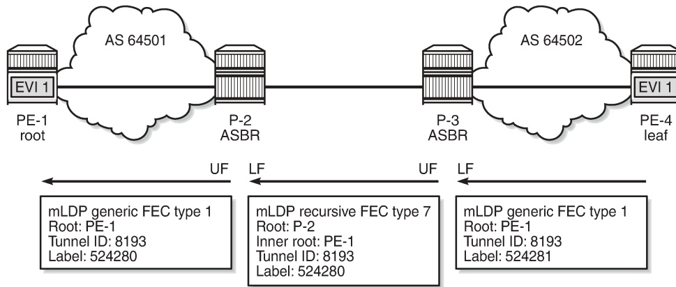
Figure 226: Non-recursive mLDP FEC for inter-AS model C
