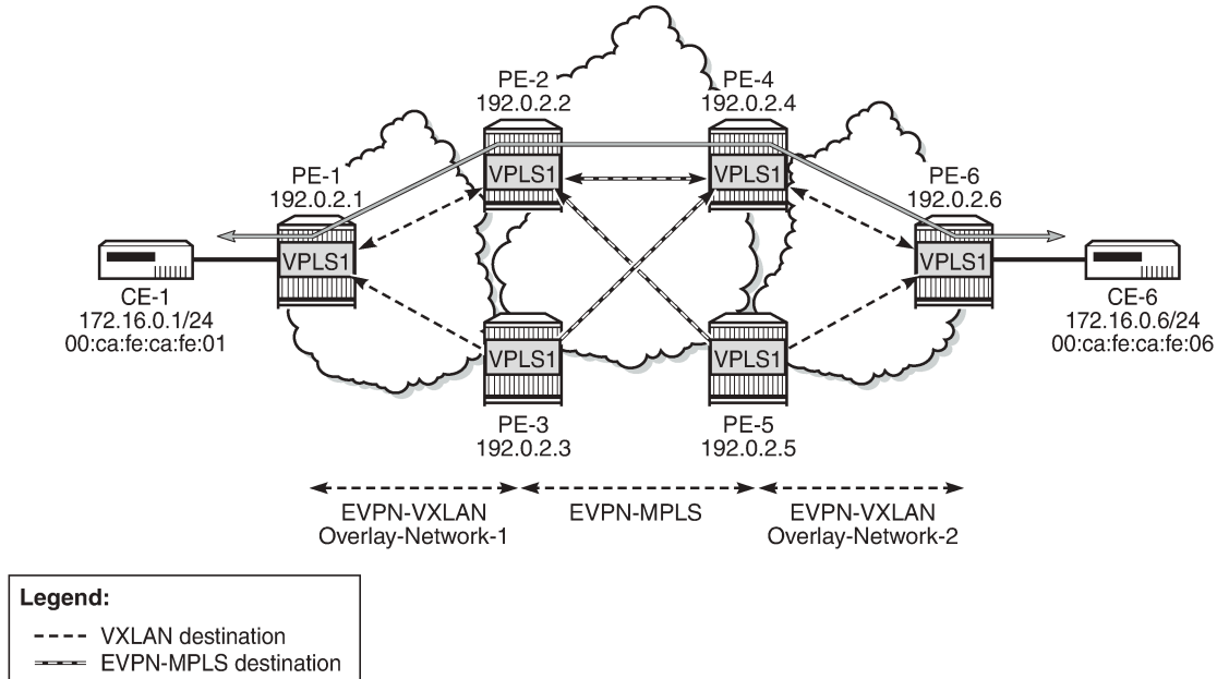
Figure 154: EVPN destinations created on multi-homed anycast DC GWs
