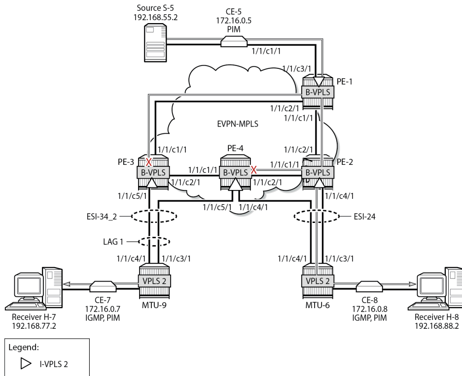
Figure 277: PBB-EVPN with MH and PIM Snooping – Receiver H-8 Joined
