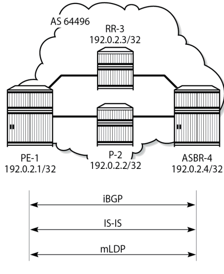
Figure 47: AS 64496 Protocols
