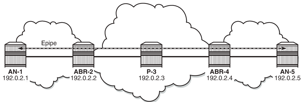
Figure 116: End-to-End Epipe service
