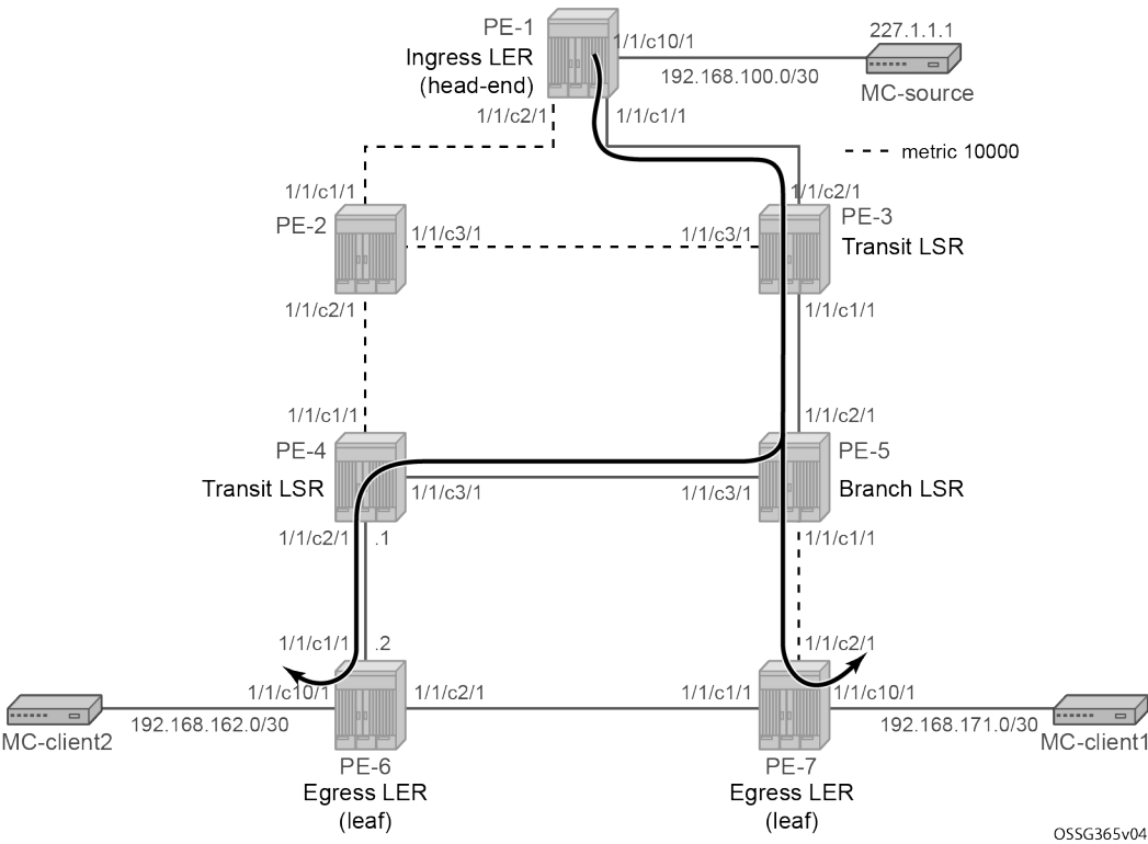
Figure 109: P2MP LSP LSP-p2mp-1 with strict S2L path toward PE-7
