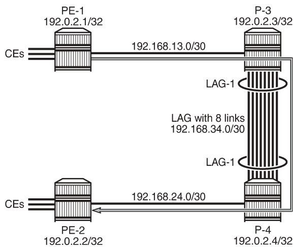
Figure 43: RSVP LSP "LSP-PE-1-PE-2" from PE-1 to PE-2 via P-3 and P-4
