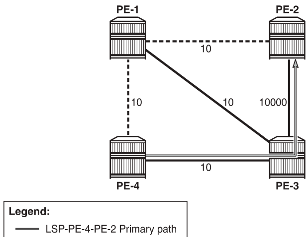
Figure 145: FRR one-to-one only supported on numbered interfaces
