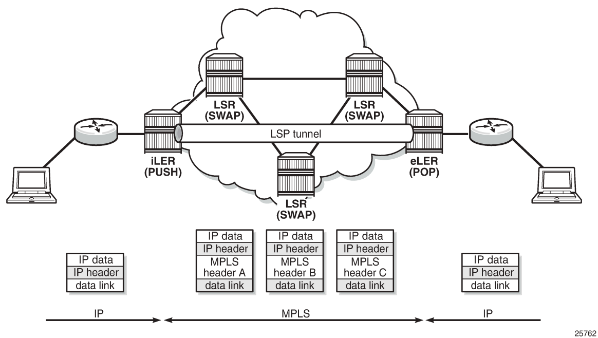
Figure 125: Generic MPLS network, MPLS label operations shows a general network topology clarifying the MPLS-related terms. A Label Edge Router (LER) is a device at the edge of an MPLS network, with at least one interface outside the MPLS domain. A router is usually defined as an LER based on its position relative to a particular LSP. The MPLS router at the head-end of an LSP is called the ingress label edge router (iLER). The MPLS router at the tail-end of an LSP is called the egress label edge router (eLER).
