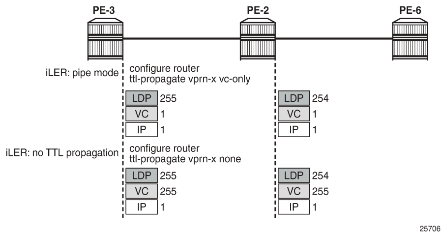
Figure 138: UDP traceroute in VPRN without TTL propagation to LDP
