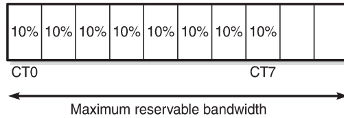
Figure 24: Bandwidth reservation for the CTs
