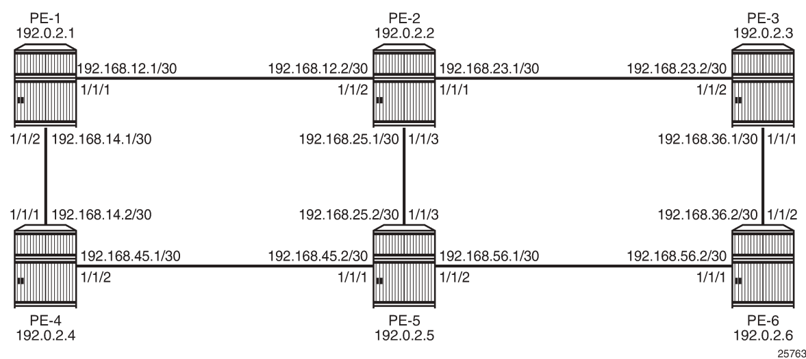
Figure 112: MPLS example topology
