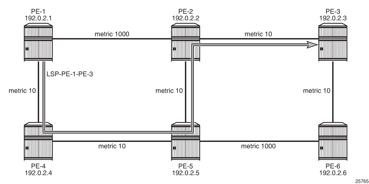
Figure 84: LSP with dynamic path takes IGP best route
