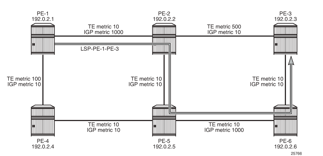
Figure 85: RSVP-TE LSP with dynamic path using TE metric
