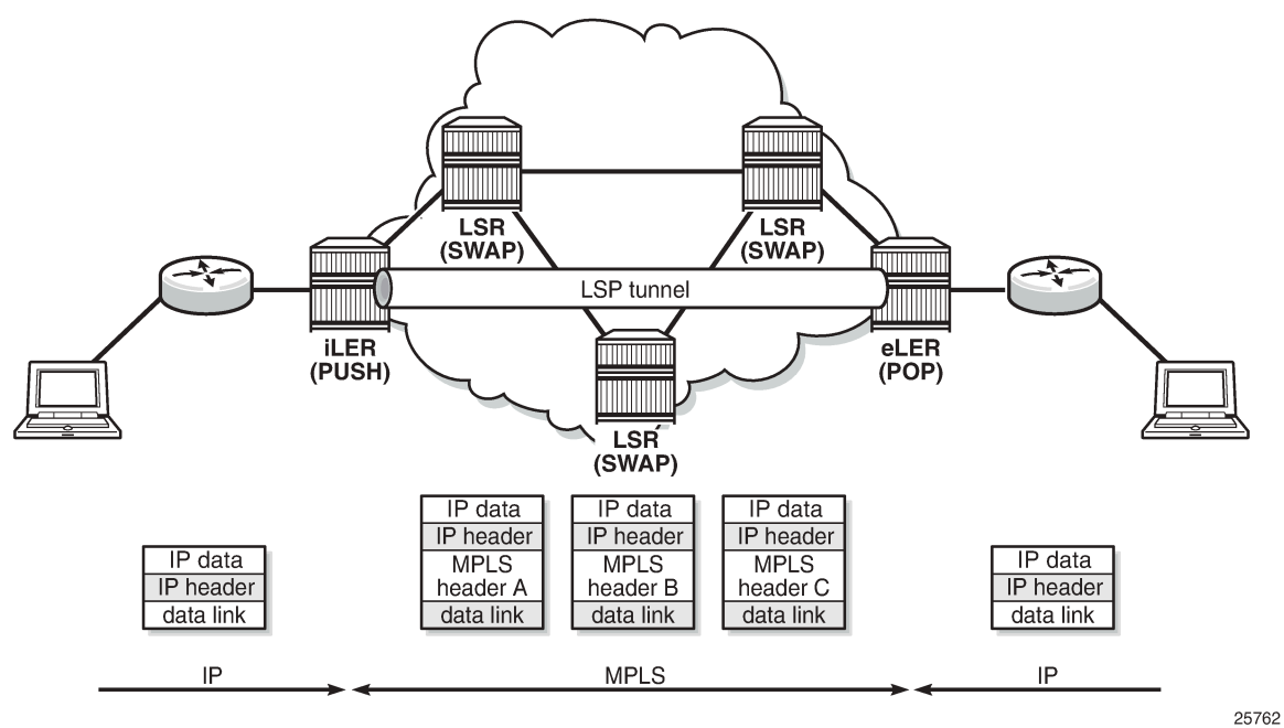
Figure 111: Generic MPLS network, MPLS label operations shows a general network topology clarifying the MPLS-related terms. A Label Edge Router (LER) is a device at the edge of an MPLS network, with at least one interface outside the MPLS domain. A router is usually defined as an LER based on its position relative to a particular LSP. The MPLS router at the head-end of an LSP is called the ingress label edge router (iLER). The MPLS router at the tail-end of an LSP is called the egress label edge router (eLER).
