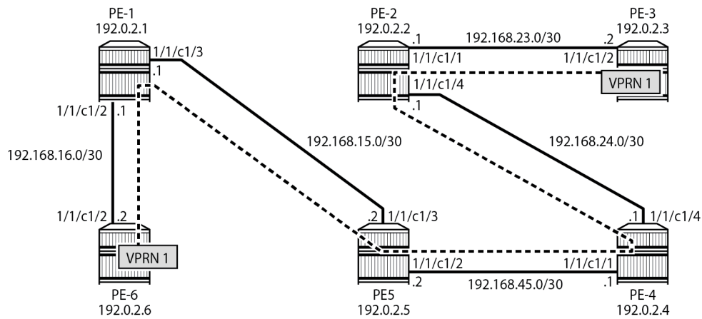
Figure 125: Tunnel from iLER PE-3 to eLER PE-6 with multiple LSRs
