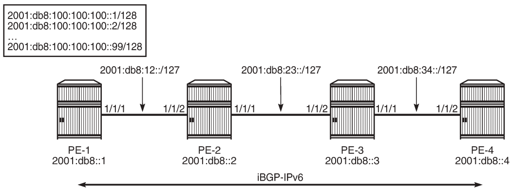
Figure 81: BGP-IPv6
