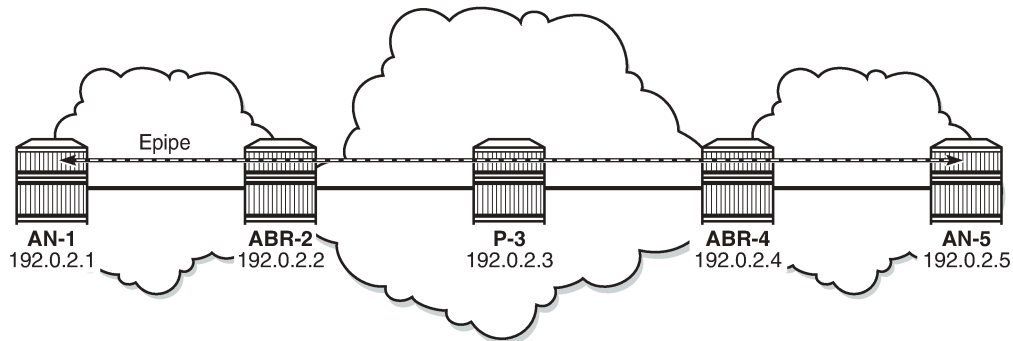
Figure 102: End-to-End Epipe service
