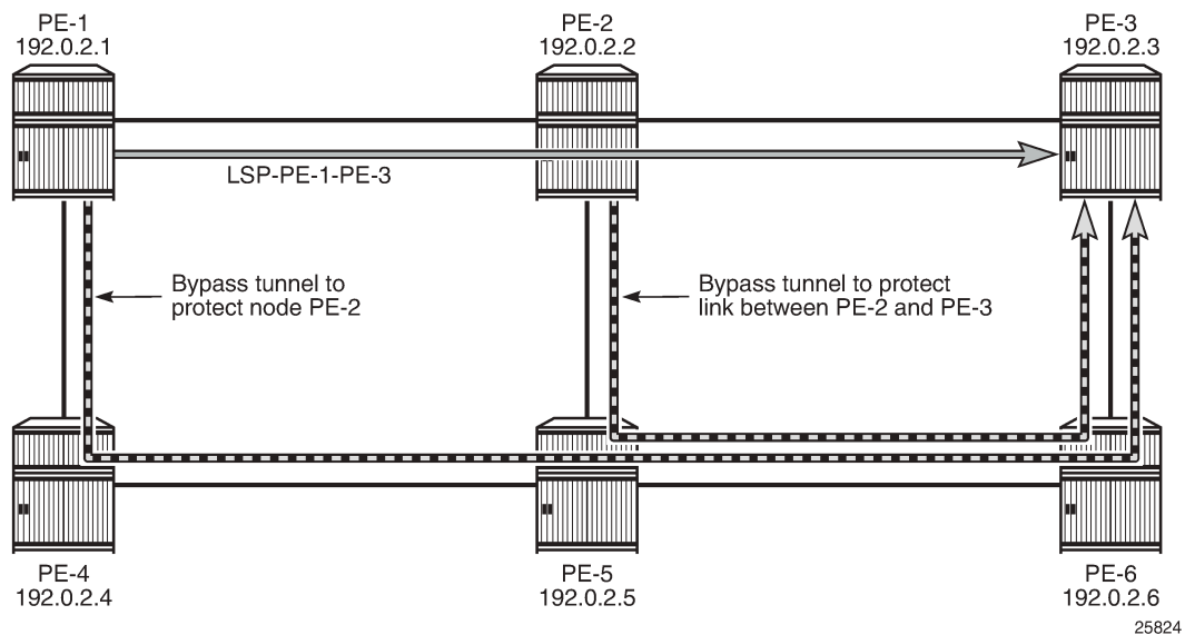
Figure 87: FRR facility bypass tunnels
