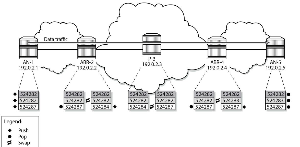
Figure 104: Label stacks for traffic from AN-1 to AN-5
