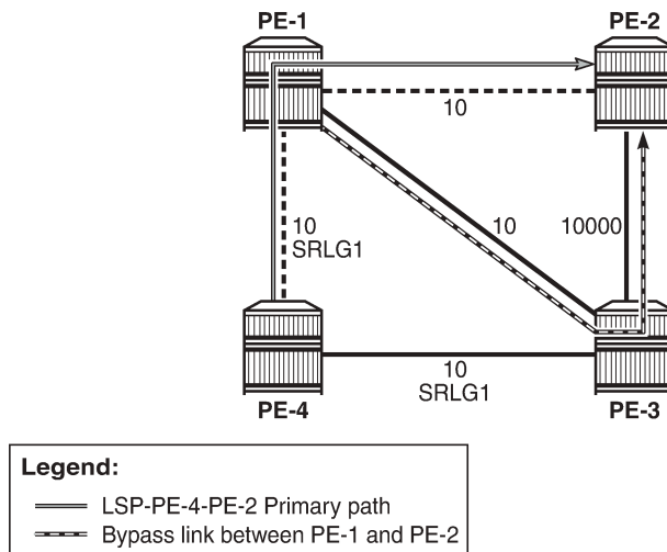
Figure 134: SRLG-FRR strict: no bypass on PE-4
