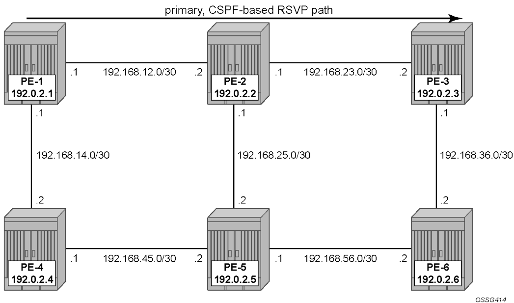
Figure 107: RSVP-TE LSP primary path
