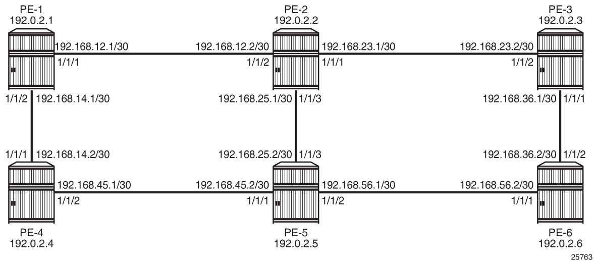
Figure 83: MPLS example topology
