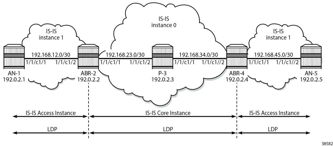
Figure 100: Seamless MPLS - IGP/LDP domains
