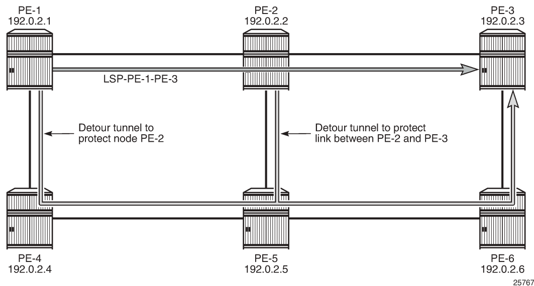
Figure 86: Fast reroute one-to-one detour tunnels
