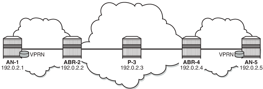
Figure 103: L3 VPN service
