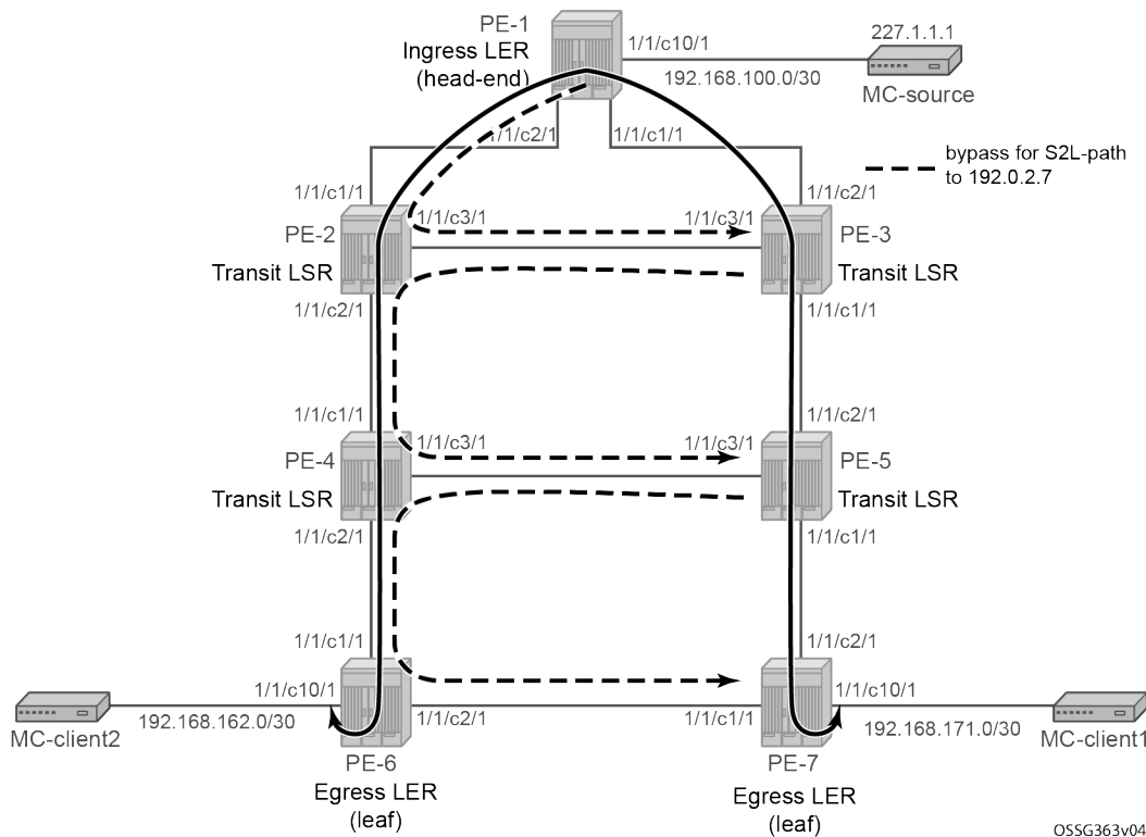
Figure 93: P2MP LSP LSP-p2mp-1 with bypass tunnels
