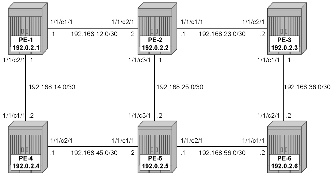
Figure 105: Example topology
