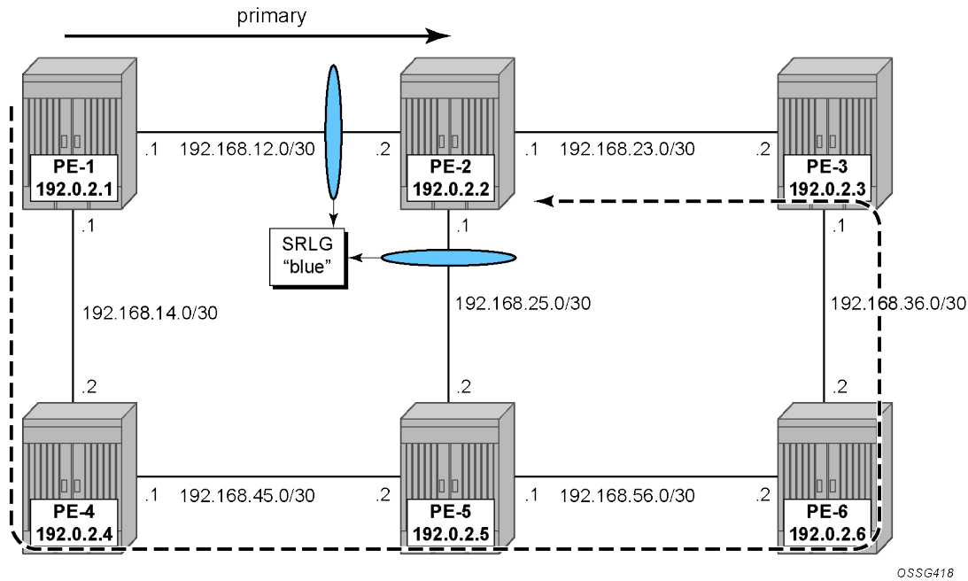
Figure 109: SRLG for secondary path
