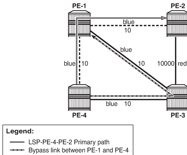
Figure 133: FRR facility and admin groups
