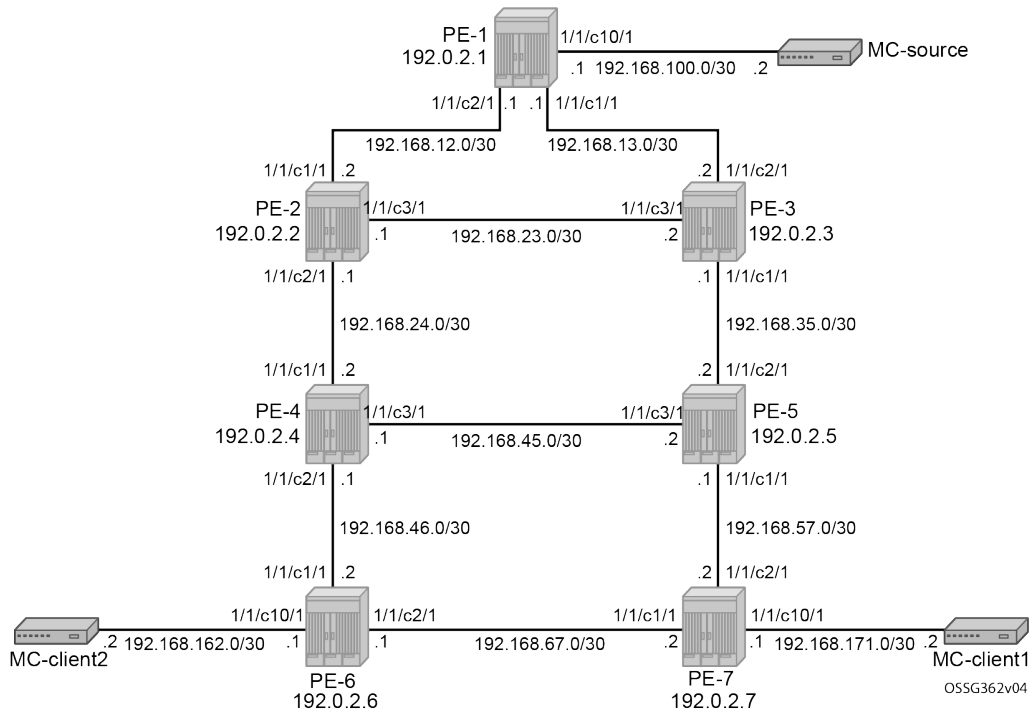
Figure 92: P2MP example topology
