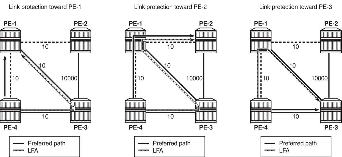
Figure 135: LDP FRR LFA link protection on PE-4
