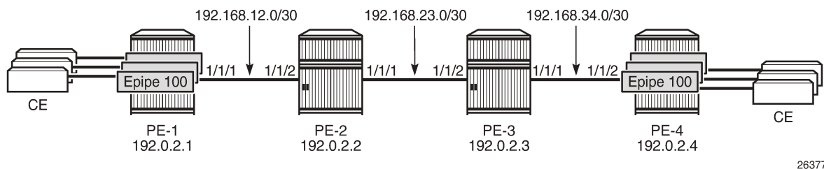
Figure 78: Multiple Epipes Using LDP SDPs
