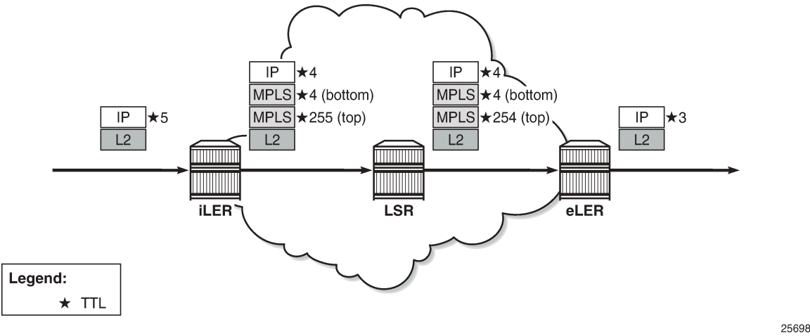
Figure 116: Use of TTL in an L3 VPN service in pipe mode
