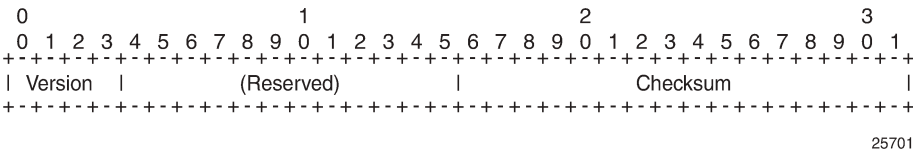
Figure 119: ICMP extension header
