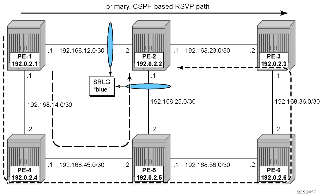
Figure 108: FRR bypass tunnels originating in PE-1 with and without SRLG
