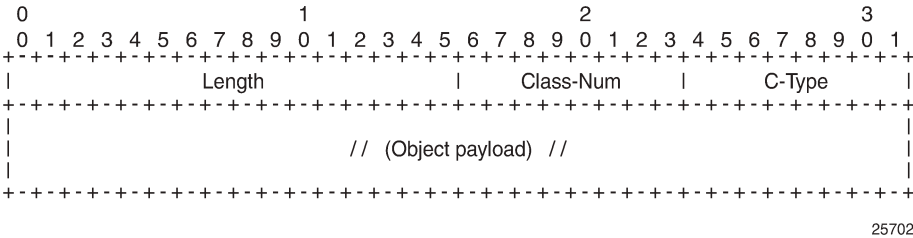
Figure 120: ICMP extension object: object header and payload
