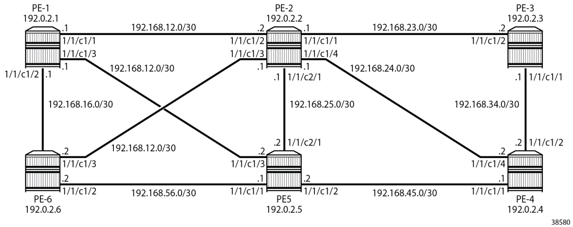
Figure 121: Example configuration
