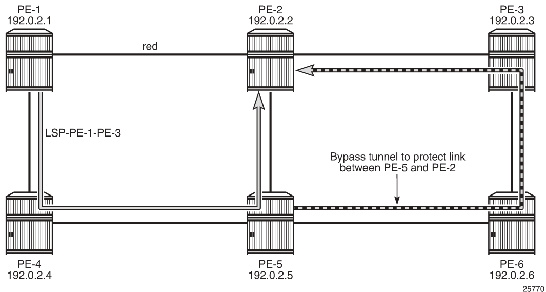
Figure 91: LSP and FRR bypass tunnel excluding admin group 'red'
