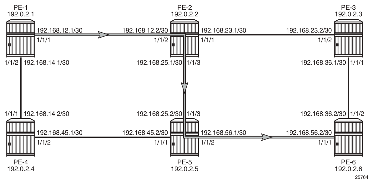
Figure 113: Static LSP running over PE-1, PE-2, PE-5, PE-6
