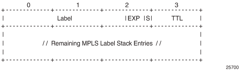
Figure 118: MPLS label stack object
