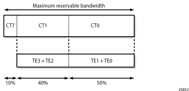
Figure 18: MAM bandwidth allocation
