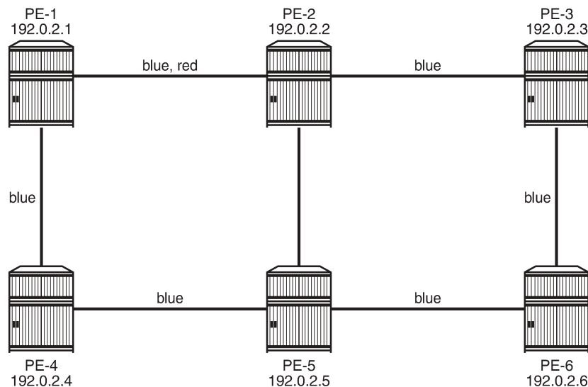
Figure 89: Admin groups 'blue' and 'red'
