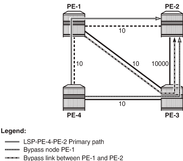
Figure 130: LSP and FRR facility bypass tunnels
