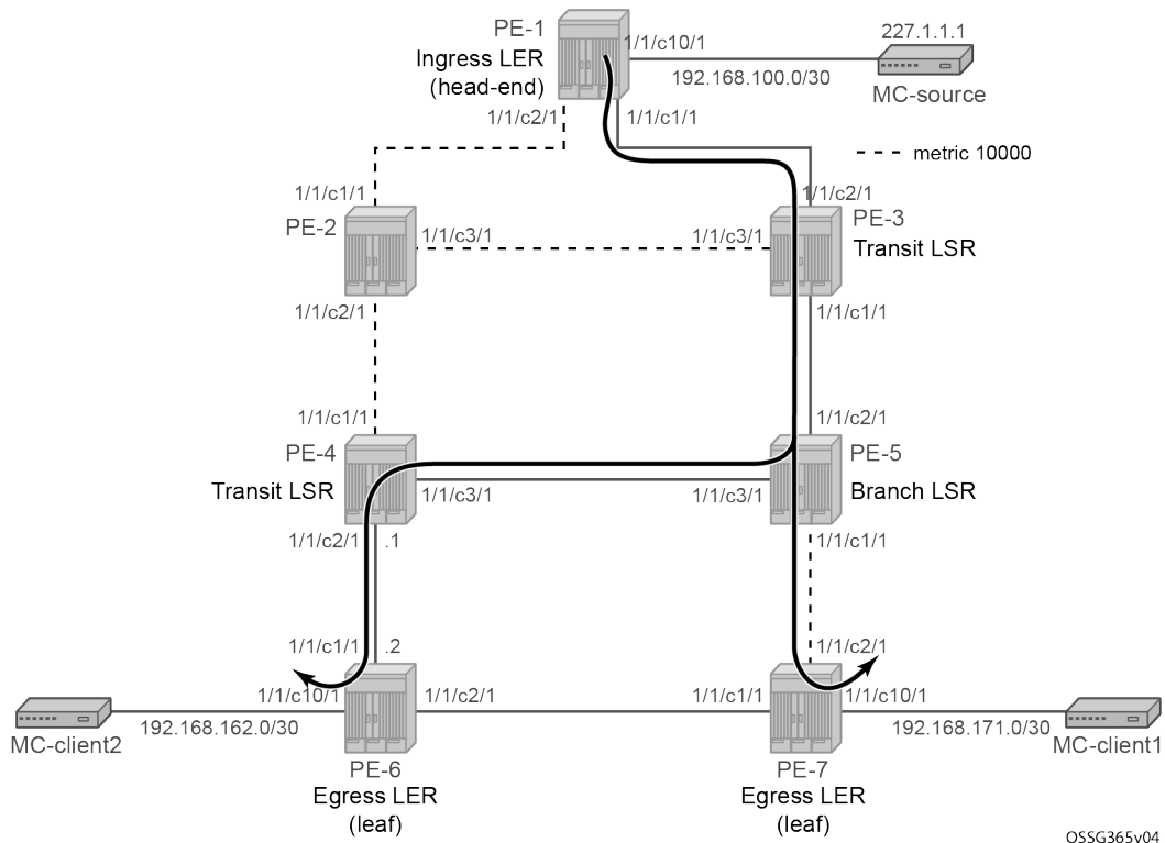
Figure 95: P2MP LSP LSP-p2mp-1 with strict S2L path toward PE-7
