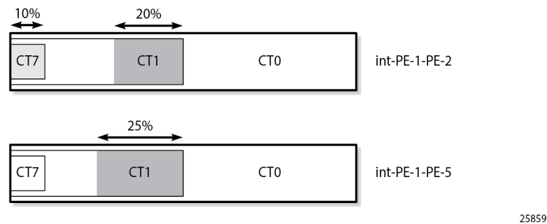
Figure 25: Reserved bandwidth on both interfaces of PE-1 (three sessions)
