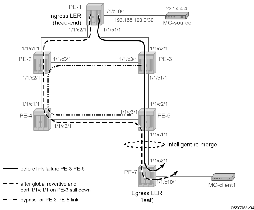
Figure 98: Intelligent remerge, case 3
