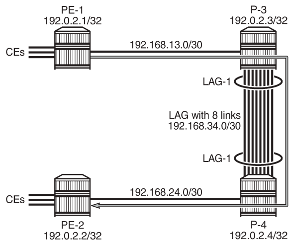
Figure 33: RSVP LSP "LSP-PE-1-PE-2" from PE-1 to PE-2 via P-3 and P-4
