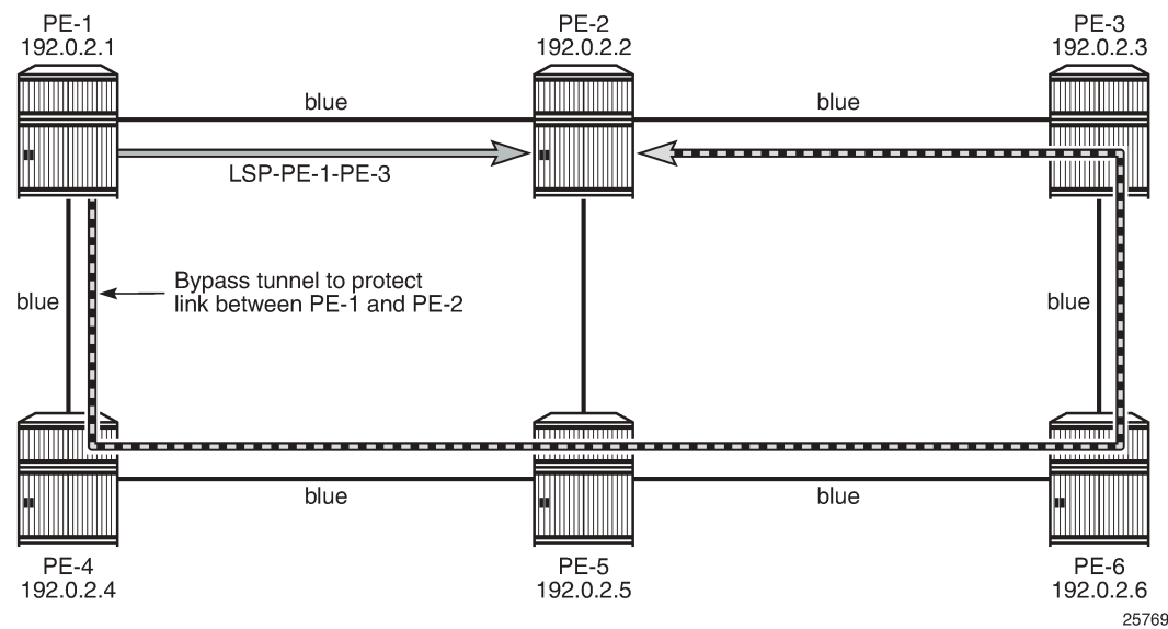
Figure 90: LSP and bypass within admin group 'blue'
