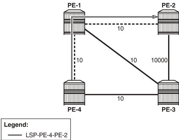
Figure 129: LSP-PE-4-PE-2 on unnumbered interfaces
