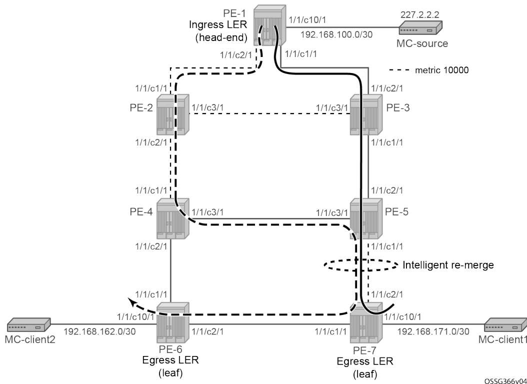
Figure 96: Intelligent remerge, case 1
