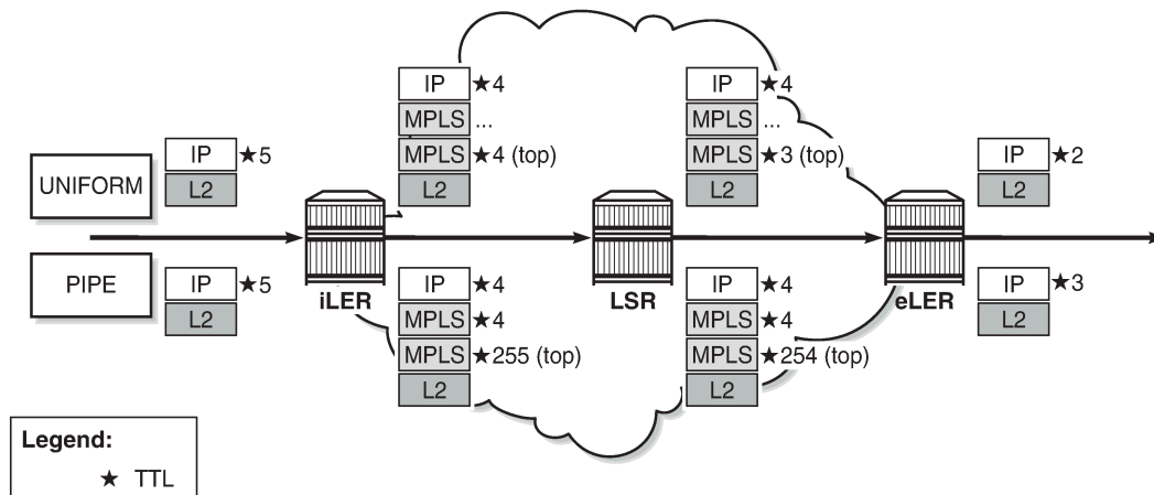
Figure 114: Use of TTL: uniform versus pipe
