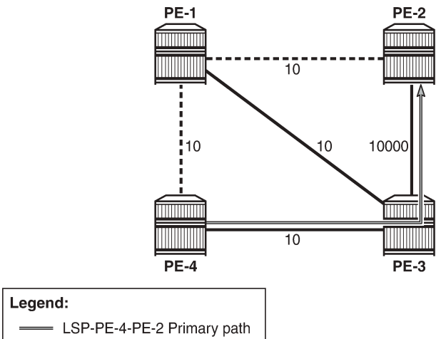
Figure 131: FRR one-to-one only supported on numbered interfaces
