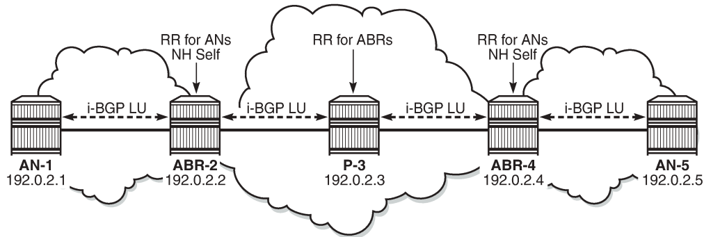
Figure 101: Seamless MPLS - BGP
