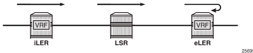
Figure 117: Tunneling of ICMP reply packets over an MPLS LSP
