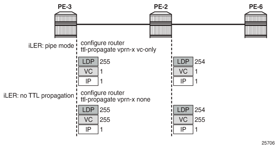
Figure 124: UDP traceroute in VPRN without TTL propagation to LDP
