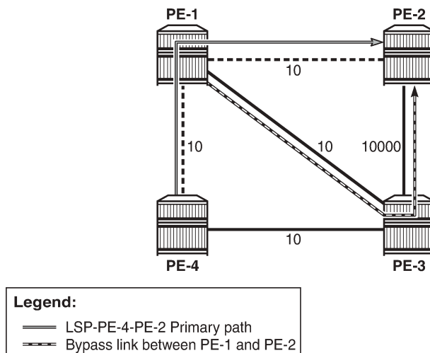
Figure 132: FRR on iLER: no bypass on unnumbered interfaces
