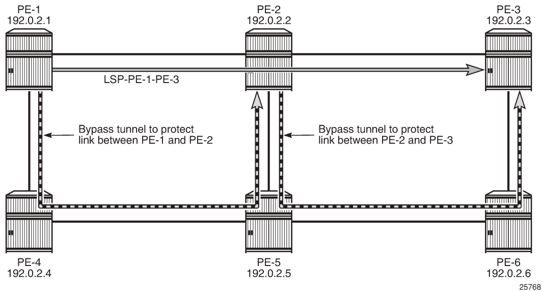
Figure 88: FRR facility without node protection
