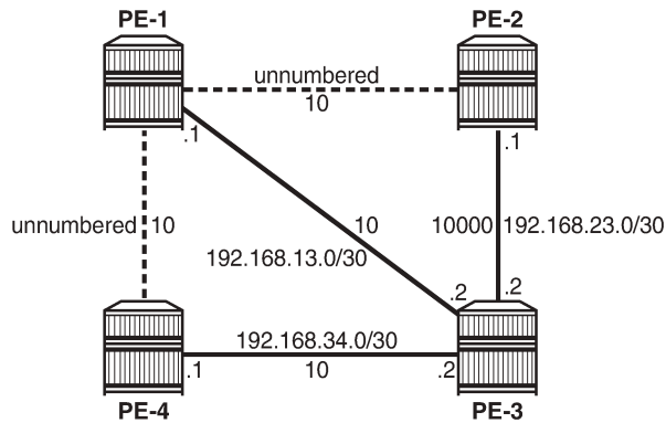
Figure 128: Configuration example for unnumbered Interfaces in RSVP and LDP
