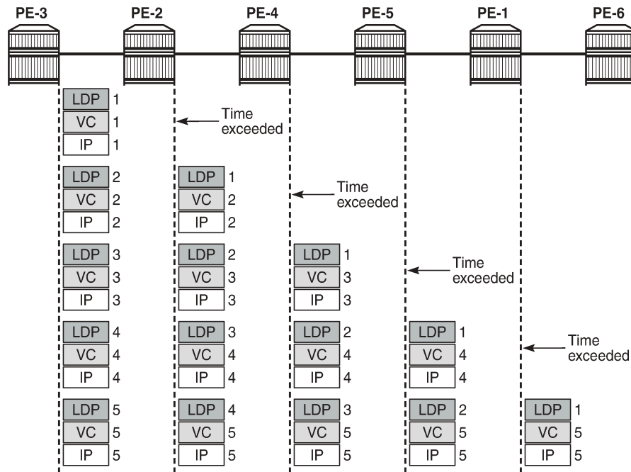
Figure 126: UDP traceroute with iLER in uniform mode
