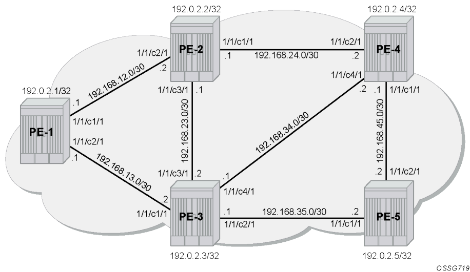
Figure 63: Initial example topology
