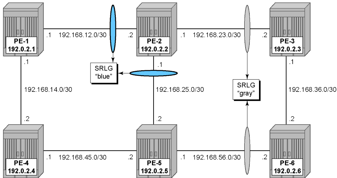
Figure 106: SRLG topology
