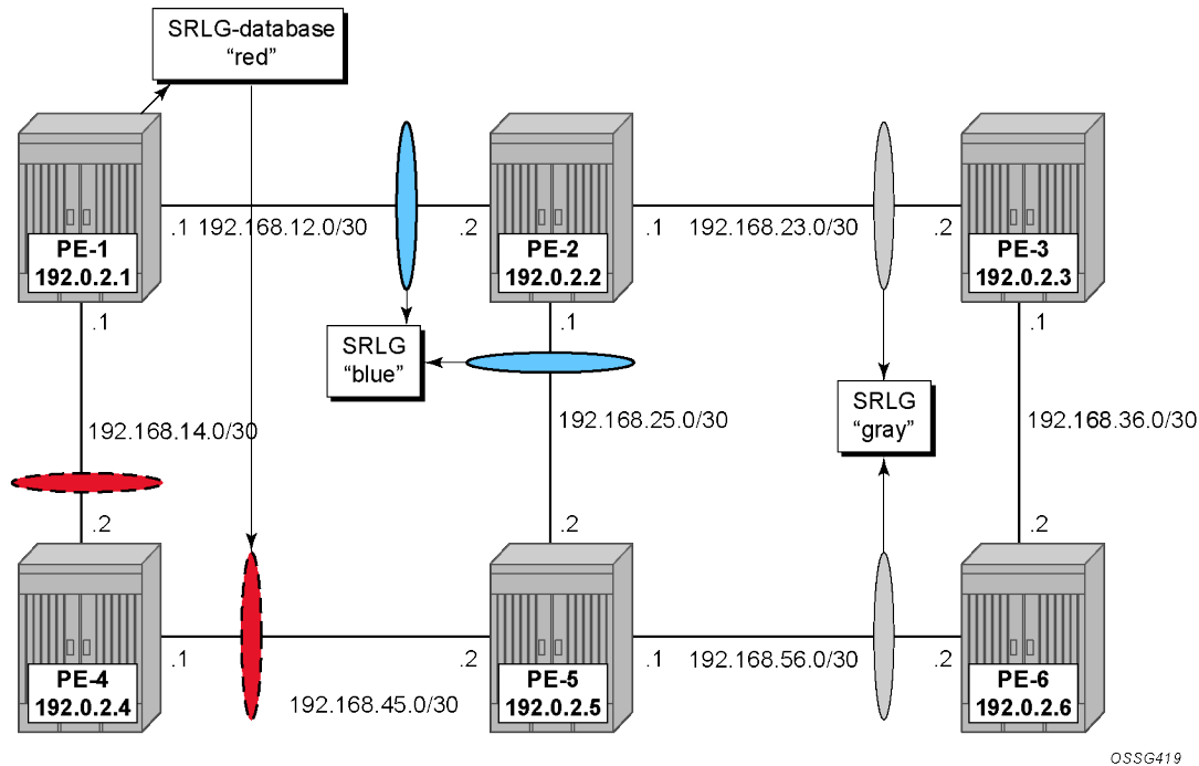
Figure 110: SRLG database example
