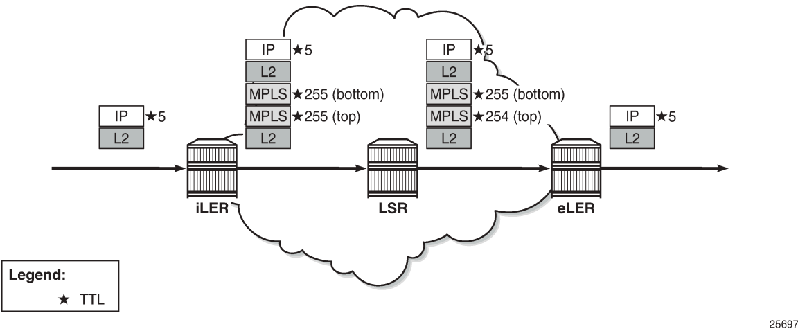
Figure 115: Use of TTL in an L2 VPN service in pipe mode
