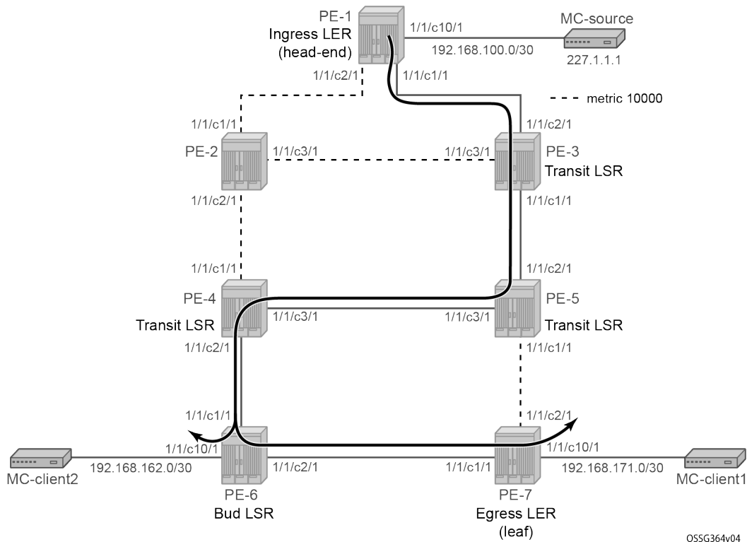
Figure 94: P2MP LSP p-to-mp-1 with metric change
