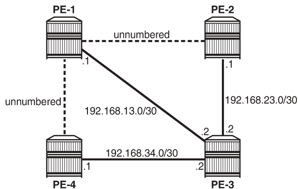
Figure 127: Example topology for unnumbered interfaces in RSVP and LDP
