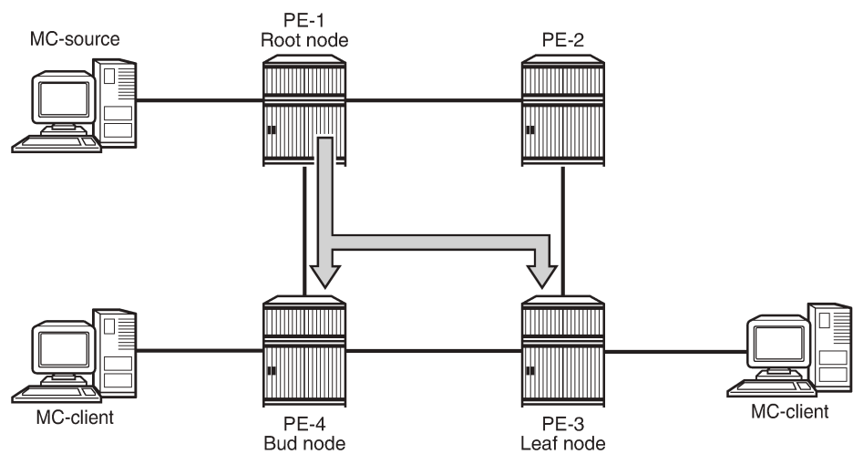
Figure 71: New LDP P2MP LSP after metric change
