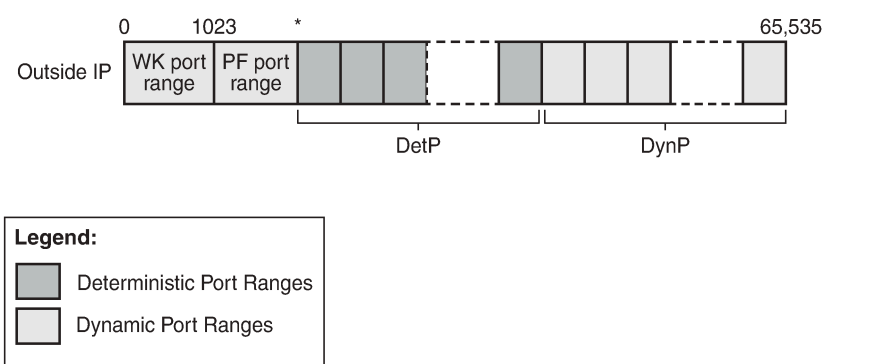
Figure 55: Deterministic mapping: outside IP port-blocks/ranges
