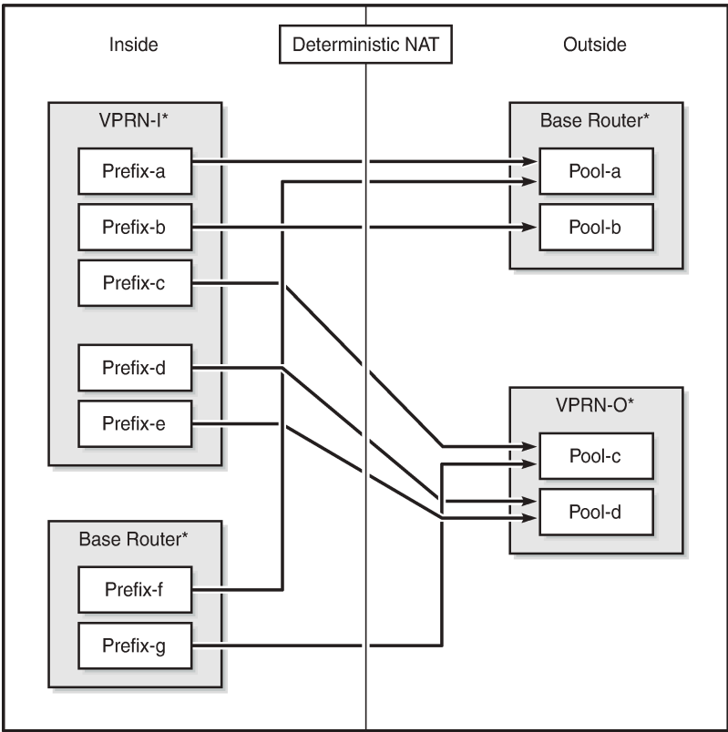
Figure 54: Deterministic mapping: inside -> outside routing instances
