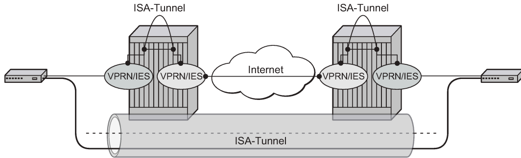
Figure 68: Implementation
