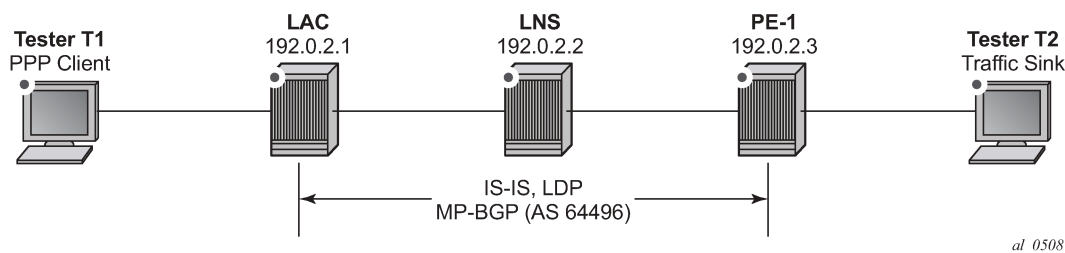
Figure 77: Example Topology
