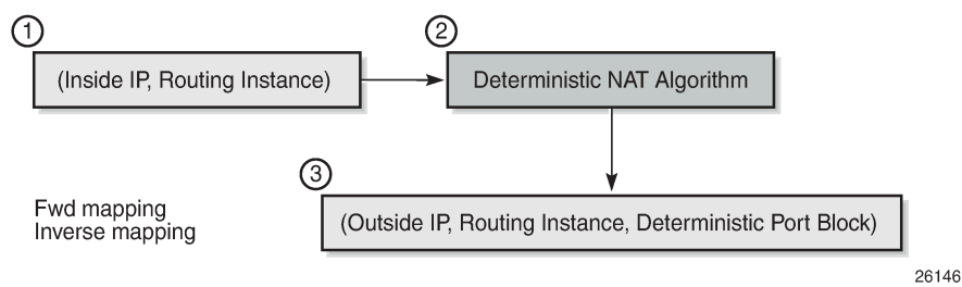
Figure 53: Deterministic NAT algorithm
