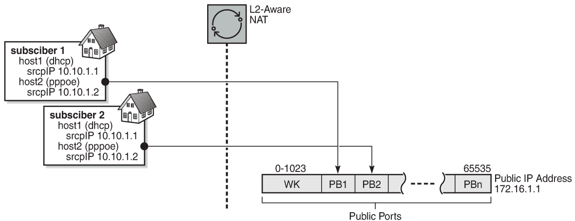
Figure 74: NAT Binding
