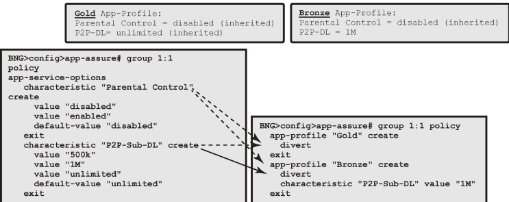
Figure 11: Service tier example using ASO, app-profile and AQP
