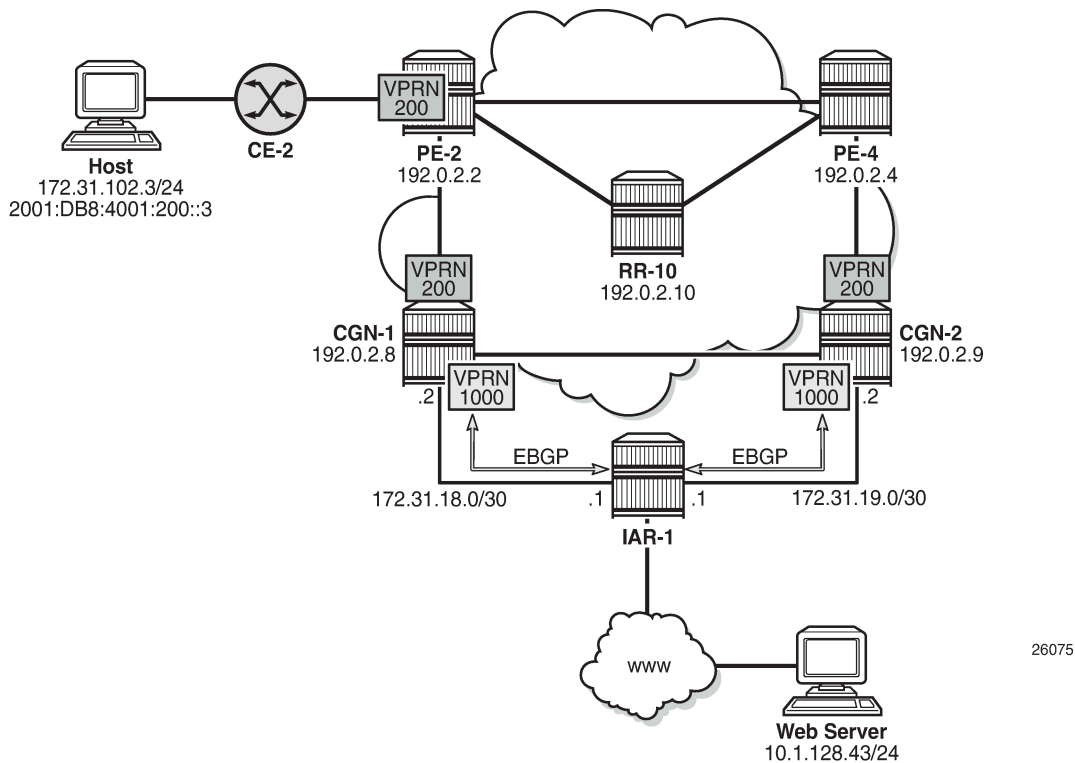
Figure 81: Example Topology
