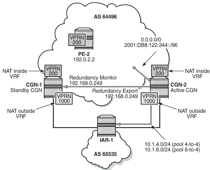
Figure 82: Redundancy Status
