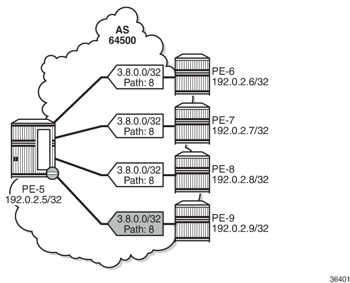
Figure 57: BGP multipath for the label-IPv4 address family
