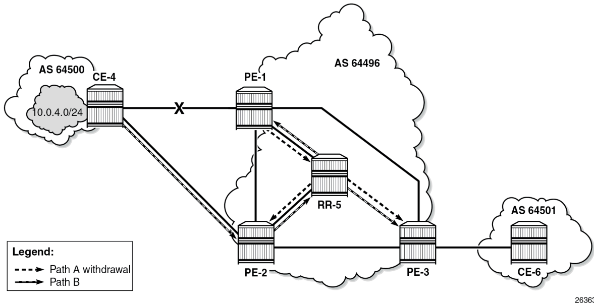
Figure 9: Reconvergence after path failure (without add-path)
