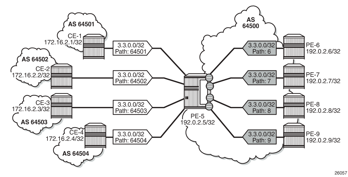
Figure 48: BGP multipath with limit 6 and eBGP preferred
