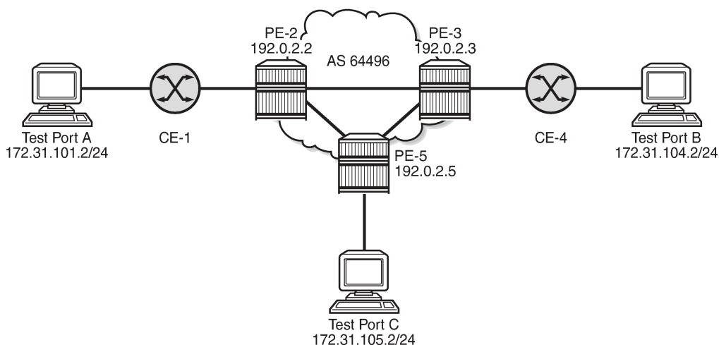
Figure 17: Example topology
