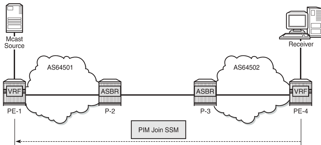
Figure 72: PIM-C Signaling
