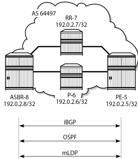
Figure 48: AS 64497 Protocols
