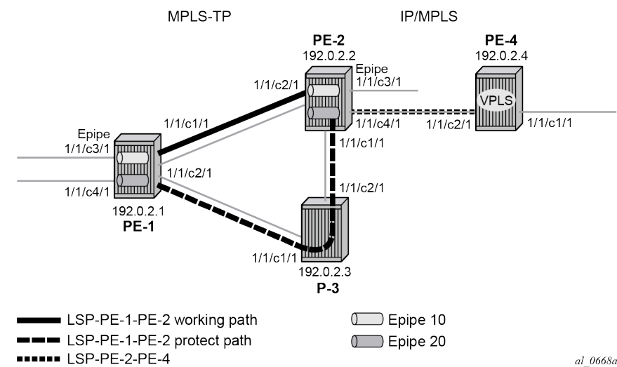
Figure 79: MPLS-TP example network showing services detail shows further details of the logical architecture of the services in the example network. The Epipe spoke-SDPs use the static MPLS-TP transport LSP between PE-1 and PE-2, and the dynamically signaled RSVP-TE LSP between PE-2 and PE-4. The MPLS-TP LSP is protected using 1:1 linear protection, with a working path from PE-1 to PE-2, and a protect path from PE-1, through LSR P-3, to PE-2. The Ethernet PW for Epipe 10 connects an Ethernet SAP on port 1/1/c3/1 on PE-1 to an Ethernet SAP on port 1/1/c3/1 on PE-2. The PW for Epipe 20 connects an Ethernet SAP on port 1/1/c4/1 on PE-1 to the VPLS on PE-4 and is switched between a static MPLS-TP segment and a dynamic targeted LDP (T-LDP) segment at PE-2. PE-2 thus acts as a gateway between the MPLS-TP domain and the IP/MPLS domain.
