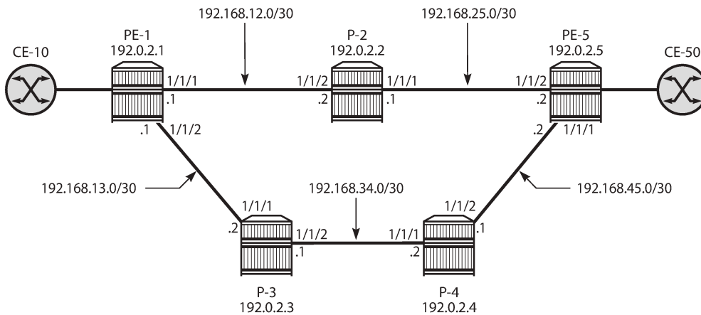
Figure 58: Example topology
