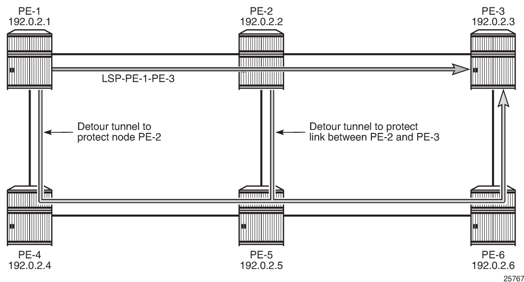
Figure 86: Fast reroute one-to-one detour tunnels
