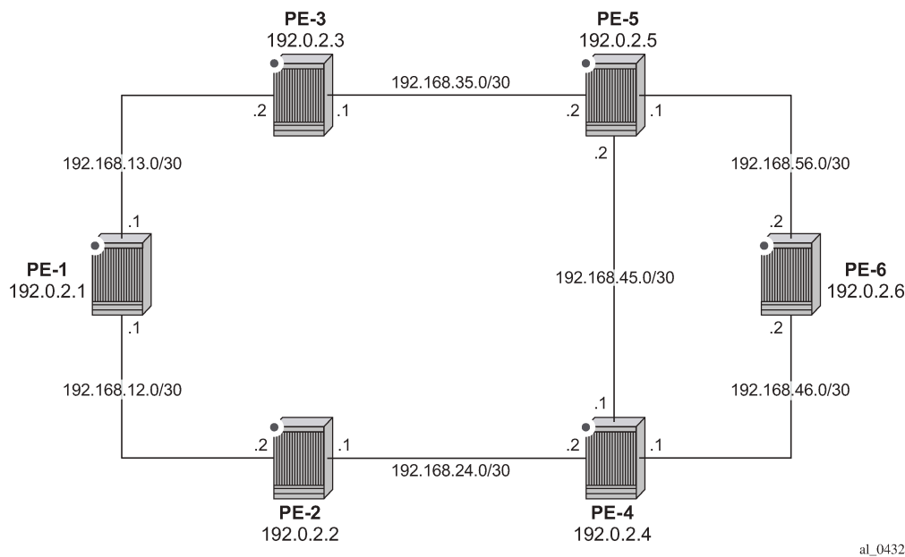
Figure 4: Example Topology
