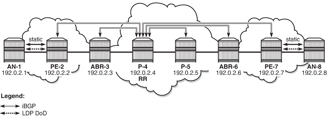
Figure 49: BGP enabled with P-4 as RR
