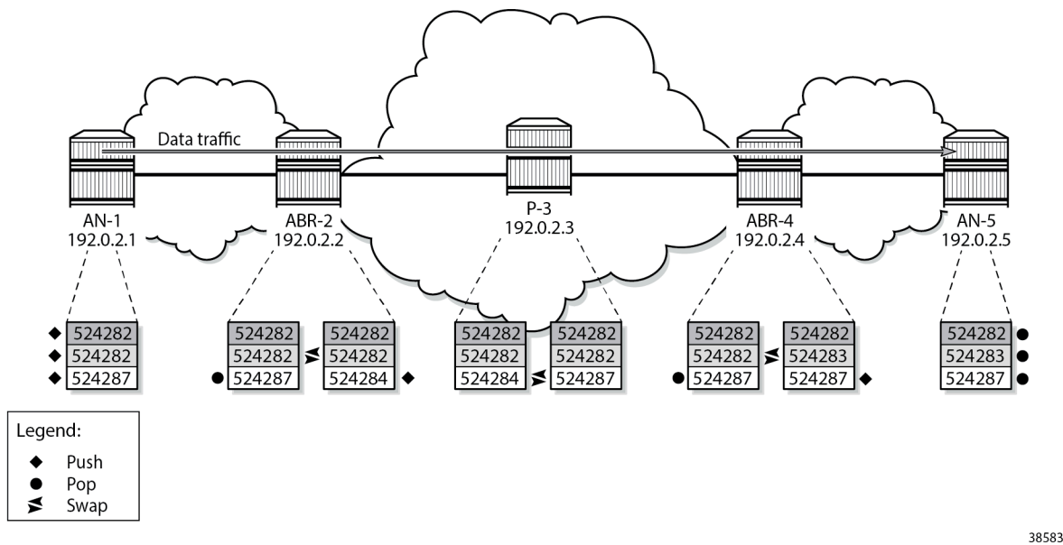
Figure 104: Label stacks for traffic from AN-1 to AN-5
