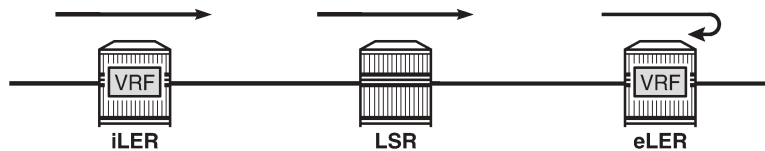
Figure 117: Tunneling of ICMP reply packets over an MPLS LSP
