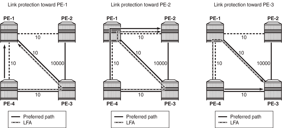
Figure 135: LDP FRR LFA link protection on PE-4
