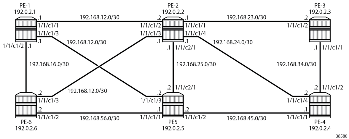
Figure 121: Example configuration
