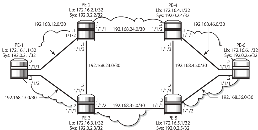
Figure 36: Example Topology
