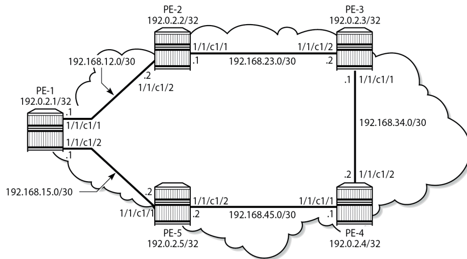
Figure 12: Example topology
