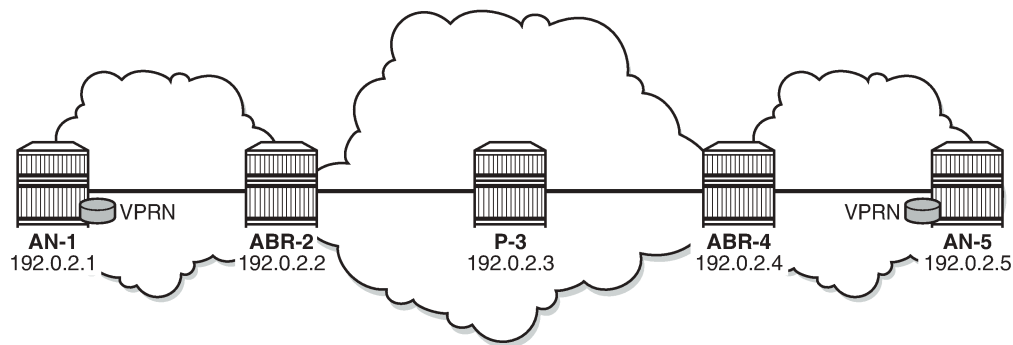
Figure 103: L3 VPN service
