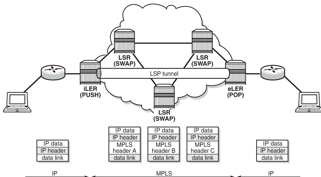
Figure 82: Generic MPLS network, MPLS label operations
