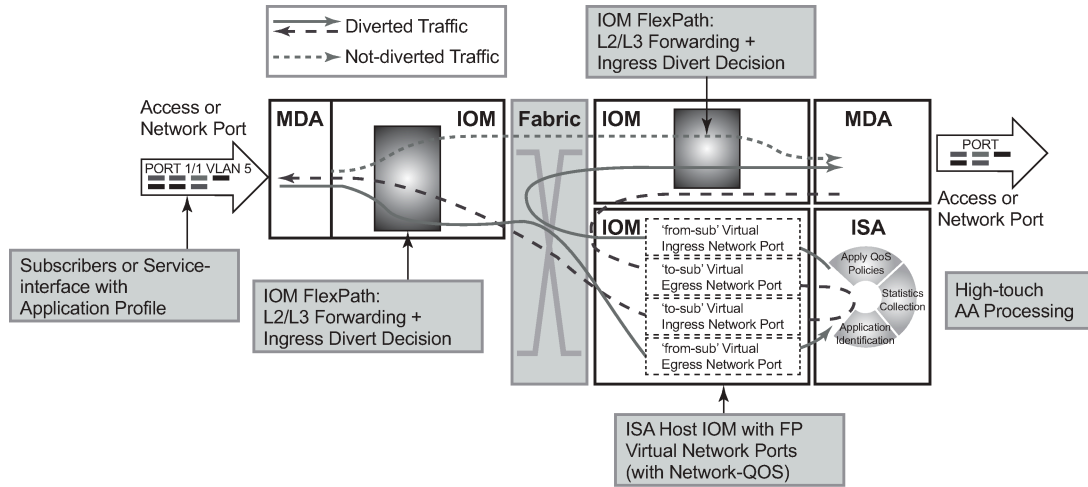
Figure 17: System packet datapath to AA ISA
