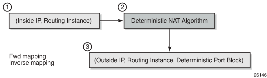
Figure 53: Deterministic NAT algorithm
