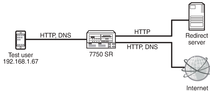
Figure 22: Example setup
