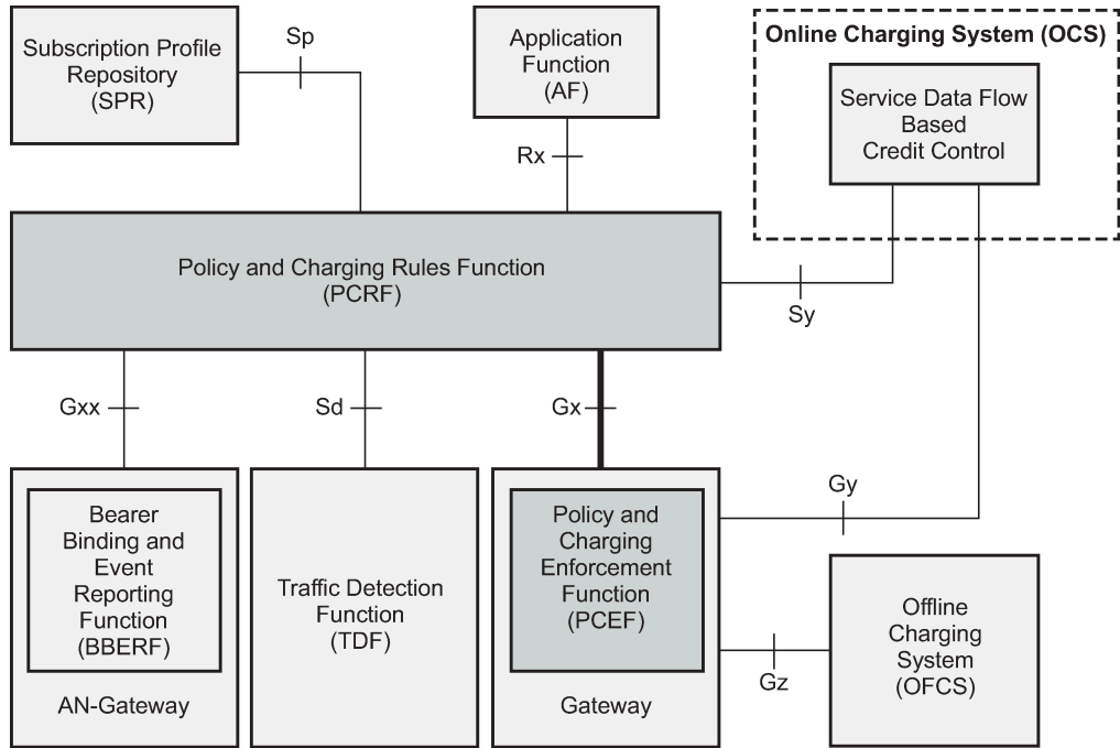
Figure 38: Gx reference point
