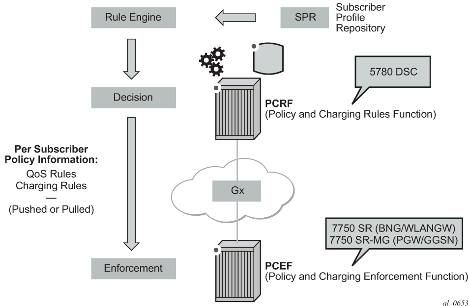
Figure 40: Gx reference point
