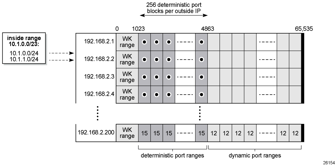
Figure 61: Case 2: Prefix 10.1.0.0/23 results
