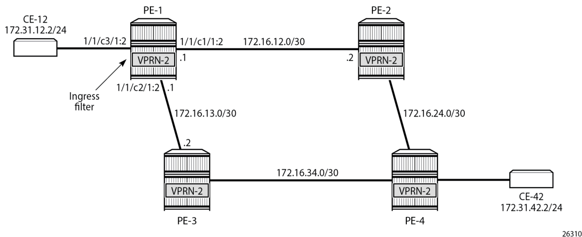
Figure 26: PBR in a VPRN
