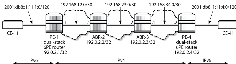
Figure 6: Example topology for seamless MPLS
