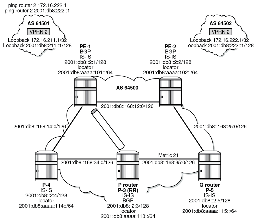
Figure 67: Example topology with metric 21 between P-3 and P-5
