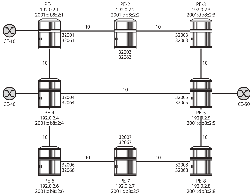
Figure 79: Example topology
