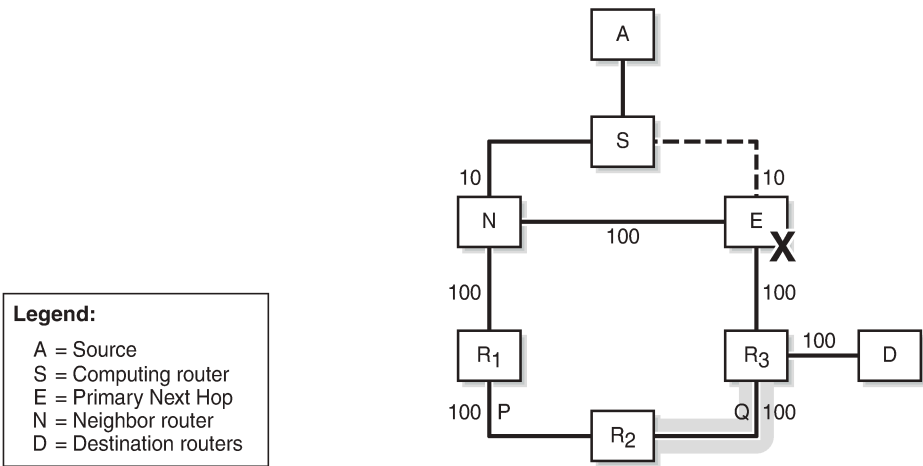
Figure 18: Link protecting Q-space
