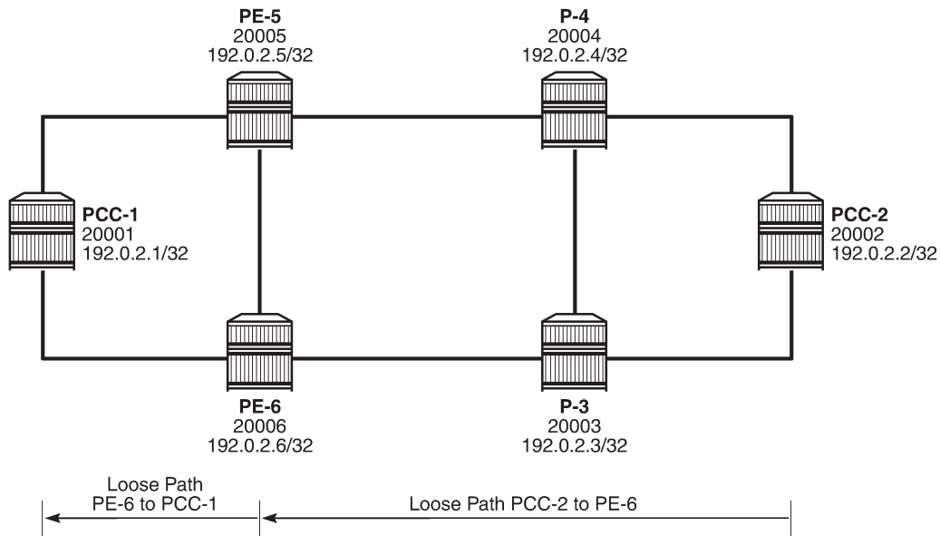
Figure 37: SR-TE LSP with loose path shows the concept of the loose path. The following configures the MPLS path containing a loose hop on PCC-2:
