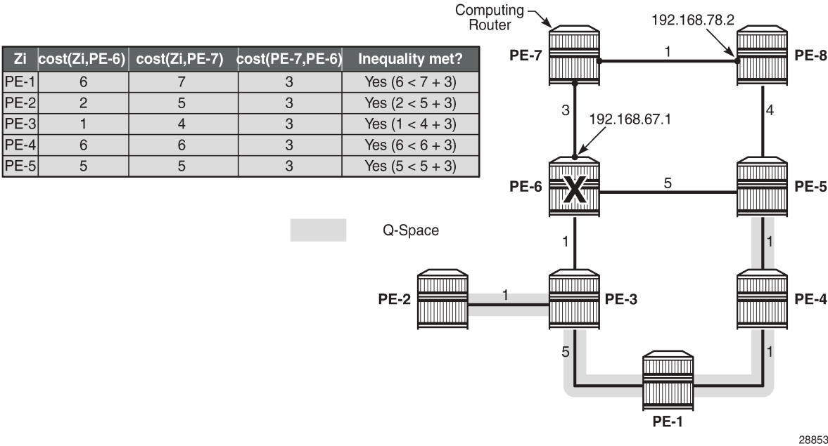
Figure 27: Validating candidate PQ routers - repair tunnel calculation shows that PE-1, PE-4, and PE-5 are the candidate PQ routers for protecting router PE-6. An additional forward SPF run is required for every candidate PQ router, to ensure that the shortest path from that candidate PQ router to destination PE-2 does not traverse the protected router PE-6. The general formula from the Overview section becomes:
