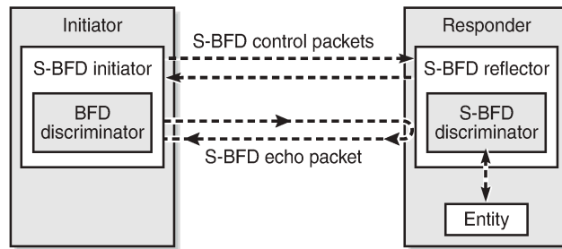
Figure 29: Relationship between S-BFD terms
