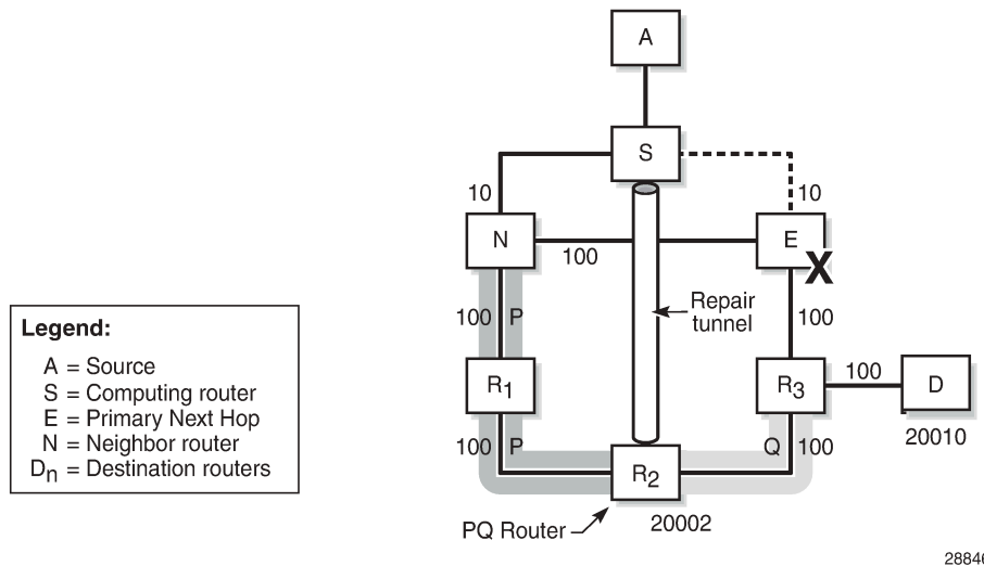
Figure 19: One candidate PQ-router – repair tunnel
