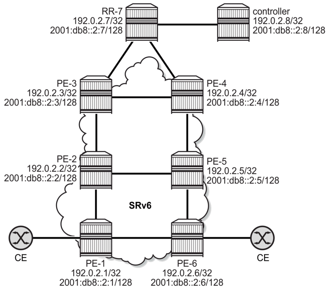
Figure 68: Example topology with system IP addresses
