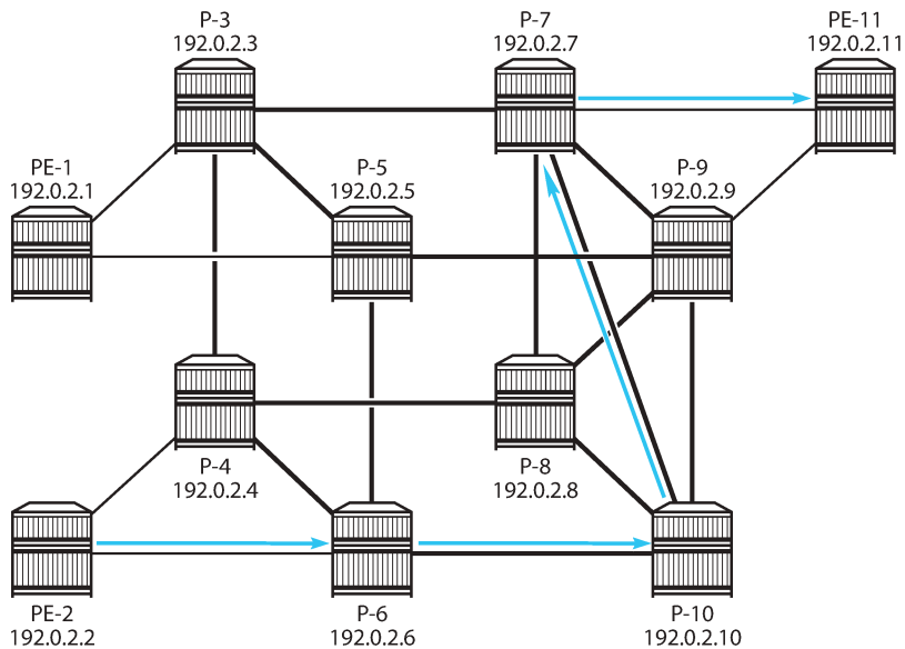
Figure 59: Empty path from PE-2 to PE-11
