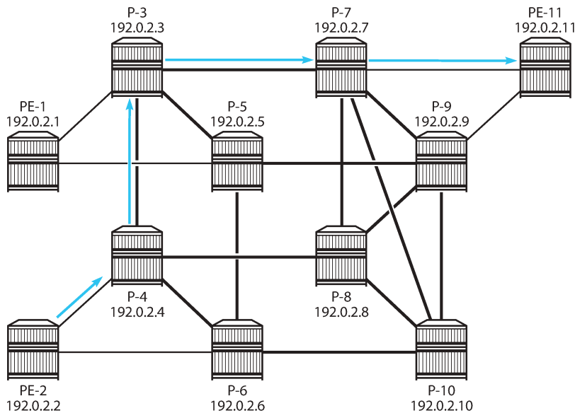
Figure 60: Path from PE-2 to PE-11 via strict hops P-4 and P-3
