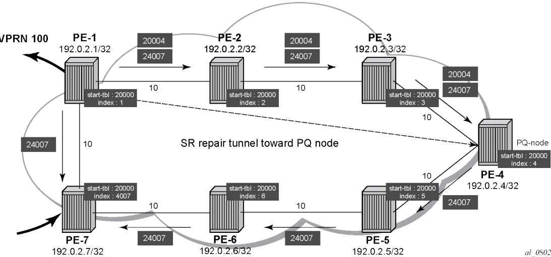
Figure 57: RLFA traffic path during protection
