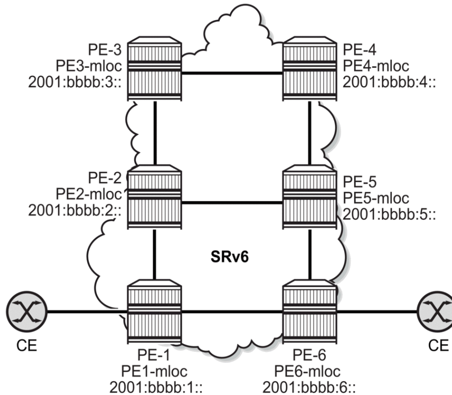
Figure 70: Example topology with micro-segment node SIDs
