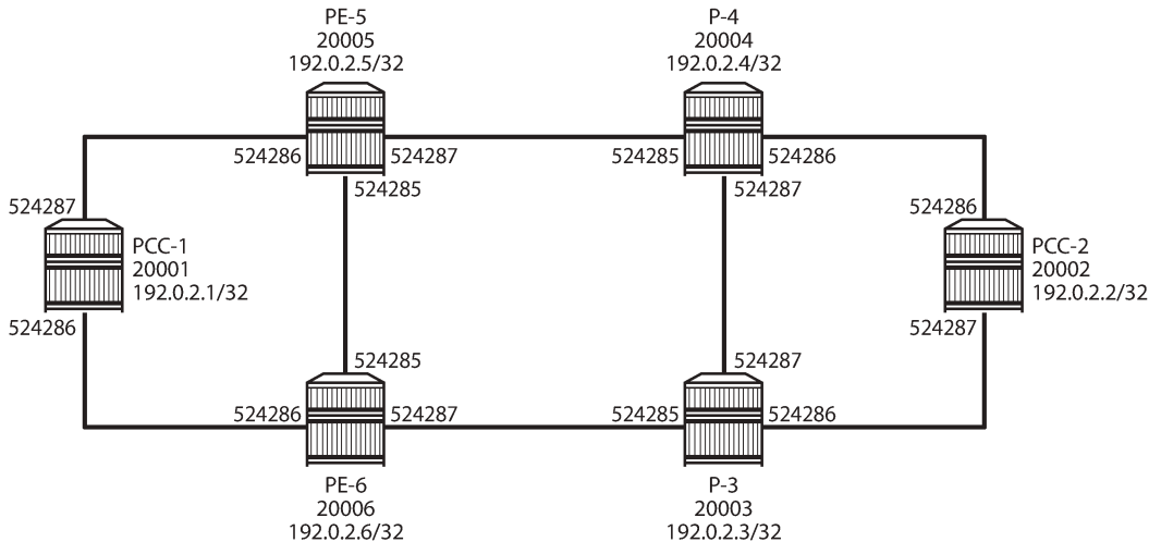
Figure 34: Node and adjacency SIDs
