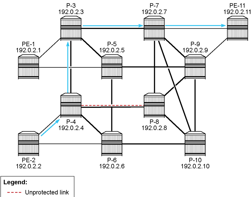
Figure 63: Path from PE-2 to PE-11 including only protected links
