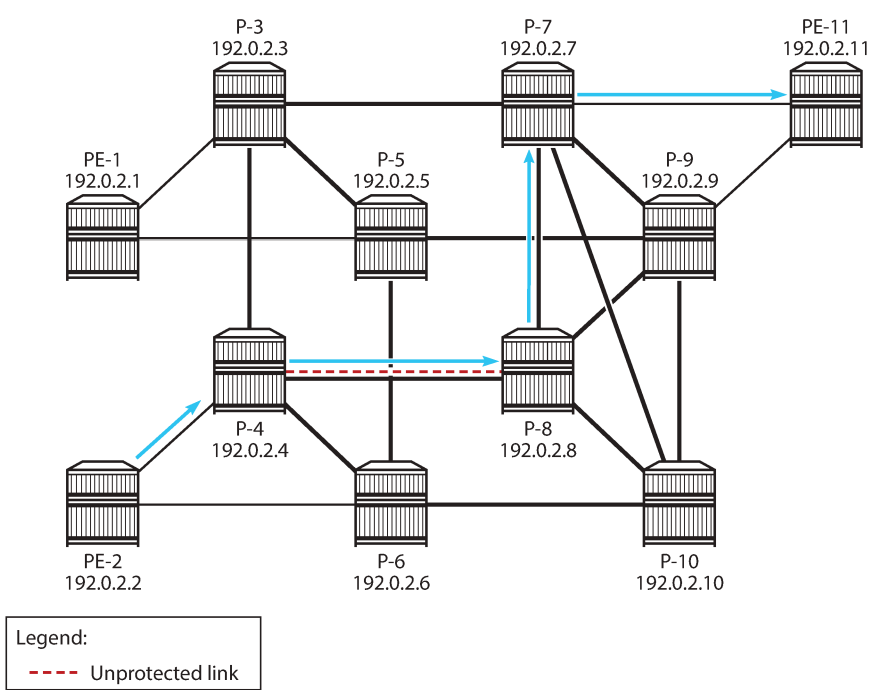
Figure 62: Path from PE-2 to PE-11 including unprotected link
