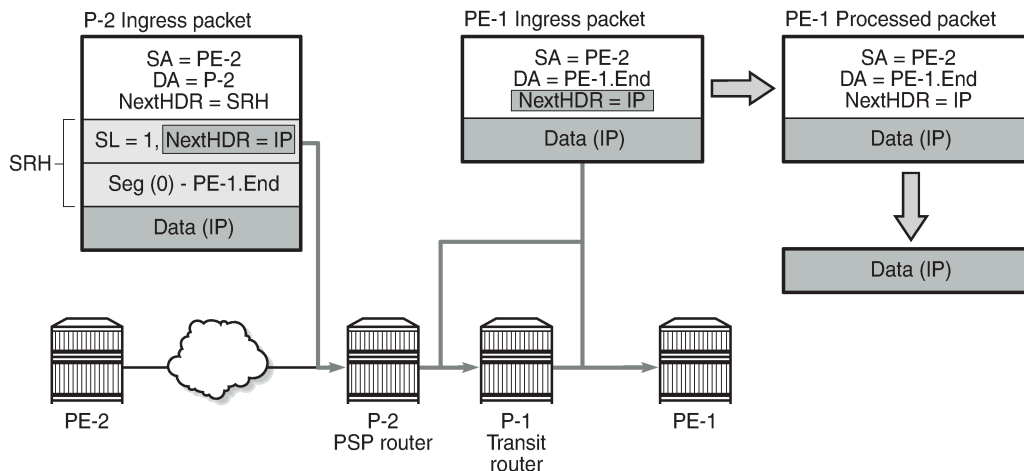
Figure 50: Penultimate SRH hop P-2 processes and removes the SRH
