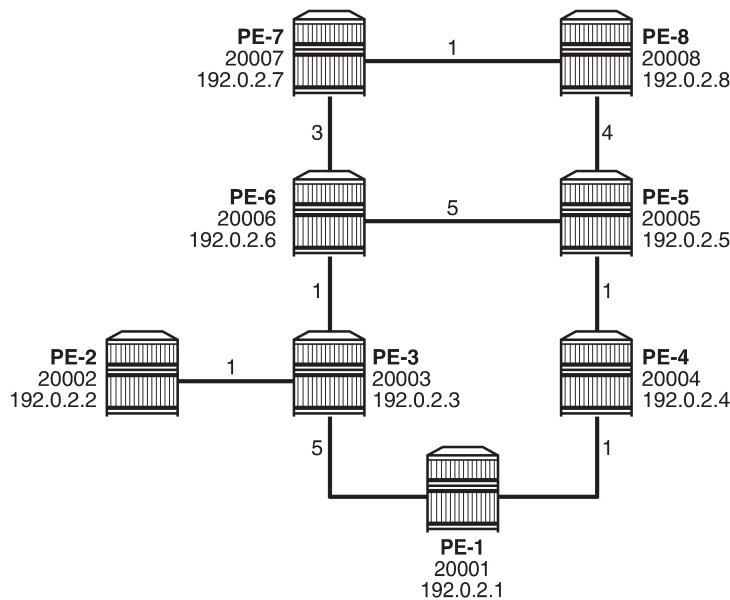
Figure 21: Example topology
