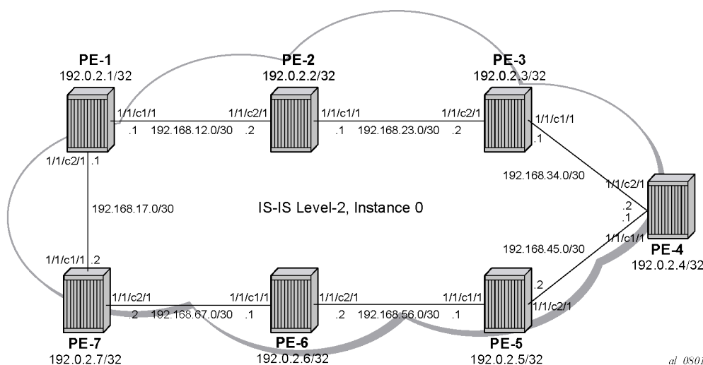
Figure 56: Example topology
