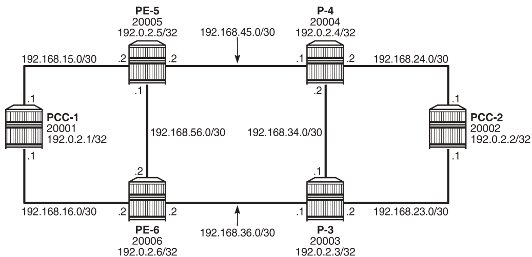
Figure 33: Segment routing network schematic
