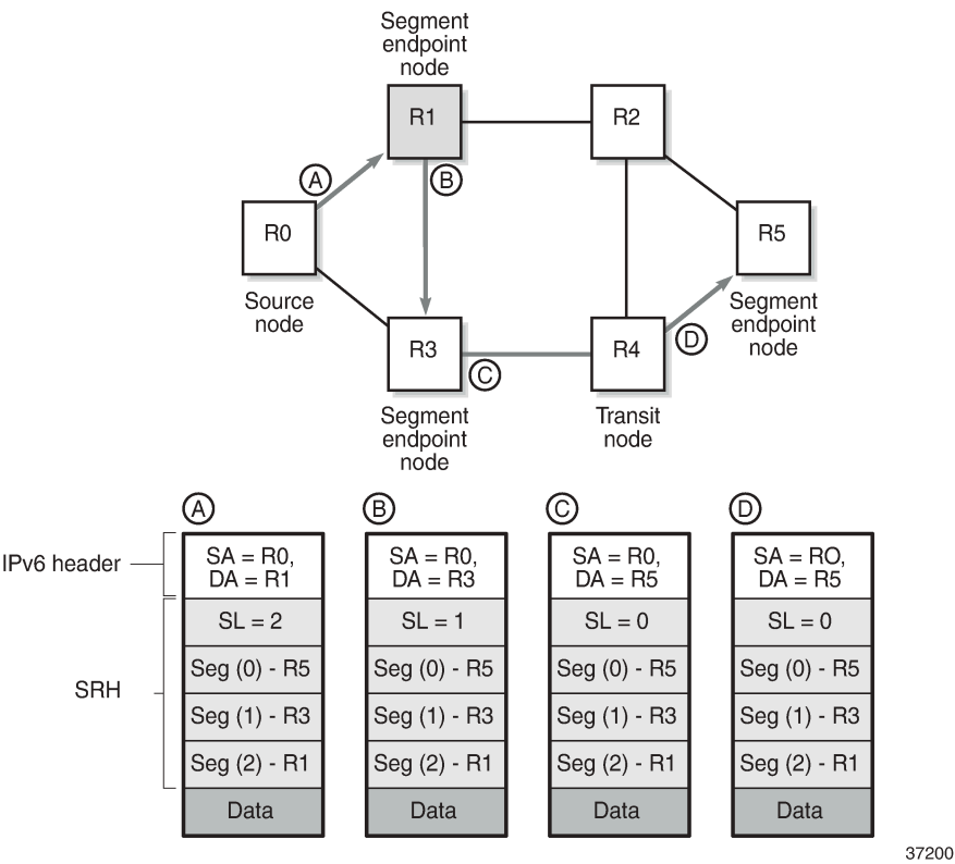
Figure 48: Data forwarding of SRv6 encapsulated packets using SRv6 SIDs
