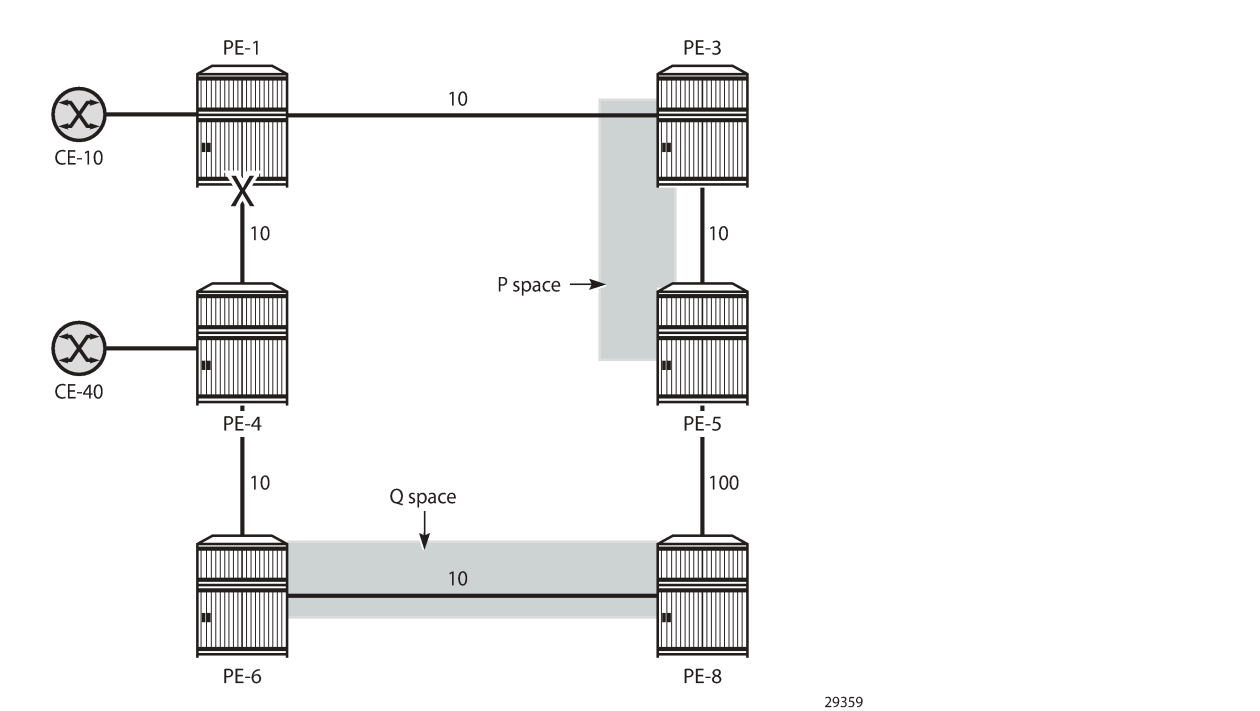
Figure 84: Extended P space of PE-1 and Q space of PE-4 are one hop apart
