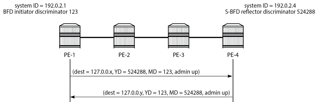
Figure 30: S-BFD session establishment - continuity check
