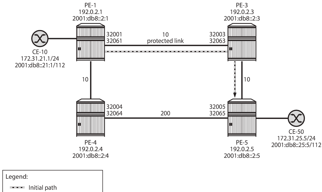
Figure 81: No post-failure LFA path when PE-4 loops back traffic
