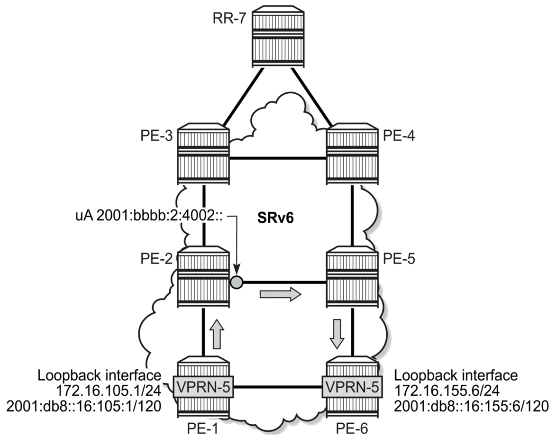
Figure 75: EVPN IFL using SRv6 policy with color 500 from PE-1 to PE-6
