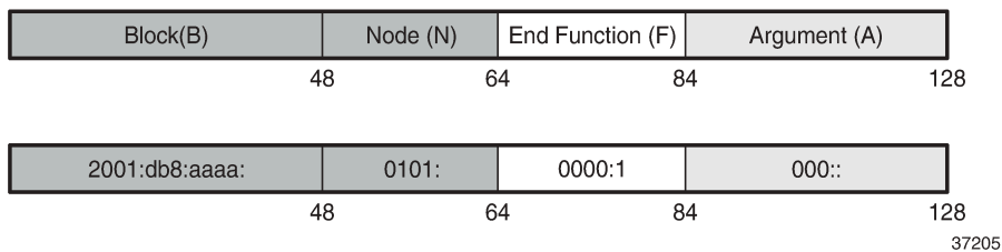
Figure 53: SRv6 End SID on PE-1
