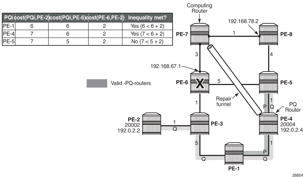
Figure 27: Validating candidate PQ routers - repair tunnel calculation
