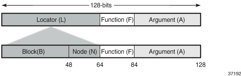
Figure 40: SRv6 SID encoding
