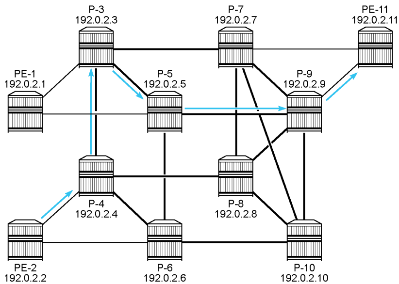
Figure 61: Path from PE-2 to PE-11 via loose hops P-3 and P-9
