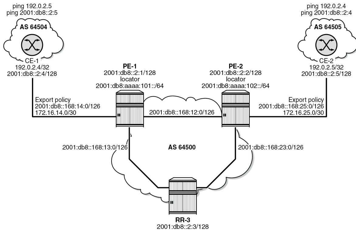
Figure 64: Example topology
