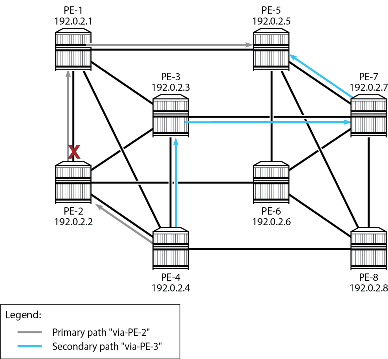
Figure 32: Failure on remote link in primary path
