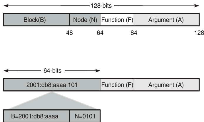
Figure 41: SRv6 SID encoding example
