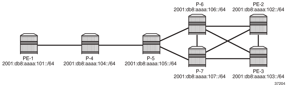
Figure 52: SRv6 router locator prefixes
