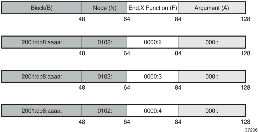
Figure 54: SRv6 End.X SIDs on PE-2
