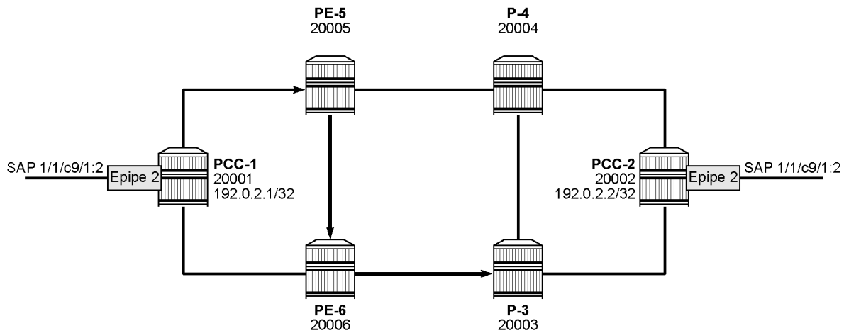
Figure 39: Epipe service schematic
