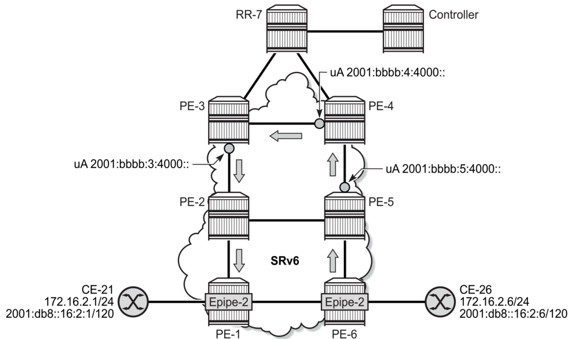
Figure 72: EVPN VPWS using SRv6 policy with color 200 from PE-6 to PE-1
