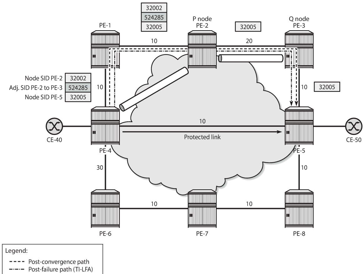
Figure 86: Post-failure TI-LFA path coincides with post-convergence path
