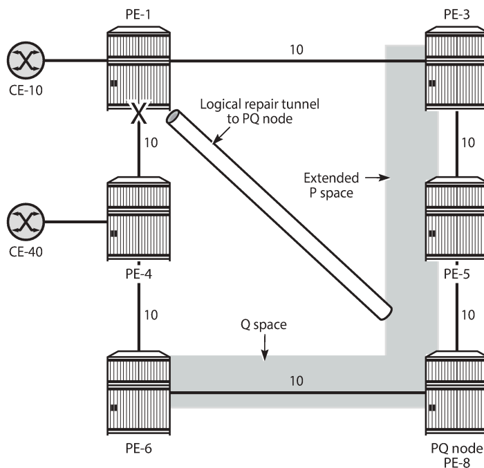
Figure 83: PQ node in remote LFA
