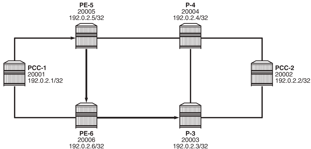
Figure 35: PCC computed strict path between PCC-1 and PCC-2
