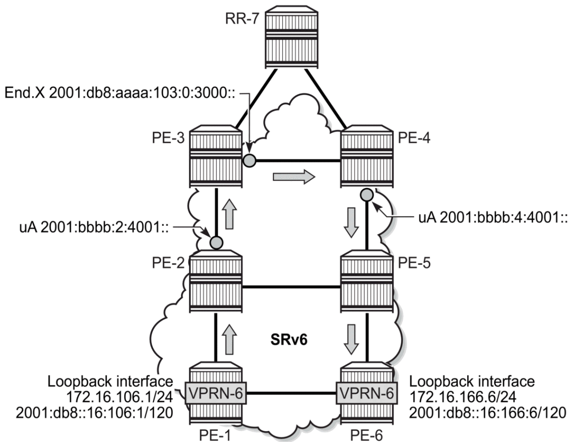
Figure 76: IP VPN using SRv6 policy with color 600 from PE-1 to PE-6
