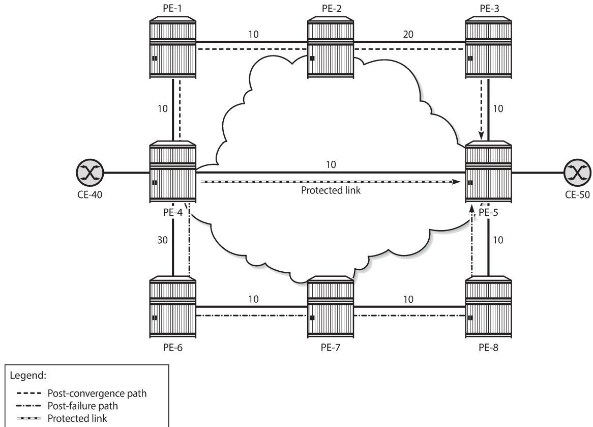
Figure 77: Post-failure LFA path does not match post-convergence path
