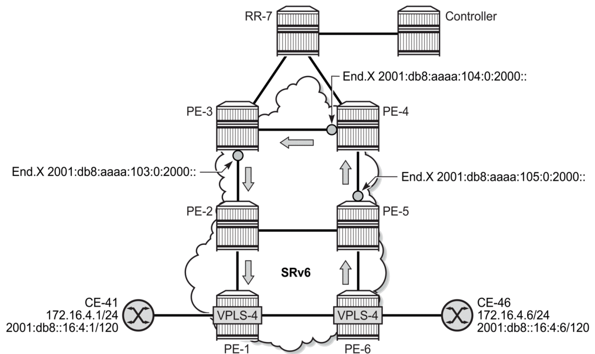
Figure 74: EVPN VPLS using SRv6 policy with color 400 from PE-6 to PE-1
