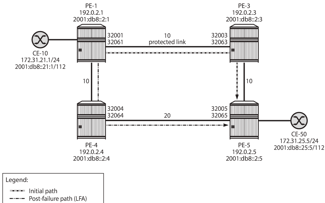
Figure 80: Example topology with regular LFA configured on PE-4
