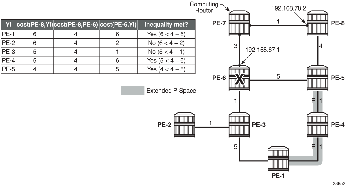
Figure 25: Node protecting extended P-space calculation
