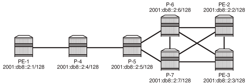
Figure 51: Example topology
