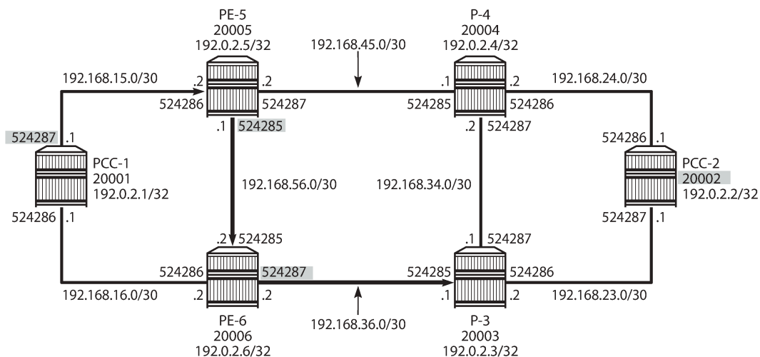
Figure 36: PCC computed LSP hop-to-label translation
