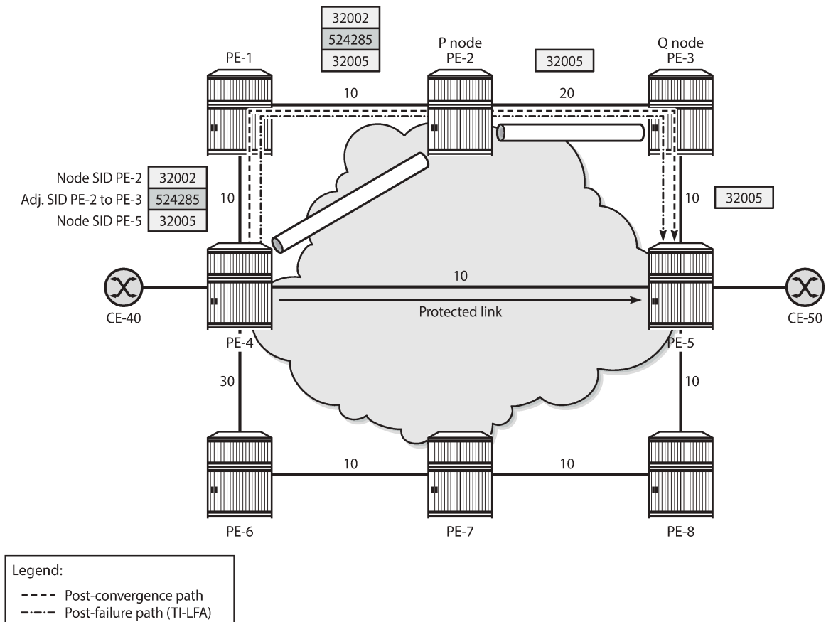
Figure 78: Post-failure TI-LFA path matches post-convergence path
