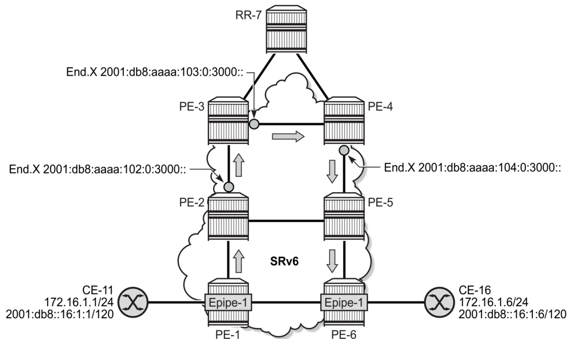
Figure 71: EVPN VPWS using SRv6 policy with color 100 from PE-1 to PE-6
