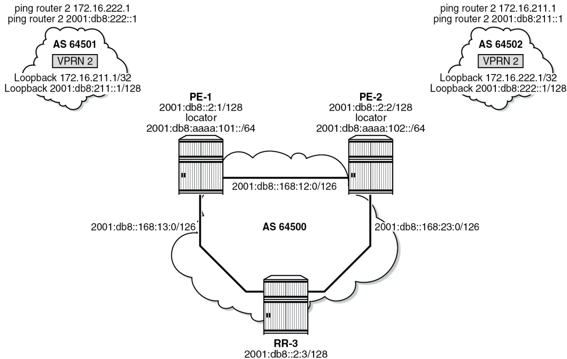
Figure 55: Example topology
