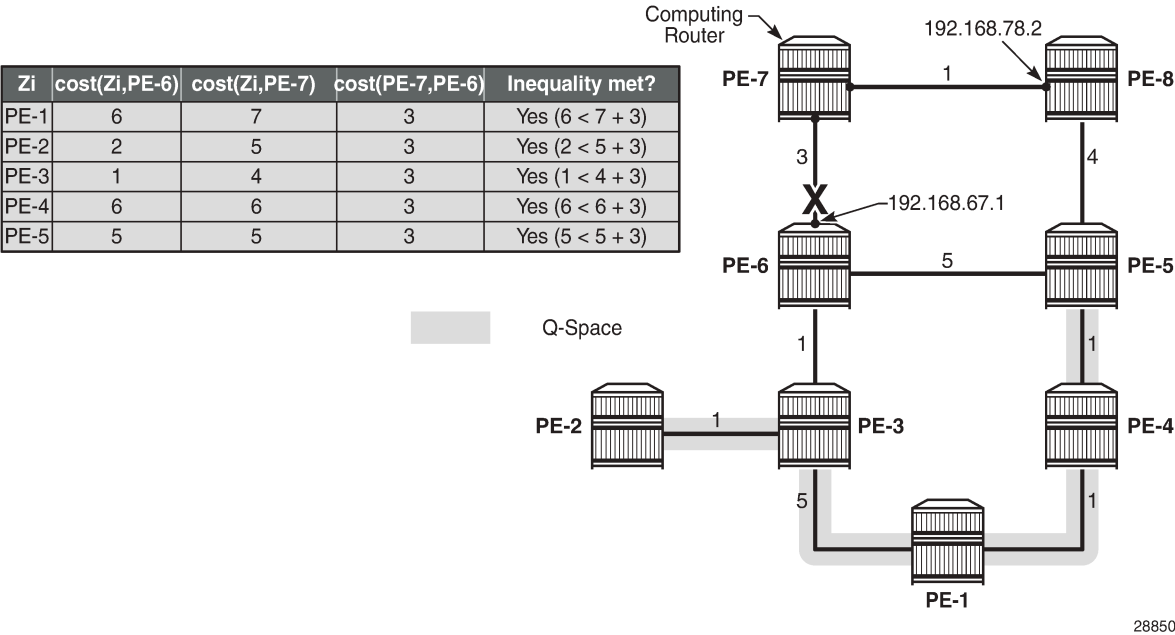
Figure 23: Link protecting Q-space calculation
