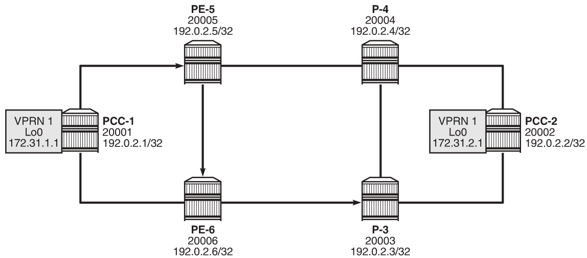
Figure 38: VPRN service schematic
