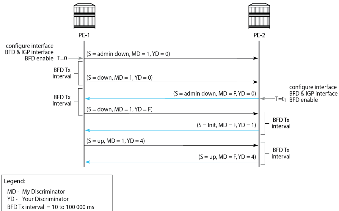
Figure 28: Classical BFD handshake
