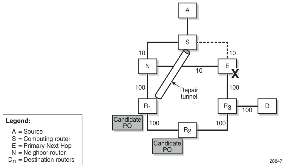
Figure 20: Two candidate PQ routers – repair tunnel
