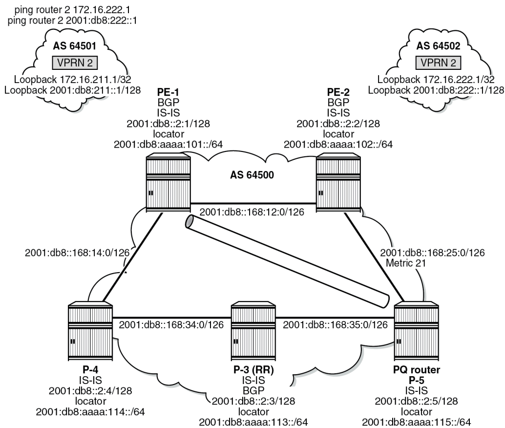
Figure 66: Example topology with metric 21 between PE-2 and P-5
