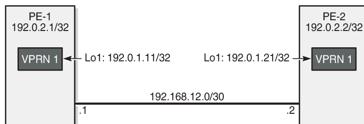
Figure 2: VPNR 1 uses a BGP transport tunnel with endpoint 192.0.1.21 on PE-2
