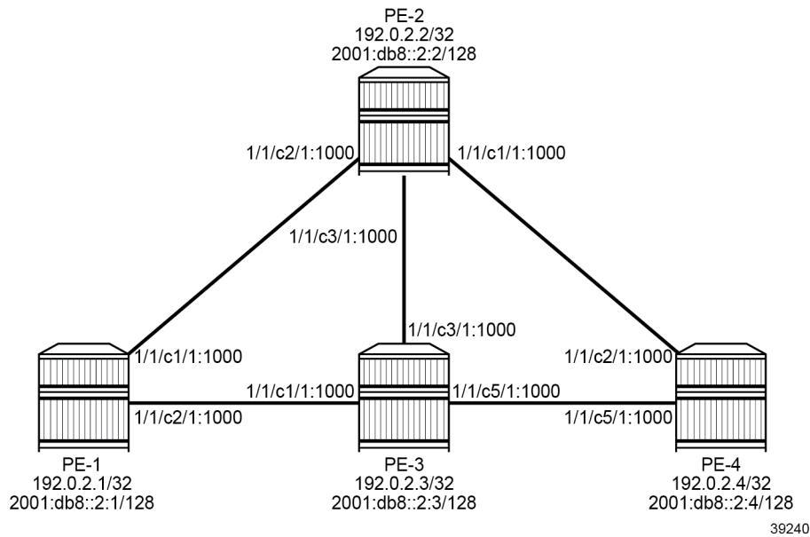
Figure 234: Example topology
