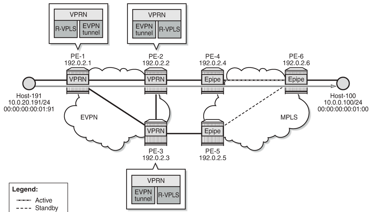
Figure 211: Initial situation with forwarding path via PE-2
