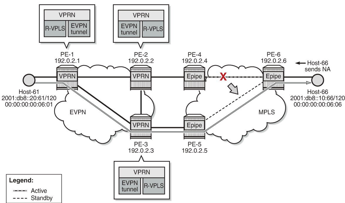
Figure 216: Host-66 sends unsolicited NA message after switchover
