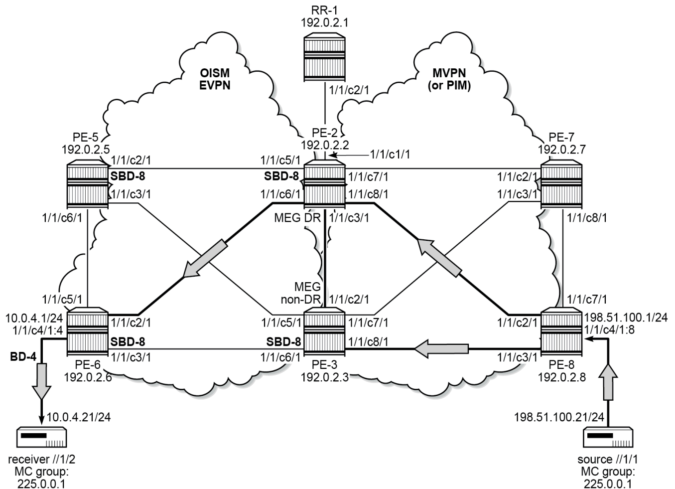
Figure 243: MVPN/PIM MC source - EVPN MC receiver example setup
