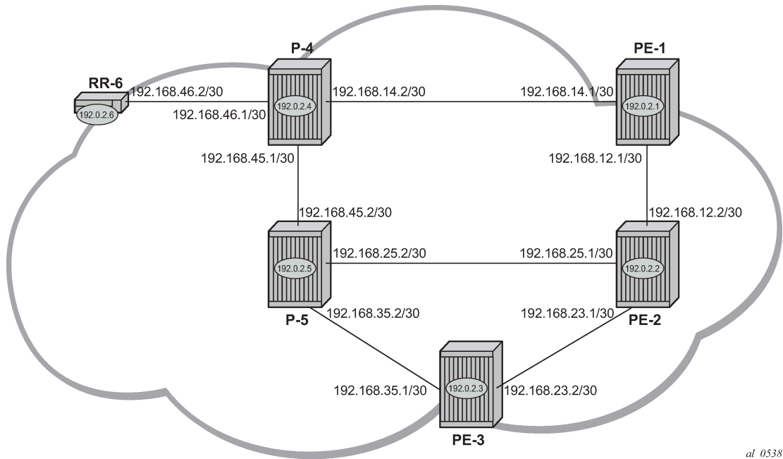
Figure 199: Example topology
