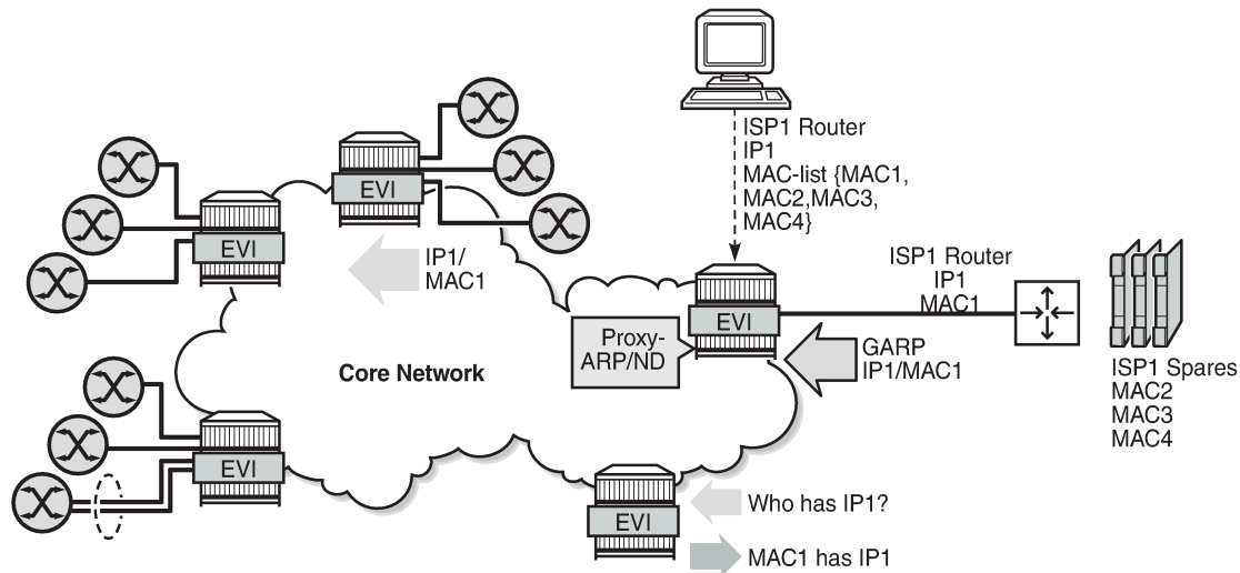
Figure 321: IXP with proxy-ARP/ND MAC list for dynamic entries
