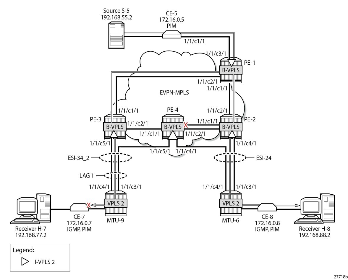
Figure 313: EVPN-MPLS with MH - PIM Snooping Disabled – Receiver H-8 Joined
