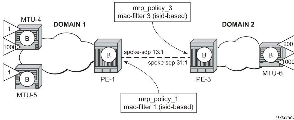
Figure 292: Inter-domain B-VPLS and MMRP policies/ISID-based filters example
