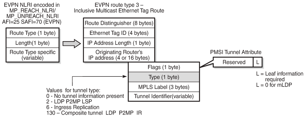
Figure 272: BGP-EVPN route type 3 with PTA
