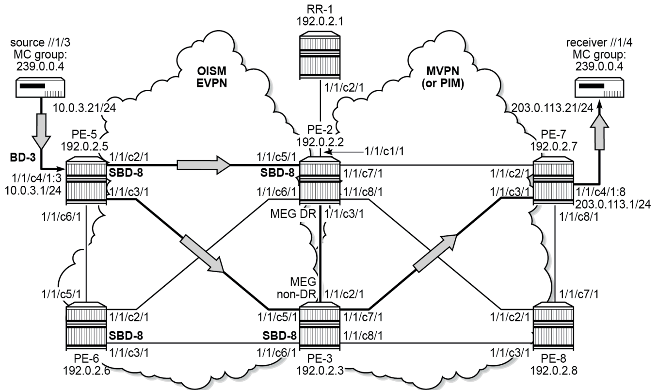
Figure 244: EVPN MC source - MVPN/PIM MC receiver example setup, with non-DR as UMH for PE-7
