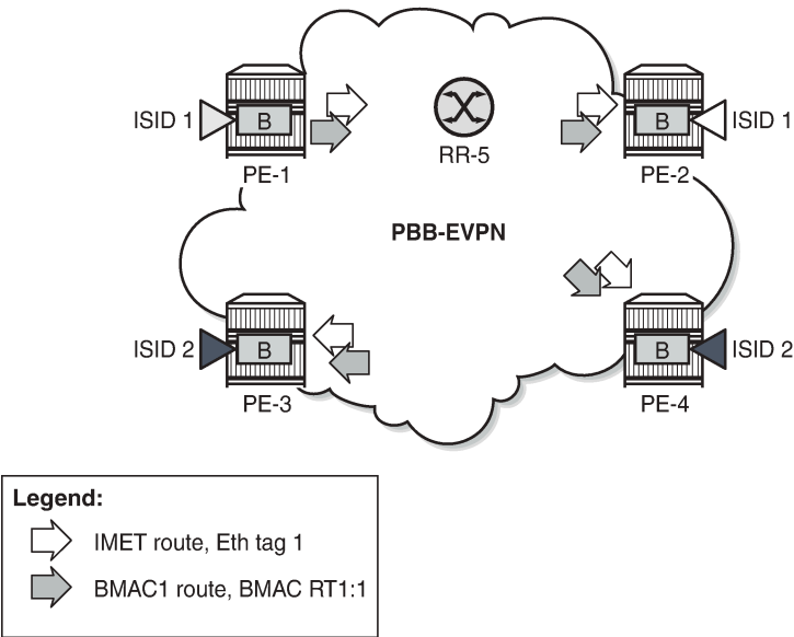
Figure 284: PBB-EVPN B-VPLS-based RT
