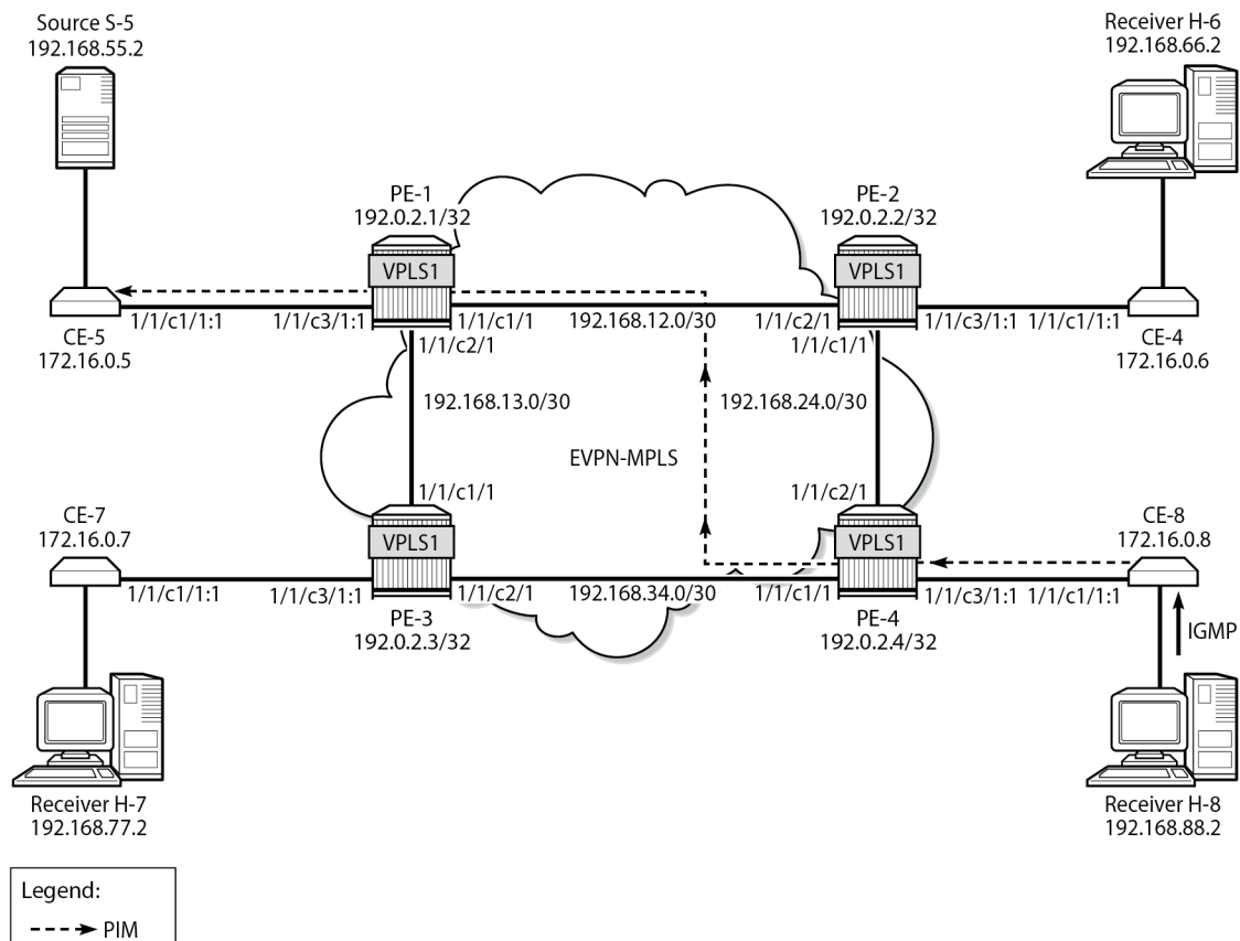
Figure 299: H-8 Joins Group (192.168.55.2, 232.1.1.1) and PIM Snooping is Disabled
