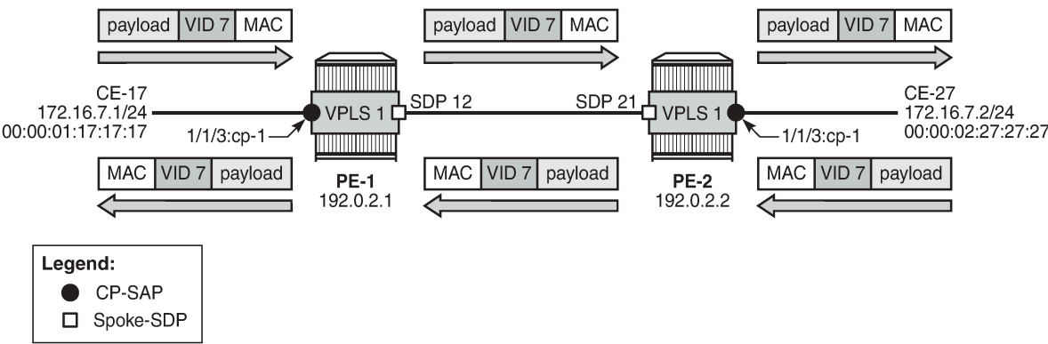
Figure 342: Customer VID is preserved between QinQ CP SAPs - no VLAN translation shows that QinQ CP SAPs only pop or push the service delimiting VID (VID 100), but not the customer VID in the CP range, as follows:
