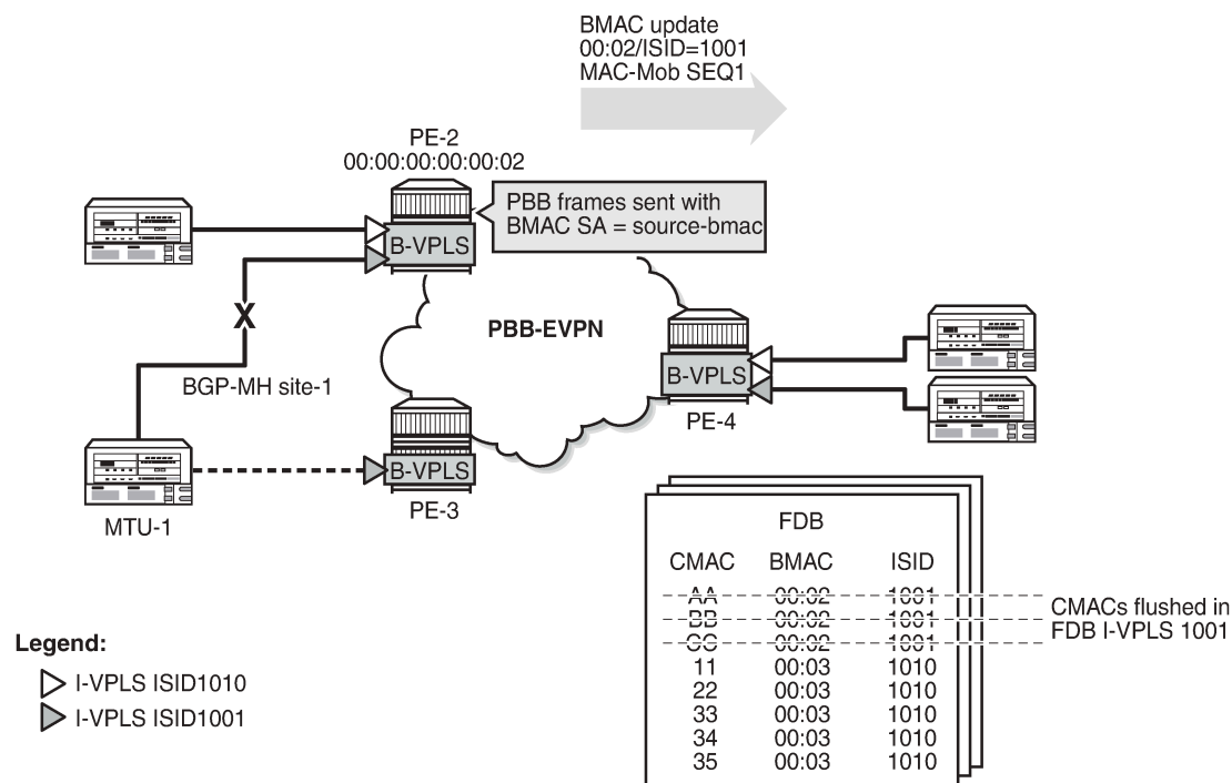
Figure 278: CMAC flush when SAP in BGP multi-homing site fails
