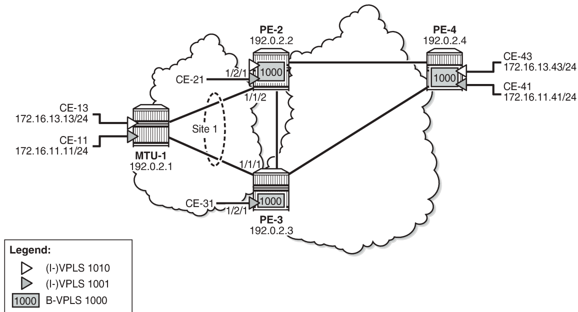
Figure 282: Example topology with BGP multi-homing
