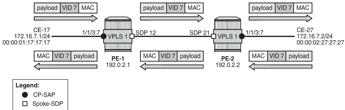
Figure 346: Customer VID is preserved between two dot1q CP SAPs
