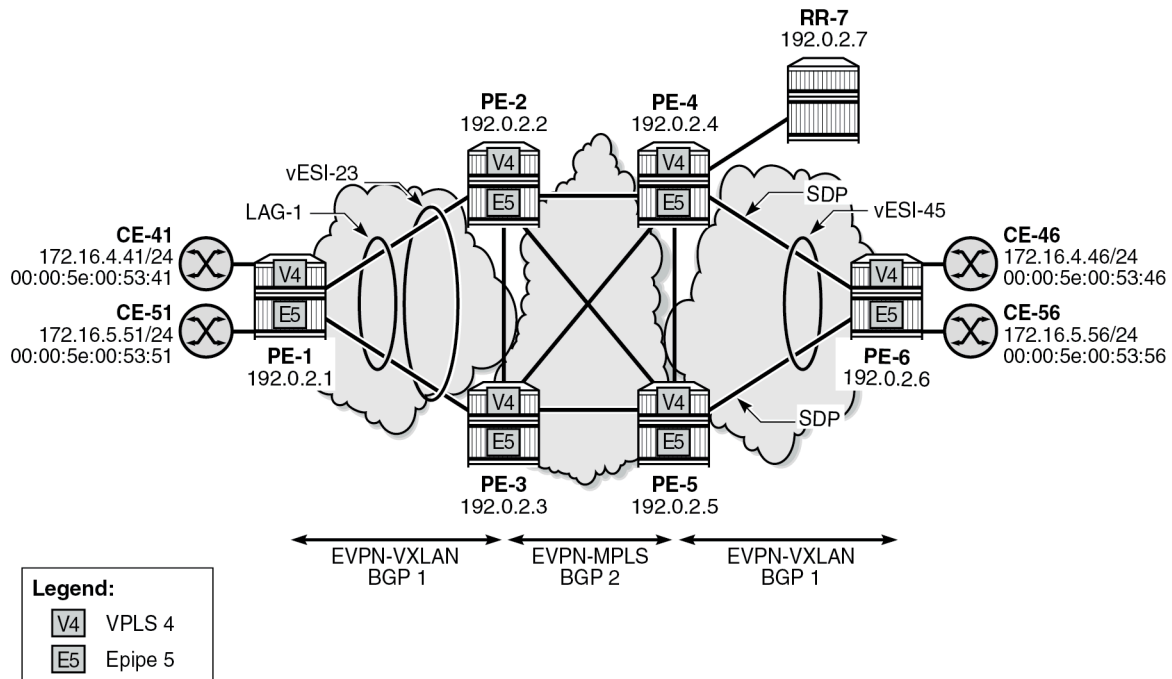
Figure 335: Example topology with VPLS 4 and Epipe 5
