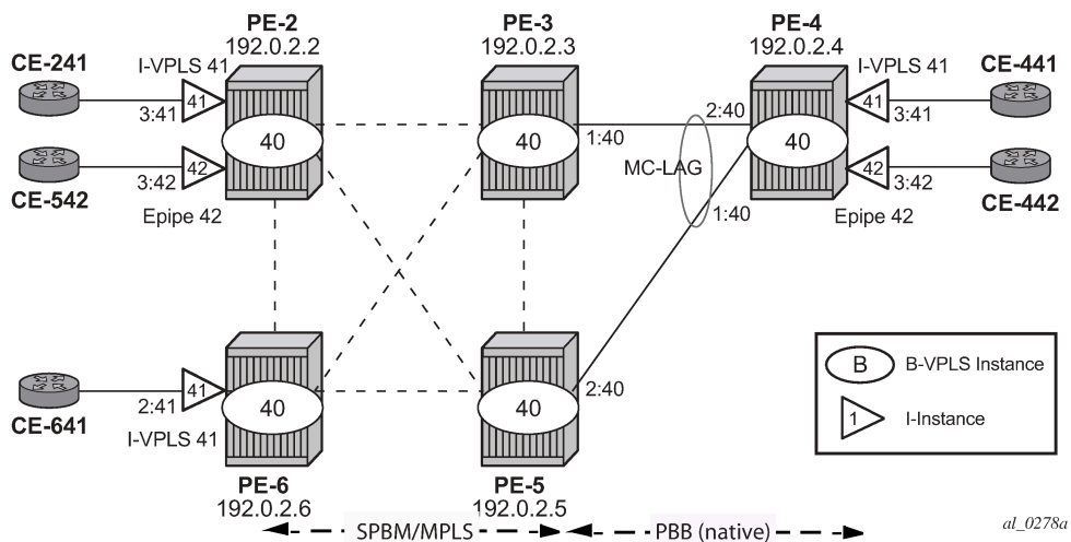
Figure 326: Access resiliency example topology
