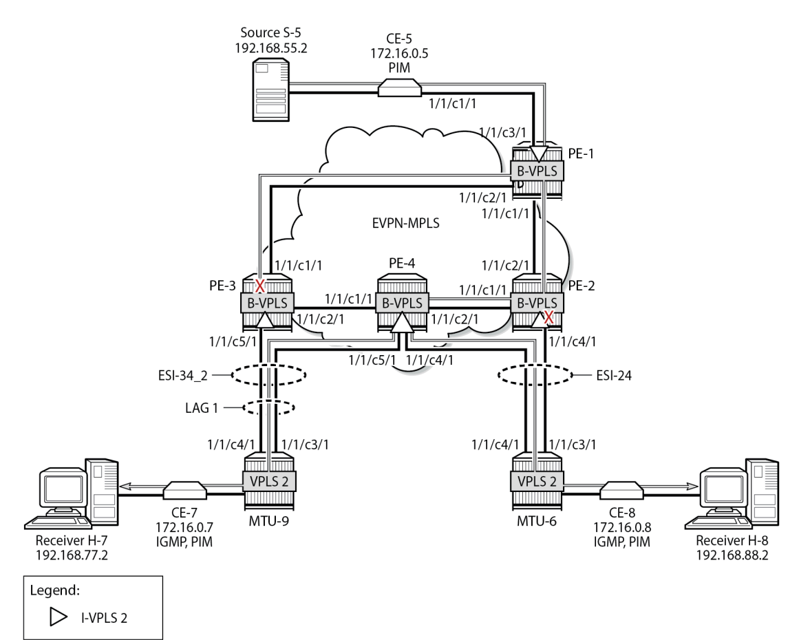
Figure 316: EVPN-MPLS with MH and PIM Snooping – Multicast Flow after Failover
