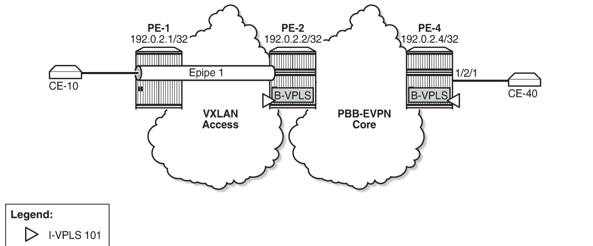
Figure 328: Static VXLAN termination on system IP addresses
