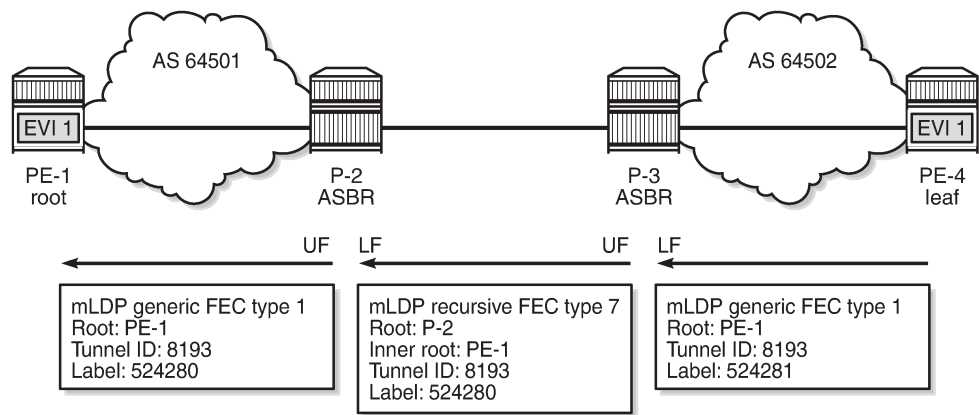
Figure 264: Non-recursive mLDP FEC for inter-AS model C
