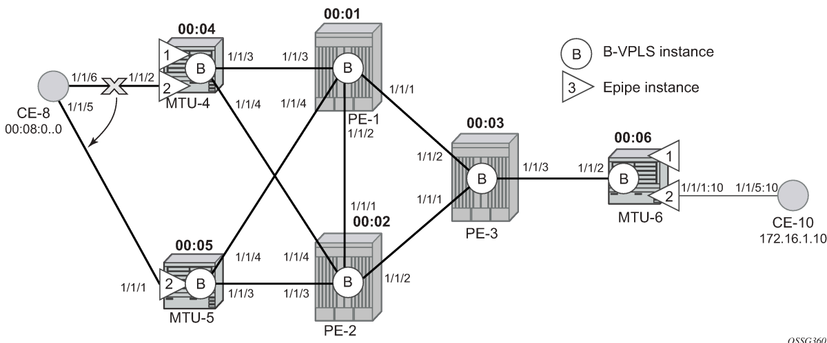
Figure 290: Black-hole
