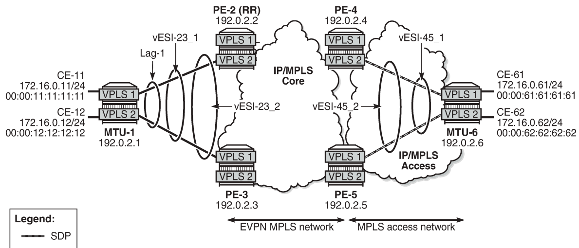
Figure 319: Example topology with all-active and single-active vESs
