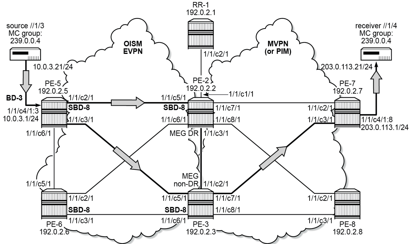
Figure 248: EVPN MC source - MVPN/PIM MC receiver example setup, with non-DR as UMH for PE-7
