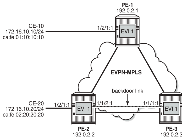
Figure 35: Example topology
