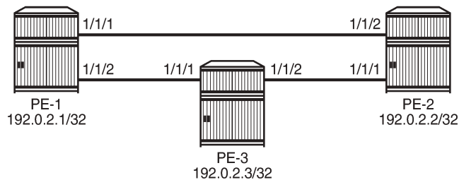
Figure 191: Example topology
