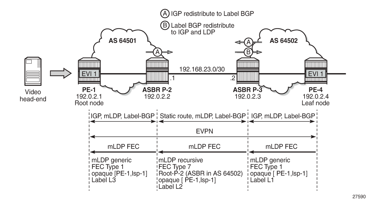
Figure 270: Example topology for optimized Inter-AS Model C for mLDP
