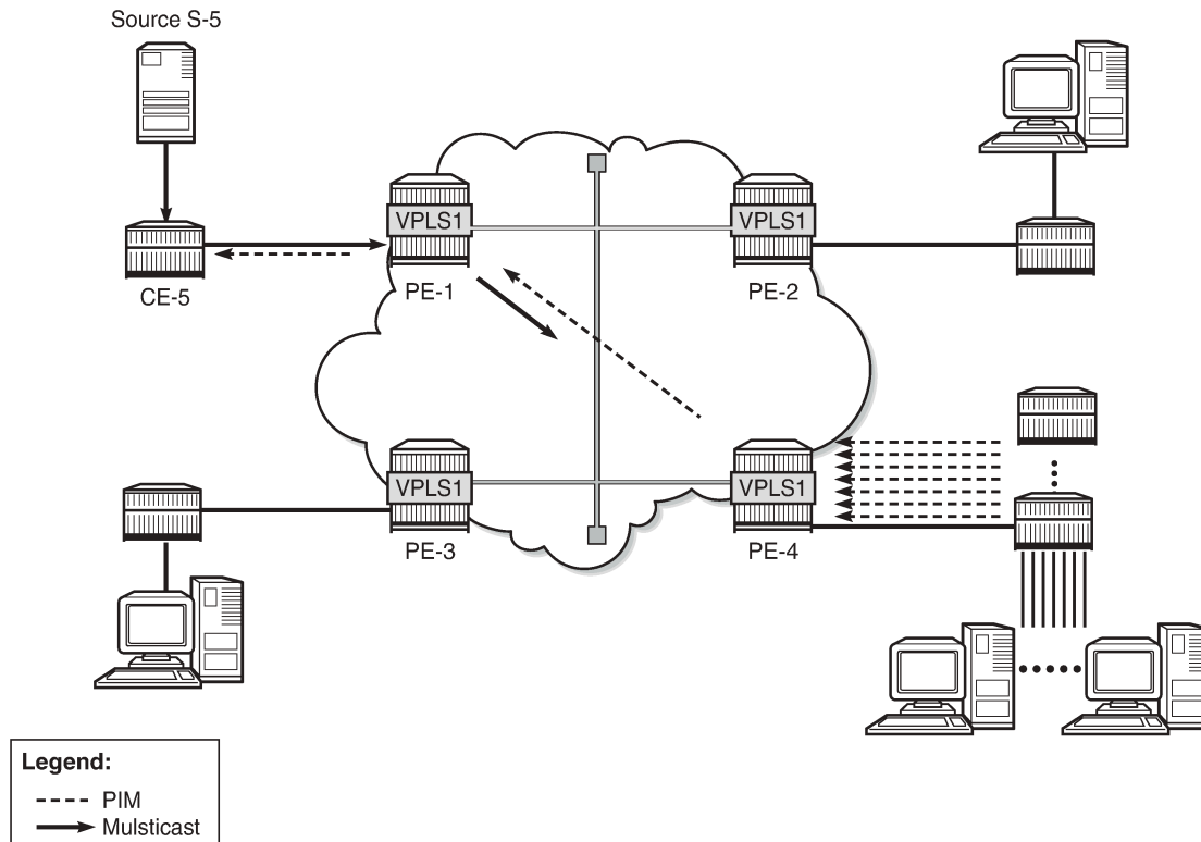
Figure 296: Multicast in VPLS with PIM Snooping in Proxy Mode - Multiple CEs
