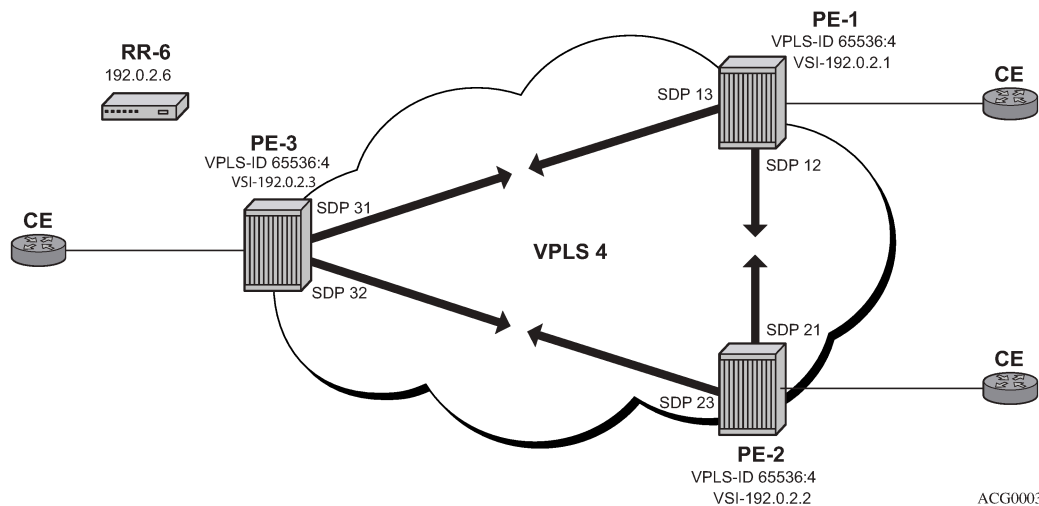
Figure 201: VPLS instance using pre-provisioned SDPs shows a VPLS instance configured across three PE routers as before.
