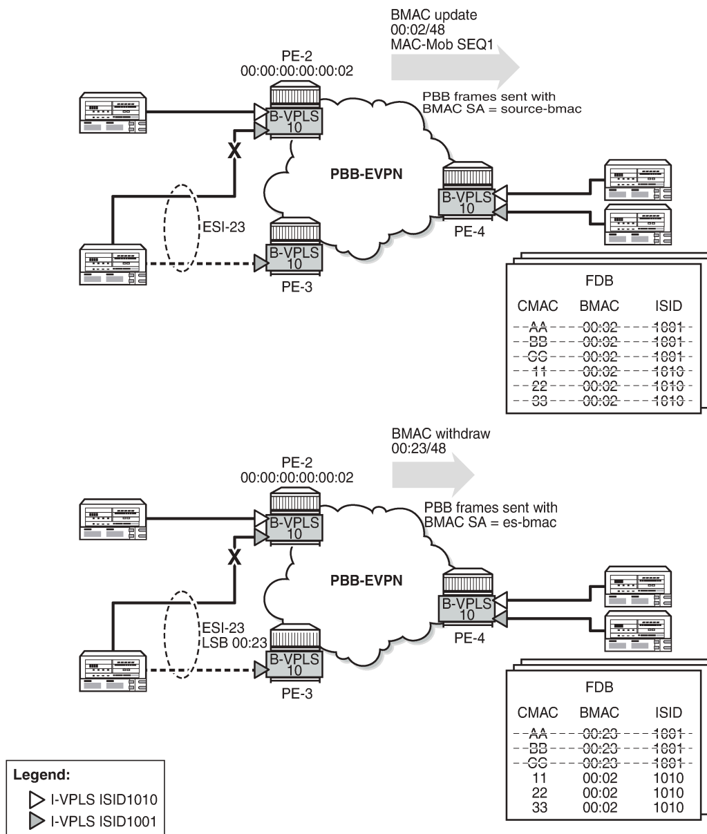
Figure 280: ISID-independent CMAC flush when ES fails
