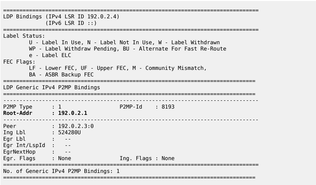
Figure 267: Leaf node sends basic FEC in seamless MPLS shows the label mapping messages when leaf node PE-4 only generates basic FEC type 1 messages.
