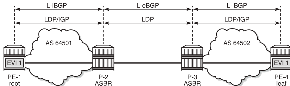
Figure 259: Example topology for inter-AS model C
