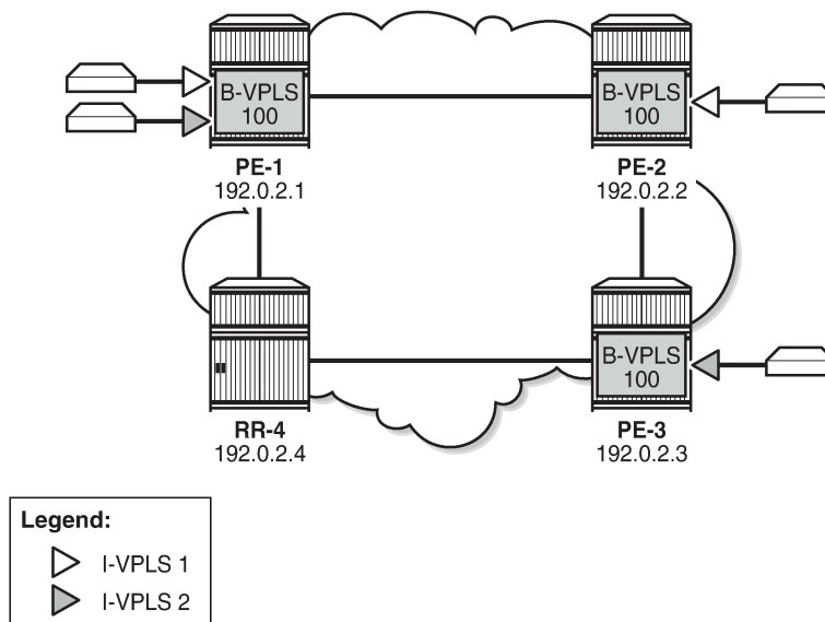
Figure 287: Example topology
