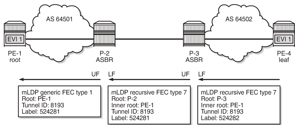
Figure 263: Recursive mLDP FEC for inter-AS model C
