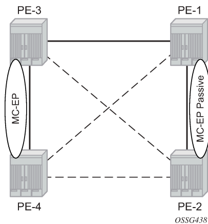
Figure 226: Multi-chassis passive mode
