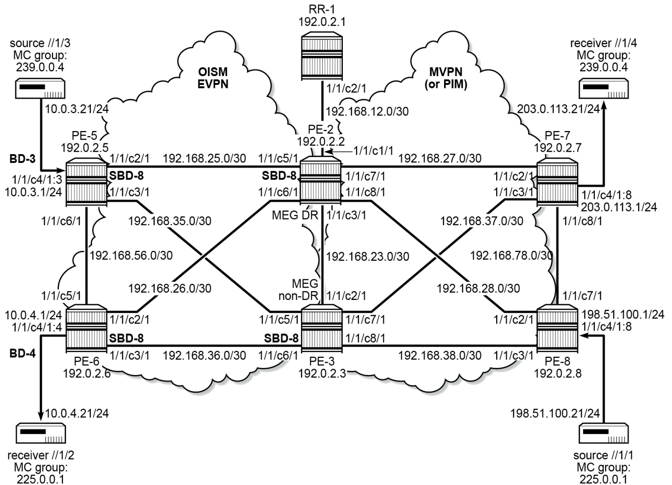
Figure 242: Example topology
