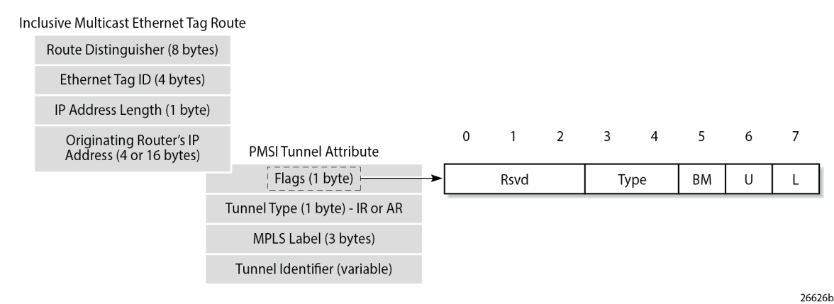
Figure 196: PMSI Tunnel Attribute - Flags
