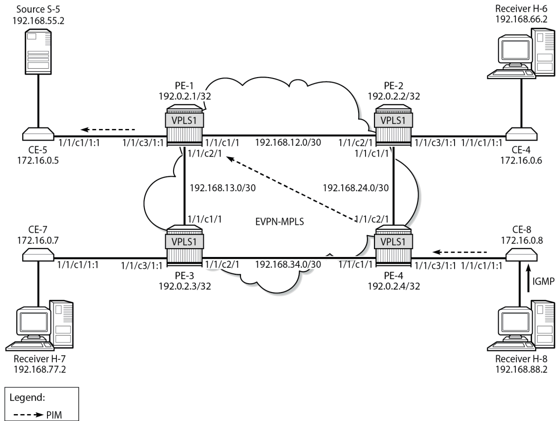
Figure 301: H-8 Joins (192.168.55.2, 232.1.1.1) and PIM Snooping is Enabled in Proxy Mode
