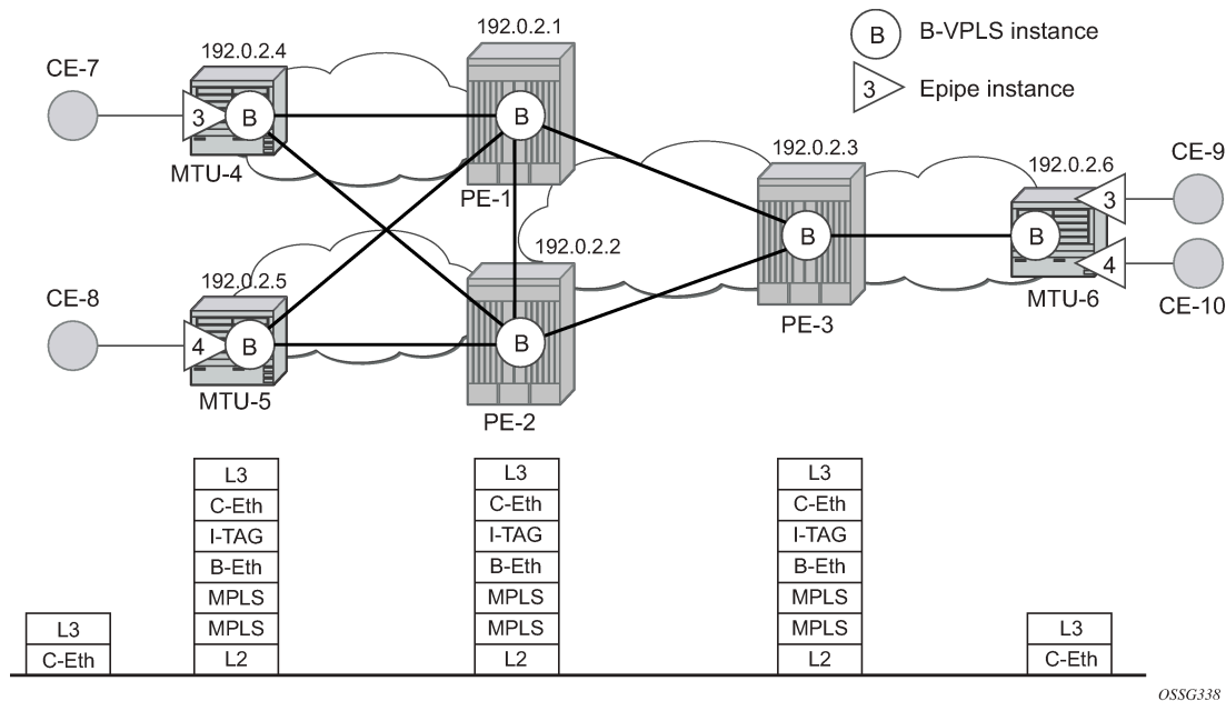
Figure 275: Example topology
