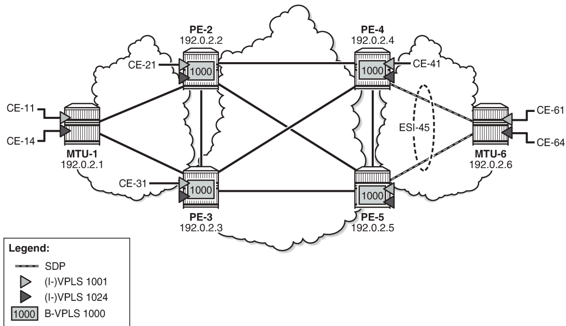
Figure 283: Example topology with single-active ES
