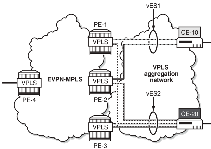
Figure 317: Virtual Ethernet Segments
