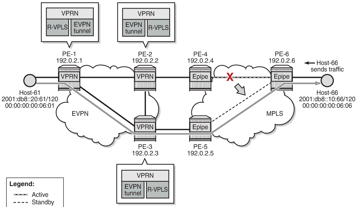
Figure 217: Host generates non-ND traffic after switchover
