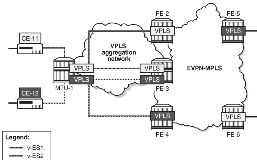
Figure 338: vESs for PWs
