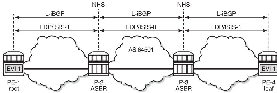
Figure 265: Example topology for seamless MPLS
