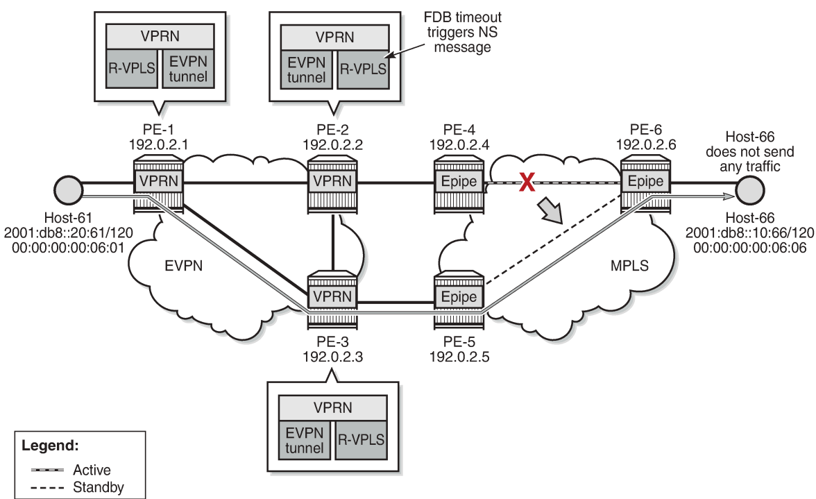
Figure 218: Host does not send any traffic after switchover
