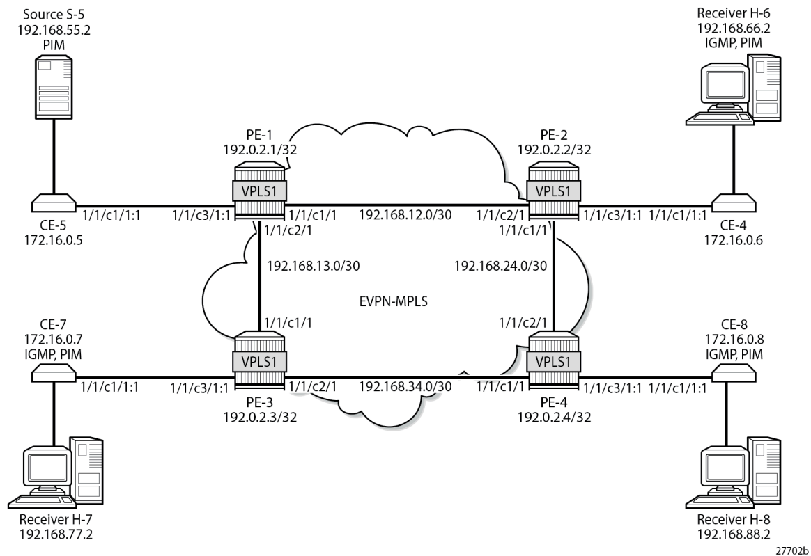
Figure 297: Example Topology
