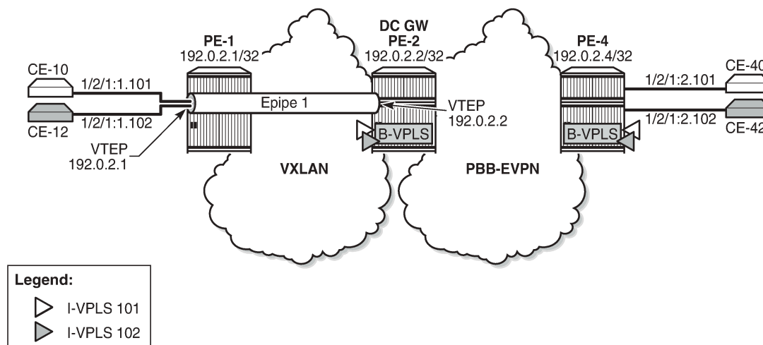
Figure 329: Example topology for static VXLAN termination on system IP addresses
