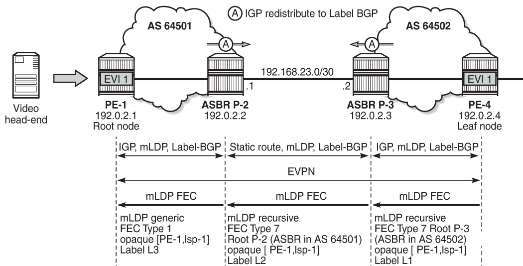
Figure 269: Inter-AS Model C for P2MP mLDP
