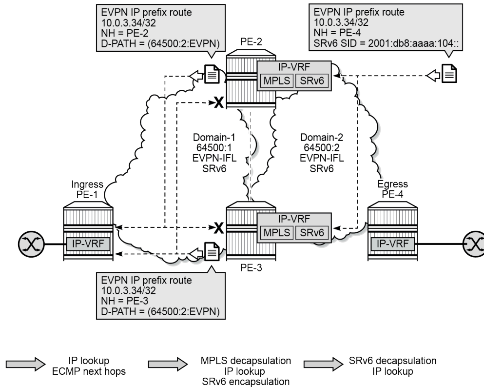
Figure 235: EVPN IP prefix routes readadvertised between SRv6 domains
