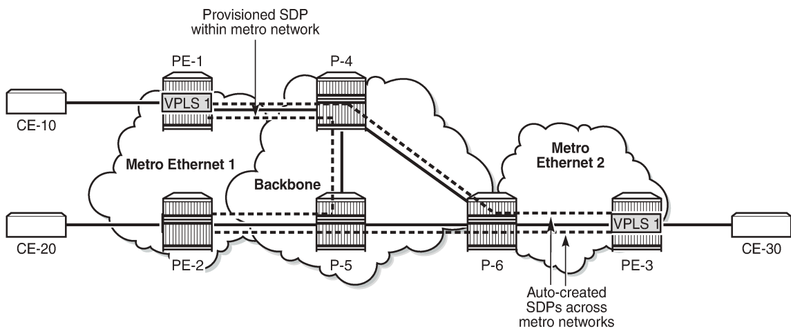
Figure 207: SDP bindings in VPLS 1 with prefer-provisioned-sdp option
