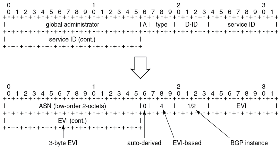
Figure 333: Auto-derived RT in RFC 8365
