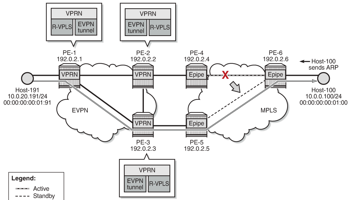
Figure 212: Host-100 sends an ARP request or GARP after switchover
