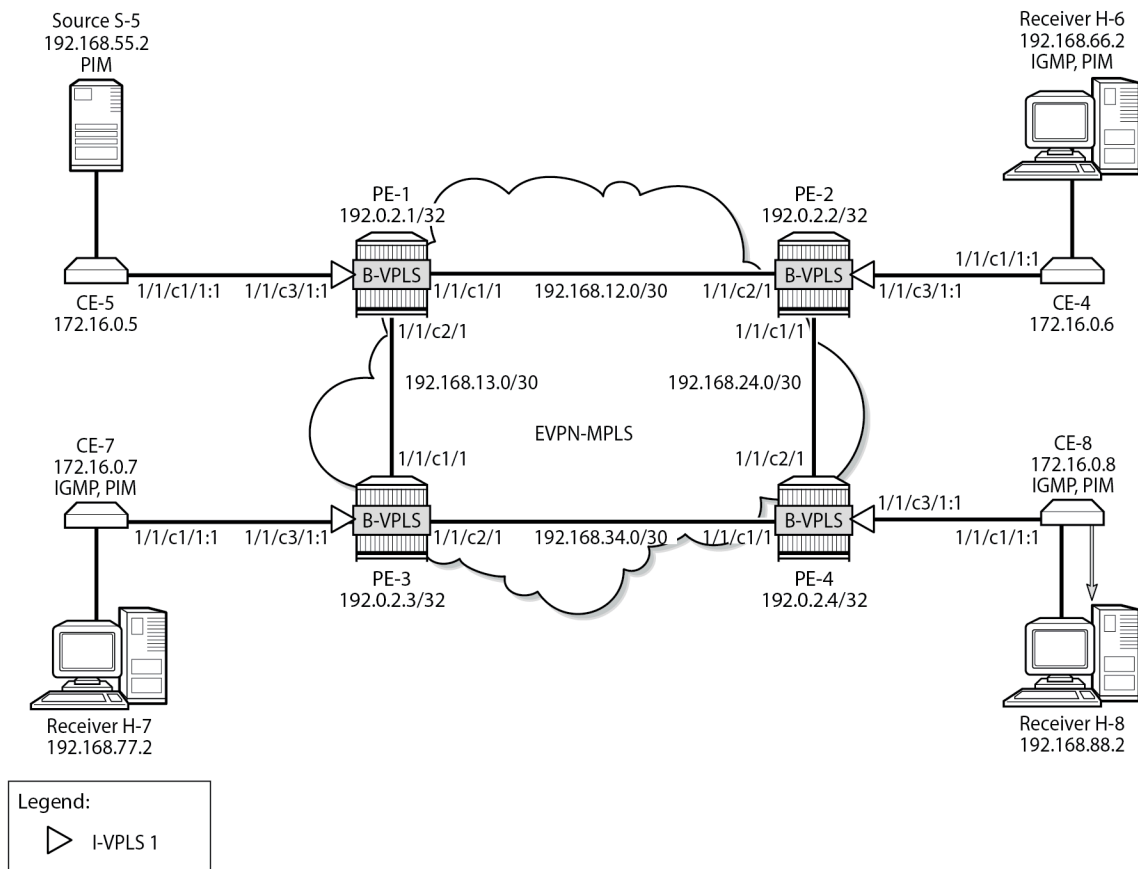
Figure 309: Example Topology for PBB-EVPN without MH
