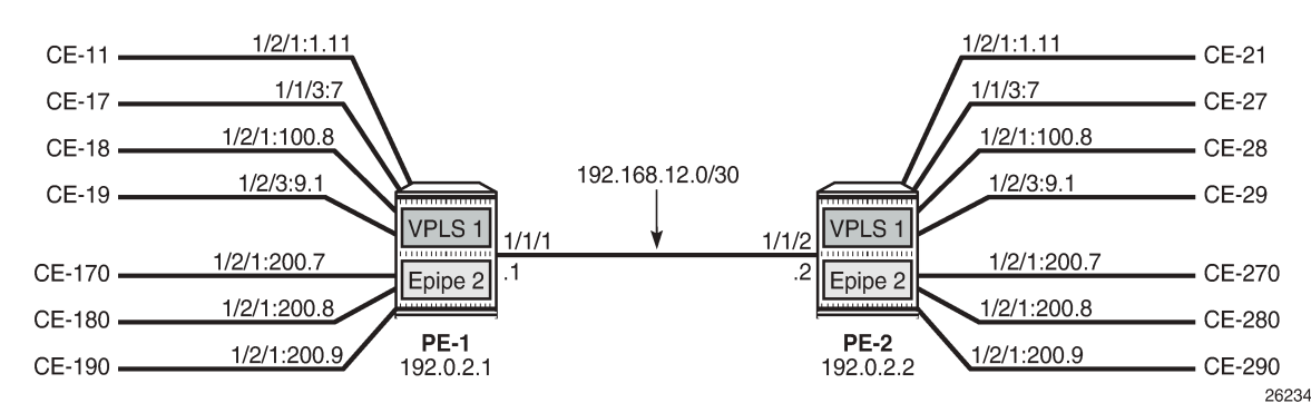
Figure 343: Example topology
