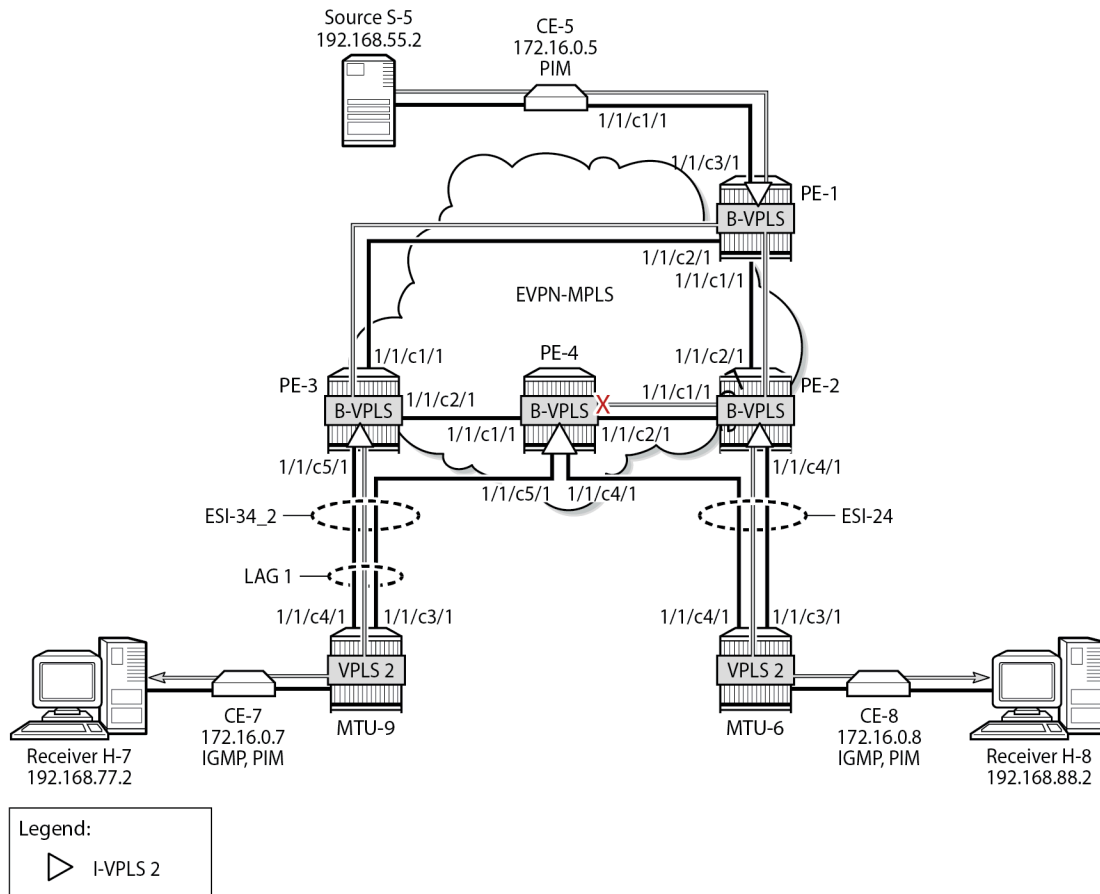
Figure 314: EVPN-MPLS with MH and PIM Snooping – Receivers H-7 and H-8 Joined
