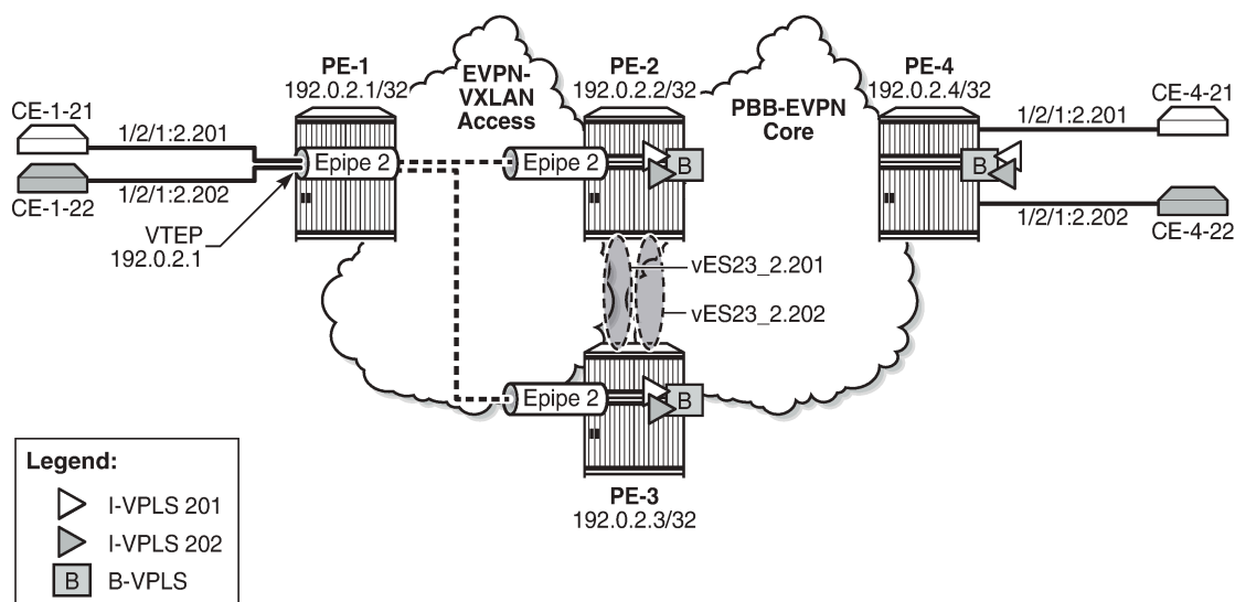
Figure 251: Epipe 2 with EVPN-VXLAN and all-active multi-homing
