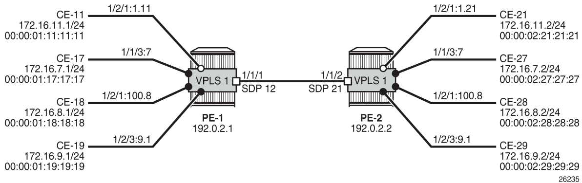
Figure 344: Example topology for VLAN ranges in VPLS 1
