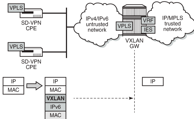
Figure 352: VXLAN GW in an SD-VPN
