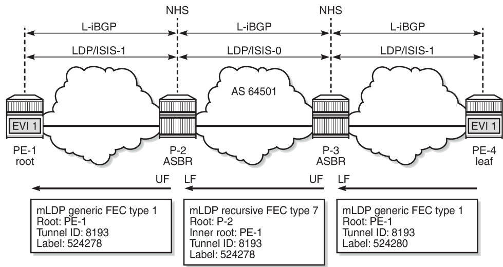
Figure 267: Leaf node sends basic FEC in seamless MPLS
