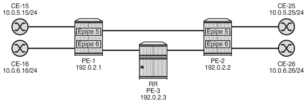
Figure 194: BGP-VPWS with auto-GRE spoke-SDPs
