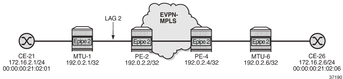
Figure 257: Sample topology with Epipe 2
