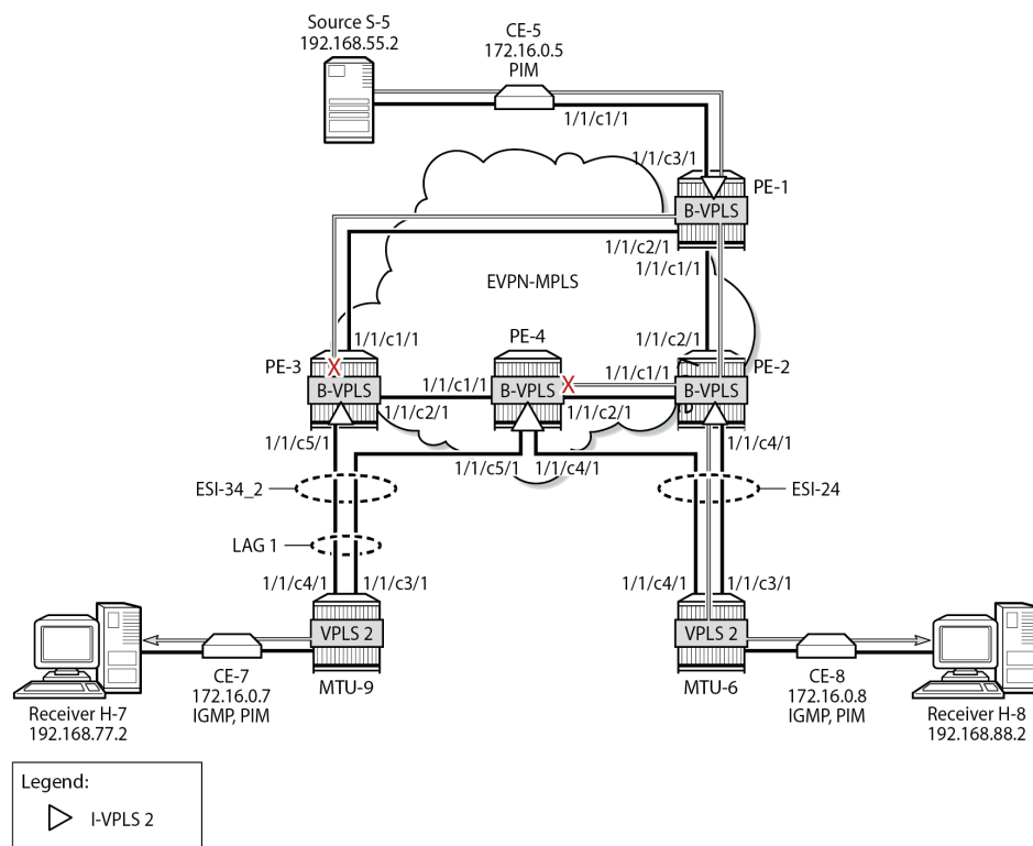
Figure 315: PBB-EVPN with MH and PIM Snooping – Receiver H-8 Joined
