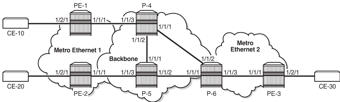
Figure 204: Example topology
