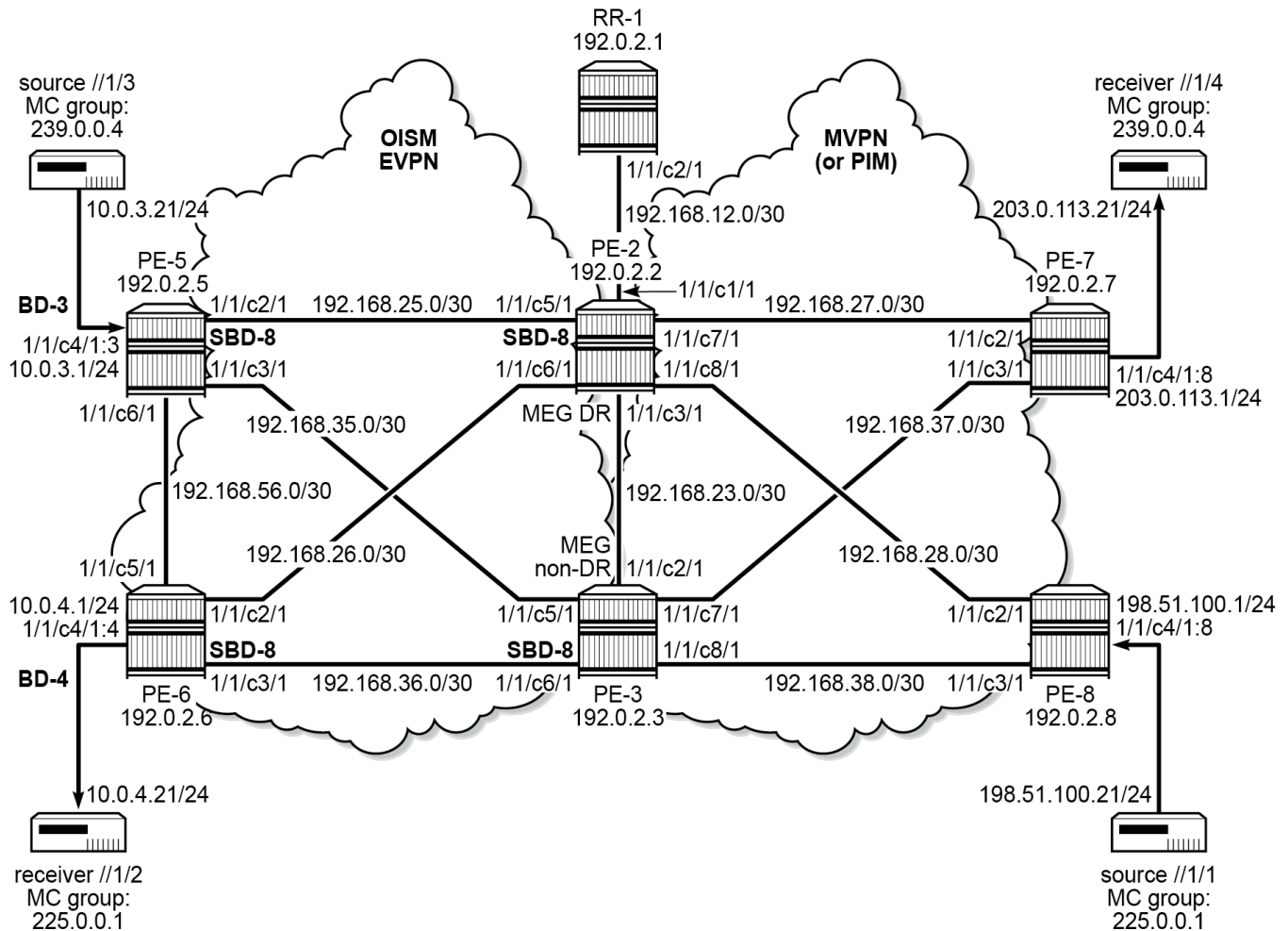
Figure 246: Example topology
