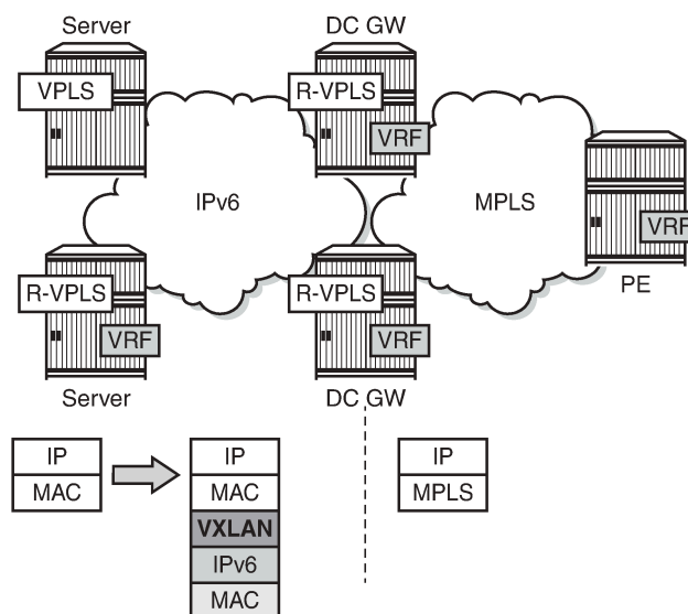
Figure 353: VXLAN IPv6 underlay for DC
