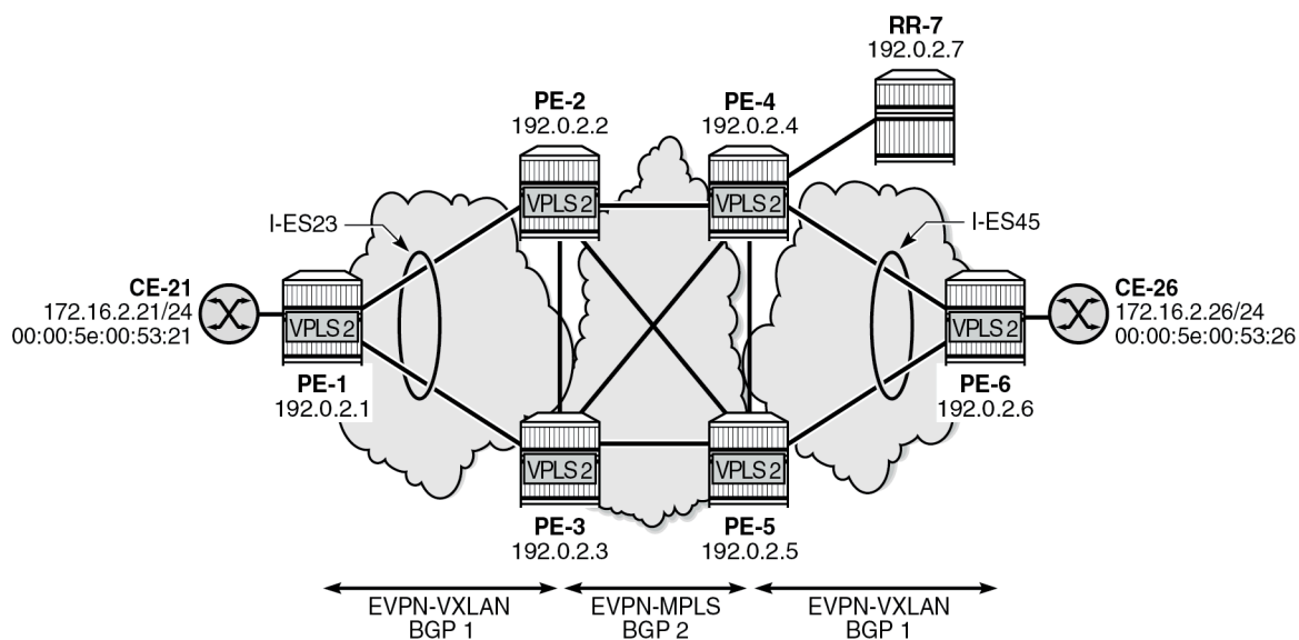
Figure 334: Example topology with dual-instance VPLS
