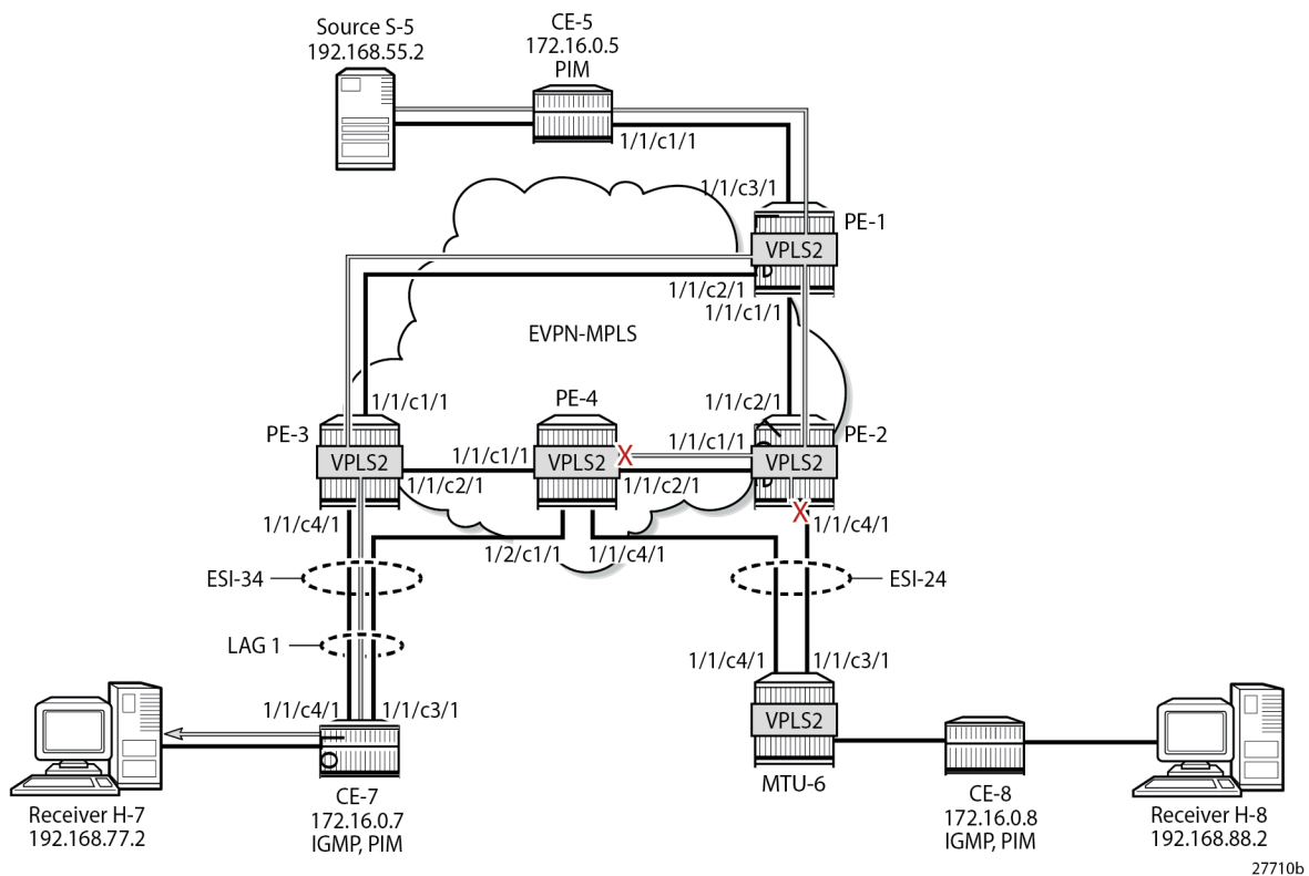
Figure 305: EVPN-MPLS with All-active Multi-homing and PIM Snooping Enabled – Receiver H-7 Joined
