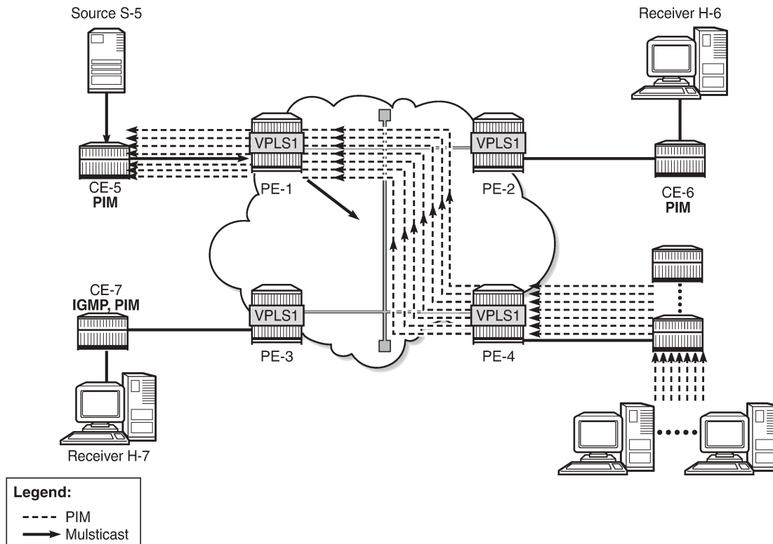
Figure 295: Multicast in VPLS with PIM Snooping in Snoop Mode – Multiple CEs
