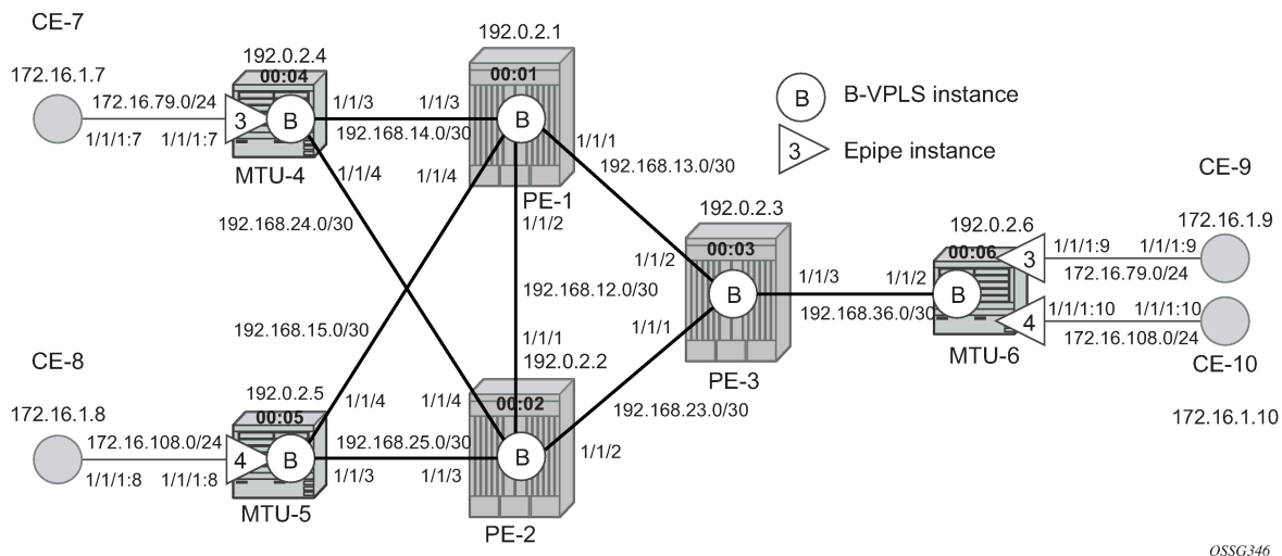
Figure 276: Setup detailed view
