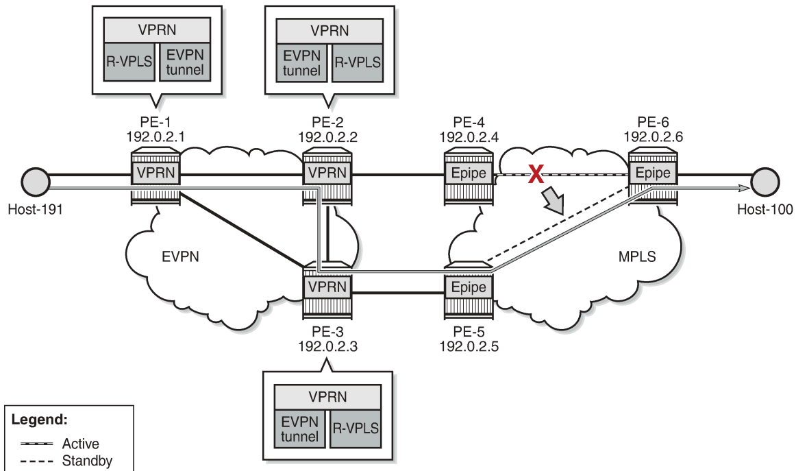
Figure 208: Hairpinning in a broadcast domain after switchover for SR OS Releases earlier than Release 19.10.R3
