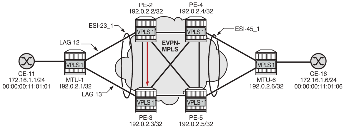
Figure 256: DF switchover in single-active ESI-23_1
