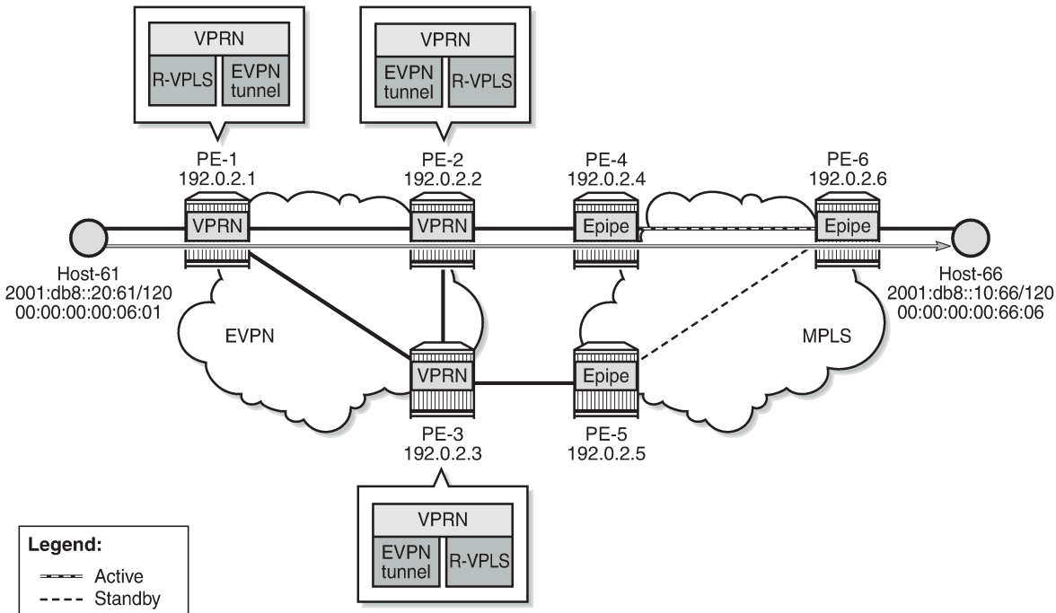
Figure 215: Example topology for initial forwarding path via PE-2 with IPv6 addresses
