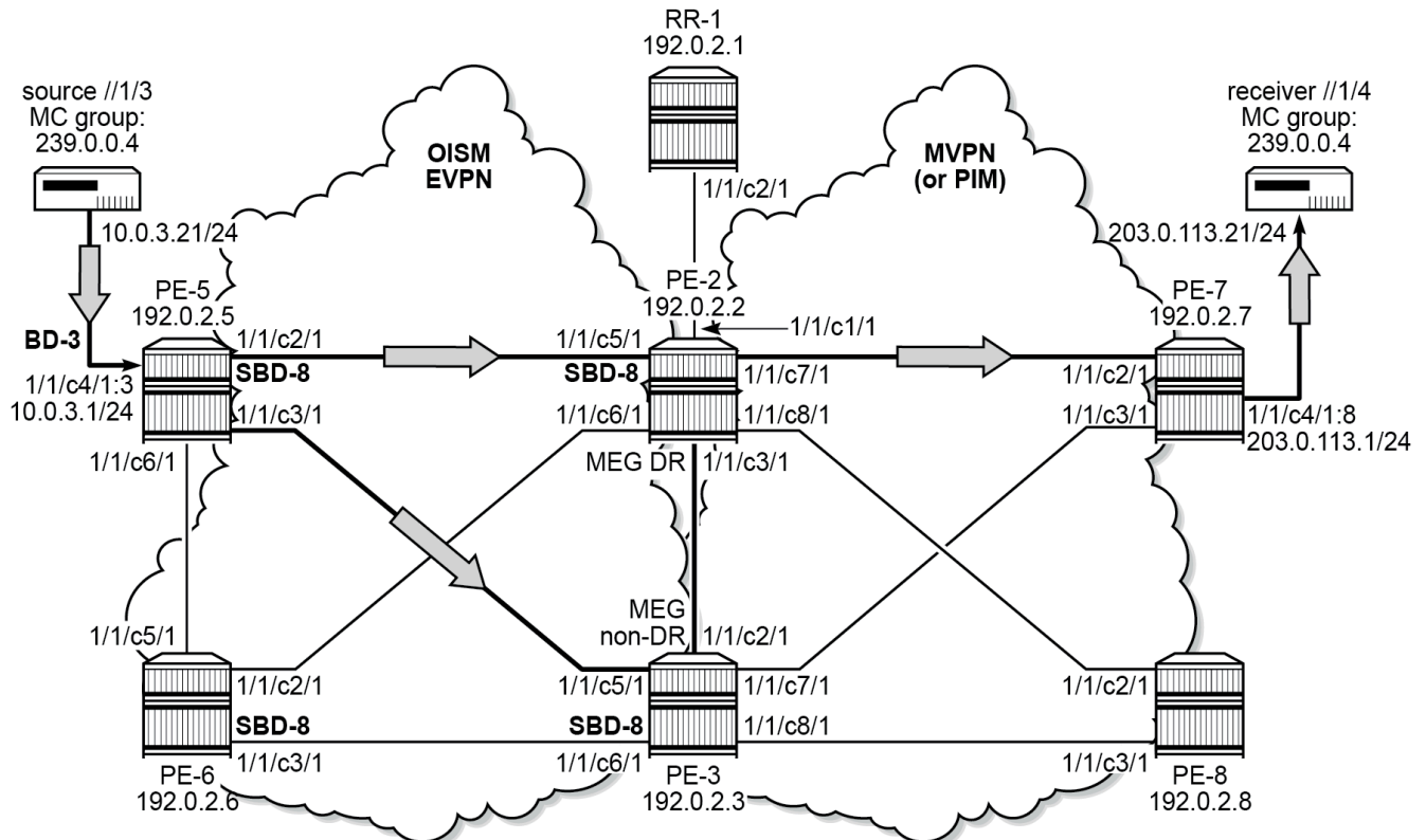
Figure 249: EVPN MC source - MVPN/PIM MC receiver example setup, with DR as UMH for PE-7
