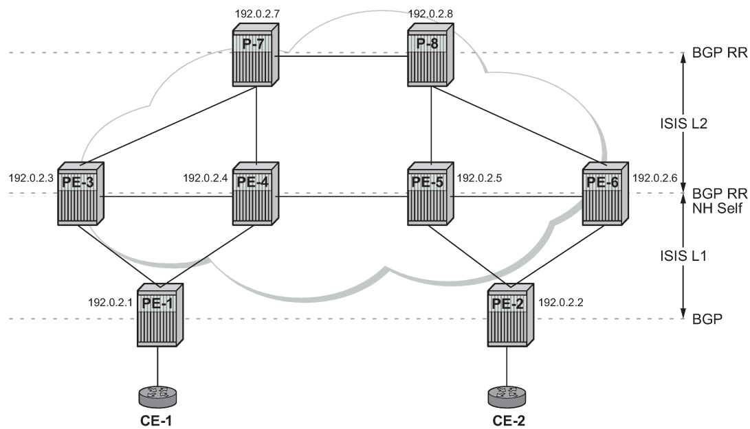
Figure 240: Intra-AS MS-PW example topology
