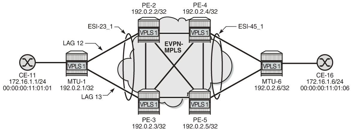
Figure 255: Sample topology with VPLS 1
