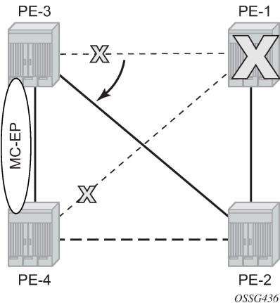
Figure 224: Core node failure
