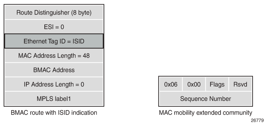
Figure 279: EVPN BMAC route with ISID indication
