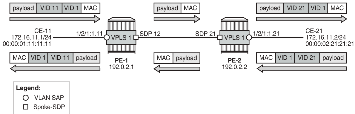
Figure 348: Traffic between two QinQ VLAN SAPs - VLAN translation
