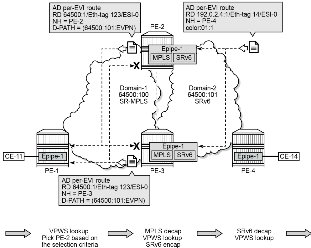
Figure 229: AD per-EVI route from SRv6 domain redistributed into MPLS domain
