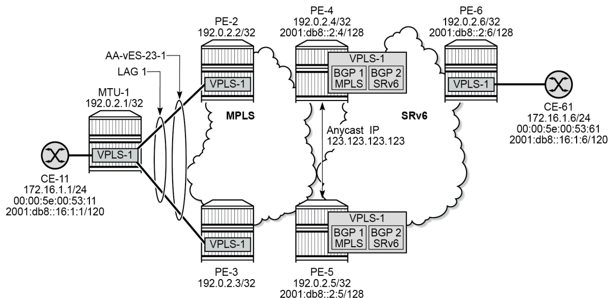
Figure 147: Example topology with VPLS-1
