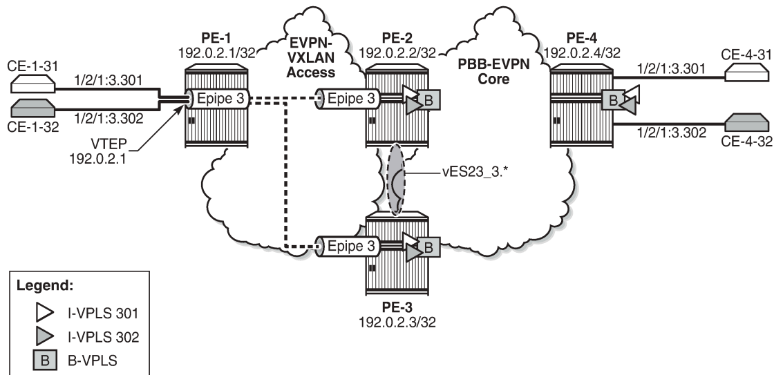
Figure 253: Epipe 3 with EVPN-VXLAN and SA MH ES
