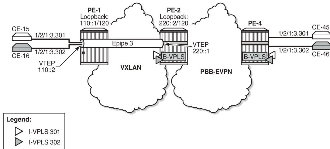
Figure 331: Example topology for static VXLAN termination on IPv6 addresses
