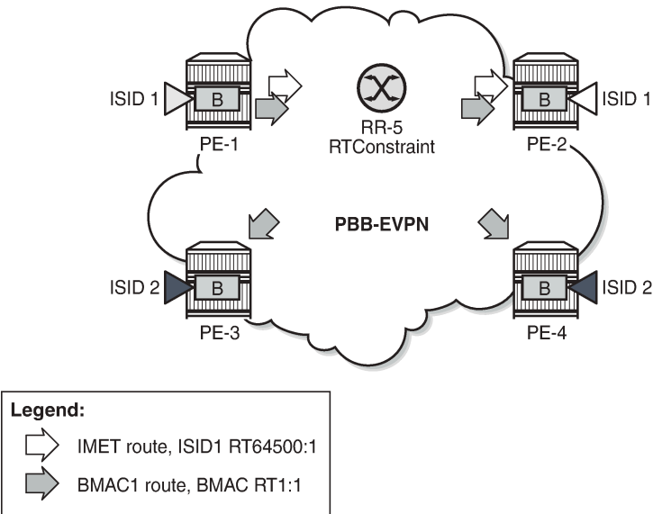
Figure 285: PBB-EVPN ISID-based RT
