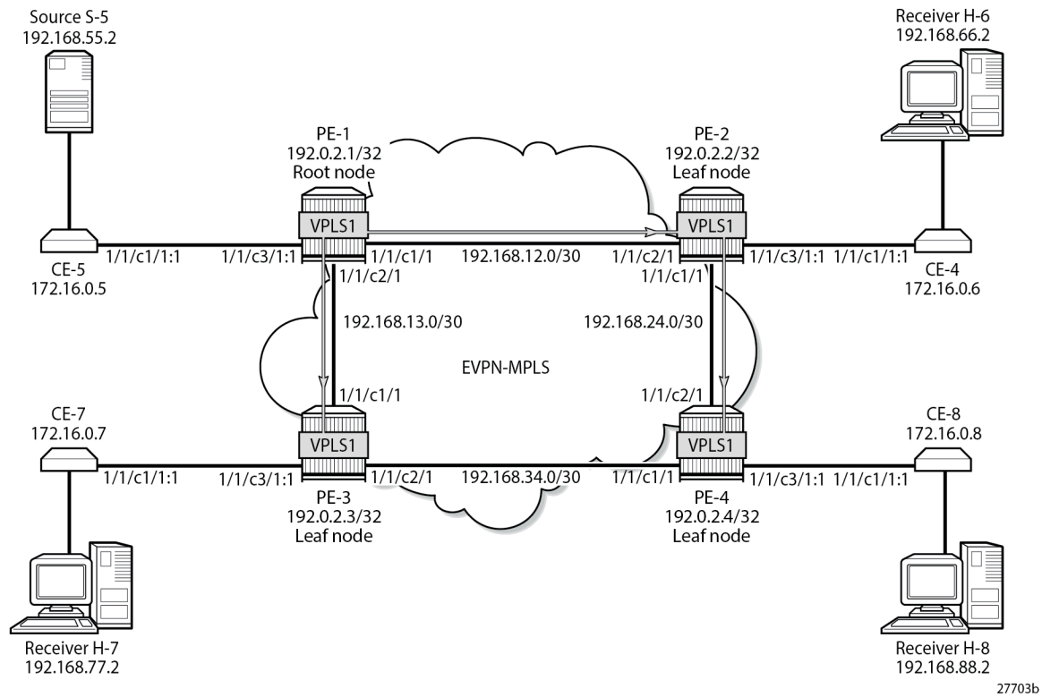
Figure 298: P2MP mLDP Multicast Tree
