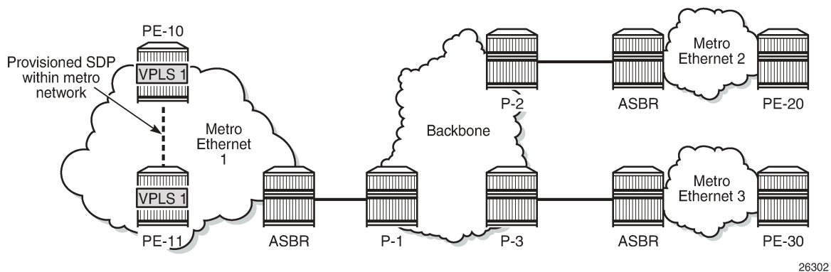
Figure 202: LDP VPLS using BGP-AD with use-provisioned-sdp option
