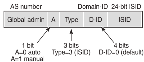
Figure 286: PBB-EVPN ISID-based RT format
