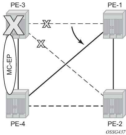
Figure 225: Multi-chassis node failure
