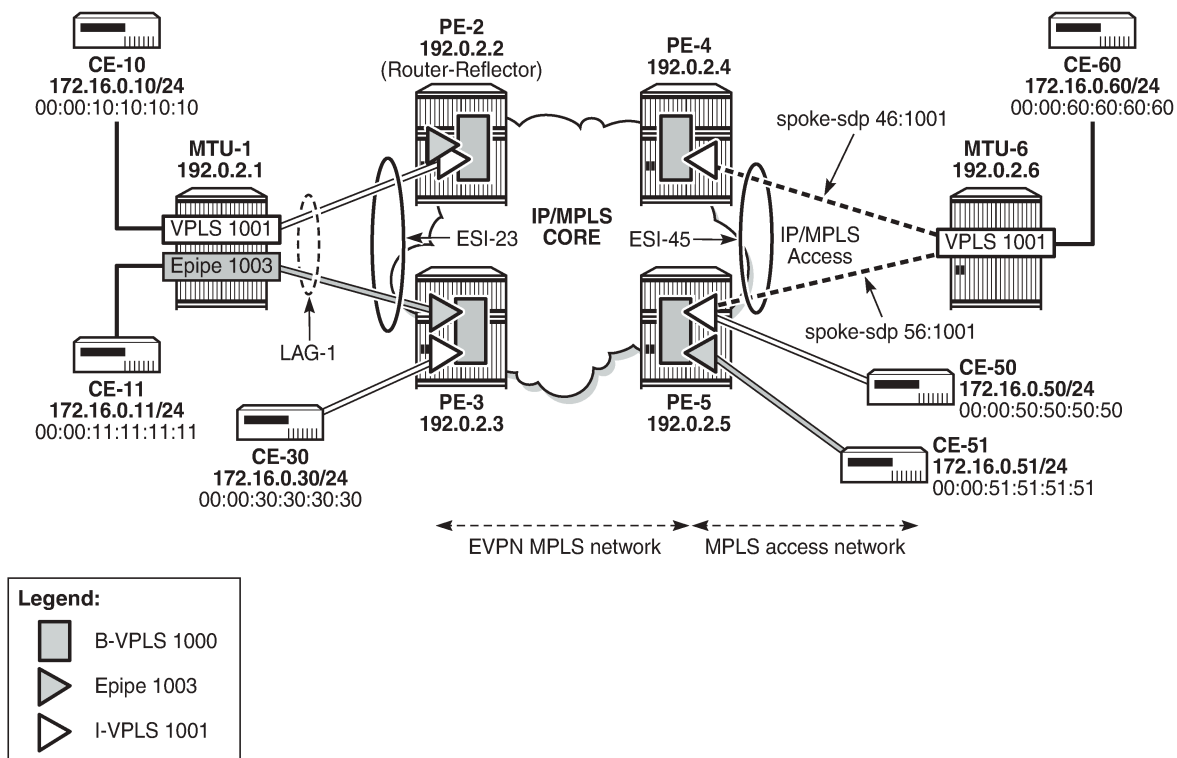
Figure 77: PBB-EVPN multi-homing
