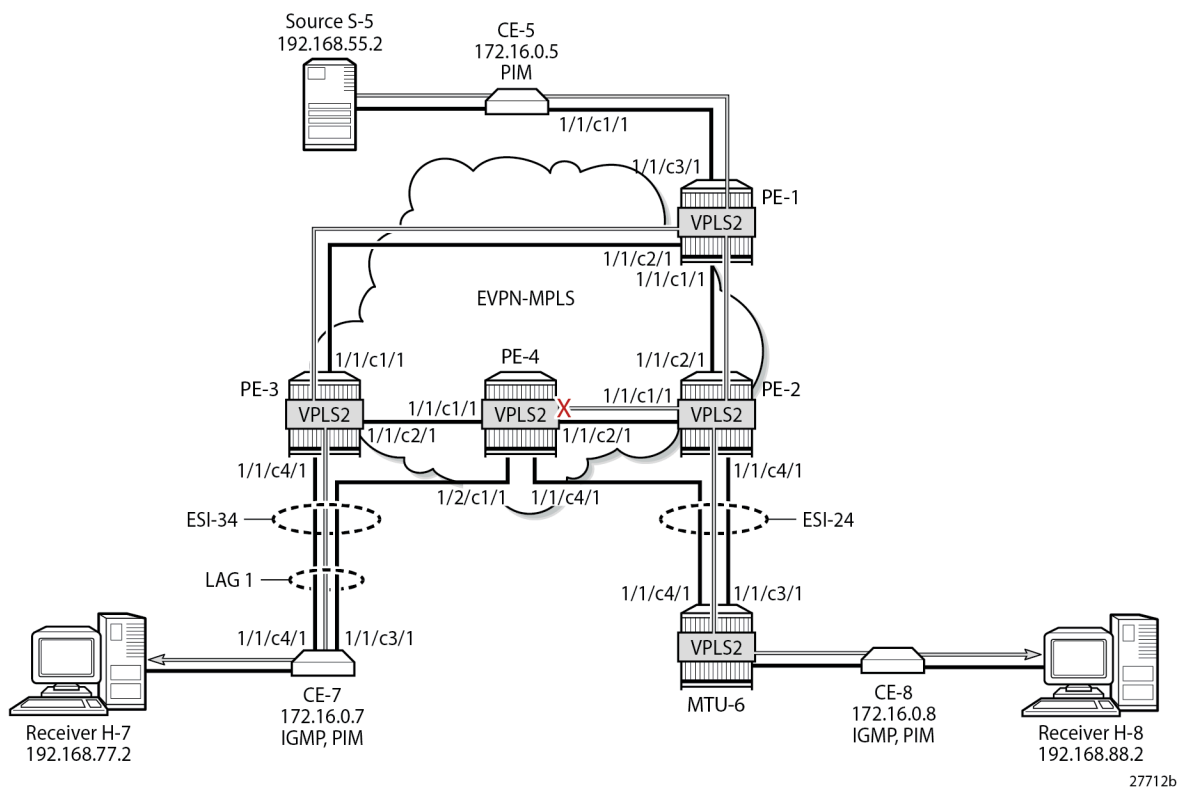
Figure 307: EVPN-MPLS with Multi-homing and PIM Snooping - Receivers H-7 and H-8 Joined
