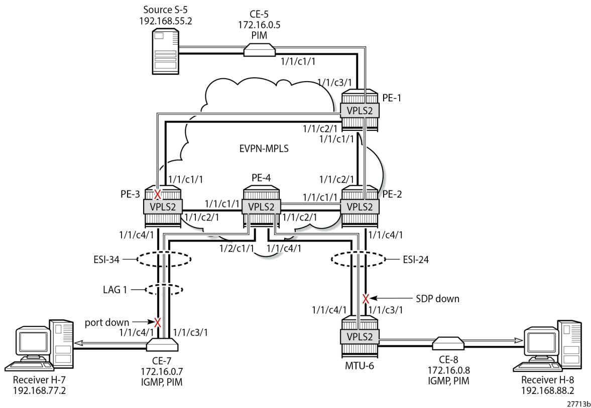
Figure 308: EVPN-MPLS with Multi-homing and PIM Snooping - Multicast Flow after Failover
