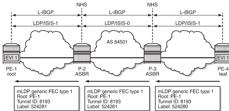
Figure 268: ABRs and leaf node send basic FEC in seamless MPLS
