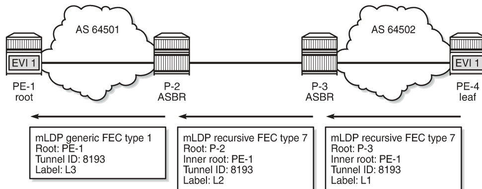
Figure 260: mLDP FEC label mapping messages for inter-AS model C
