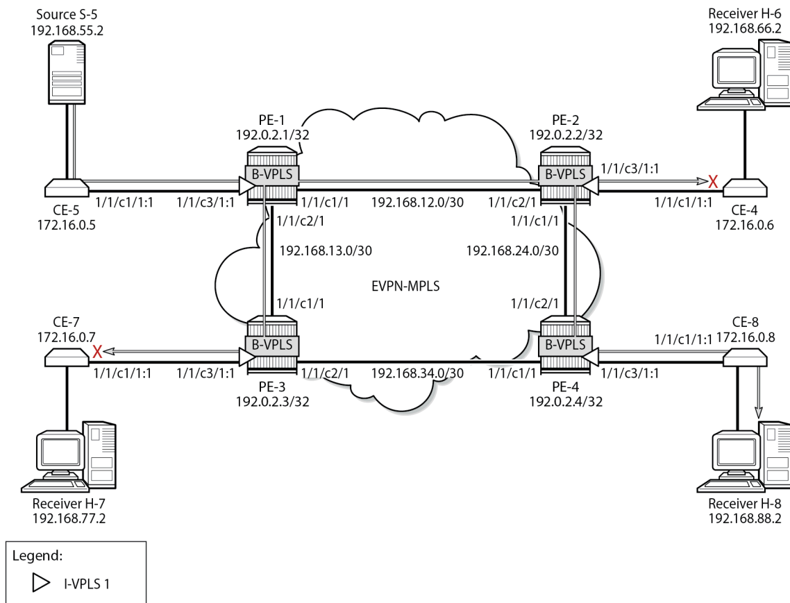
Figure 310: Multicast Stream to Receiver H-8 with PIM Snooping Disabled
