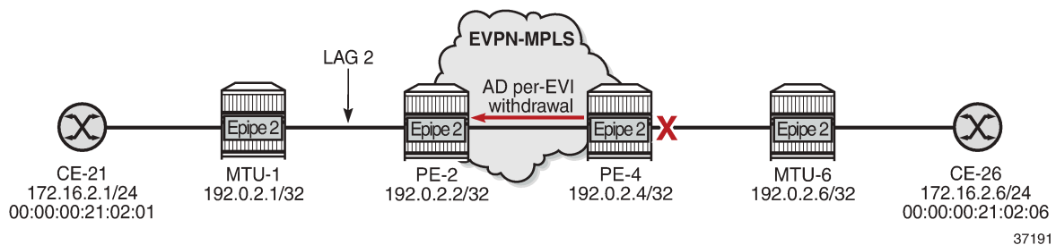
Figure 258: LLF in Epipe 2 - PE-4 failure
