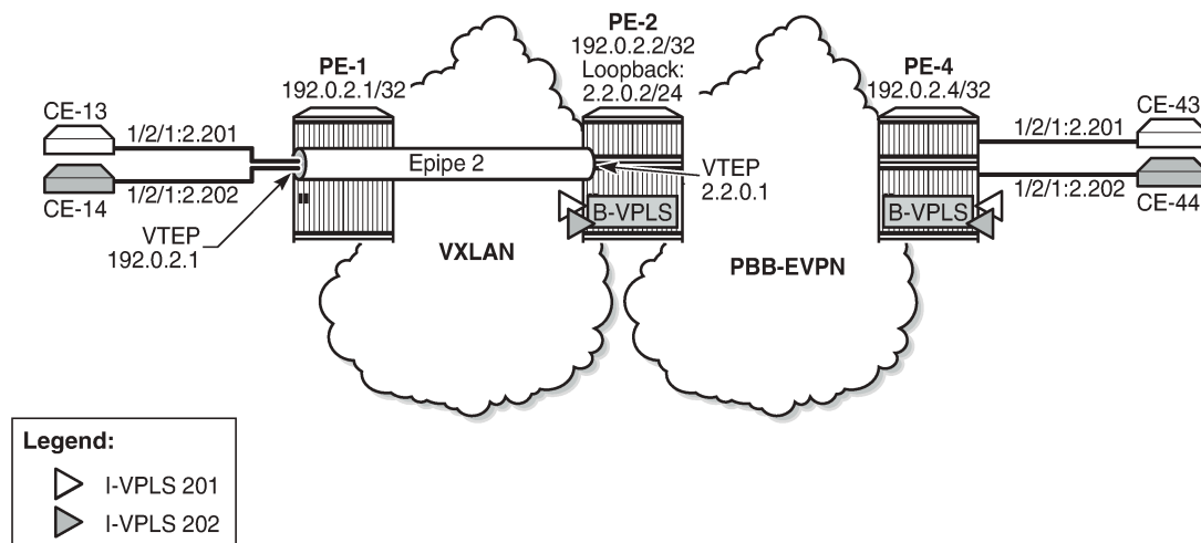
Figure 330: Example topology for static VXLAN termination on non-system IPv4 addresses
