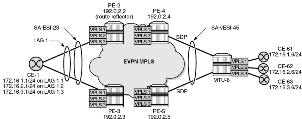
Figure 6: Example topology
