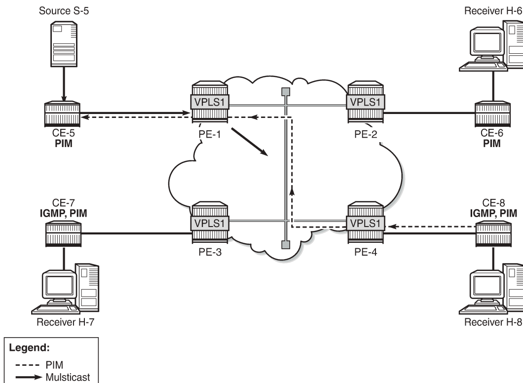
Figure 294: Multicast in VPLS with PIM Snooping in Snooping Mode
