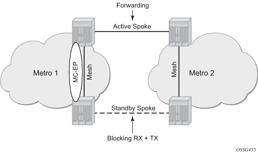
Figure 222: Multi-chassis endpoint with square resiliency
