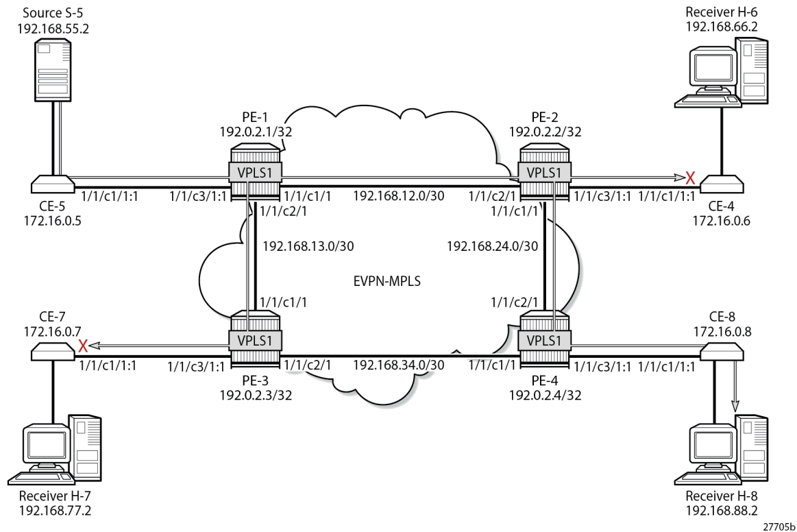
Figure 300: Multicast Stream (192.168.55.2, 232.1.1.1) with PIM Snooping Disabled
