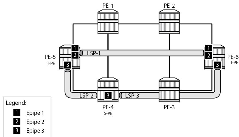
Figure 337: Example topology
