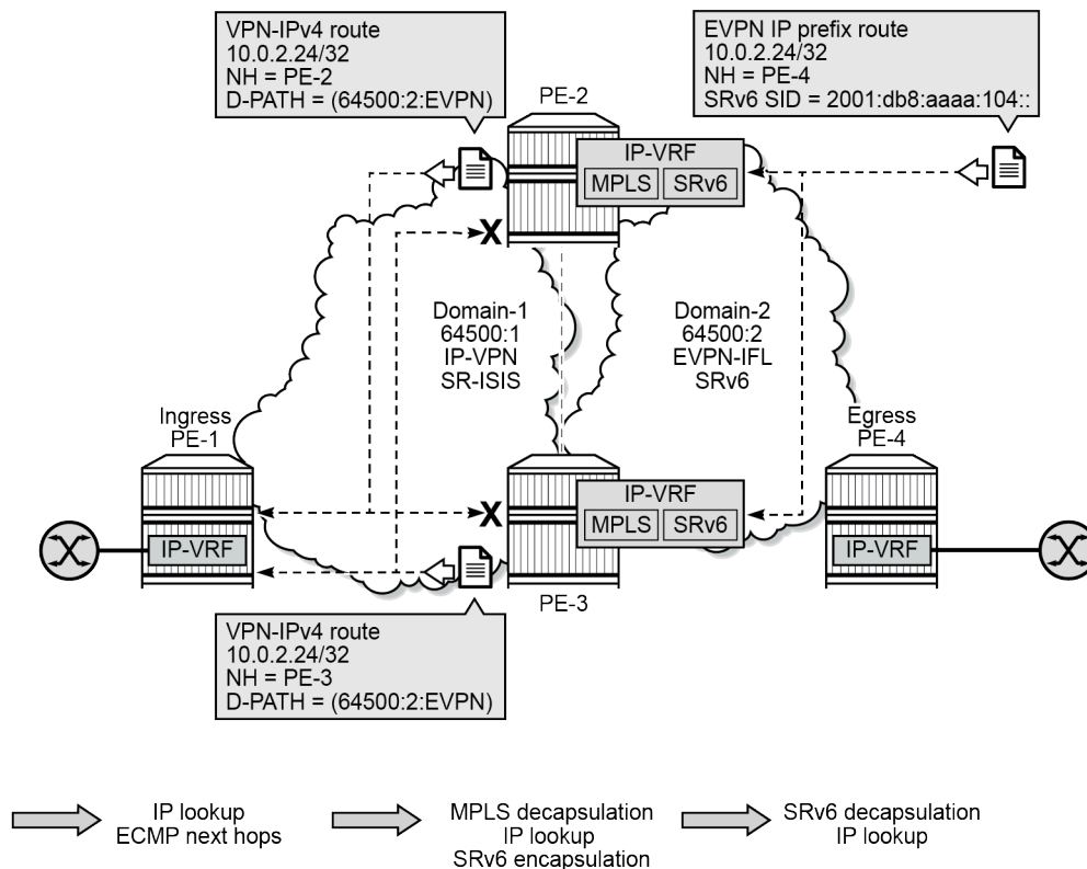
Figure 233: Interworking between EVPN-IFL and IP-VPN
