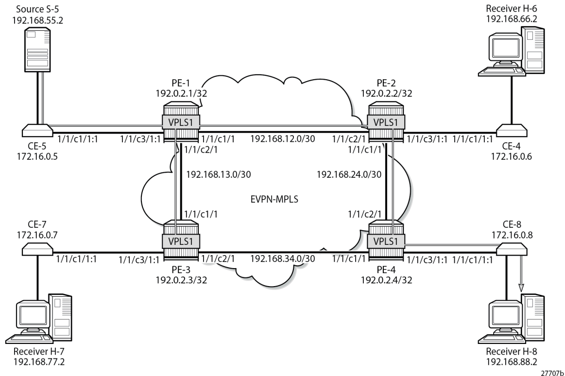
Figure 302: Multicast Stream (192.168.55.2, 232.1.1.1) with PIM Snooping Enabled
