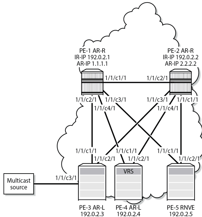
Figure 198: Example topology
