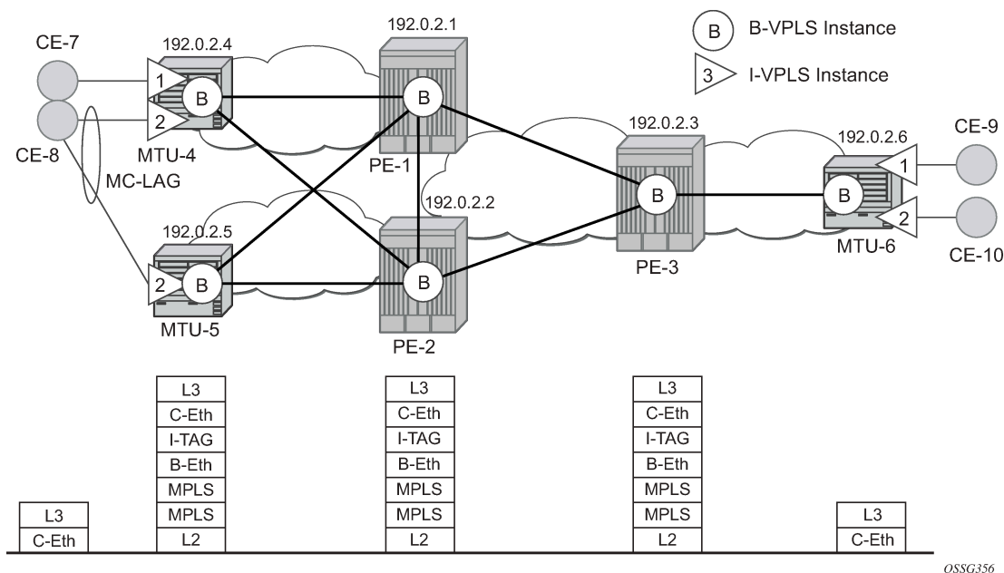
Figure 288: Example topology including B-VPLS, I-VPLSs, and protocol stacks
