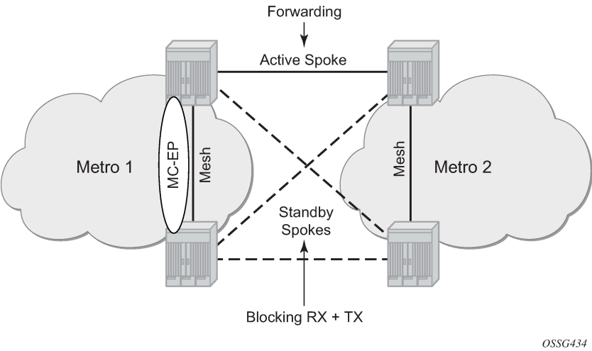
Figure 221: Multi-chassis endpoint with mesh resiliency
