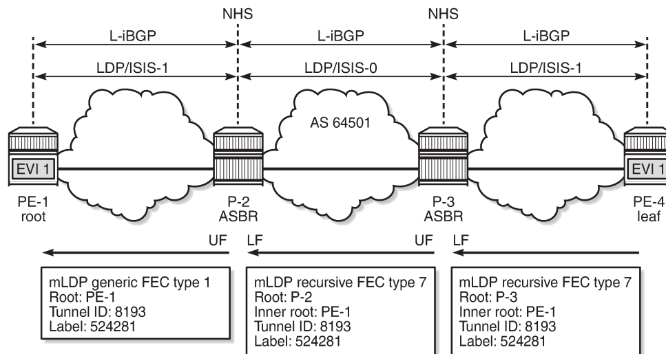
Figure 266: Recursive mLDP FEC for seamless MPLS
