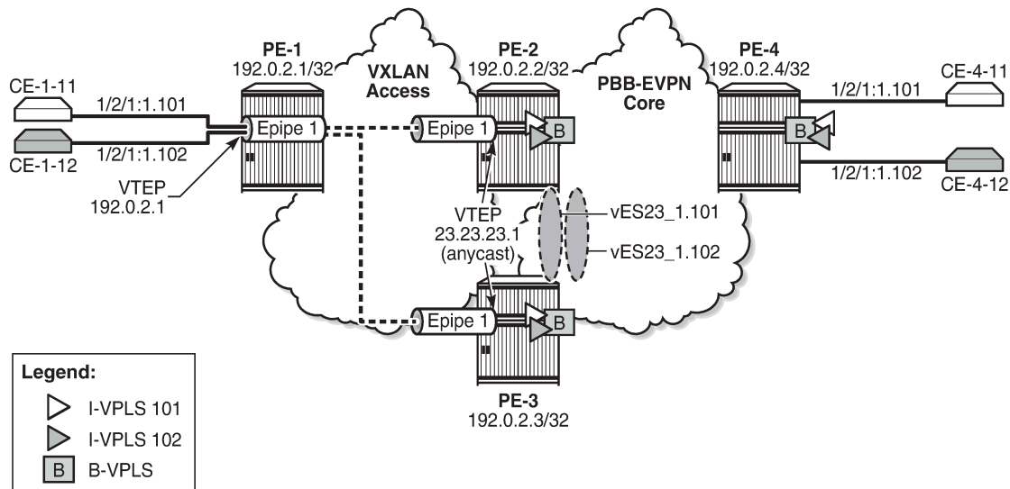
Figure 250: Epipe with static VXLAN termination
