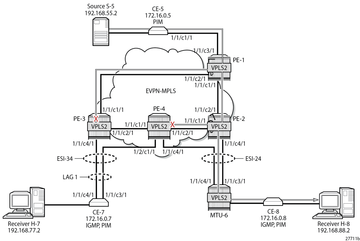
Figure 306: EVPN-MPLS with Single-active Multi-homing and PIM Snooping Enabled – Receiver H-8 Joined
