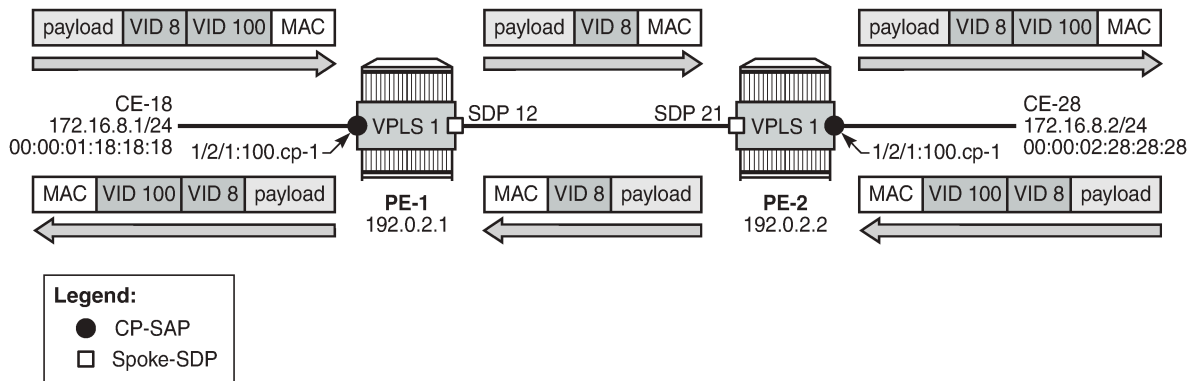
Figure 342: Customer VID is preserved between QinQ CP SAPs - no VLAN translation
