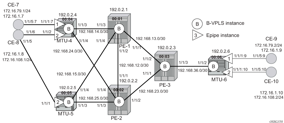
Figure 289: Example topology with port numbers and IP addresses
