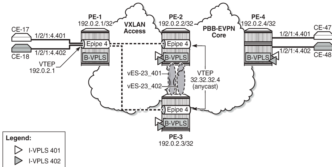
Figure 332: Example topology for static VXLAN termination using anycast
