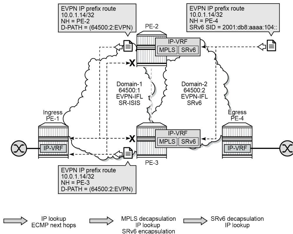
Figure 232: EVPN IP prefix routes readvertised between domains
