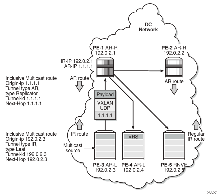
Figure 197: EVPN Assisted Replication for VXLAN
