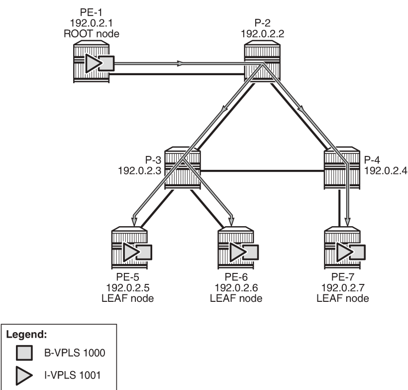
Figure 274: P2MP mLDP in PBB-EVPN
