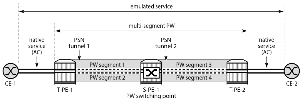
Figure 336: PW reference model
