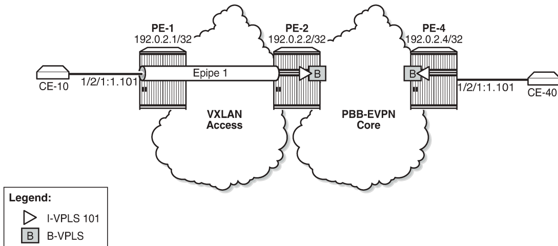
Figure 320: Static VXLAN termination on system IP addresses
