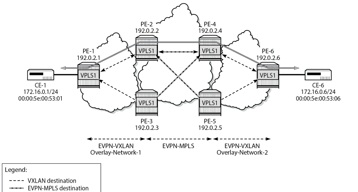
Figure 172: EVPN destinations created on multi-homed anycast DC GWs
