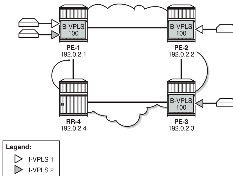
Figure 280: Example topology
