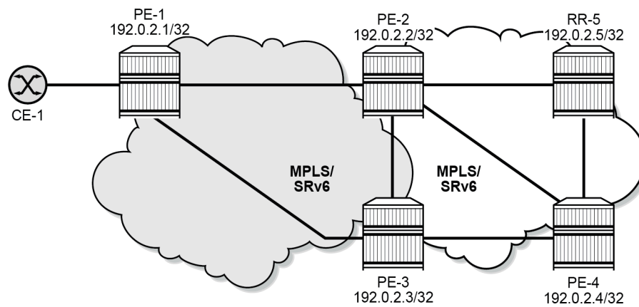
Figure 151: Example topology
