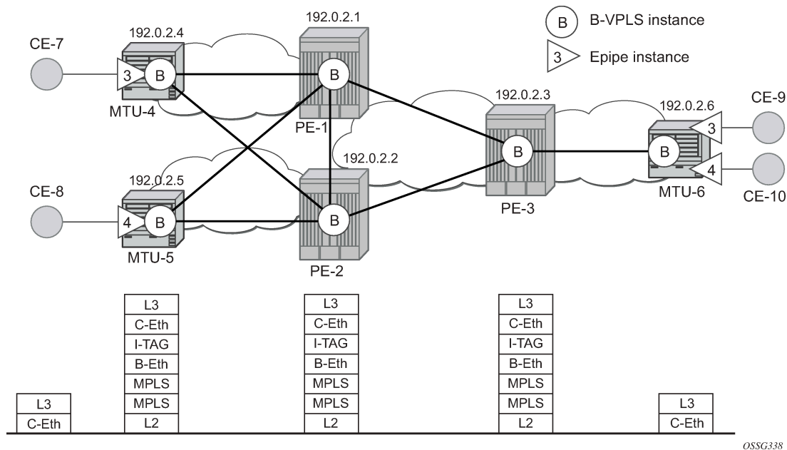
Figure 268: Example topology
