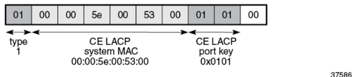
Figure 59: ESI type 1 example
