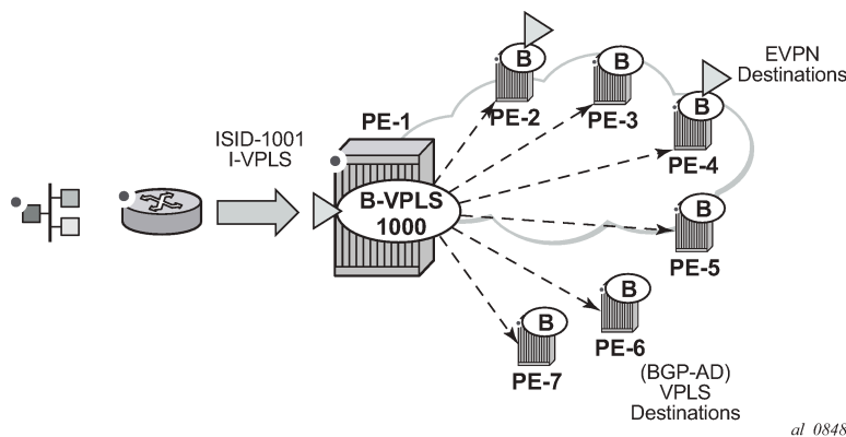
Figure 76: PBB-EVPN — flooding lists
