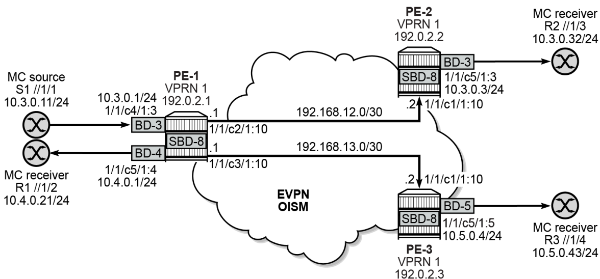
Figure 126: EVPN OISM example topology
