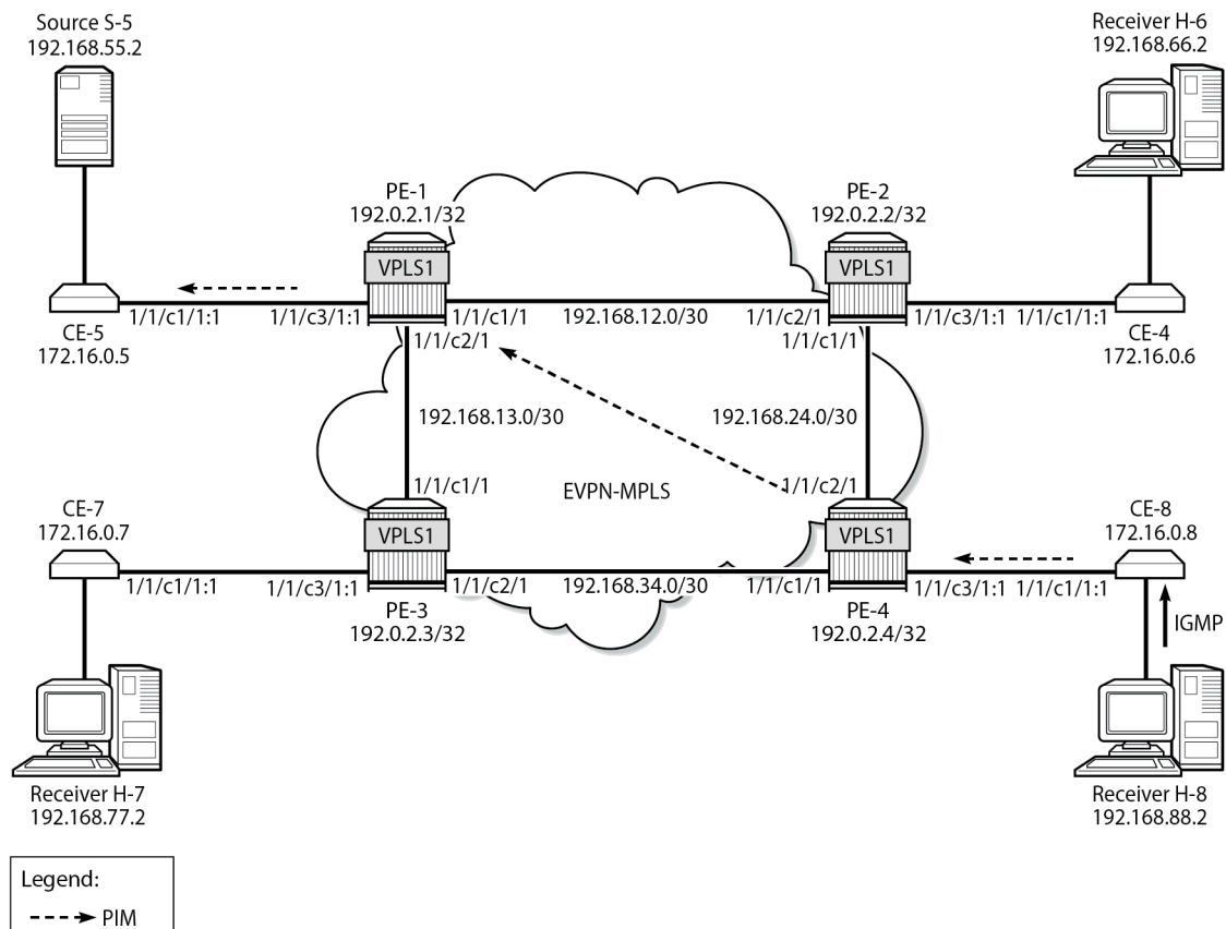
Figure 294: H-8 Joins (192.168.55.2, 232.1.1.1) and PIM Snooping is Enabled in Proxy Mode
