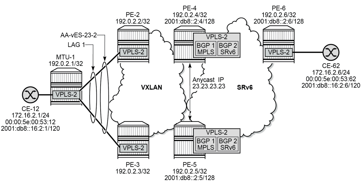
Figure 148: Example topology with VPLS-2
