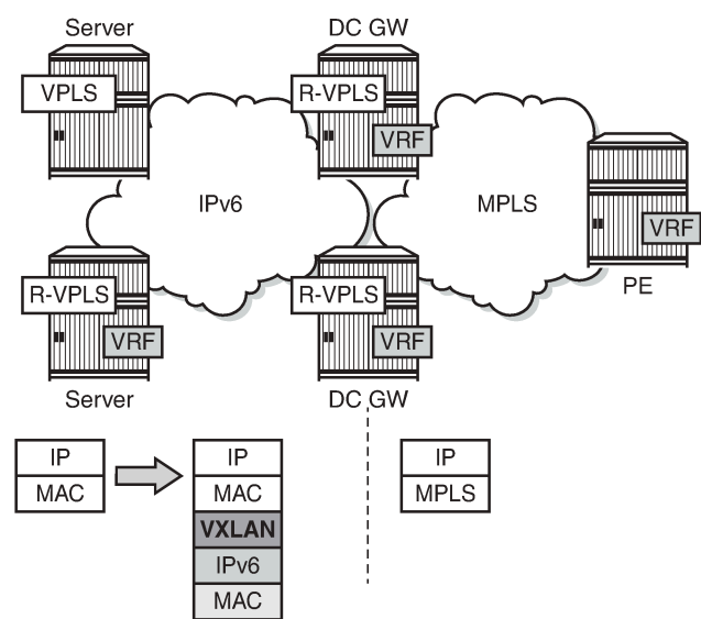
Figure 345: VXLAN IPv6 underlay for DC
