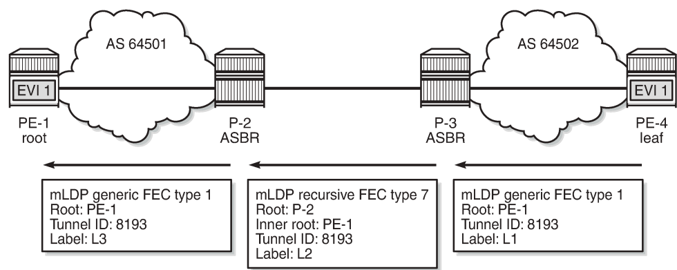
Figure 254: Non-recursive mLDP FEC for inter-AS model C
