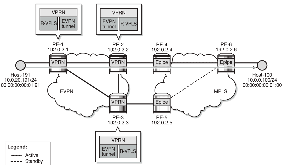
Figure 210: Initial situation with forwarding path via PE-2
