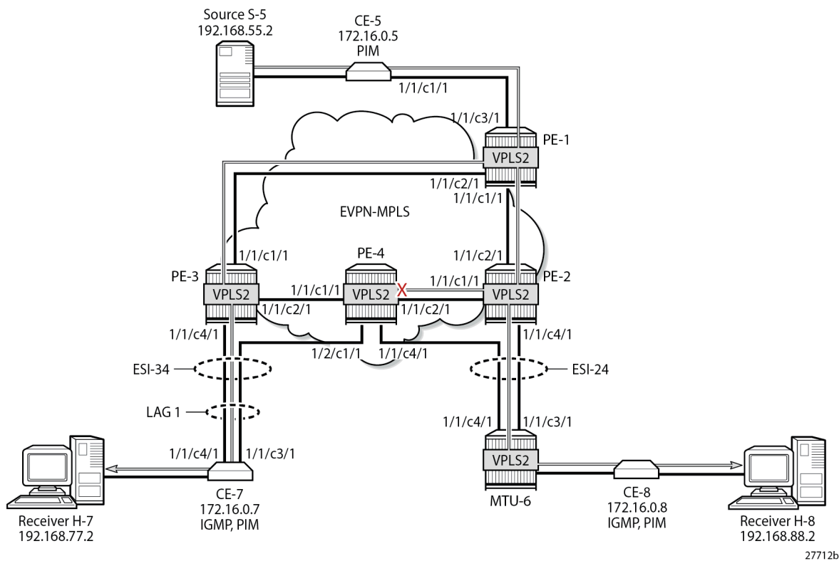
Figure 300: EVPN-MPLS with Multi-homing and PIM Snooping - Receivers H-7 and H-8 Joined
