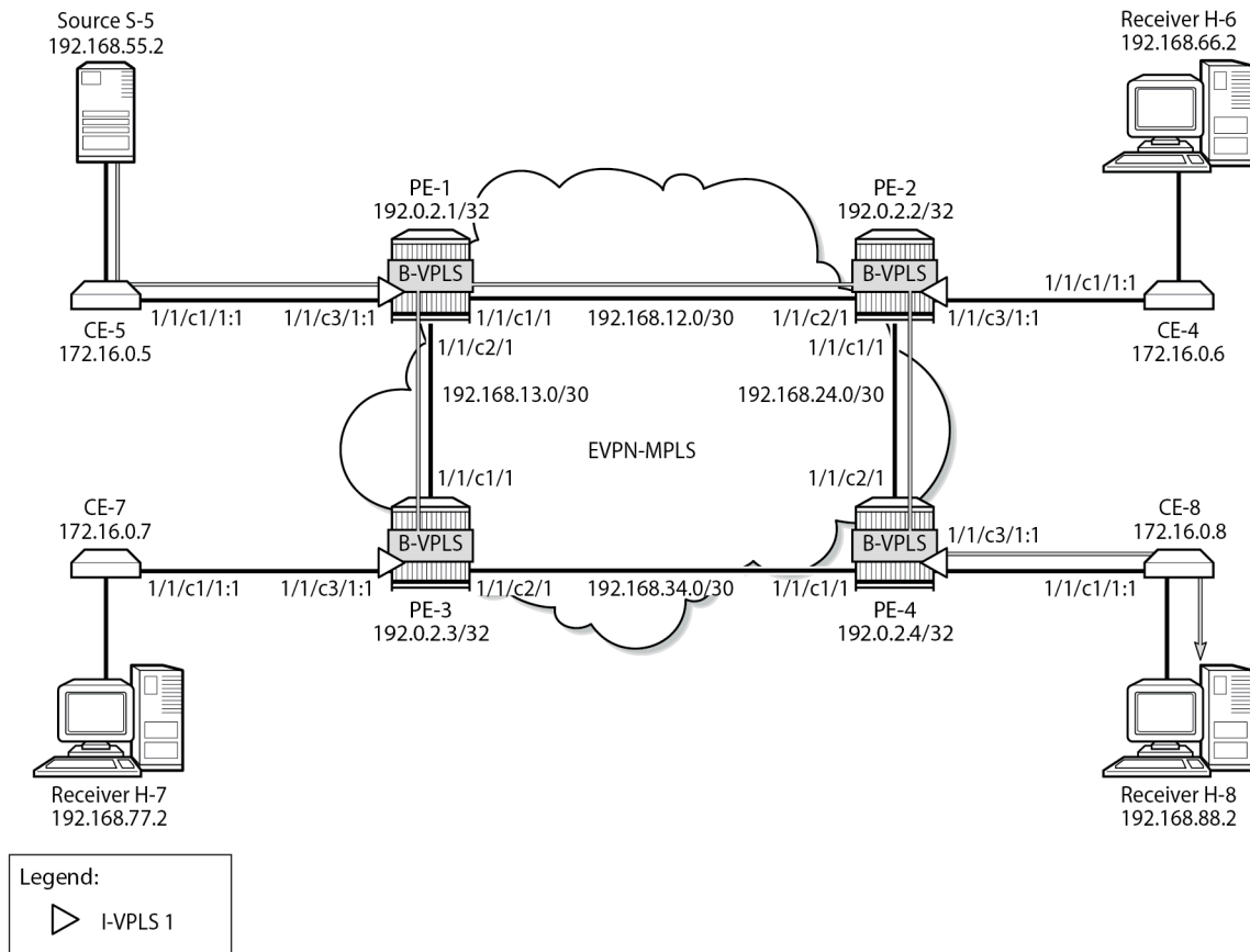
Figure 304: Multicast Stream to Receiver H-8 with PIM Snooping Enabled
