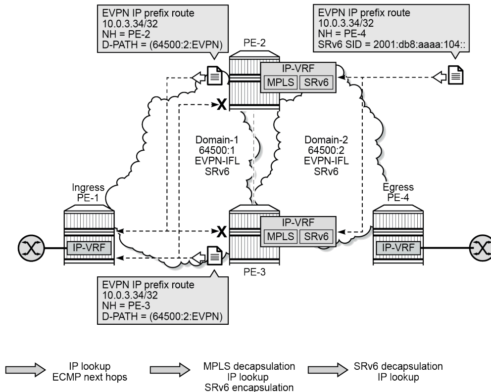
Figure 234: EVPN IP prefix routes readadvertised between SRv6 domains
