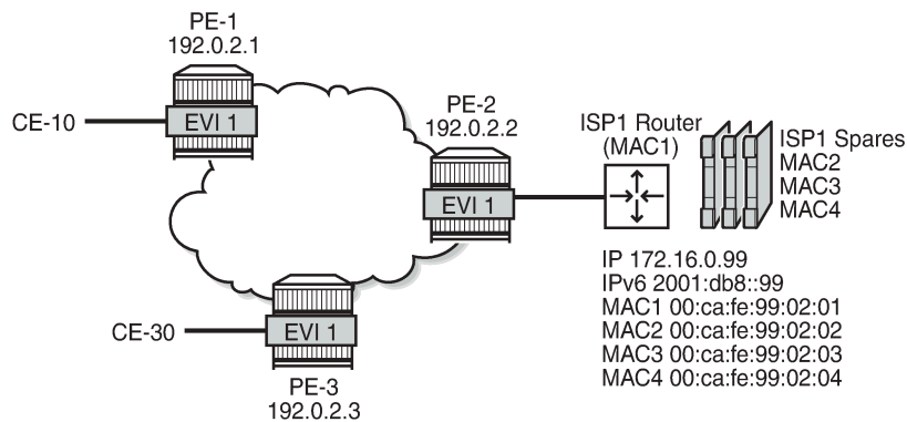
Figure 314: Example topology
