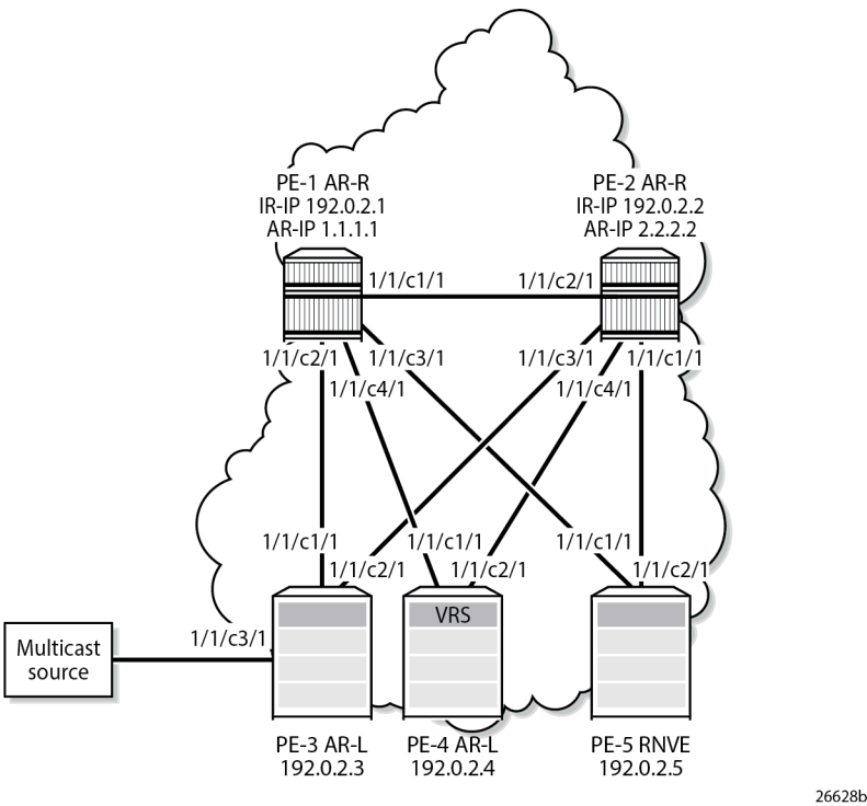
Figure 197: Example topology
