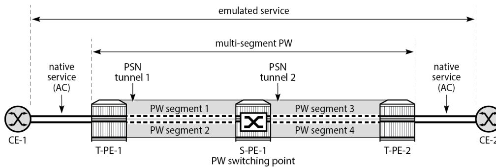
Figure 328: PW reference model
