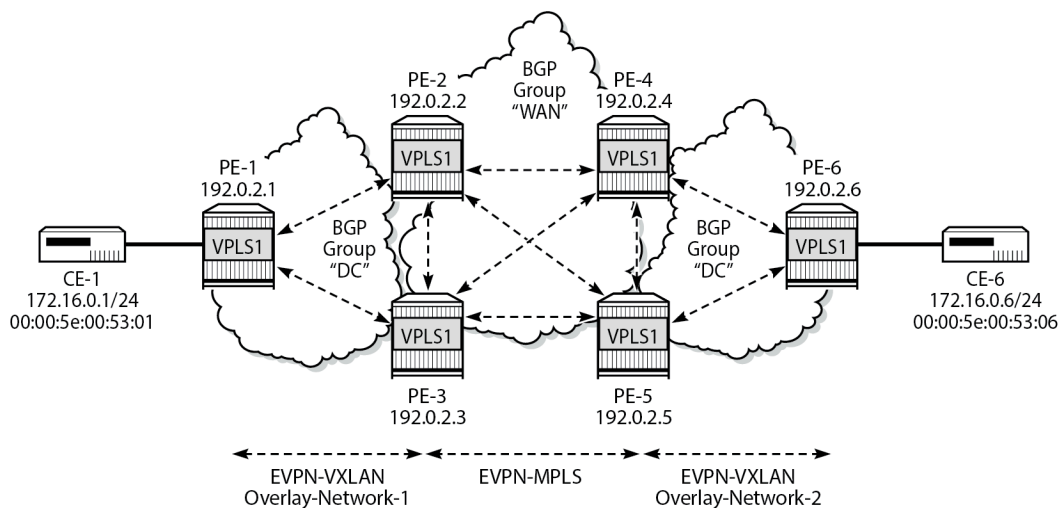
Figure 171: EVPN-MPLS interconnect for EVPN-VXLAN - example topology
