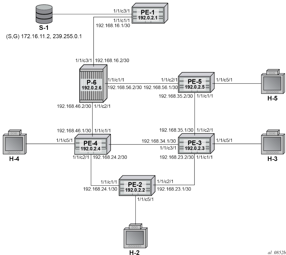
Figure 62: Schematic Topology
