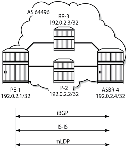
Figure 47: AS 64496 Protocols
