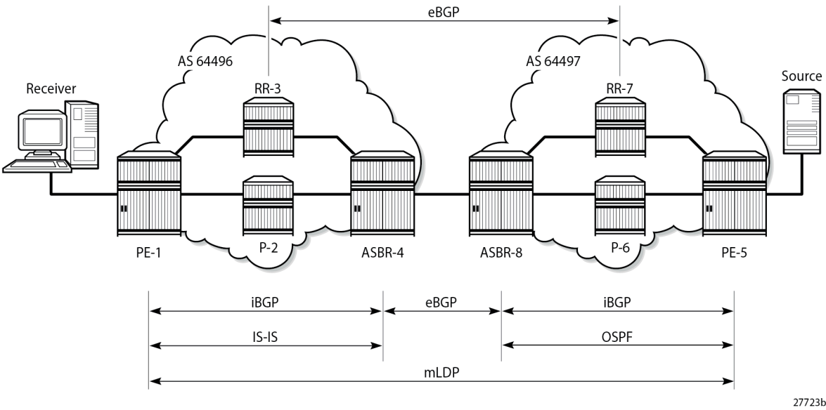
Figure 46: Inter-AS MVPN Protocol Requirements
