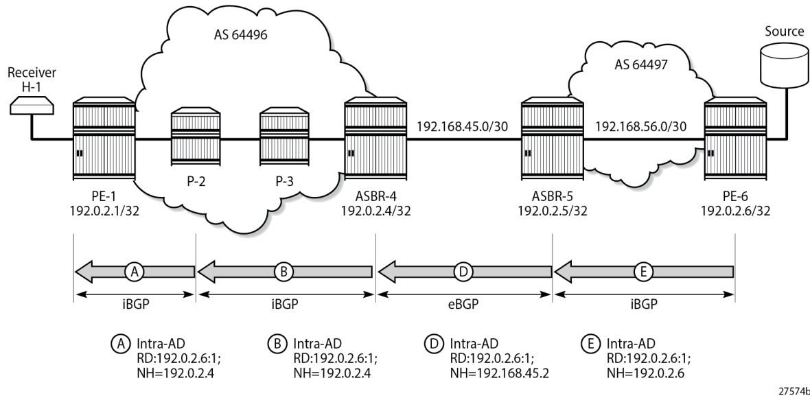
Figure 43: BGP MVPN Intra-AD Route Advertisement
