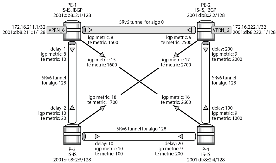
Figure 10: Example topology
