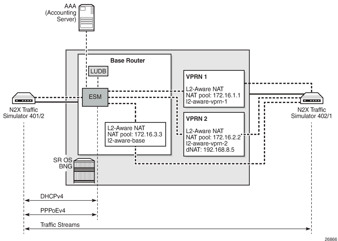
Figure 75: Test Setup
