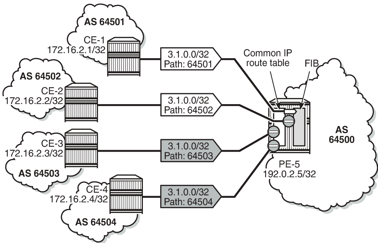
Figure 46: eBGP multipath with limit 2 and ECMP disabled
