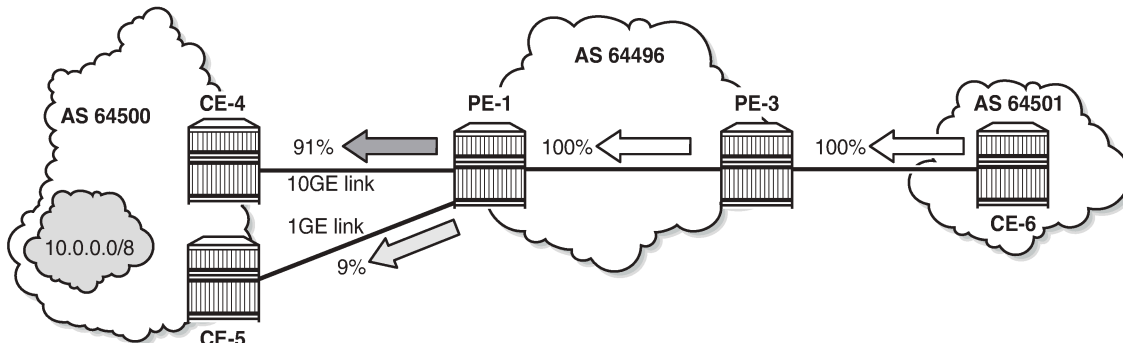
Figure 104: Standard ECMP - Unequal bandwidth links with EGBP
