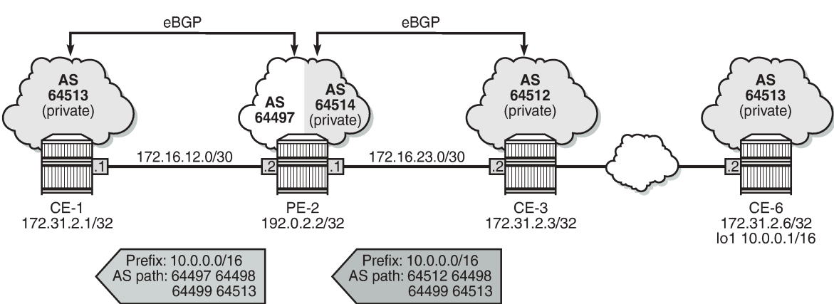
Figure 84: PE-2 removes the private ASNs except peer ASN 64513
