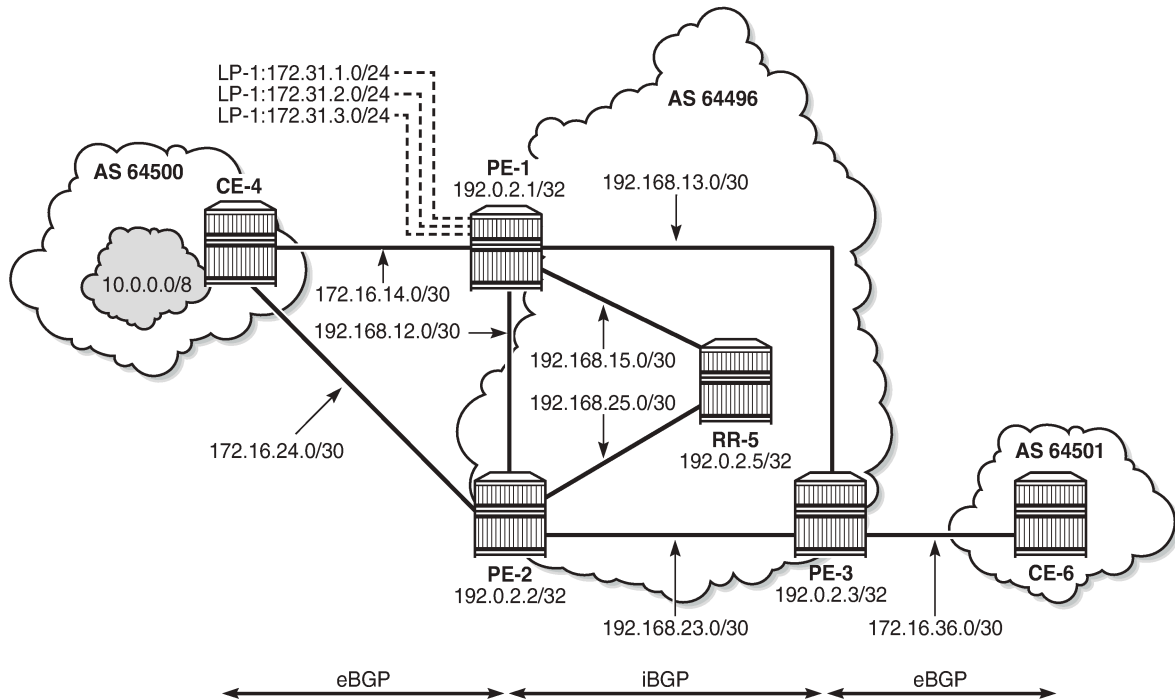
Figure 28: Example Topology
