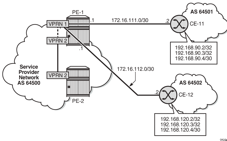
Figure 88: BGP IPv4 route leaking between VPRNs
