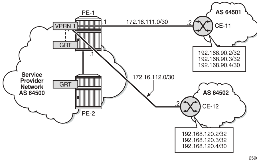
Figure 89: BGP IPv4 route leaking from VPRN to GRT
