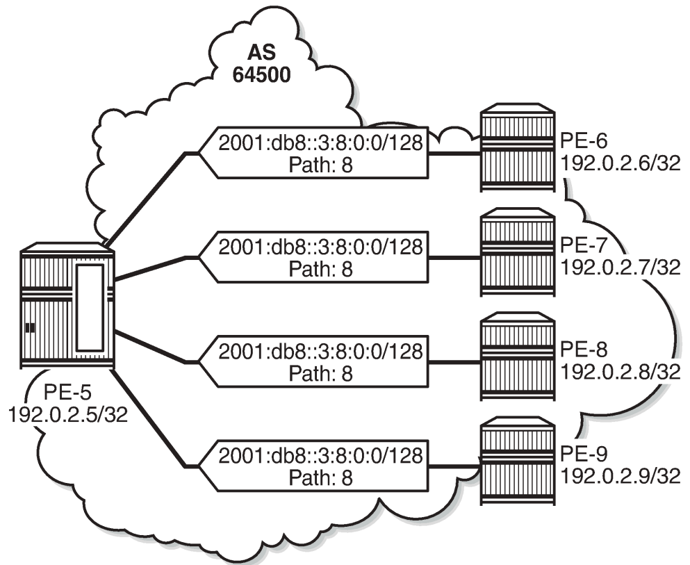
Figure 58: BGP multipath for the label-IPv6 address family
