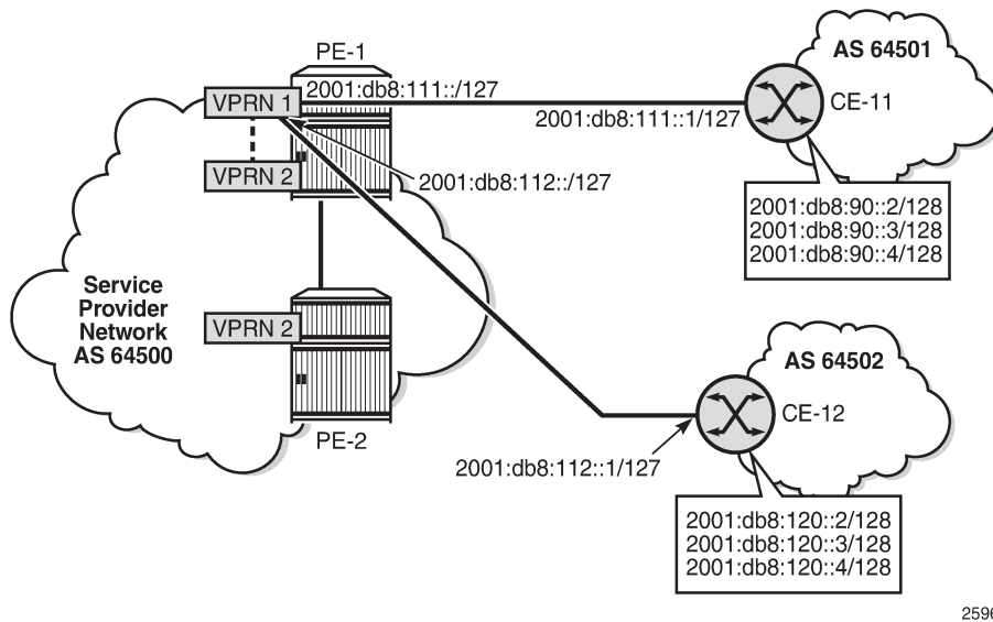
Figure 91: BGP IPv6 route leaking between VPRNs
