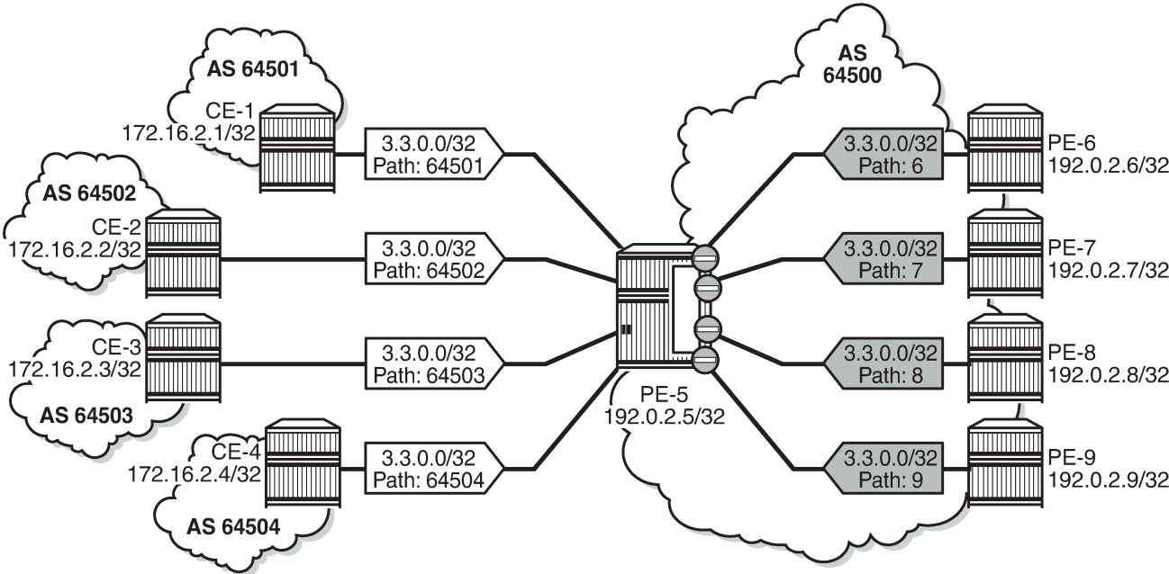
Figure 48: BGP multipath with limit 6 and eBGP preferred
