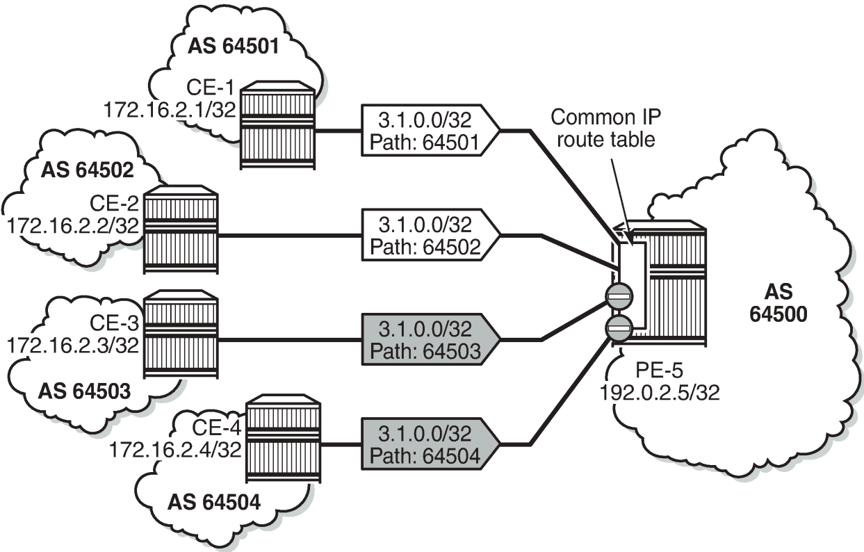
Figure 45: BGP multipath with eBGP limit 2
