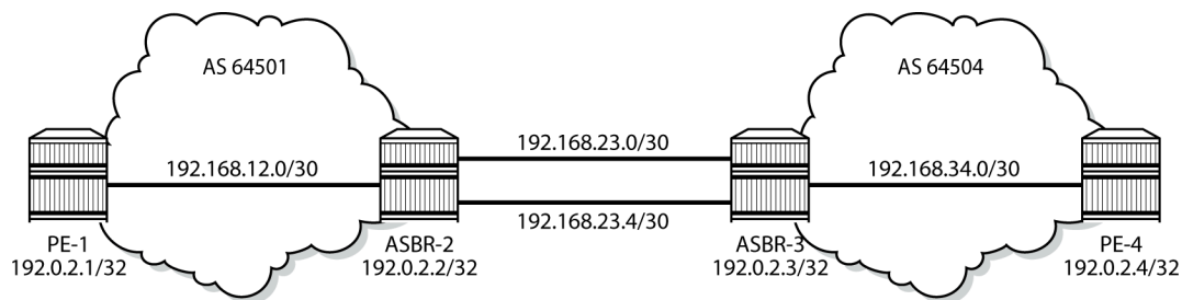
Figure 113: Example topology
