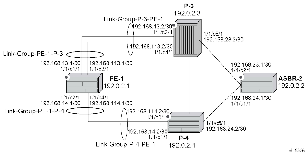
Figure 123: Example topology
