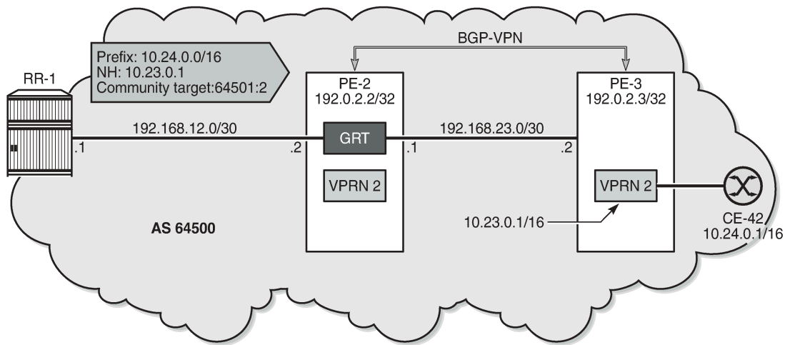
Figure 97: Leaked route 10.24.0.0/16 with next-hop resolved in VPRN 2 using VPN-IP
