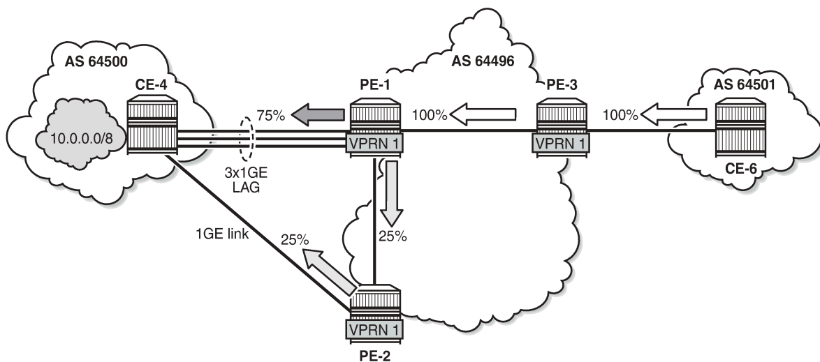
Figure 105: Weighted ECMP - Unequal bandwidth links with VPRN
