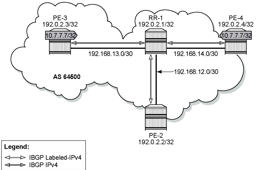
Figure 143: RR with labeled and unlabeled BGP sessions
