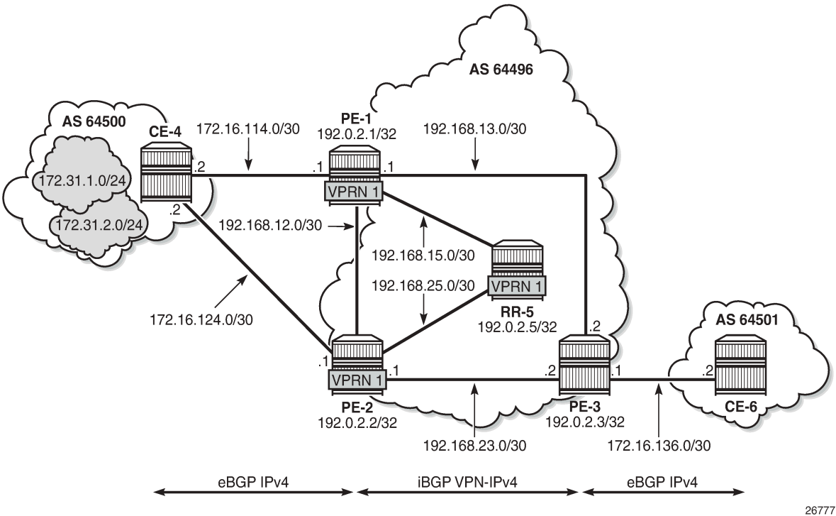
Figure 17: Example topology - VPN-IPv4
