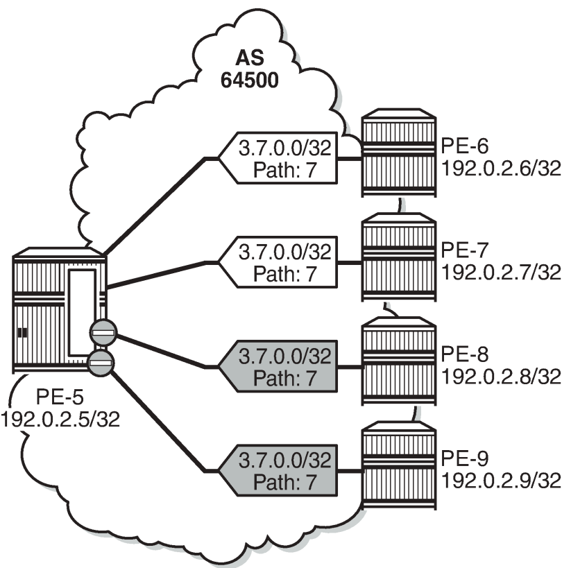
Figure 56: BGP multipath for the IPv4 address family
