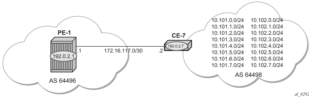
Figure 6: CE-7 connectivity
