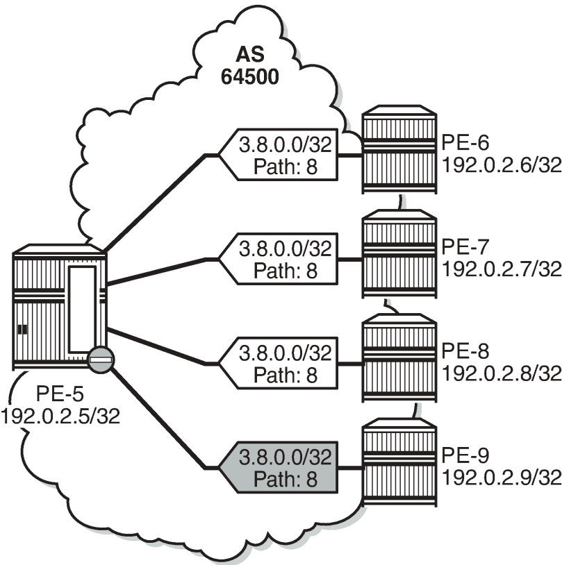
Figure 57: BGP multipath for the label-IPv4 address family
