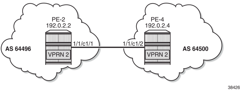
Figure 128: VPRN 2 in AS 64496 and in AS 64500
