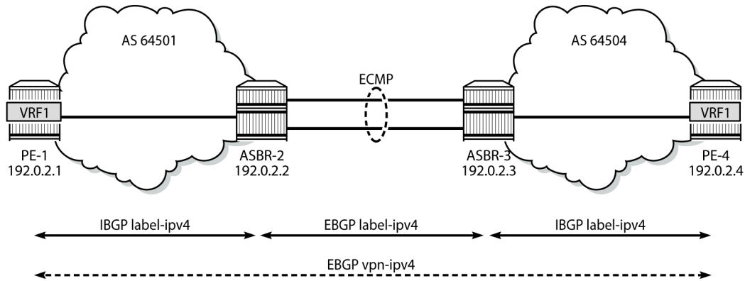
Figure 114: BGP peering
