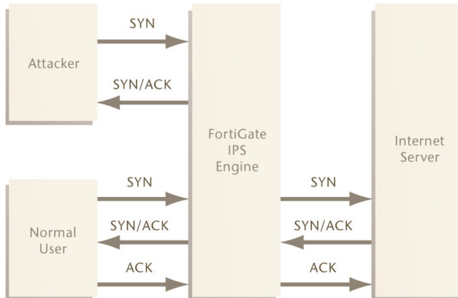
Figure 18: IPS operation after syn_flood threshold is reached
