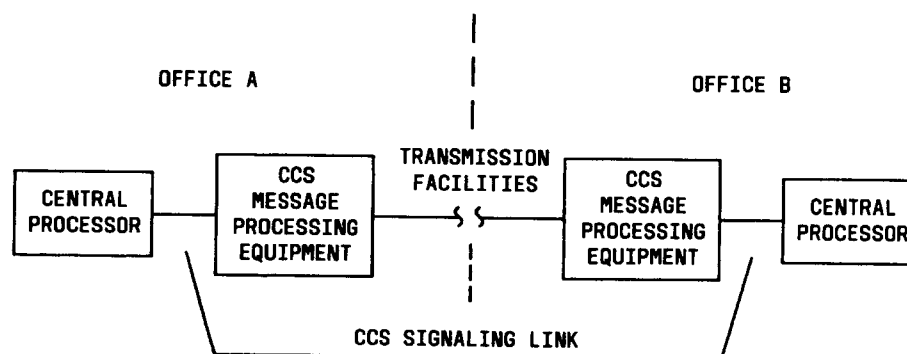
Fig. 1 — CCS Signaling Link
