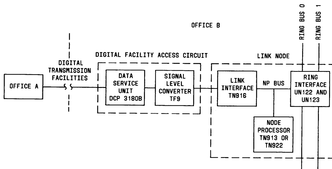
Fig. 9—Digital Facility Access Circuit (DCP 3180B Data Service Unit)
