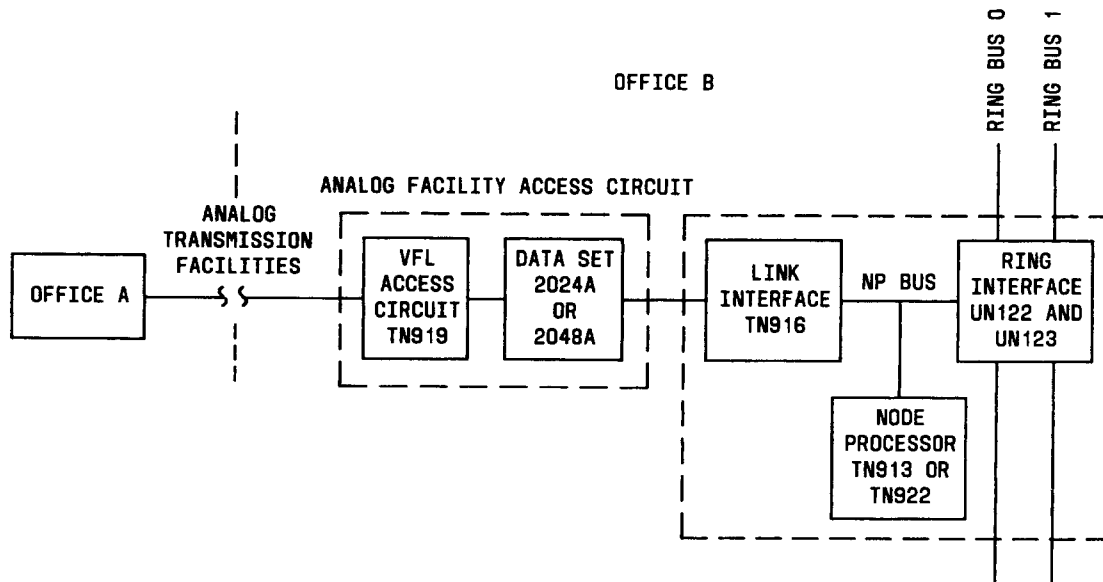
Fig. 3—Analog Signaling Link and STP Interface
