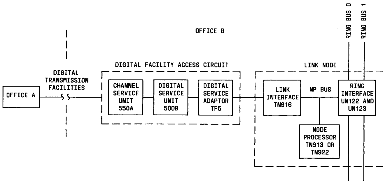
Fig. 6—Digital Facility Access Circuit (500B DSU/550A CSU)
