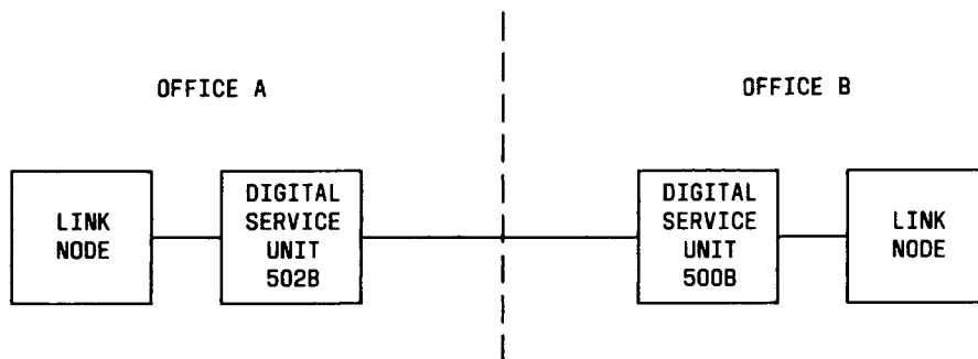
Fig. 7—Digital Signaling Link (1000 Feet or Less)
