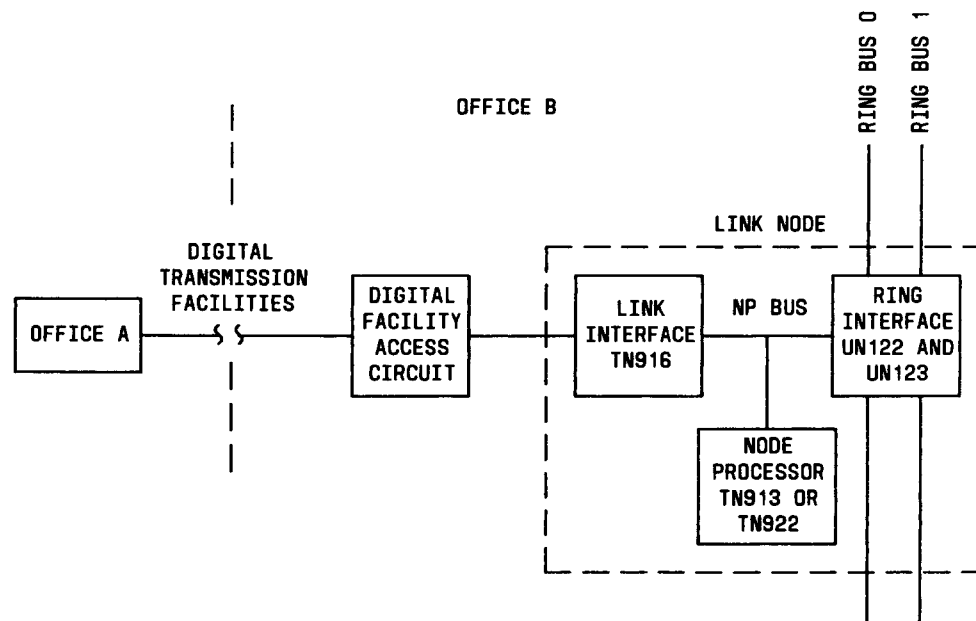
Fig. 5—Link Node Block Diagram
