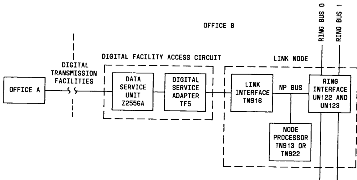
Fig. 10—Digital Facility Access Circuit (Z2556A Data Service Unit)
