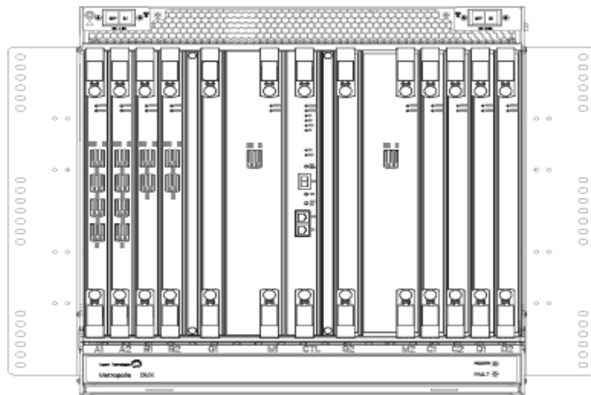
Figure 2-2 Metropolis® DMX High-Capacity shelf
