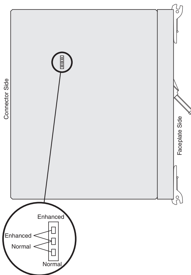
Figure 2-3 LNW26B, LNW28, LNW77 jumper location
