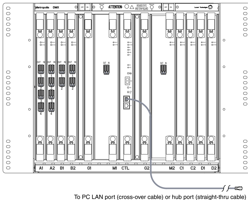
Figure 1-20 LAN cable installation to front of Metropolis® DMX High-Capacity shelf
