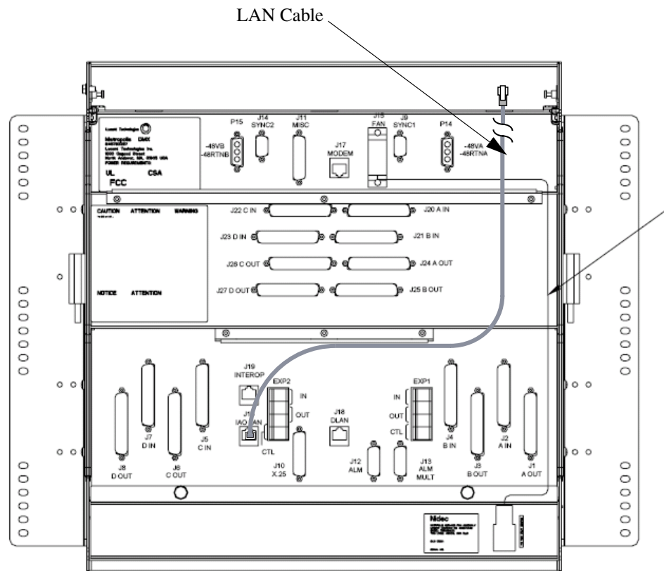
Figure 1-21 IAO LAN/TCP-IP cable installation to rear of Metropolis® DMX High-Capacity shelf
