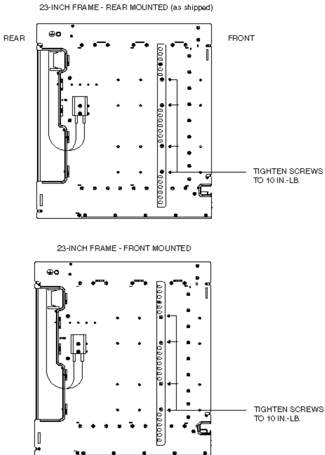
Figure 1-2 Metropolis® DMX High-Capacity shelf mounting bracket positions — 23-inch frame
