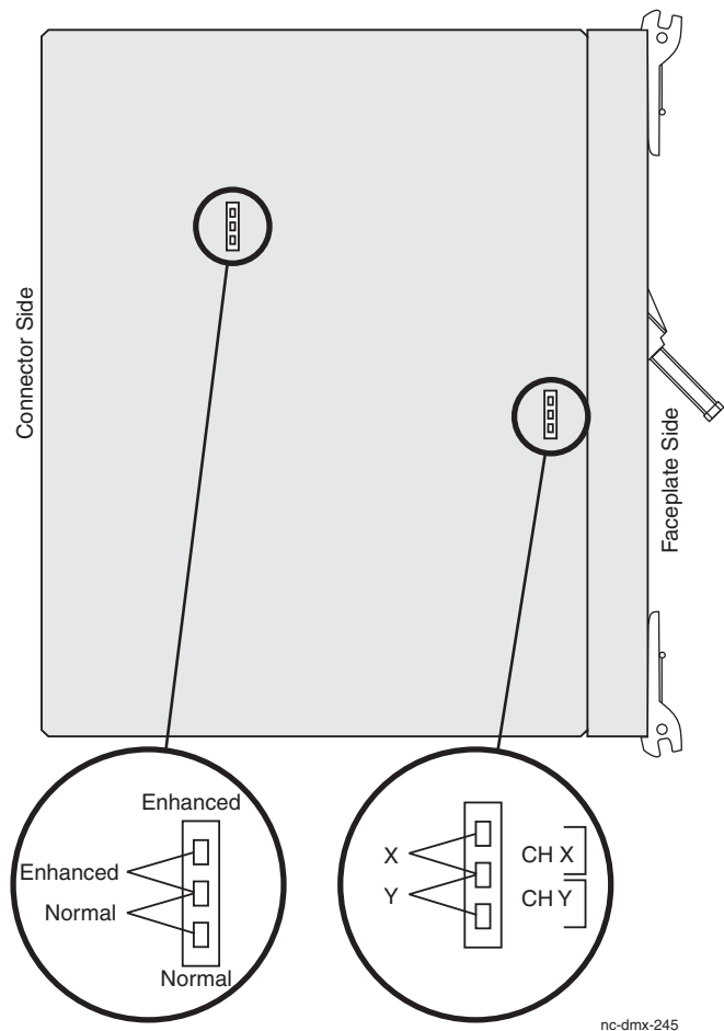
Figure 2-4 LNW121B - 159B channel positions
