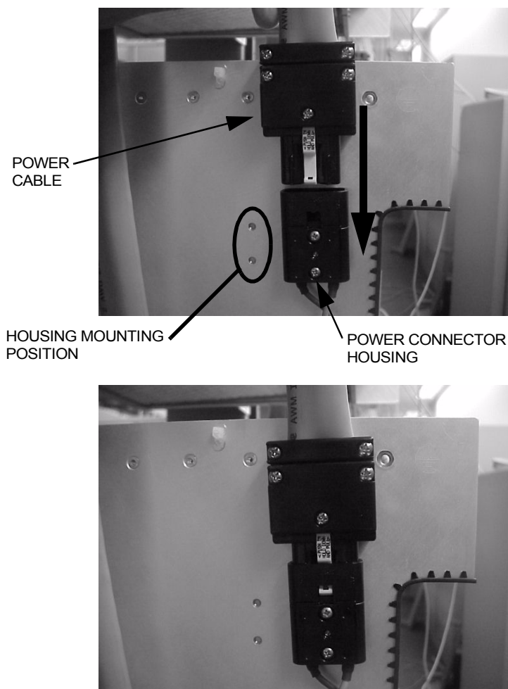
Figure 1-9 Power connection
