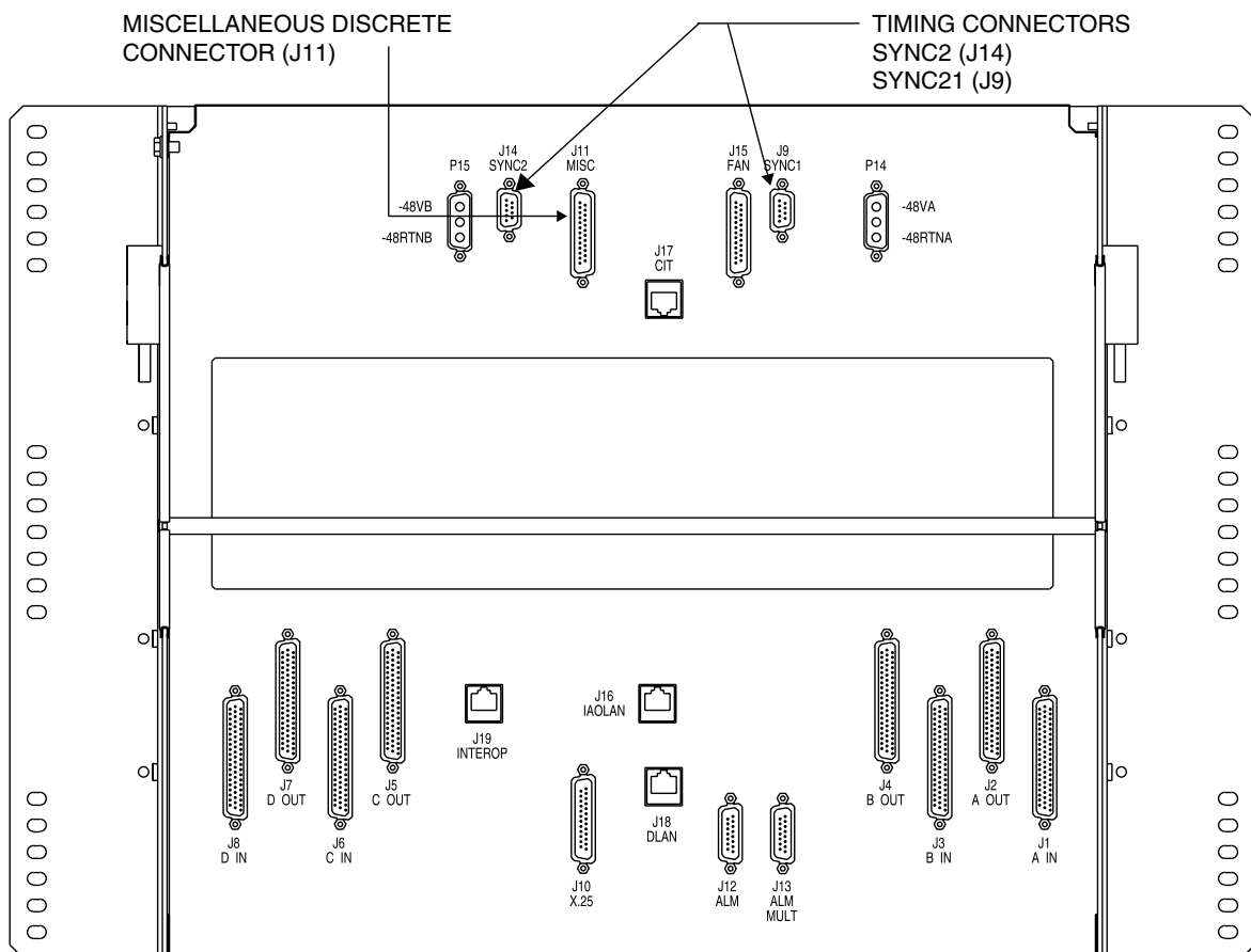
Figure 5-1 Metropolis® DMX Shelf Backplane
