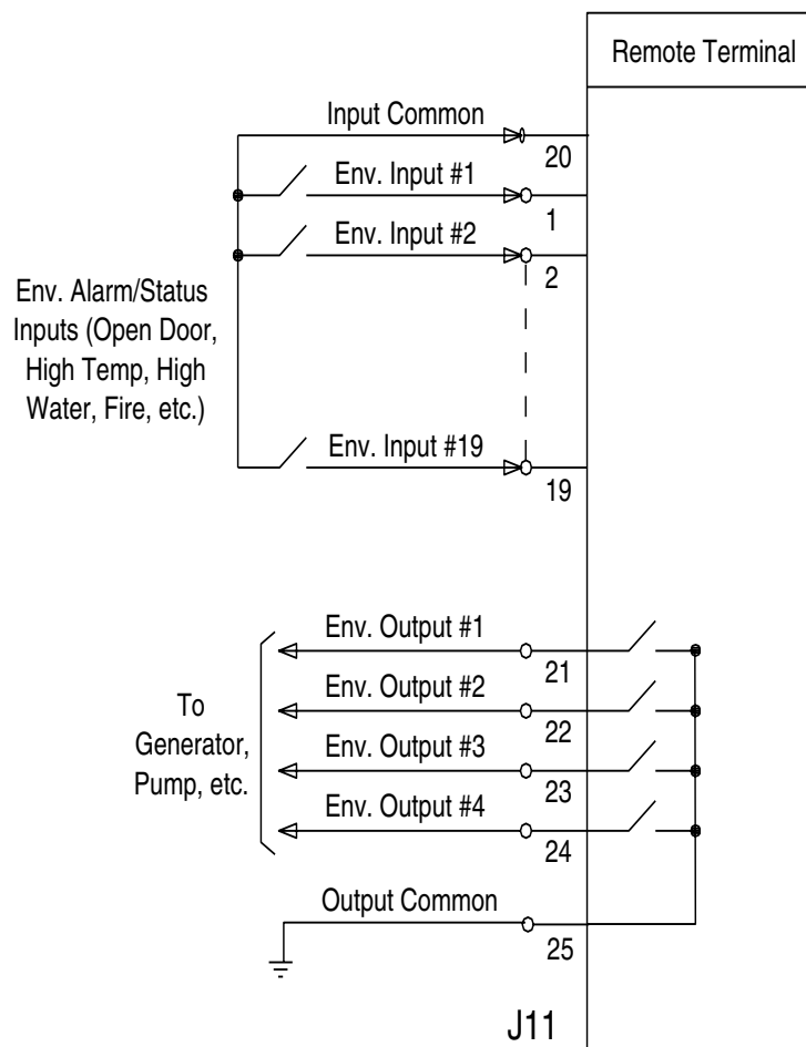
Figure 5-2 Miscellaneous (Environmental) Discrete Functions
