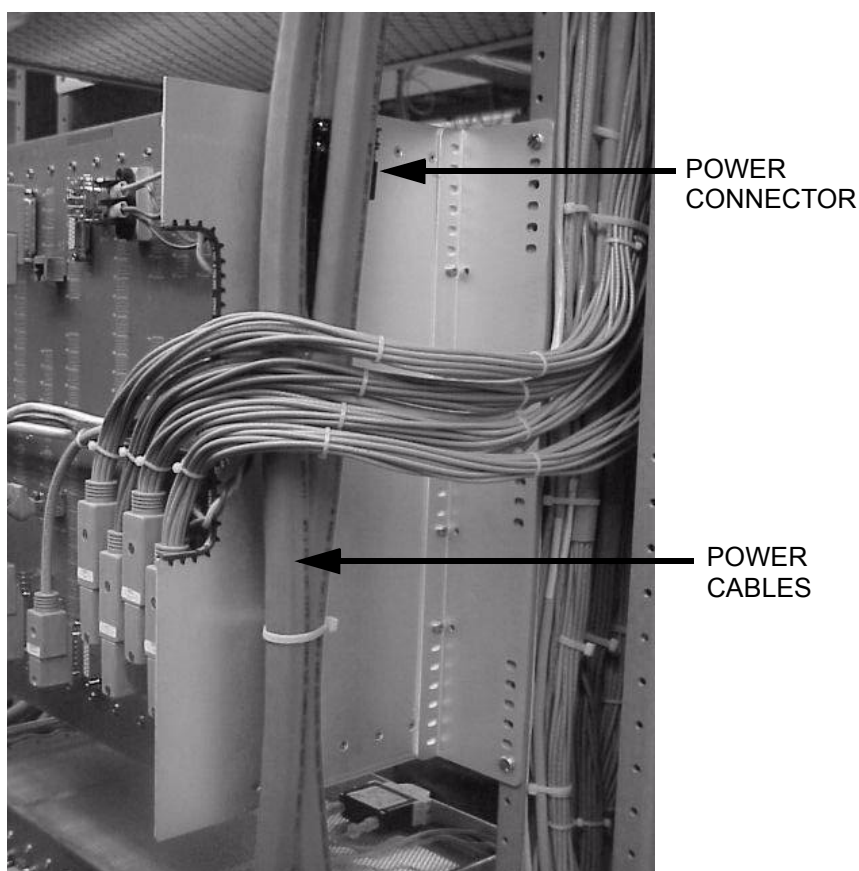
Figure 1-11 Power cable routing without cable bracket
