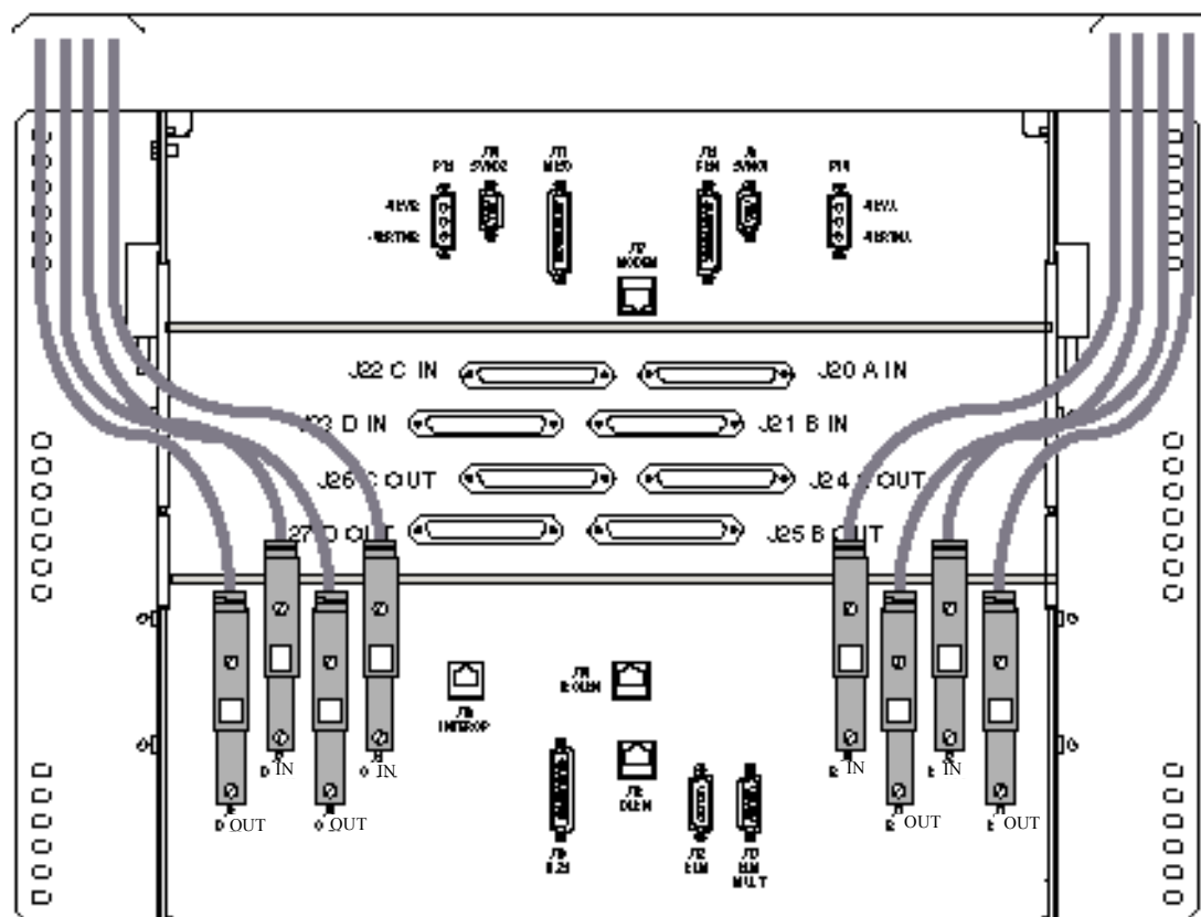
Figure 1-16 12TMUX cable installation
