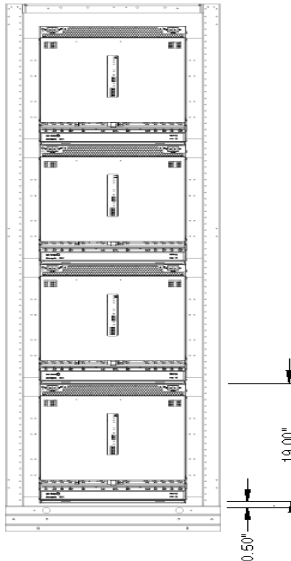
Figure 1-4 Typical Metropolis® DMX High-Capacity shelf bay mounting arrangements
