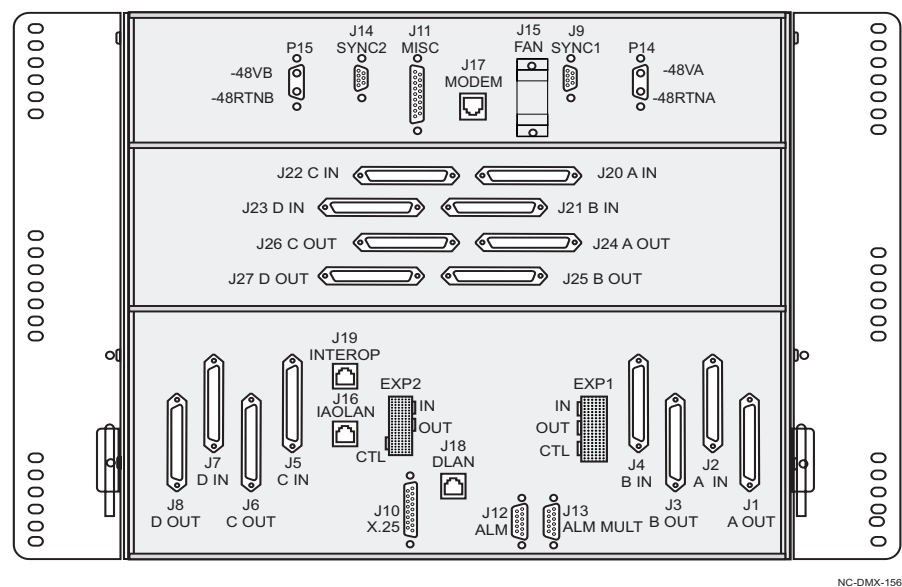
Figure 1-1 High-Capacity Metropolis® DMX shelf backplane
