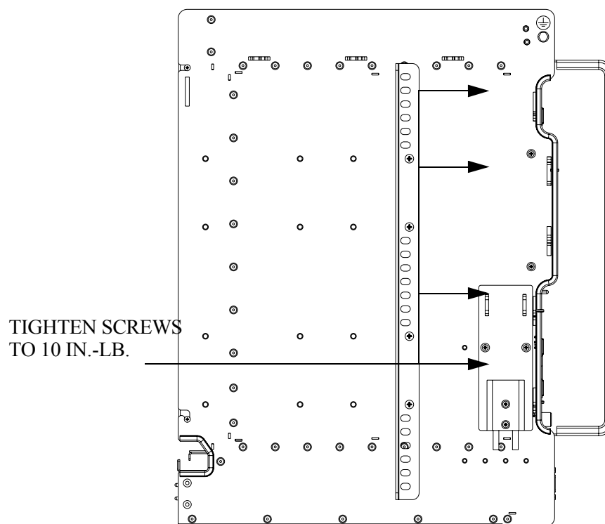
Figure 1-3 Metropolis® DMX High-Capacity shelf mounting bracket positions — 19-inch frame
