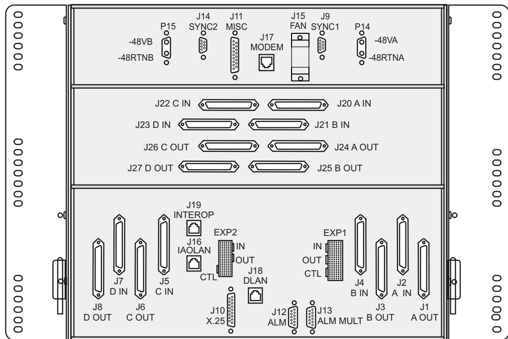
Figure 2-1 Power connections on Metropolis® DMX High-Capacity shelf backplane
