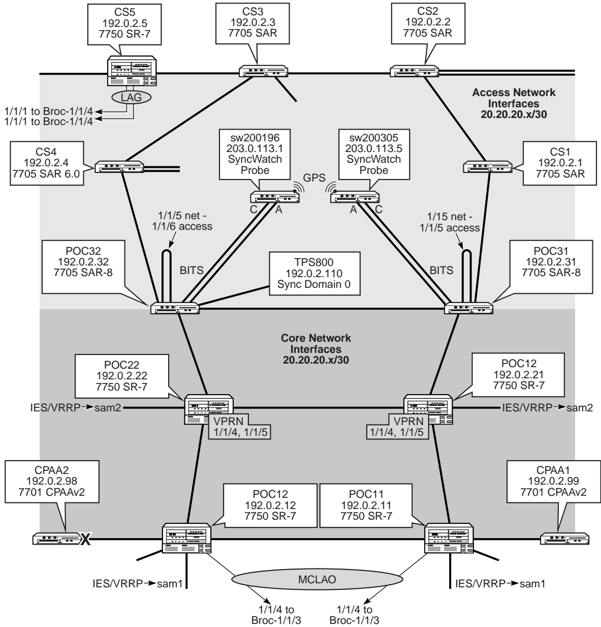
Figure 4-4 Mobile backhaul network with synchronization
