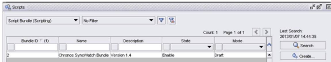
Figure 4-6 Scripts manager
