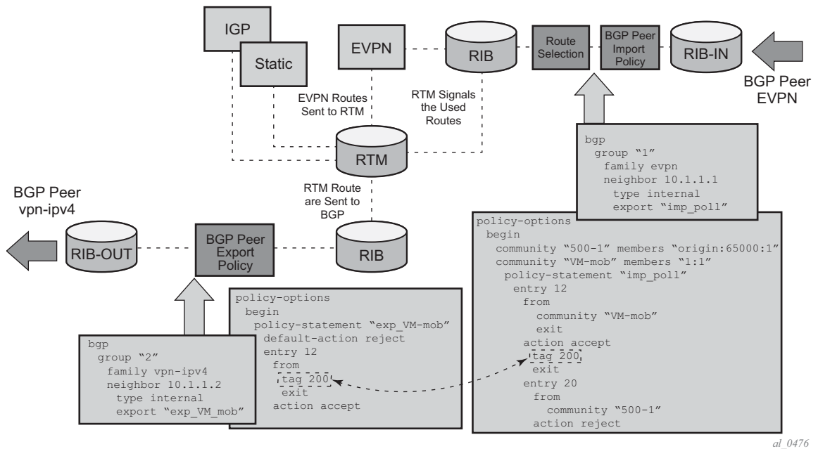
Figure 175: IEVPN Import and I-VPN Export BGP Workflow
