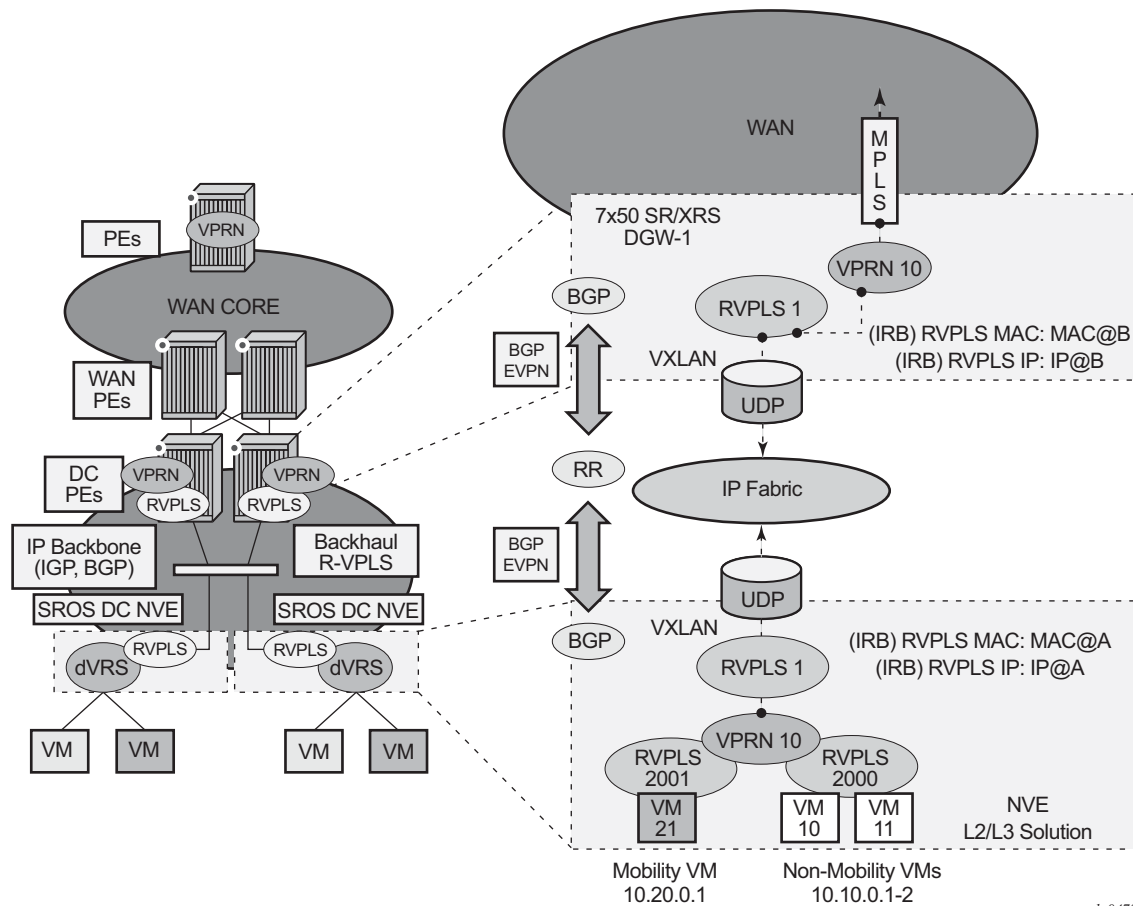
Figure 143: GW IRB on the DC PE for an L3 EVPN/VXLAN DC
