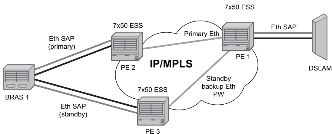
Figure 29: VLL Resilience
