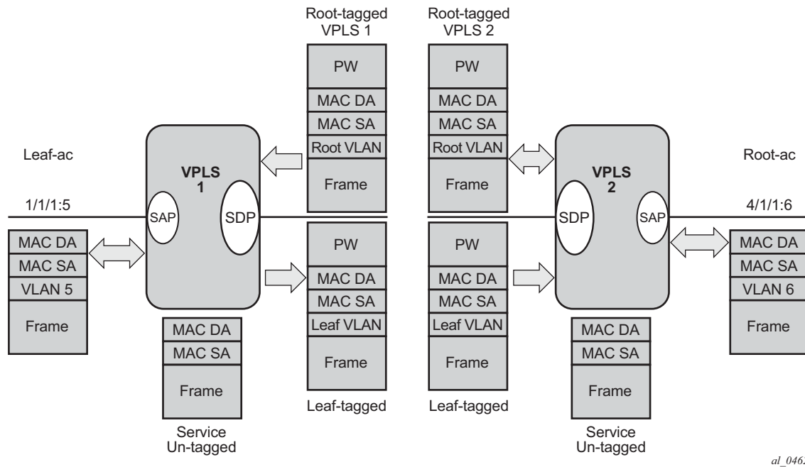
Figure 94: Leaf and Root Tagging PW
