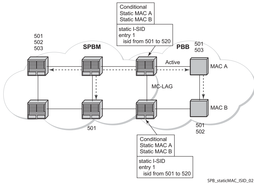
Figure 119: Static ISIDs Example
