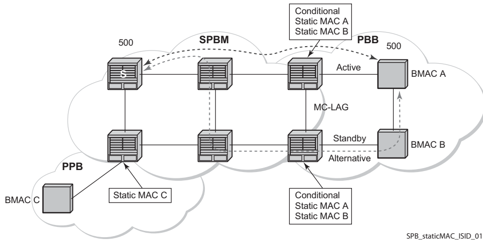
Figure 118: Static MACs Example
