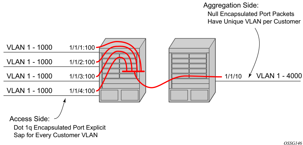
Figure 20: Ingress VLAN Translation
