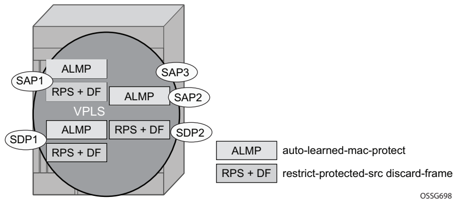
Figure 65: Auto-Learn-Mac-Protect Operation
