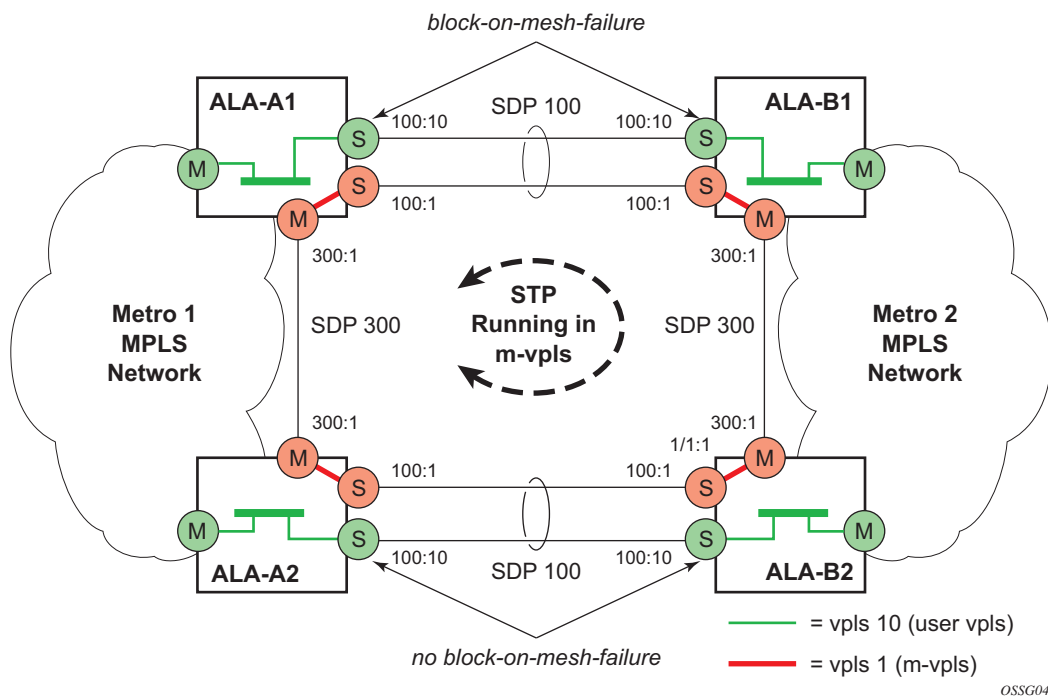
Figure 97: Example Configuration for Protected VPLS Spoke SDP
