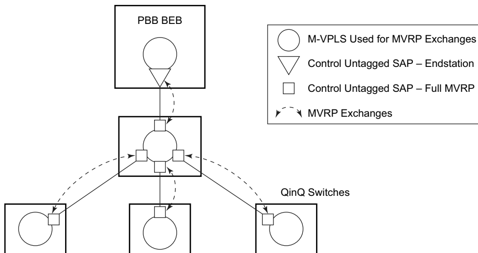
Figure 89: Infrastructure for MVRP Exchanges
