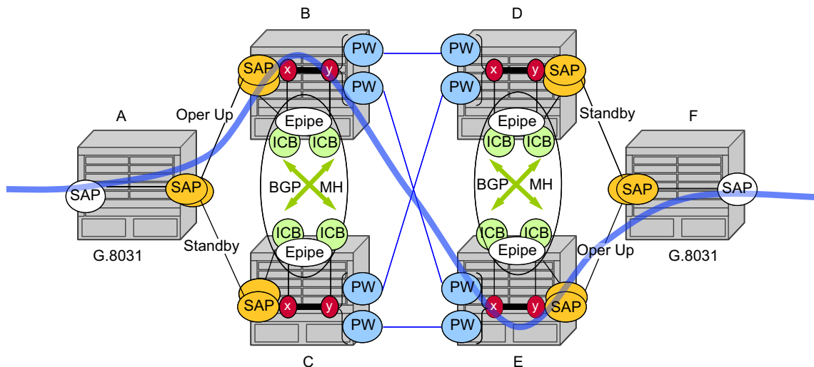
Figure 36: Full Redundancy G.8031 Epipe & BGP-MH
