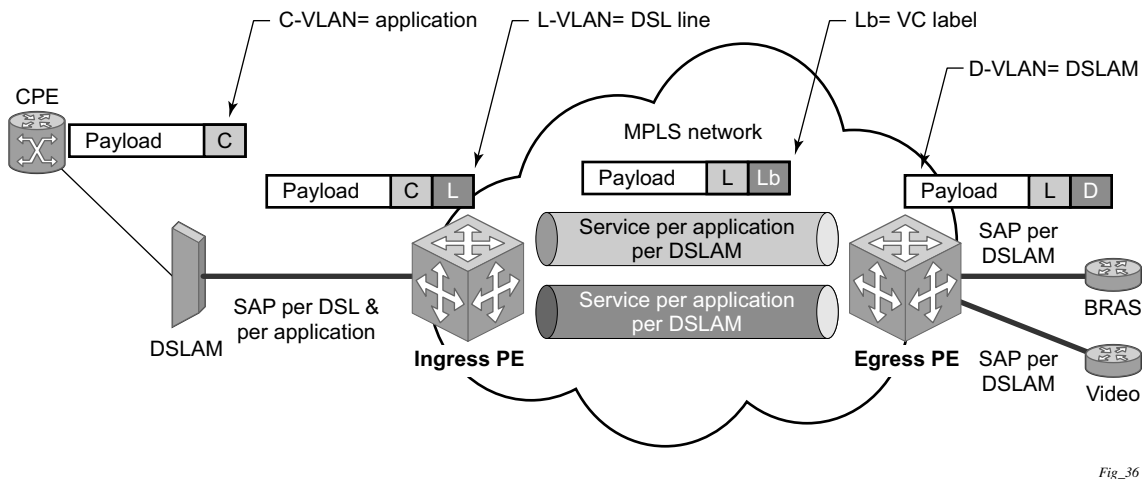
Figure 88: Ingress VLAN Swapping
