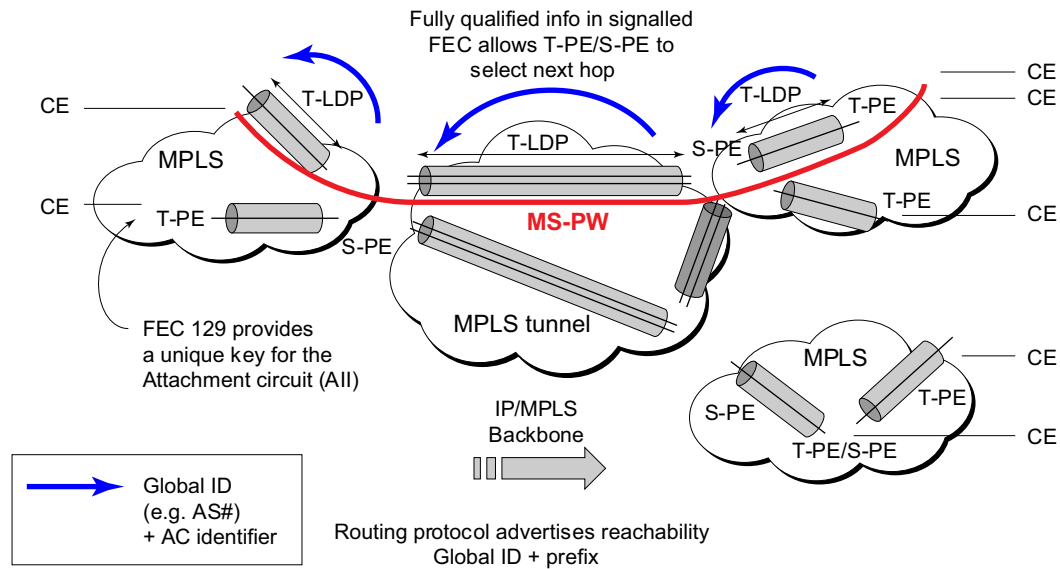
Figure 21: Dynamic MS-PW Overview
