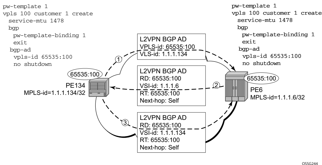
Figure 100: BGP AD Configuration Example
