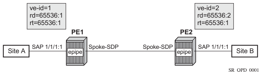
Figure 56: Single-Homed BGP VPWS Configuration Example
