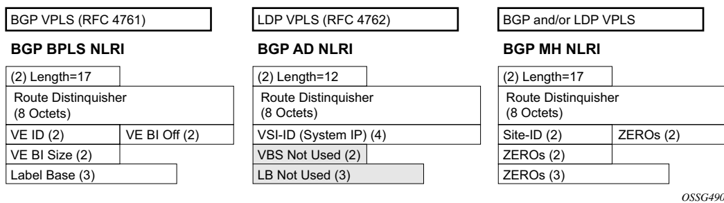
Figure 85: BGP MH-NLRI for VPLS Multi-Homing
