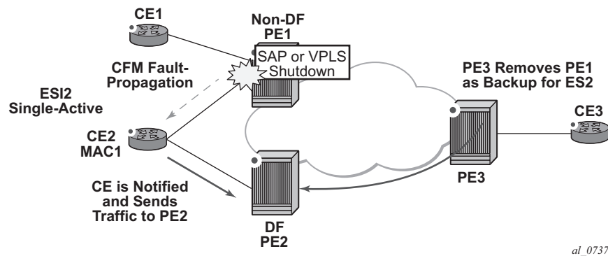
Figure 164: Single-Active Multi-Homing SAP/SDP/Service Shutdown
