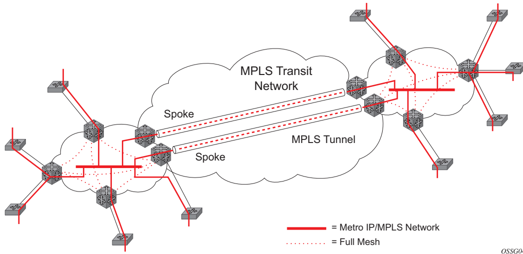
Figure 68: HVPLS with Spoke Redundancy
