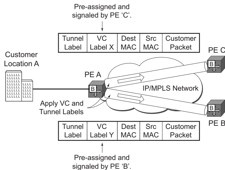
Figure 62: Access Port Egress Packet Format and Lookup
