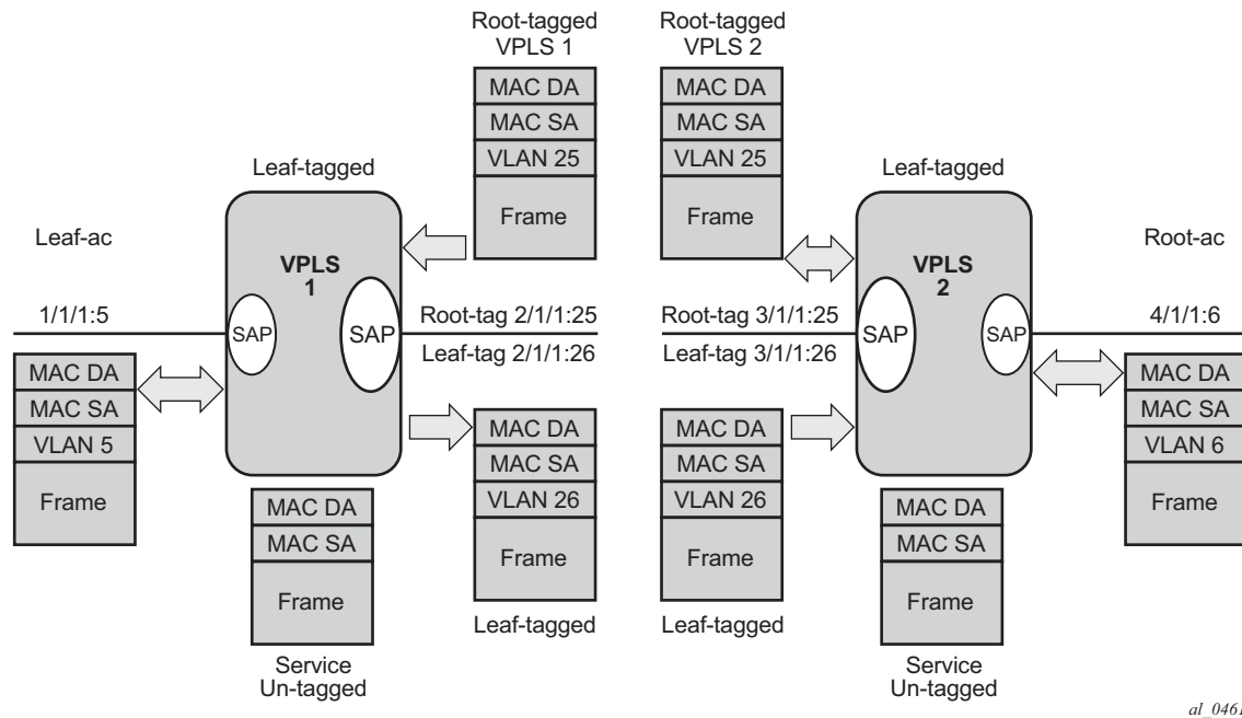
Figure 93: Leaf and Root Tagging Dot1q
