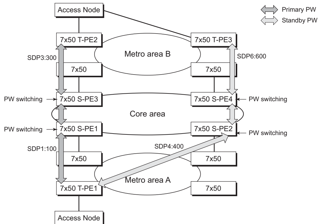
Figure 53: VLL Resilience with Pseudowire Redundancy and Switching
