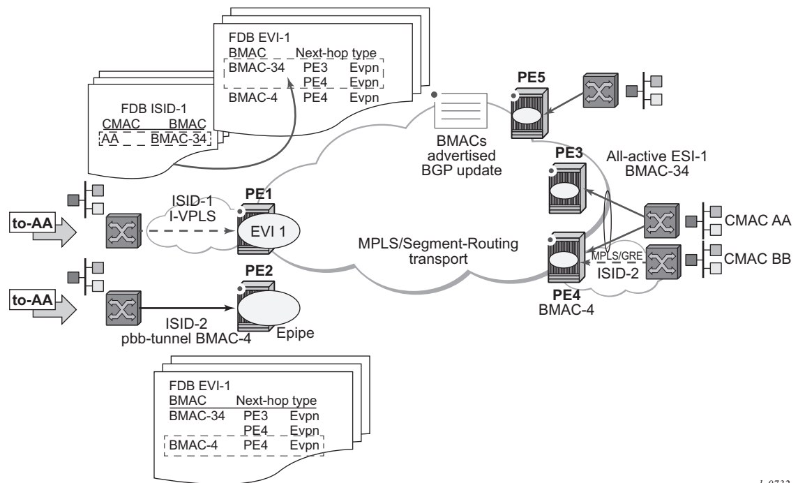
Figure 165: PBB-EVPN for I-VPLS and PFF Epipe Services
