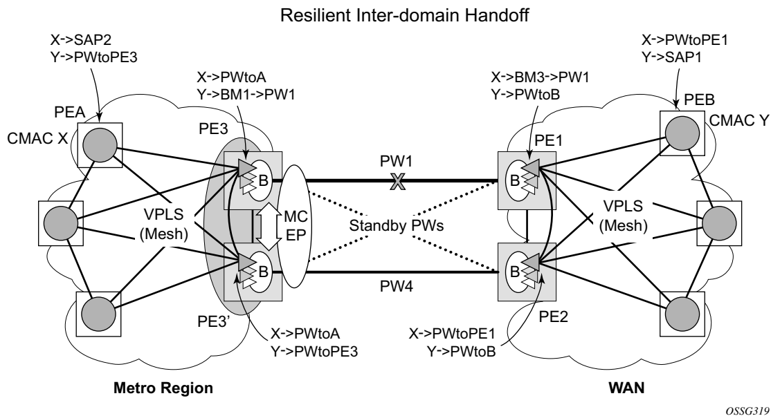
Figure 74: MC-EP with B-VPLS Failure Scenario
