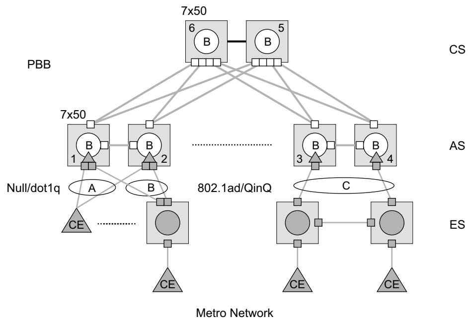
Figure 67: Access Resiliency
