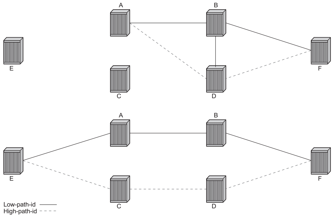
Figure 116: Unicast Paths for Low-path-id and High-path-id
