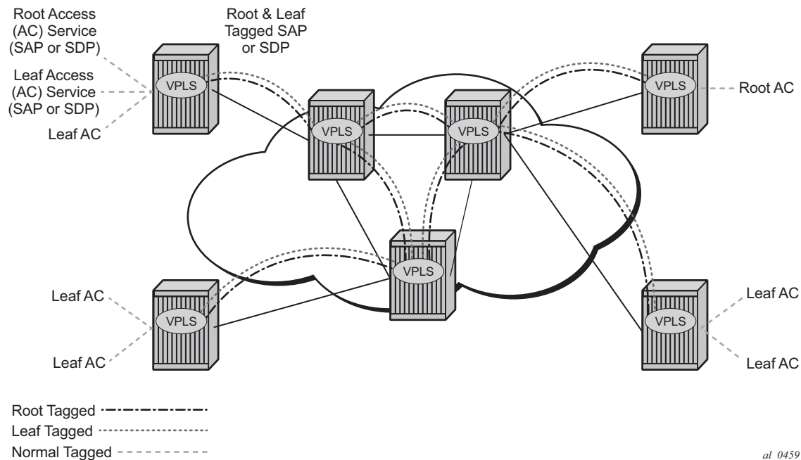
Figure 91: E-Tree Service
