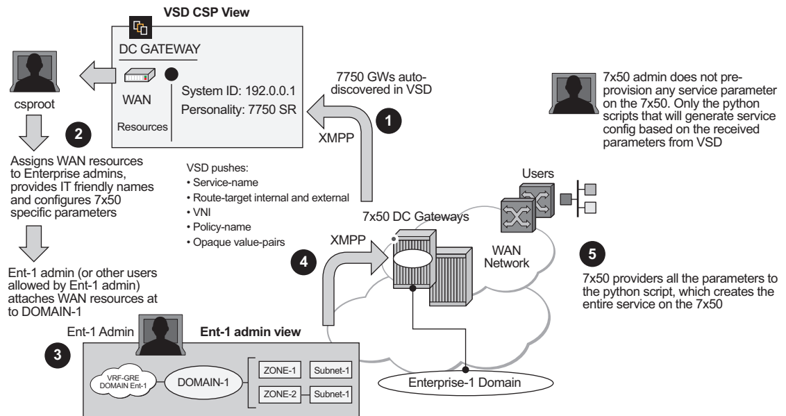
Figure 152: Fully-Dynamic VSD Integration Model Workflow
