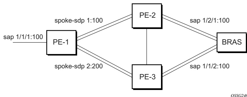
Figure 55: VLL Resilience with Pseudowire Switching
