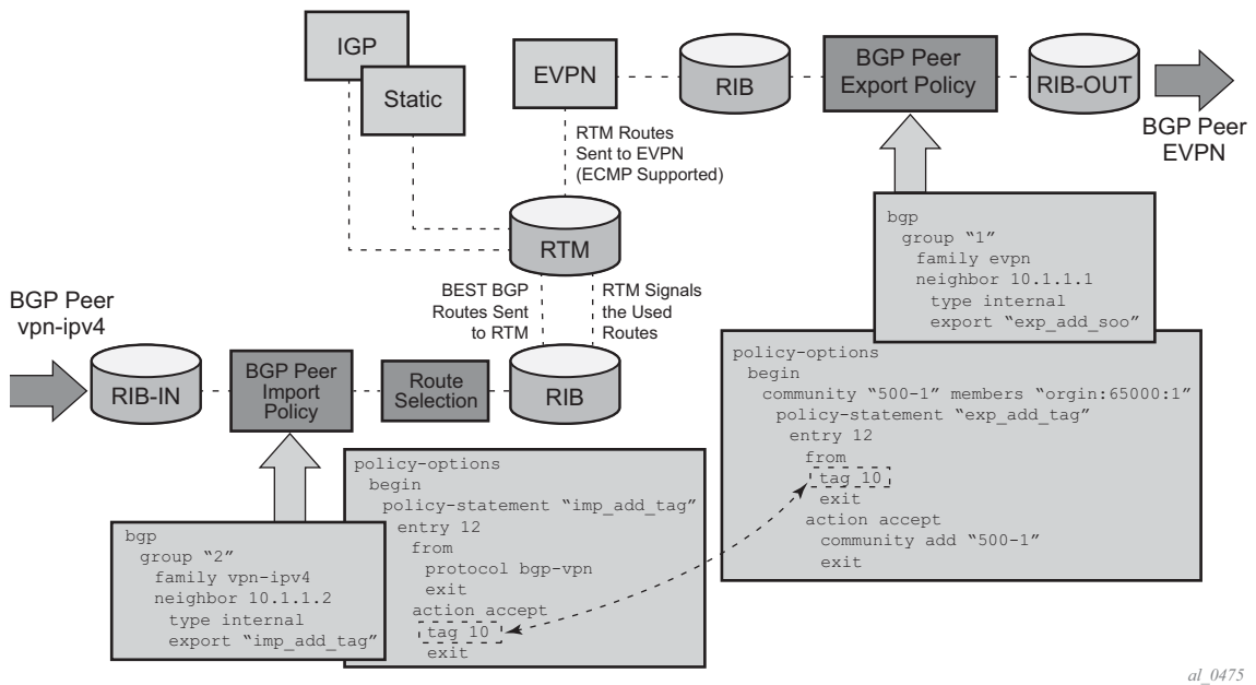
Figure 174: IP-VPN Import and EVPN Export BGP Workflow
