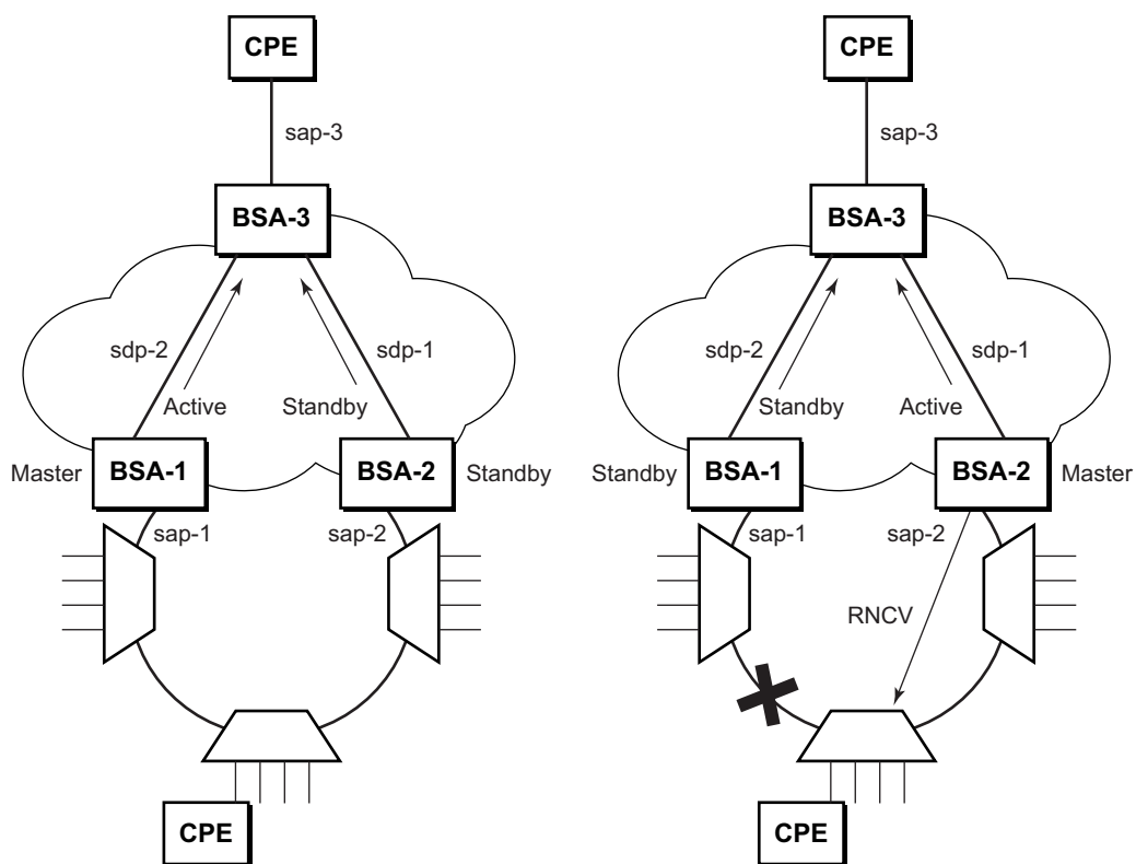
Figure 11: MC-Ring in a Combination with VLL Service
