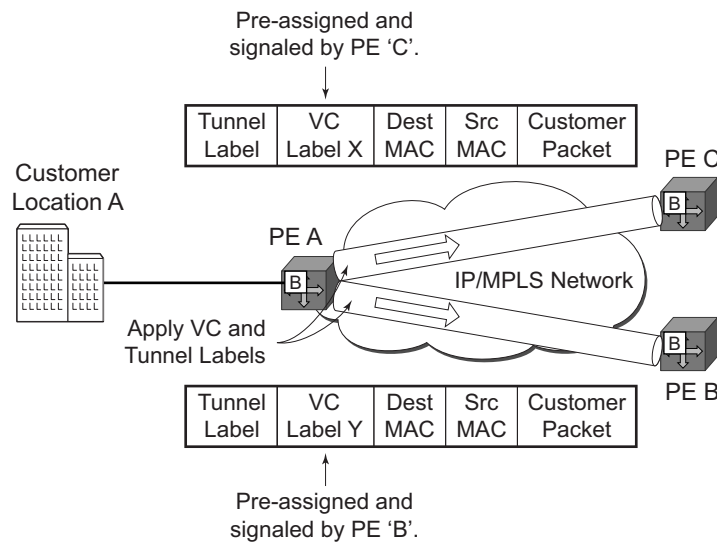
Figure 61: Network Port Egress Packet Format and Flooding
