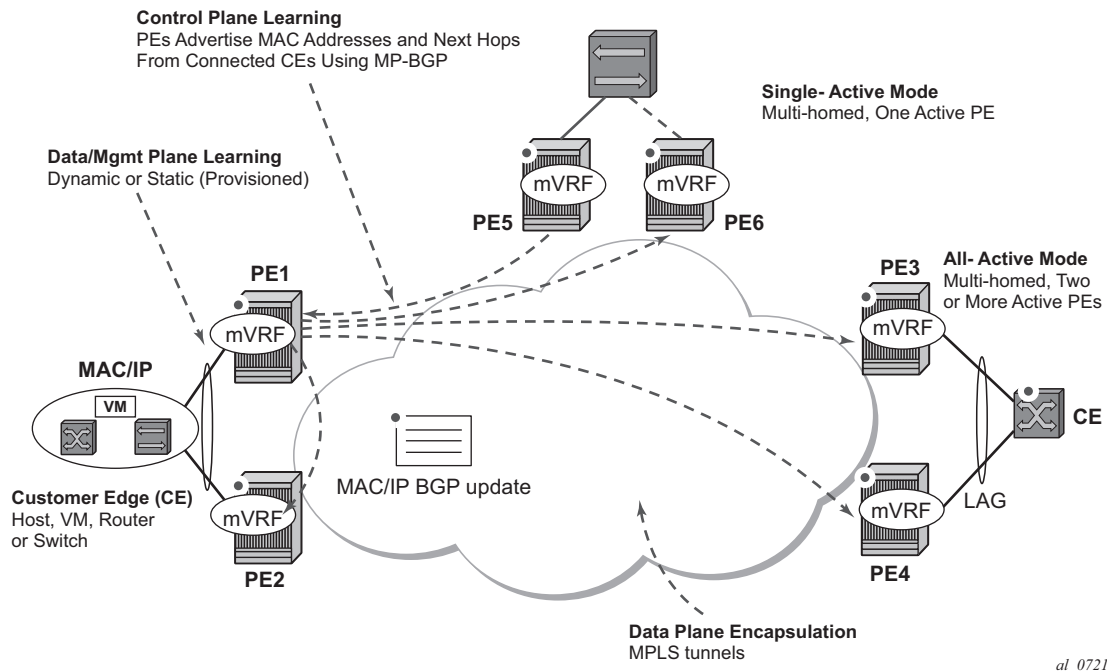
Figure 145: EVPN for MPLS in VPLS Services
