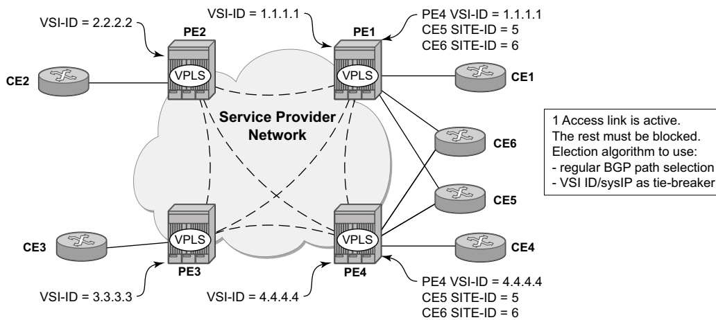
Figure 84: BGP Multi-Homing for VPLS
