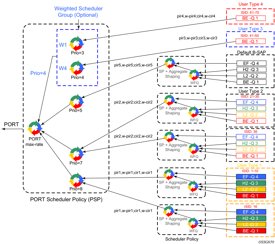
Figure 139: Egress Queue Scheduling
