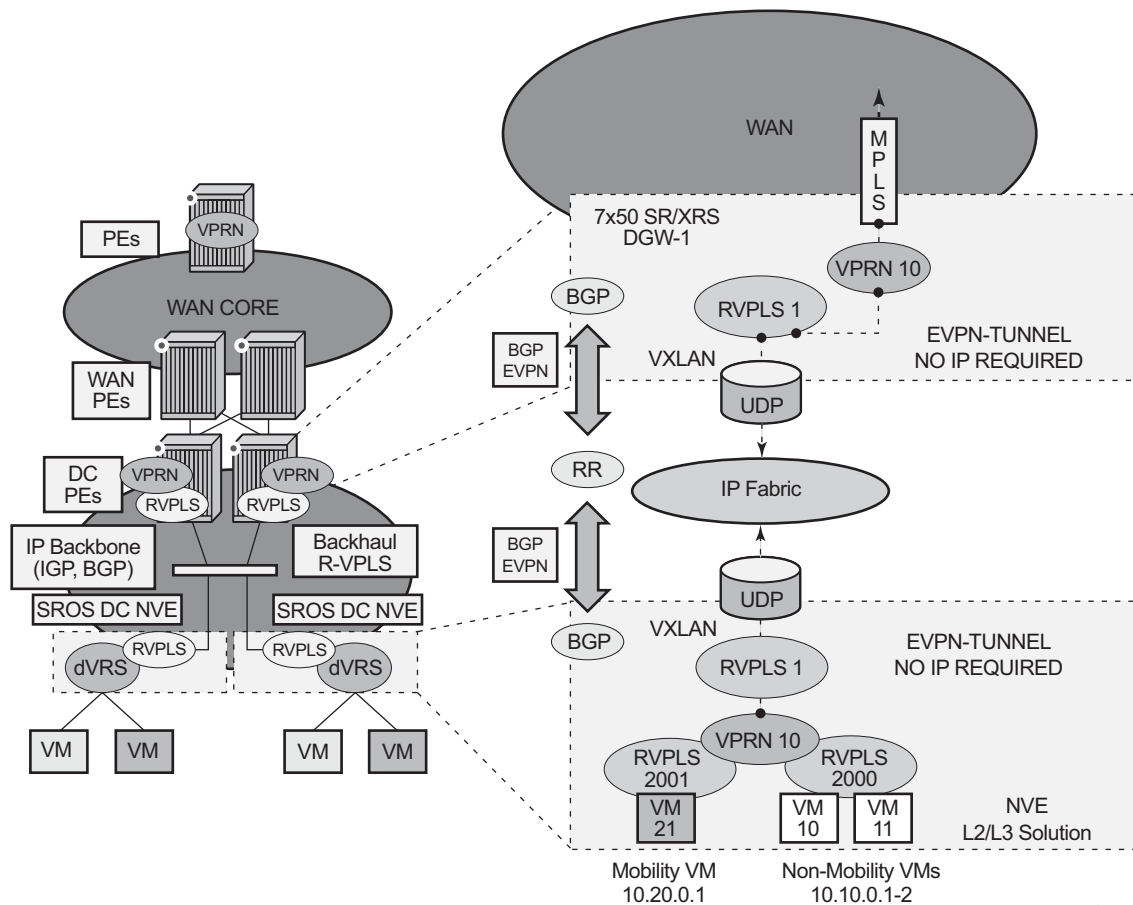
Figure 144: EVPN-Tunnel GW IRB on the DC PE for an L3 EVPN/VXLAN DC
