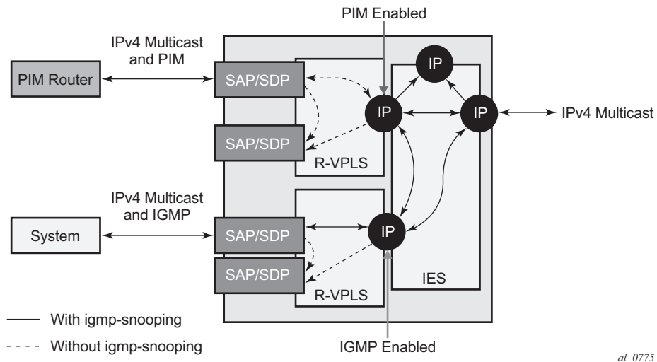
Figure 87: IPv4 Multicast with a Router VPLS service
