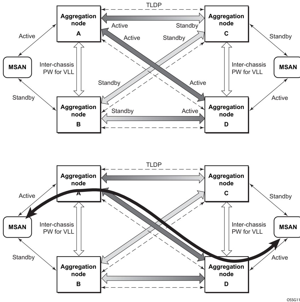
Figure 38: Access Node Resilience
