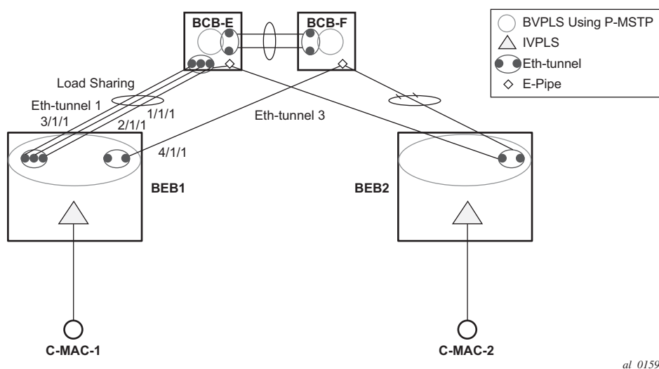
Figure 129: Ethernet Tunnel Overlay
