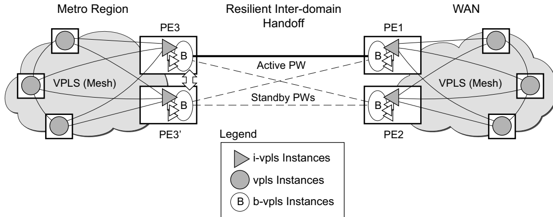
Figure 73: MC-EP with B-VPLS
