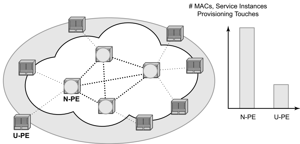
Figure 109: Large HVPLS Deployment
