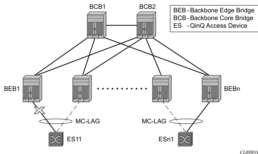
Figure 135: Access Dual-Homing for PBB ELINE - BEB Failure
