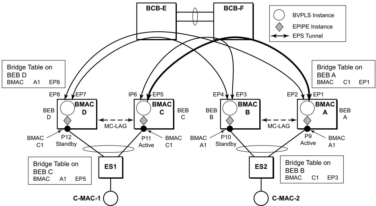
Figure 134: Access Multi-Homing Solution for PBB Epipe
