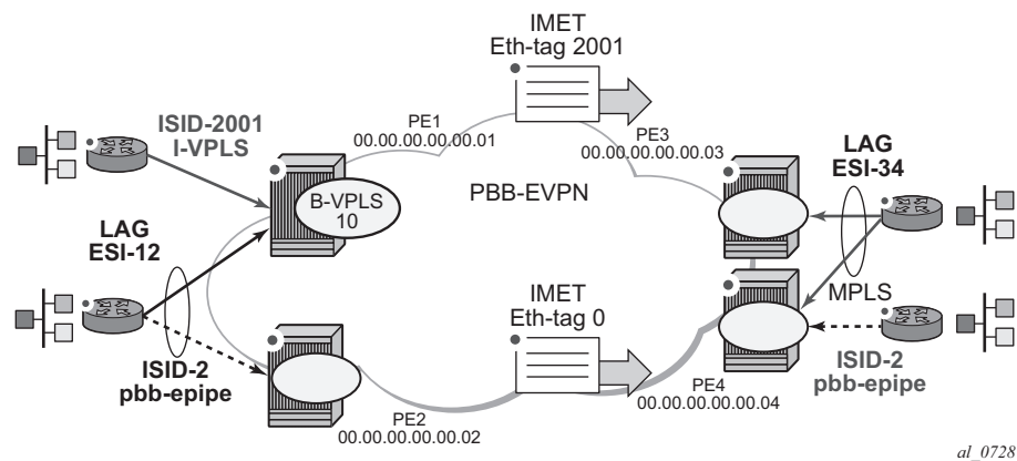
Figure 166: PBB-EVPN and I-VPLS Flooding Containment
