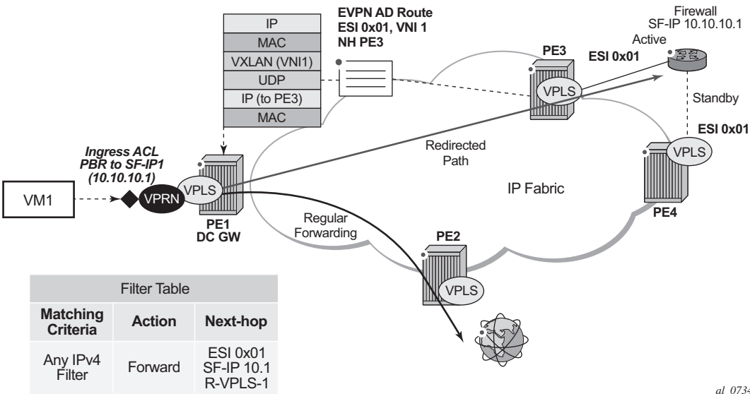
Figure 173: PBR to ESI Function
