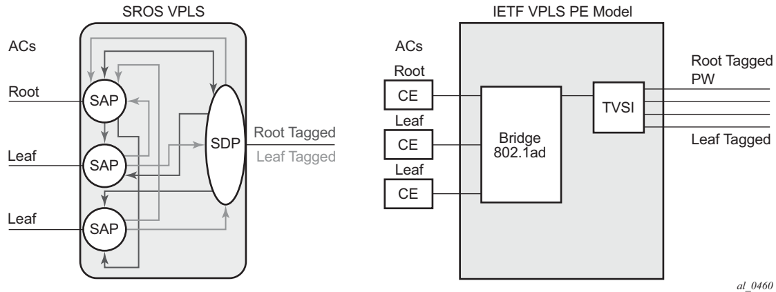
Figure 92: Mapping PE Model to 7x50 VPLS Service
