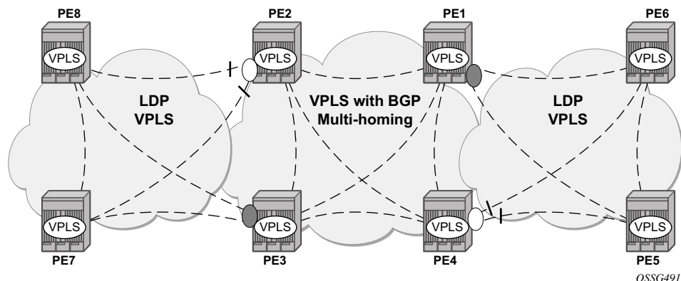
Figure 86: BGP MH Used in an HVPLS Topology
