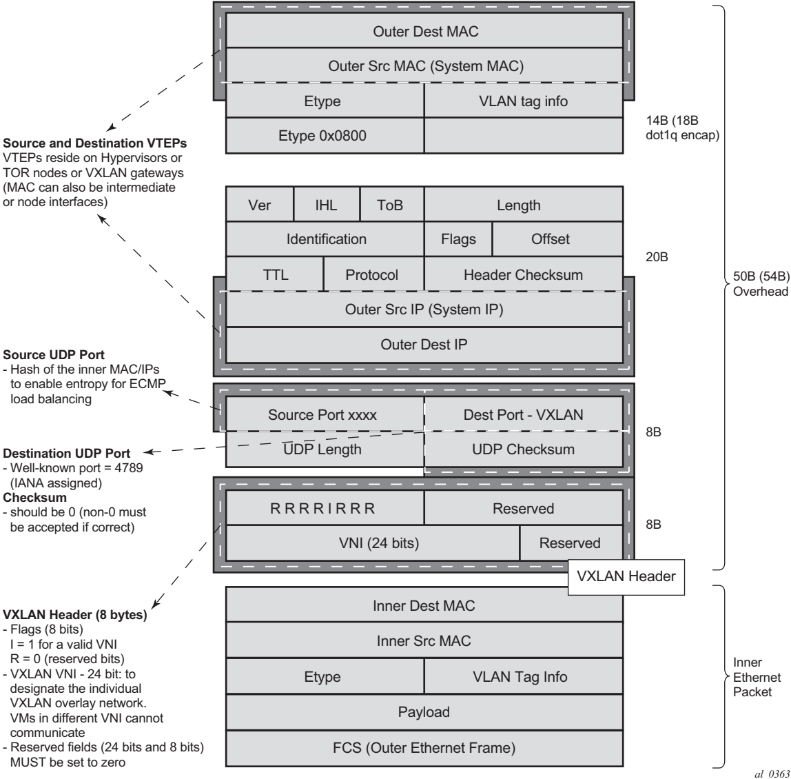
Figure 147: VXLAN Frame Format
