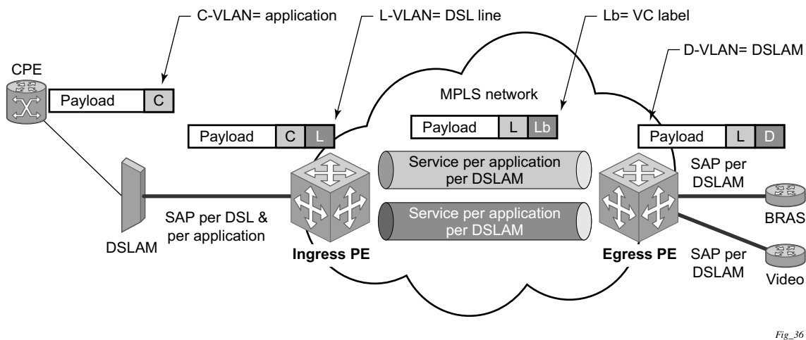
Figure 19: Ingress VLAN Swapping
