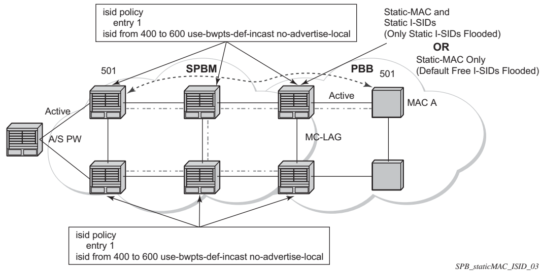
Figure 120: ISID Policy Example
