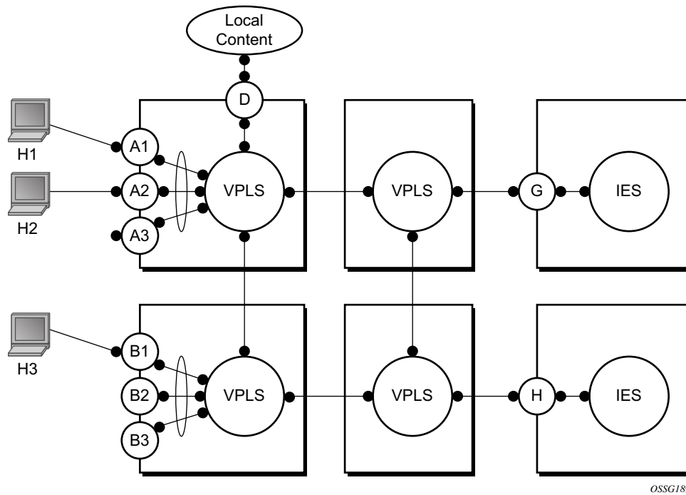
Figure 63: MAC Learning Protection
