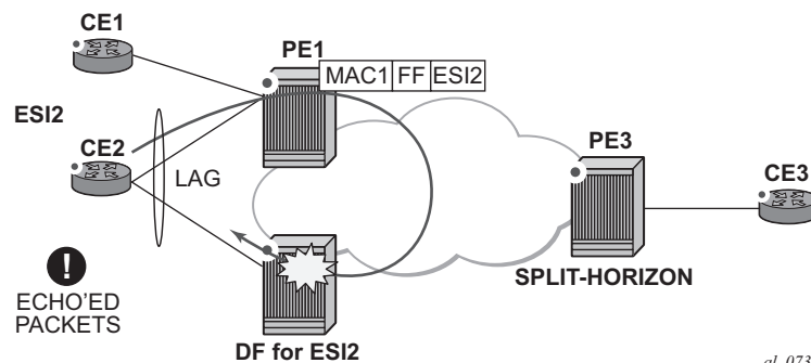
Figure 156: Split-Horizon
