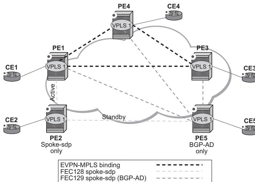
Figure 154: EVPN-VPLS Integration
