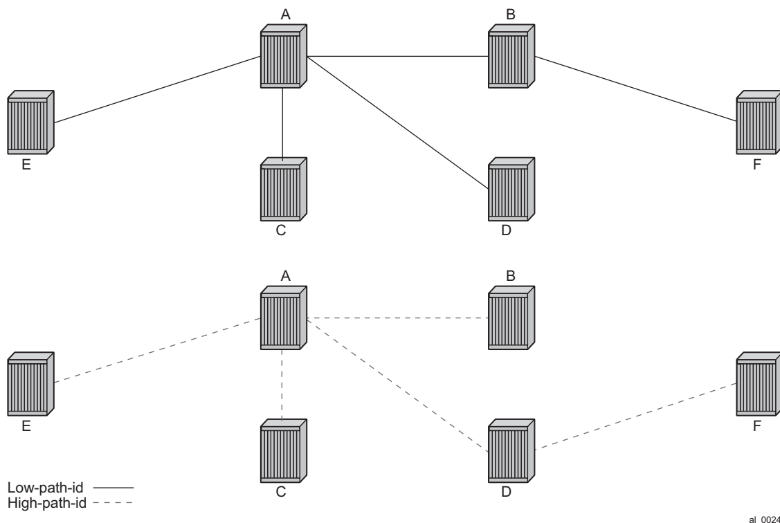
Figure 117: Multicast Paths for Low-path-id and High-path-id
