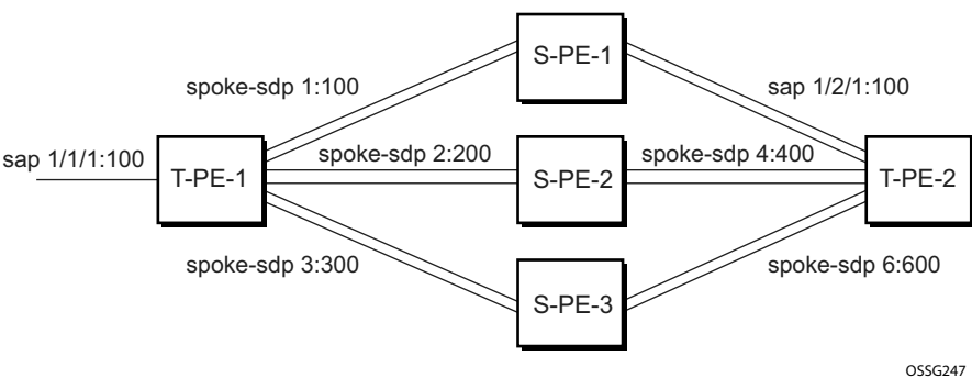
Figure 102: BGP AD Triggering LDP Functions
