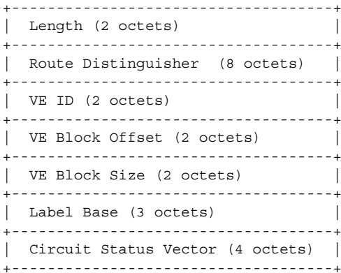
Figure 48: BGP VPWS NLRI
