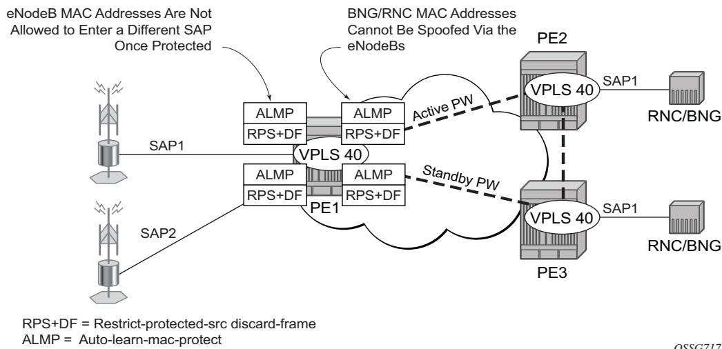
Figure 66: Auto-Learn-Mac-Protect Example
