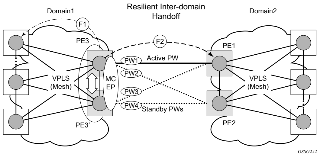
Figure 72: MAC Flush in the MC-EP Solution
