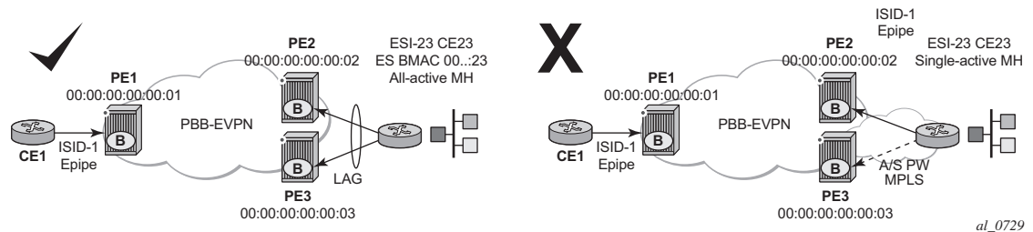
Figure 169: PBB-EVPN MH in a Three-Node Scenario
