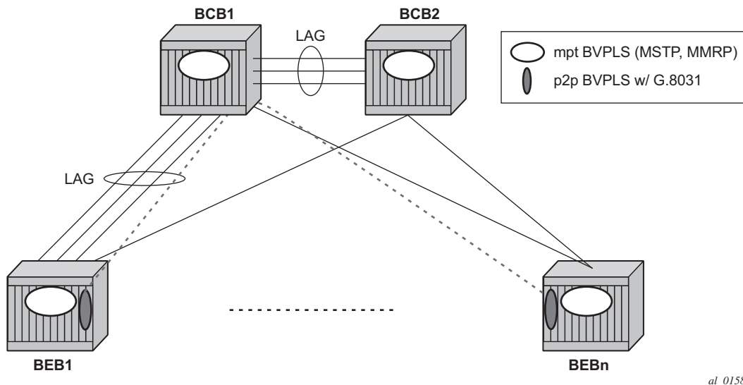
Figure 128: G.8031 P2P Tunnels and LAG-Like Loadsharing Co-Existence
