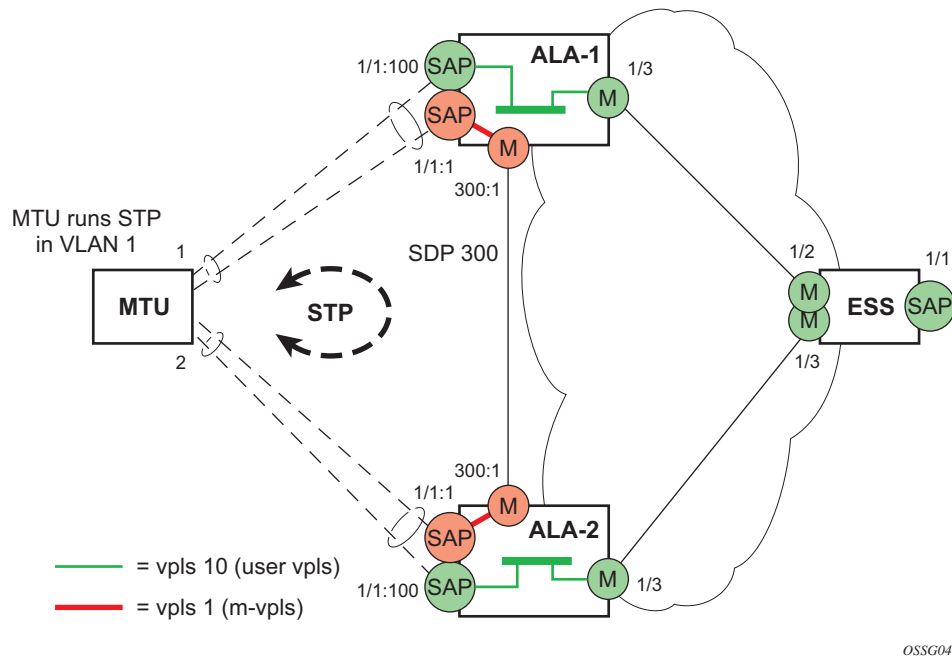
Figure 96: Example Configuration for Protected VPLS SAP
