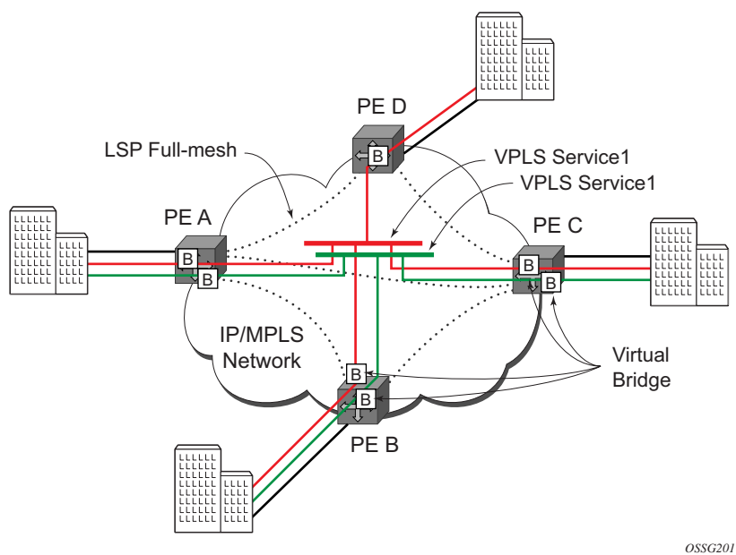
Figure 59: VPLS Service Architecture
