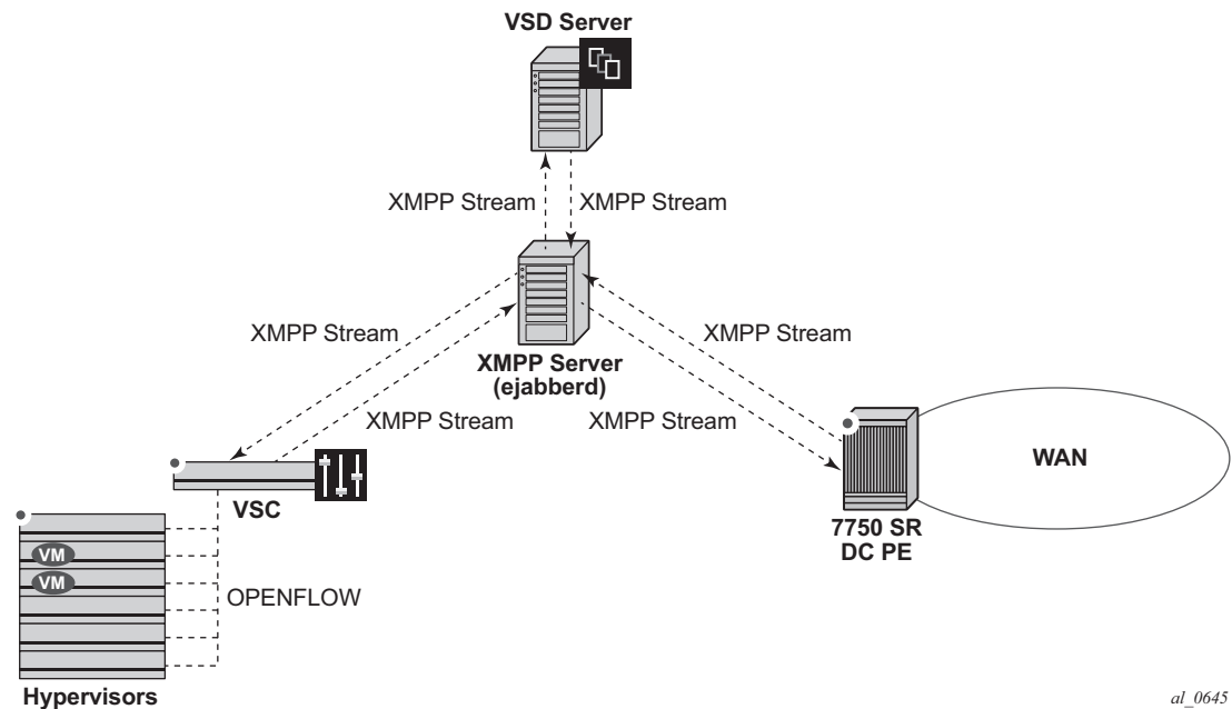
Figure 150: Basic XMPP Architecture
