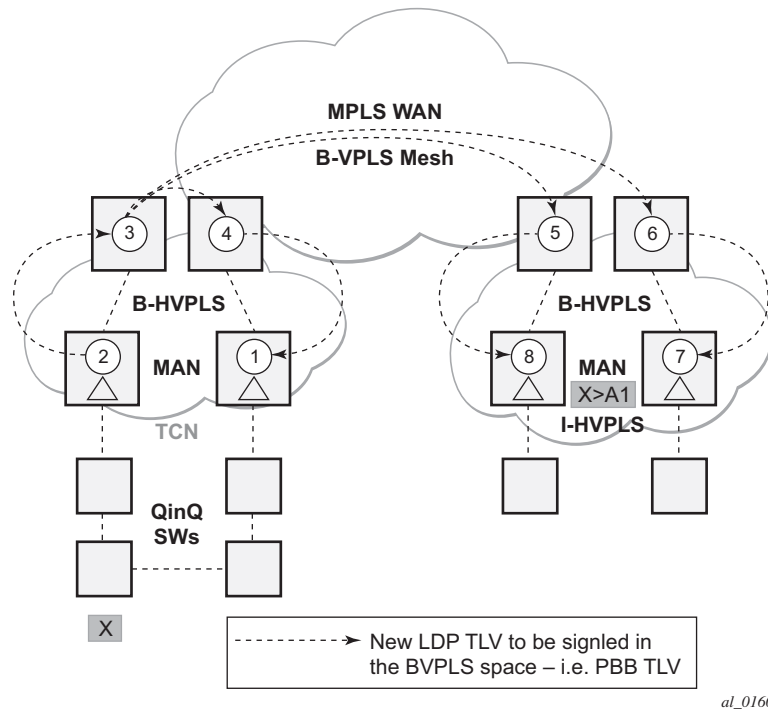
Figure 130: TCN Triggered PBB Flush-ALI-But-Mine Procedure
