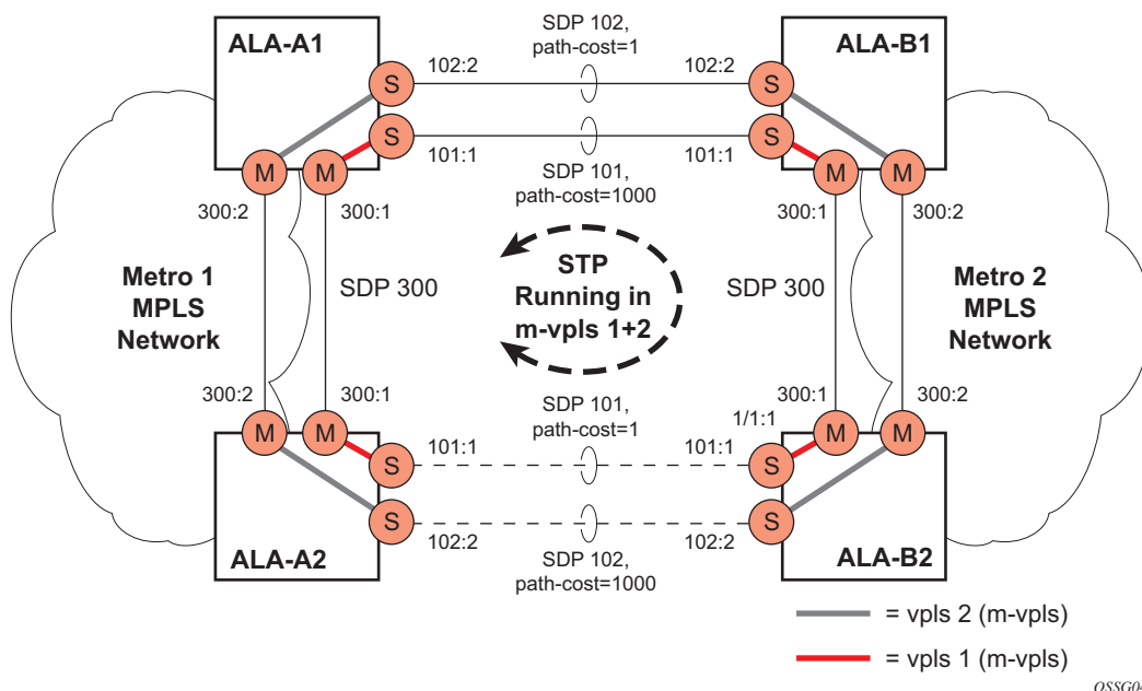
Figure 98: Example Configuration for Load Balancing Across Two Protected VPLS Spoke SDPs
