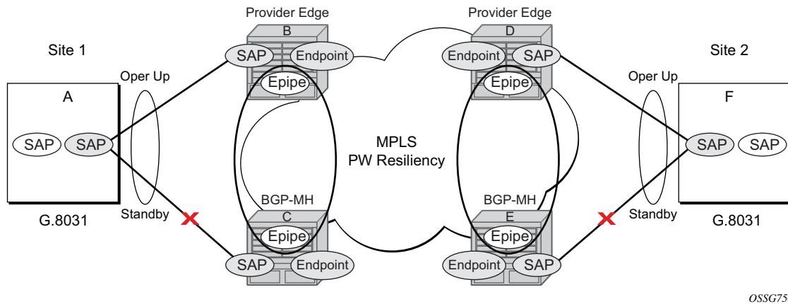
Figure 34: BGP-MH Site Support for Ethernet Tunnels
