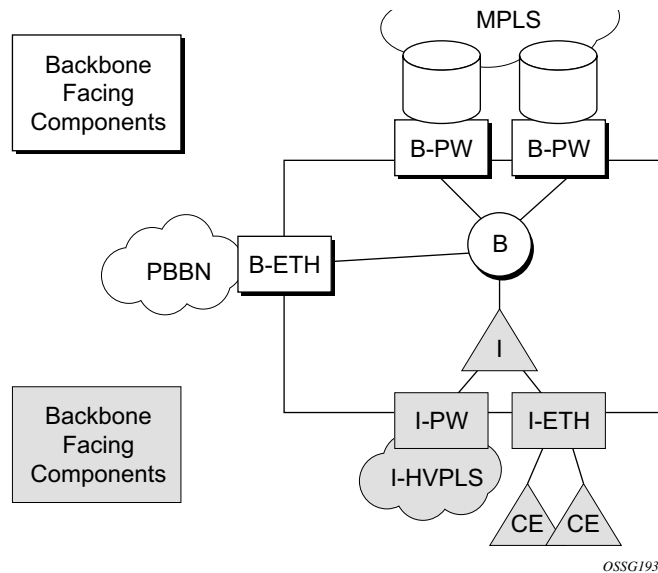
Figure 111: QinQ Payload in Provider Header Example
