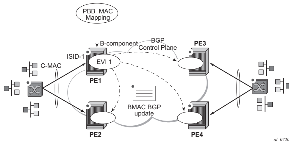
Figure 146: EVPN for PBB over MPLS
