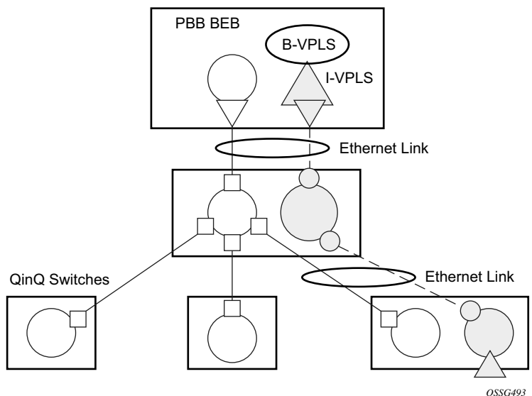
Figure 90: Service Instantiation with MVRP - QinQ to PBB Example
