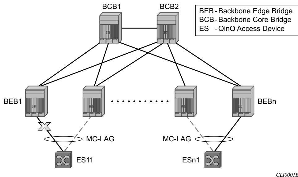
Figure 131: Access Dual-Homing into PBB BEBs - Topology View
