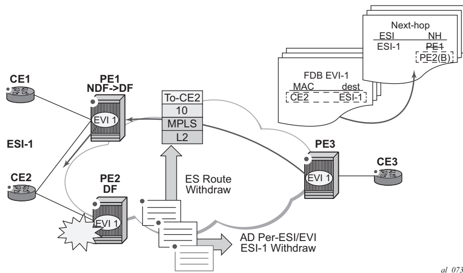
Figure 163: Single-Active Multi-Homing ES Failure
