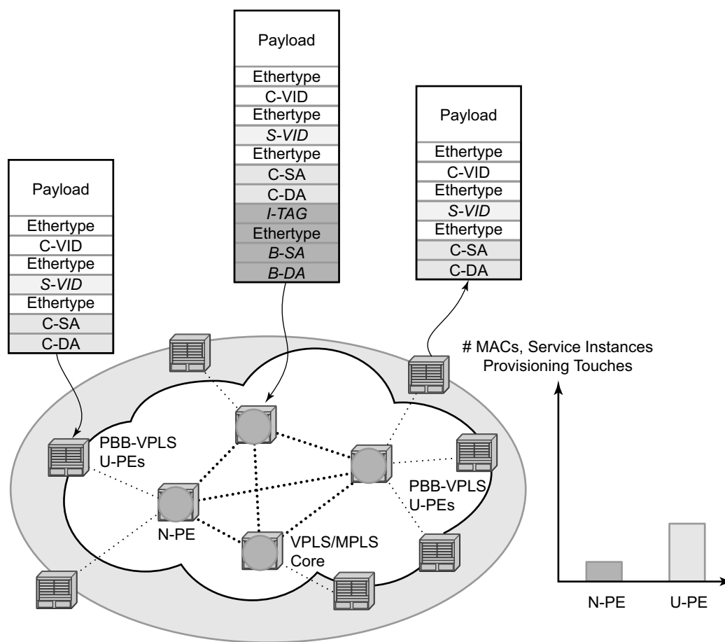
Figure 110: Large PBB-VPLS Deployment
