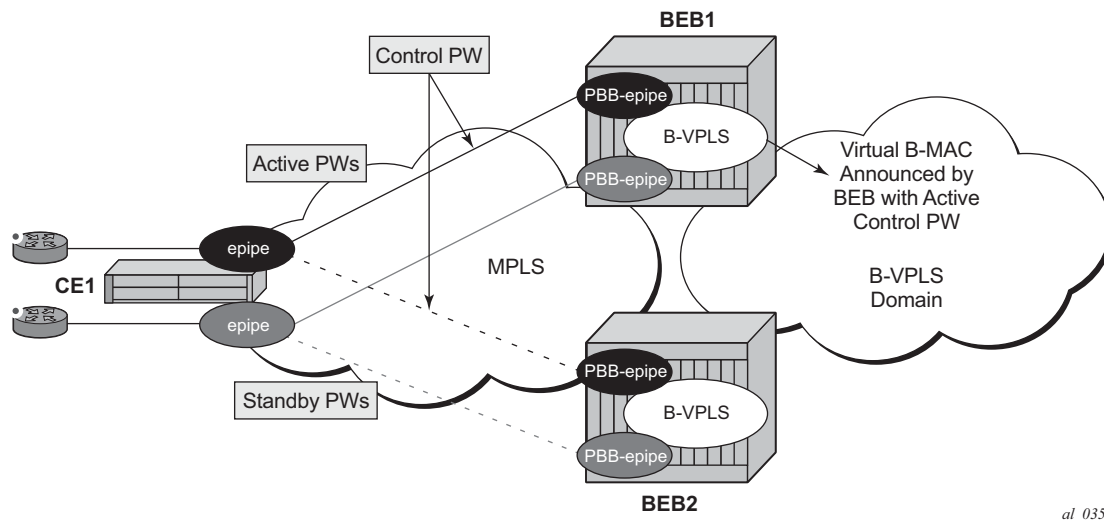
Figure 137: Active/Standby PW into PBB Epipes
