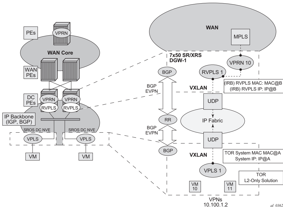
Figure 141: Layer-2 DC PE with VPLS to the WAN
