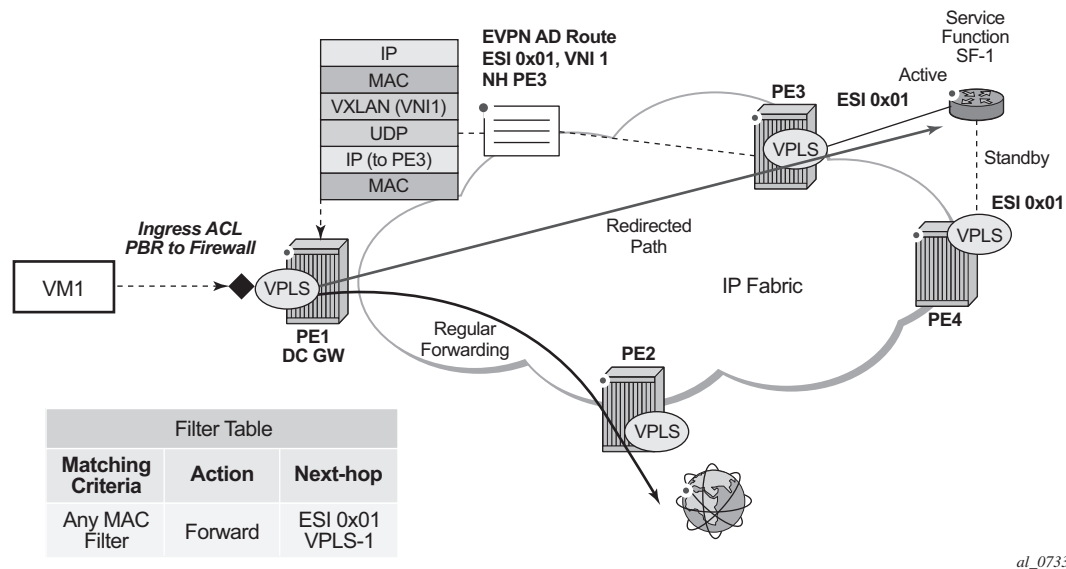
Figure 172: PBF to ESI Function
