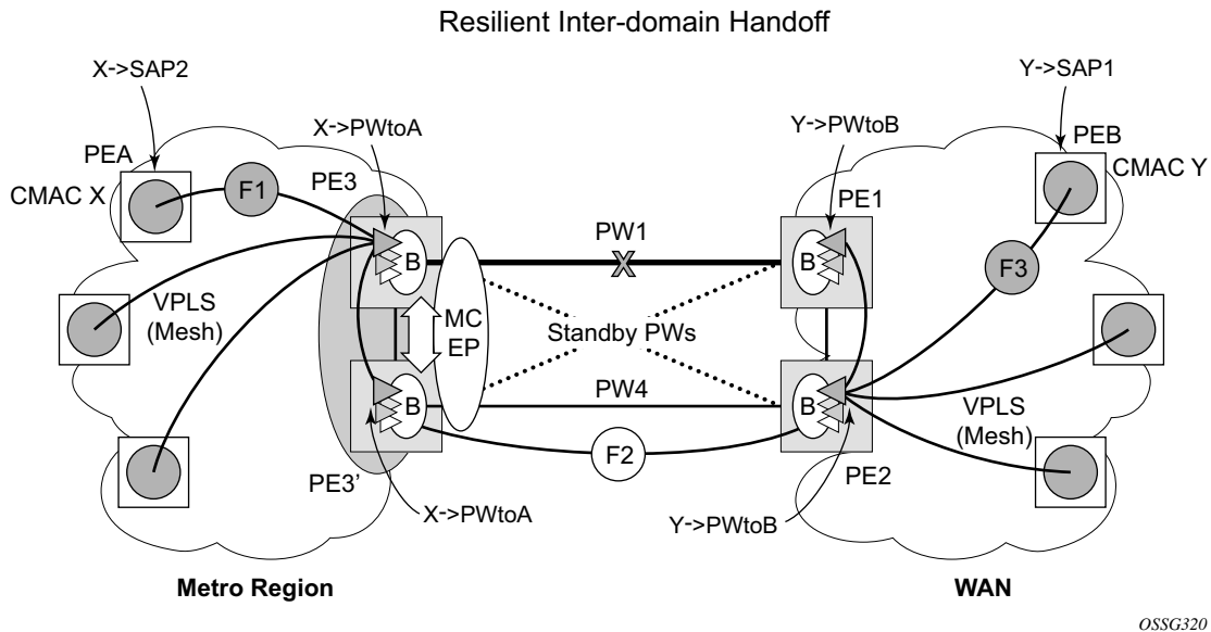
Figure 75: MC-EP with B-VPLS Mac Flush Solution
