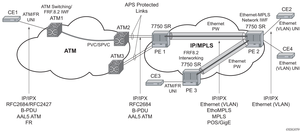
Figure 10: Application of Ethernet Interworking VLL Example
