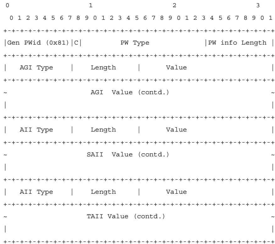
Figure 81: Generalized Pseudowire-ID FEC Element
