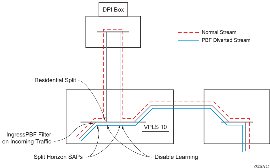
Figure 108: Policy-Based Forwarding For Deep Packet Inspection
