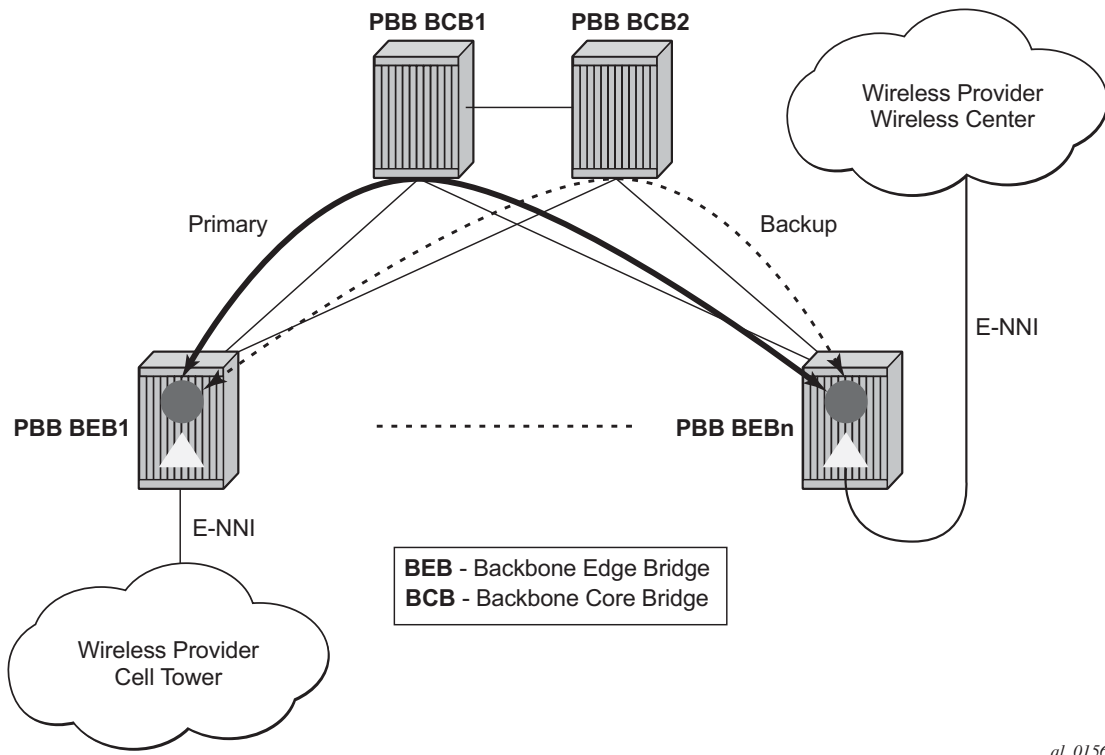
Figure 126: Mobile Backhaul Use Case
