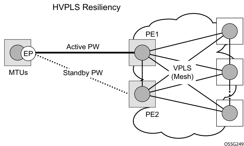
Figure 69: HVPLS Resiliency Based on AS Pseudowires
