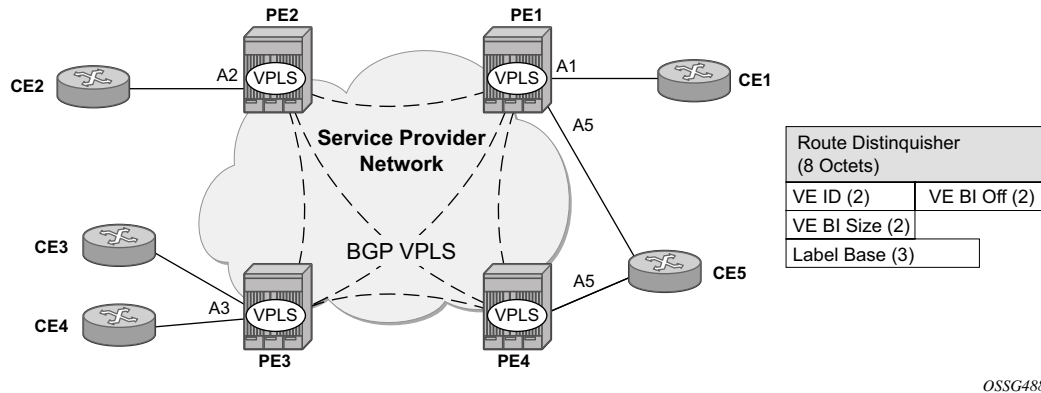
Figure 83: BGP VPLS Solution
