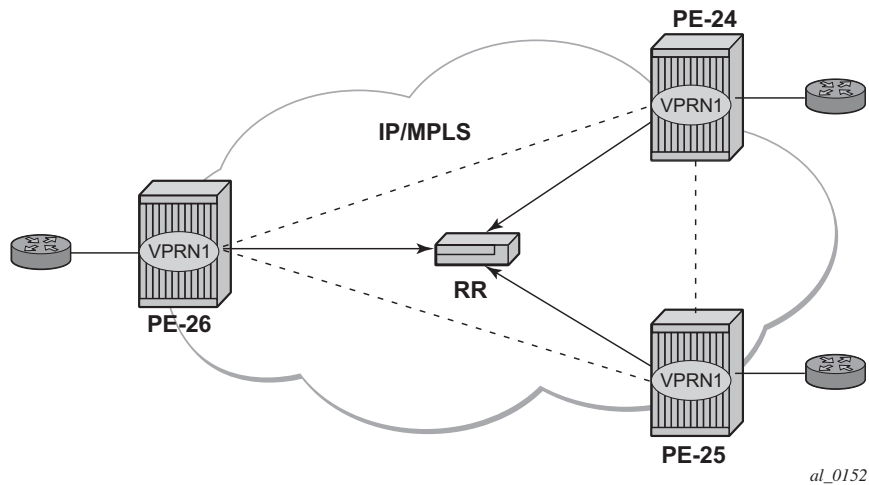
Figure 107: BGP VPLS Example
