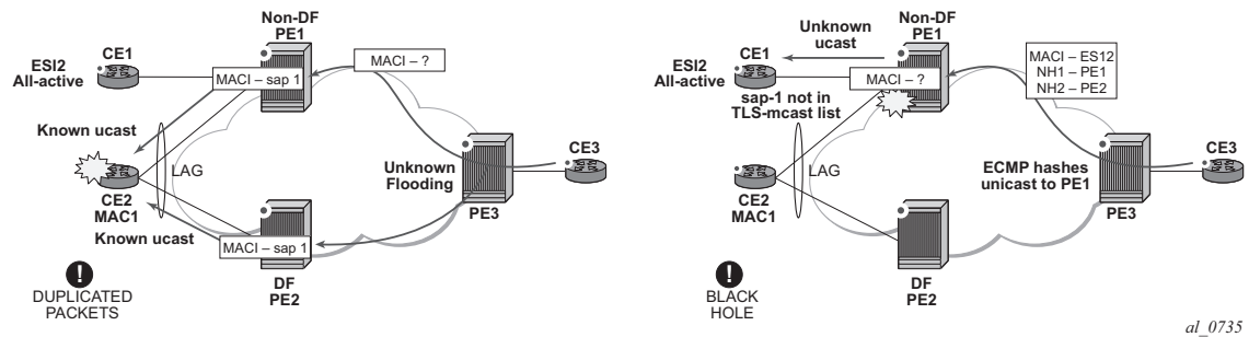
Figure 161: Transient Issues Caused by “slow” MAC Learning
