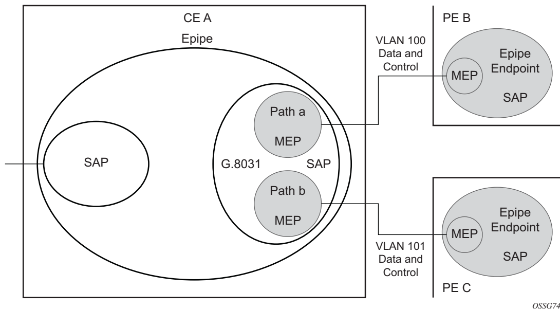
Figure 35: G.8031 for Slave Operation
