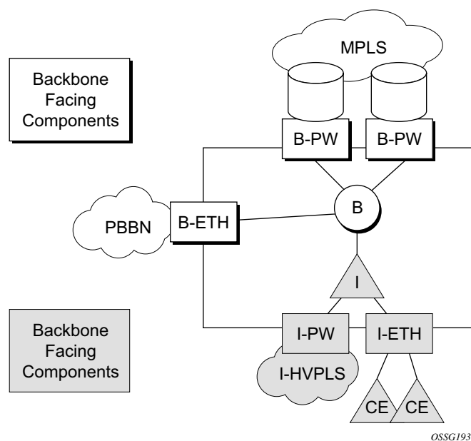
Figure 112: PBB Mapping to VPLS Constructs
