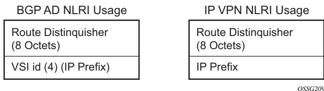
Figure 80: BGP AD NLRI versus IP VPN NLRI
