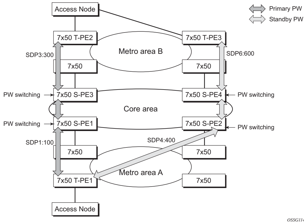
Figure 18: VLL Resilience with Pseudowire Redundancy and Switching
