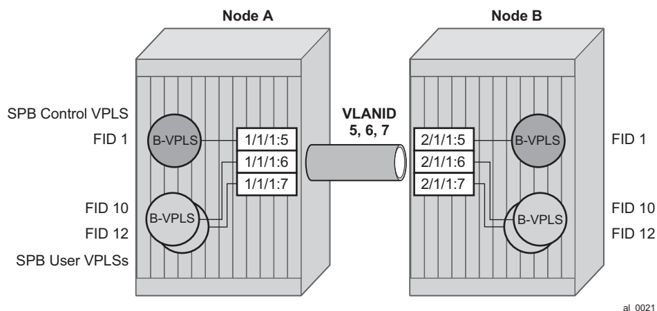
Figure 114: Control and User B-VPLS with FIDs
