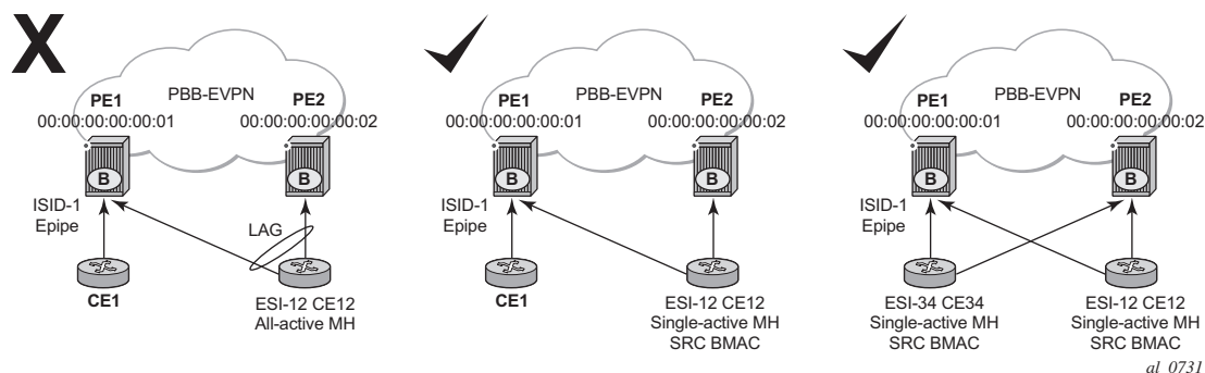
Figure 170: PBB-EVPN MH in a Two-Node Scenario
