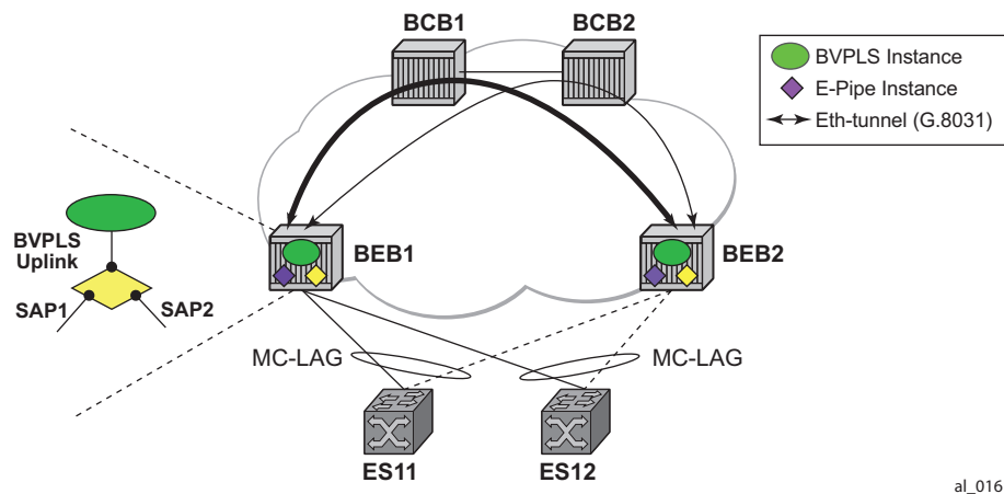
Figure 136: Solution for Access Dual-Homing with Local Switching for PBB Eline/Epipe
