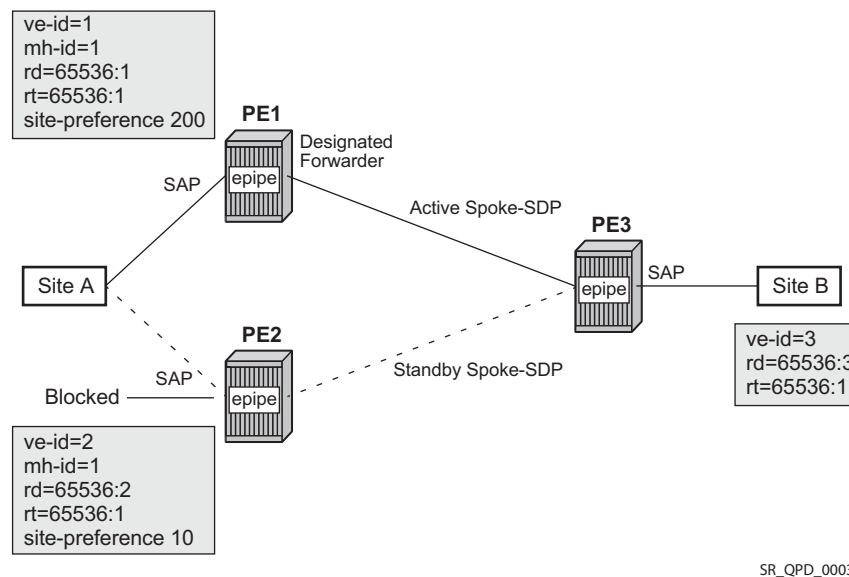
Figure 58: Example of Dual-homed BGP VPWS with Active/Standby Pseudowires
