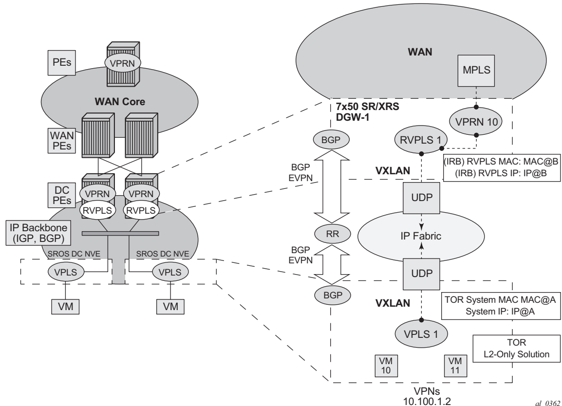
Figure 142: GW IRB on the DC PE for an L2 EVPN/VXLAN DC
