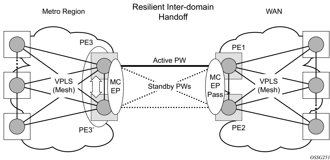
Figure 71: MC-EP in Passive Mode
