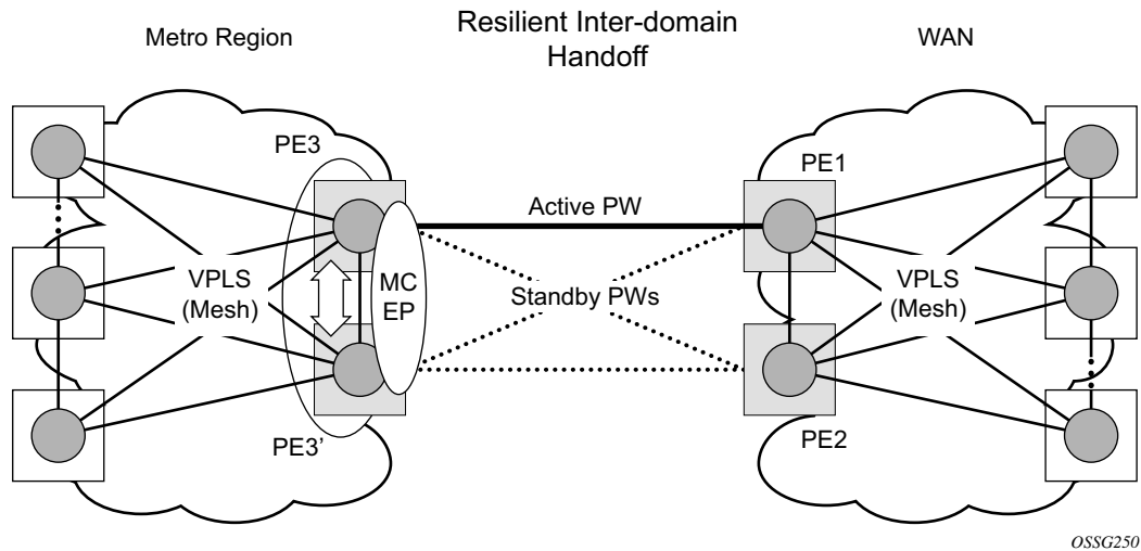
Figure 70: Multi-Chassis Pseudowire Endpoint for VPLS
