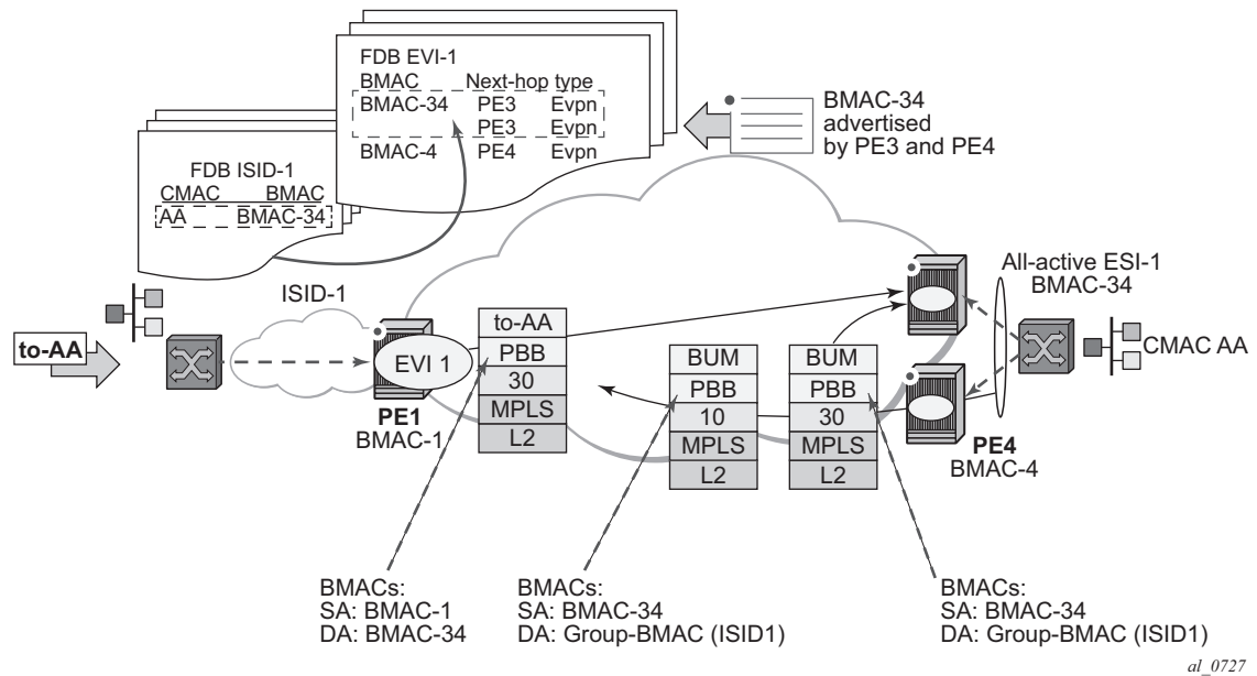
Figure 167: PBB-EVPN All-Active Multi-Homing
