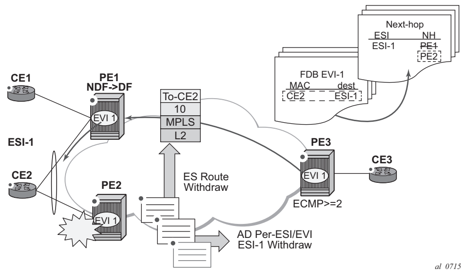
Figure 159: All-Active Multi-Homing ES Failure
