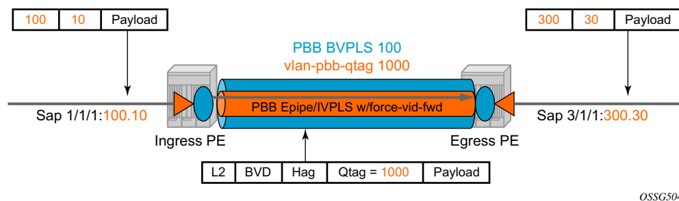
Figure 138: PCP, DE Bits Transparency in PBB
