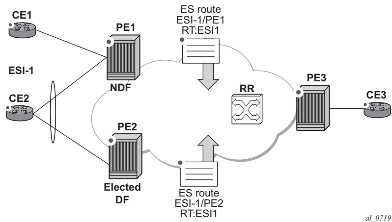
Figure 158: ES Discovery and DF Election
