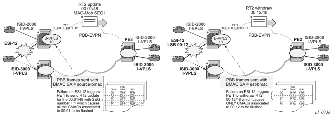
Figure 168: Source-Bmac Versus Es-Bmac CMAC Flushing
