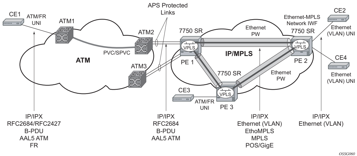
Figure 99: ATM/Frame Relay PVC Access and Termination on a VPLS Example
