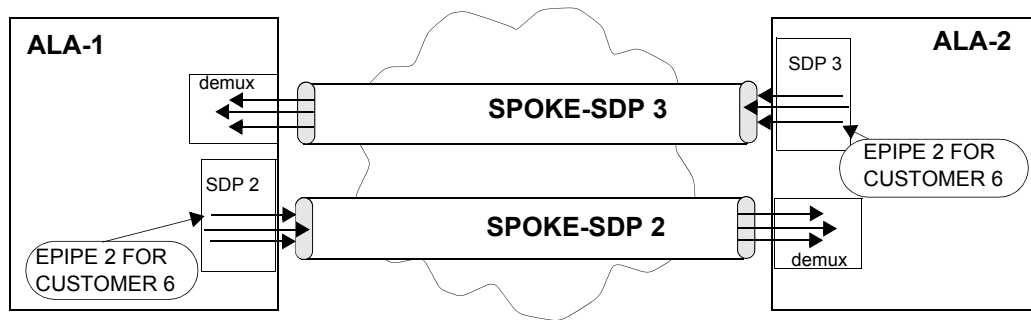
Figure 52: SDPs — Uni-Directional Tunnels
