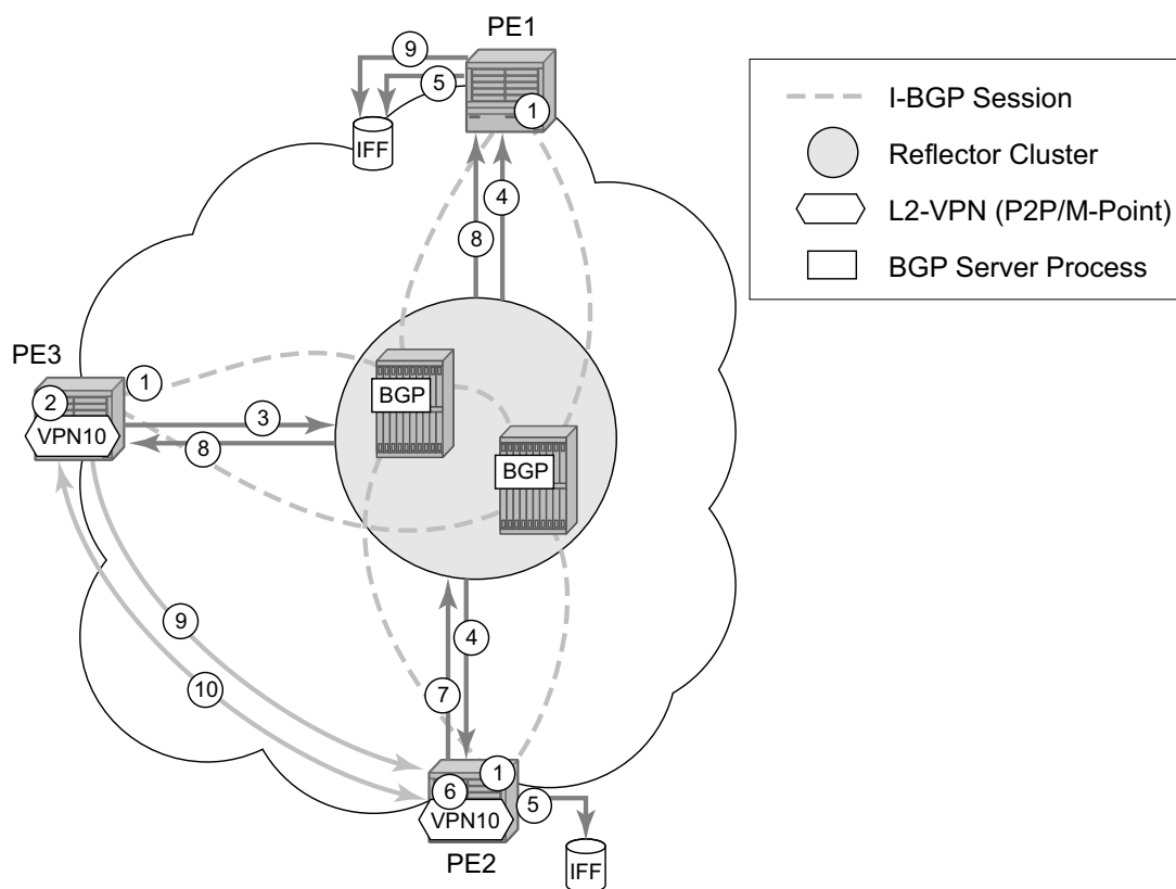
Figure 82: BGP-AD and T-LDP Interaction
