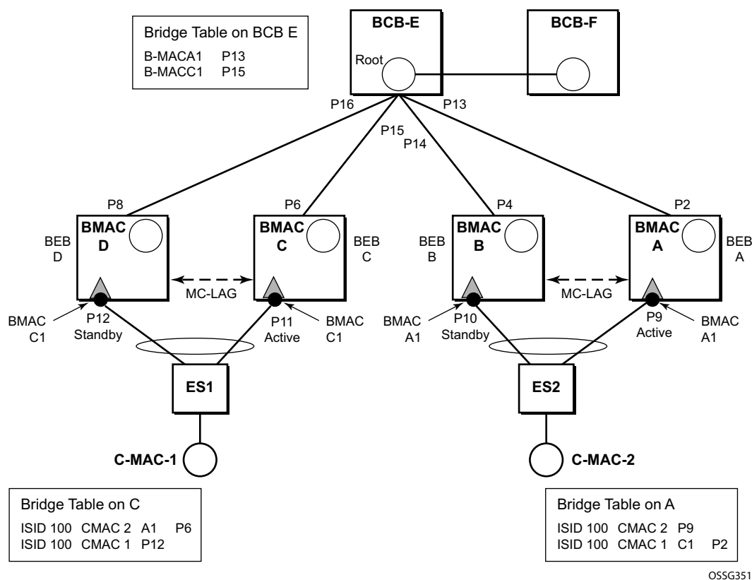
Figure 132: PBB Active Topology and Access Multi-Homing
