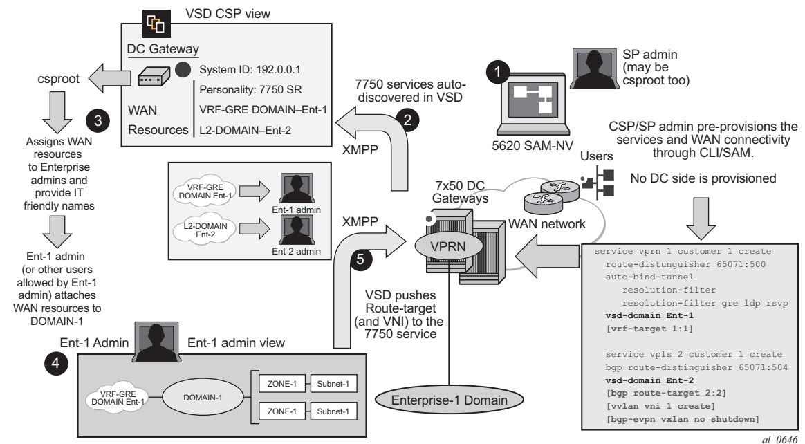
Figure 151: WAN Services Attachment Workflow
