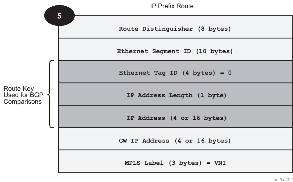
Figure 149: EVPN Route-Type 5
