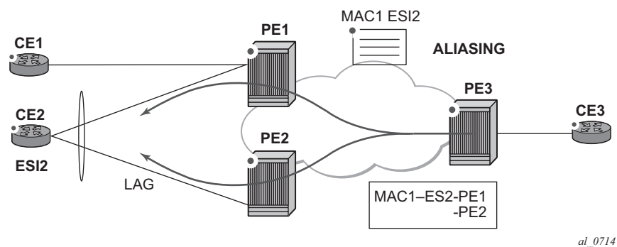
Figure 157: Aliasing
