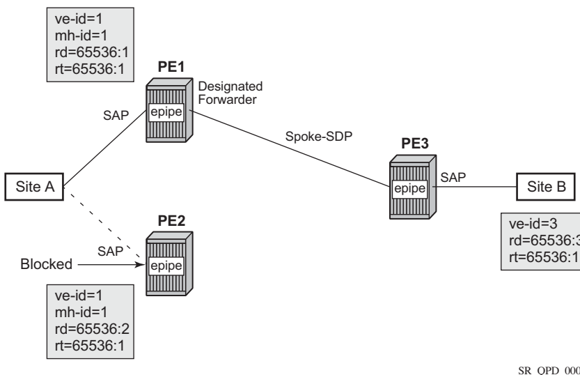
Figure 57: Example of Dual-Homed BGP VPWS with Single Pseudowire
