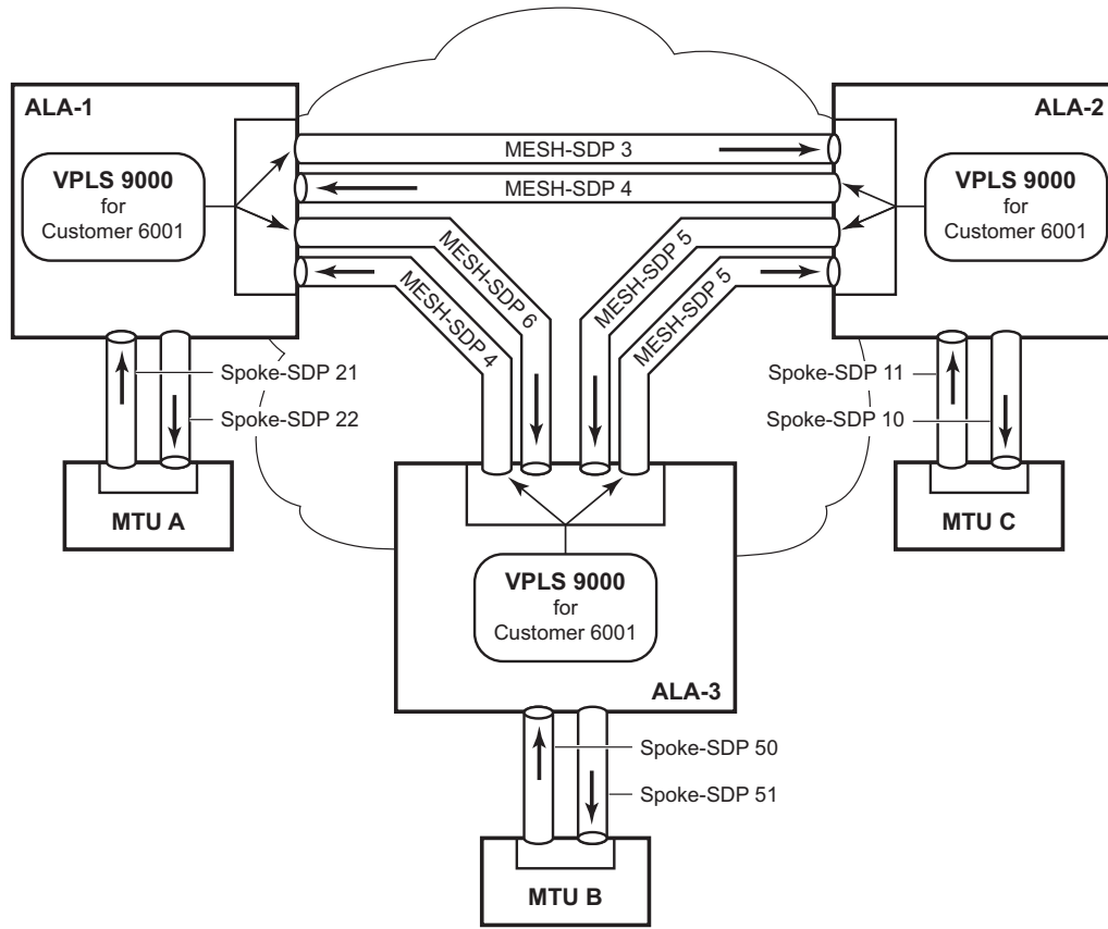
Figure 95: SDPs — Uni-Directional Tunnels
