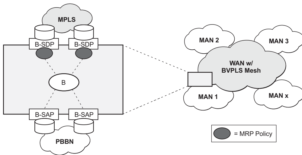
Figure 125: Limiting the Scope of MMRP Advertisements
