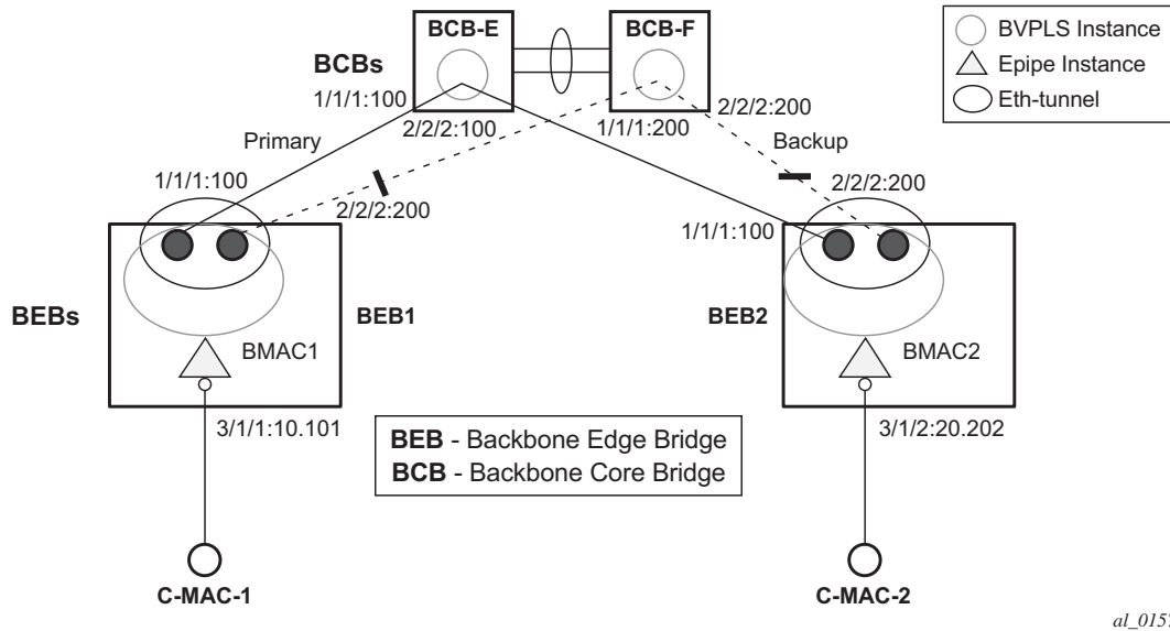
Figure 127: PBB-Epipe with B-VPLS over Ethernet Tunnel
