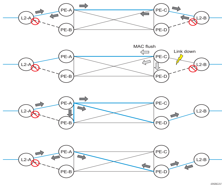
Figure 77: Dual Homed CE Connection to VPLS
