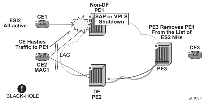
Figure 160: Black-hole Caused by SAP/SVC Shutdown
