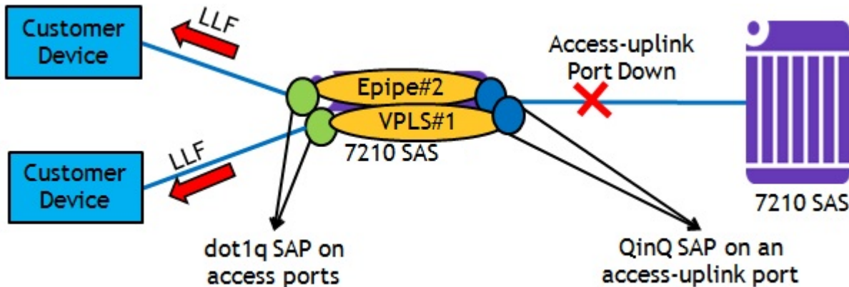
Figure 12: Local Fault Propagation
