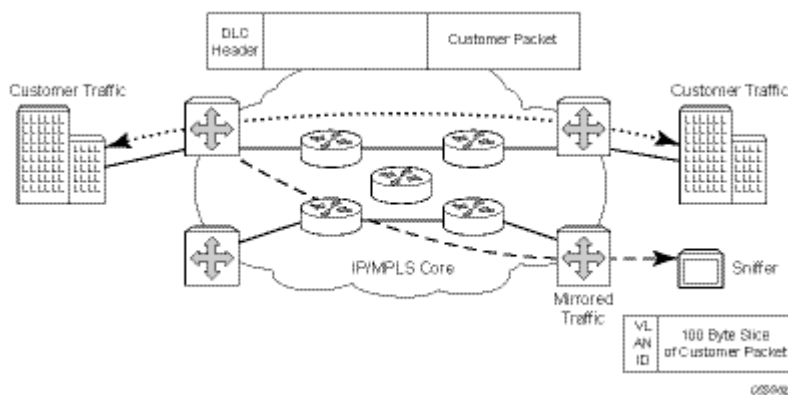
Figure 1: Service Mirroring
