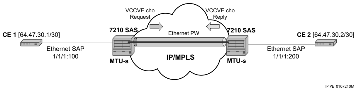
Figure 9: VCCV-Ping Application
