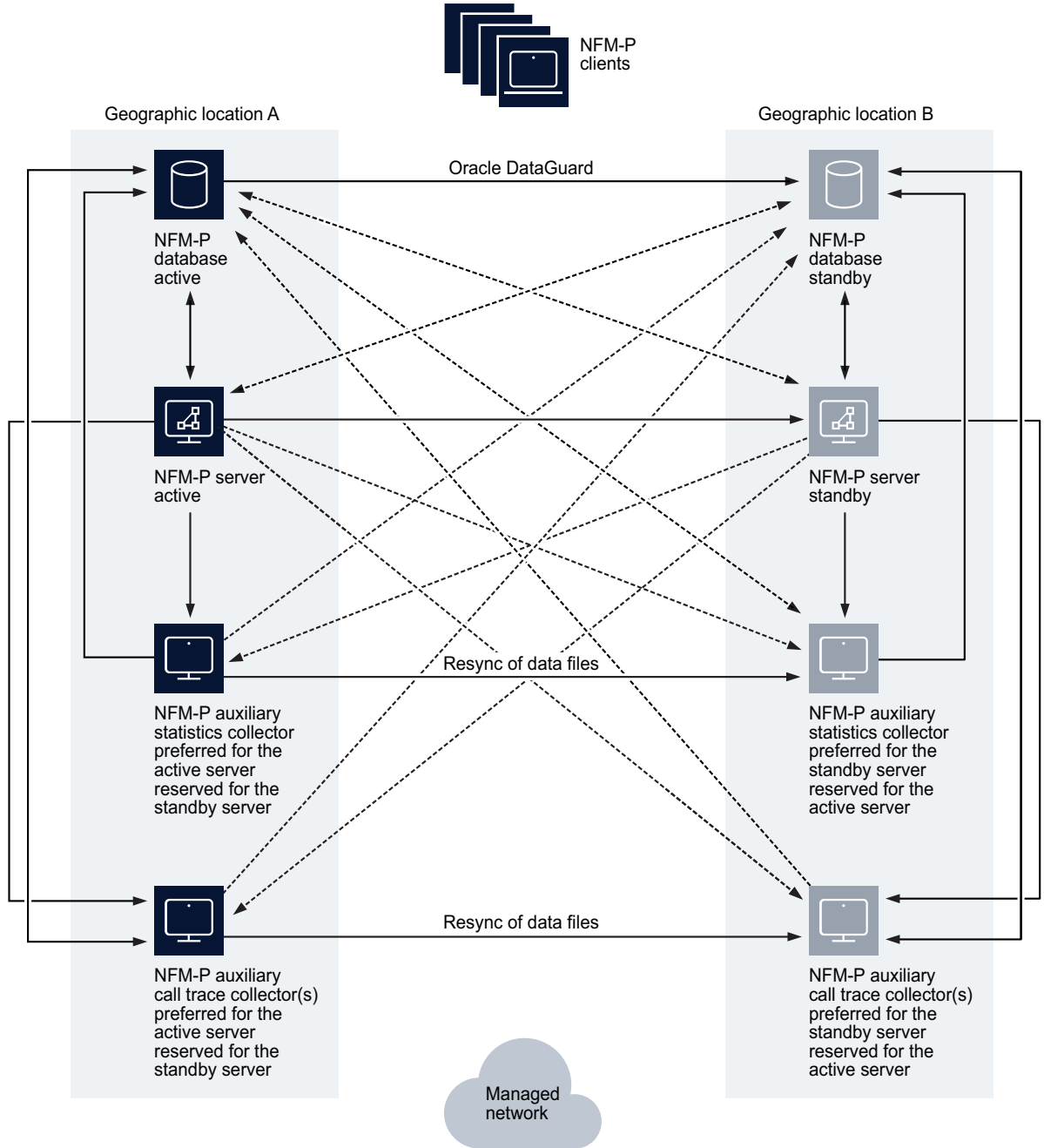
Figure 8 NFM-P distributed server/database redundant deployment with redundant NFM-P auxiliaries that crosses geographic boundaries
