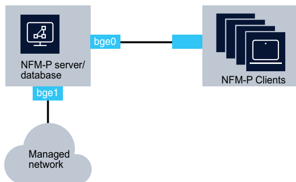
Figure 12 Collocated NFM-P server/database deployment with multiple network interfaces
