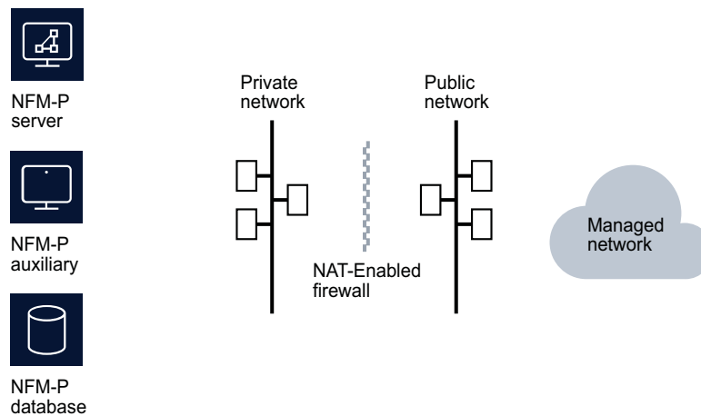
Figure 14 NFM-P server deployments with NAT between the server and the managed network
