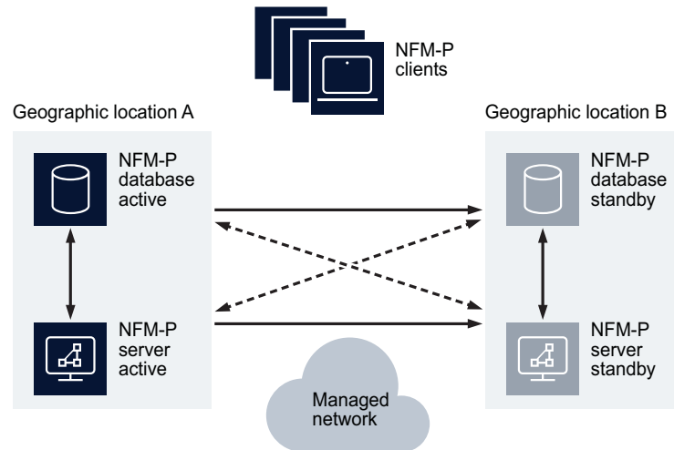
Figure 7 NFM-P distributed server/database redundancy deployment in a geographically redundant setup.
