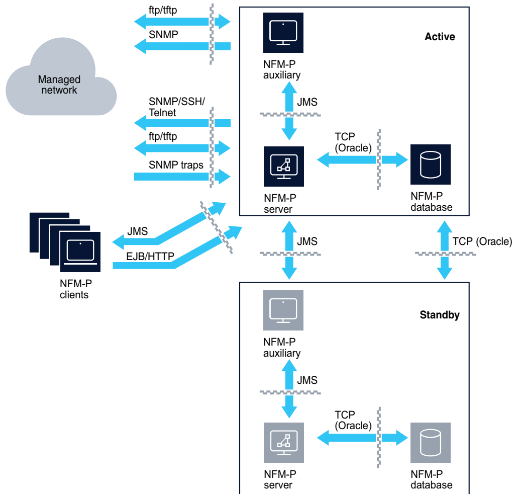
Figure 11 Firewalls and NFM-P redundant deployments
