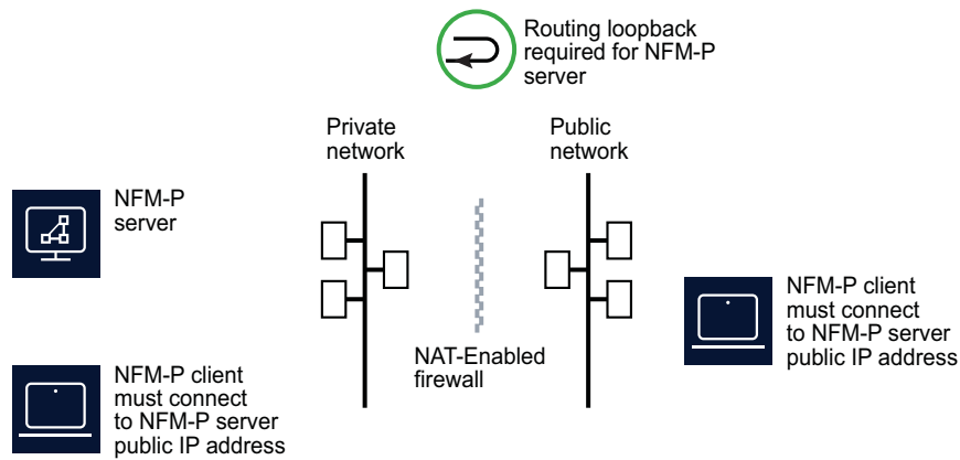
Figure 15 NFM-P server deployment using NAT with IP Address communication
