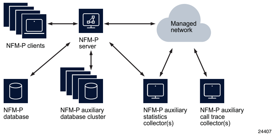
Figure 5 NFM-P standalone deployment - distributed NFM-P server and NFM-P database configuration and NFM-P auxiliary collectors with statistics collection using the NFM-P auxiliary database
