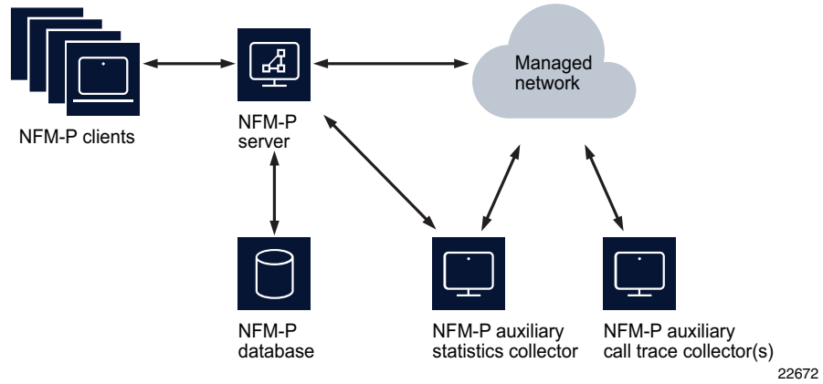
Figure 4 NFM-P standalone deployment - distributed NFM-P server and NFM-P database configuration and NFM-P auxiliary collectors
