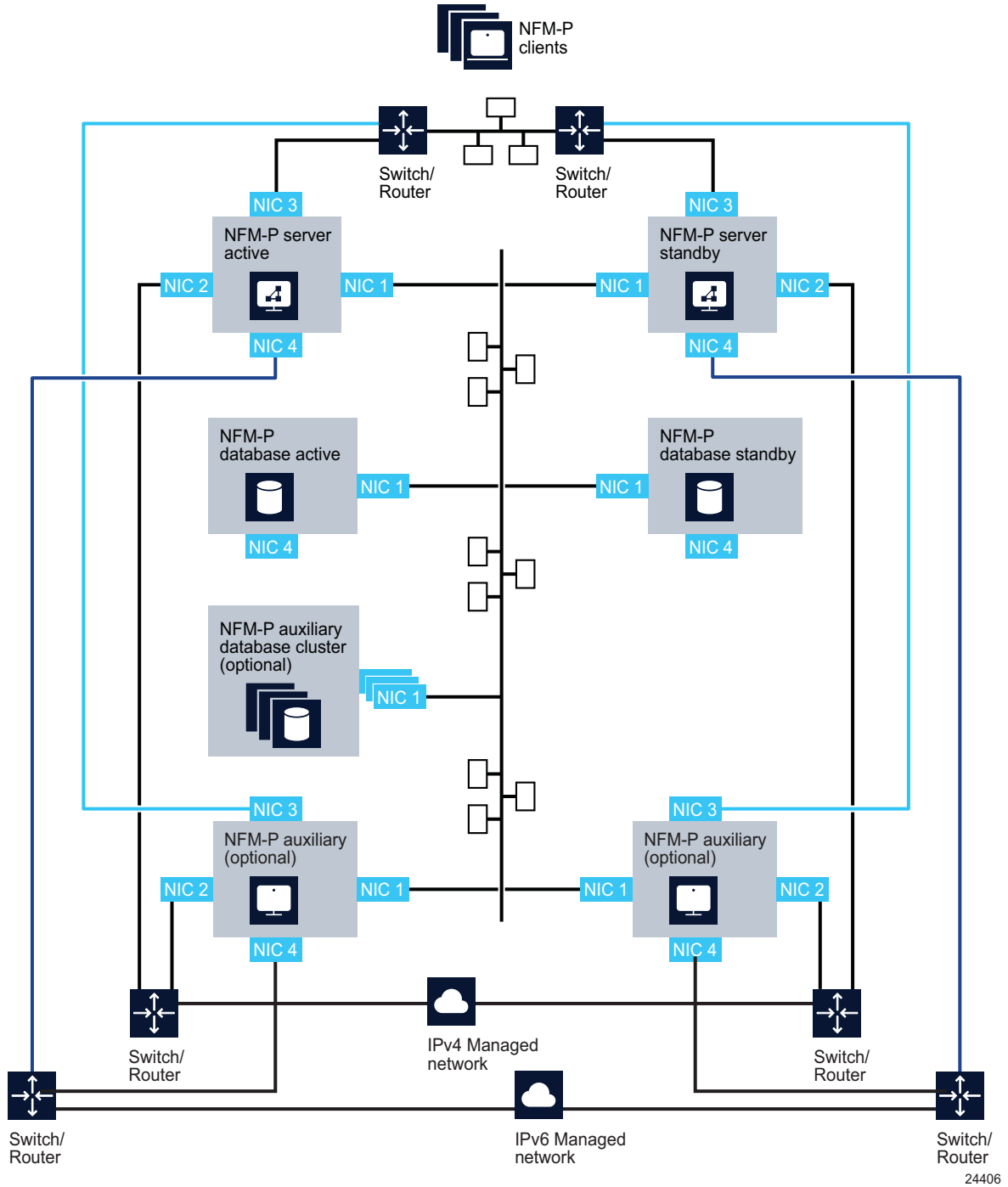
Figure 13 Distributed NFM-P server/database deployment with multiple network interfaces
