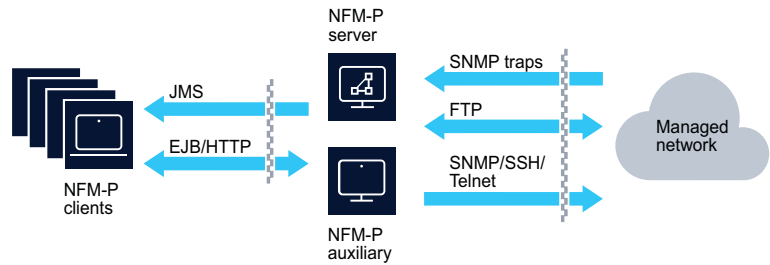
Figure 10 Firewalls and NFM-P standalone deployments
