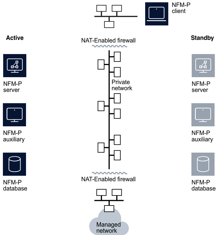
Figure 17 NFM-P deployment with NAT
