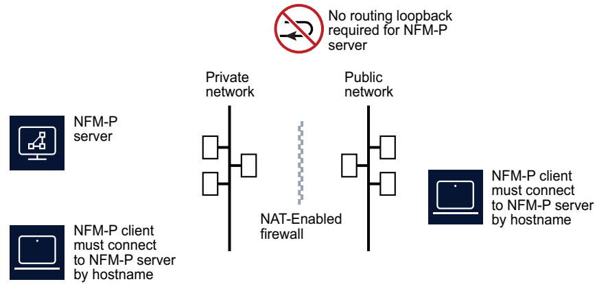
Figure 16 NFM-P server deployment using NAT with name resolution based communication
