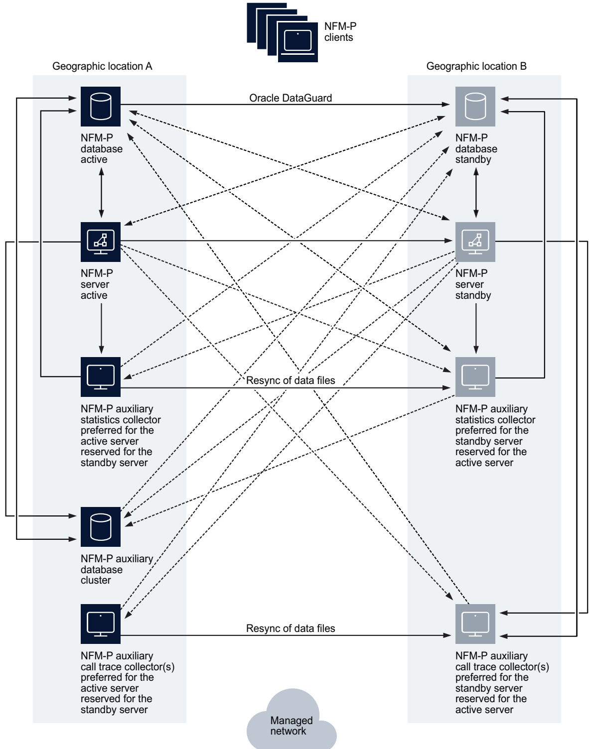
Figure 9 NFM-P distributed server/database redundant deployment with redundant NFM-P auxiliaries using the NFM-P auxiliary database for statistics collection
