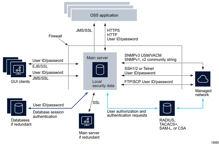
Figure 4 NFM-P security mechanisms
