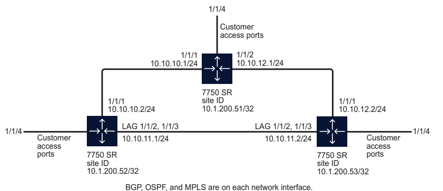
Figure 4-1 Sample network
