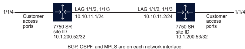
Figure 3-1 Sample network
