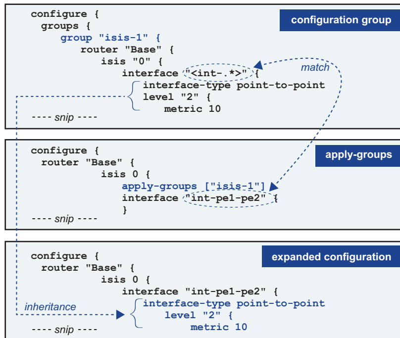
Figure 11 Configuration Groups
