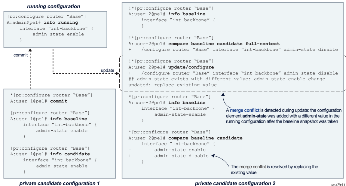
Figure 6 Simultaneous Configuration Sessions - Merge Conflict
