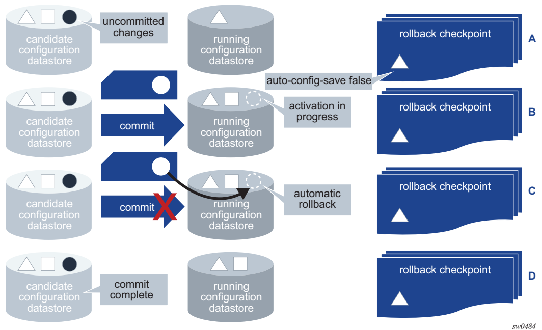
Figure 10 Failed commit
