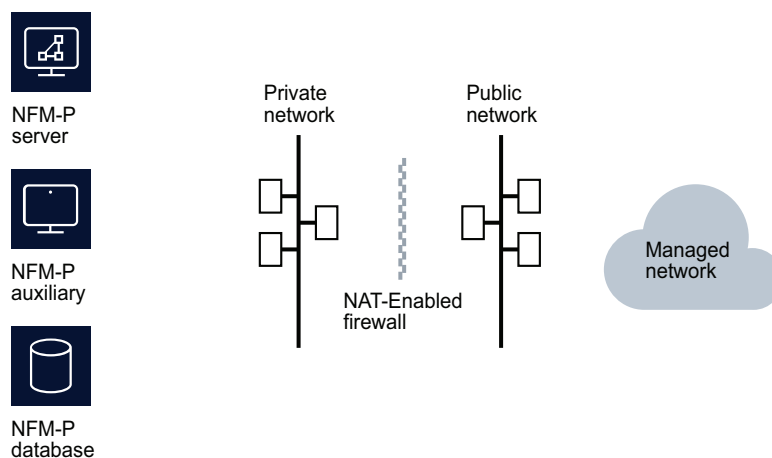
Figure 8-3 NFM-P server deployments with NAT between the server and the managed network
