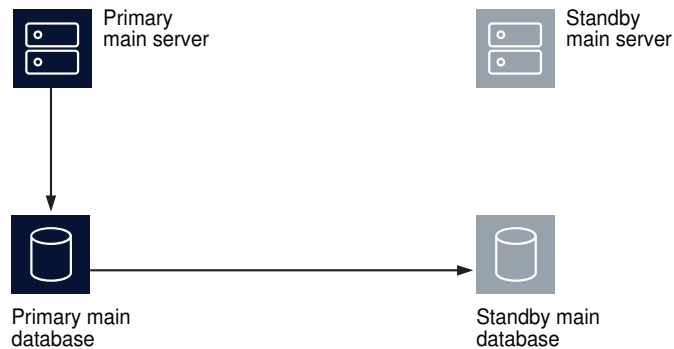
Figure 7-6 Server and database roles before database switchover
