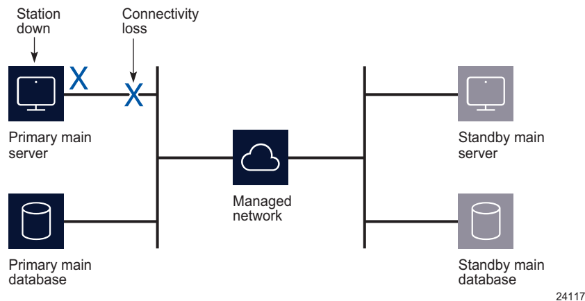
Figure 7-12 Primary server unreachable, distributed system
