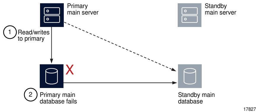
Figure 7-8 Server and database roles before database failover
