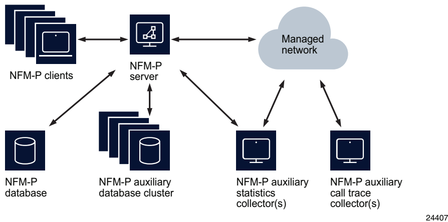
Figure 1-5 NFM-P standalone deployment - distributed NFM-P server and NFM-P database configuration and NFM-P auxiliary collectors with statistics collection using the NFM-P auxiliary database
