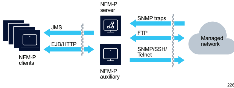
Figure 7-1 Firewalls and NFM-P standalone deployments
