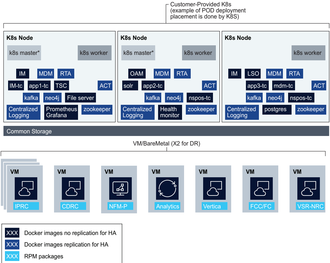
Figure 1-3 NSP deployment example
