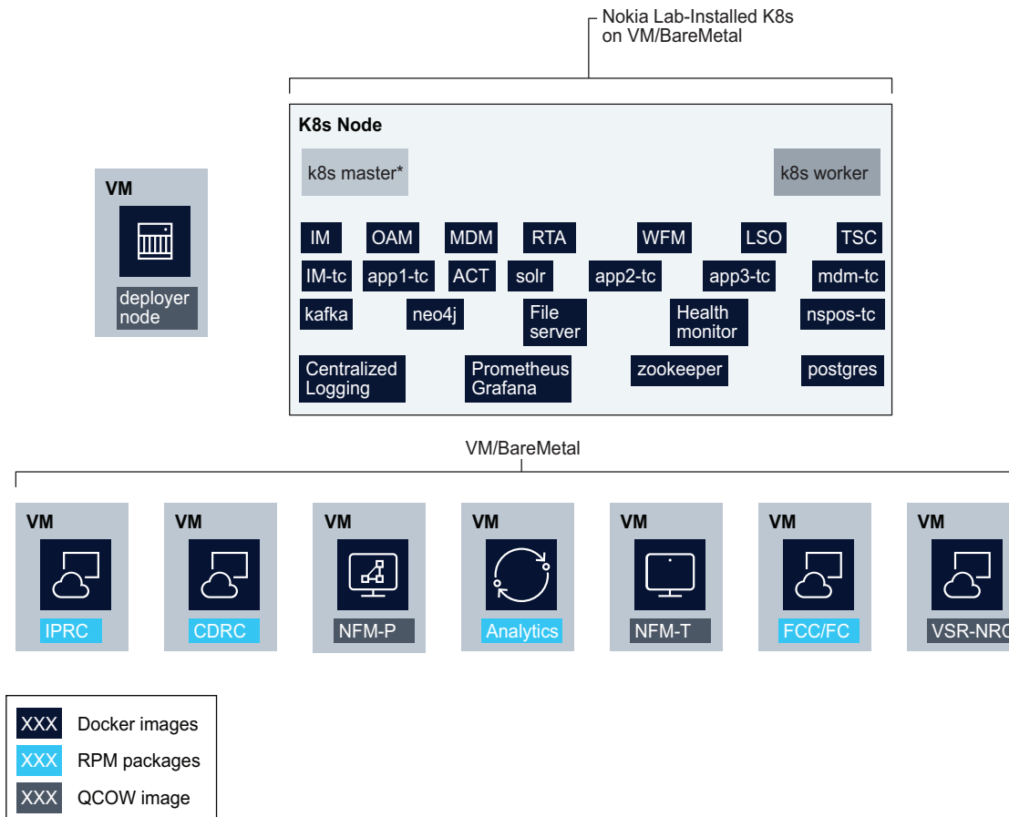
Figure 1-4 Containerized NSP lab deployment example
