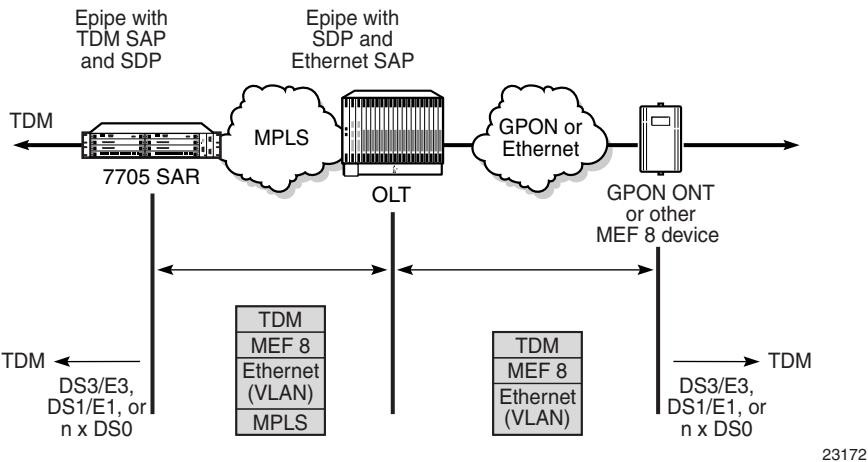
Figure 52 TDM SAP to Spoke SDP
