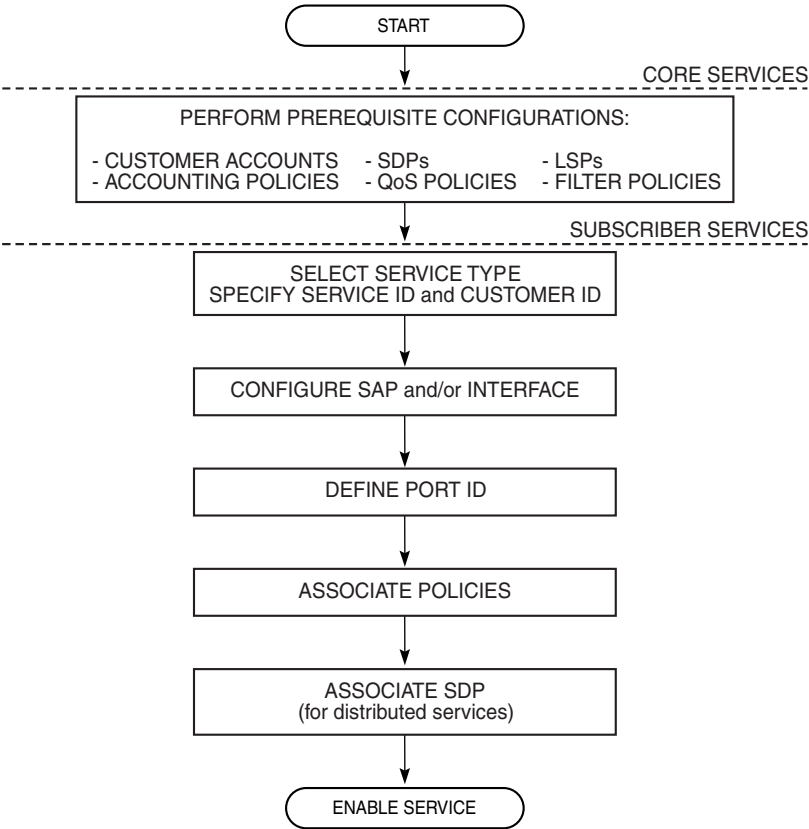
Figure 38 Service Creation and Implementation Flowchart
