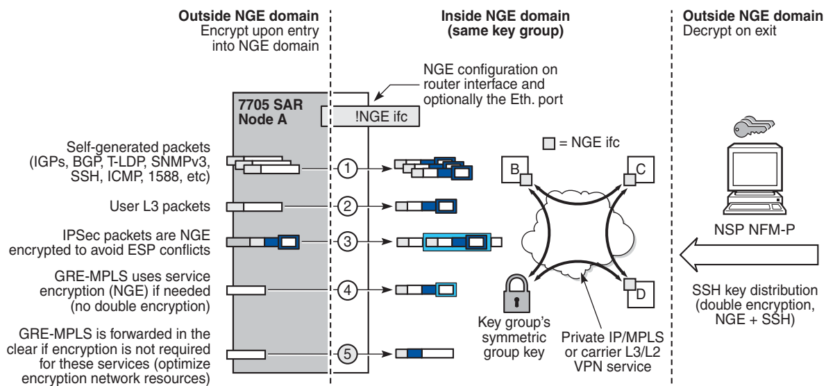
Figure 141 NGE Domain Transit
