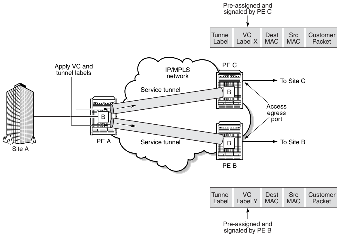
Figure 86 Network Port Egress Packet Format and Flooding
