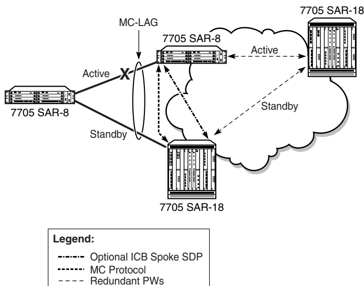
Figure 76 Access Side Failure with ICB Protection
