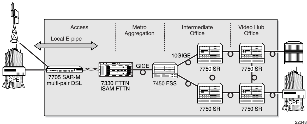
Figure 11 Pure DSL Backhaul Network Example
