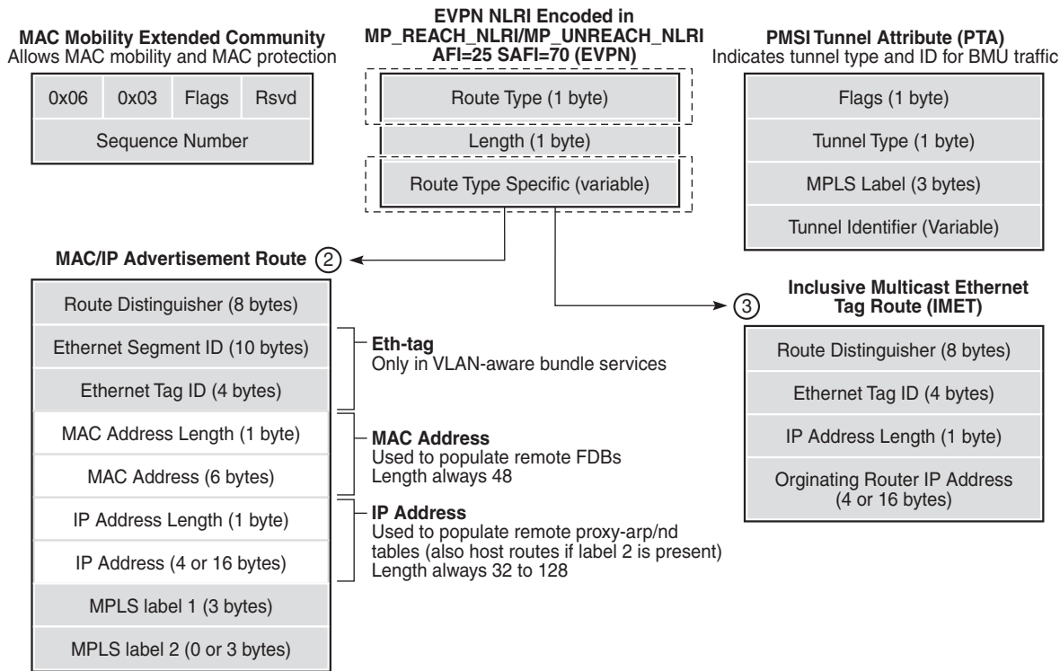
Figure 157 EVPN-MPLS Route Type 2 and Type 3 (Required Routes and Communities)
