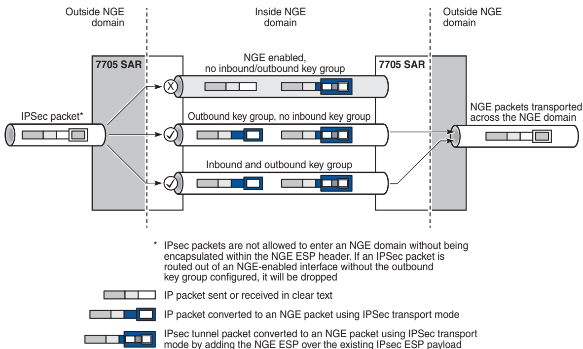
Figure 151 IPsec Packets Transiting an NGE Domain
