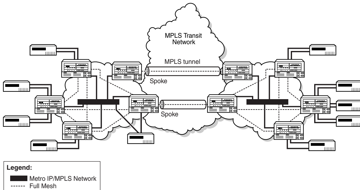
Figure 100 H-VPLS with Spoke Redundancy
