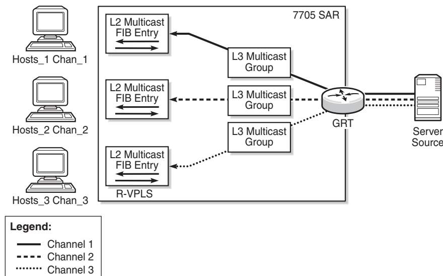
Figure 97 Multiple Hosts in an r-VPLS Receiving Different Channels
