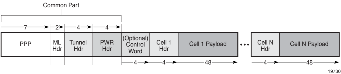
Figure 70 N-to-1 Cell Mode Encapsulation
