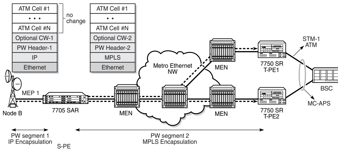
Figure 67 Simplex to Redundant Pseudowire Switching
