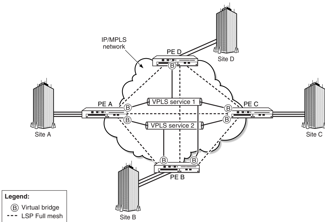
Figure 84 VPLS Service Architecture
