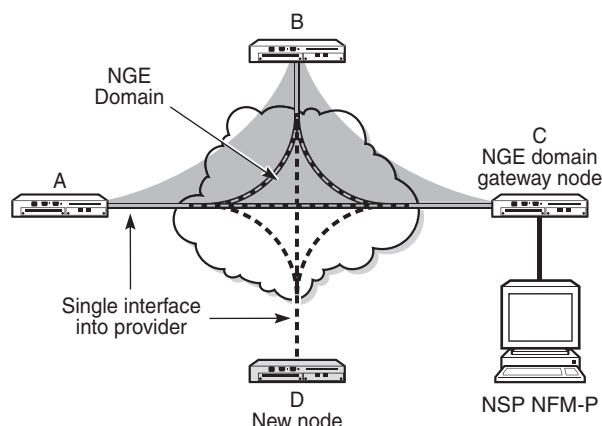
Figure 143 Private Over Intermediary Network NGE Domain
