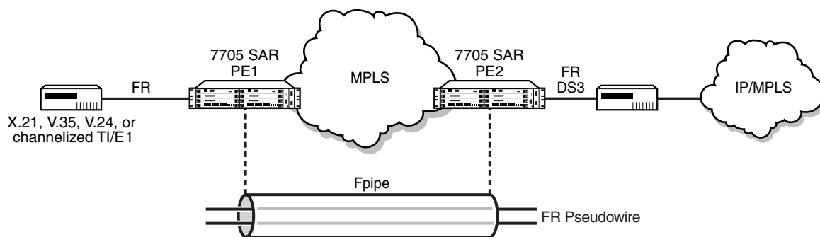
Figure 53 FR VLL for End-to-End FR Service
