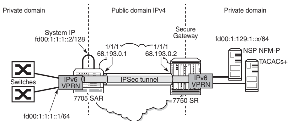
Figure 115 IPv6 In-Band Management Using a VPRN Configured with GRT Lookup
