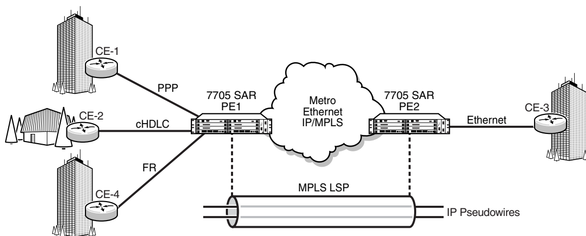
Figure 61 IP Pseudowires Between SAR Nodes
