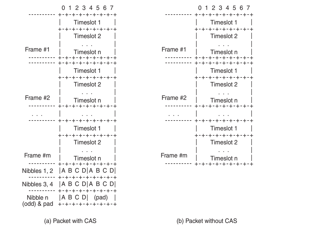
Figure 44 CESoPSN Packet Payload Format for Trunk-Specific n \times 64 kb/s (With and Without CAS Transport)
