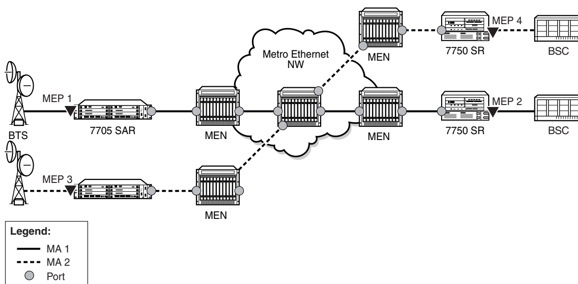
Figure 13 MEPs and MAs
