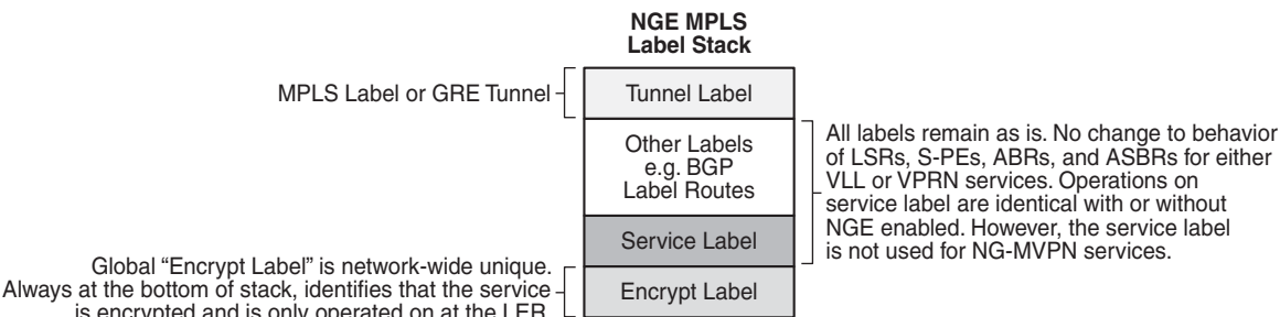
Figure 145 NGE MPLS/GRE Label Stack
