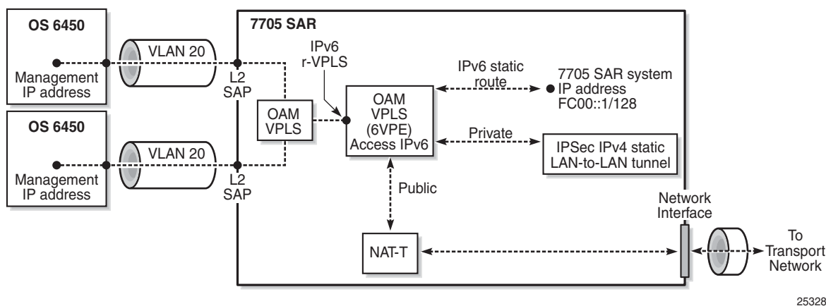
Figure 129 Access IPv6 Traffic Aggregation and Encryption
