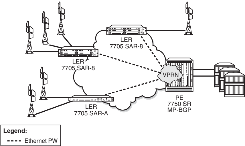
Figure 126 Pseudowire-Based Backhaul (Spoke SDP Termination at 7750 SR)
