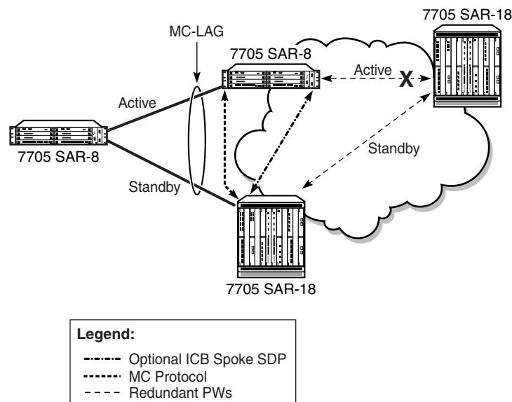
Figure 77 Network Side Failure with ICB Protection
