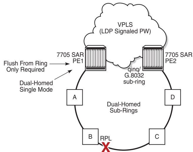
Figure 29 Multi-Ring Hierarchy
