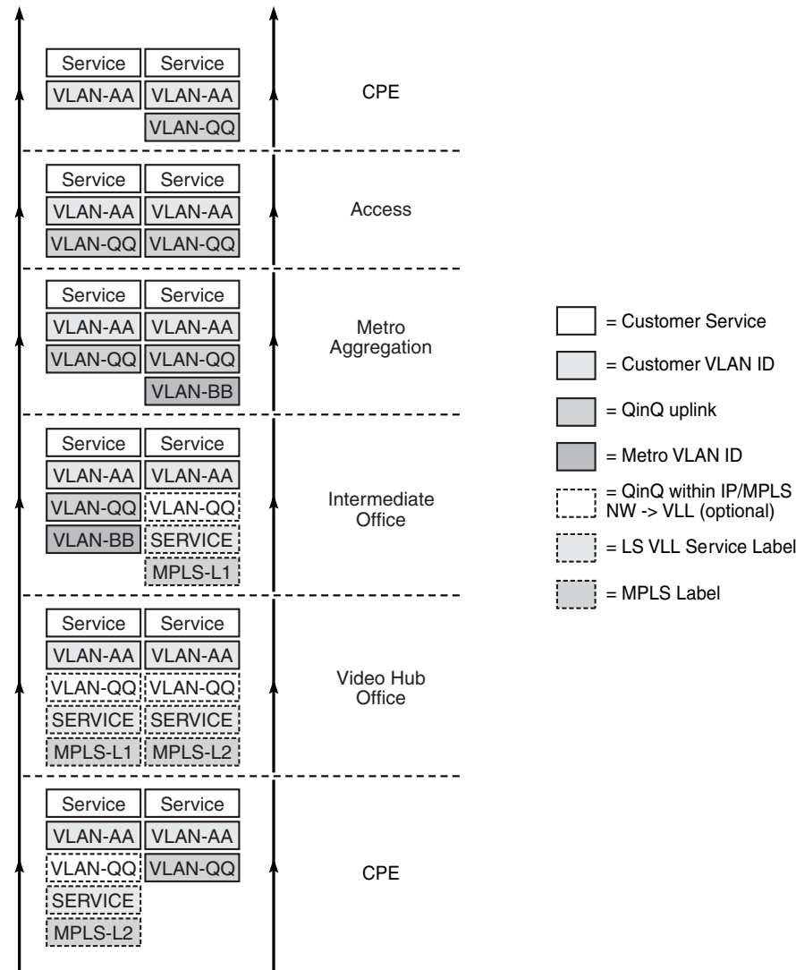
Figure 12 DSL Network Traffic
