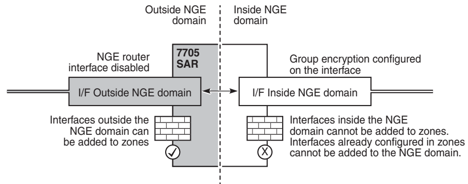
Figure 153 Firewall Considerations
