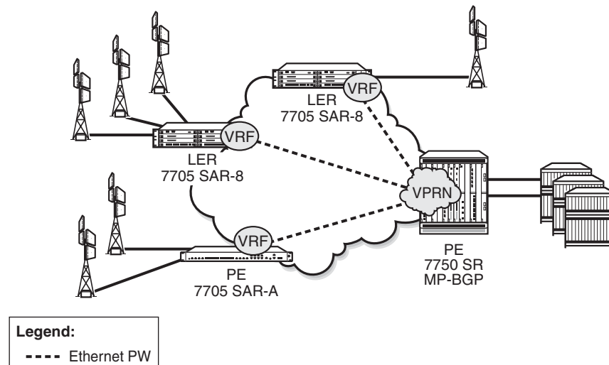
Figure 128 Spoke-SDP Termination to VPRN
