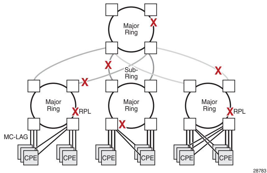
Figure 26 G.8032 Sub-Ring
