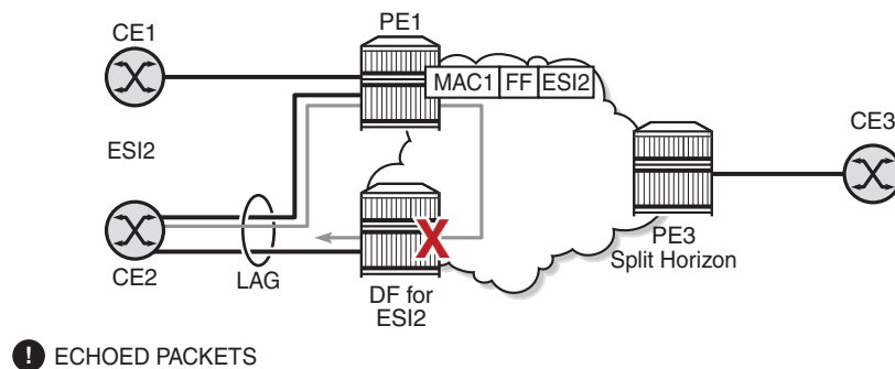
Figure 162 Split Horizon
