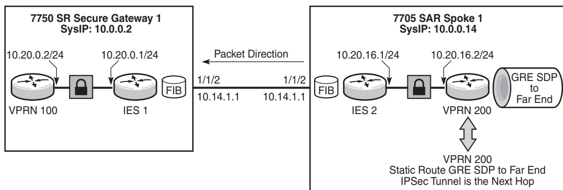
Figure 132 Routing GRE-Encapsulated Packets over IPSec
