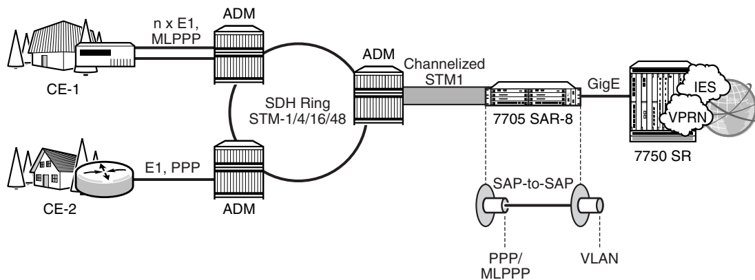
Figure 65 PPP and MLPPP to IP PWs on 2-port OC3/STM1 Channelized Adapter Cards
