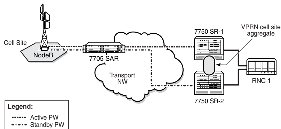
Figure 88 Typical Pseudowire-based Mobile Backhaul
