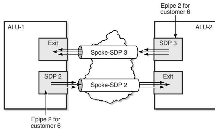
Figure 83 SDPs—Unidirectional Tunnels
