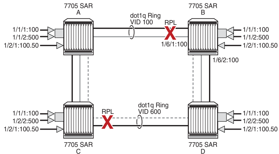
Figure 25 Ring Example
