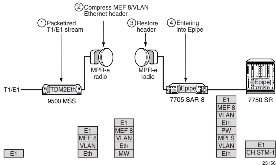
Figure 81 Mixed Microwave Link Scenario
