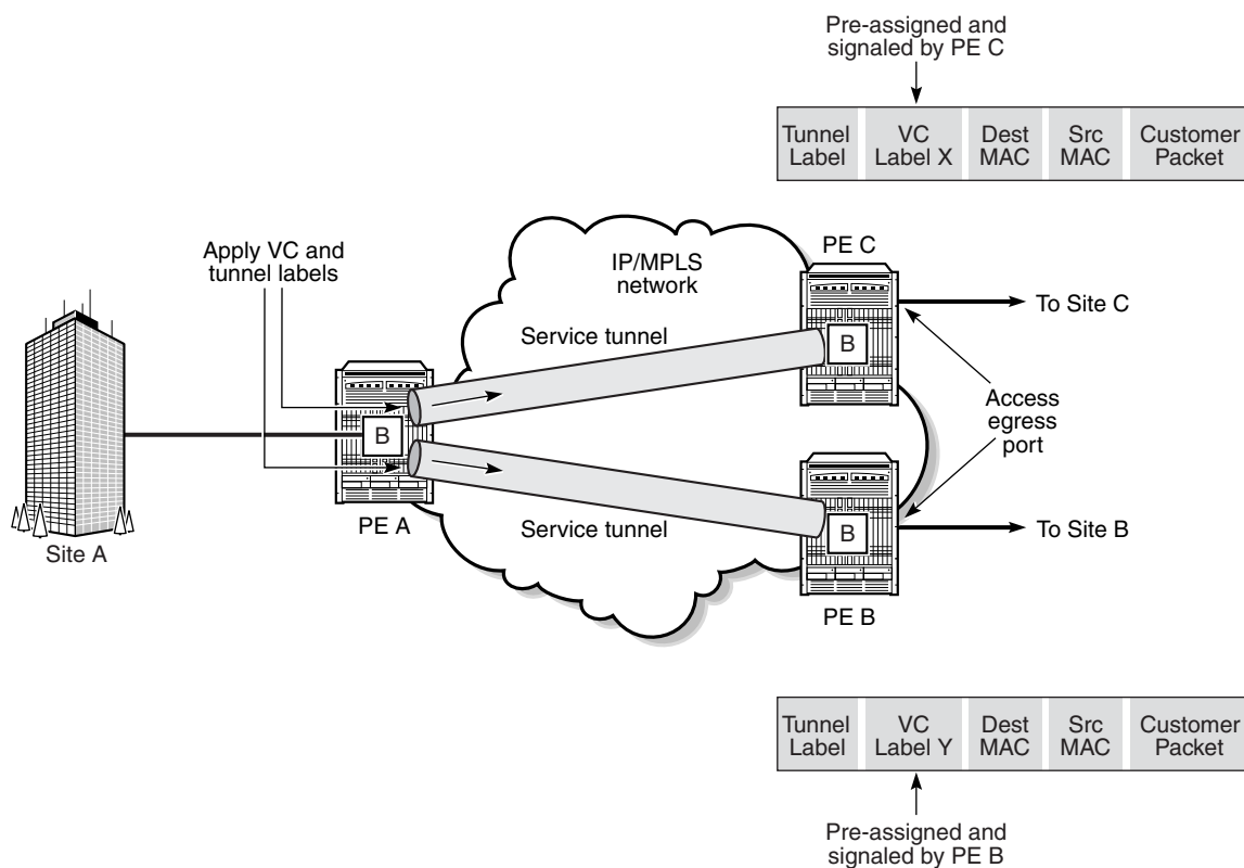
Figure 87 Access Port Egress Packet Format and Lookup
