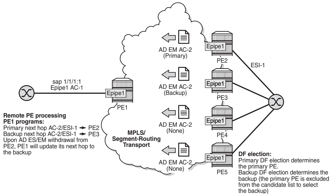
Figure 173 EVPN-VPWS Single-active Multihoming
