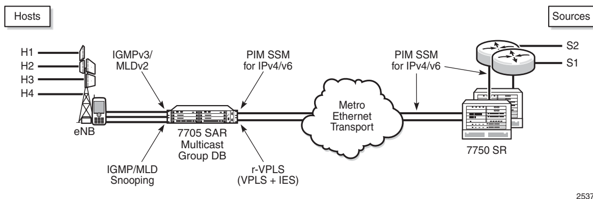
Figure 94 Video over Mobile Backhaul
