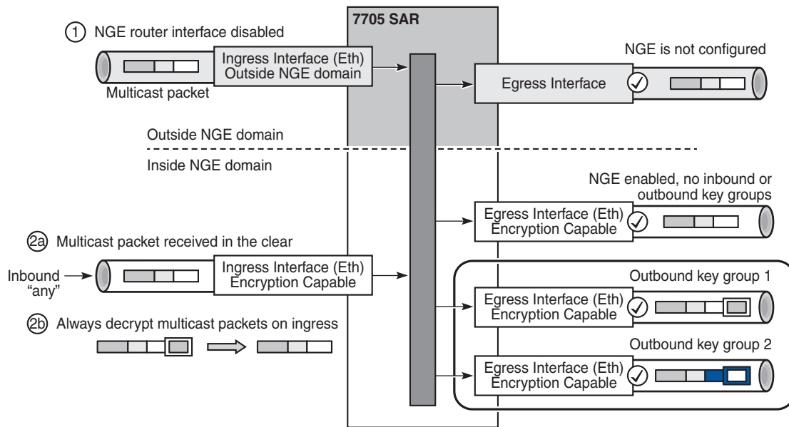
Figure 152 Processing Multicast Packets
