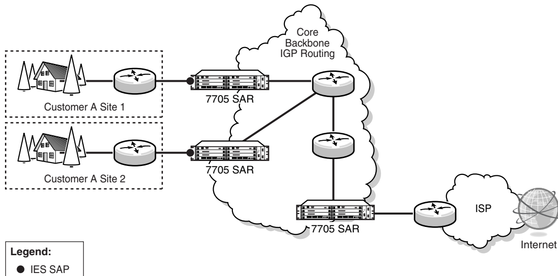
Figure 105 IES for Customer Access to the Internet
