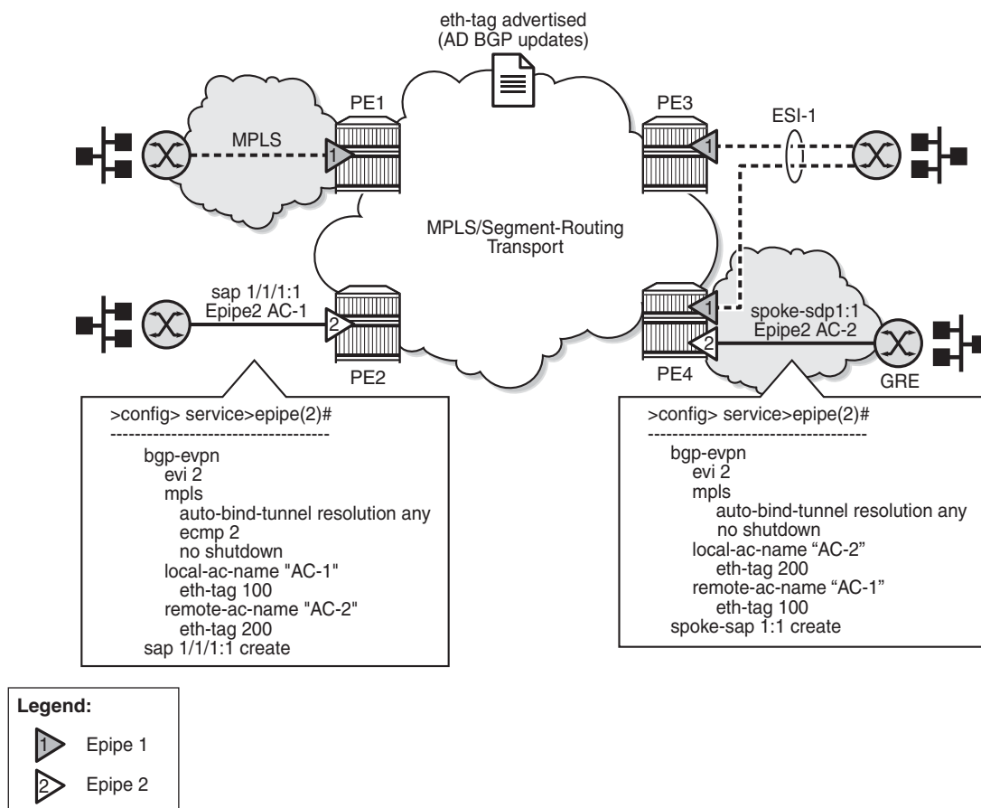
Figure 171 EVPN-MPLS in Epipe Services
