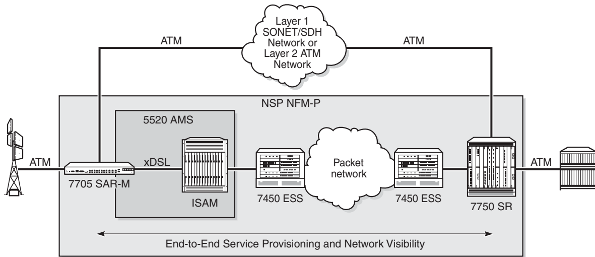
Figure 9 7705 SAR-M With 8-port xDSL Module for HSDPA Offload
