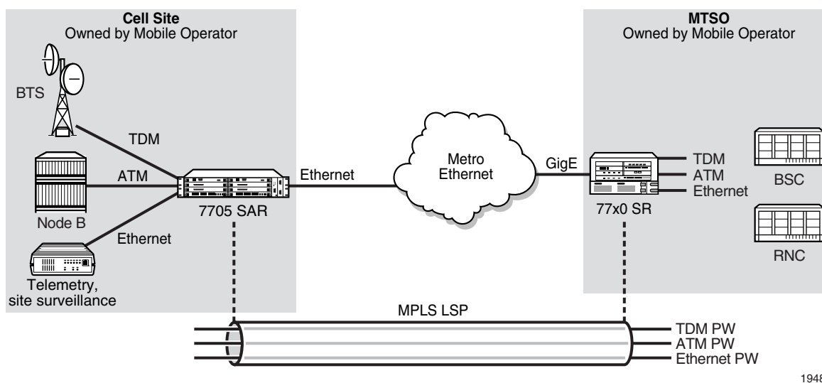
Figure 39 ATM VLL for End-to-End ATM Service
