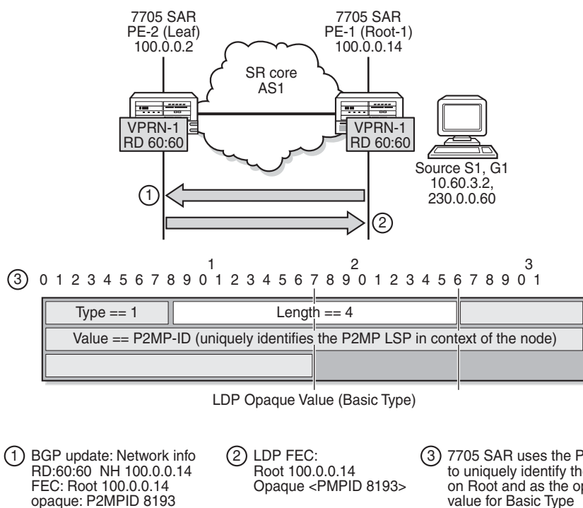
Figure 120 BGP MVPN Address Family Updates
