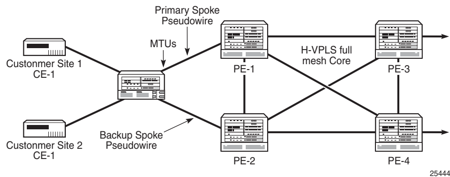
Figure 101 Dual Homed MTUs in Two-Tier Hierarchical VPLS
