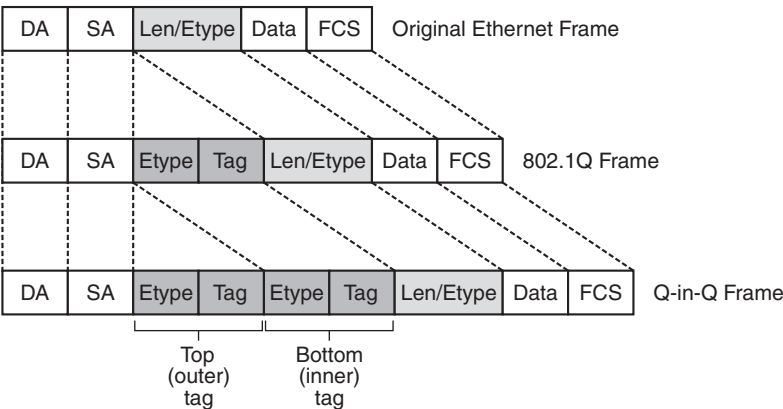
Figure 30 QinQ Frame
