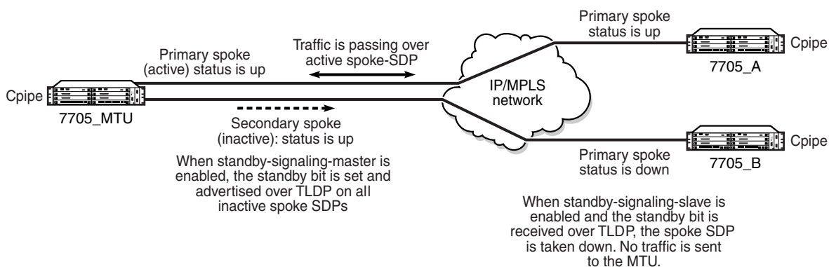
Figure 80 Standby-signaling-slave Enabled
