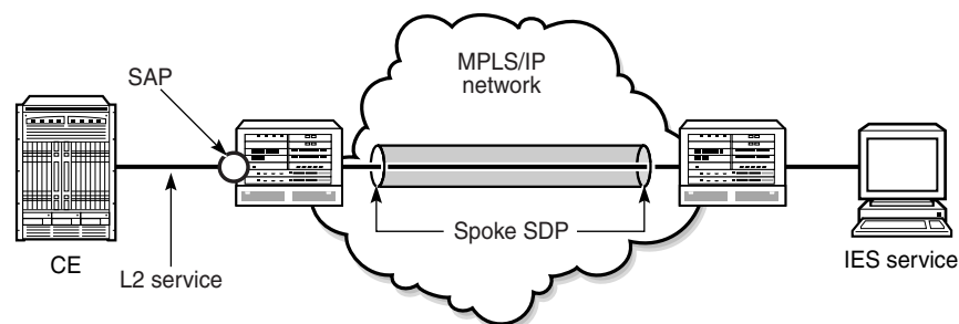
Figure 107 IES Spoke SDP Termination
