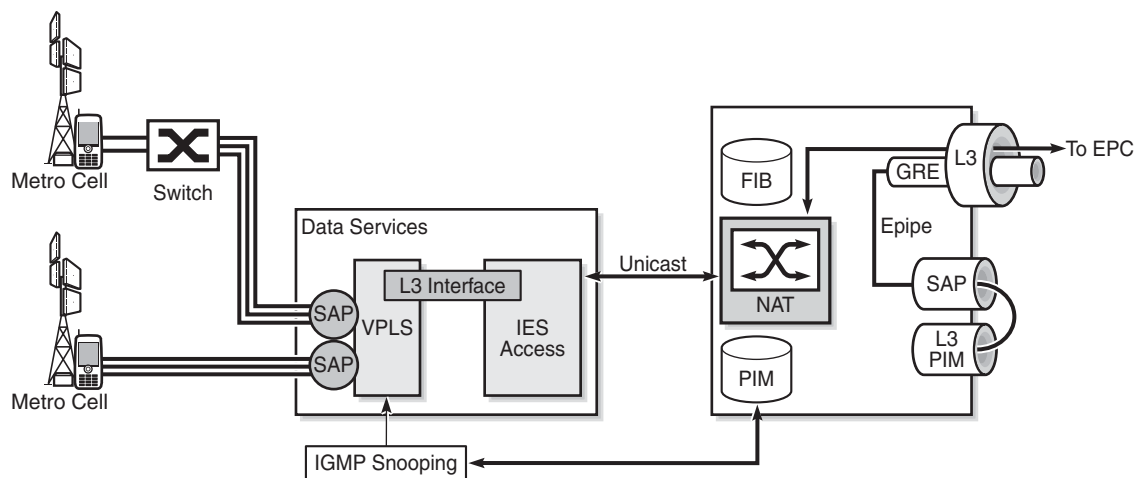
Figure 95 Metro Cell Multicast
