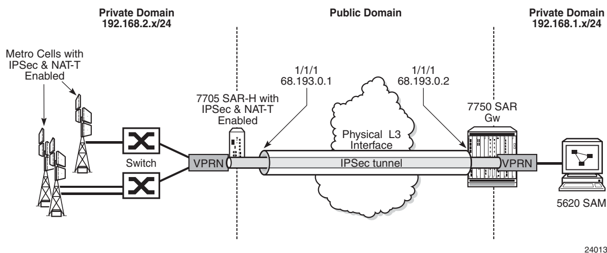
Figure 135 Typical Metrocell Deployment
