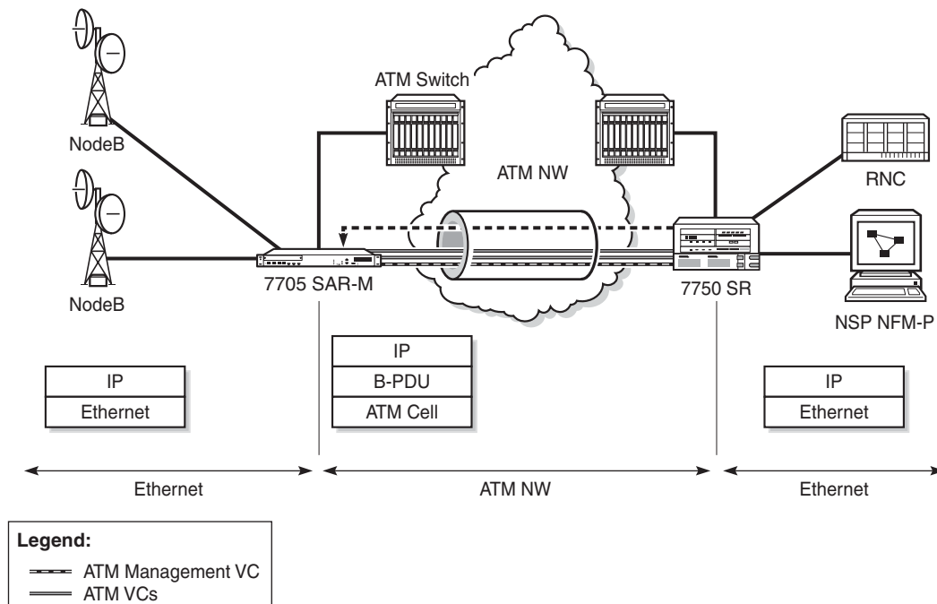
Figure 82 Ethernet-to-ATM Interworking on the 7705 SAR-M
