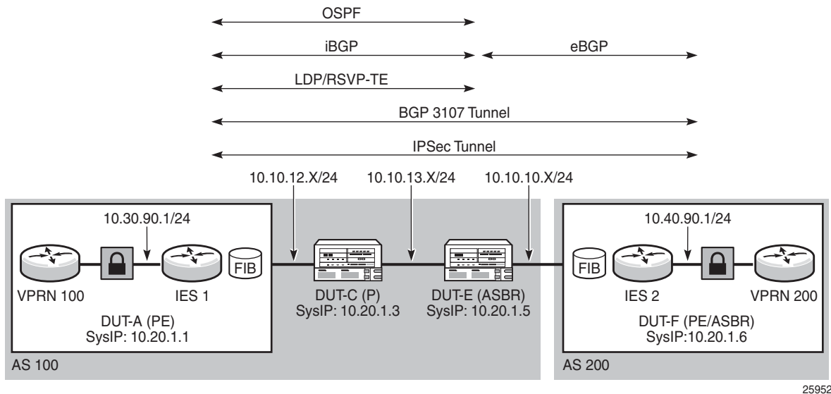
Figure 138 IPSec over BGP 3107 Label Route
