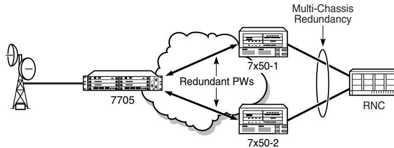
Figure 73 Pseudowire Redundancy
