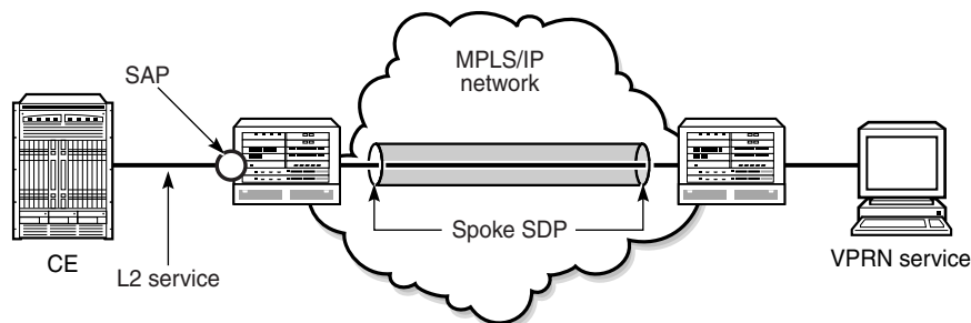
Figure 125 VPRN Spoke SDP Termination
