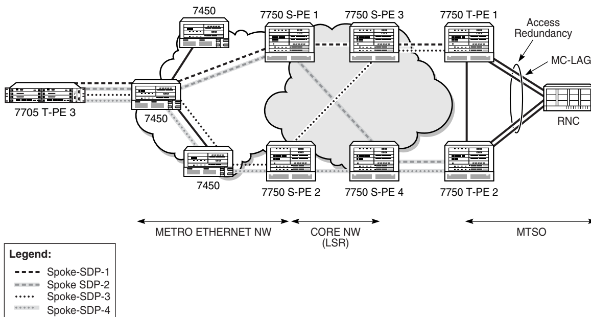
Figure 75 Pseudowire Redundancy with Four Spoke SDPs
