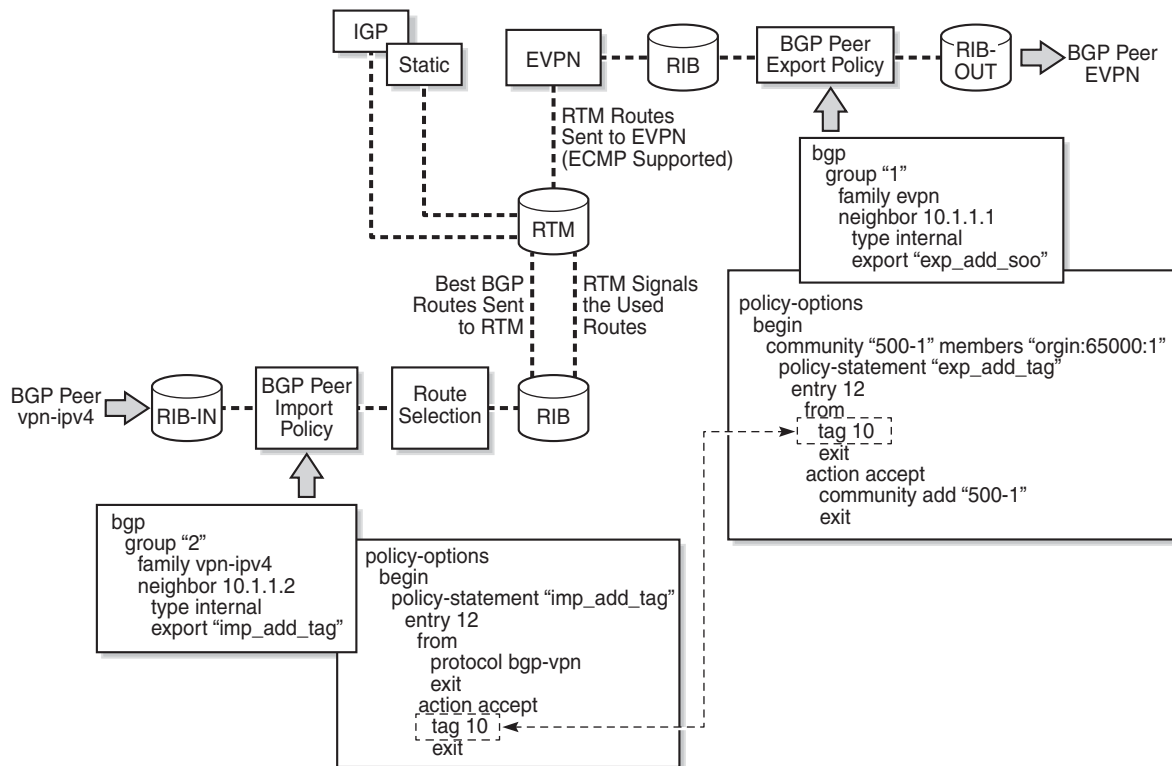
Figure 175 IP-VPN Import and EVPN Export BGP Workflow
