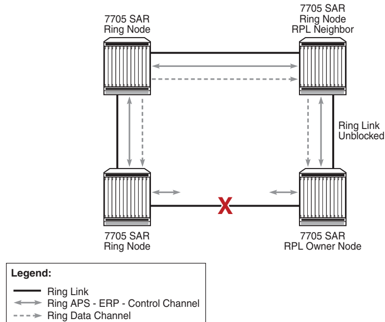
Figure 24 G.8032 Ring in the Protecting State
