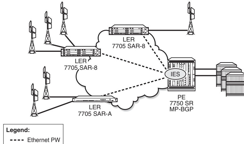
Figure 108 Pseudowire-Based Backhaul (Spoke SDP Termination at 7750 SR)
