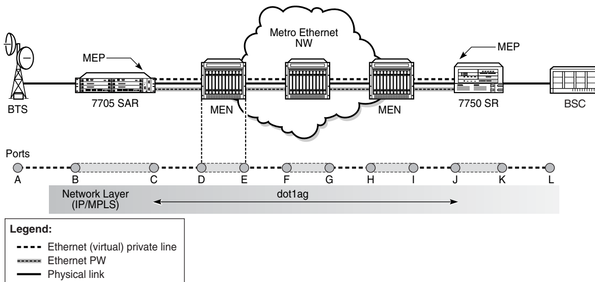
Figure 20 Dot1ag Down MEPs on Spoke SDPs
