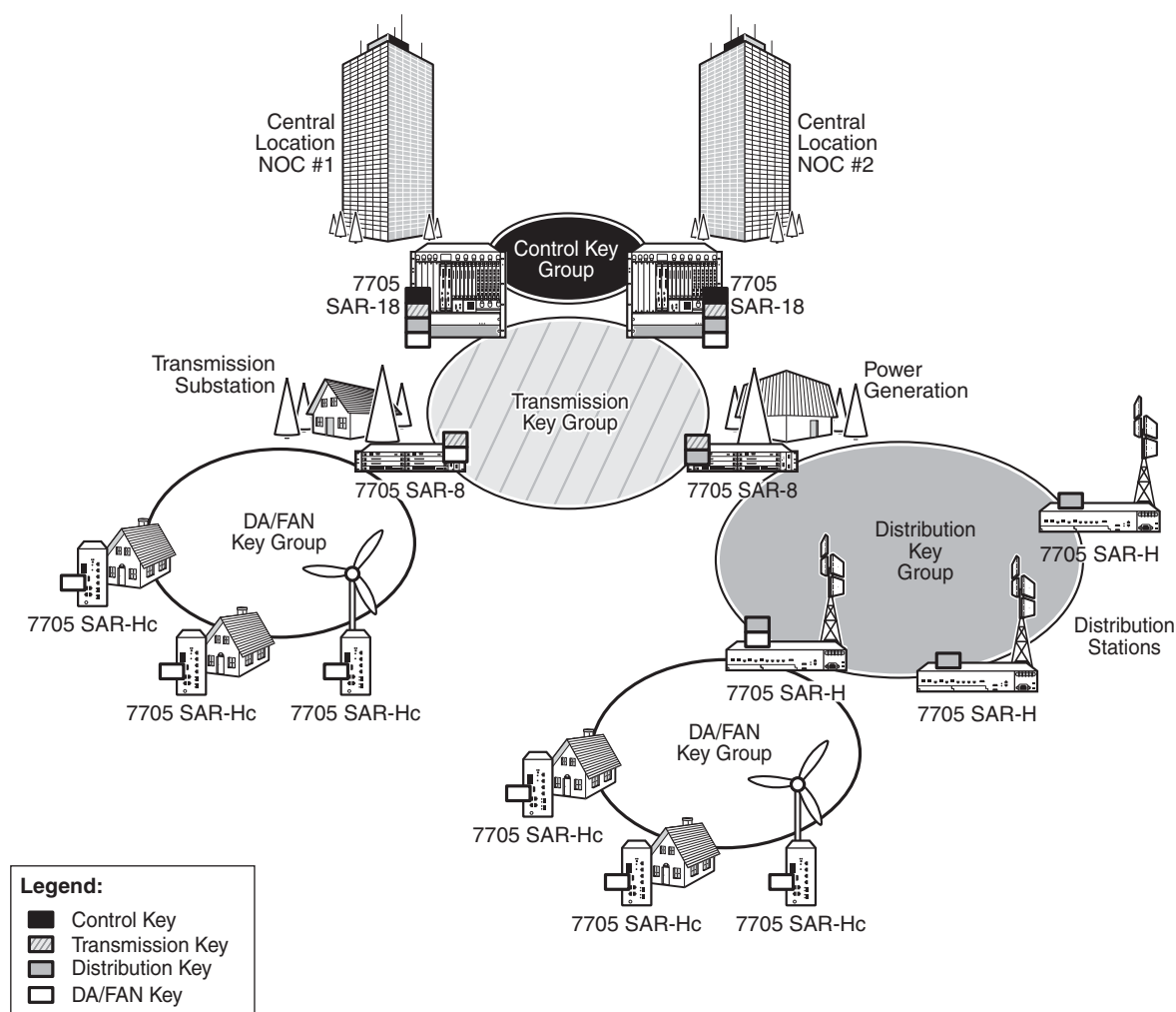
Figure 140 Key-Group Partitioning
