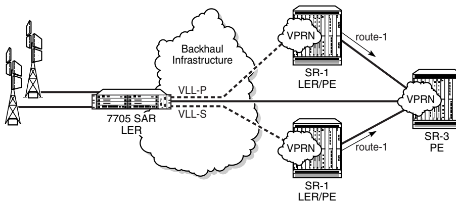
Figure 78 Active/Standby Mode for Redundant Pseudowires
