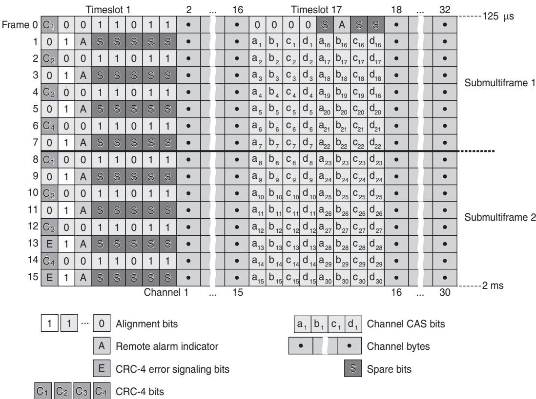
Figure 41 E1 Framing for CAS Support in an E1 Multiframe
