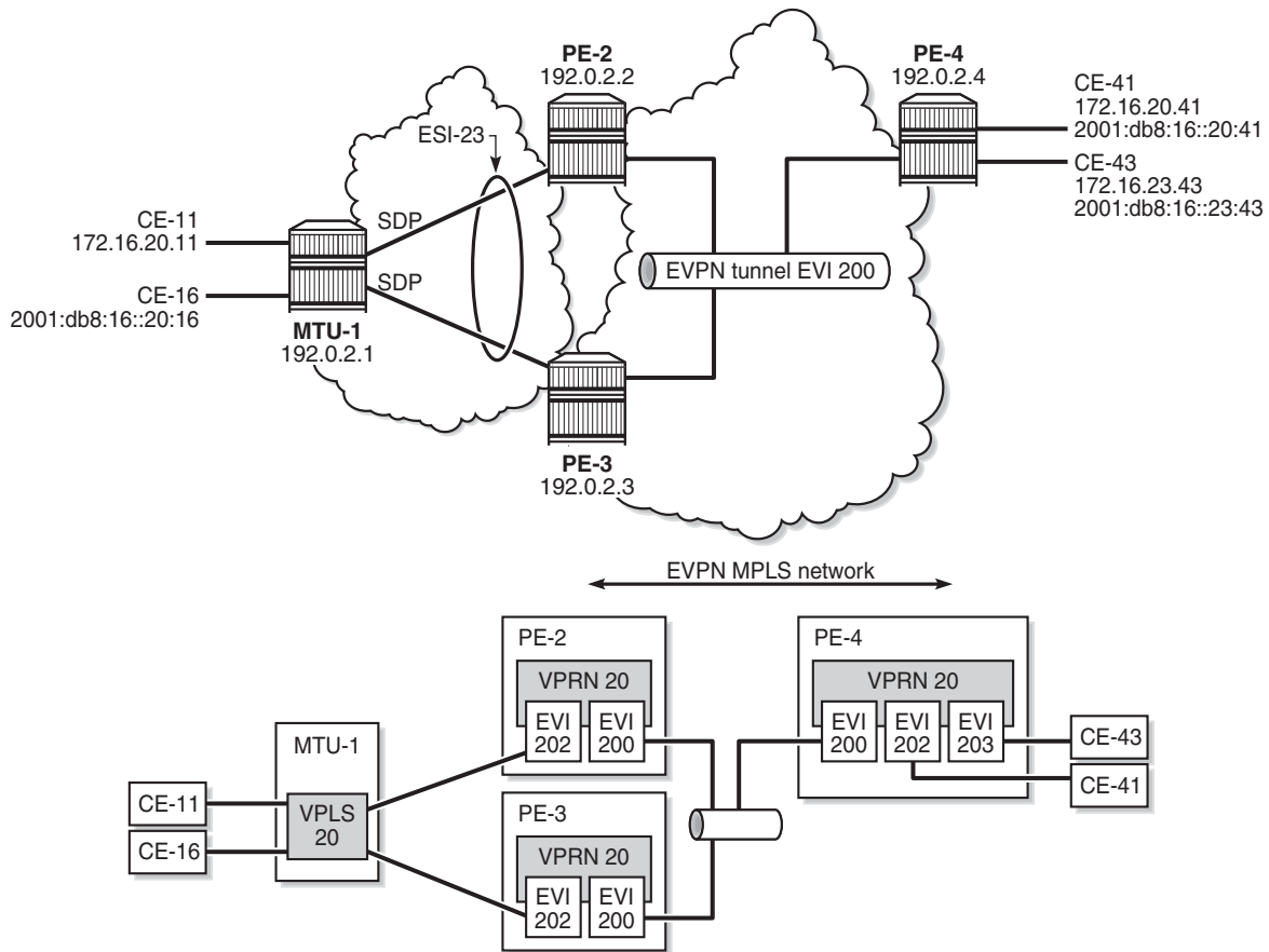
Figure 179 EVPN-MPLS r-VPLS With Single-Active Multihoming
