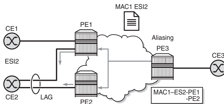
Figure 163 Aliasing
