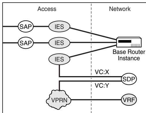
Figure 124 SDP ID and VC Label Service Identifiers (Conceptual View of the Service)
