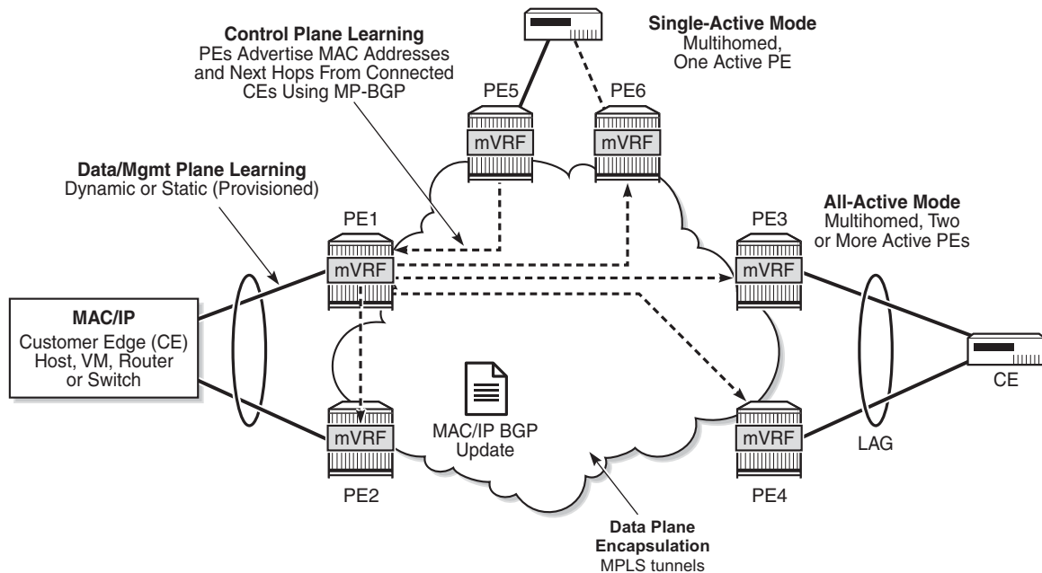
Figure 156 EVPN for MPLS in VPLS Services
