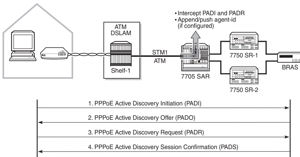
Figure 92 PPPoE Initialization and Agent-Id Push Function
