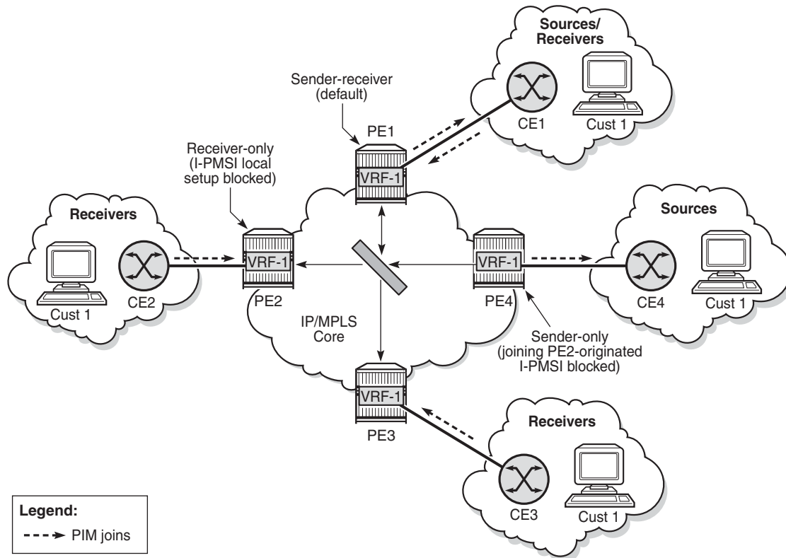
Figure 121 I-PMSI Sender-Receiver, Sender-Only, and Receiver-Only: Optimized I-PMSI Mesh
