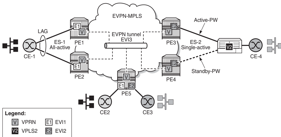
Figure 174 EVPN-MPLS Multi-Homing in r-VPLS Services
