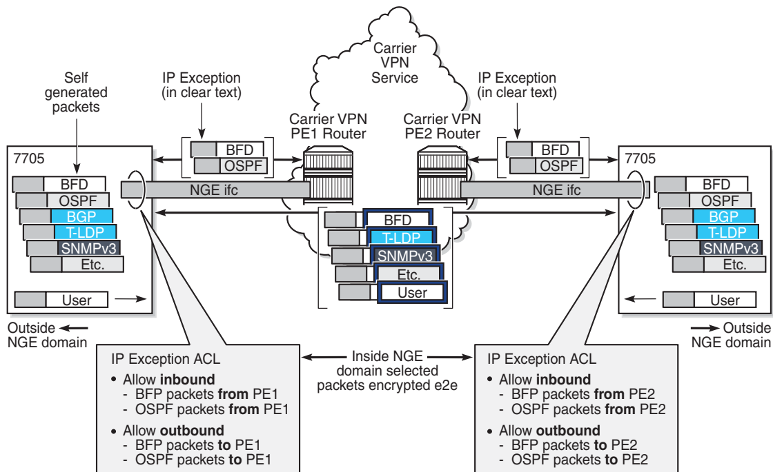
Figure 150 Router Interface NGE Exception Filter Example
