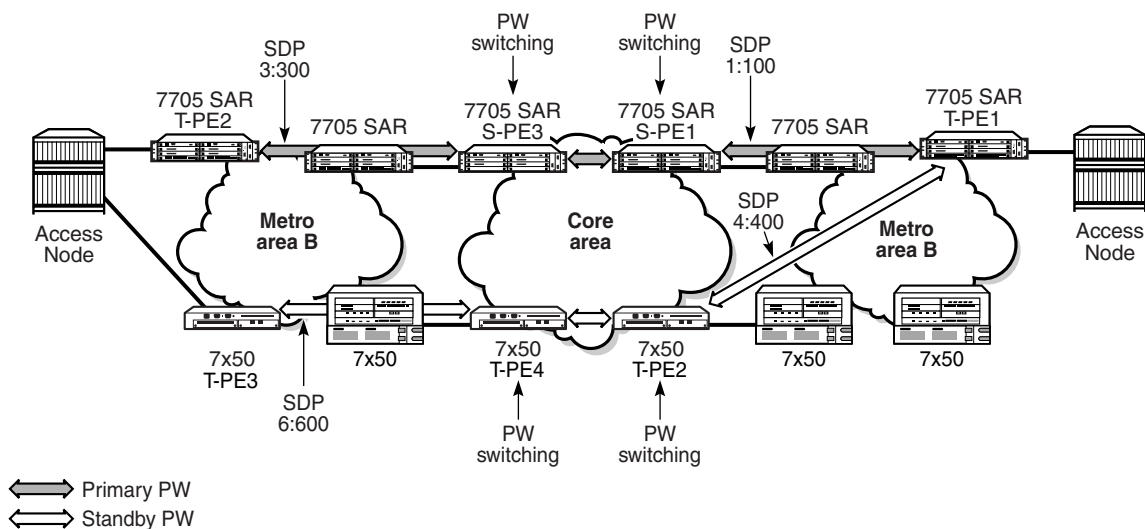
Figure 68 Pseudowire Switching Network
