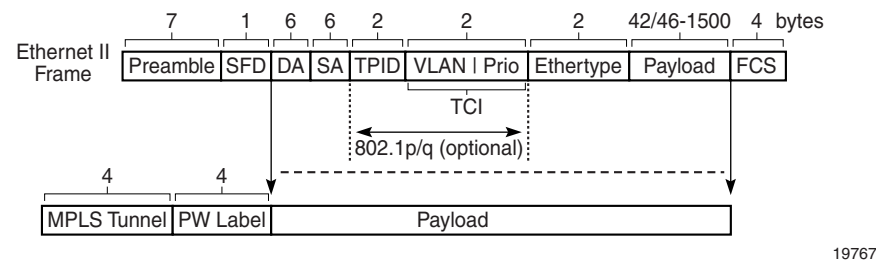
Figure 46 Ethernet VLL Frame with MPLS Encapsulation
