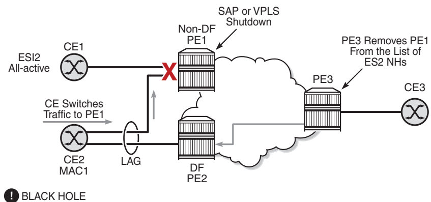
Figure 166 Black Hole Caused by SAP or Service Shutdown
