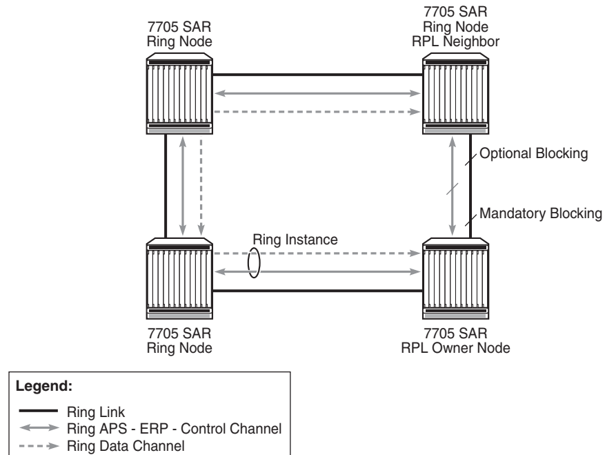
Figure 23 G.8032 Ring in the Idle State
