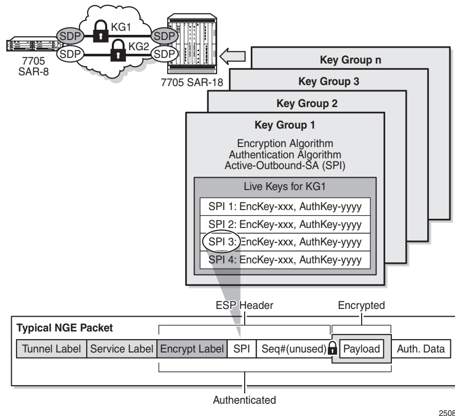
Figure 144 Key Groups and a Typical NGE Packet
