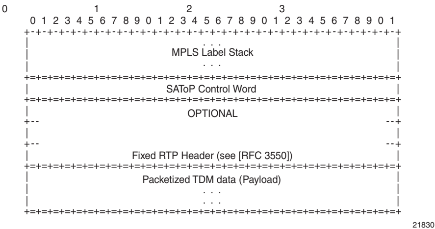
Figure 42 SAToP MPLS Encapsulation
