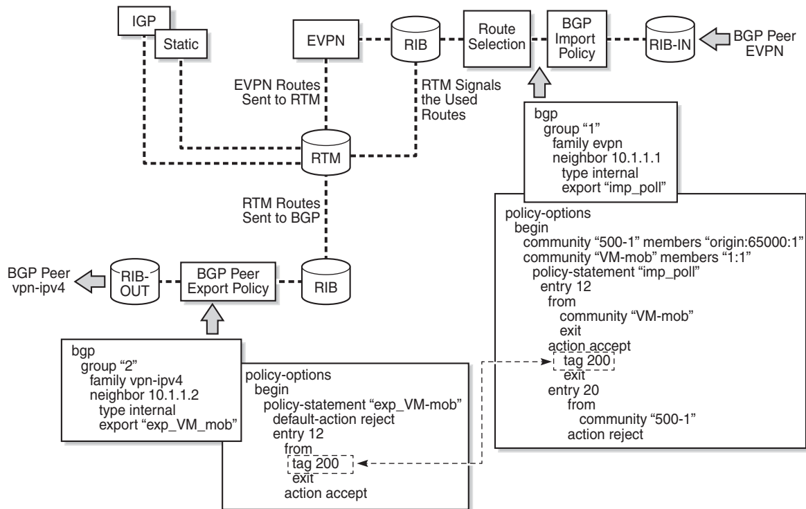
Figure 176 EVPN Import and IP-VPN Export BGP Workflow
