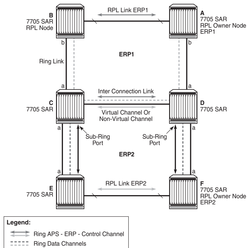
Figure 27 Sub-Ring Configuration Example
