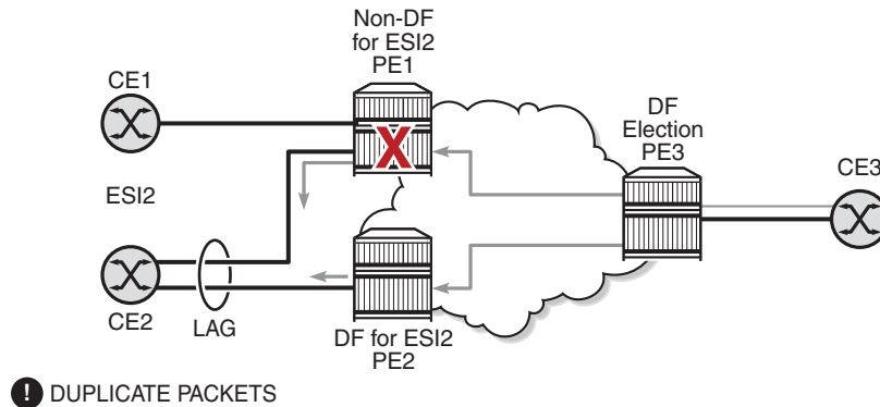
Figure 161 DF Election
