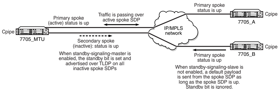
Figure 79 Standby-signaling-master Enabled
