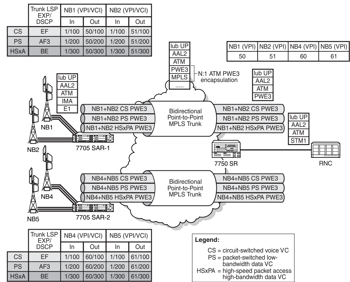
Figure 71 VCC Cell Mode Encapsulation with N > 1
