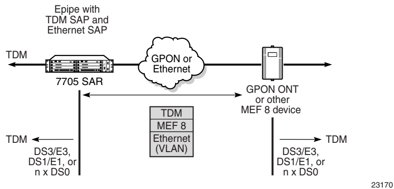
Figure 50 TDM SAP to Ethernet SAP
