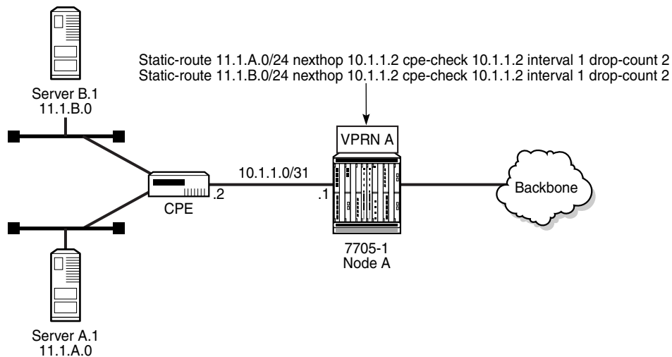
Figure 112 Directly Connected IP Target
