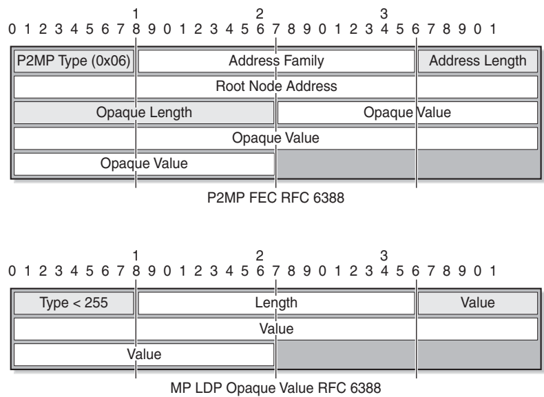
Figure 119 P2MP FEC and MP LDP Opaque Value as per RFC 6388
