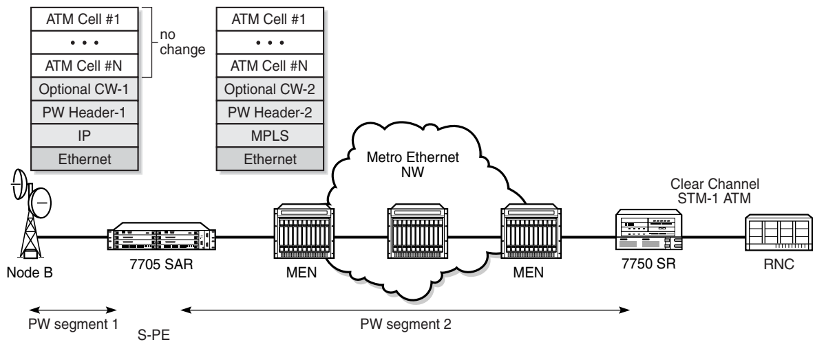
Figure 66 Simplex to Simplex Pseudowire Switching
