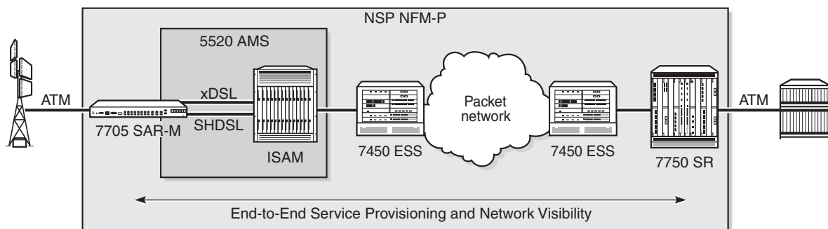
Figure 10 7705 SAR-M With 6-port DSL Combination Module for HSDPA Offload
