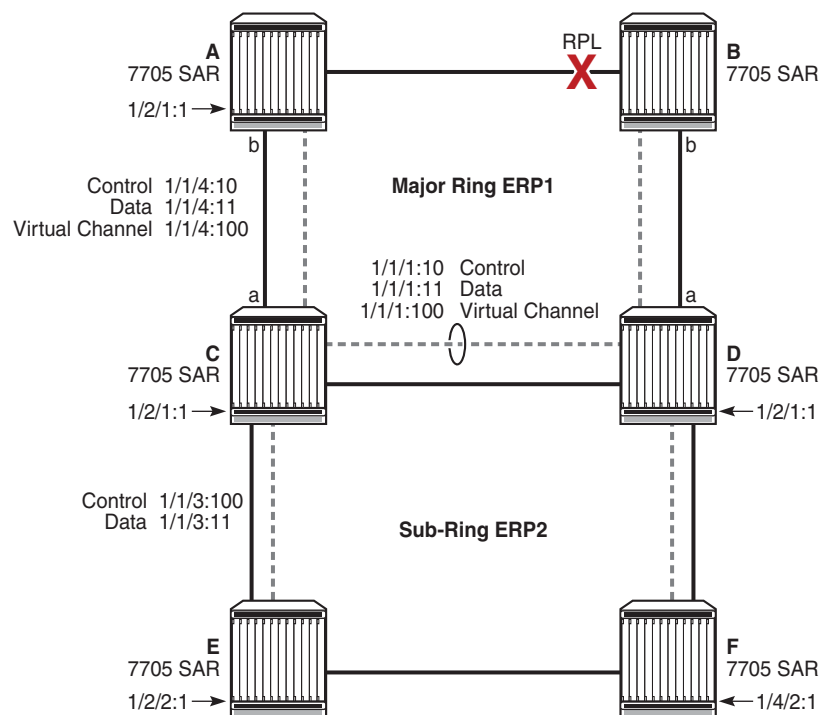
Figure 28 Sub-Ring Homed to VPLS
