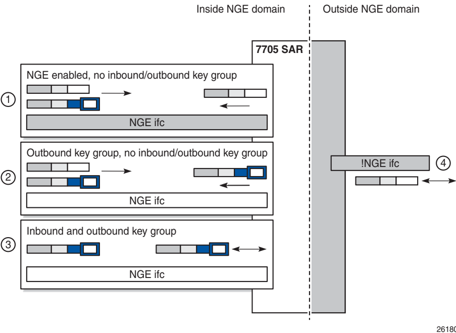
Figure 149 Inside and Outside NGE Domains
