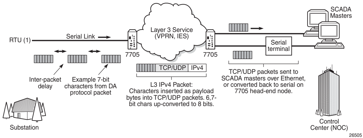
Figure 35 TCP/UDP Packet Transport Over IP/MPLS
