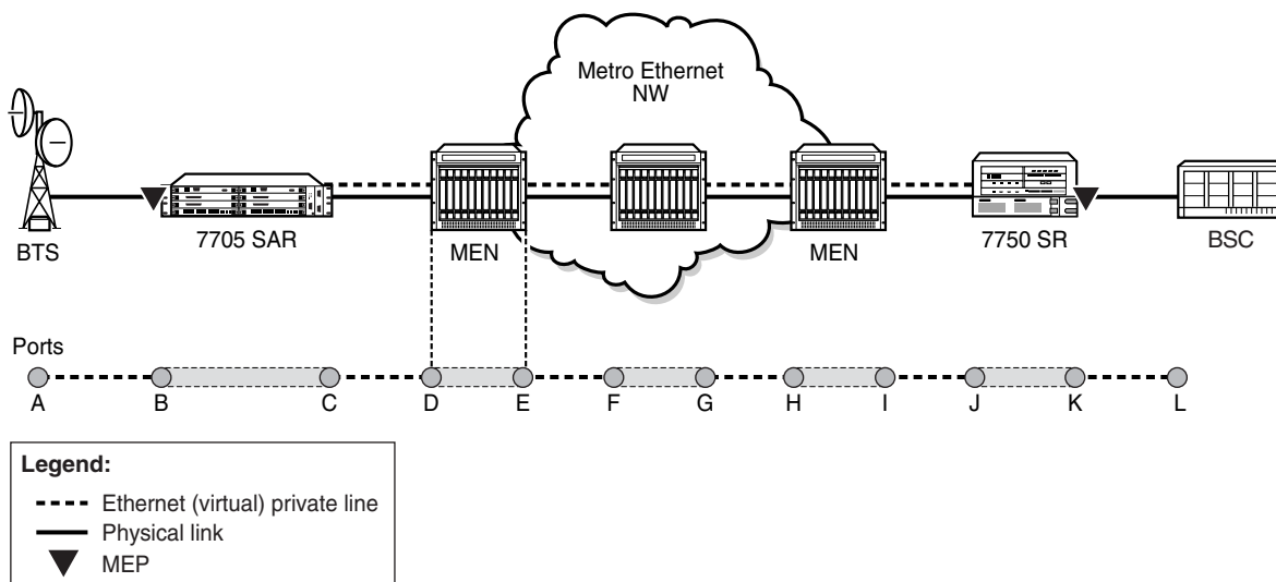
Figure 18 MEP on Ethernet Access
