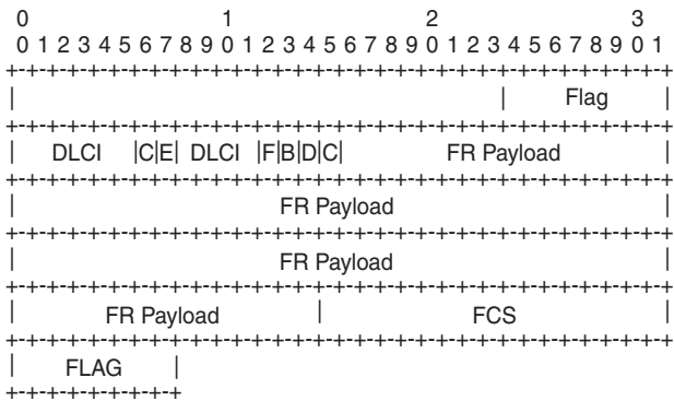
Figure 54 FR Frame
