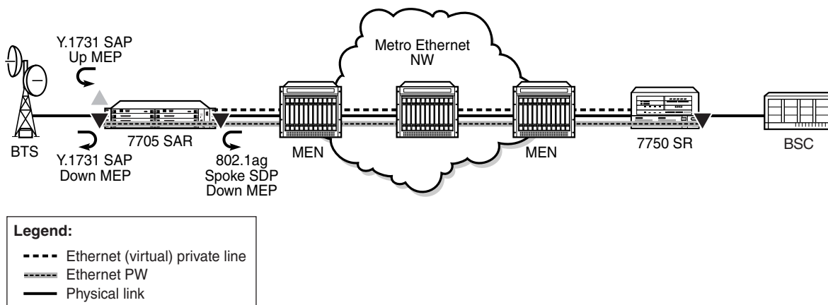
Figure 21 Y.1731 MEP Support on the 7705 SAR
