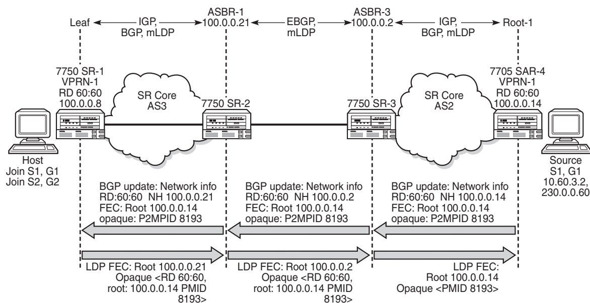
Figure 122 Inter-AS Option B: Non-Segmented Solution
