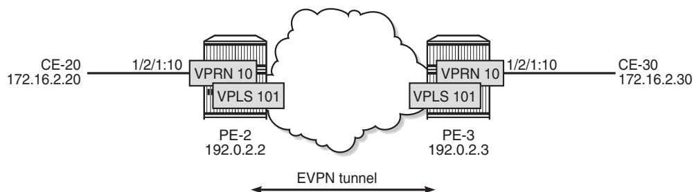
Figure 177 r-VPLS With EVPN Tunnel, Without Multihoming
