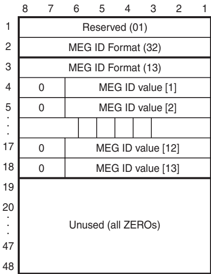
Figure 16 ICC-based MEG-ID Format
