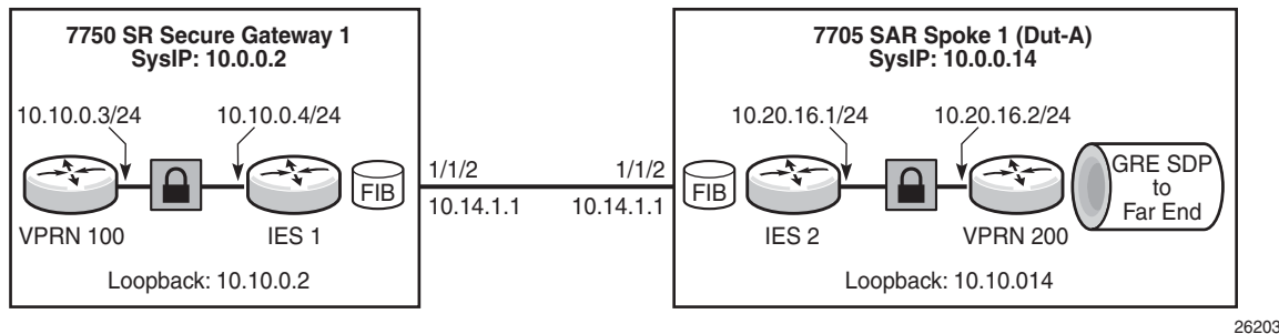
Figure 134 VLL/VPLS over IPSec over MPLS using a Loopback Address
