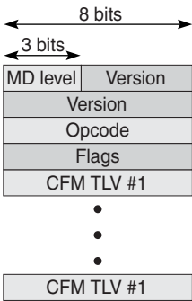
Figure 15 ETH-CFM OAMPDU Message
