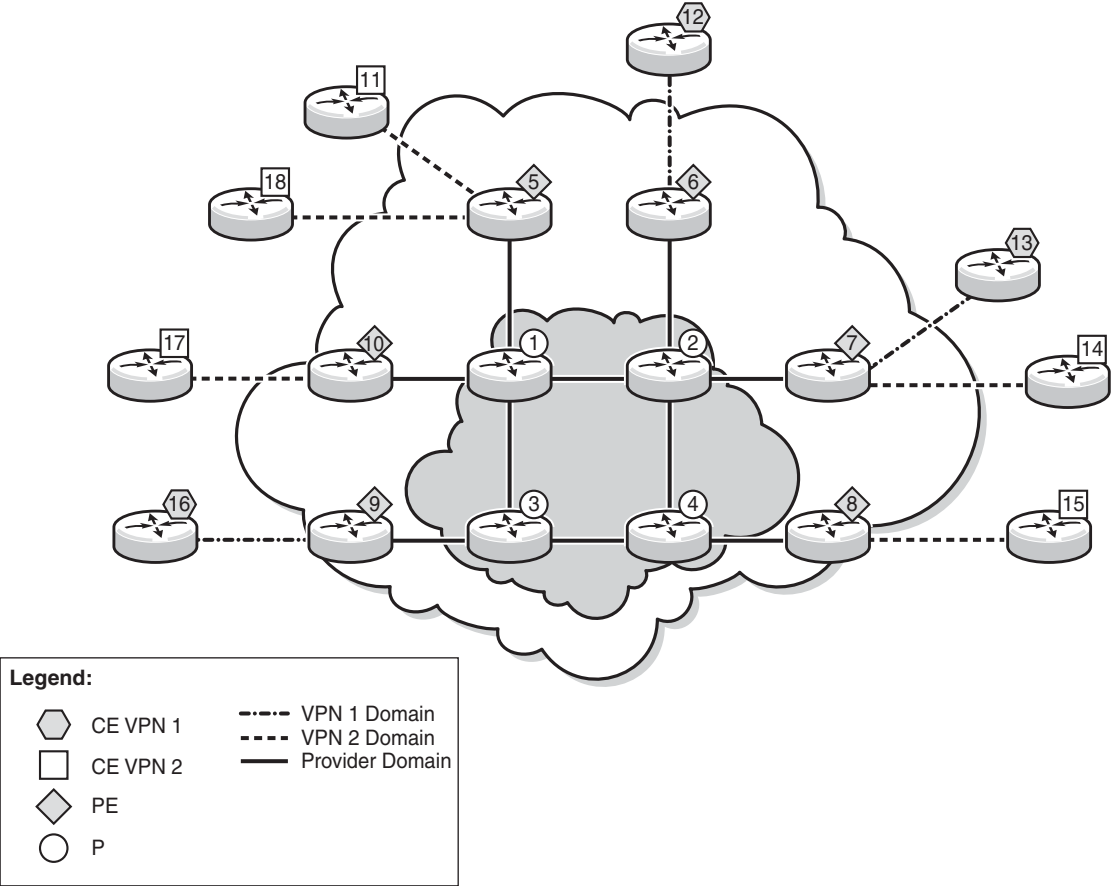
Figure 117 Multicast in an IP-VPN Application
