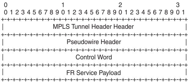
Figure 55 FR PW 1-to-1 MPLS PSN Encapsulation
