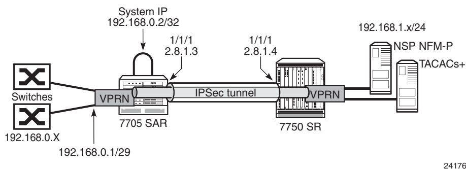
Figure 114 IPv4 In-Band Management Using a VPRN Configured with GRT Lookup
