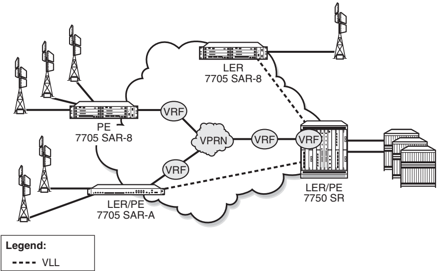
Figure 127 VPRN in Mobile Backhaul Application
