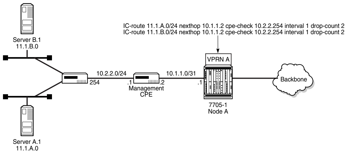
Figure 113 Multiple Hops to IP Target
