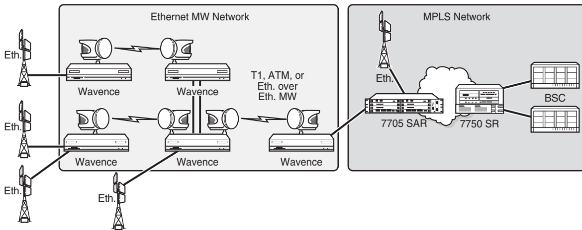
Figure 19 Down MEP at Ethernet SAP
