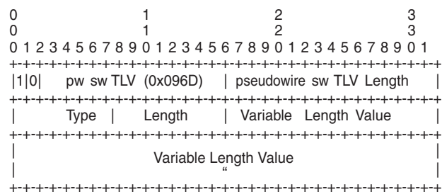
Figure 69 Pseudowire Switching TLV
