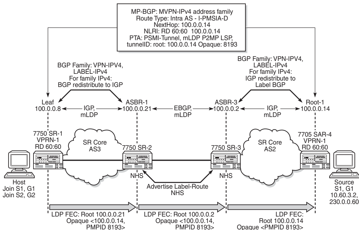
Figure 123 Inter-AS Option C: Non-Segmented Solution
