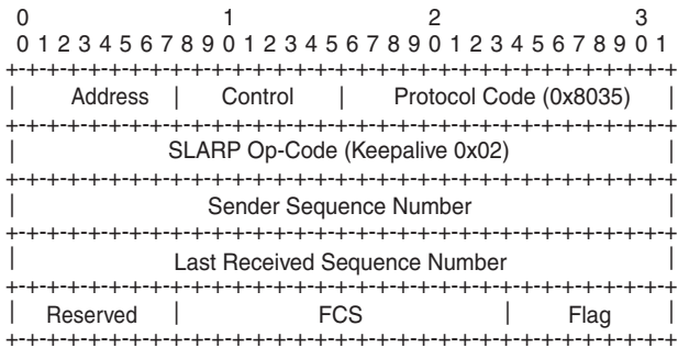
Figure 64 SLARP Keepalive Frame
