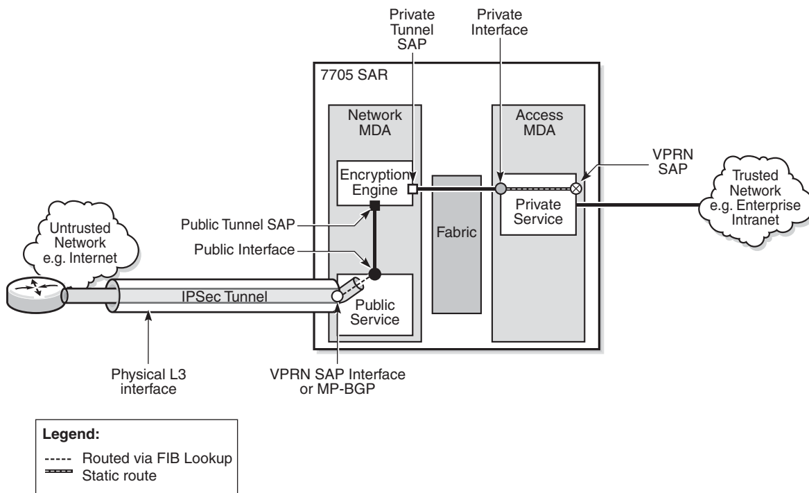
Figure 131 VPRN Public Service IPSec Transport Tunnels
