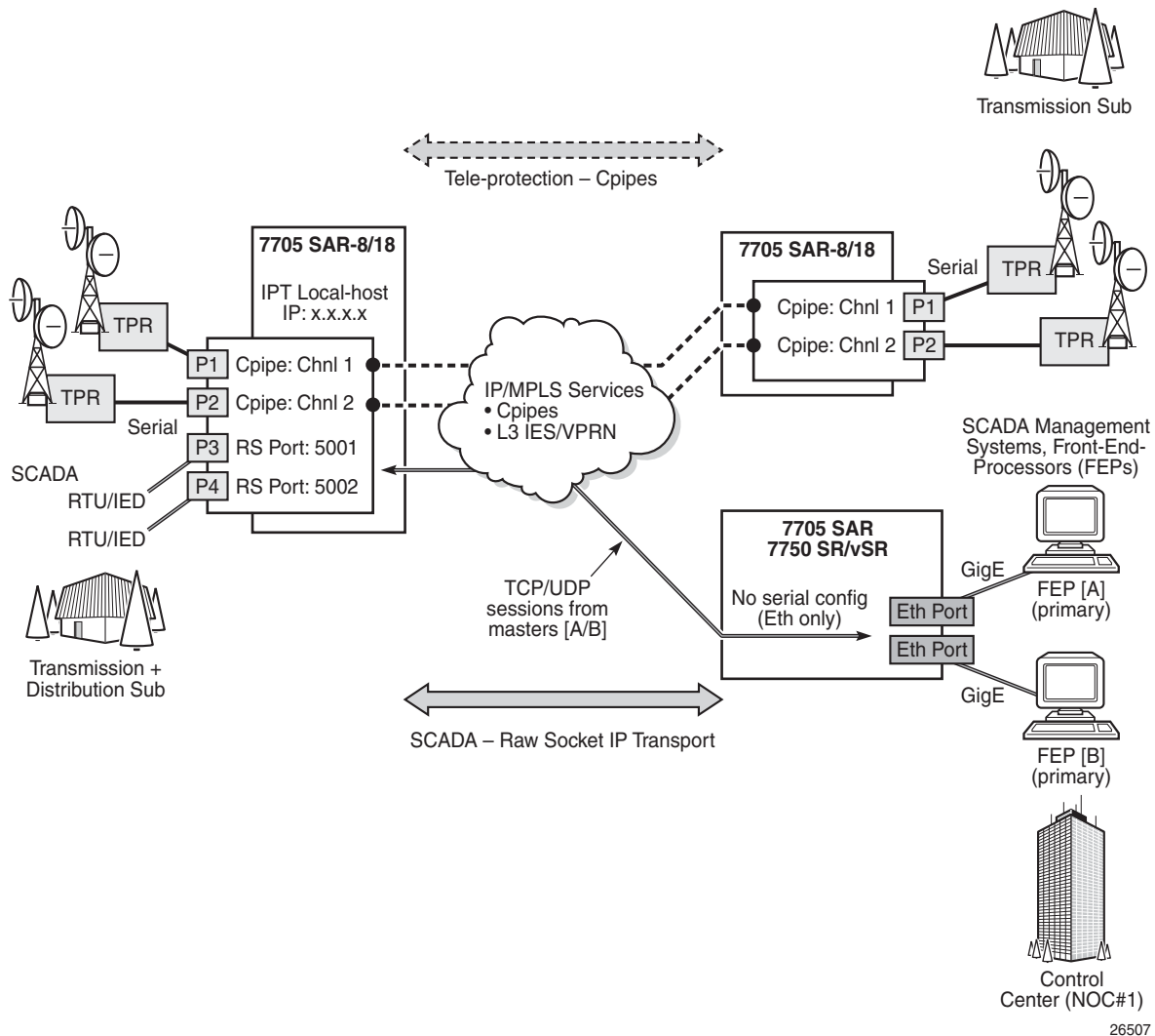
Figure 37 Raw Socket and Cpipe Support on the 7705 SAR
