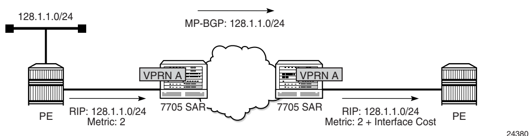
Figure 116 RIP Metric Propagation in VPRNs
