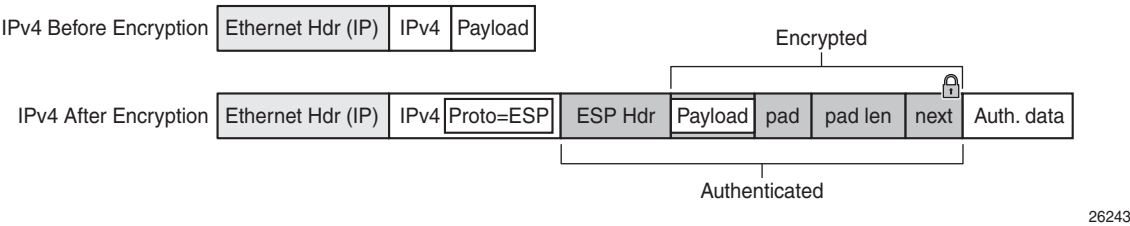
Figure 148 Router Interface Encryption Packet Format (IPsec Transport Mode)
