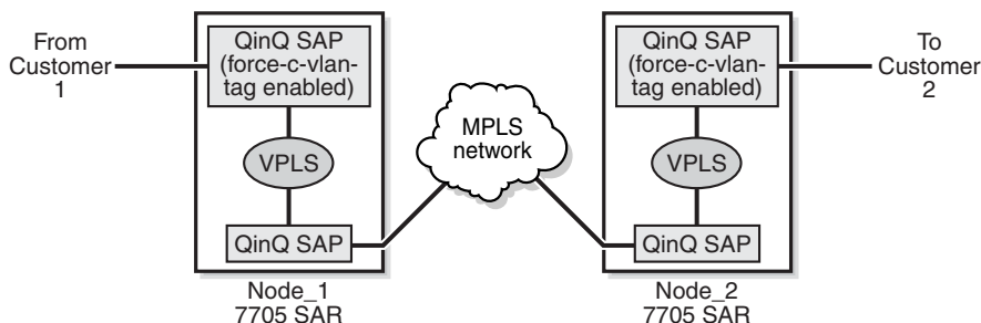
Figure 32 QinQ Using VPLS Ethernet SAPs
