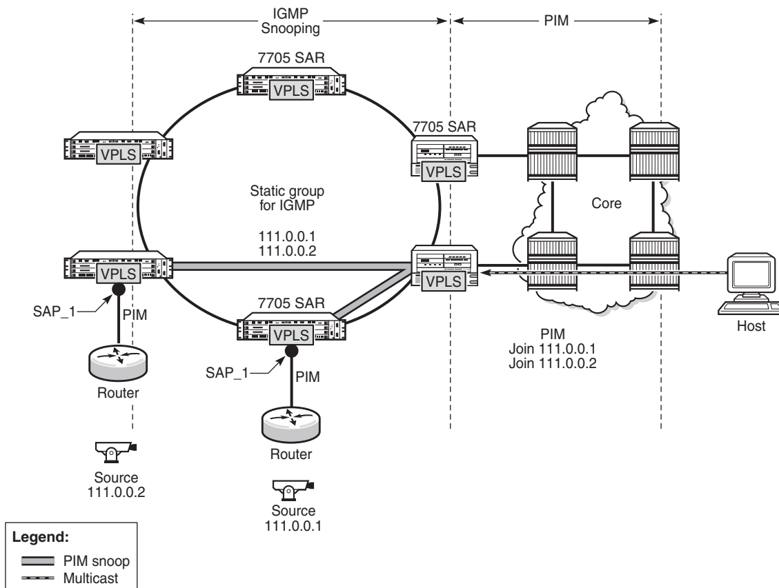
Figure 98 PIM Snooping Example
