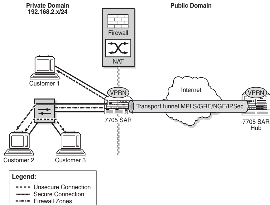
Figure 110 Firewall Protection for the Network Core
