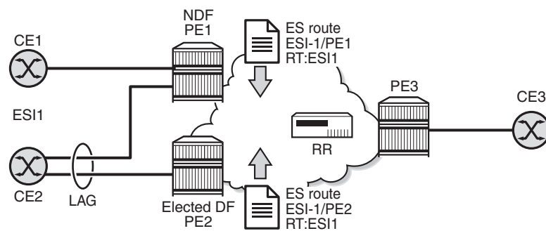
Figure 164 ES Discovery and DF Election
