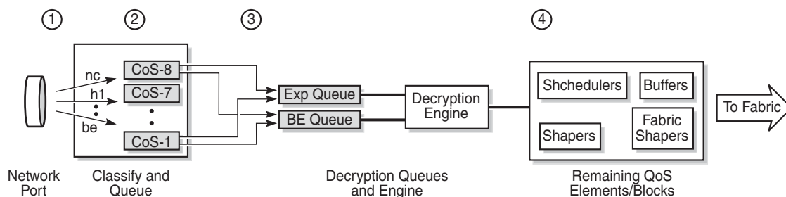
Figure 155 QoS for NGE Traffic (Network Ingress)
