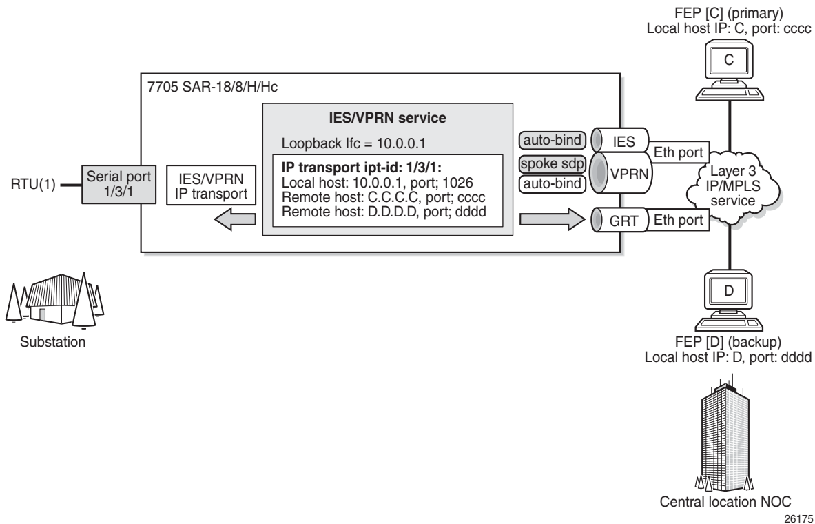
Figure 36 IES/VRN IP Transport Service
