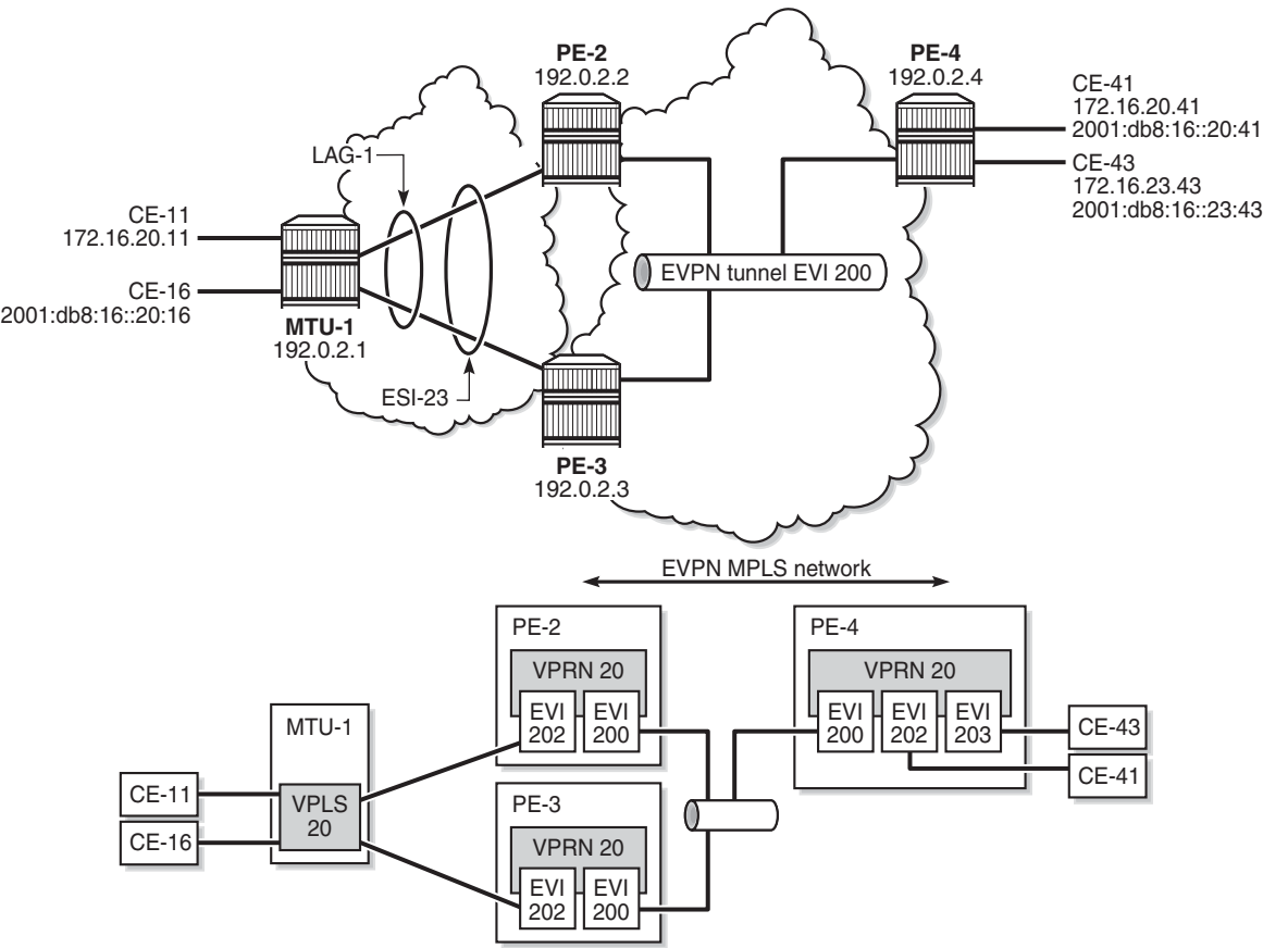
Figure 178 EVPN-MPLS r-VPLS With All-Active Multihoming ES
