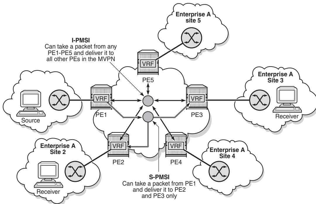
Figure 118 I-PMSI and S-PMSI
