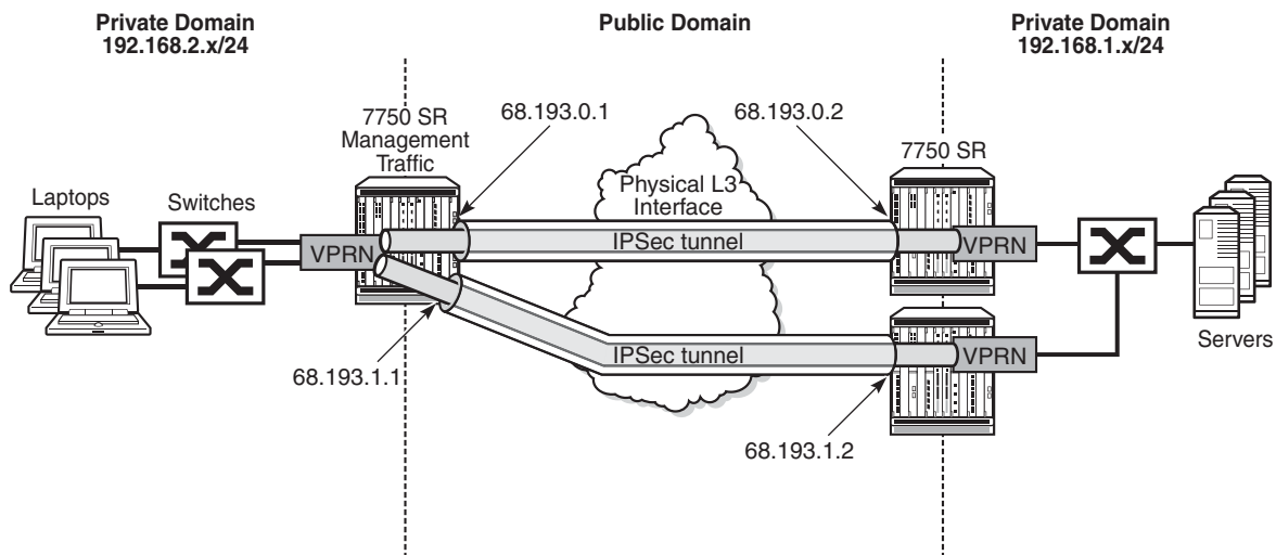
Figure 136 Typical Small Business Deployment
