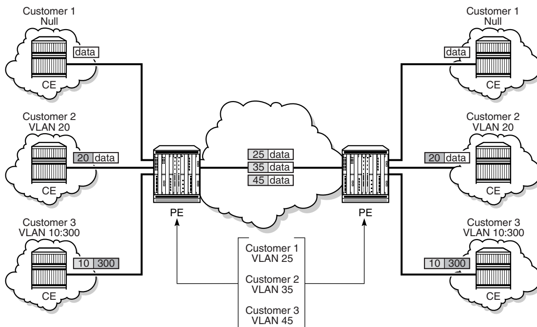
Figure 31 QinQ Tagging Example
