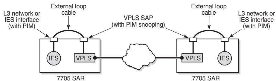
Figure 99 Simulating r-VPLS
