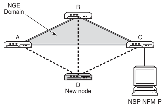
Figure 142 Private IP/MPLS Network NGE Domain
