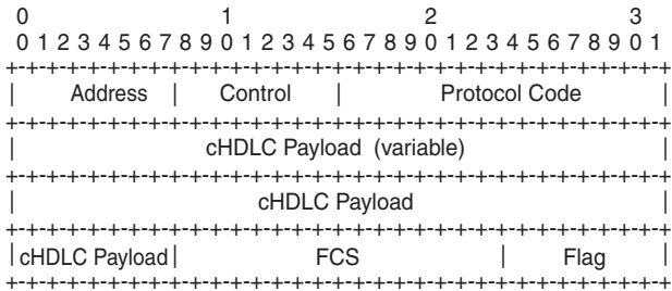
Figure 63 cHDLC Header Frame
