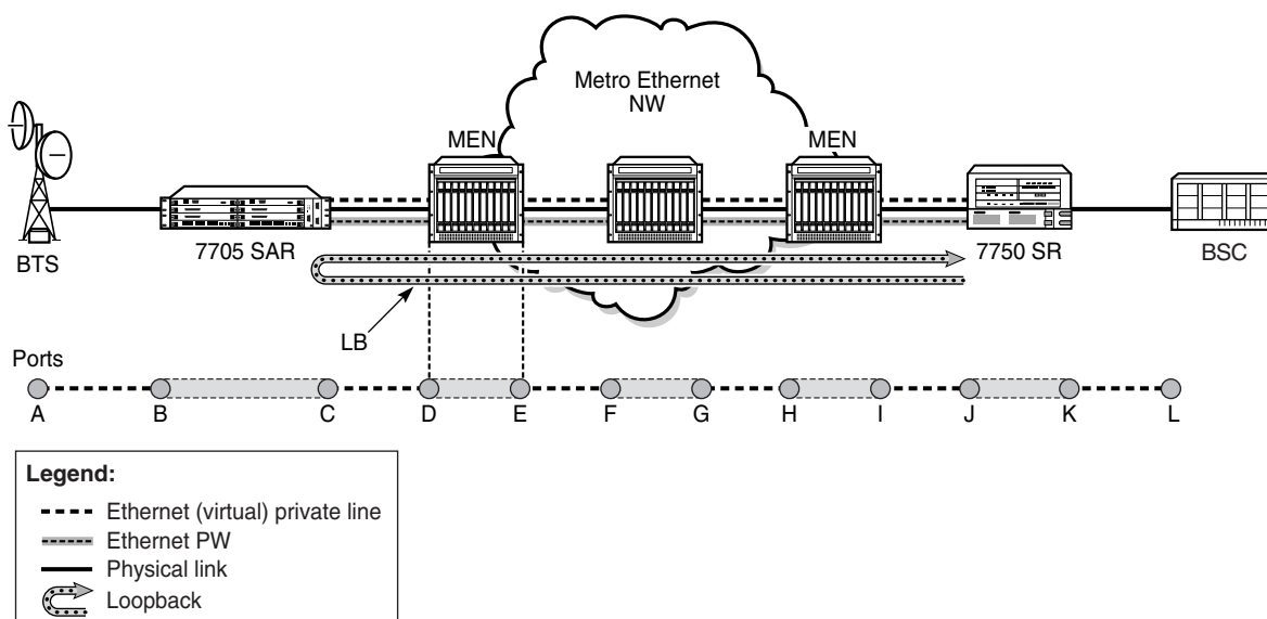
Figure 17 Dot1ag Loopback Test
