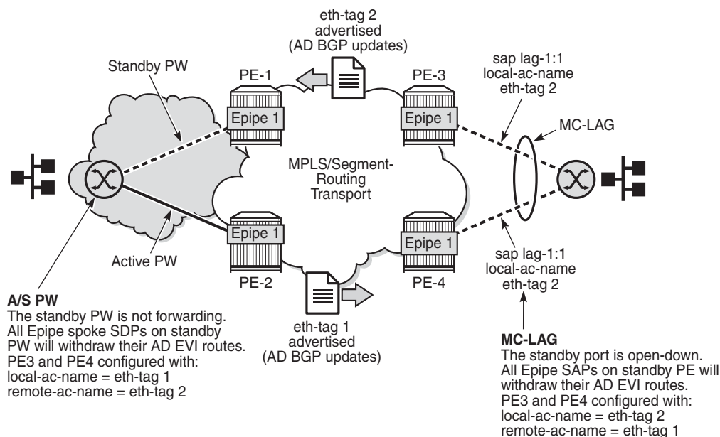
Figure 172 A/S PW and MC-LAG Support on EVPN-VPWS
