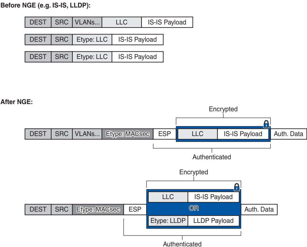
Figure 154 Encrypted Layer 2 Packet
