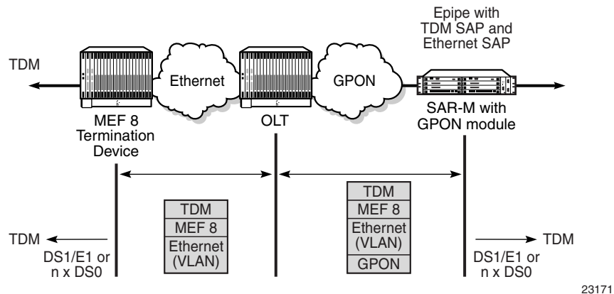
Figure 51 TDM SAP to Ethernet SAP via 7705 SAR-M GPON Module
