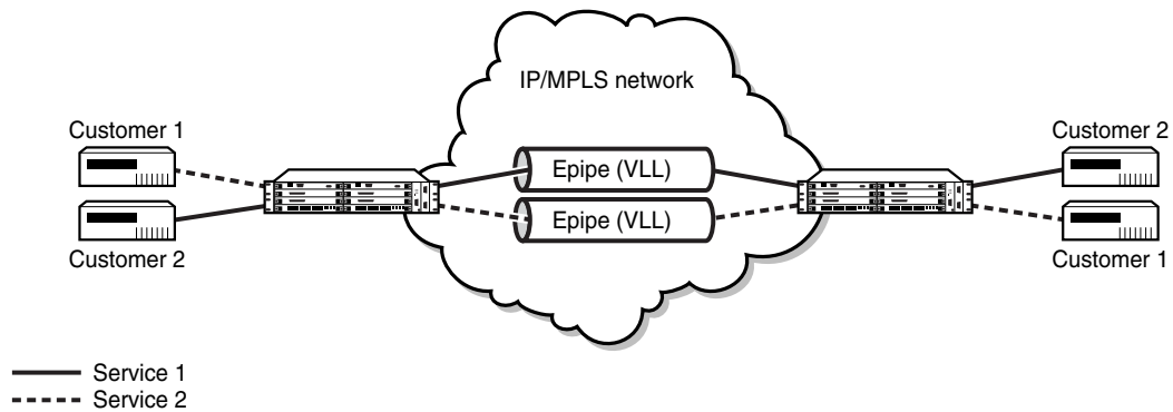
Figure 47 Epipe Service
