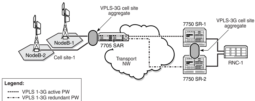
Figure 89 Local VPLS on 7705 SAR in Mobile Backhaul
