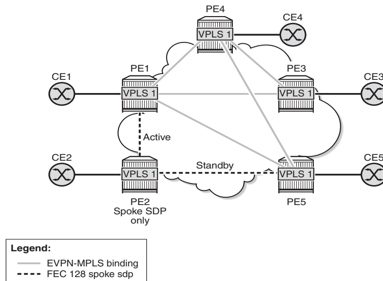
Figure 160 EVPN-VPLS Integration
