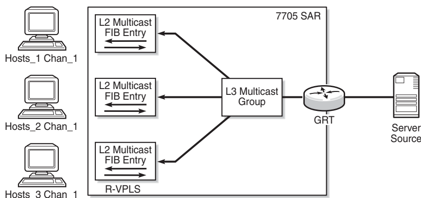
Figure 96 Multiple Hosts in an r-VPLS Receiving the Same Channel
