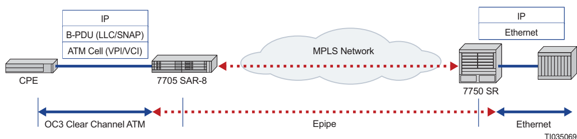
Figure 48 Epipe Network Configuration with ATM SAP
