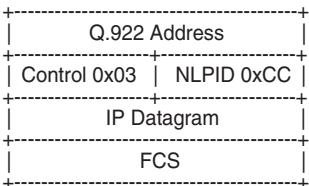
Figure 62 FR Header with NLPID Support for IP Interworking PW
