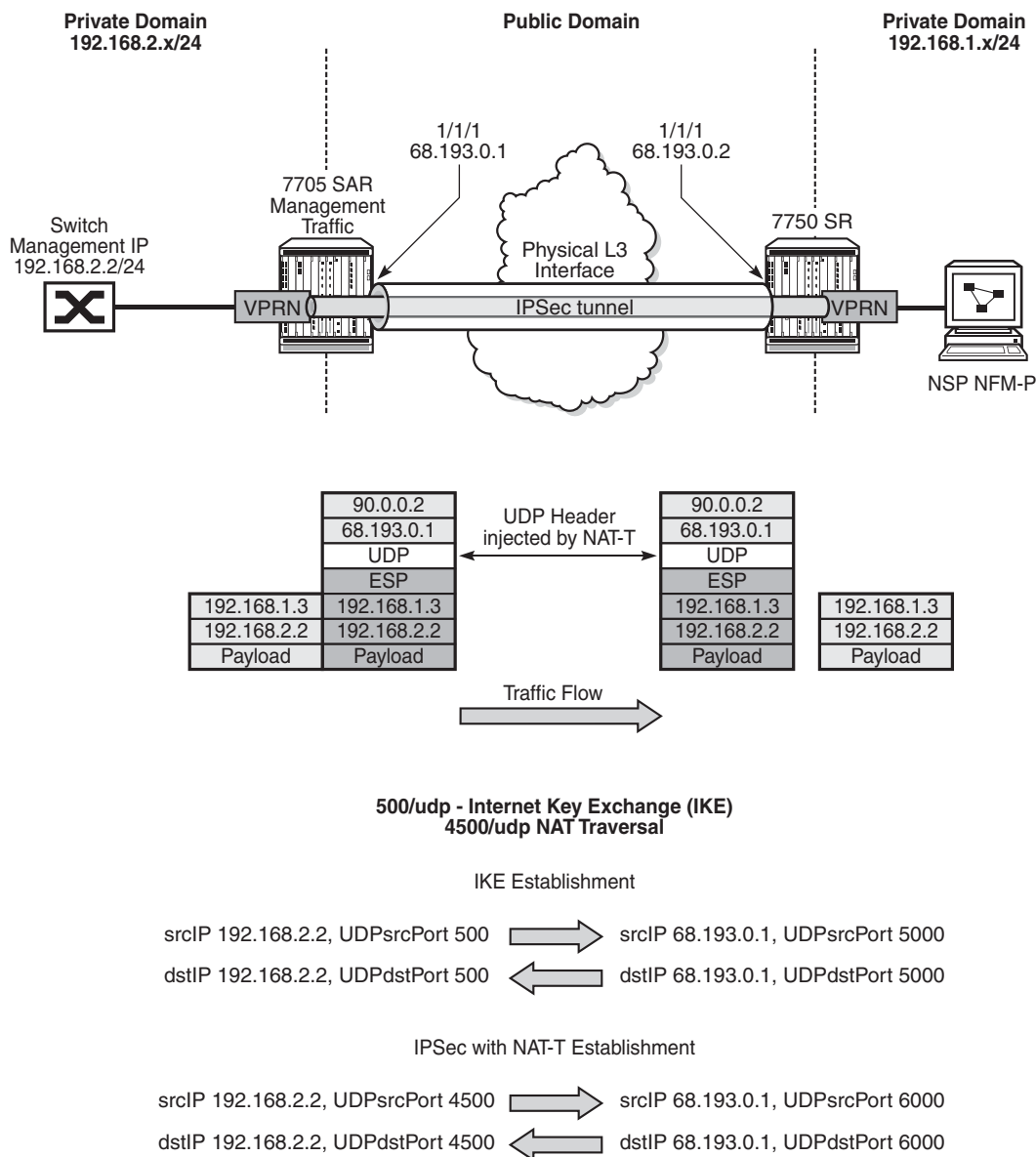
Figure 137 UDP Header Injected by a NAT-T-enabled IPSec Tunnel
