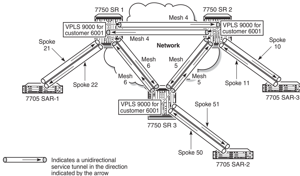
Figure 104 SDPs—Unidirectional Tunnels
