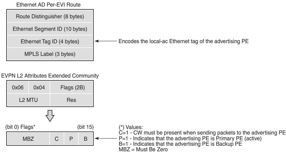
Figure 170 EVPN-VPWS BGP Extensions
