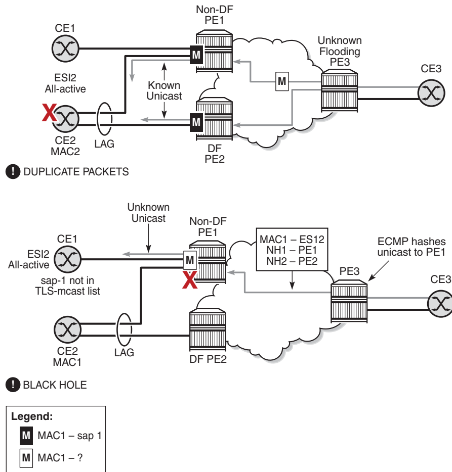
Figure 167 Transient Issues Caused by Slow MAC Learning
