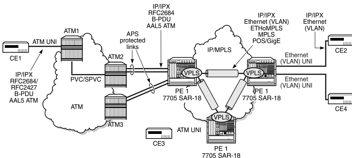
Figure 103 Example of ATM PVC Access and Termination on a VPLS
