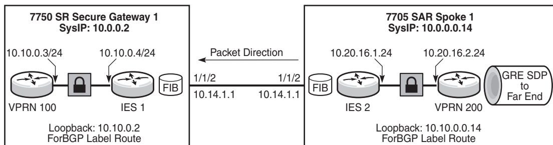
Figure 133 VLL/VPLS over IPSec over MPLS Using BGP 3107 Label Routes
