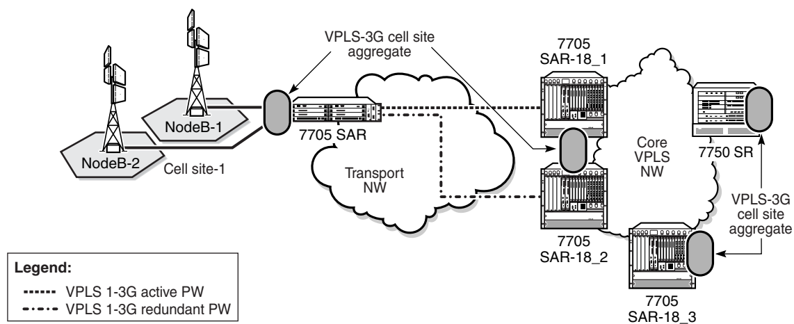
Figure 90 Spoke-SDP Termination to VPLS using 7705 SAR-18 Routers
