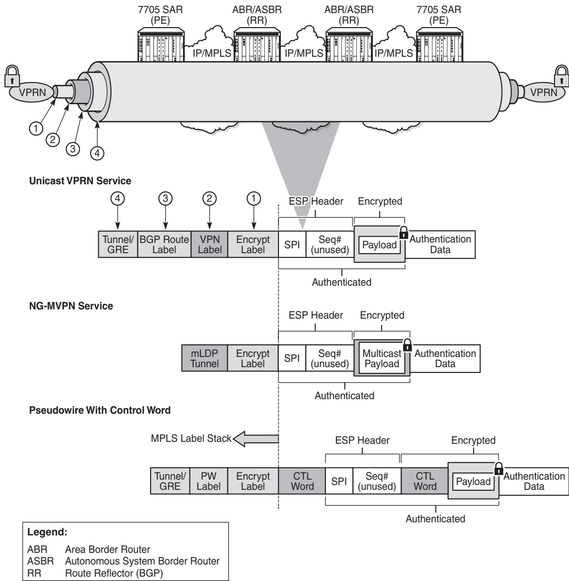
Figure 146 NGE Encryption and Packet Formats
