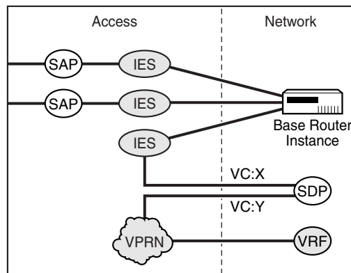
Figure 106 SDP ID and VC Label Service Identifiers (Conceptual View of the Service)
