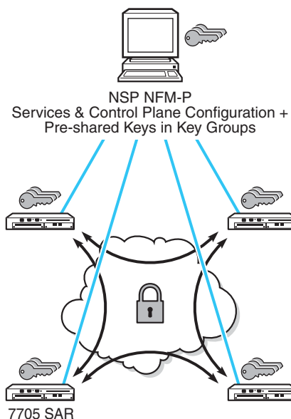
Figure 139 NGE Network with NSP NFM-P Management
