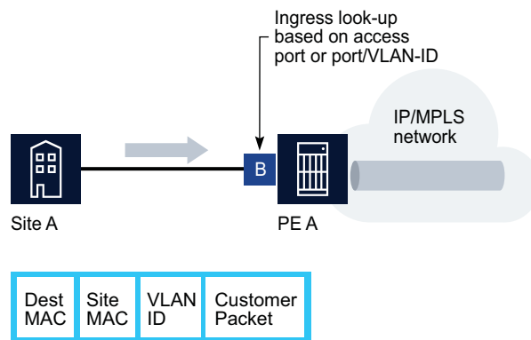
Figure 85 Access Port Ingress Packet Format and Lookup
