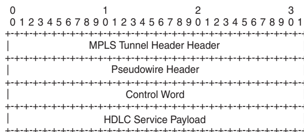
Figure 59 HDLC VLL Frame with MPLS Encapsulation
