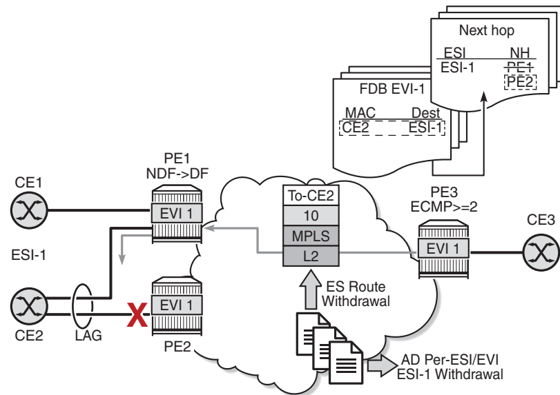
Figure 165 All-Active Multihoming ES Failure
