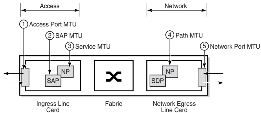
Figure 72 MTU Points on the 7705 SAR
