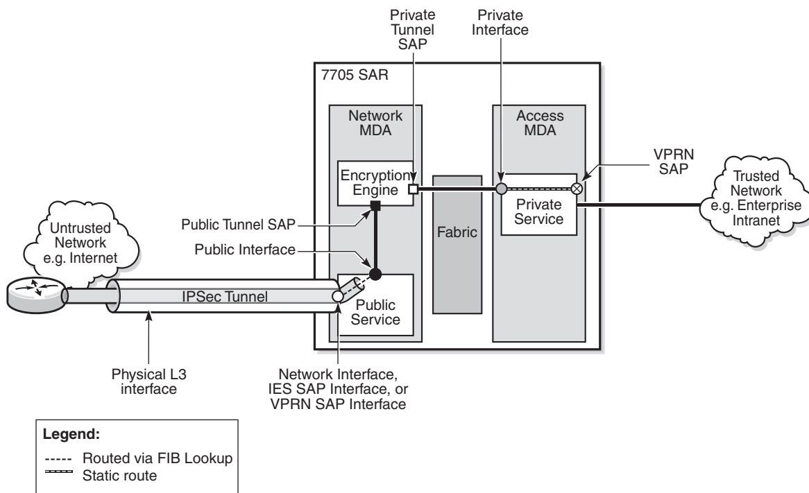
Figure 130 IPSec Implementation Architecture
