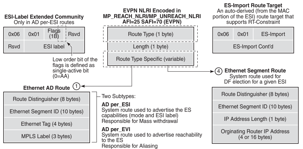
Figure 158 EVPN Route Type 1 and Type 4
