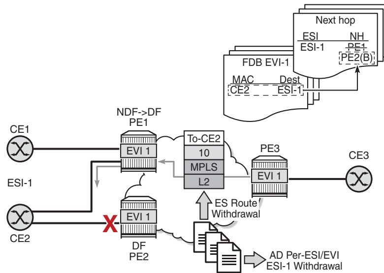
Figure 169 Single-Active Multihoming ES Failure
