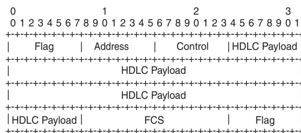
Figure 58 HDLC VLL Frame
