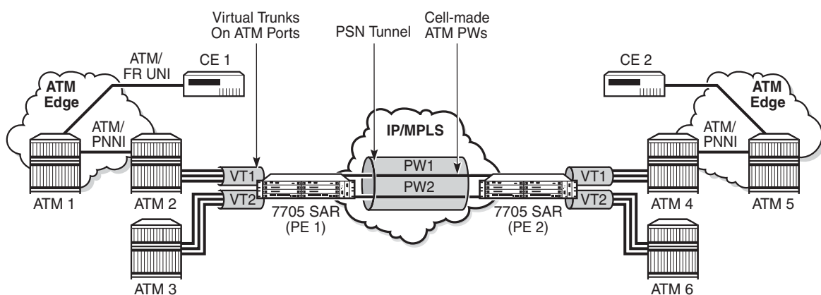
Figure 40 ATM Virtual Trunk Over IP/ MPLS Packet-Switched Network
