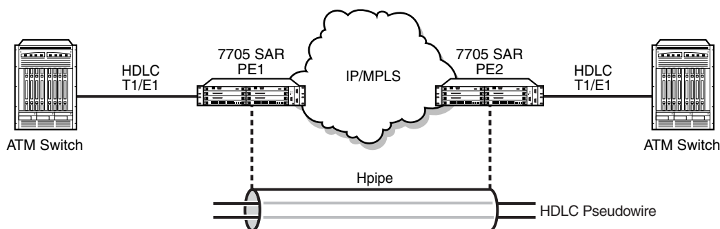
Figure 57 HDLC VLL for End-to-End HDLC Service
