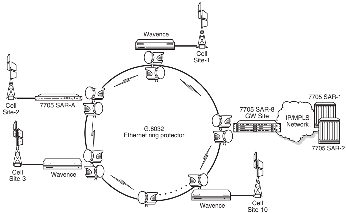
Figure 22 Ethernet Protection Switching
