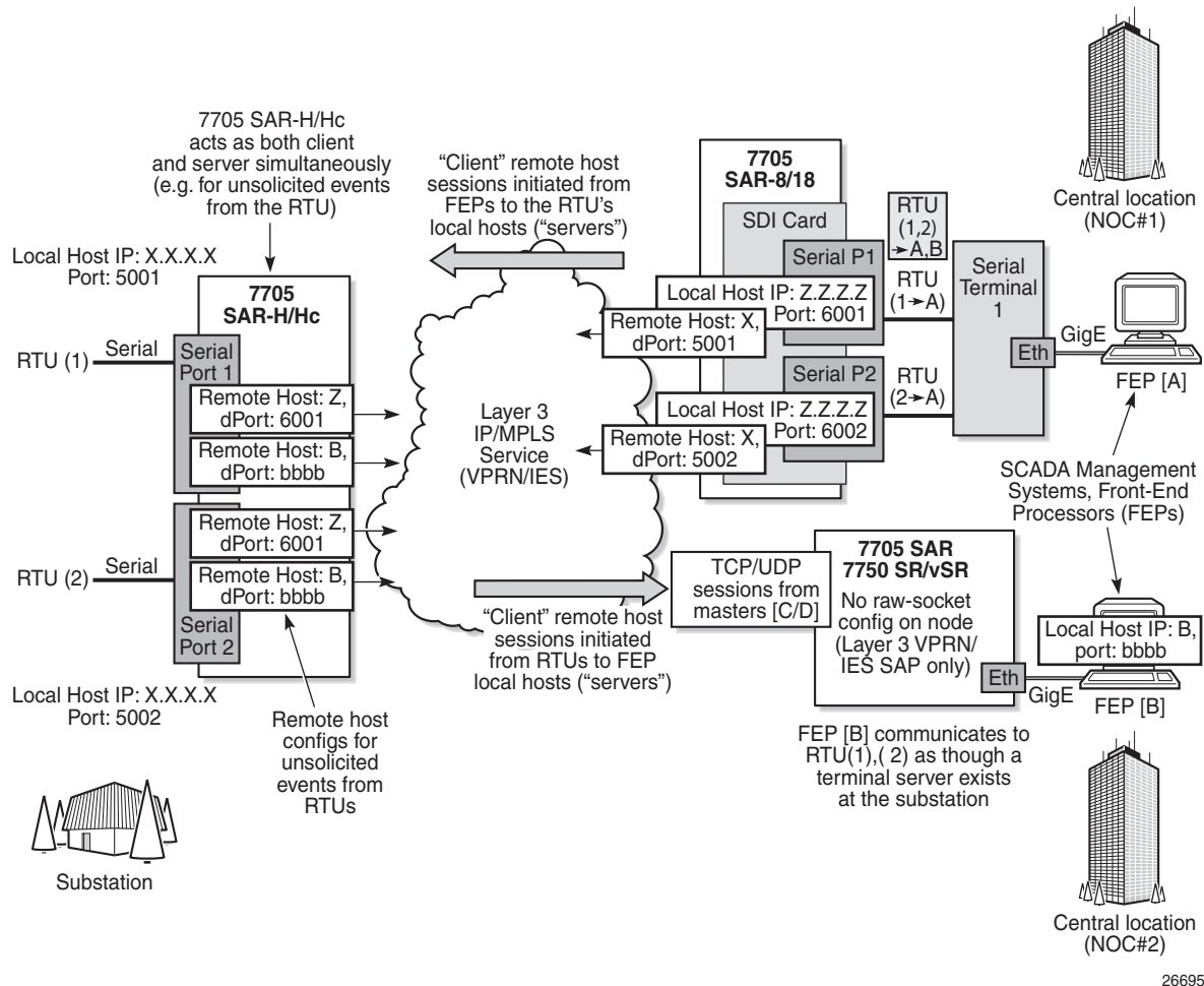
Figure 34 IP Transport Service
