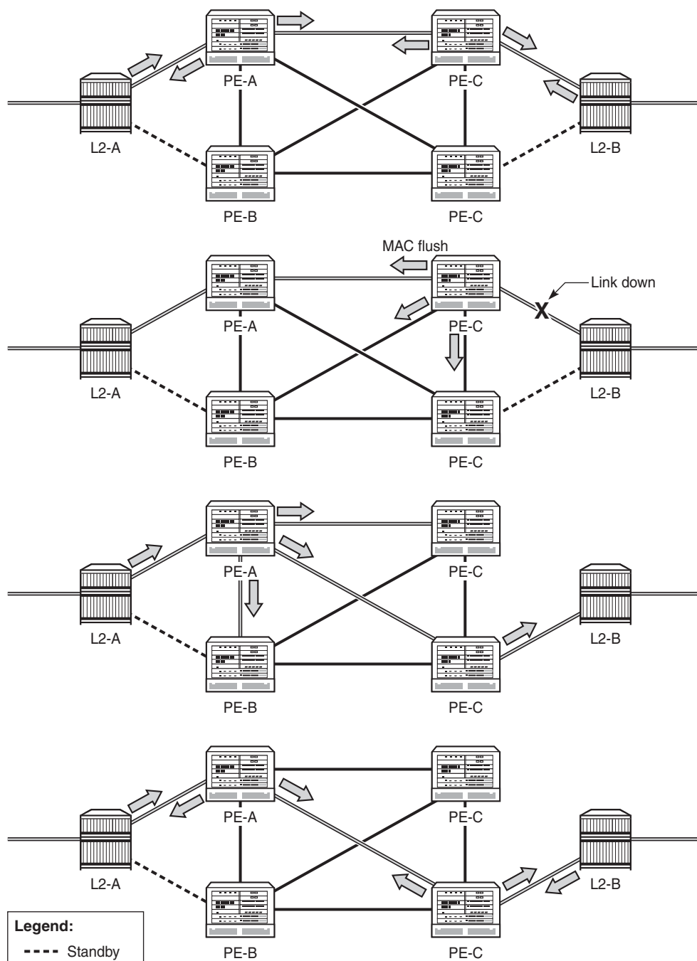
Figure 102 Dual-Homed CE Connection to VPLS
