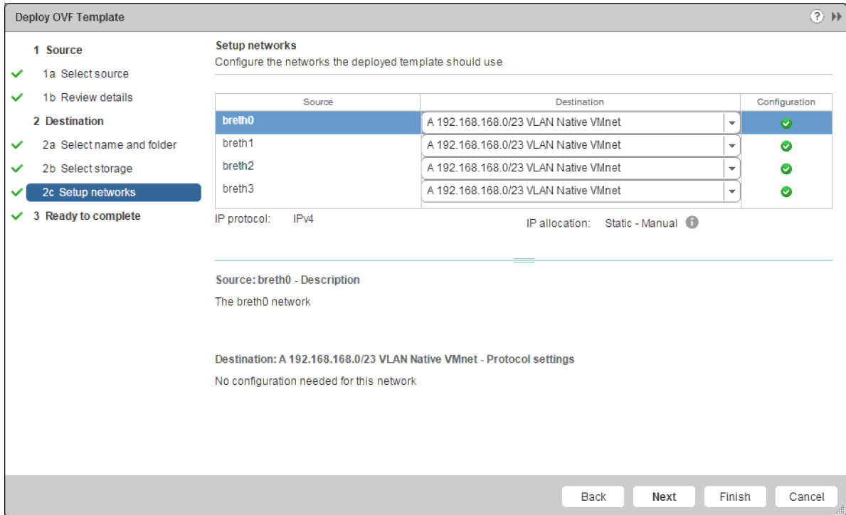
Figure 10: Configure the Network Interfaces
