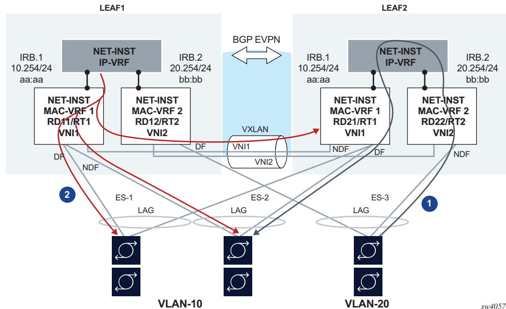
Figure 9 EVPN-VXLAN L3 model – multi-homing and anycast GW
