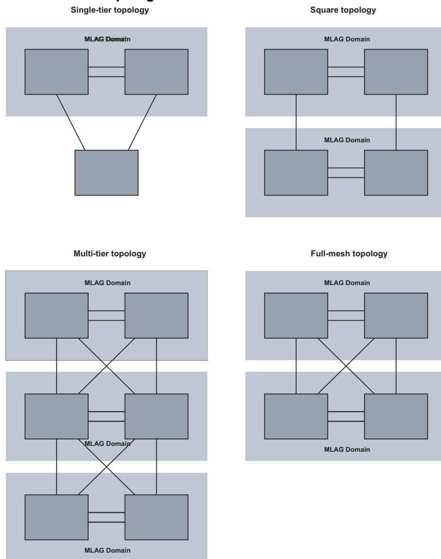
Figure 14 MLAG topologies
