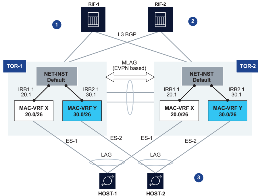
Figure 11 Active-active connectivity example
