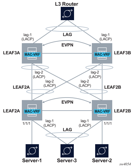
Figure 13 EVPN Multi-Homing as standalone MC-LAG solution
