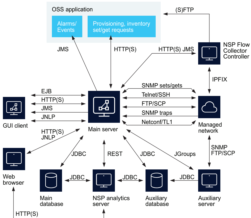
Figure 1-1 NFM-P component communication
