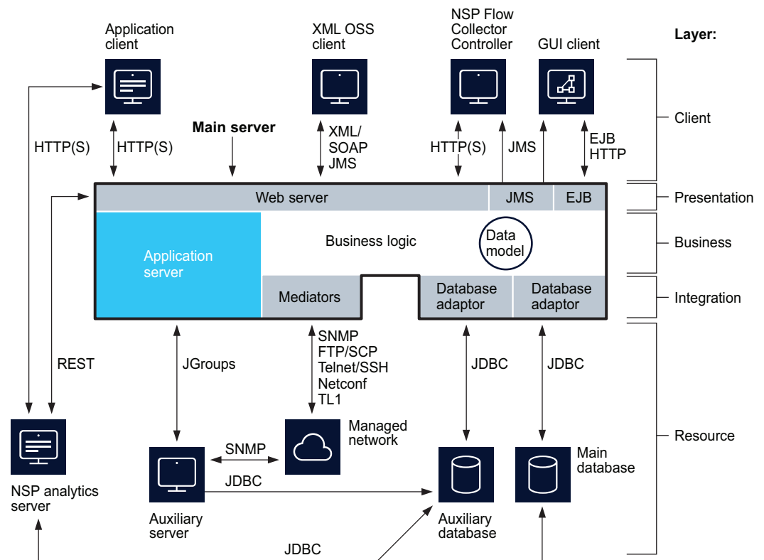
Figure 1-2 NFM-P multi-layer model
