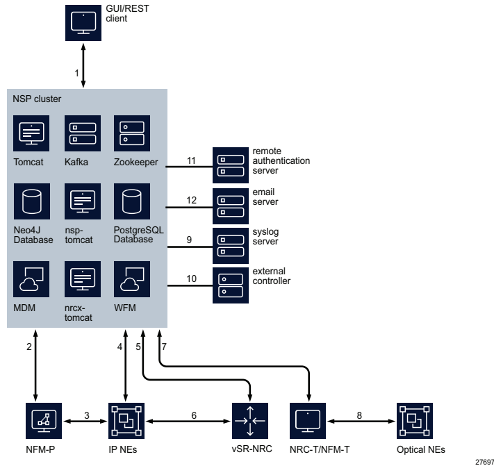
Figure 6-1 Standalone NSP deployment
