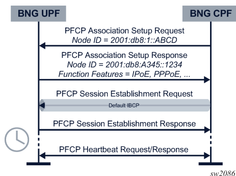
Figure 1: BNG UPF PFCP association setup flow
