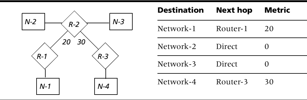
Figure 47. Shortest-path tree and resulting routing table for Router-2
