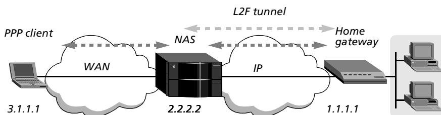
Figure 41. L2F tunneling
