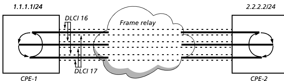
Figure 50. MFR peers with three data links supporting two DLCIs
