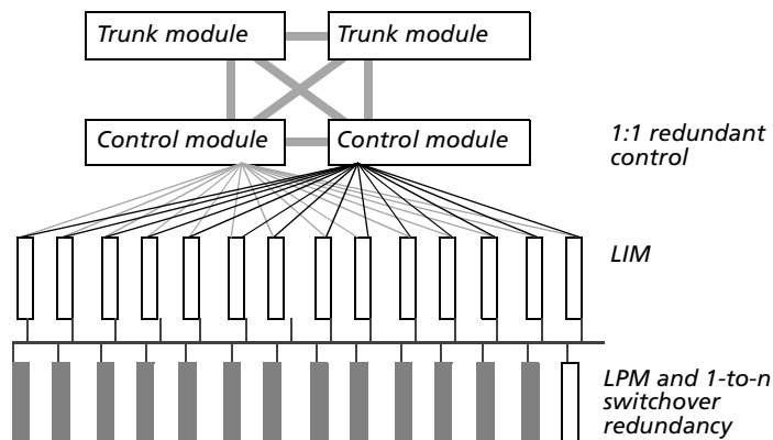
Figure 15. Redundant paths from each control module
