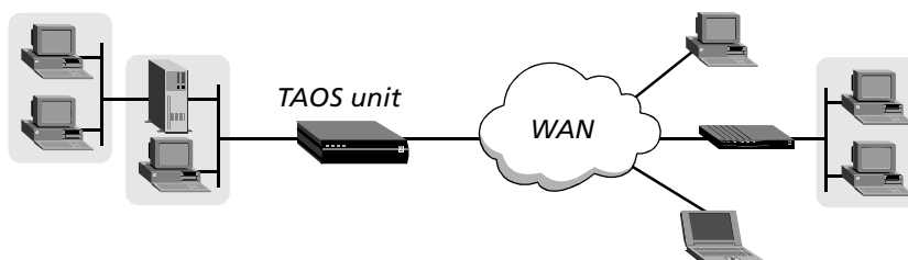
Figure 39. IPX-routing configuration
