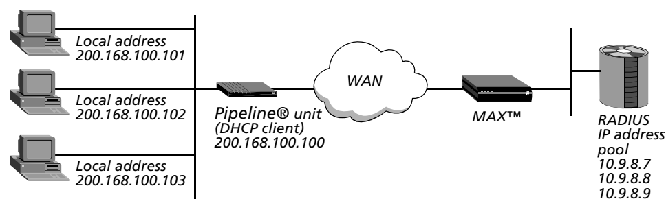
Figure 57. NAT for LAN setup
