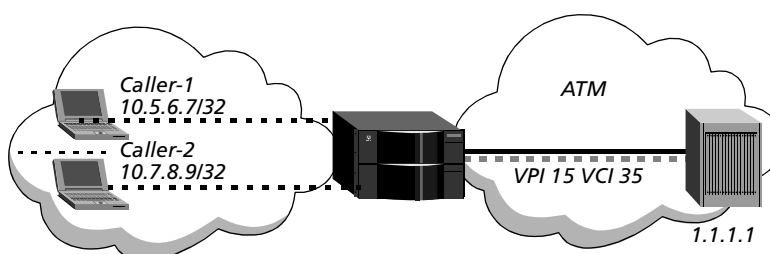
Figure 6. Concentrating PPP calls to an ATM interface using ATM direct
