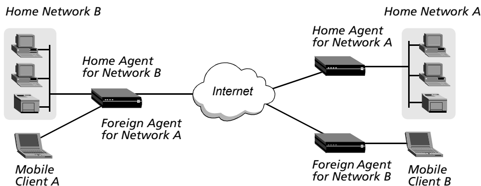
Figure 54. TAOS unit acting as both Home Agent and Foreign Agent
