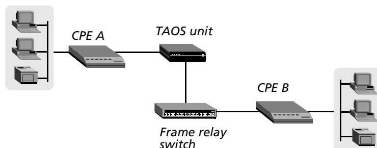
Figure 14. Circuit connection
