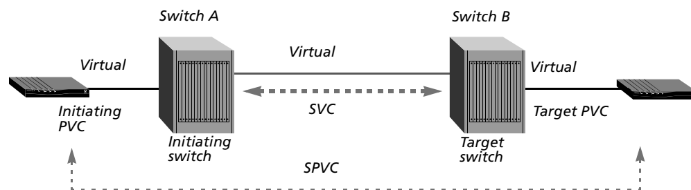
Figure 74. SPVC
