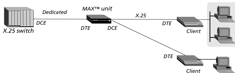
Figure 59. Net2Net circuit mode
