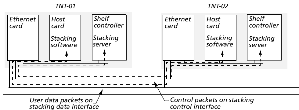
Figure 79. Stacking data and control packets
