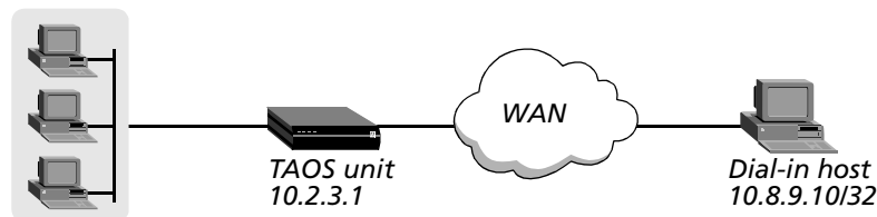
Figure 35. Dial-in host requiring a static IP address (a host route)
