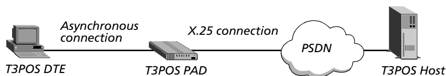
Figure 86. T3POS setup
