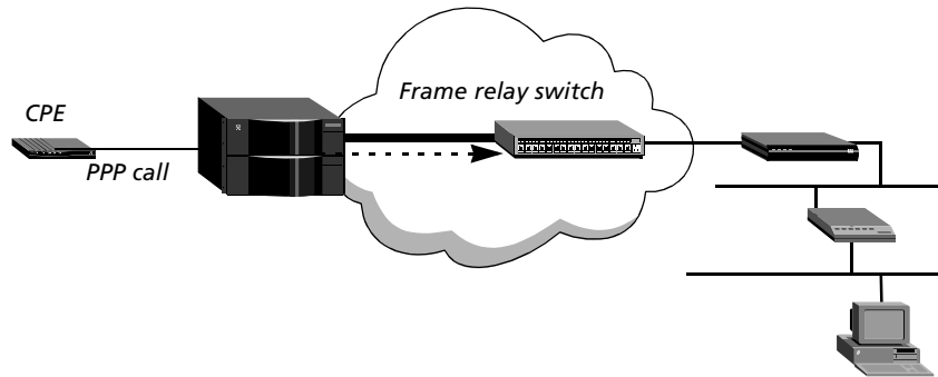
Figure 32. Dial-out SVC on a frame relay interface
