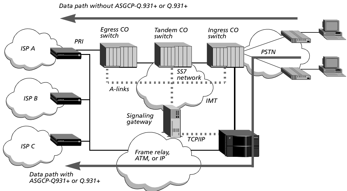
Figure 75. TAOS unit terminating data calls in an SS7 network
