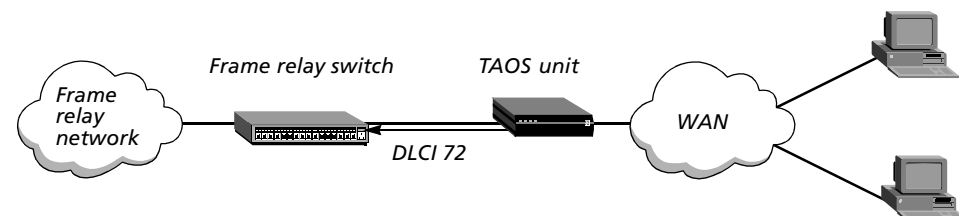
Figure 29. Frame relay direct connections using the same DLCI
