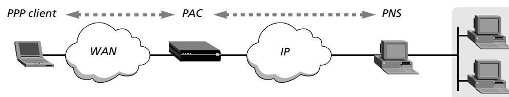
Figure 67. PPTP tunnel
