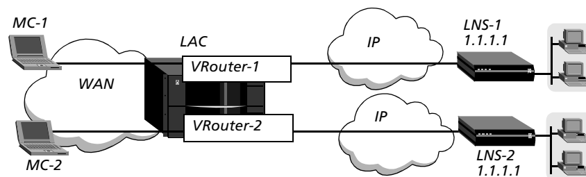
Figure 43. L2TP tunnels built on separate VRouters
