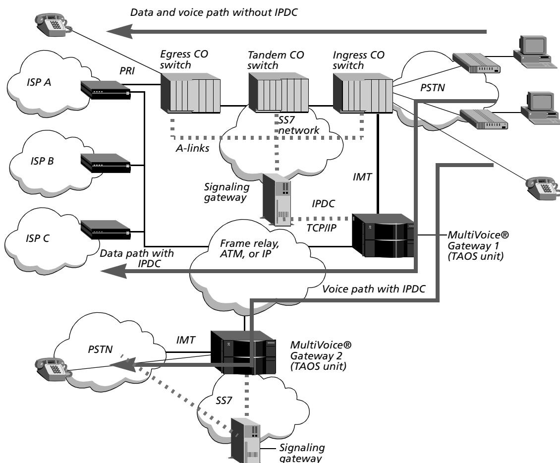
Figure 76. TAOS unit terminating voice and data calls in an SS7 network
