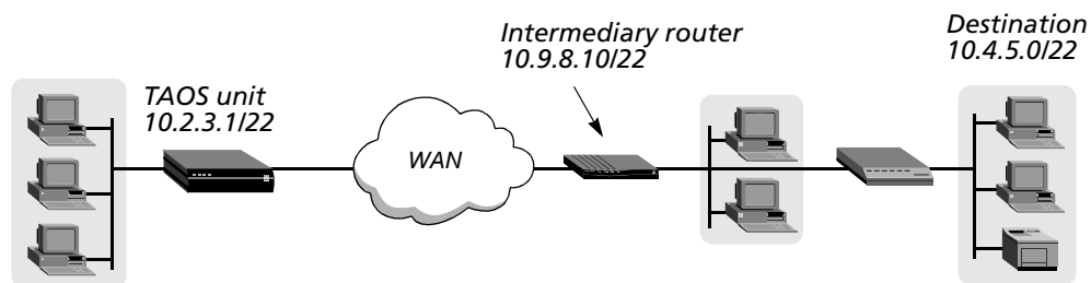
Figure 82. Static route to a remote subnet
