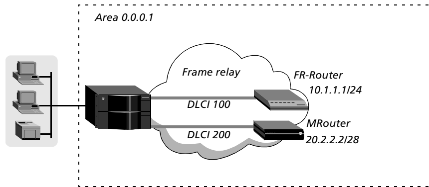
Figure 58. NBMA network
