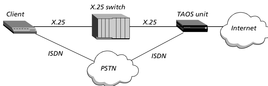
Figure 40. ISDN packet mode
