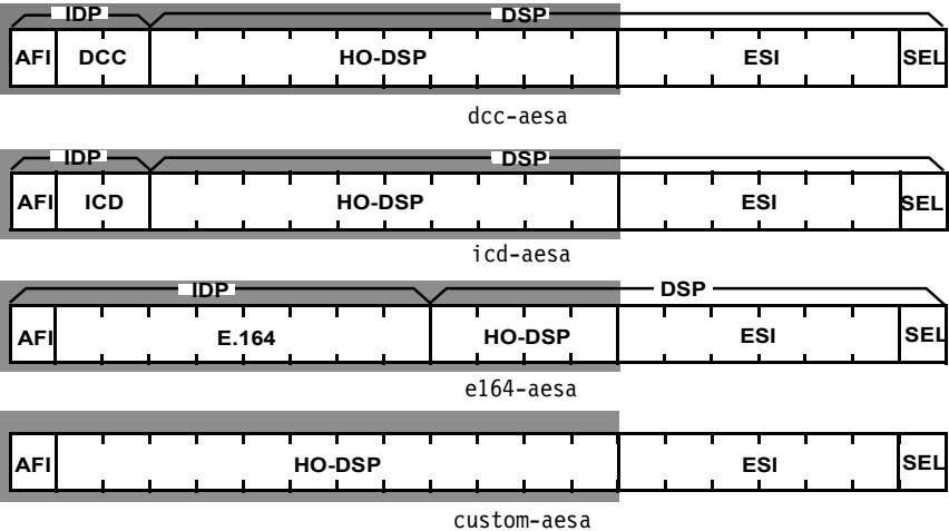
Figure 2. Subfields in the AESA address formats
