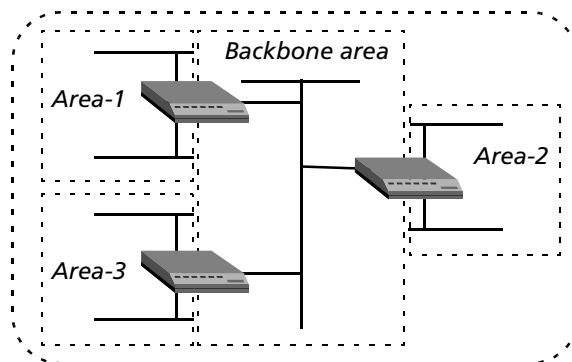
Figure 3. Dividing an autonomous system into areas
