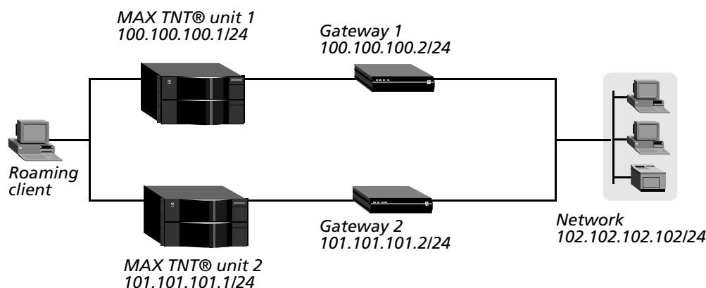
Figure 68. Using a pseudogateway
