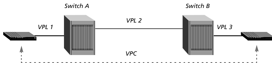
Figure 94. VPLs forming a VPC
