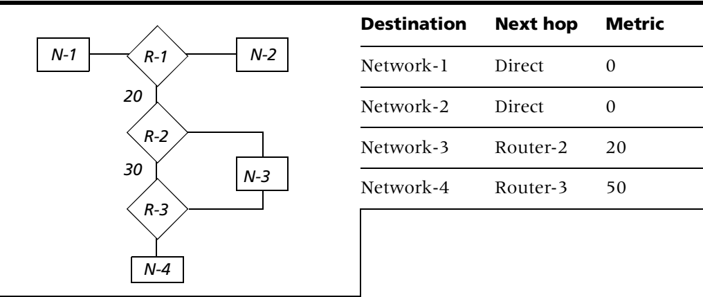
Figure 46. Shortest-path tree and resulting routing table for Router-1
