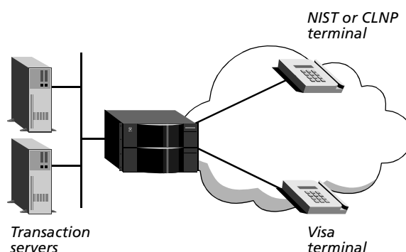
Figure 73. Sample SDTN setup
