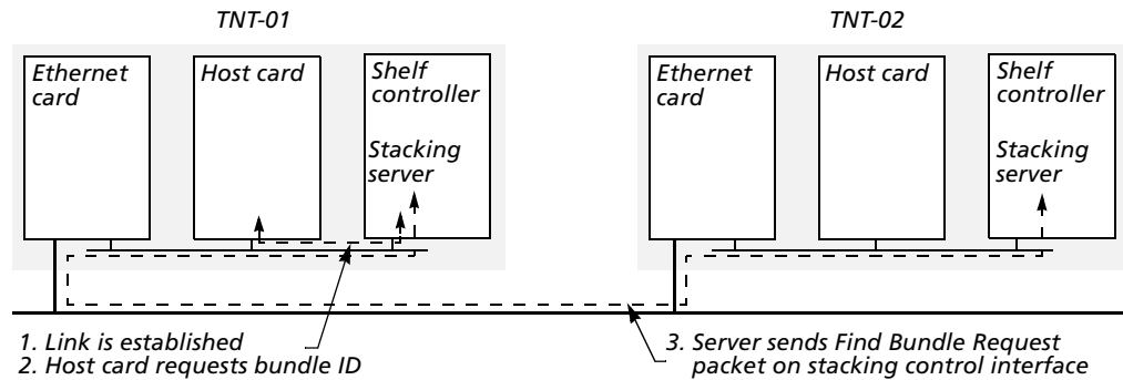
Figure 78. Stacking control messages to establish a bundle
