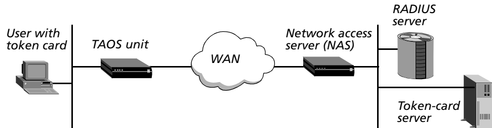
Figure 89. Token-card authentication for dial-out connections
