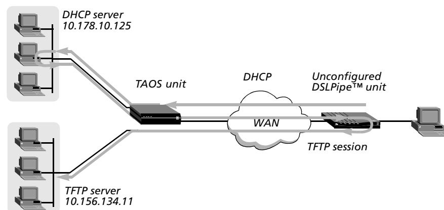
Figure 23. DSLPipe unit obtaining its configuration (plug-and-play)
