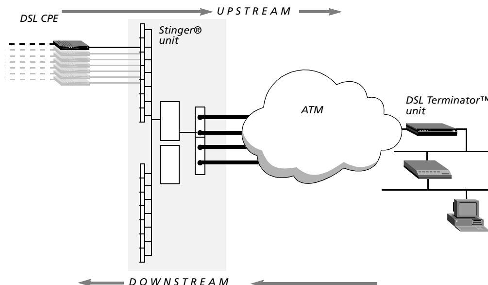
Figure 83. Stinger® configuration
