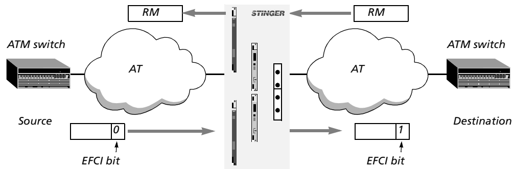
Figure 26. Congestion management with EFCI
