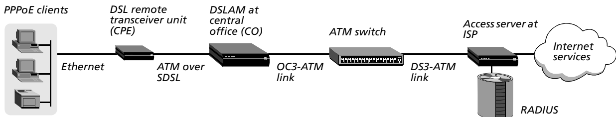
Figure 66. PPPoE configuration
