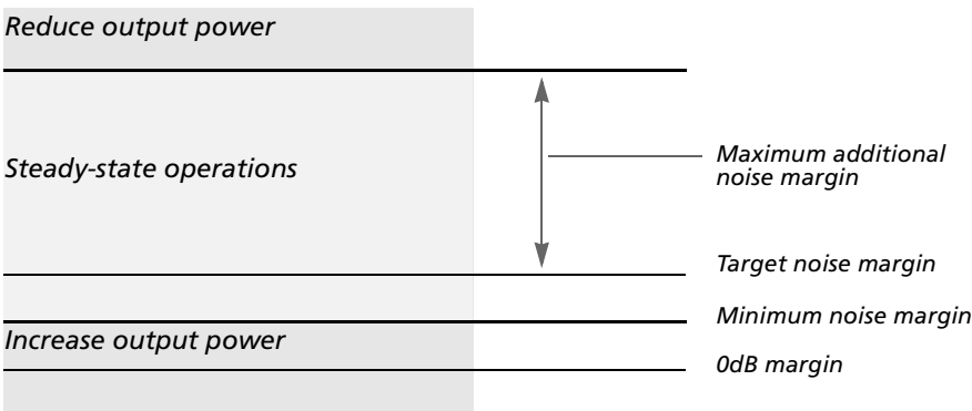
Figure 61. Noise margins
