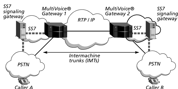
Figure 56. MultiVoice in an SS7 environment
