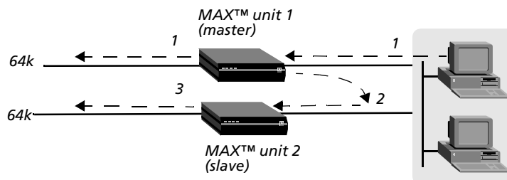
Figure 81. Packet flow from the Ethernet network
