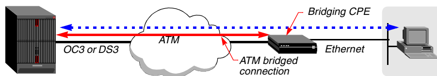
Figure 11. Access to the TAOS unit through a bridging CPE
