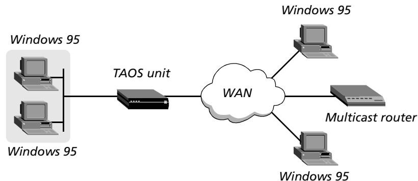
Figure 37. Forwarding multicast traffic on both Ethernet and WAN interfaces
