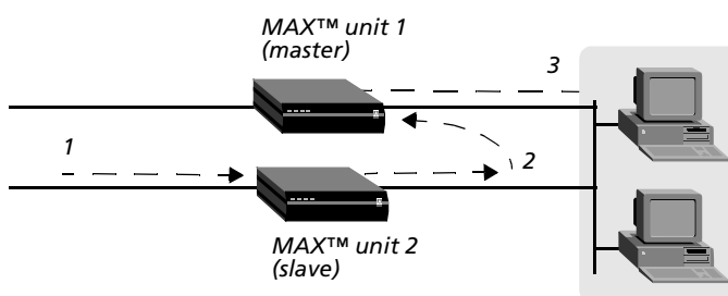
Figure 71. Packet flow from the slave channel to the Ethernet network
