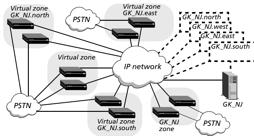
Figure 34. Example of a MultiVoice® network using gatekeeper virtual zones
