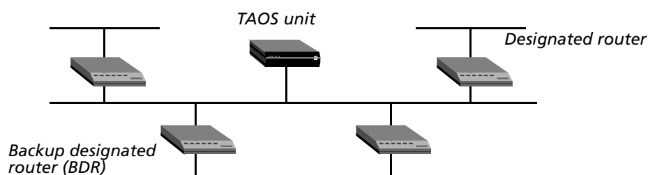
Figure 20. Designated and backup designated routers
