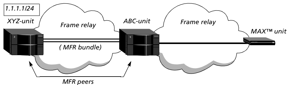
Figure 51. MFR circuit switching from a bundle to a single T1 interface
