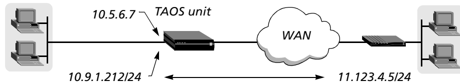
Figure 62. How numbered interfaces work
