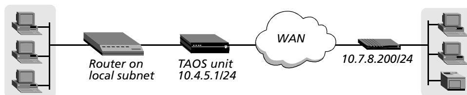
Figure 19. Default route to a local IP router
