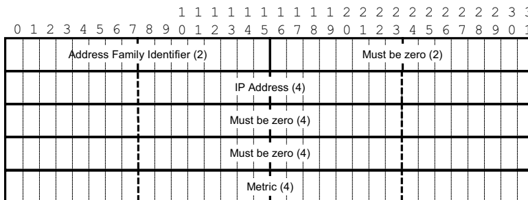
Figure 5: RIPv1 Format
