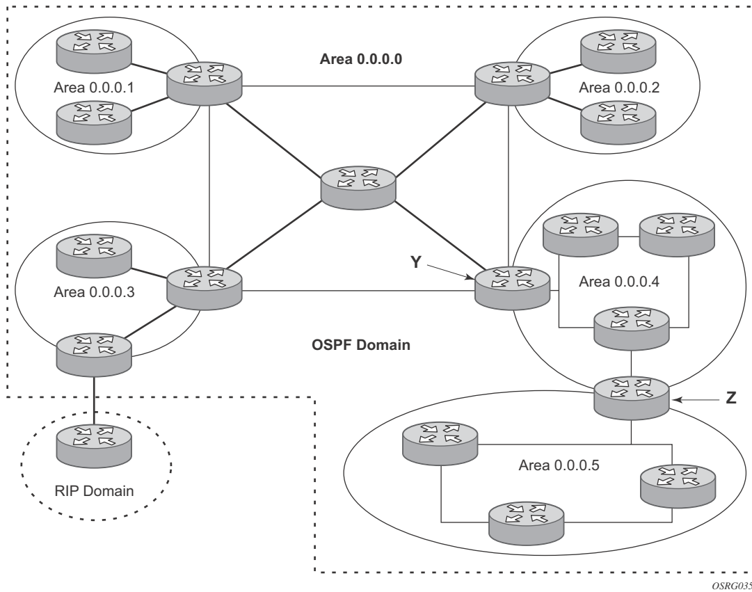
Figure 8: Backbone Area
