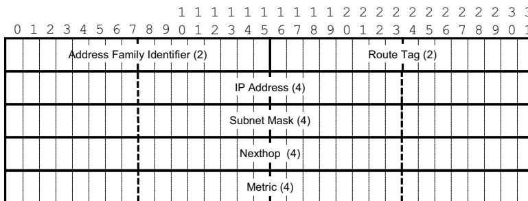
Figure 6: RIPv2 Format
