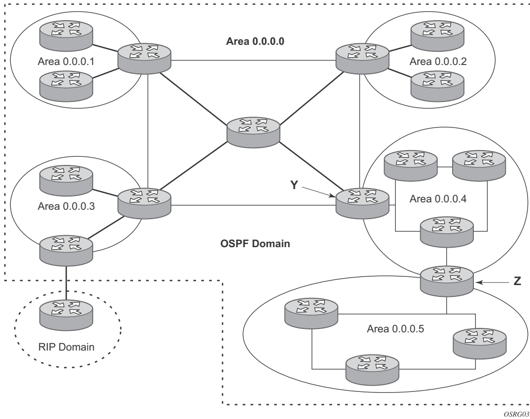
Figure 15: OSPF Areas
