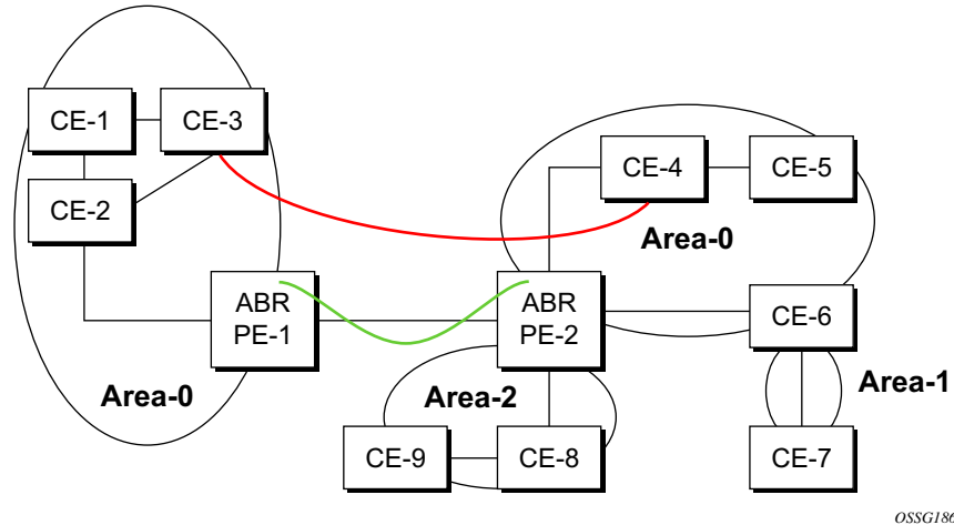
Figure 10: Sham Links
