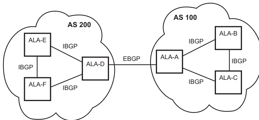
Figure 21: BGP Sessions
