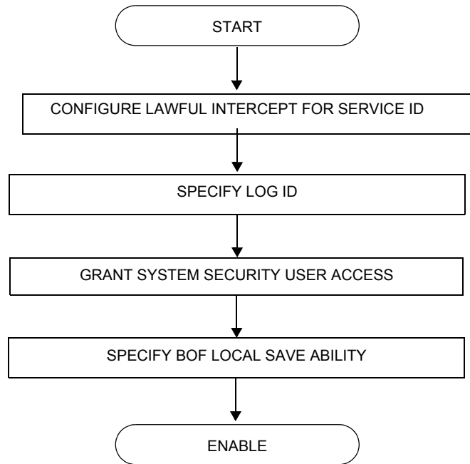
Figure 10: Lawful Intercept Configuration and Implementation Flow
