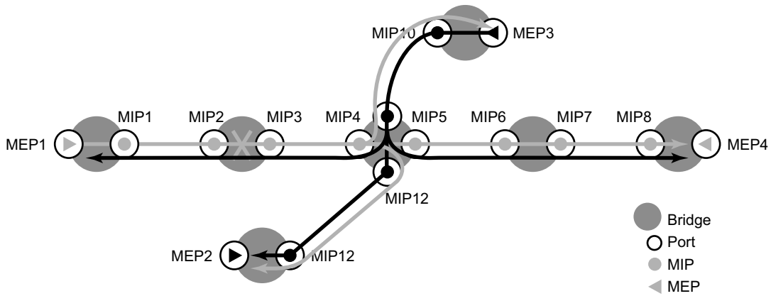
Figure 26: CFM Continuity Check
