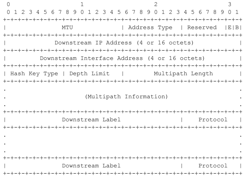
Figure 16: Modifications to the Downstream Mapping TLV
