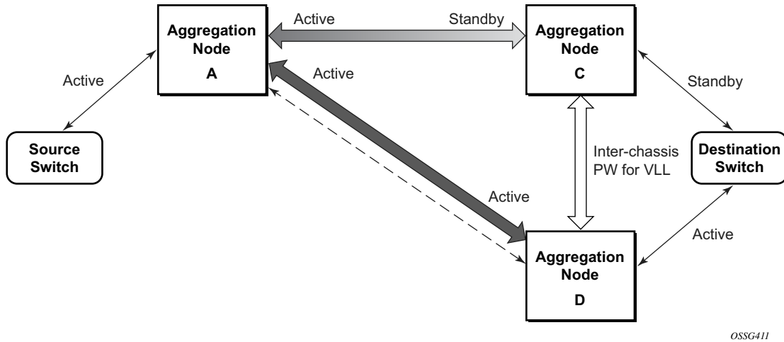
Figure 8: State Engine for a Non-Redundant Service to a Redundant Mirror Service
