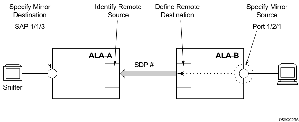
Figure 13: Remote Mirrored Service Configuration Example
