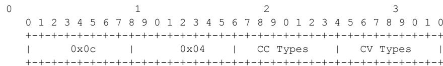
Figure 18: VCCV TLV
