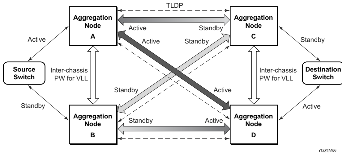
Figure 15: State Engine for Redundant Service to a Redundant Mirror Service
