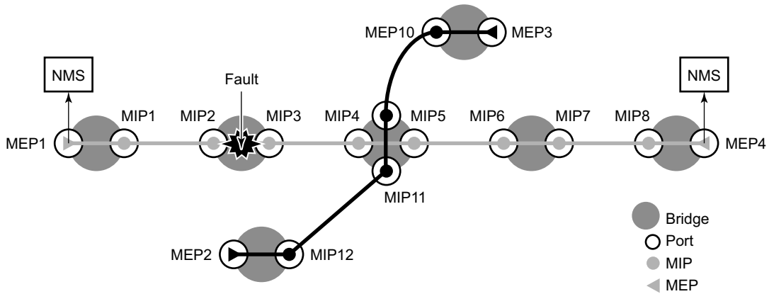
Figure 27: CFM CC Failure Scenario
