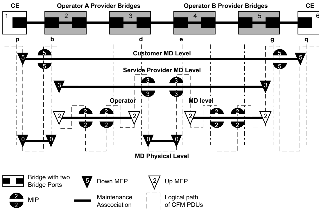
Figure 23: MEP, MIP and MD Levels
