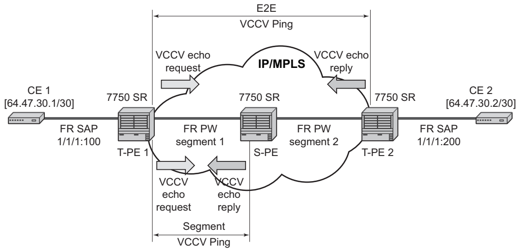
Figure 20: VCCV-Ping over a Multi-Segment Pseudowire
