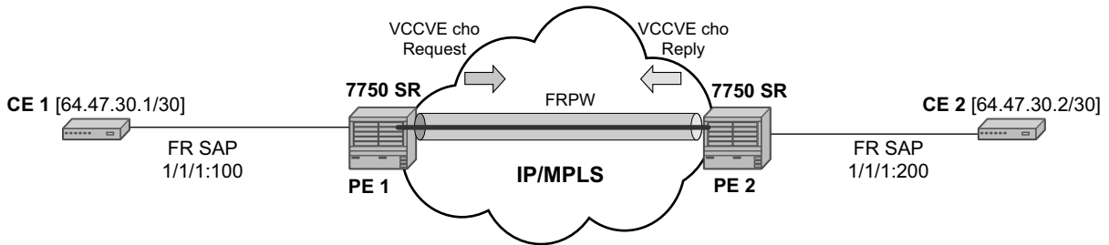
Figure 19: VCCV-Ping Application
