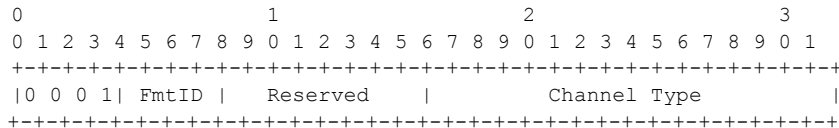
Figure 17: OAM Control Word Format
